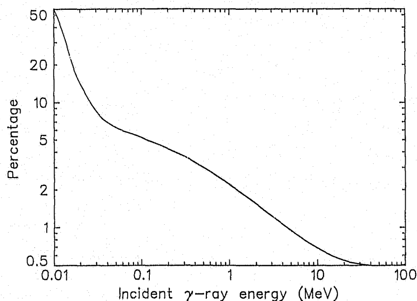
Figure 8.1. Percentage of incident \gamma -rays that will interact with a diamond 1 mm thick.
