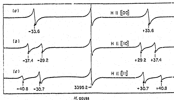
Figure 7.3. ESR spectra of single substitutional nitrogen in diamond at 22 °C. (a) H \parallel [100] , (b) H \parallel [110] , and (c) H \parallel [111] . (Taken from Smith et al 1959).
