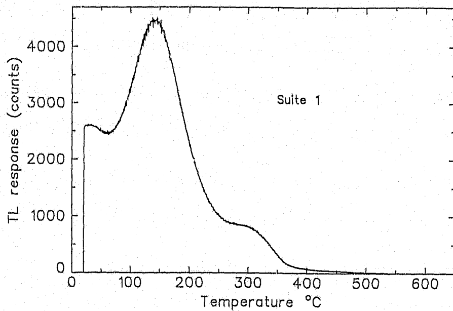
Figure A.4. Thermoluminescent spectrum of Suite 1.
