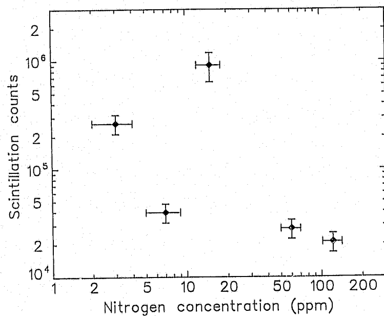
Figure 7.7. Scintillation counting response as a function of single substitutional nitrogen concentration.
