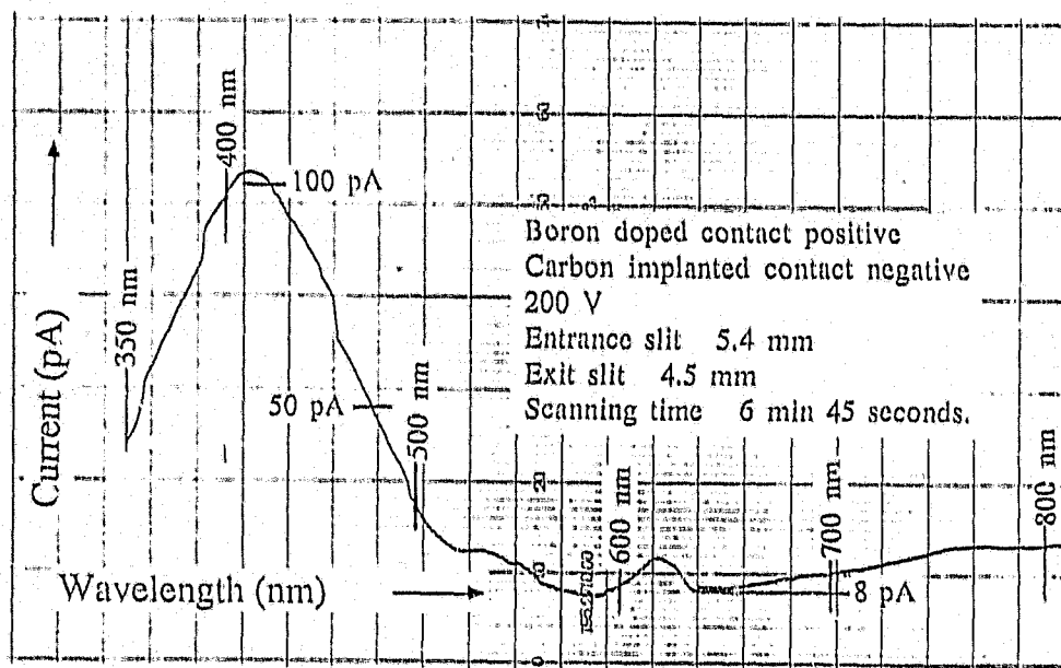
Figure 5.4. A typical photoconduction spectrum. Diamond; Suite 2. (Not corrected for light intensity variation).
