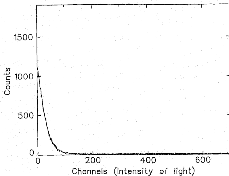
Figure 6.2. Typical scintillation spectrum from synthetic diamond used for pulse counting measurements. Diamond: Suite 2 no. 2.
