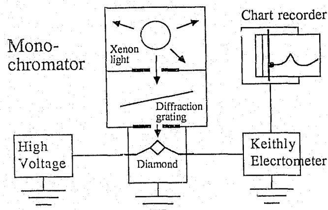
Figure 5.5. Schematic diagram of the photoconduction circuit.
