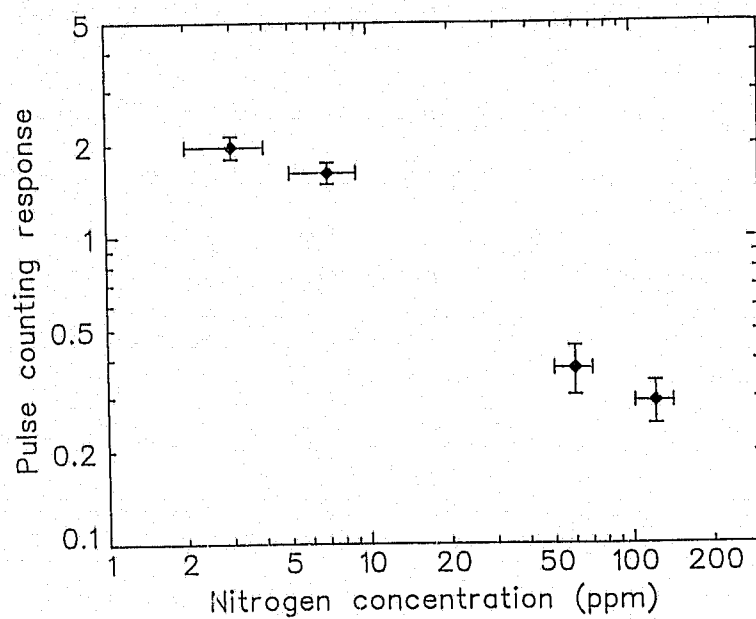
Figure 7.6. Pulse counting response as a function of single substitutional nitrogen concentration.
