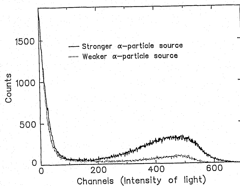
Figure 6.5. Scintillation spectra for two different intensities of 5.5 MeV \alpha -particle sources, both incident on the same position of a synthetic diamond. Diamond: CoFe stone 6.
