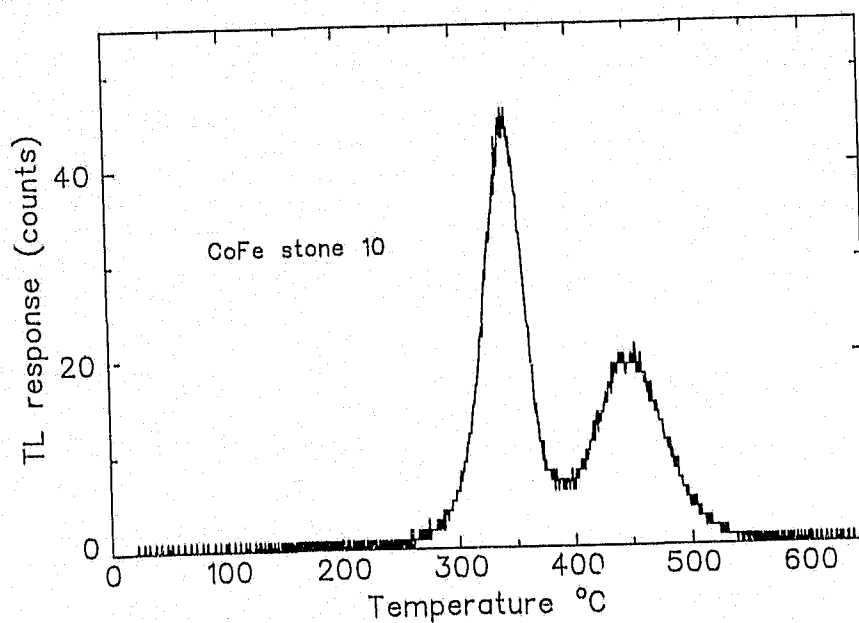
Figure A.1. Thermoluminescent spectrum of CoFe stone 10.
