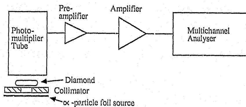
Figure 6.1. Schematic diagram of apparatus to measure scintillation spectra of diamond.
