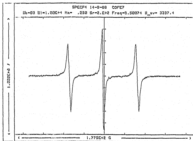
Figure 7.4. A typical ESR spectrum. Diamond: CoFe stone 6.
