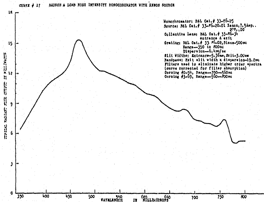
Figure 5.3. Intensity of the monochromator light as a function of wavelength.
