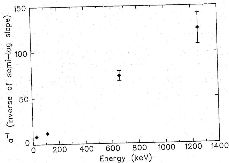
Figure 8.6. Inverse of the semi-log slope of the pulse height spectrum as a function of radiation energy.
