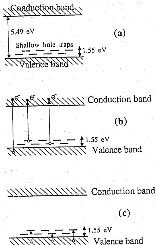
Figure 5.8. Procedures affecting the shallow hole traps in diamond. (a) Position of possible hole trapping levels above the valence band. (b) Pre-irradiation causing hole to be trapped. (c) Red light or heat exciting electron from valence band, releasing trapped hole and returning the trap to its neutral state.
