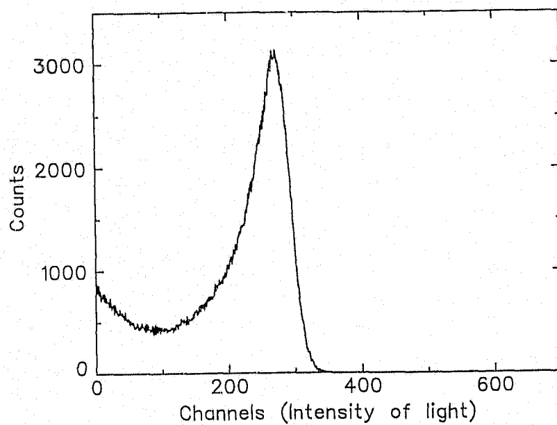
Figure 6.3. Scintillation spectrum of an iron free synthetic diamond. Measured by Nam et al (1989), using the same apparatus that is described in this chapter.
