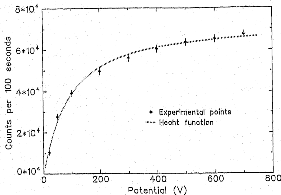
Figure 8.4. Hecht function fit for the pulse counting rate as a function of potential across the diamond contacts. Diamond: Suite 2.
