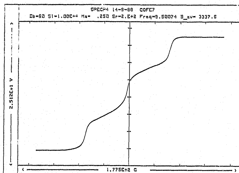
Figure 7.5. The ESR spectrum in figure 7.4 integrated twice.
