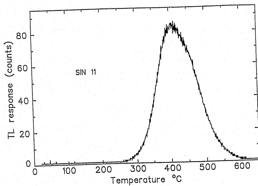
Figure A.6. Thermoluminescent spectrum of SIN 11.
