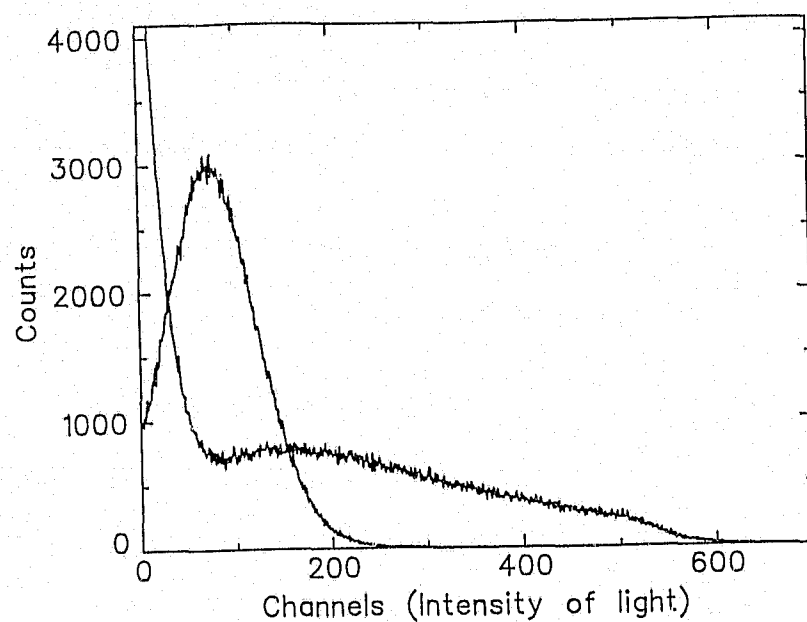
Figure 6.4. Scintillation spectra for two surfaces of the same synthetic diamond. Diamond: CoFe stone 6.
