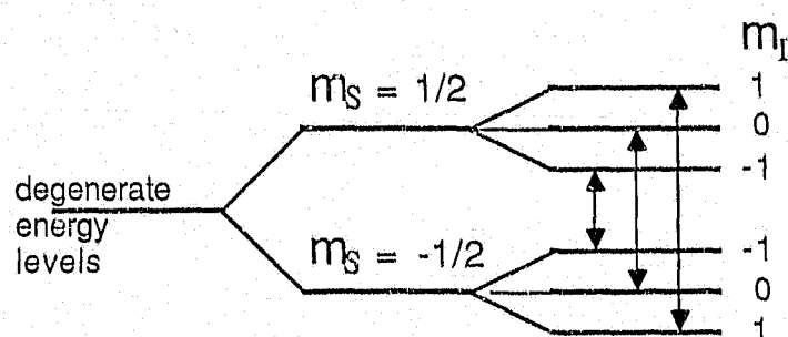
Figure 7.2. Electron energy level splitting for the single substitutional nitrogen impurity in diamond. The arrows show the allowed energy transitions. ( S = \frac{1}{2} , ( m_S = -\frac{1}{2}, +\frac{1}{2} ) and I = 1 , ( m_I = -1, 0, +1 )).
