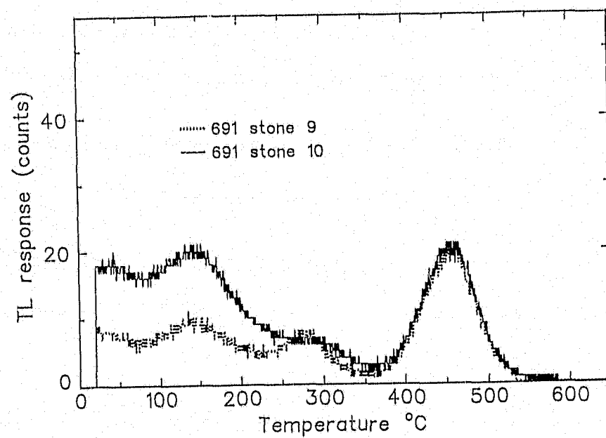
Figure A.2. Thermoluminescent spectrum of 691 stones 9 and 10.
