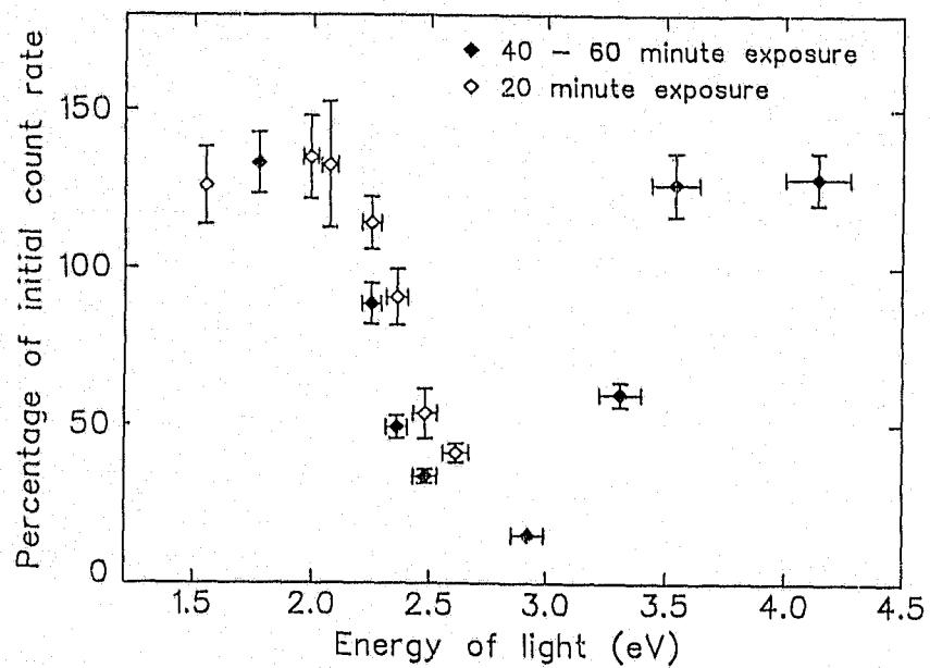
Figure 5.7. Effect on the pulse counting response as a function of energy after exposing the diamond to light. Diamond: Suite 2.
