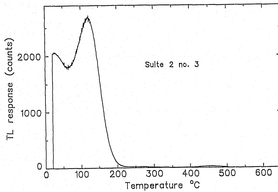
Figure A.3. Thermoluminescent spectrum of Suite 2 no. 3.
