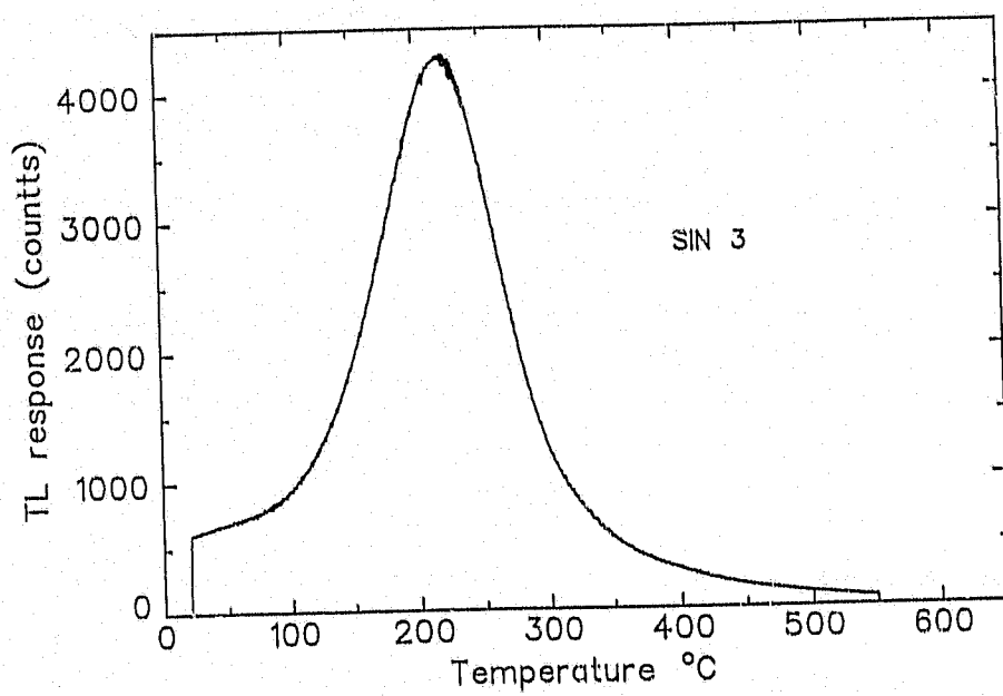
Figure A.7. Thermoluminescent spectrum of SIN 3.
