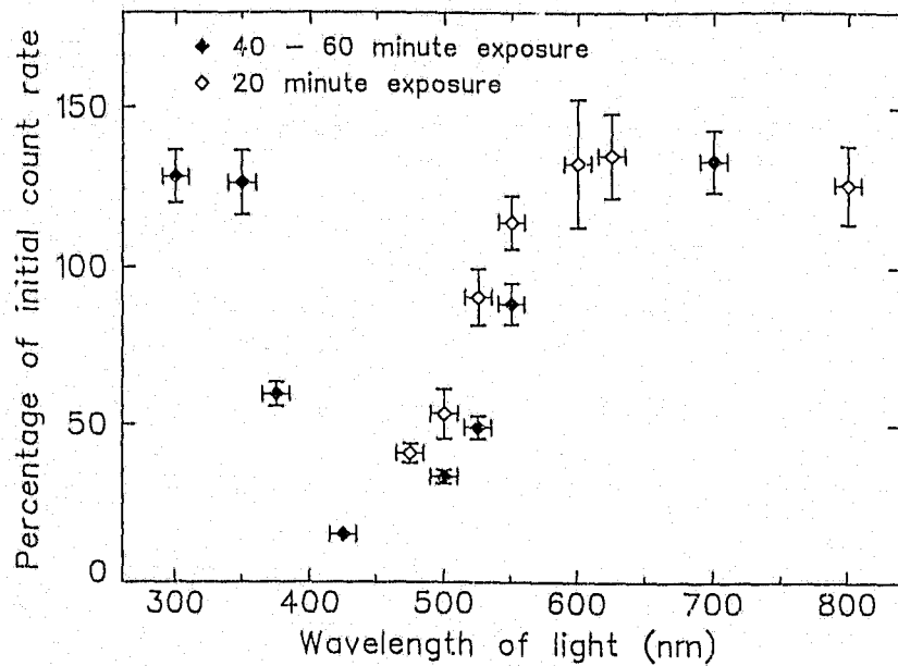
Figure 5.6. Effect on the pulse counting response as a function of wavelength after exposing the diamond to light. Diamond: Suite 2.
