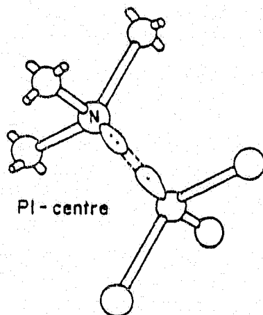
Figure 7.1. Schematic diagram of the single substitutional (paramagnetic) nitrogen impurity in the diamond lattice. Also referred to as the P1 centre.
