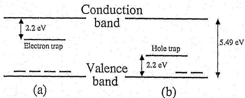
Figure 5.9. Band structure diagram with the trapping level which causes decreased counting response - (a) possible electron trap 2.2 eV below the conduction band, or (b) possible hole trap 2.2 eV above the valence band.
