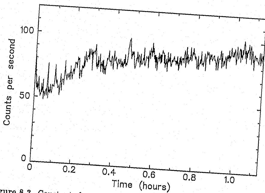
Figure 8.2. Count rate as a function of the time after pre-irradiation. Diamond: SIN 12.
