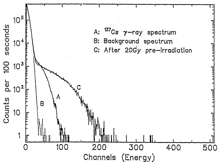
Figure 8.5. Pulse height spectra for the SIN 12 diamond.
