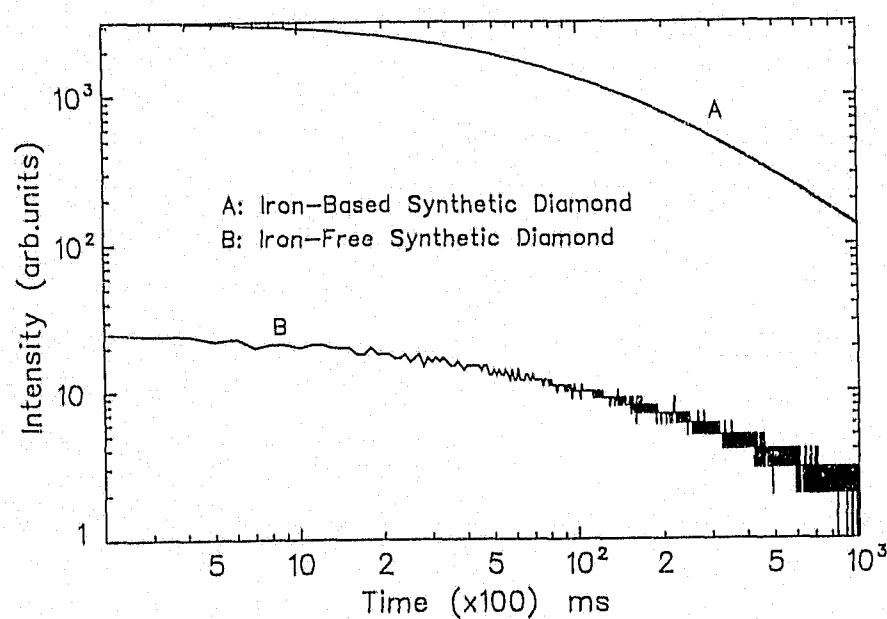
Figure 6.6. Phosphorescence decay curves from Nam et al 1989.
