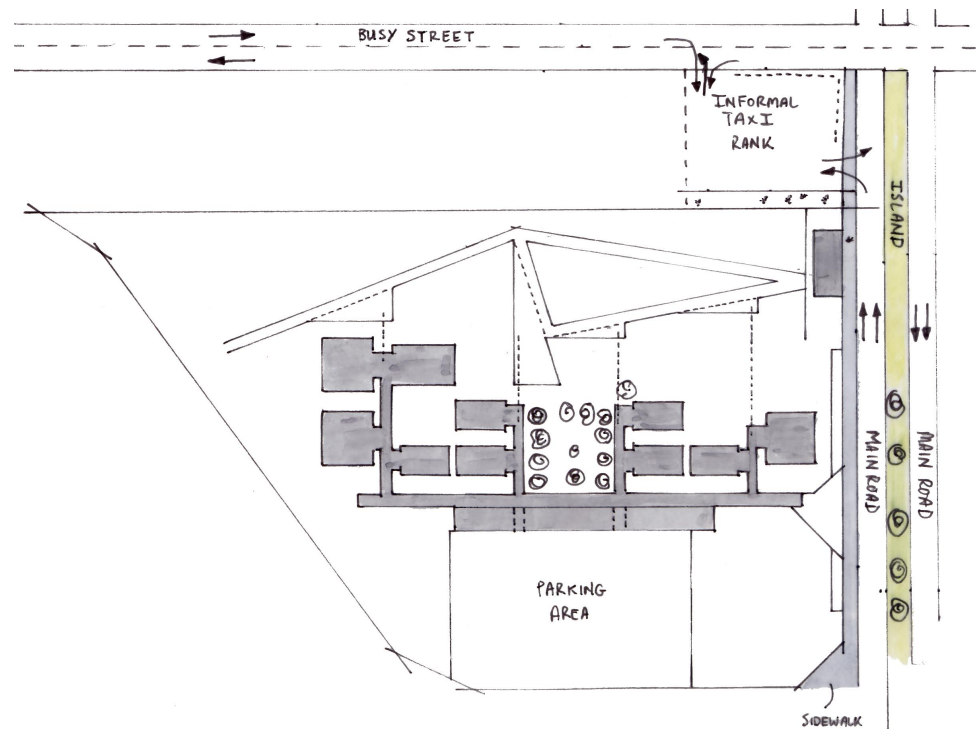
Figure 39 - Circulation sketch plan. (R.Hartmann)
