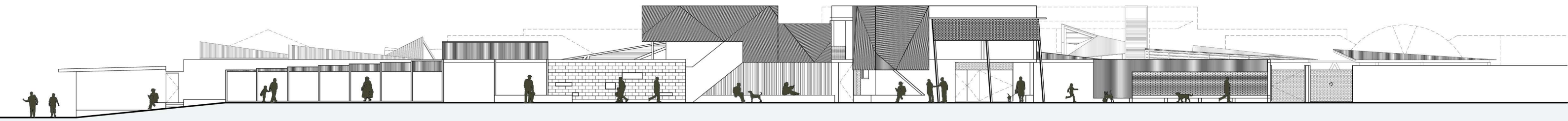
North Elevation 1:250
