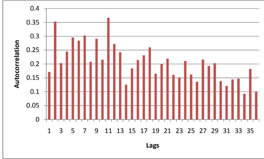
Figure 11: Autocorrelogram of the squared returns of Dow Jones Industrial Index
