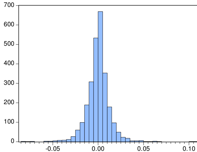
Figure 4: Distribution of daily returns of US Dow Jones Industrial Index
