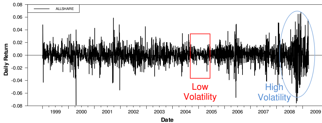
Figure 7: South African JSE All Share Index illustrating volatility clustering
