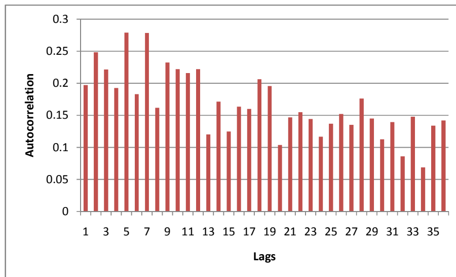
Figure 10: Autocorrelogram of the squared returns of JSE All Share Index
