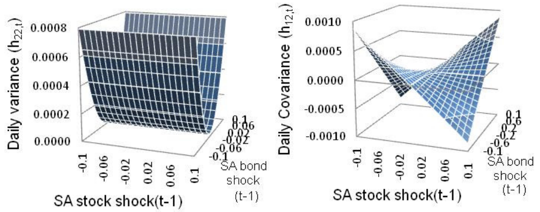
Figure 12: News impact surface for the variance and covariance of the South African bond market using South African bond and stock market shocks
