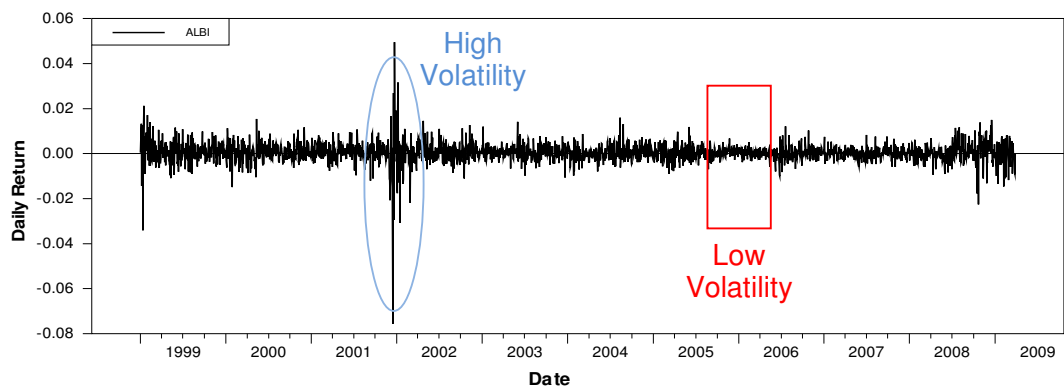
Figure 6: South African All Bond Total Return Index illustrating volatility clustering
