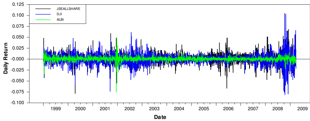
Figure 5: South African All Bond Total Return Index, JSE All Share Index and Dow Jones Industrial Index daily returns
