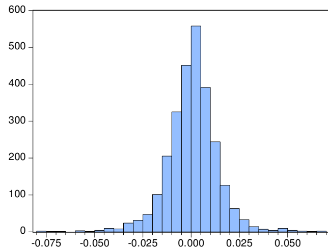
Figure 3: Distribution of daily returns of JSE All Share Index
