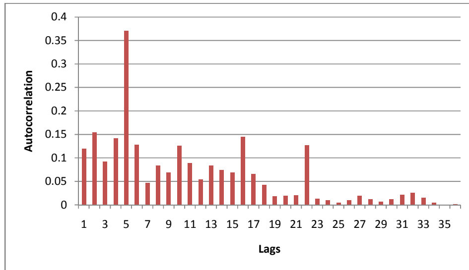
Figure 9: Autocorrelogram of the squared returns of South African All Bond Total Return
