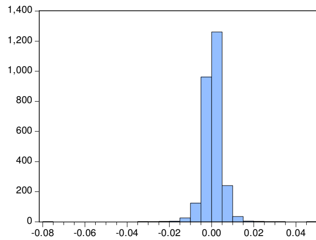
Figure 2: Distribution of daily returns of South African All Bond Total Return Index
