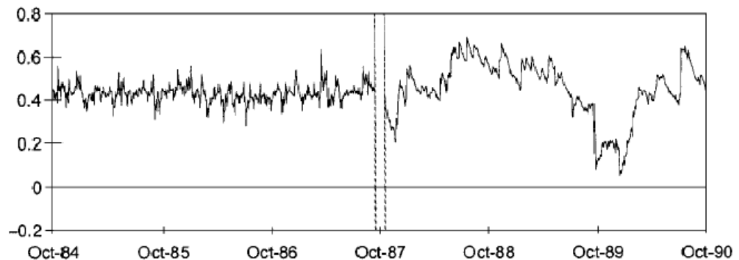
Figure 1: Cross-market correlations between US stock and bond markets (Darbar and Deb 2002)
