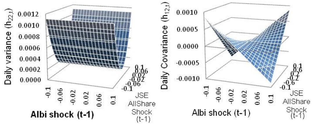
Figure 13: News impact surface for the variance and covariance of the South African stock market using South African bond and stock market shocks.
