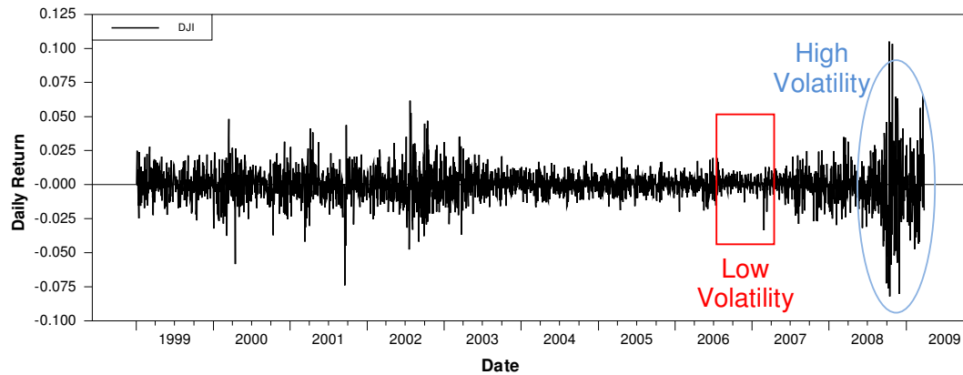
Figure 8: Dow Jones Industrial Index illustrating volatility clustering
