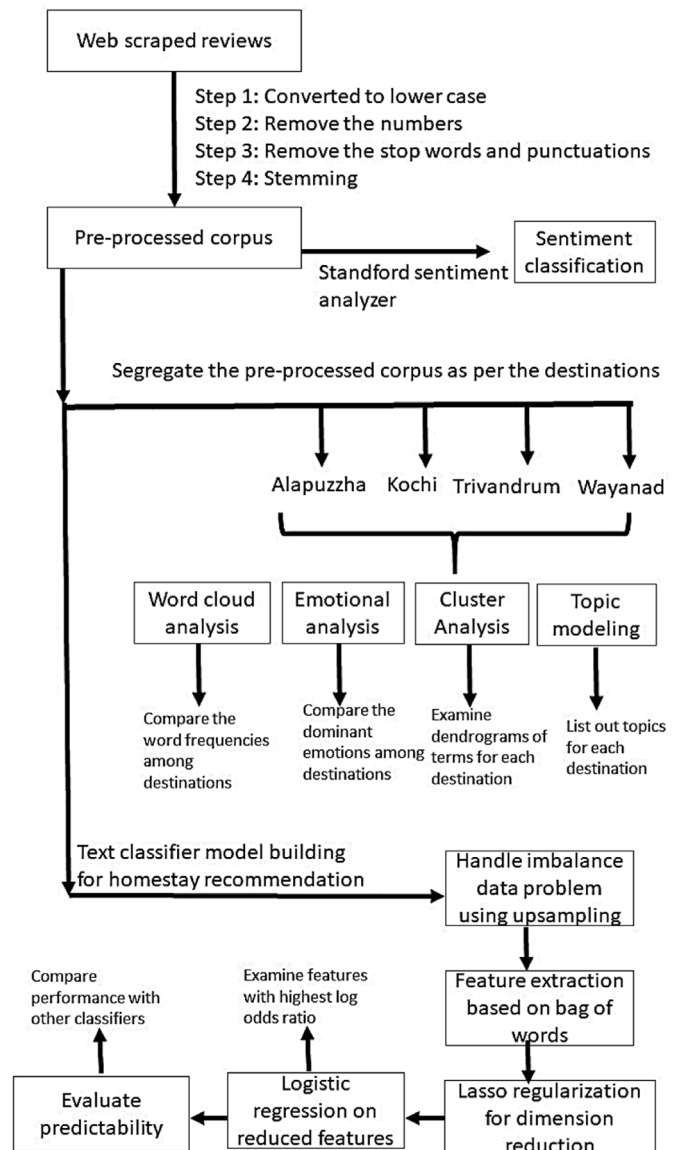
Fig. 1. Analytical workflow of the study.
