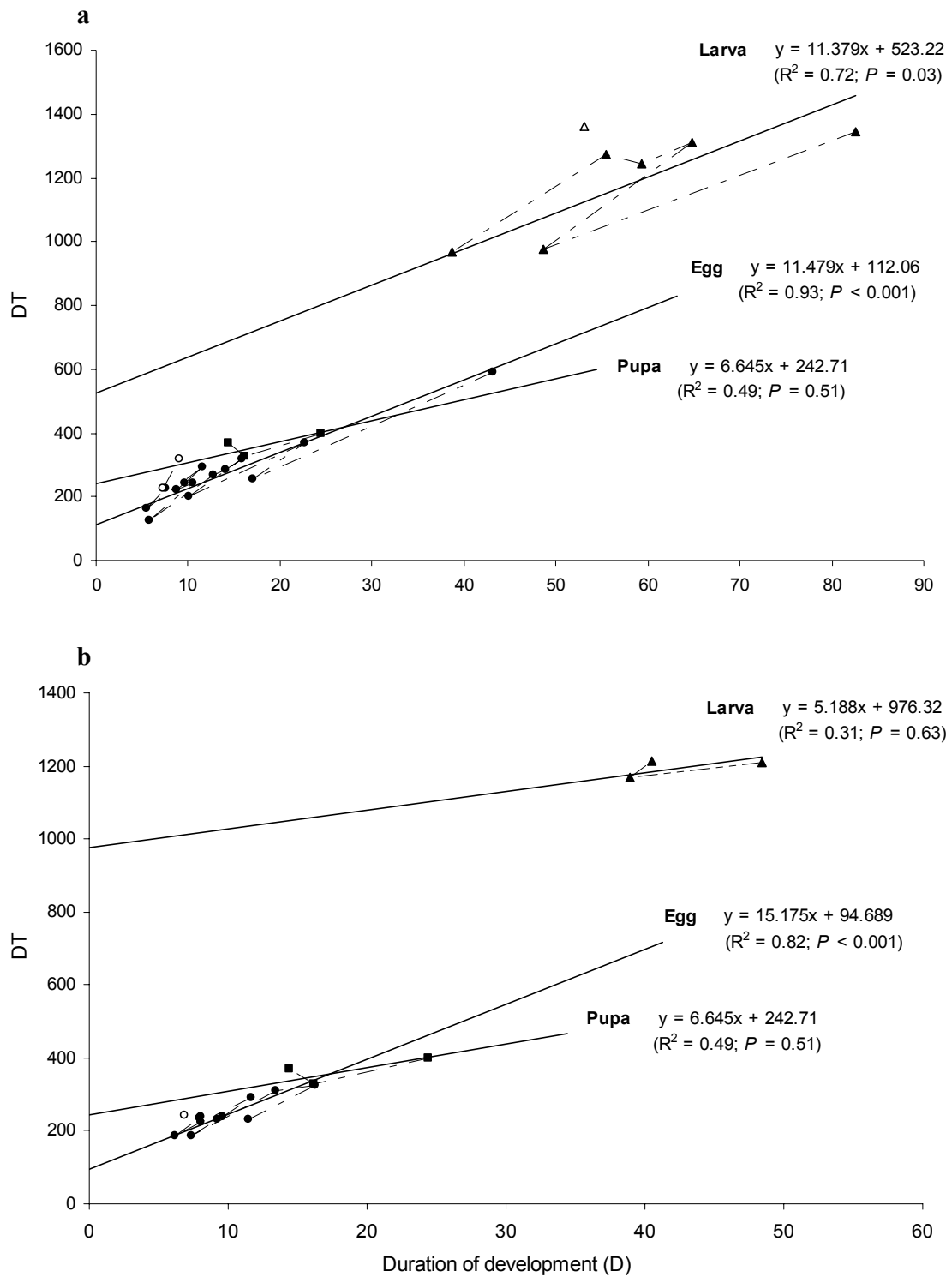
Fig. 2.2. Temperature dependent development of (a) Neochetina bruchi and (b) Neochetina eichhorniae egg, larval and pupal stages using the reduced major axis regression technique (Ikemoto and Takai, 2000). Unshaded points were omitted from the regression.
