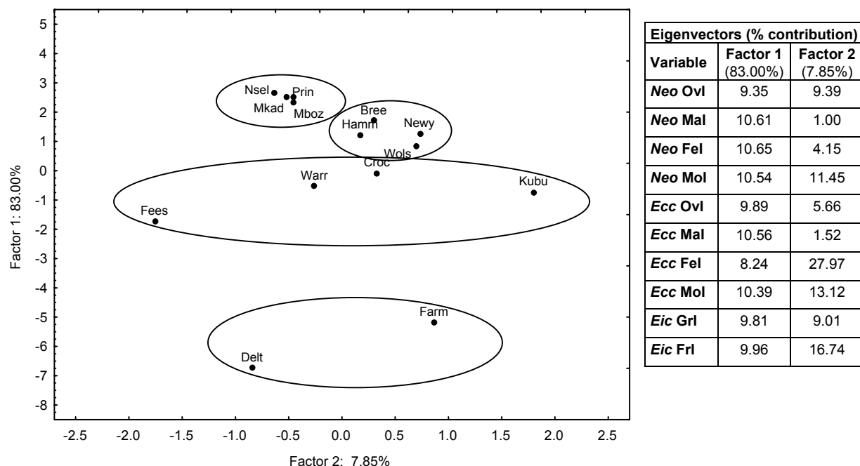
Fig. 3.23. Grouping of field sites using principle components analysis incorporating 10 thermal stress indices determined for the Neochetina weevils ( Neo ), Eccritotarsus catarinensis ( Ecc ) and Eichhornia crassipes ( Eic ).
