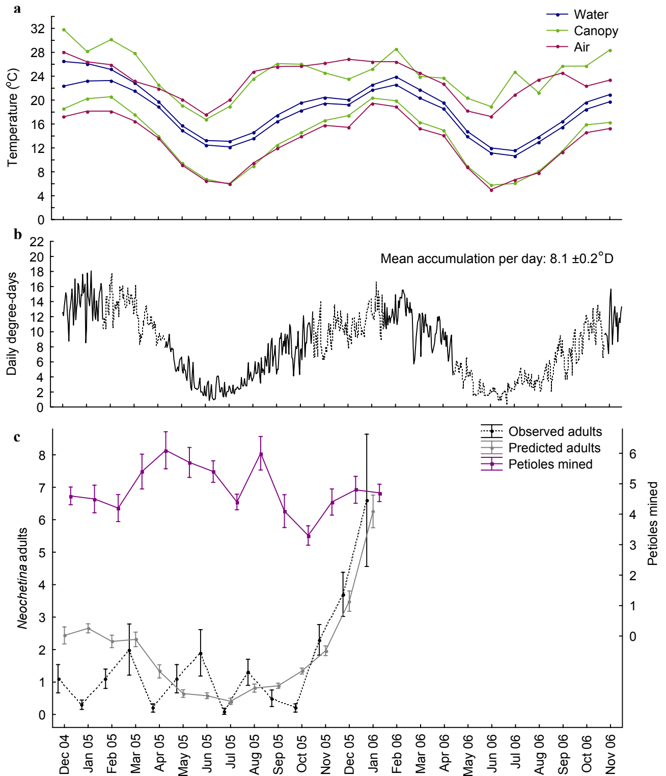
Fig. 3.11. Hammarsdale Dam: Monthly mean daily maximum and minimum temperature (a) for three microsites; daily degree-days ( t = 9.6^{\circ}\text{C} ) and predicted Neochetina cohorts ( K = 984.4^{\circ}\text{D} ) starting from 24 October 2005 (b) derived from canopy temperature (different line styles denote cohorts); and Neochetina phenology (c) from 2004 to 2006. Weevil phenology is inferred from observed counts of larval mines and adults, and predicted adult numbers are calculated from feeding scars adjusted for monthly leaf production (mean of 10 plants \pm SE).
