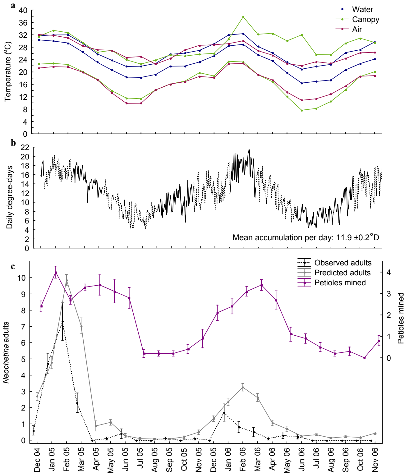
Fig. 3.13. Mbozambo Swamp: Monthly mean daily maximum and minimum temperature (a) for three microsites; daily degree-days ( t = 9.6^{\circ}\text{C} ) and predicted Neochetina cohorts ( K = 984.4^{\circ}\text{D} ) starting from 24 October 2005 (b) derived from canopy temperature (different line styles denote cohorts); and Neochetina phenology (c) from 2004 to 2006. Weevil phenology is inferred from observed counts of larval mines and adults, and predicted adult numbers are calculated from feeding scars adjusted for monthly leaf production (mean of 10 plants \pm SE).
