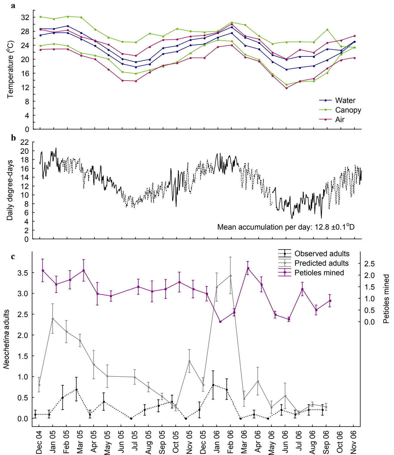
Fig. 3.16. Nseleni River: Monthly mean daily maximum and minimum temperature (a) for three microsites; daily degree-days ( t = 9.6^{\circ}\text{C} ) and predicted Neochetina cohorts ( K = 984.4^{\circ}\text{D} ) starting from 24 October 2005 (b) derived from canopy temperature (different line styles denote cohorts); and Neochetina phenology (c) from 2004 to 2006. Weevil phenology is inferred from observed counts of larval mines and adults, and predicted adult numbers are calculated from feeding scars adjusted for monthly leaf production (mean of 10 plants \pm SE).
