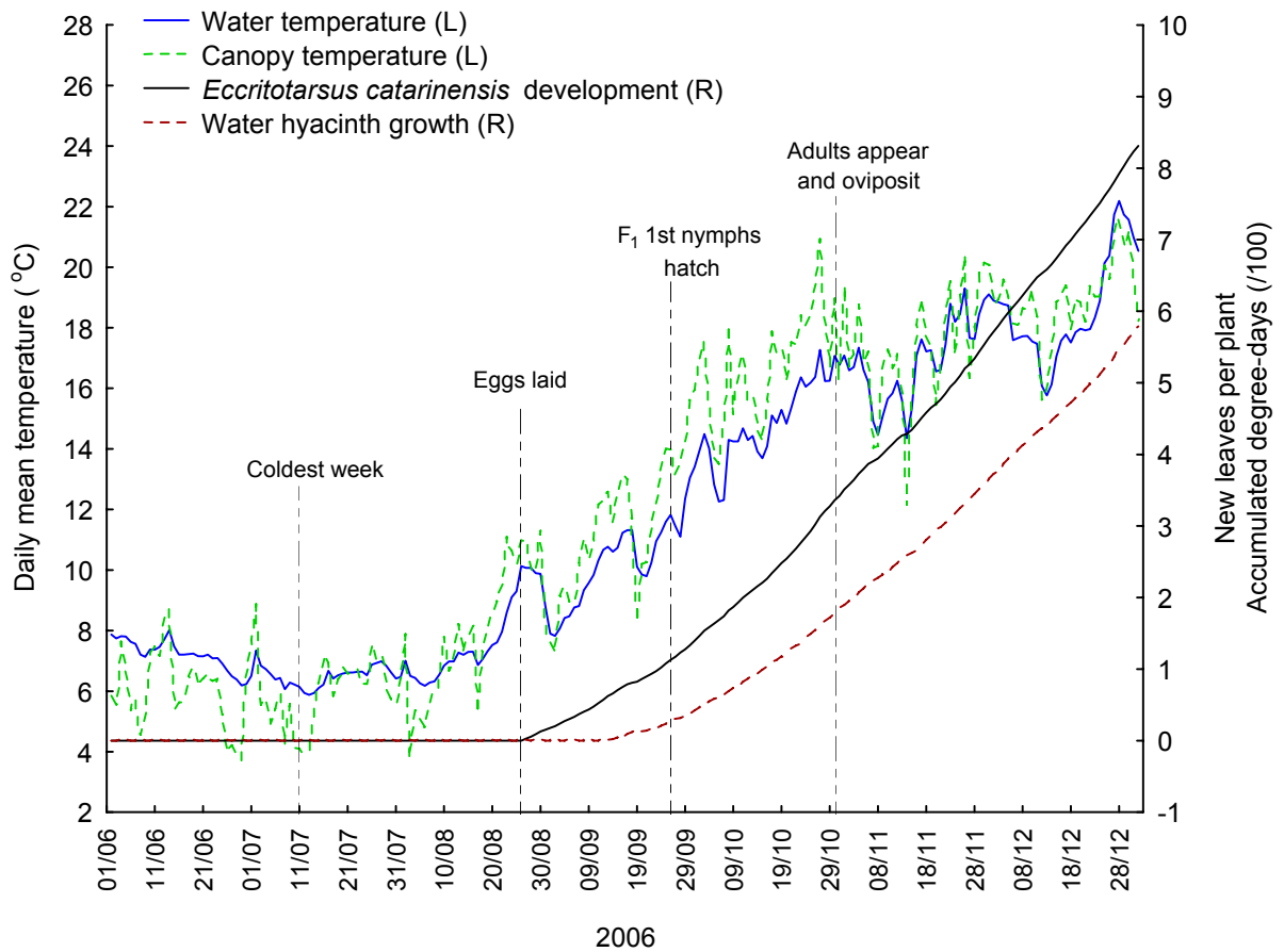
Fig. 2.15. Predicted water hyacinth and Eccritotarsus catarinensis recovery following adverse conditions during a highveld winter. Leaf production rates are in response to water temperature. Eccritotarsus catarinensis accumulation of degree-days is in response to plant canopy temperature.
