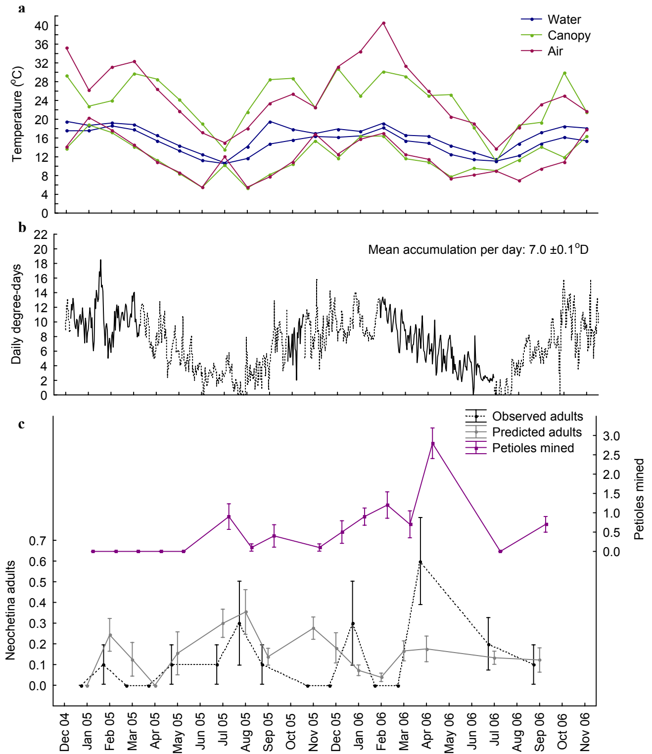
Fig. 3.19. Wolseley: Monthly mean daily maximum and minimum temperature (a) for three microsites; daily degree-days ( t = 9.6^{\circ}\text{C} ) and predicted Neochetina cohorts ( K = 984.4^{\circ}\text{D} ) starting from 24 October 2005 (b) derived from canopy temperature (different line styles denote cohorts); and Neochetina phenology (c) from 2004 to 2006. Weevil phenology is inferred from observed counts of larval mines and adults, and predicted adult numbers are calculated from feeding scars adjusted for monthly leaf production (mean of 10 plants \pm SE).
