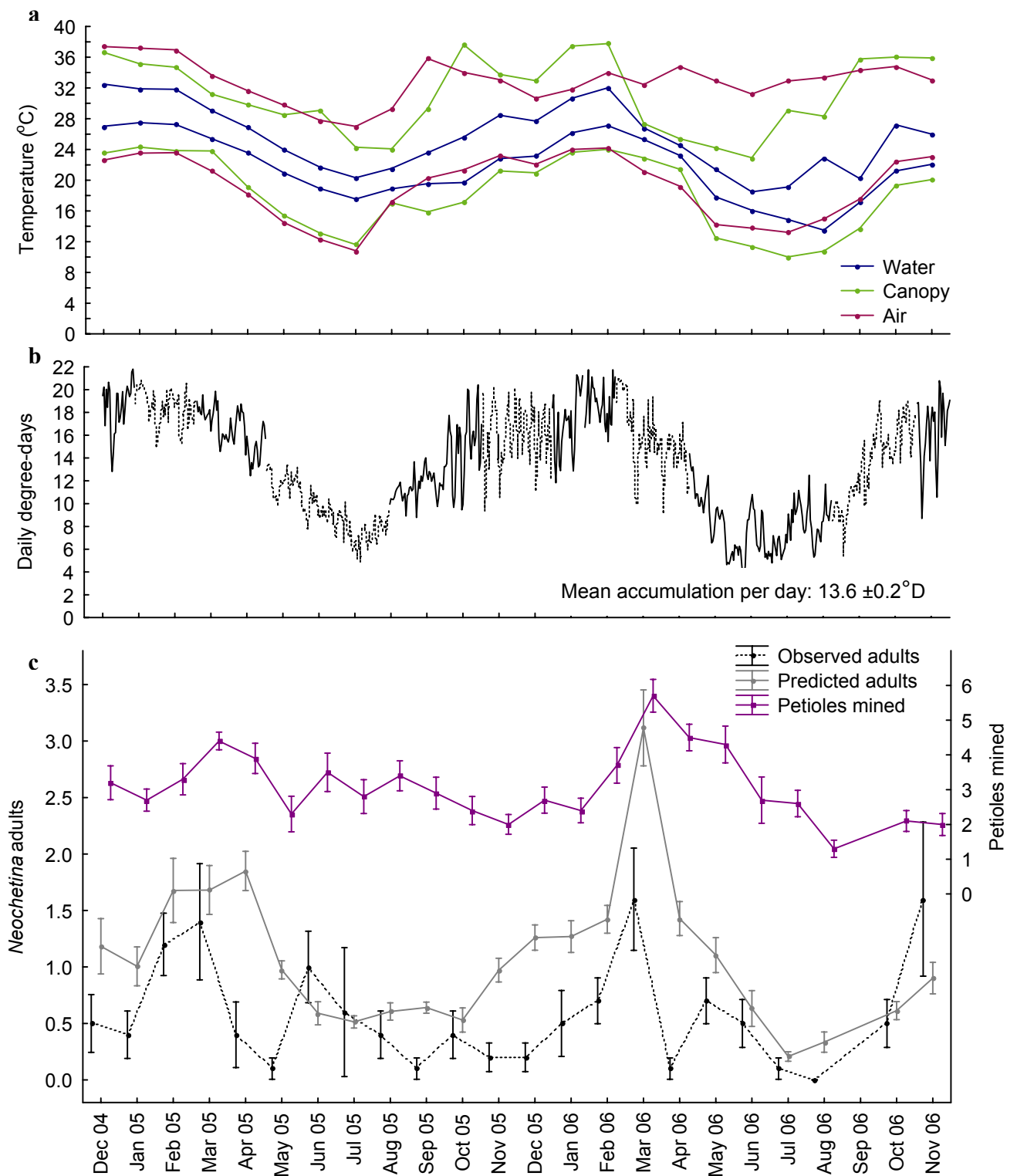
Fig. 3.14. Mkadhzi Spruit: Monthly mean daily maximum and minimum temperature (a) for three microsites; daily degree-days ( t = 9.6^{\circ}\text{C} ) and predicted Neochetina cohorts ( K = 984.4^{\circ}\text{D} ) starting from 24 October 2005 (b) derived from canopy temperature (different line styles denote cohorts); and Neochetina phenology (c) from 2004 to 2006. Weevil phenology is inferred from observed counts of larval mines and adults, and predicted adult numbers are calculated from feeding scars adjusted for monthly leaf production (mean of 10 plants \pm SE).
