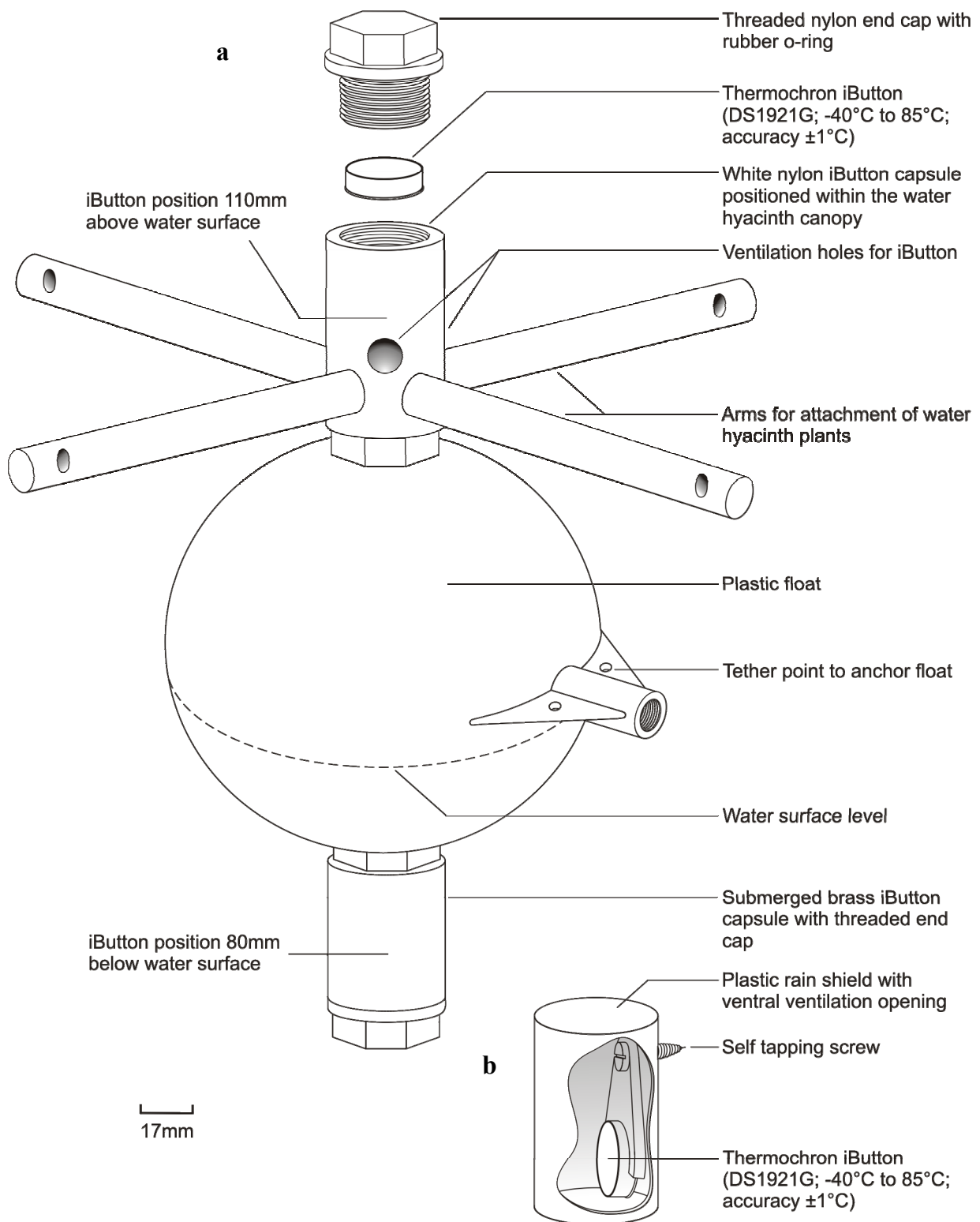
Fig. 3.1. Devices used to monitor temperature (a) within a water hyacinth canopy, water temperature, and (b) air temperature 1.2m above the water surface.
