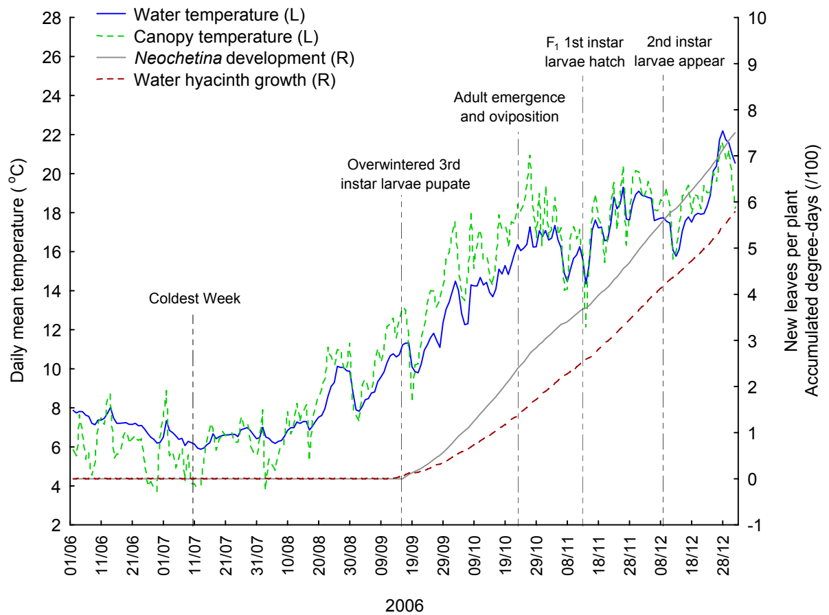
Fig. 2.14. Predicted water hyacinth and Neochetina recovery following adverse conditions during a highveld winter. Leaf production rate and Neochetina accumulation of degree-days during pupation are in response to water temperature. Subsequent Neochetina development is in response to plant canopy temperature.
