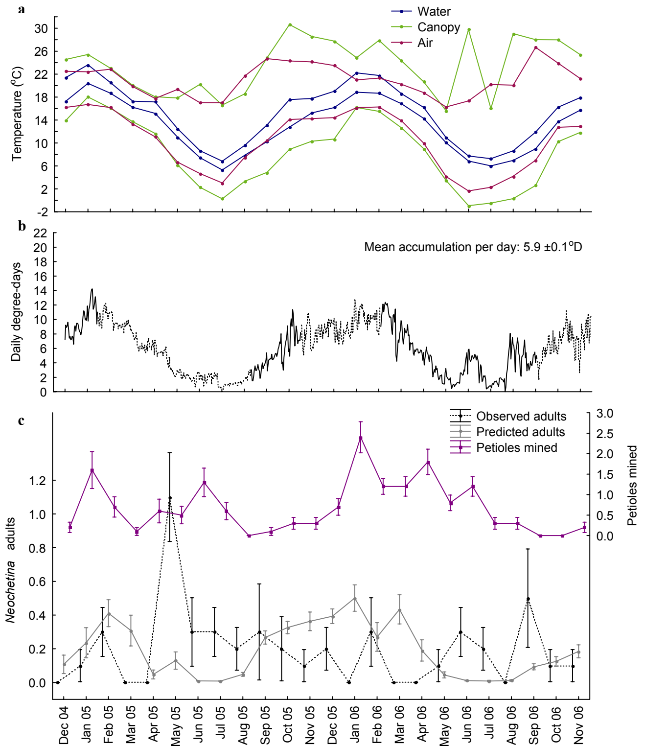
Fig. 3.8. Delta Park: Monthly mean daily maximum and minimum temperature (a) for three microsites; daily degree-days ( t = 9.6^\circ\text{C} ) and predicted Neochetina cohorts ( K = 984.4^\circ\text{D} ) starting from 24 October 2005 (b) derived from canopy temperature (different line styles denote cohorts); and Neochetina phenology (c) from 2004 to 2006. Weevil phenology is inferred from observed counts of larval mines and adults, and predicted adult numbers are calculated from feeding scars adjusted for monthly leaf production (mean of 10 plants \pm SE).
