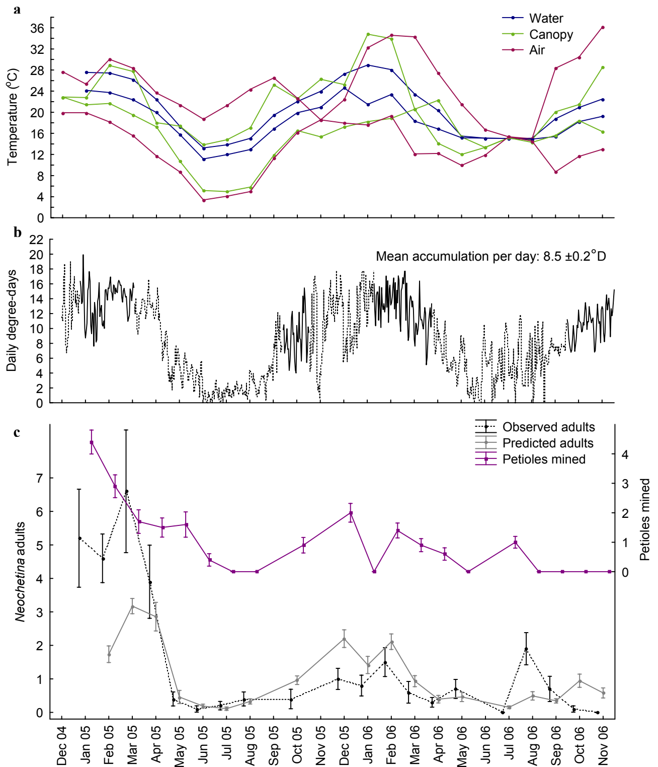
Fig. 3.15. New Years Dam: Monthly mean daily maximum and minimum temperature (a) for three microsites; daily degree-days ( t = 9.6^\circ\text{C} ) and predicted Neochetina cohorts ( K = 984.4^\circ\text{D} ) starting from 24 October 2005 (b) derived from canopy temperature (different line styles denote cohorts); and Neochetina phenology (c) from 2004 to 2006. Weevil phenology is inferred from observed counts of larval mines and adults, and predicted adult numbers are calculated from feeding scars adjusted for monthly leaf production (mean of 10 plants \pm SE).
