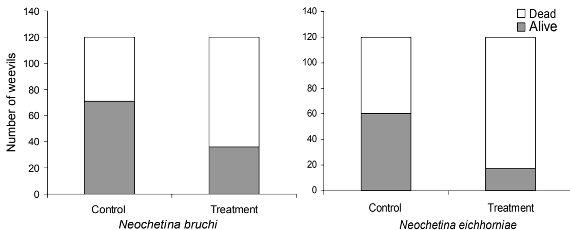
Fig. 2.8. Relative mortality of Neochetina bruchi and Neochetina eichhorniae in response to simulated low and moderate winter temperature regimes (see Table 2.2) from two sites where the weevils have failed to establish (Treatment) and have successfully established (Control) respectively.
