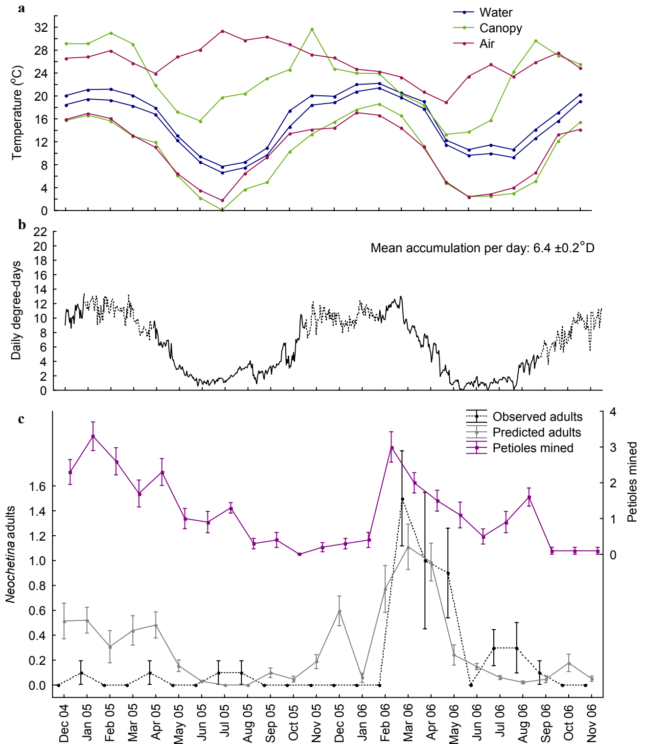
Fig. 3.9. Farm Dam: Monthly mean daily maximum and minimum temperature (a) for three microsites; daily degree-days ( t = 9.6^{\circ}\text{C} ) and predicted Neochetina cohorts ( K = 984.4^{\circ}\text{D} ) starting from 24 October 2005 (b) derived from canopy temperature (different line styles denote cohorts); and Neochetina phenology (c) from 2004 to 2006. Weevil phenology is inferred from observed counts of larval mines and adults, and predicted adult numbers are calculated from feeding scars adjusted for monthly leaf production (mean of 10 plants \pm SE).
