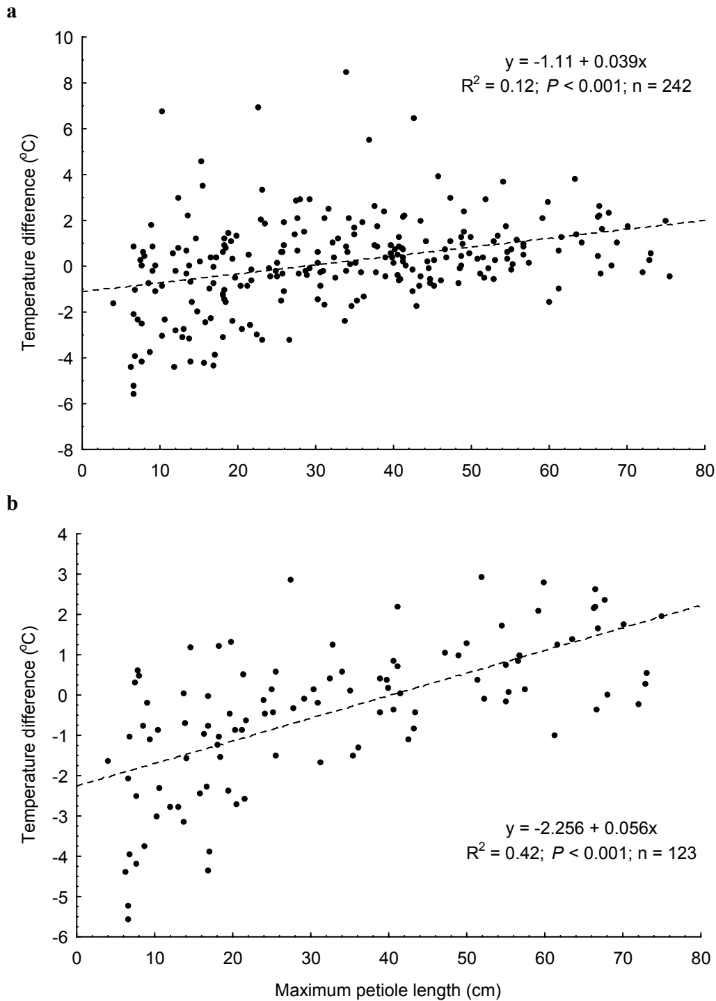
Fig. 3.20. Buffering of lower canopy temperature extremes relative to air temperature lows for all sites (a) and only the relatively colder sites (b) in relation to maximum petiole length (monthly mean from 10 plants). Temperature difference was calculated by subtracting the mean monthly minimum canopy temperature from the corresponding air temperature value.
