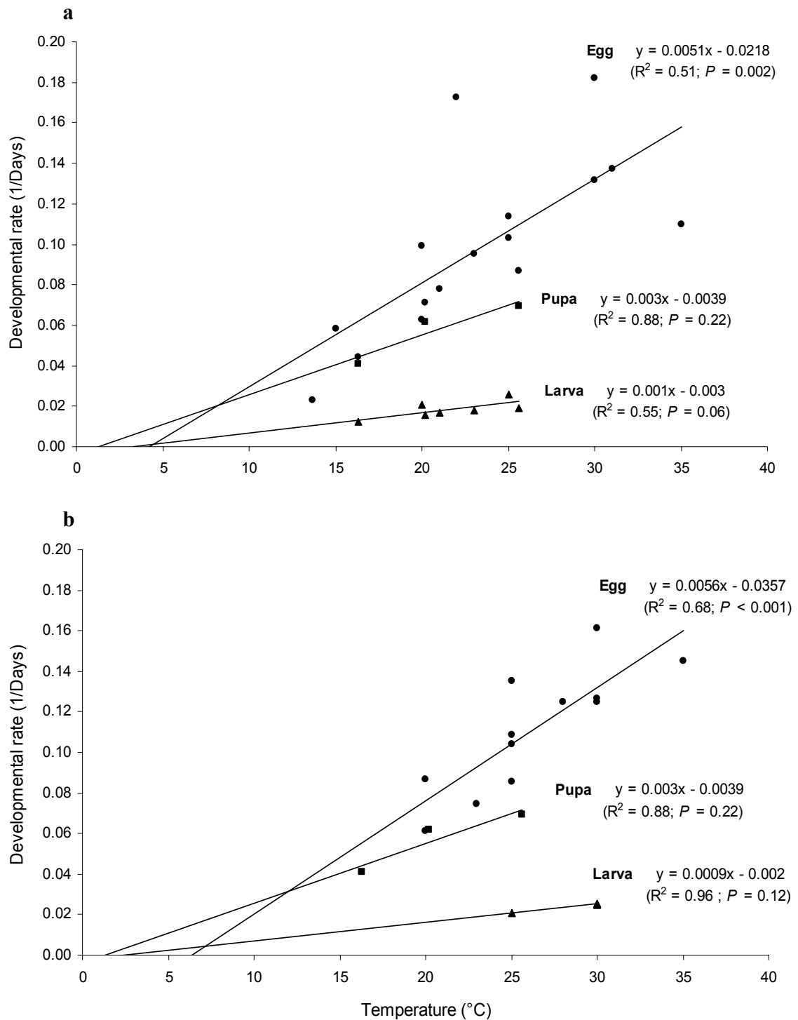
Fig. 2.1. Temperature dependent development of (a) Neochetina bruchi and (b) Neochetina eichhorniae egg, larval and pupal stages using the linear intercept method (Campbell et al. 1974).
