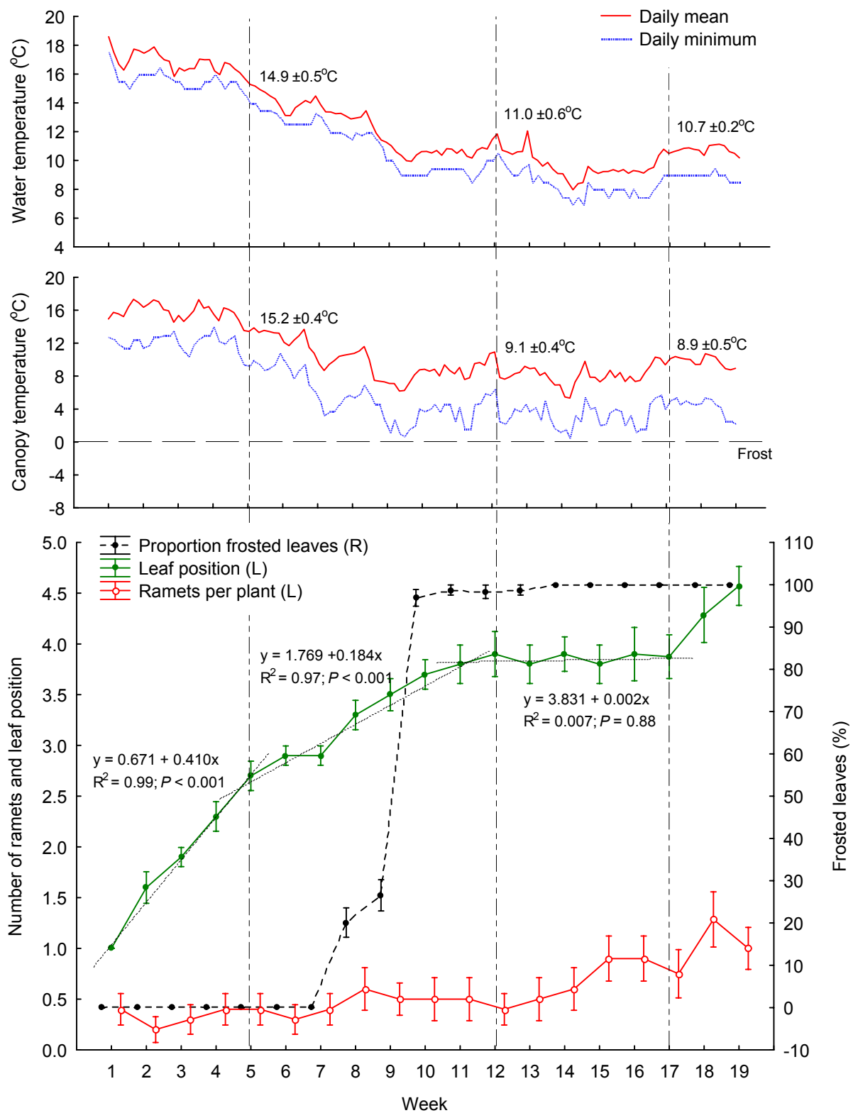
Fig. 2.5. Water hyacinth growth and ramet production (mean of 10 plants \pm SE) at Delta Park upper dam, in response to frost and daily mean and minimum water and plant canopy temperature from March to July 2006. Vertical lines demarcate distinct rates of leaf production.
