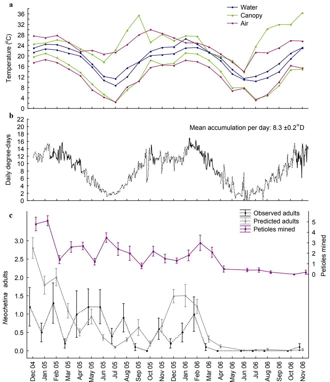
Fig. 3.7. Crocodile River: Monthly mean daily maximum and minimum temperature (a) for three microsites; daily degree-days ( t = 9.6^{\circ}\text{C} ) and predicted Neochetina cohorts ( K = 984.4^{\circ}\text{D} ) starting from 24 October 2005 (b) derived from canopy temperature (different line styles denote cohorts); and Neochetina phenology (c) from 2004 to 2006. Weevil phenology is inferred from observed counts of larval mines and adults, and predicted adult numbers are calculated from feeding scars adjusted for monthly leaf production (mean of 10 plants \pm SE).
