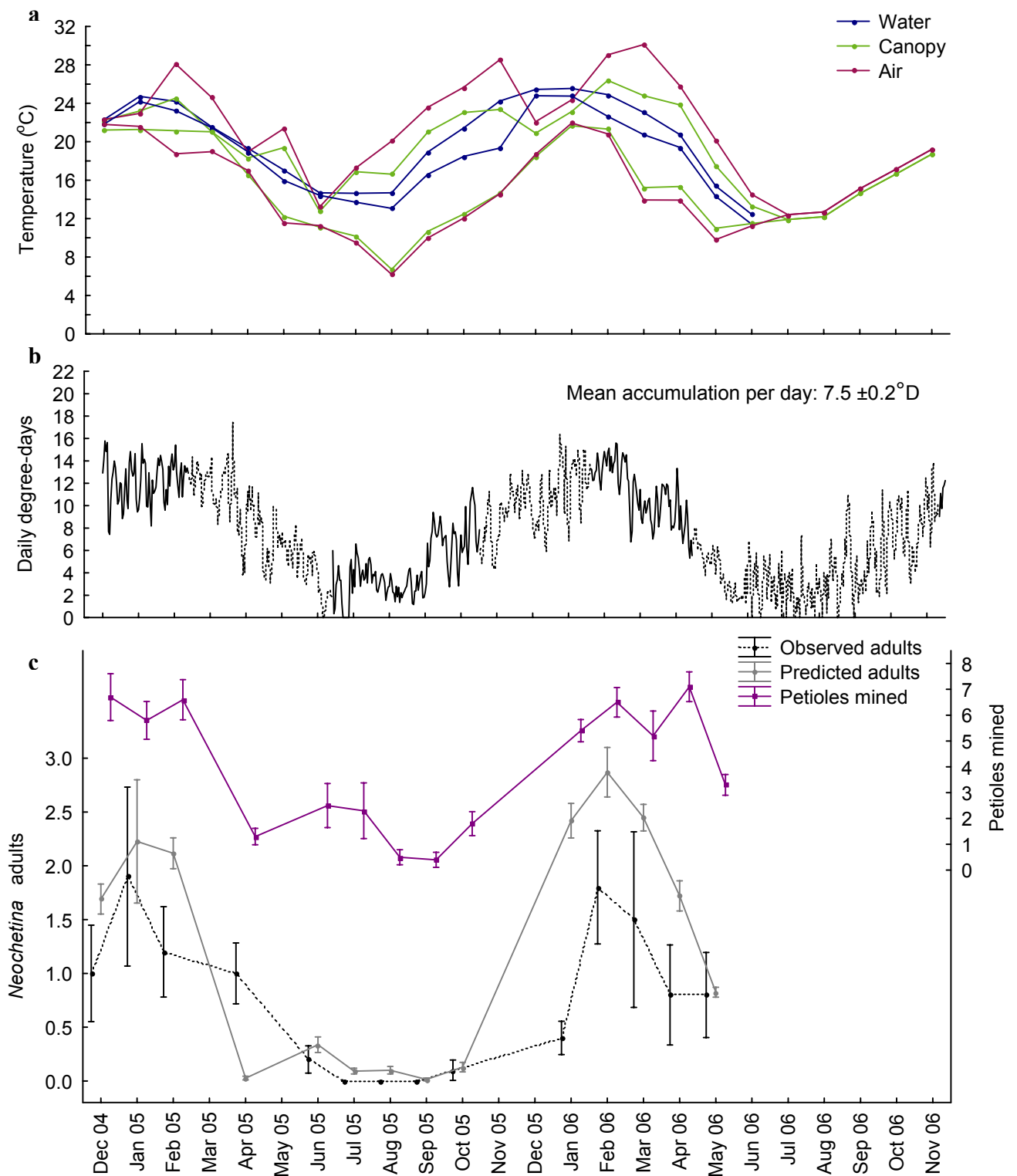
Fig. 3.6. Breede River: Monthly mean daily maximum and minimum temperature (a) for three microsites; daily degree-days ( t = 9.6^\circ\text{C} ) and predicted Neochetina cohorts ( K = 984.4^\circ\text{D} ) starting from 24 October 2005 (b) derived from canopy temperature (different line styles denote cohorts); and Neochetina phenology (c) from 2004 to 2006. Weevil phenology is inferred from observed counts of larval mines and adults, and predicted adult numbers are calculated from feeding scars adjusted for monthly leaf production (mean of 10 plants \pm SE).
