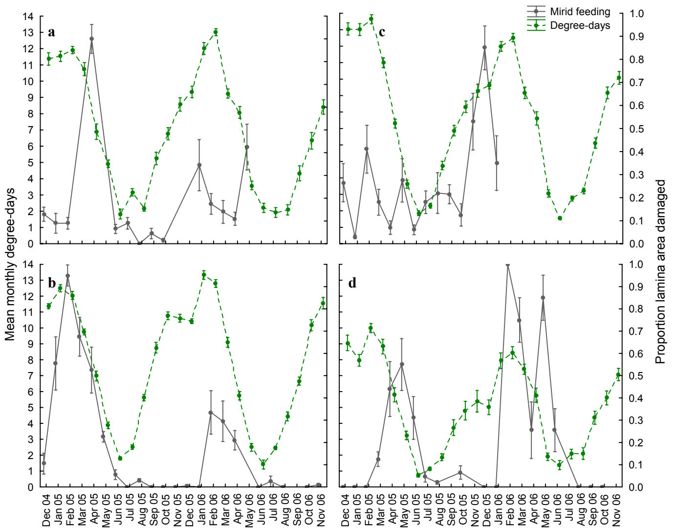
Fig. 3.22. Eccritotarsus catarinensis feeding intensity relative to the mean monthly degree-days (calculated from degree-hours) recorded from 2004 to 2006 at four field sites, Breede River (a), Crocodile River (b), Hammarisdale Dam (c), and Kubusi River (d). Feeding damage was ranked between 0 (no leaf area damaged) and 1 (50 to 100% leaf area damaged) (mean from 10 plants \pm SE).
