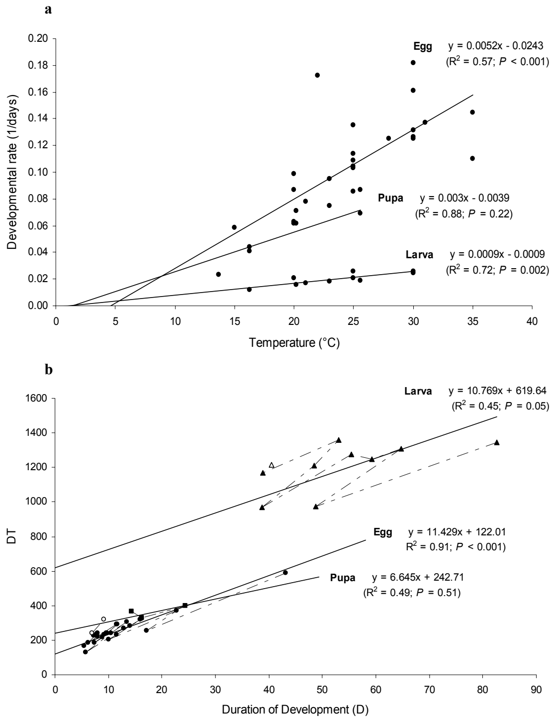
Fig. 2.3. Temperature dependent development of Neochetina bruchi and Neochetina eichhorniae combined using (a) the linear intercept (Campbell et al. 1974) and (b) reduced major axis regression (Ikemoto and Takai, 2000) methods. Unshaded points were omitted from the regression.
