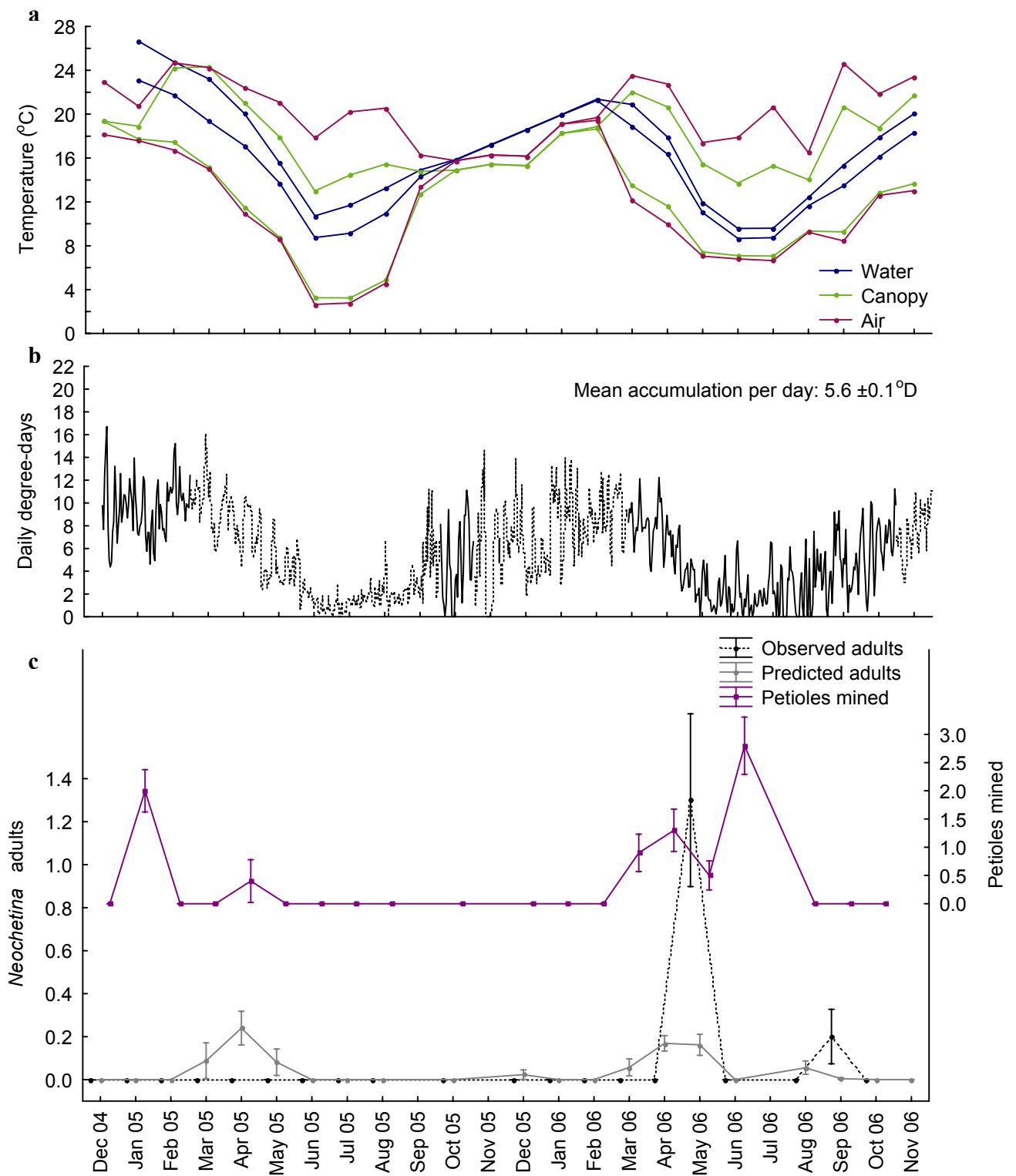
Fig. 3.12. Kubusi River: Monthly mean daily maximum and minimum temperature (a) for three microsites; daily degree-days ( t = 9.6^{\circ}\text{C} ) and predicted Neochetina cohorts ( K = 984.4^{\circ}\text{D} ) starting from 24 October 2005 (b) derived from canopy temperature (different line styles denote cohorts); and Neochetina phenology (c) from 2004 to 2006. Weevil phenology is inferred from observed counts of larval mines and adults, and predicted adult numbers are calculated from feeding scars adjusted for monthly leaf production (mean of 10 plants \pm SE).
