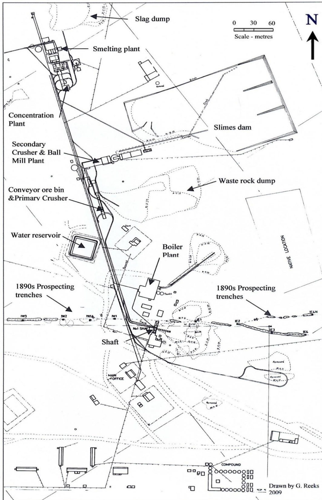
Appendix 1 Central portion of the re-drawn 1920s plan of the surface plant of the Transvaal Silver and Base Metals Ltd mine. Traced from the original plan.
