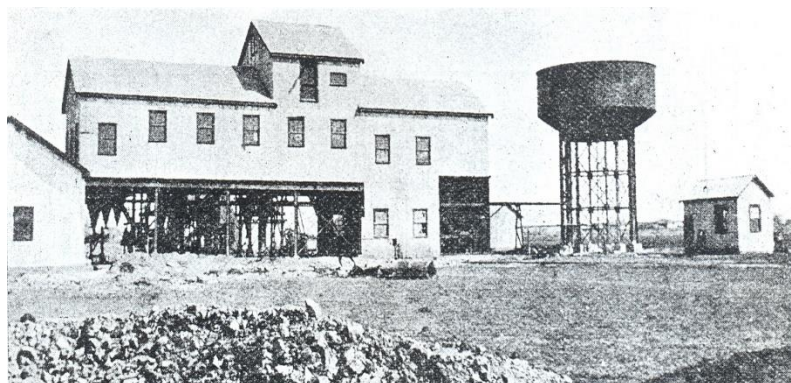
Figure 37. Historical photograph of the Secondary crushing plant which contained the wash trommels, crushing rolls and Harz jig machines (Clayden 1922). 58
