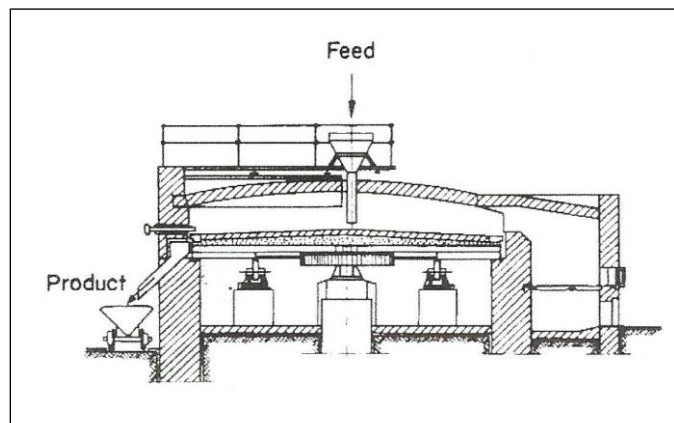
Figure 70. Godfrey type of rotary roasting or sintering furnace. (Habashi 2005)
