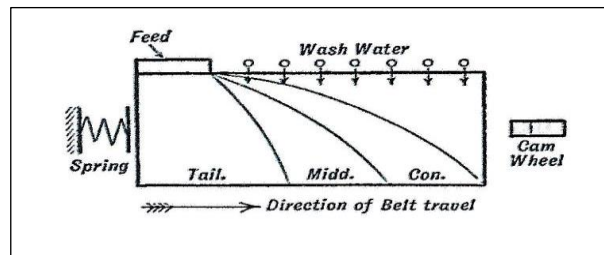
Figure 30. Diagram illustrating the direction of feed, water and eventual separation of tailings, middlings and concentrates on a Lührig Vanner (Truscott 1923:358).
