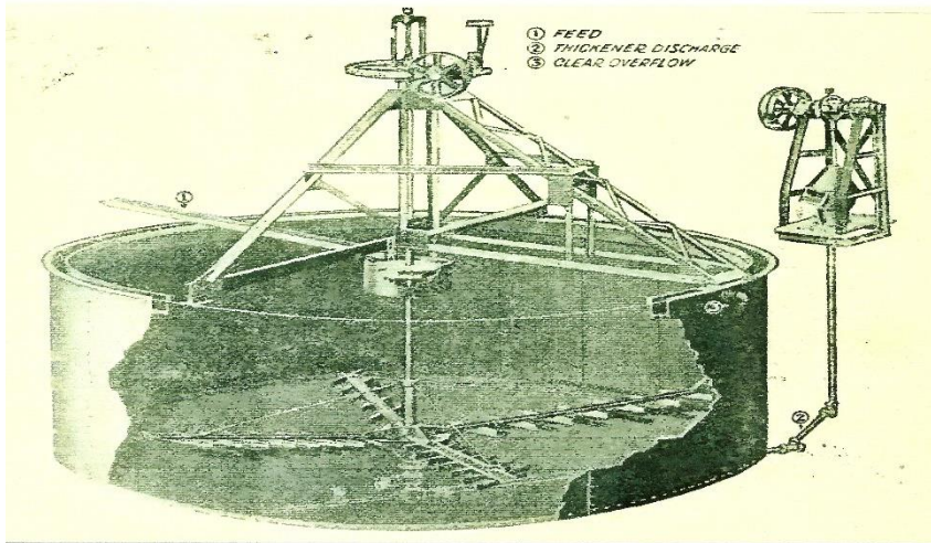
Figure 66. Dorr Thickener. (Truscott 1919:274)
