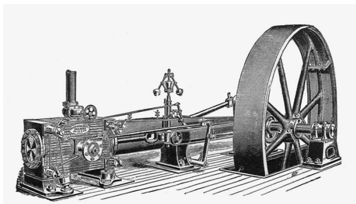
Figure 13. Fraser and Chalmers Horizontal Corliss Engine (Hawkins 1904:182).
