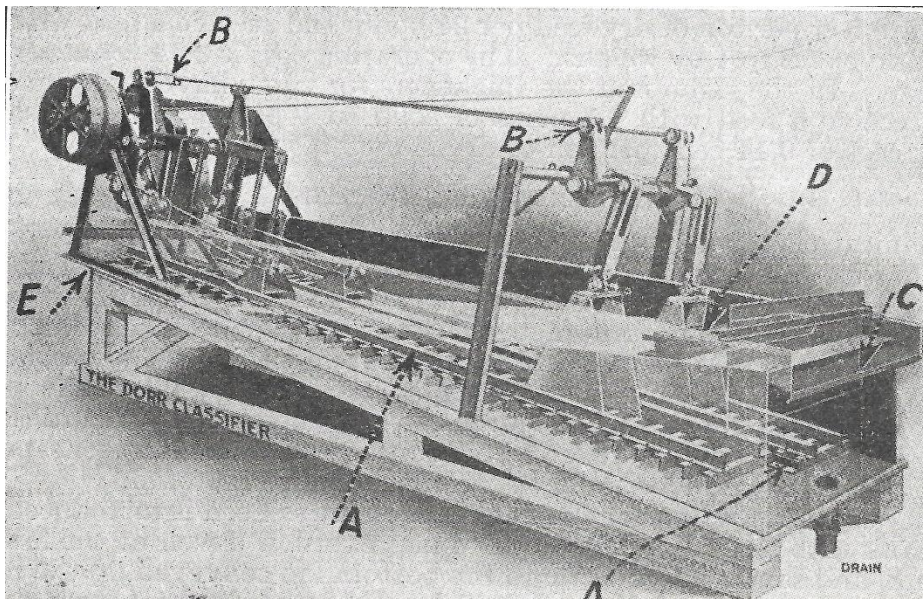
Figure 64. Dorr Rake Classifier (Richards & Locke 1940:164).
