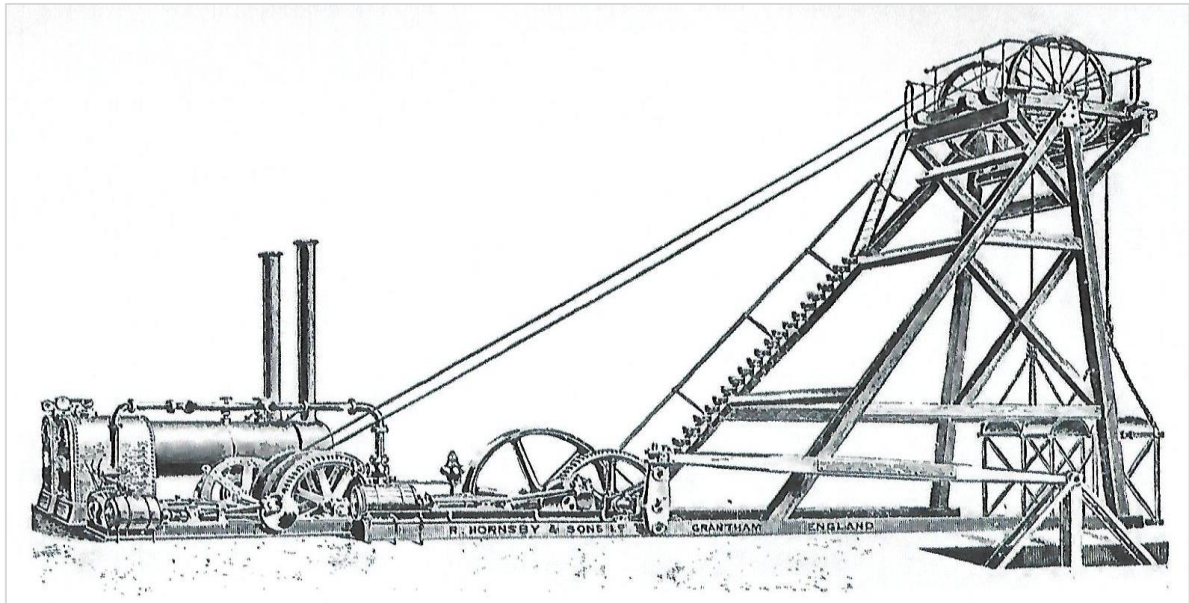
Figure 10. Arrangement of winding gear coupled with a pumping engine attached to a flat rod and the Tee bob. Note although this shows a different make of engine namely R Hornsby & Son Ltd the arrangement is the same as was installed at Argent (Davies 1902:91).
