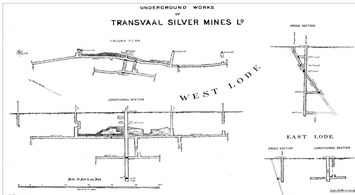
Figure 14. Transvaal Silver Mine Ltd. 1892 underground mine plan. Note some of the details on the plans may be poor, due to the reduction from an A1 size original. The plan is reproduced as Appendix 3.0 in a larger scale.
