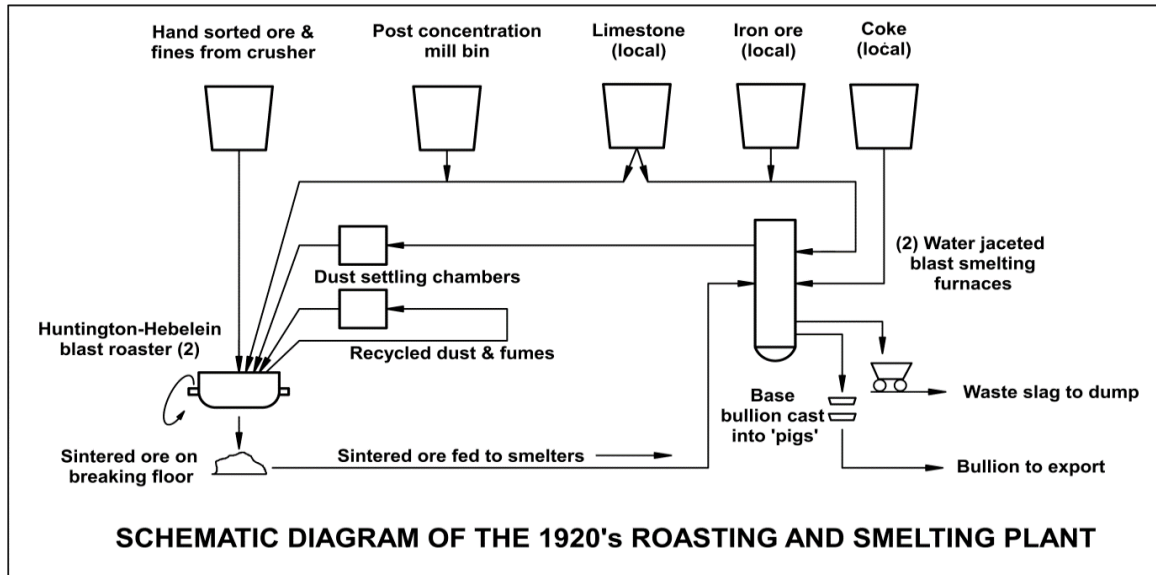
Figure 40. Schematic diagram of the 1920s roasting and smelting process. Based on part of the original Flow sheet, 69 and text descriptions (Clayden 1922). (Drawn by G. Reeks).
