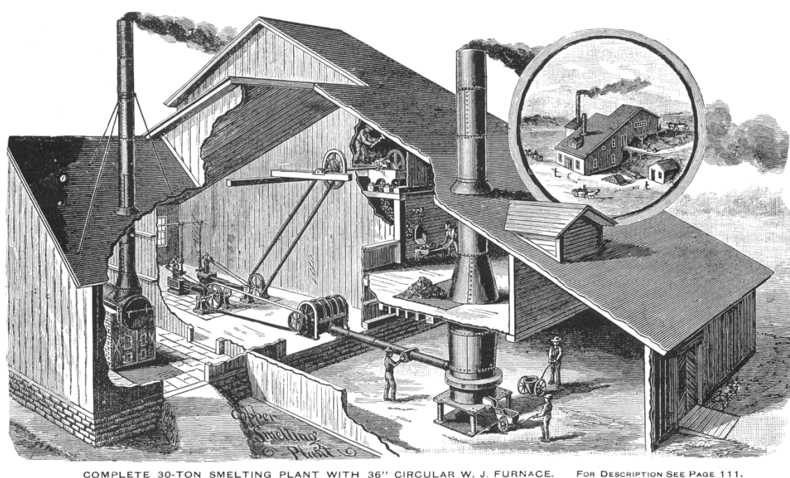
Figure 44. Artist's impression of a smelting plant for copper or lead ores using a water jacket blast furnace. c1890s through to 1920s. Such a plant is similar to what would have existed at the TSM and TSBM mine at Argent in the 1890s and 1920s. 84
