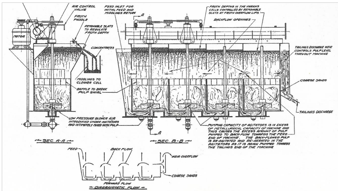
Figure 68. Drawing showing the flows and principle parts of a Minerals Separation Ltd Sub-Aeration Flotation Cell machine. (Richards & Locke. 1940:253).
