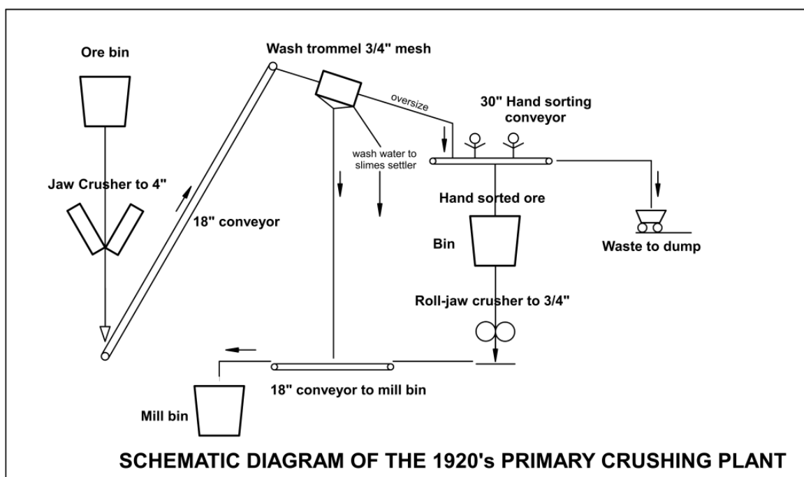
Figure 35. Flow diagram of the Crushing process at the TSBM mine c 1919-1926 based on part of the original Flow sheet, 50 and text descriptions (Clayden 1922). (Drawn by G. Reeks).
