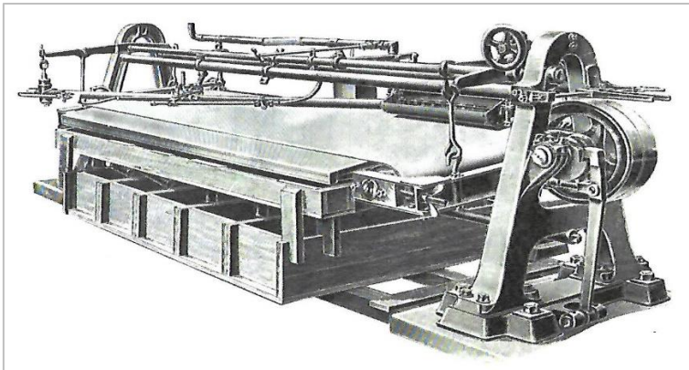
Figure 20. Bilharz-Stein bumping table (Louis 1909:362)
