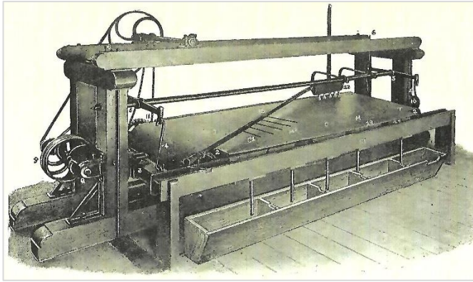
Figure 31. Lührig Vanner (Davies 1902:345)
