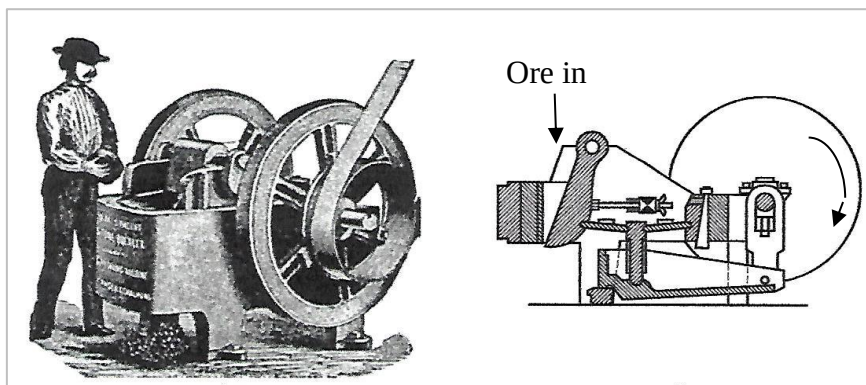
Figure 22. Blake Jaw crusher (Lynch & Rowland 2005:62).
