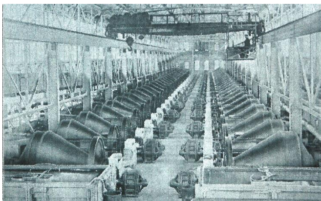
Figure 60. An early example of the significant use of Hardinge Conical Ball Mills at the Calumet and Hecla Mine, Michigan, USA in 1910. 19
