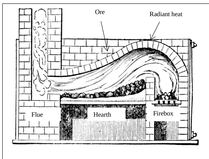
Figure 17. Principle of operation of a reverberatory furnace for roasting the ore. The reflected heat roasts the ore. 75
