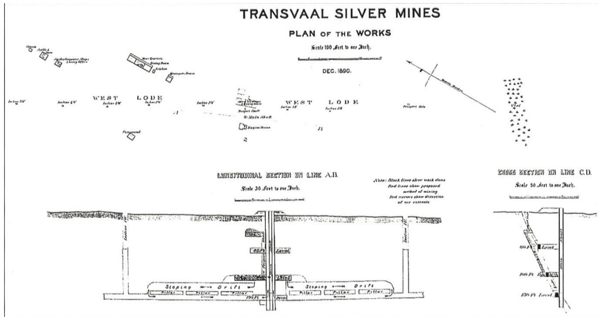
Figure 9. Transvaal Silver Mine Ltd. 1890 mine plan – underground and surface structures. Some of the details on the plan may be poor, due to the reduction from an A1 size original. The plan is reproduced as Appendix 2.0 as a full A4 page copy.
