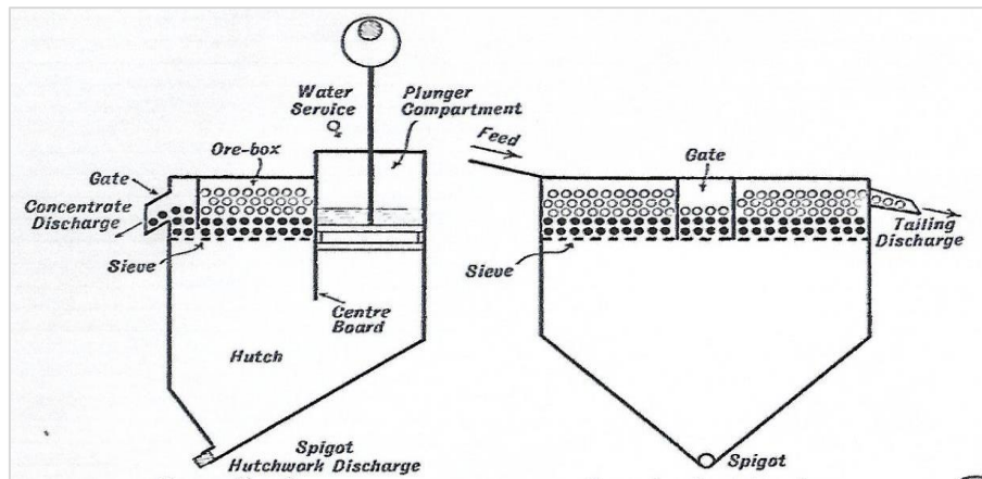
Figure 28. Diagrammatic sections of a single cell in a Harz Jig. The sections illustrate the gate discharge for concentrate, spigot discharge for fines and overflow discharge for tailings (Truscott 1923:303).
