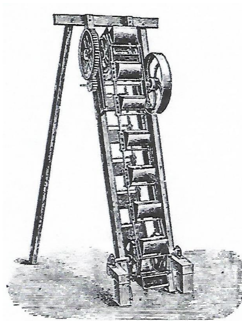
Figure 25. Bucket elevator (Davies 1902:409)
