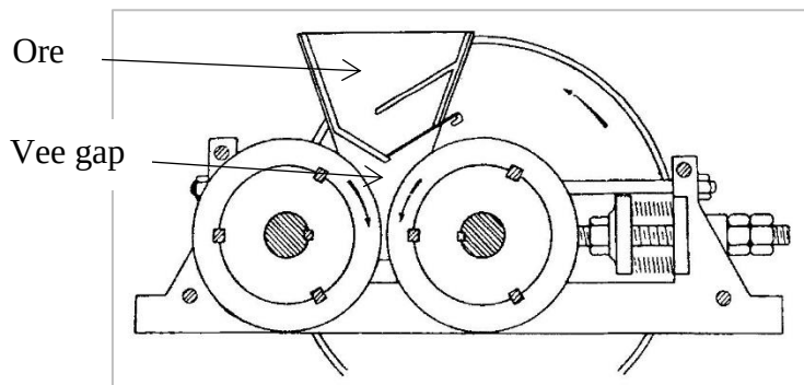
Figure 23. Cornish Roll showing directions of rotation and vee gap (Wills 1979:168).
