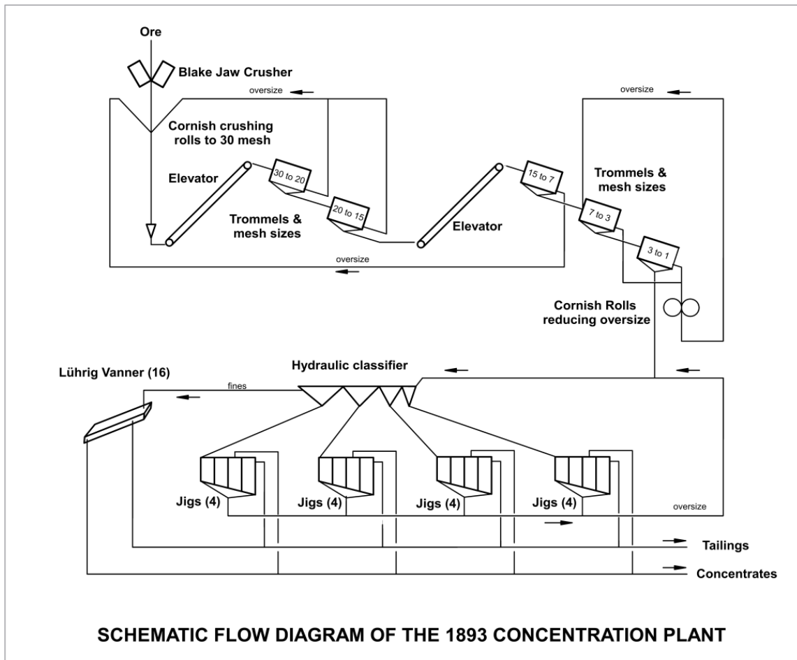
Figure 21. Schematic flow diagram of the concentration plant on the TSM 1893-1895. It is based on the known items of equipment purchased by Wertheman, along with various engineering journal articles (as quoted). The sizes shown on the trommels and Cornish Rolls are hypothetical but are based on flow diagrams in various textbooks. (Truscott, 1923; Richards & Locke 1940). The bold numbers in brackets refer to the number of machines in the references. It is unclear if there was more than one hydraulic classifier. It is however more likely that there were four classifiers feeding the 16 Jigs (P. den Hoed and M. Dworzanowski at School of Chemistry and Metallurgy, University of the Witwatersrand, 2017 – pers. comm. 15 May 2017) (Diagram drawn by G. Reeks).
