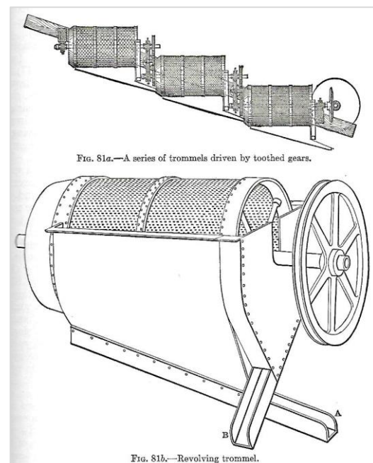
Figure 26. Revolving trommel and a Series Trommel. (Richards & Locke 1940:121)
