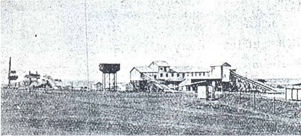
Figure 33. Historical photograph of the Argent mine - general view of the 1920s beneficiation plant. 27 The main part to the right of the picture is the incline conveyor leading to the primary crusher and then the secondary crusher plant (see Figs 36 and 37).
