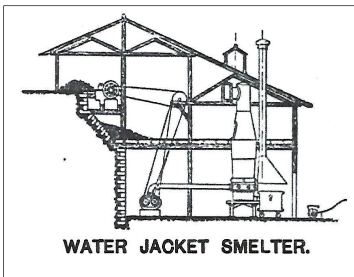
Figure 16. Idealised sketch of a smelting house with a Water Jacket smelter and charging floors (Eissler 1891:435).
