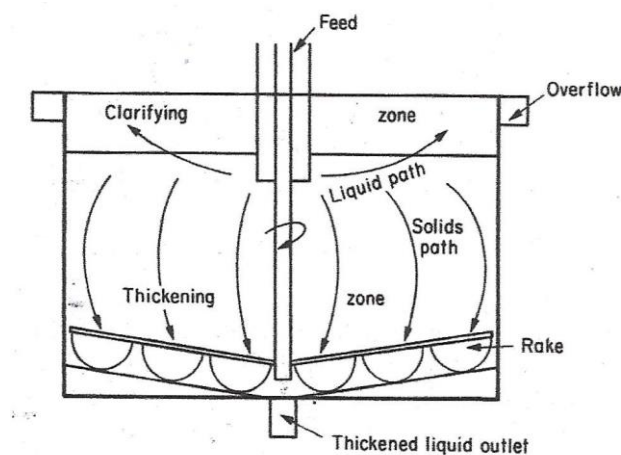
Figure 67. The principle of action within a Dorr Thickener (Wills 1979:376).
