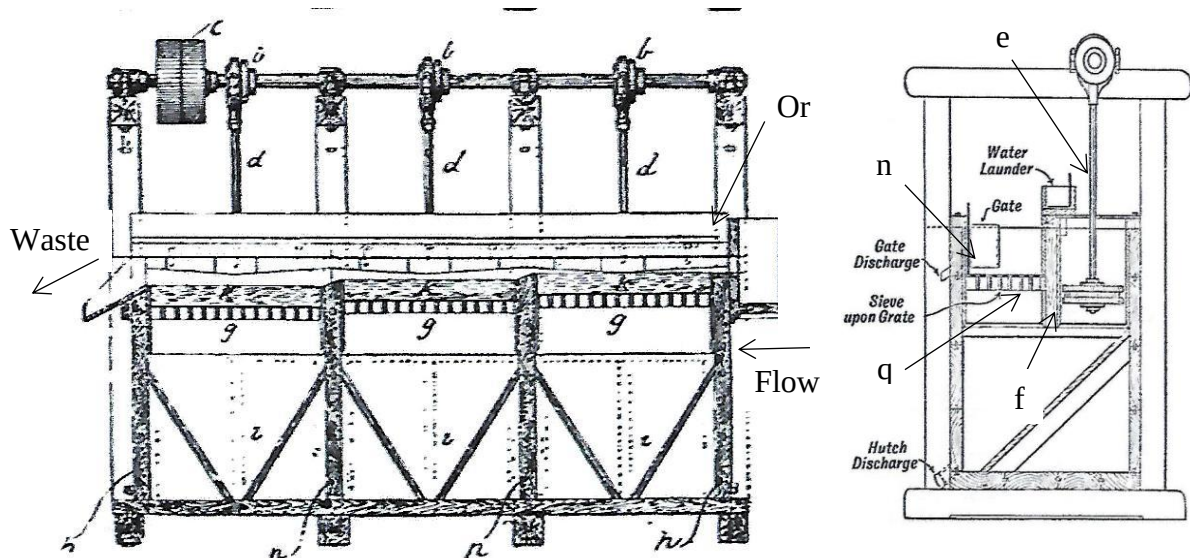
Figure 27. Longitudinal and cross section of a three stage Harz Jig - water flow, right to left. (Davies 1902:294 and Truscott 1923:303)
