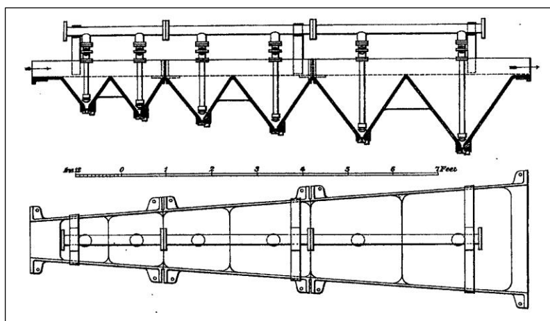
Figure 29. Lenique hydraulic classifier dating to c1888. Flow of water and concentrate from left to right (Louis 1909:237)
