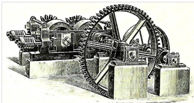
Figure 24. Cornish Rolls machine with the feed chute and machine covers removed. (Davies 1902:238).
