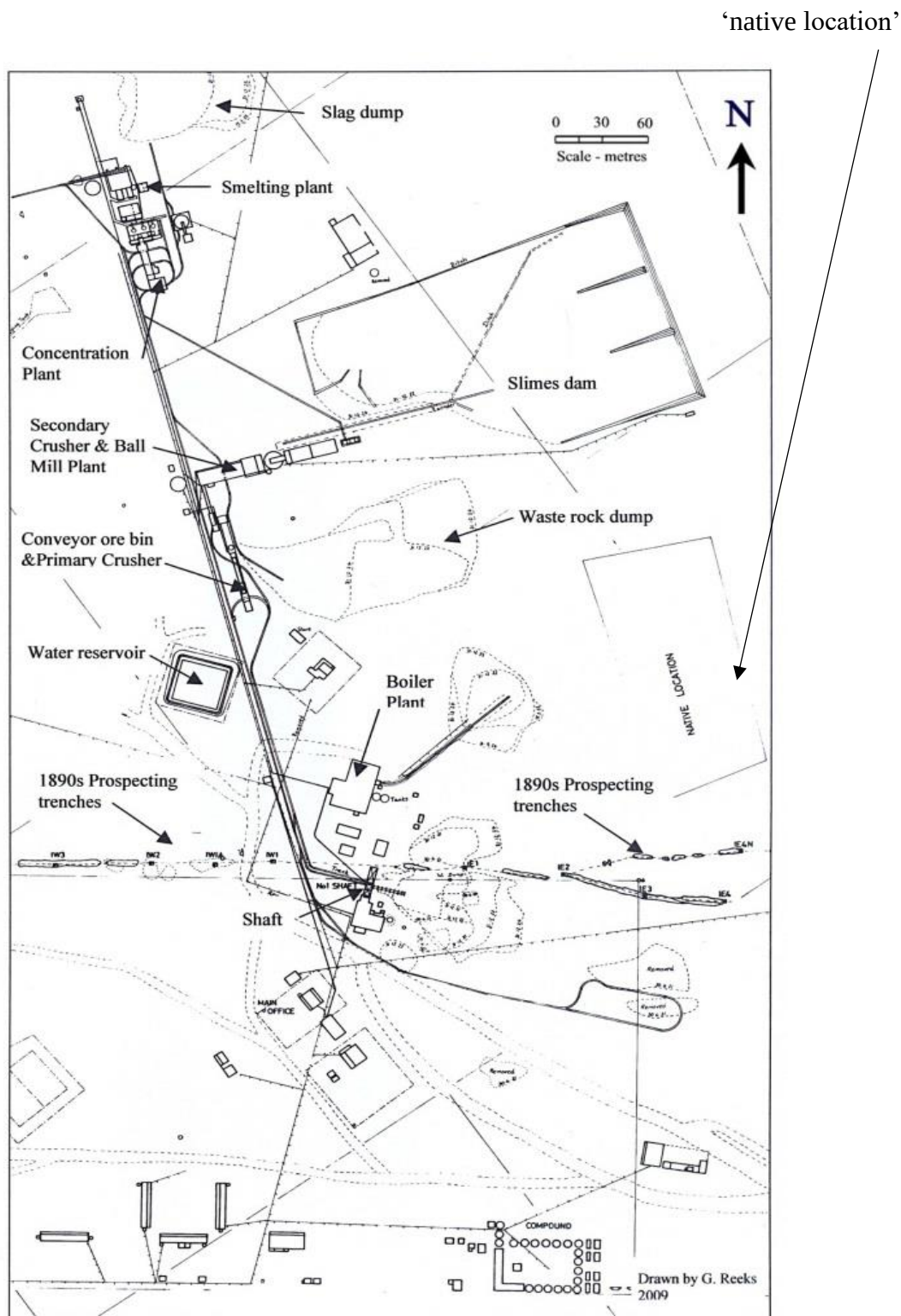
Figure 73. Part of the 1920s surface plan of the TSBM mine plan (Drawn G. Reeks).
