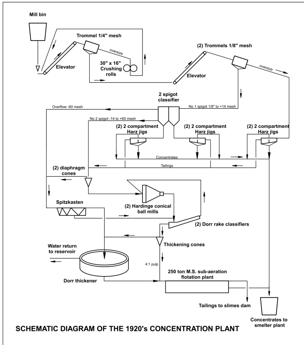
Figure 38. Schematic diagram of the Concentration process at the TSBM mine c 1919-1922 based on part of the original Flow sheet, 62 and text descriptions (Clayden 1922). (Drawn by G. Reeks).
