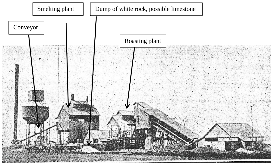
Figure 42. Historical photograph of the smelting and roasting sintering plant at TSBM c1922. 75
