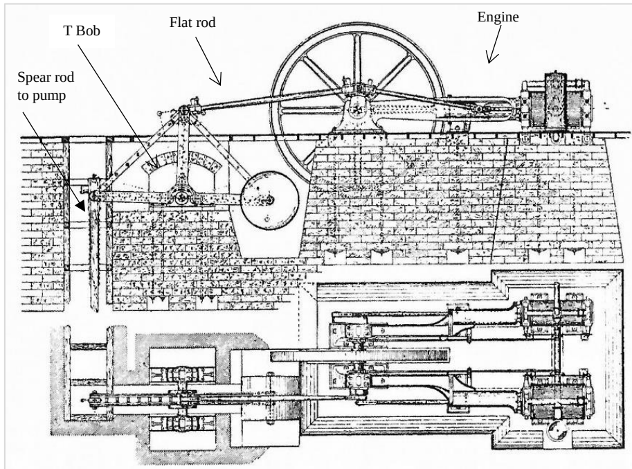
Figure 11. Showing a detail of a T bob, engine, and spear rod at the pumping shaft. (Davies 1902:115).
