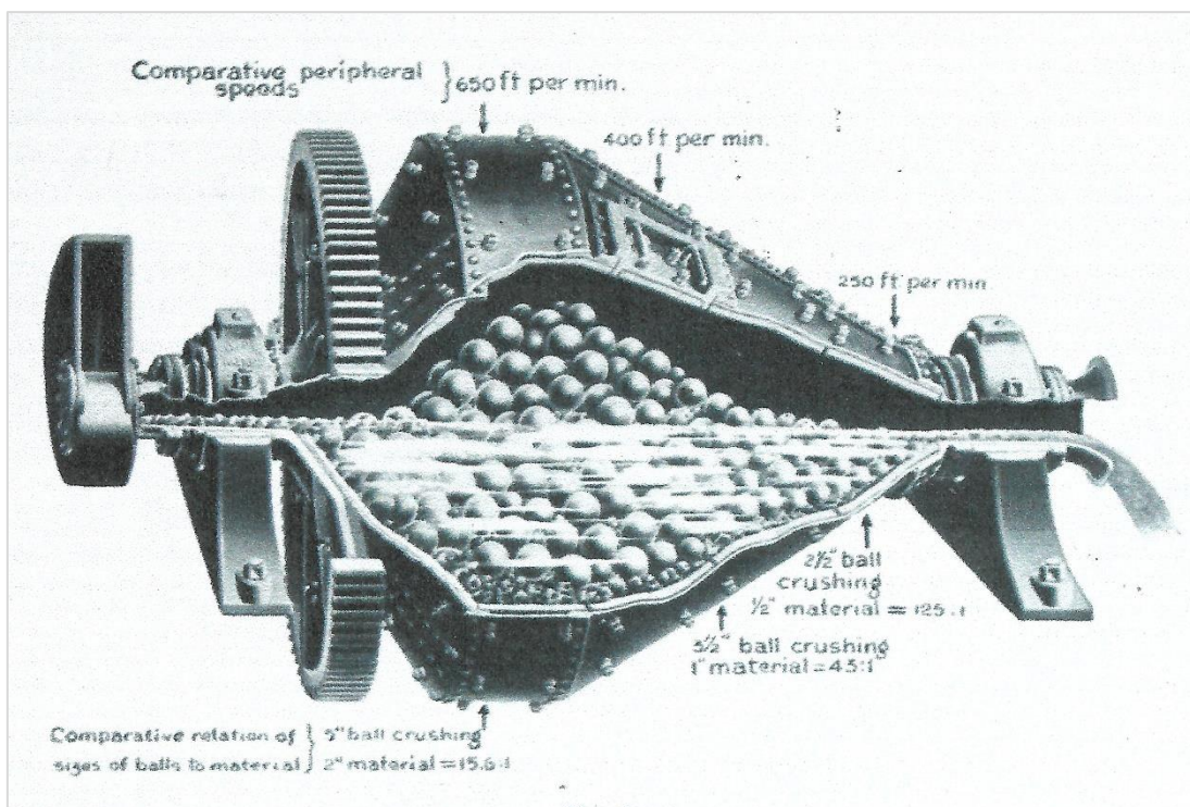
Figure 59. Hardinge Conical Ball Mill. 17
