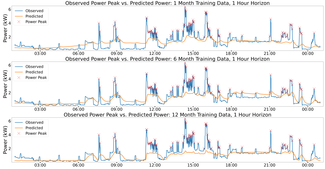
FIGURE 4.8: Comparison of observed peaks vs predicted power profile for the 1, 6 and 12-month prediction models.
