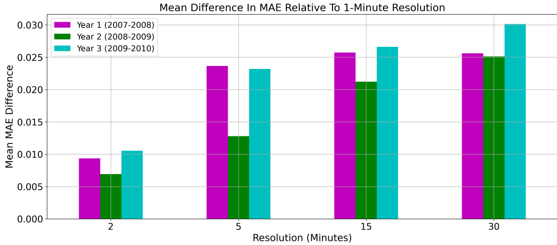
FIGURE 4.16: Mean Difference In MAE For Lower Resolution Models Relative to 1-Minute Resolution Models.
