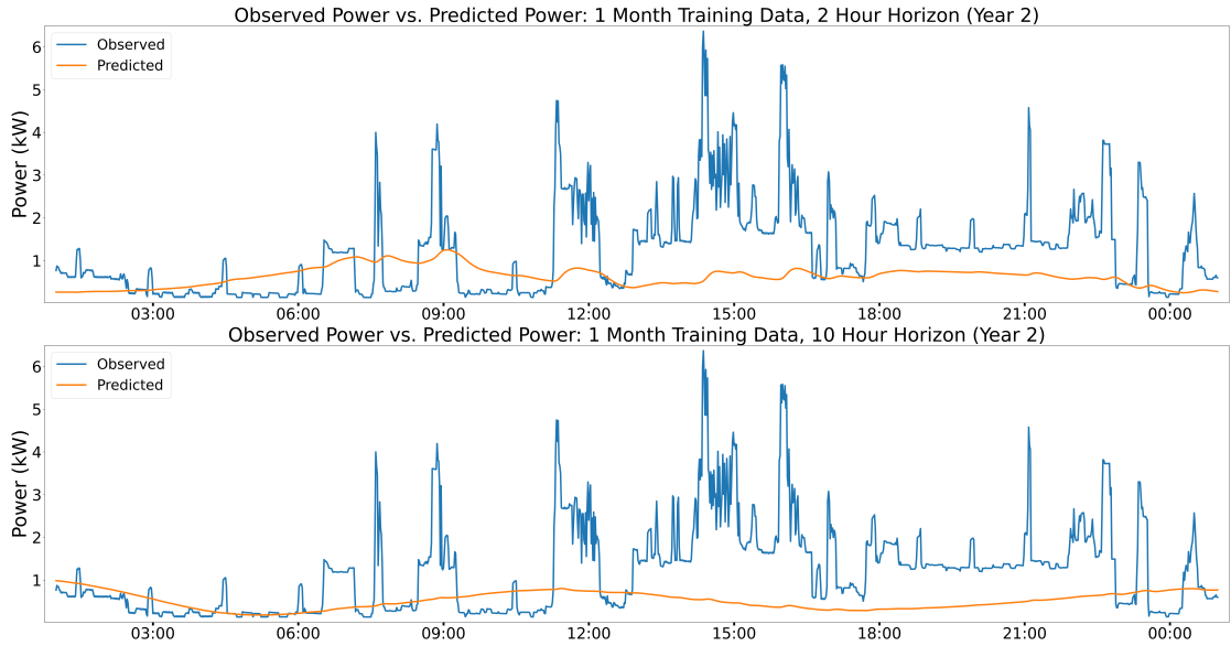
FIGURE 4.14: Comparison of observed and predicted power between 2-hour and 10-hour horizon length models.
