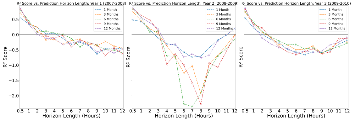
FIGURE 4.9: Comparison of R^2 scores for 1, 3, 6, 9 and 12-month training size models over three years.
