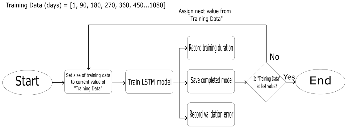
FIGURE 3.6: Flow diagram of Experiment A algorithm
