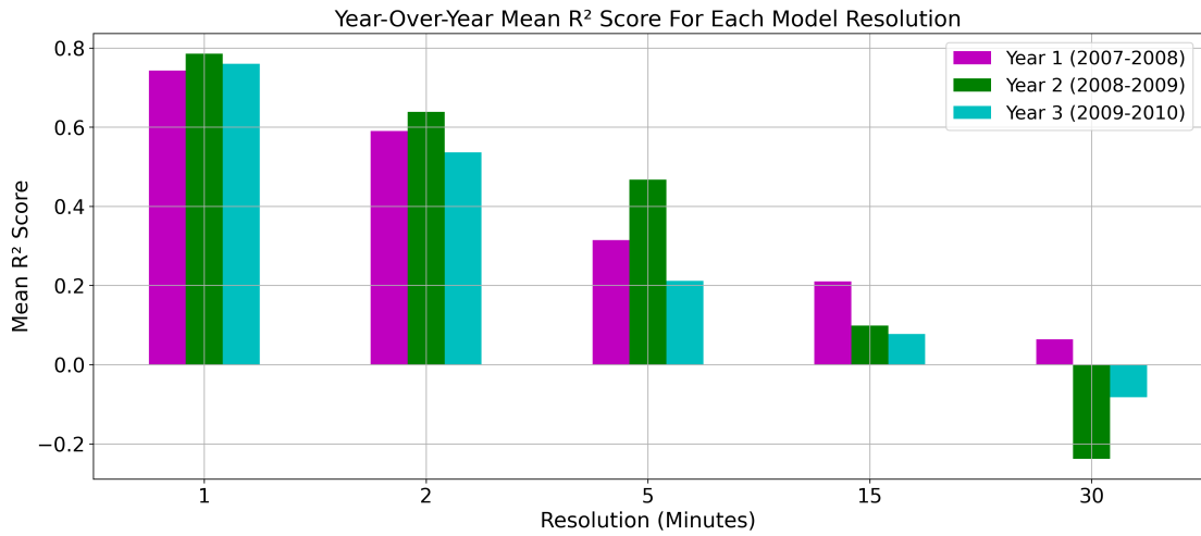
FIGURE 4.21: Mean R^2 scores of each year for 1, 5, 15, and 30-minute resolution models.
