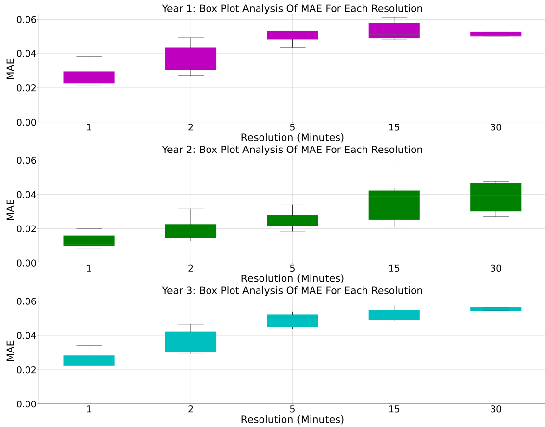
FIGURE 4.17: Box plot analysis of MAE distributions for models of each resolution.
