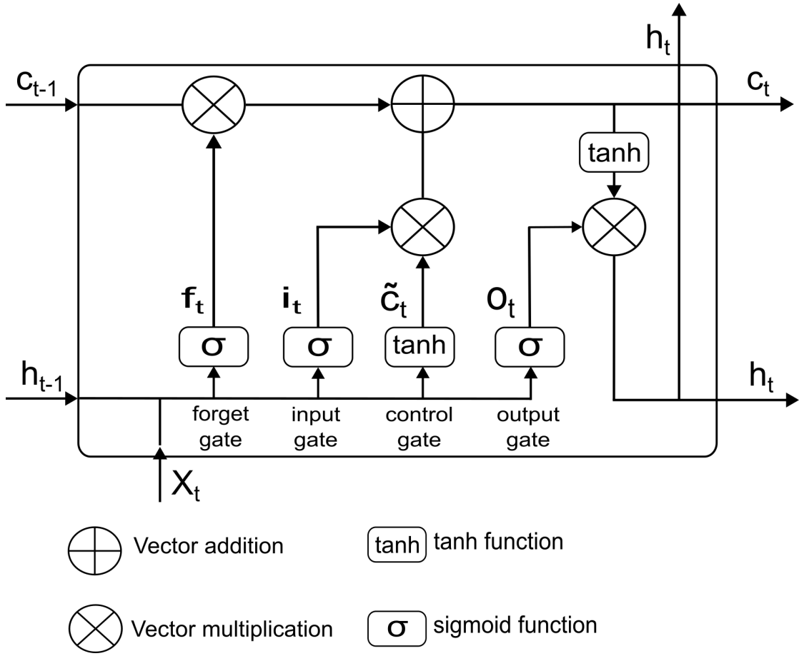
FIGURE 2.2: Architecture of a single LSTM cell adapted from [93]
