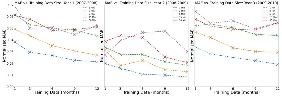
FIGURE 4.15: Comparison of model prediction errors and training data size for various data resolutions.
