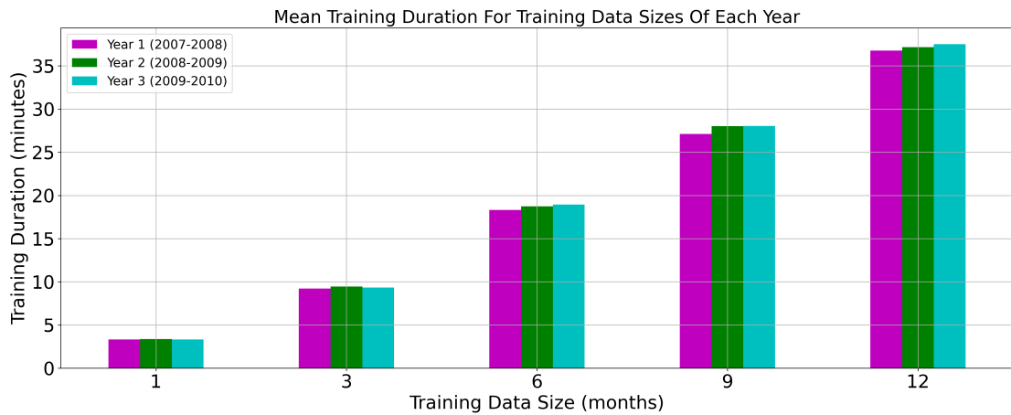
FIGURE 4.11: Comparison of mean model training time for each year of training data up to a horizon length of three hours.
