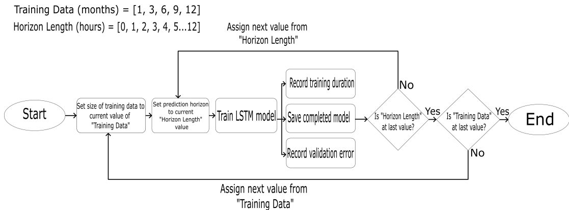
FIGURE 3.7: Flow diagram of Experiment B algorithm
