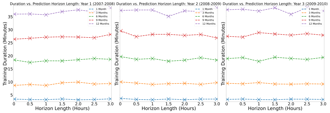
FIGURE 4.10: Comparison of training durations for each training data size up to a prediction horizon length of three hours
