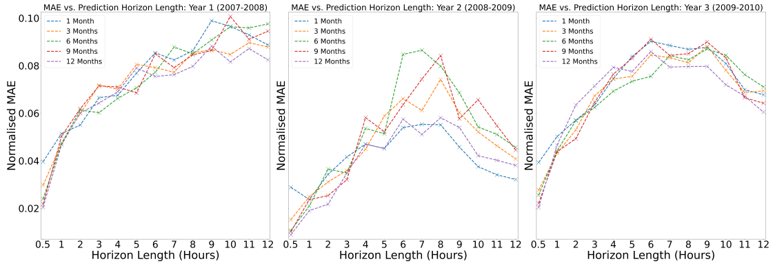
FIGURE 4.5: Comparison of model prediction errors and training data size for various prediction horizon lengths
