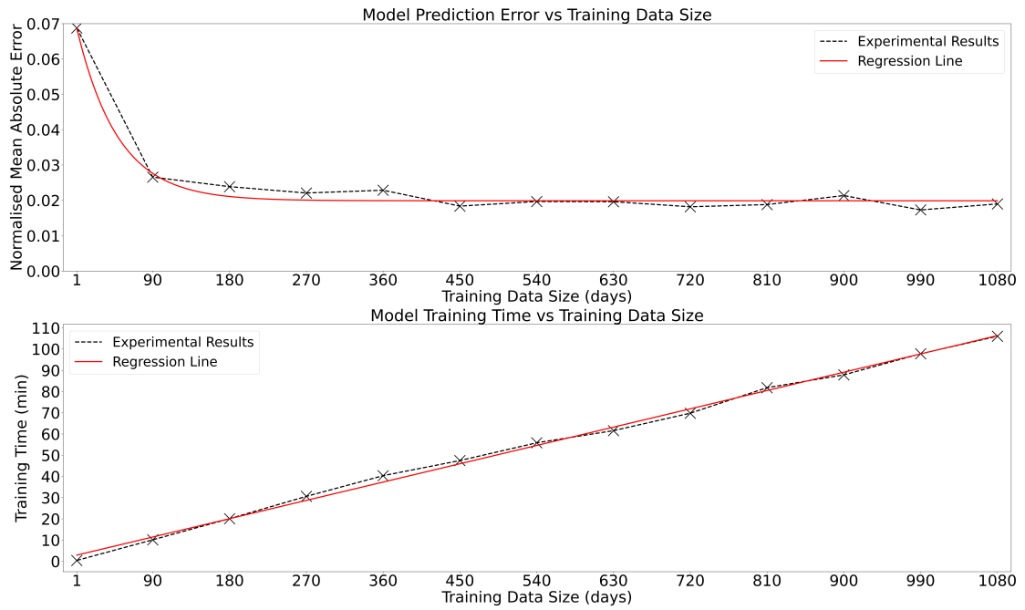
FIGURE 4.1: Comparison of model prediction errors and training time against training data size
