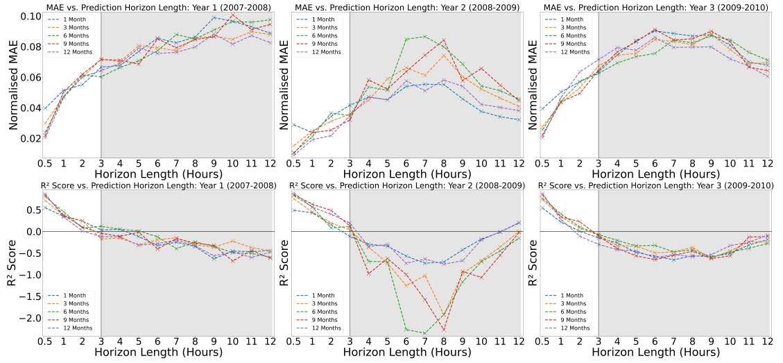
FIGURE 4.13: Illustration of the MAE and R^2 scores within the 3 hour prediction horizon length.
