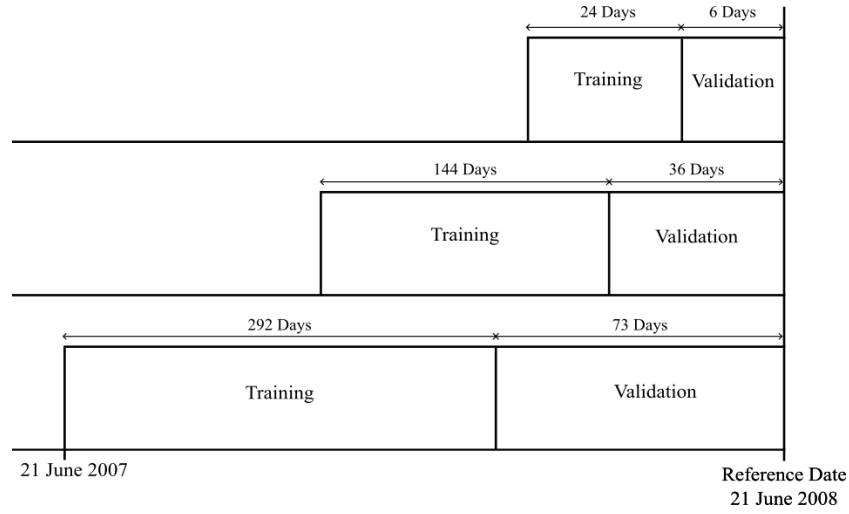
FIGURE 3.10: Selection of measurements for the 1, 6 and 12-month sizes of training-validation data in the Year 1 subset.
