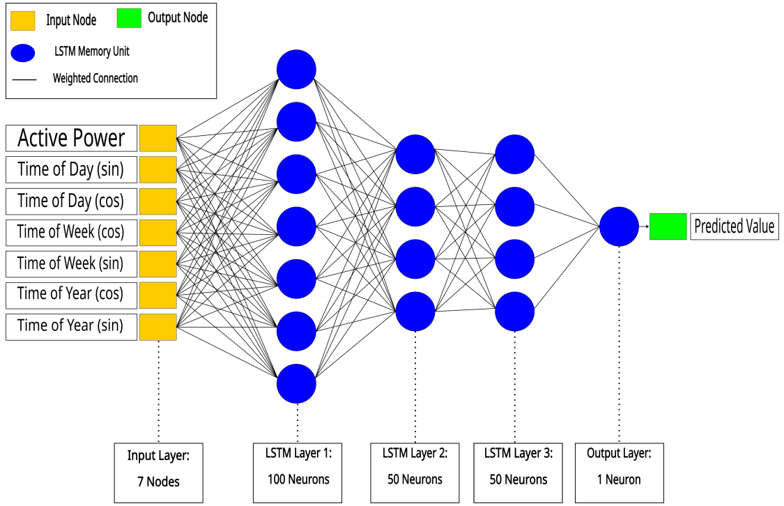
FIGURE 3.5: Outline of the stacked-LSTM neural network architecture
