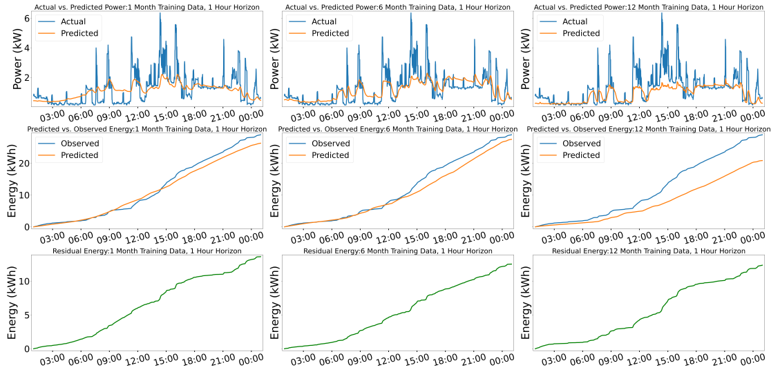
FIGURE 4.7: Comparison of predicted and observed power and energy for 1, 6 and 12-month training data sizes at a 1-hour prediction horizon
