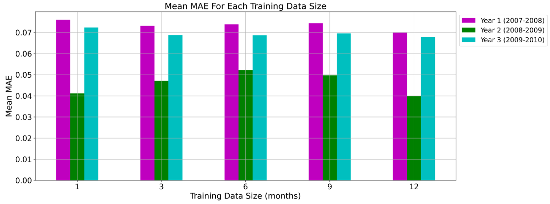
FIGURE 4.6: Comparison of mean MAEs for models of each training data size.
