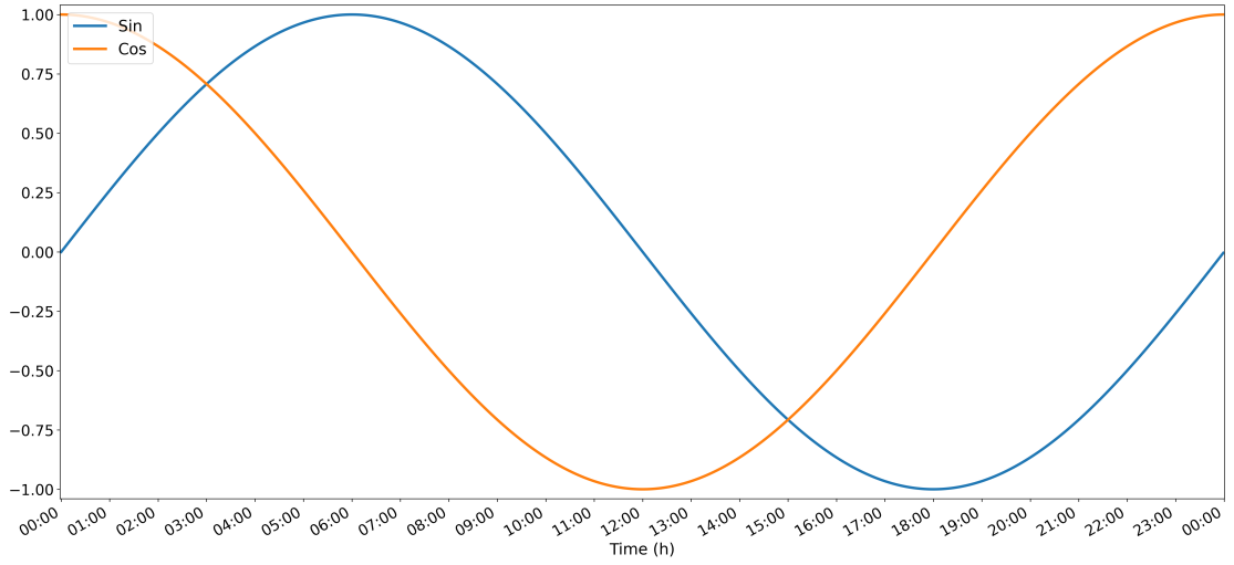
FIGURE 3.2: Encoding of timestamp labels over a 24-hour period into a numerical signal using sine and cosine transforms.
