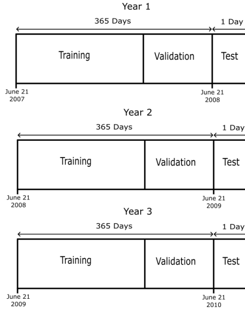
FIGURE 3.4: Test data allocations for the training-validation subsets of each year
