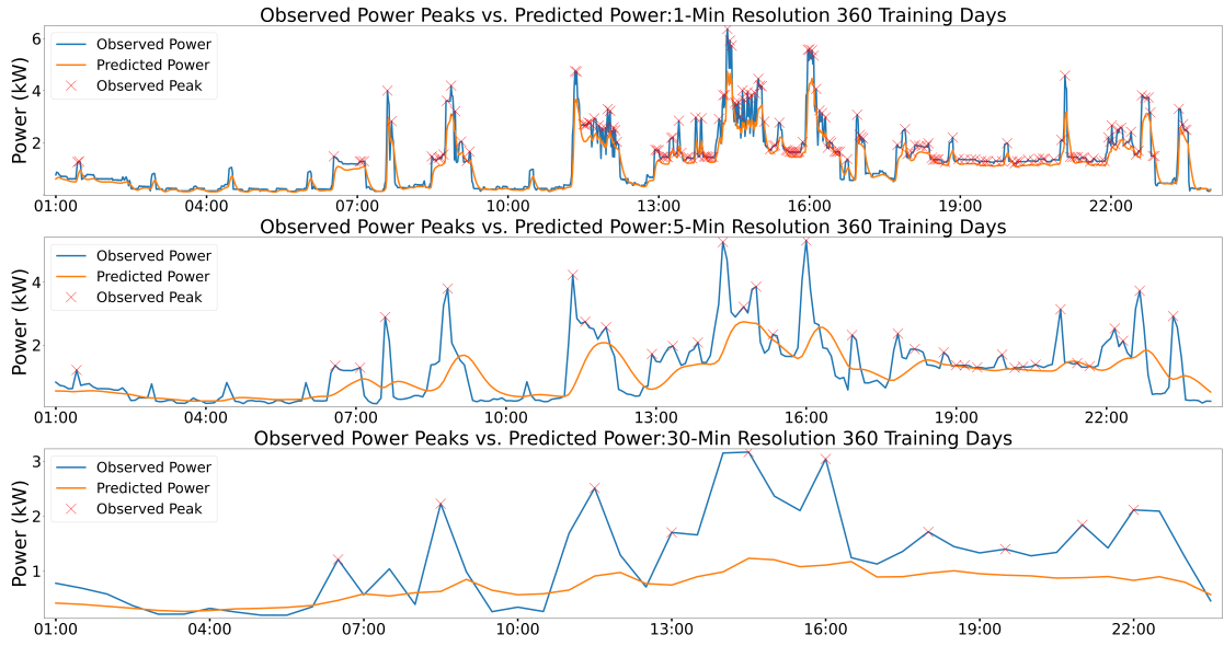
FIGURE 4.19: Comparison of the observed power peaks and predicted power for the 1, 5 and 30-minute resolution models
