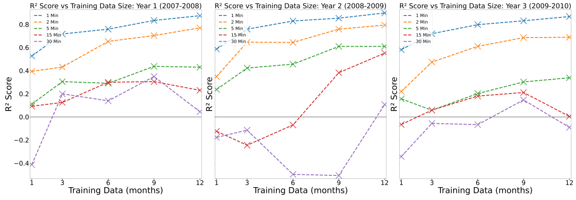
FIGURE 4.20: Comparison of R^2 scores for 1, 5, 15, and 30-minute resolution models over 3 years.
