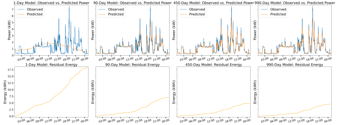
FIGURE 4.2: Comparison of predicted vs actual power and cumulative residual energy for 1, 90, 450 and 990-day prediction models.
