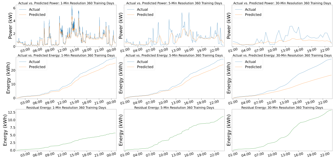
FIGURE 4.18: Comparison of predicted and observed power and energy for 1, 5 and 30-minute resolution models.
