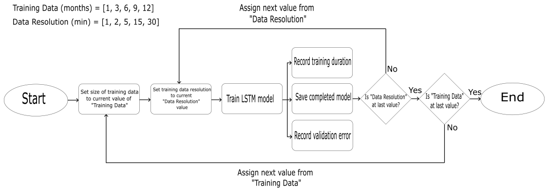
FIGURE 3.9: Flow diagram of the Experiment C algorithm
