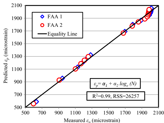
Fig. 8. Measured plastic strain versus predicted plastic strain using logarithmic model for fly ash aggregates.
