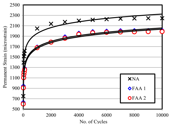
Fig. 7. Variation of permanent strain with loading cycles for different aggregates.
