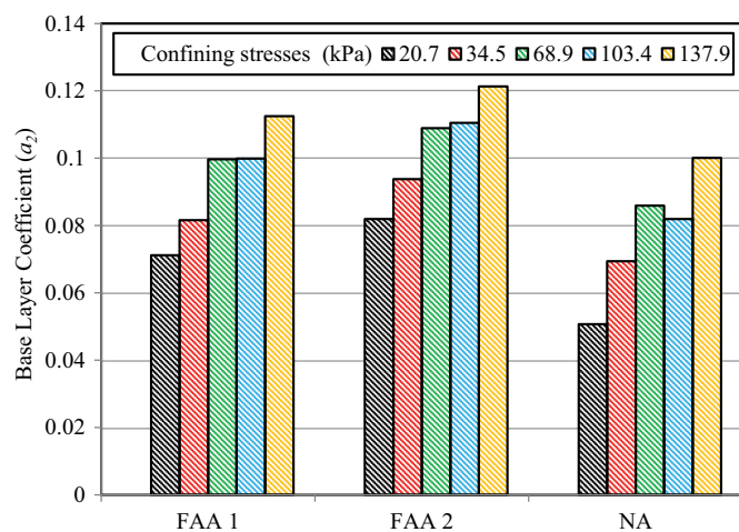
Fig. 10. Interpreted base layer structural coefficients of fly ash and natural aggregates.
