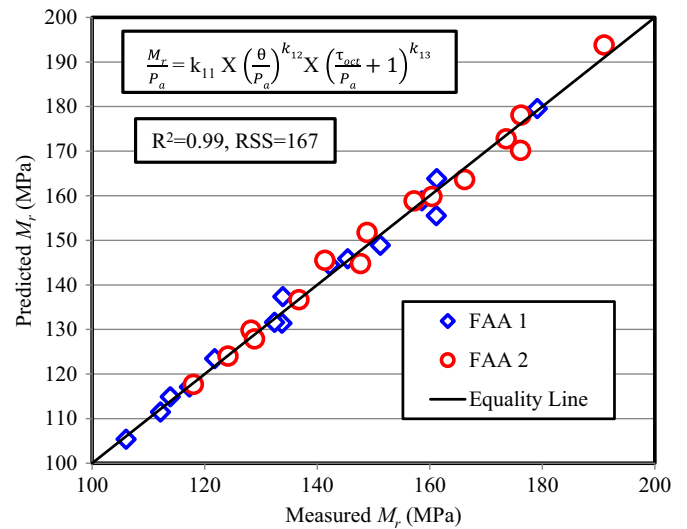
Fig. 6. Measured resilient modulus versus predicted resilient modulus using Model 5 for fly ash aggregates.
