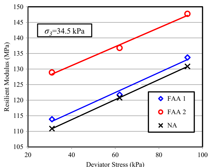
Fig. 5. Resilient modulus versus deviator stress relationship for fly ash aggregates and natural aggregates (WMM Grading) at a constant cell pressure of 34.5 kPa.
