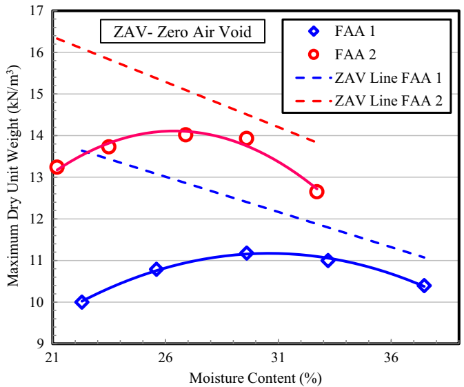
Fig. 3. Variation of maximum dry unit weight with moisture content for fly ash aggregates.
