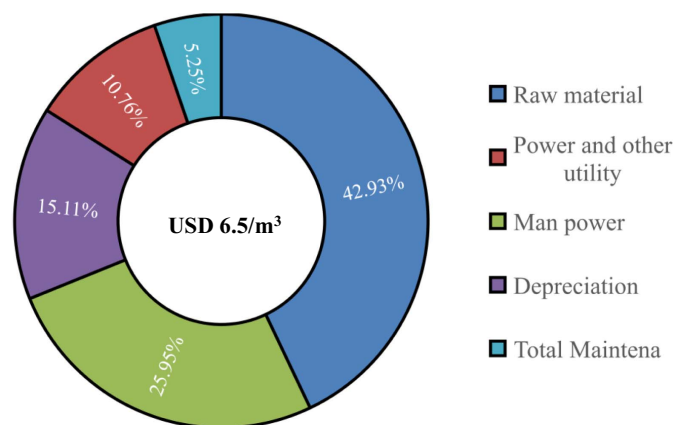
Fig. 11. Breakup of production cost for angular-shaped fly ash aggregate determined for plant capacity of 40 tons/day.
