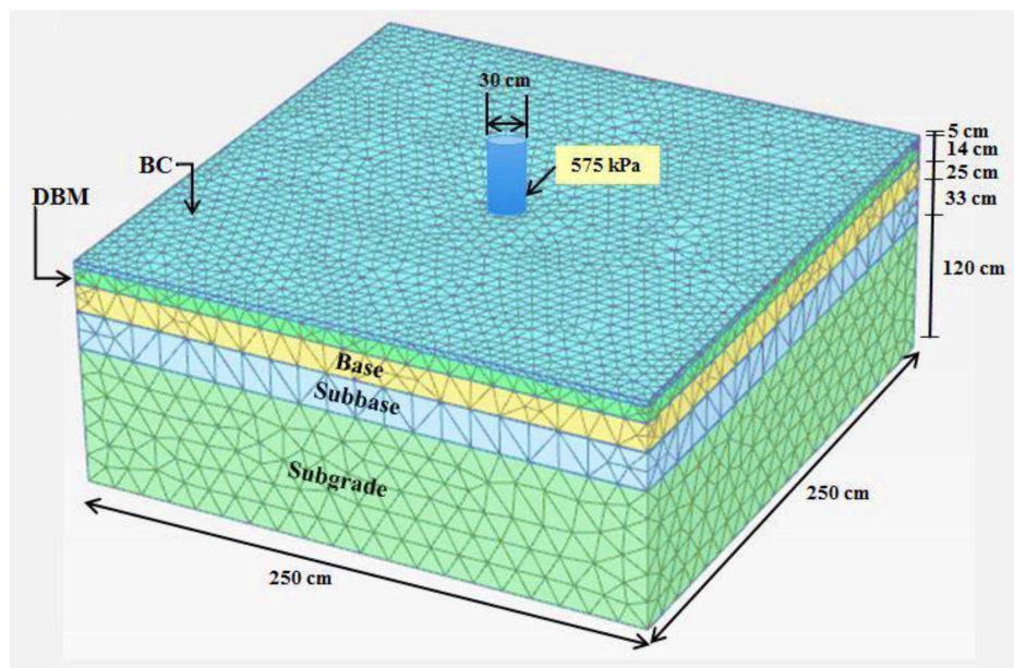
Fig. 9. Finite-element analysis of flexible pavement system using Plaxis for traffic intensity of 100 msa and subgrade CBR of 4%.
