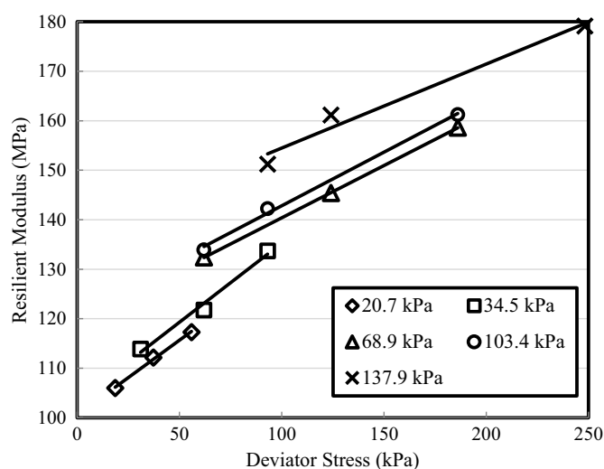
Fig. 4. Influence of deviatoric and confining stresses on resilient modulus of FAA 1.
