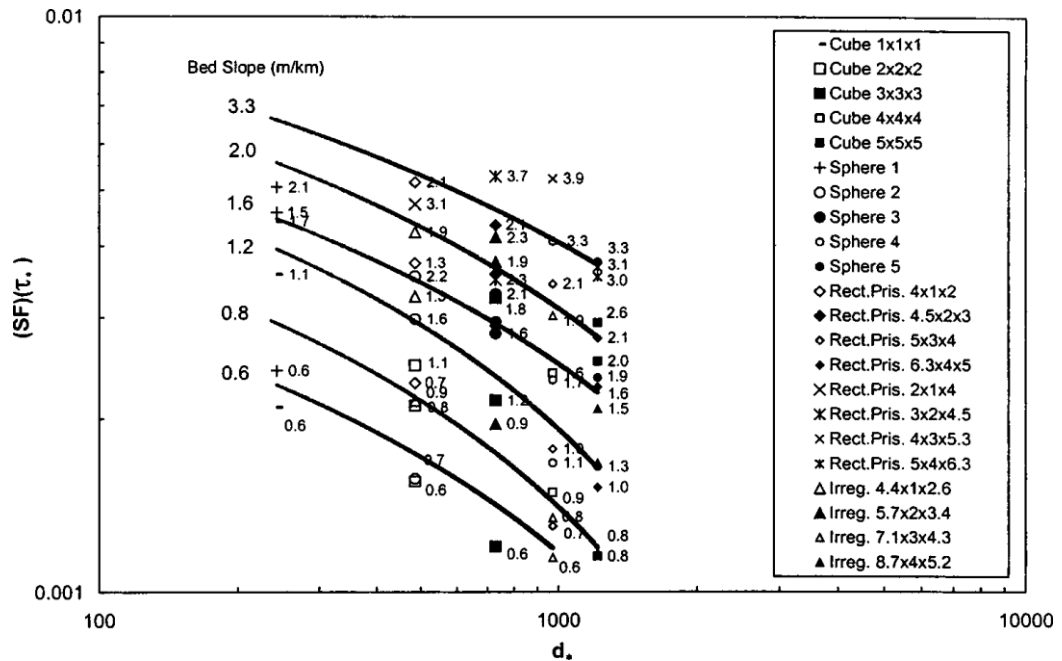
Figure 2-4: Shape Factor Correction for \tau^* versus d_* for different slopes (Gögüs and Defne 2005).
