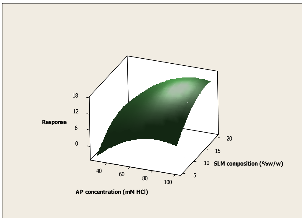
Figure 29 Surface plot of EF values of MUS versus the interrelated effect of SLM composition and AP concentration
