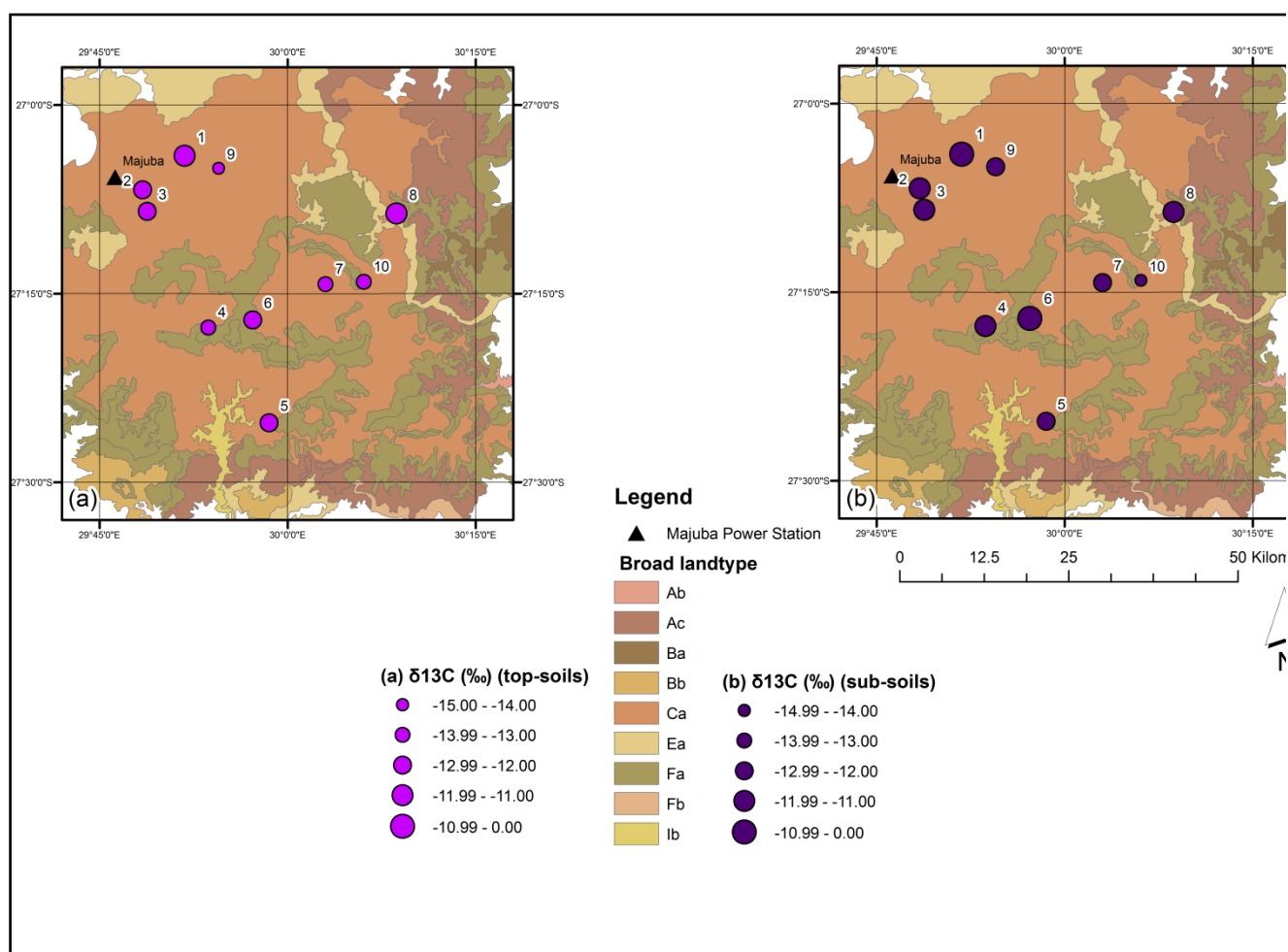
Figure 33. Map of sample sites showing spatial variation in \delta^{13}\text{C} (‰), for both soil depths combined ( n = 59 ) for Majuba soils.
