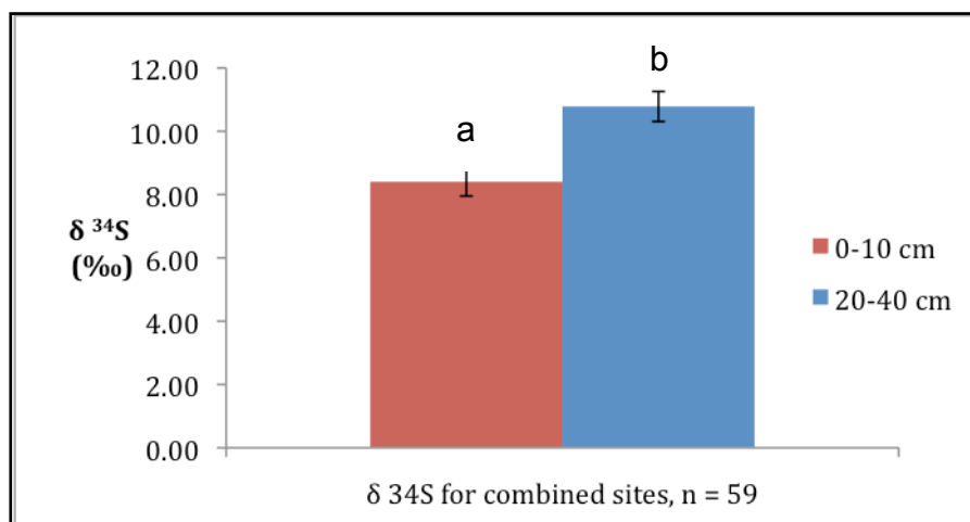
Figure 16. Mean \pm standard error \delta^{34}\text{S} ‰ values for Majuba soils for all ten sites, representing top ( n = 30 ) and sub ( n = 29 ) soil depths. Means associated with different letters are statistically different ( p \leq 0.05 ).
