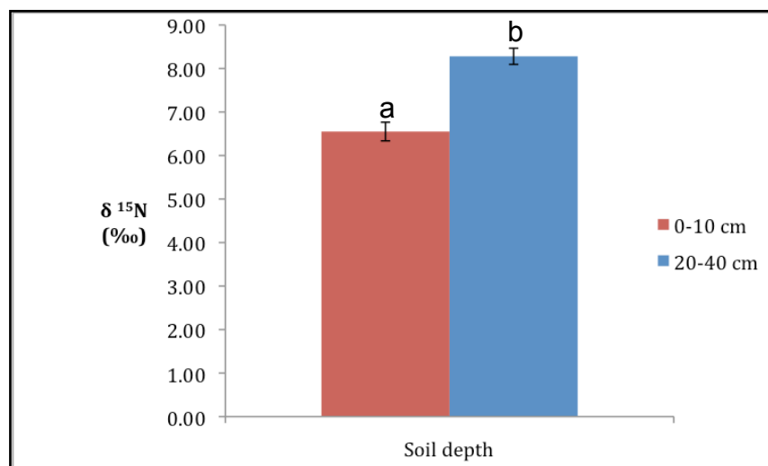
Figure 23. Mean \pm standard error \delta^{15}\text{N} ‰ values for Majuba soils for all ten sites, representing top ( n = 30 ) and sub ( n = 29 ) soil depths. Means associated with different letters are statistically different ( p \leq 0.05 ).
