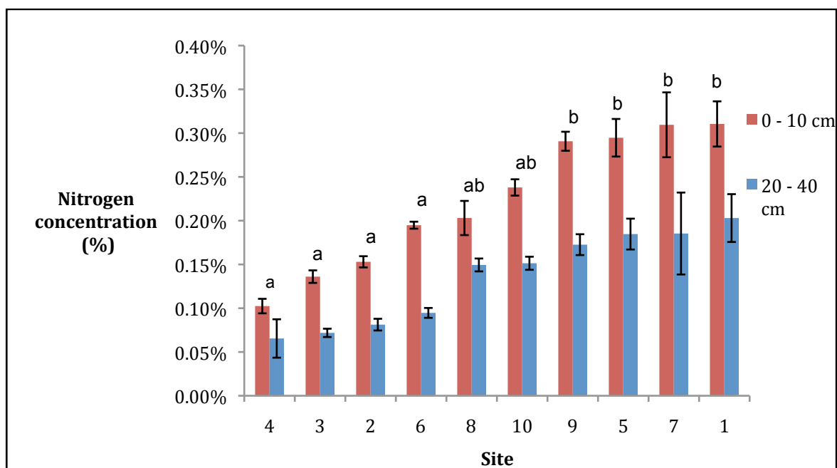
Figure 21. Nitrogen concentration (%) found in the Majuba soils across the two soil depths (0-10 cm and 20-40 cm) and the 10 sites sampled. Means associated with the different letters are significantly different ( p \leq 0.05 ).
