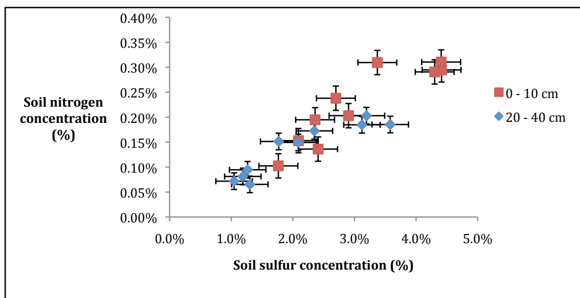
Figure 37. Graph showing mean soil N concentration versus mean S concentration for both top-soils ( r^2 = 0.814 ) and sub-soil depths ( r^2 = 0.851 ) for Majuba soils.
