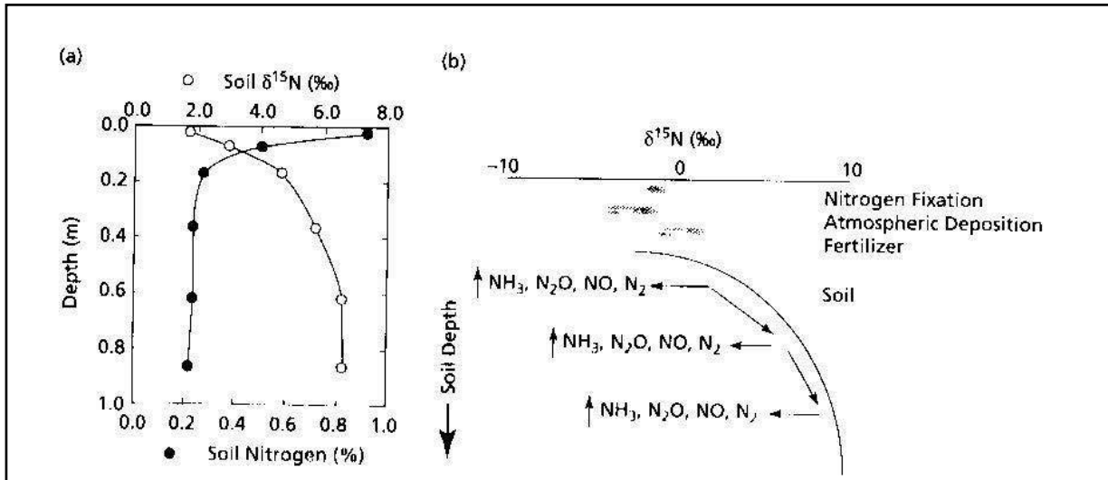
Figure 4 (Left panel) Soil \delta^{15}\text{N} and nitrogen content of a typical soil profile (from Sperry et al. , 2006). Closed symbols are soil nitrogen content and open symbols are soil \delta^{15}\text{N} . (Right panel) Conceptual model based on Nadelhoffer & Fry (1988, 1994) proposing the mechanisms for the increase in soil \delta^{15}\text{N} with depth. Horizontal arrows represent mineralization and nitrification; vertical arrows represent gaseous nitrogen loss. Fractionation during each transformation causes the remaining soil nitrogen to become progressively enriched in ^{15}\text{N} as nitrogen moves down the soil profile.
