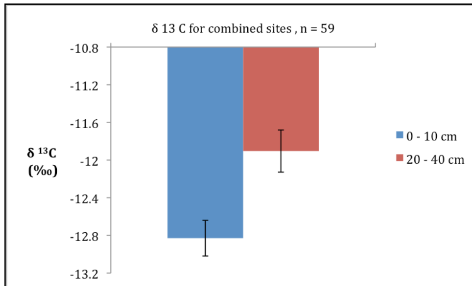
Figure 31. Mean \pm standard error \delta^{13}\text{C} ‰ values for Majuba soils for all ten sites, representing top ( n = 30 ) and sub ( n = 29 ) soil depths ( p \leq 0.05 ).
