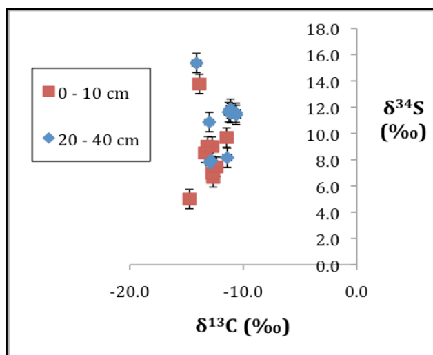
Figure 39. Graph showing mean soil \delta^{34}\text{S} signal versus mean soil \delta^{13}\text{C} signal for both top-soils ( r^2 = 0.007 ) and sub-soil depths ( r^2 = 0.006 ) for Majuba soils.
