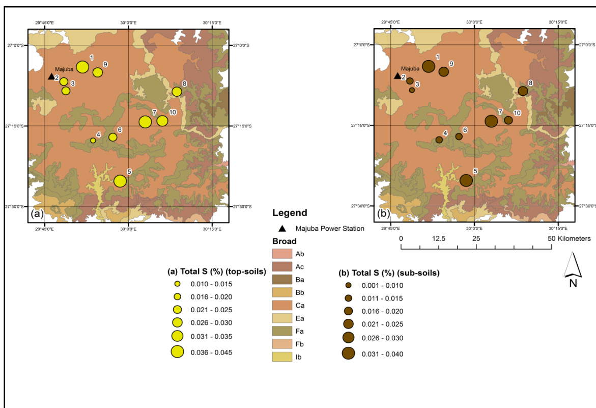
Figure 15 Map of sample sites showing spatial variation in percentage soil S, showing both top-soil (n = 29) and sub - soil depths (n = 30) for Majuba soils.
