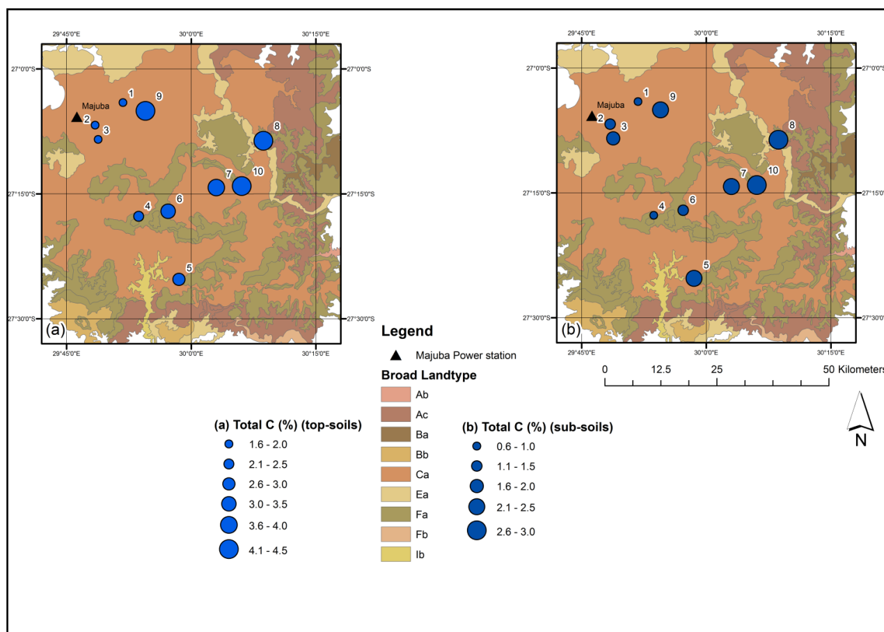
Figure 30. Map of sample sites showing spatial variation in C concentration (%), showing both top-soil (n = 29) and sub-soils (n = 30) for Majuba soils.
