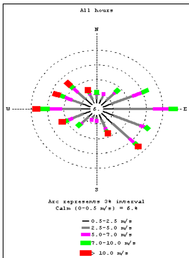
Figure 9. Wind rose for all hours. Data collected from Majuba 1 air quality monitoring station during the period 2000 –
