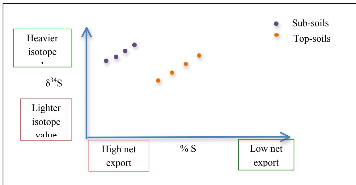
Figure 43. Conceptual diagram illustrating the correlation between \delta^{34}\text{S} and % S in the top-soil and sub-soil depth.
