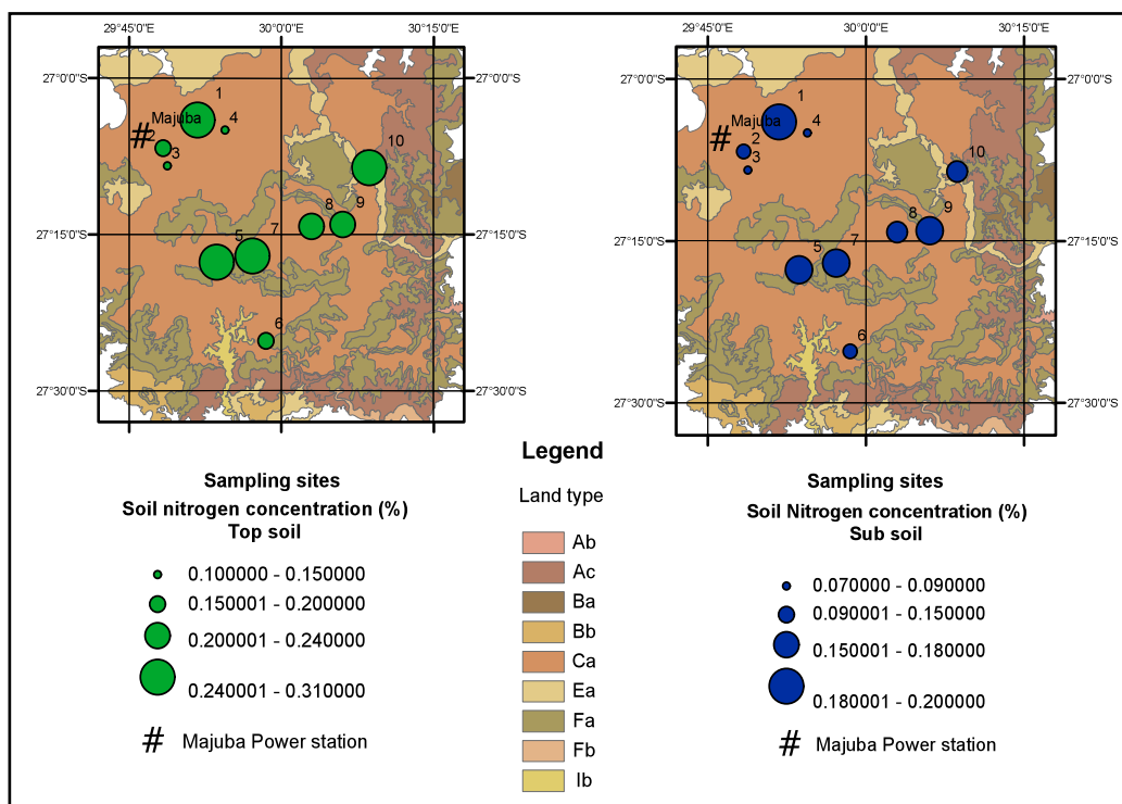
Figure 22. Map of sample sites showing spatial variation (significant interaction between site and depth, F = 2.26 , p = 0.0382 ) in percentage soil N, for top-soil ( n = 30 ) and sub-soil ( n = 29 ) depths for Majuba soils.
