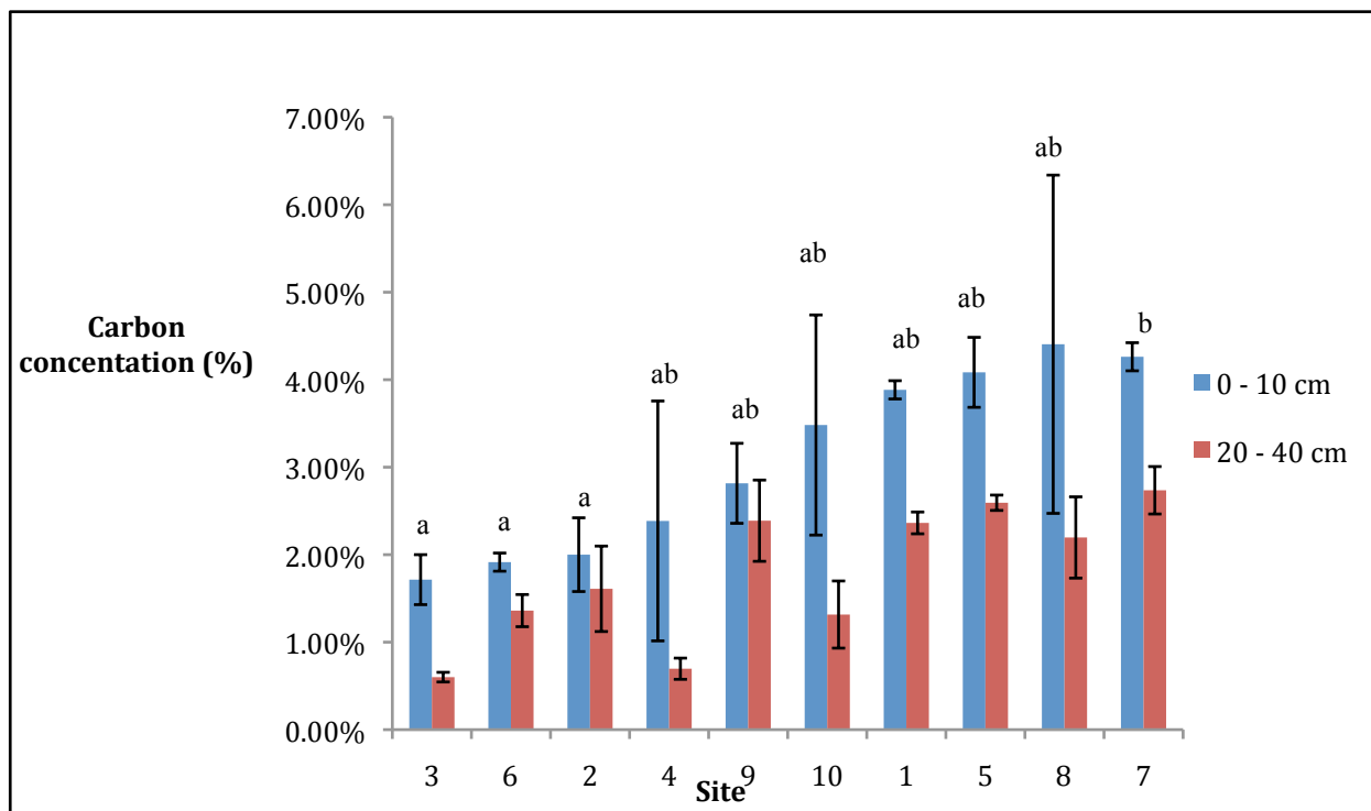
Figure 29. Mean \pm standard error soil C concentration (%) values for Majuba soils, for both top-soils ( n = 30 ) and sub-soils ( n = 29 ), across the ten sampled sites. means associated with a different letter are significantly different ( p \leq 0.05 ).
