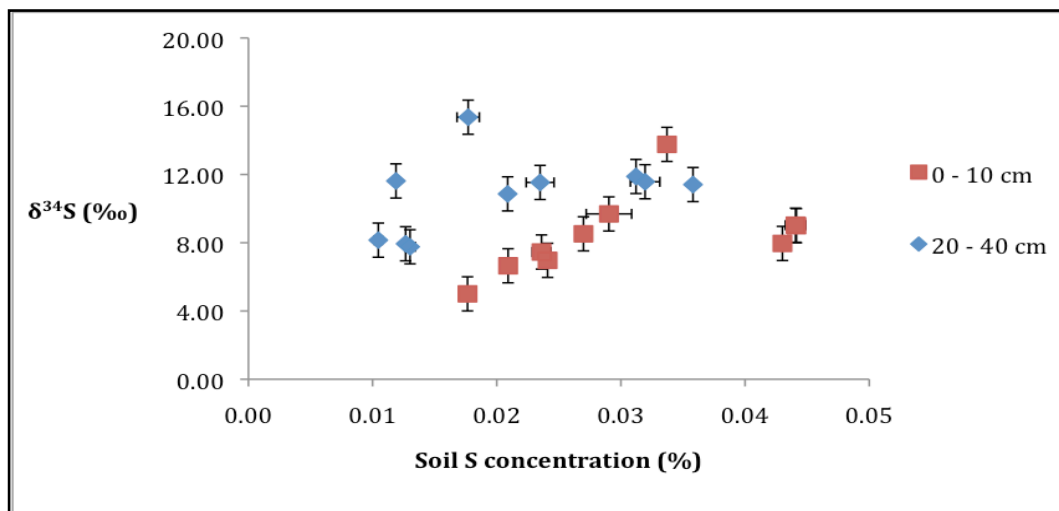
Figure 19. Graph showing mean soil \delta^{34}\text{S} (‰) signal versus mean S concentration for both top-soils ( r^2 = 0.237 ) and sub-soil depths ( r^2 = 0.183 ) for Majuba soils.
