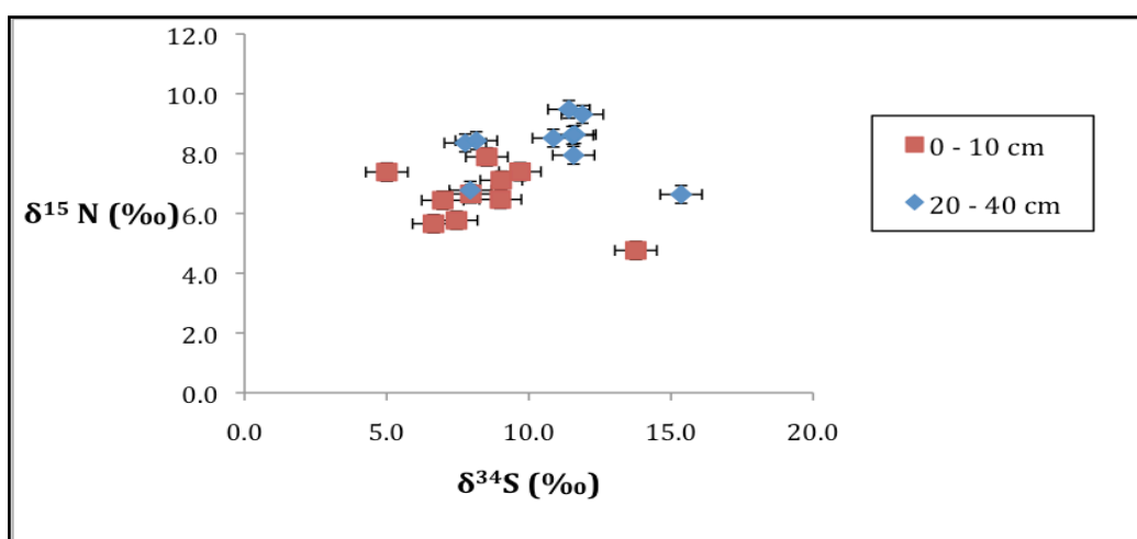
Figure 40. Graph showing mean soil \delta^{15}\text{N} signal versus mean soil \delta^{34}\text{S} signal for both top-soils ( r^2 = 0.178 ) and sub-soil depths ( r^2 = 0.007 ) for Majuba soils
