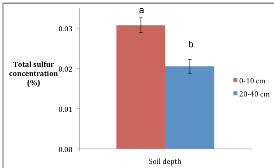
Figure 13. Mean percentage soil S concentration ( \pm standard error) found in the Majuba soils for all 10 sites, representing both top ( n = 30 ) and sub-soil ( n = 29 ) depths. Means associated with different letters are statistically different ( p \leq 0.05 ).
