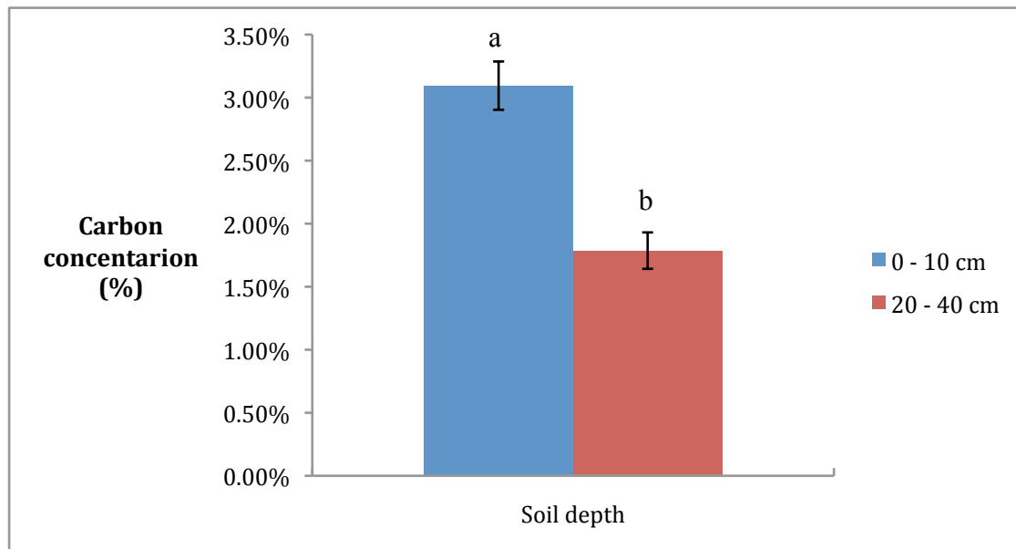
Figure 28. Mean percentage soil C concentration ( \pm standard error) found in the Majuba soils for all 10 sites, representing both top ( n = 30 ) and sub-soil ( n = 29 ) depths. Means associated with different letters are statistically different ( p \leq 0.05 ).
