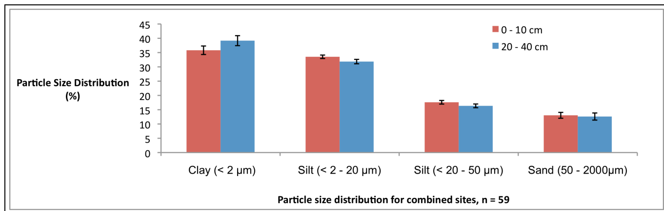
Figure 41. Graph showing particle size distribution for all 10 sites combined, indicating both top-soil (n = 29) and sub-soil (n = 30) depth for Majuba soils.
