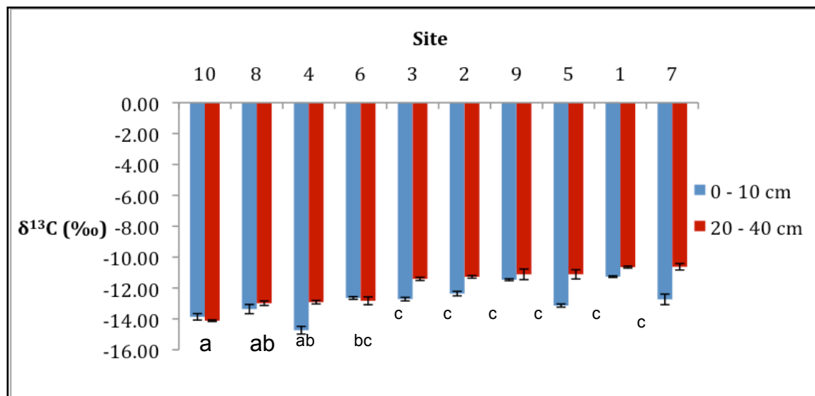
Figure 32. Mean \pm standard error \delta^{13}\text{C} (‰) values for Majuba soils, for both top-soils ( n = 30 ) and sub-soils ( n = 29 ), across the ten sampled sites. Means associated with a different letter are significantly different ( p \leq 0.05 ).
