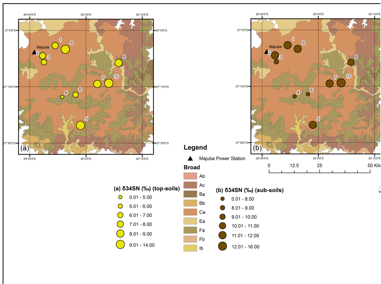
Figure 18. Map of sample sites showing spatial variation in the mean \delta^{34}\text{S} (‰) signal, showing both top-soil ( n = 29 ) and sub-soil depths ( n = 30 ) for Majuba soils.
