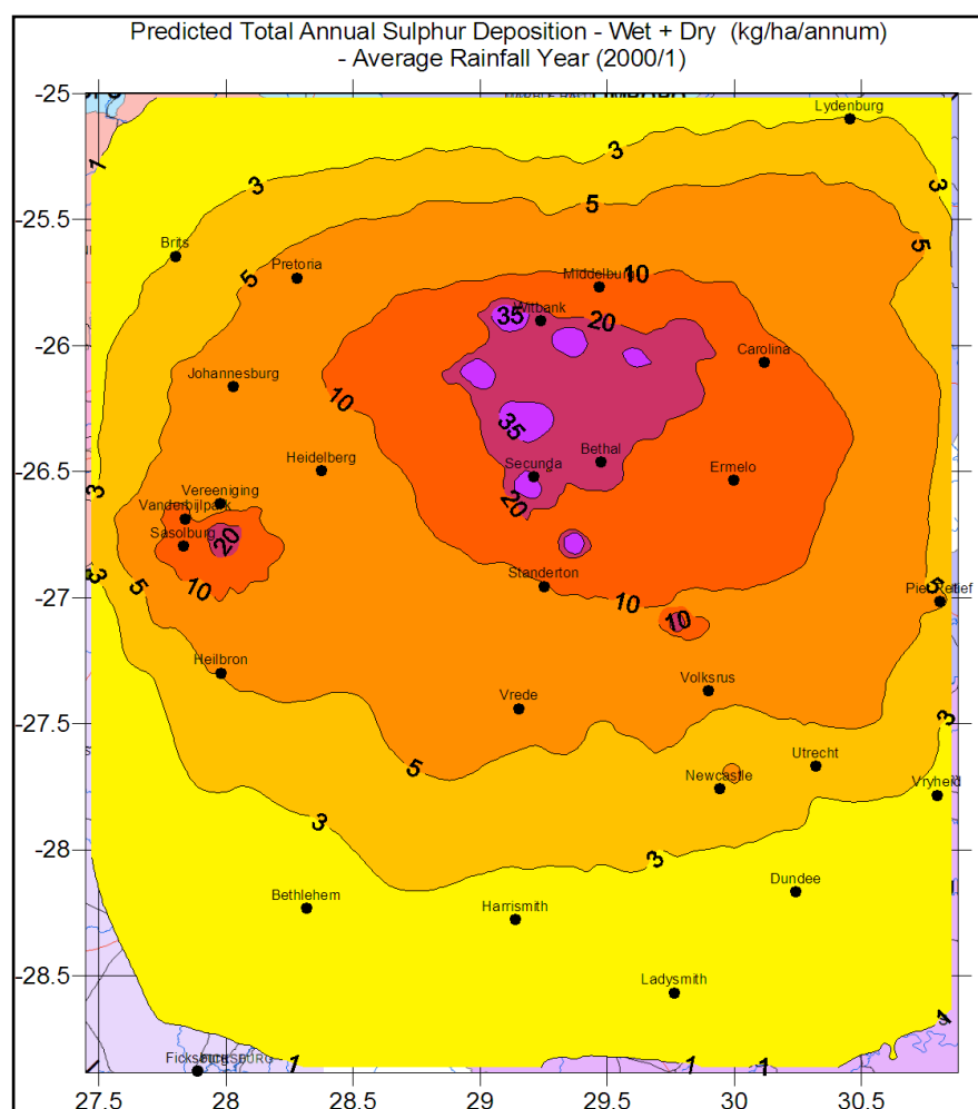
Figure 11. Predicted total annual S deposition for average rainfall year \text{kg} \cdot \text{ha}^{-1} \cdot \text{yr}^{-1} (2000/1).
