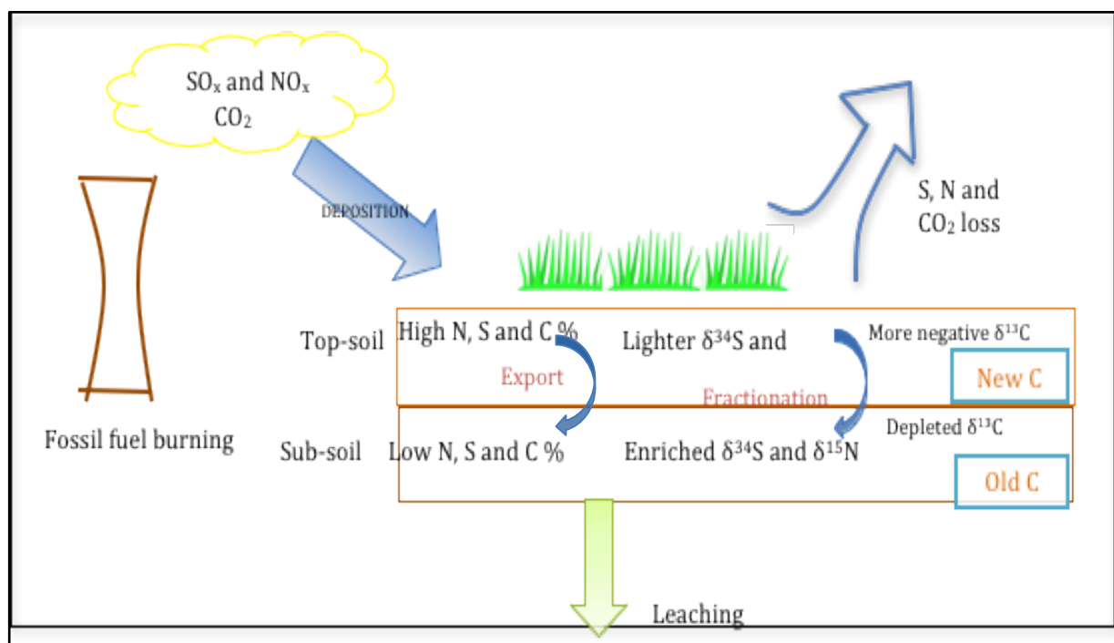
Figure 42. Schematic diagram illustrating the pathway of S, N and C from the atmosphere to the soil system.
