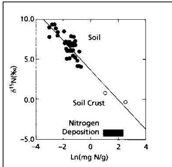
Figure 5. Relationship between soil \delta^{15}N and Ln. (soil nitrogen content) in soils and in two potential sources of N in cold dessert ecosystems (Evans and Ehleringer, 1993).
