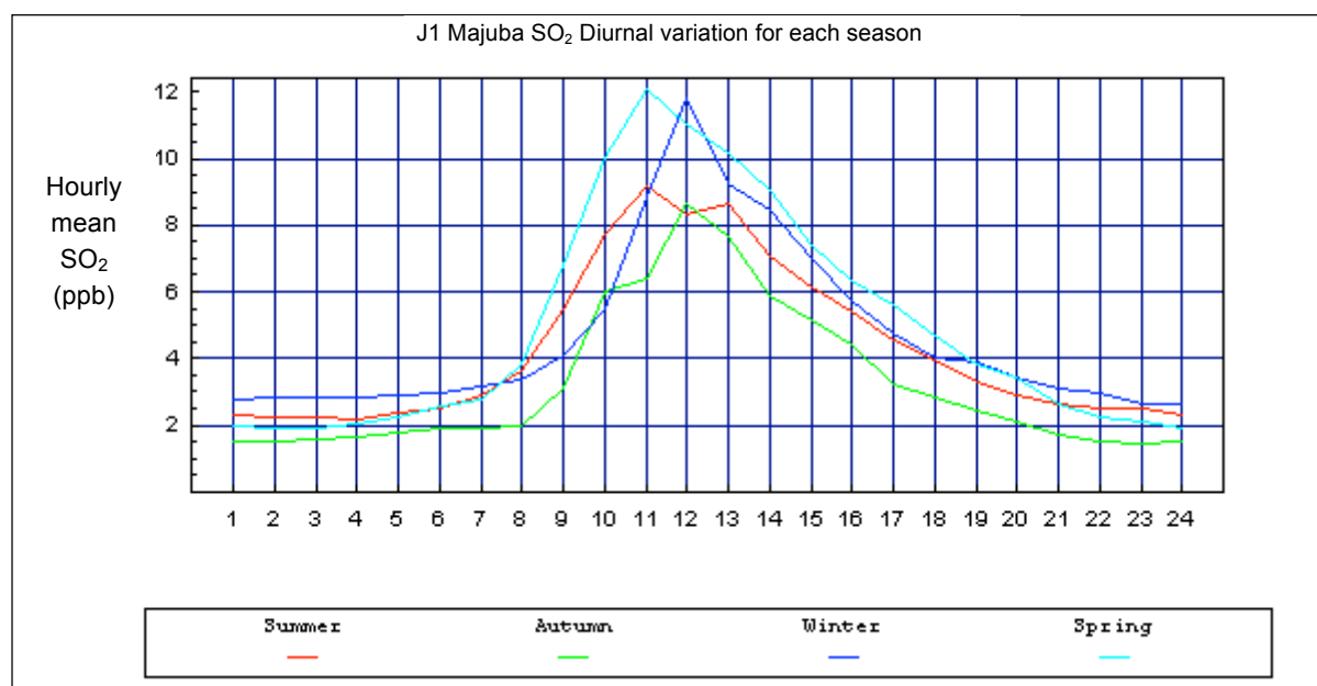
Figure 10. Variance in the hourly mean SO 2 concentration (ppb) with season, taken from the Majuba 1 air quality control station during the period 1995 - 2000.
