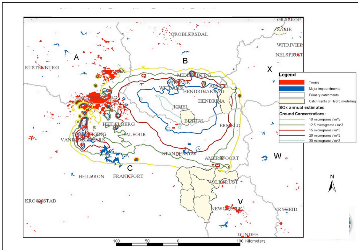
Figure 7. Map showing estimated annual SO x ground level concentrations across the Mpumalanga and Gauteng area
