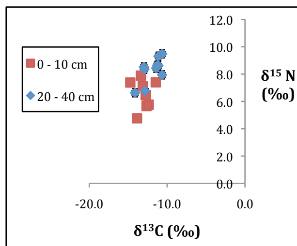
Figure 38: Graph showing mean soil \delta^{15}\text{N} signal versus mean soil \delta^{13}\text{C} signal for both top-soils ( r^2 = 1 \times 10^{-5} ) and sub-soil depths.
