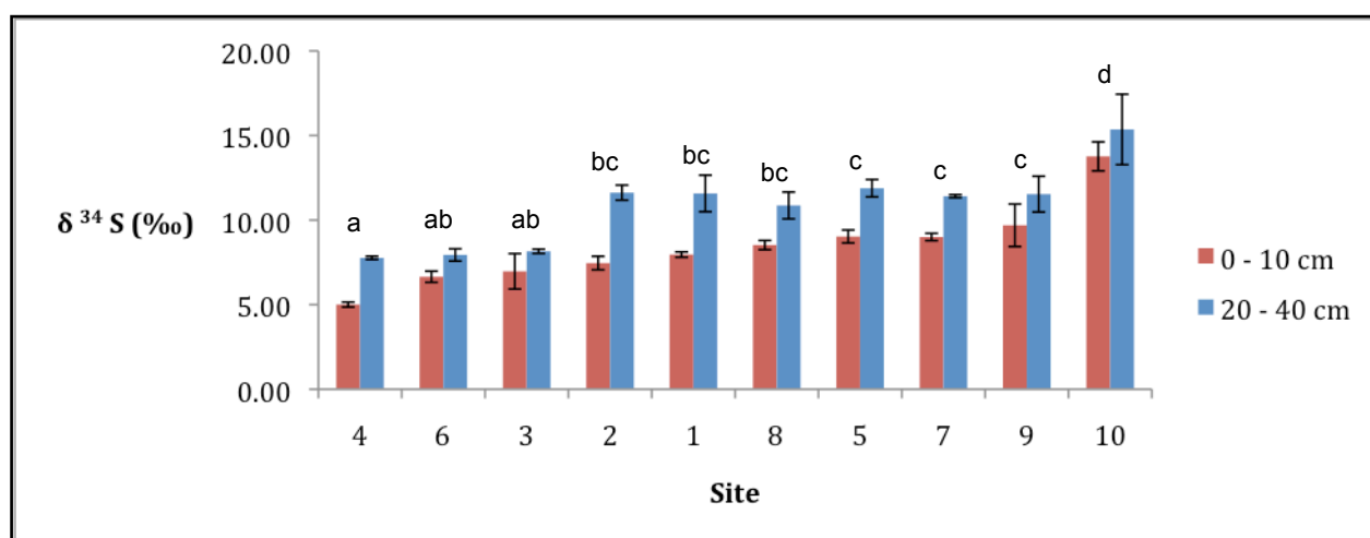
Figure 17. Mean \pm standard error \delta^{34}\text{S} (‰) values for Majuba soils, for both top-soils ( n = 30 ) and sub-soils ( n = 29 ), across the ten sampled sites. Means associated with a different letter are significantly different ( p \leq 0.05 ).
