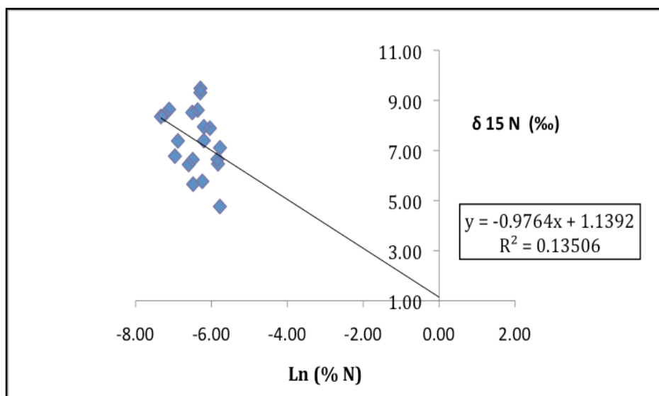
Figure 27 Graph showing mean soil \delta^{15}\text{N} versus natural log mean N concentration for the pooled data for Majuba soils.
