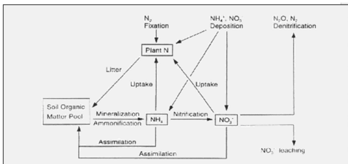
Figure 2: Nitrogen transformations and processes affecting \delta^{15}\text{N} values in forest ecosystems (Nadelhoffer and Fry, 1994).
