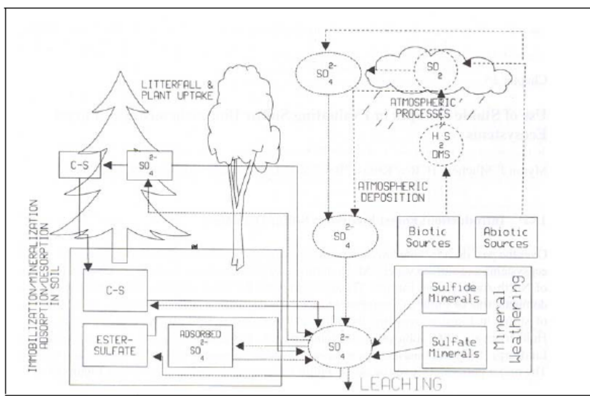
Figure 1: Schematic representation of the S cycle affecting S isotope composition (Mitchell et al. , 1998).
