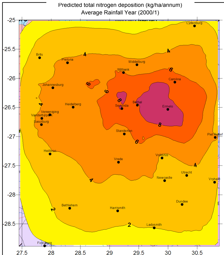
Figure 12. Predicted total N deposition for an average rainfall year \text{kg} \cdot \text{ha}^{-1} \cdot \text{yr}^{-1} (2000/1).
