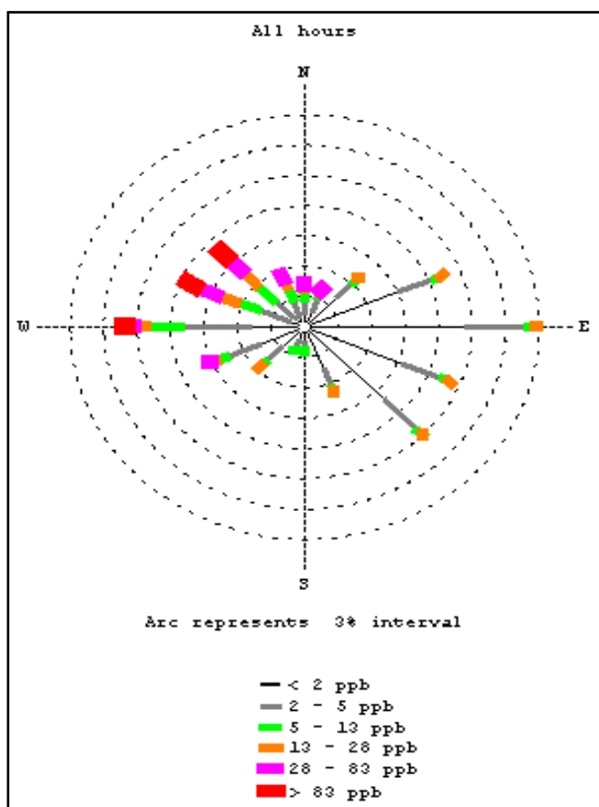
Figure 8. Sulfur dioxide pollution rose for all hours. Data collected from Majuba 1 air quality monitoring station during the period 2000 – 2005.
