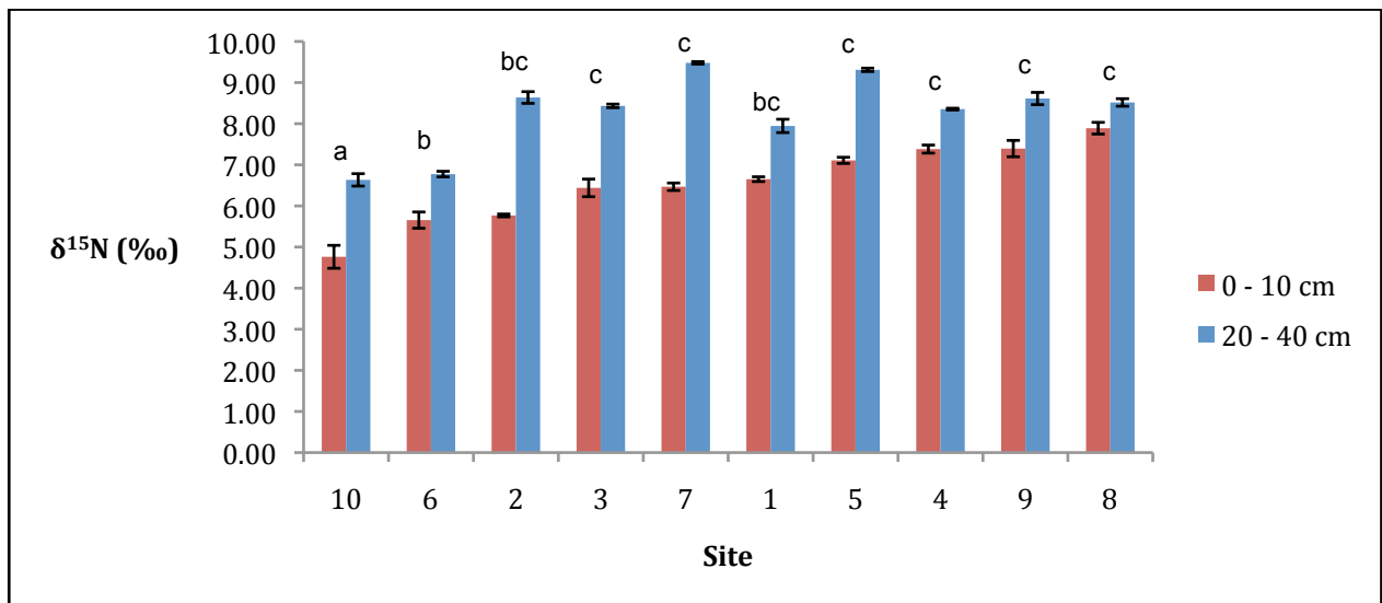
Figure 24. Mean \pm standard error \delta^{15}\text{N} (‰) values for Majuba soils, for both top-soils ( n = 30 ) and sub-soils ( n = 29 ), across the ten sampled sites. Means associated with a different letter are significantly different ( p \leq 0.05 ).
