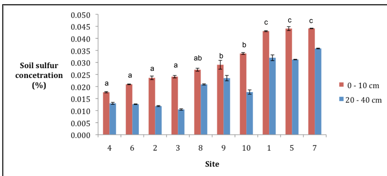
Figure 14. Soil S concentration found in the Majuba soils across the two soil depths and the 10 sites sampled. Means associated with the different letters are significantly different ( p \leq 0.05 ).
