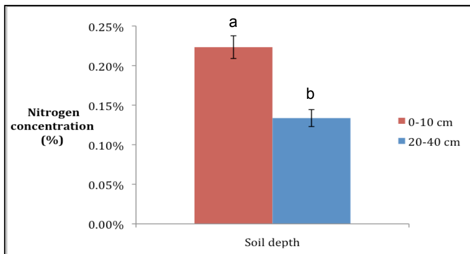
Figure 20. Mean percentage soil N values ( \pm standard error) for all sites, representing both top-soil ( n = 30 ) and sub-soil ( n = 29 ) depths. Means associated with different letters are statistically different ( p \leq 0.05 ).
