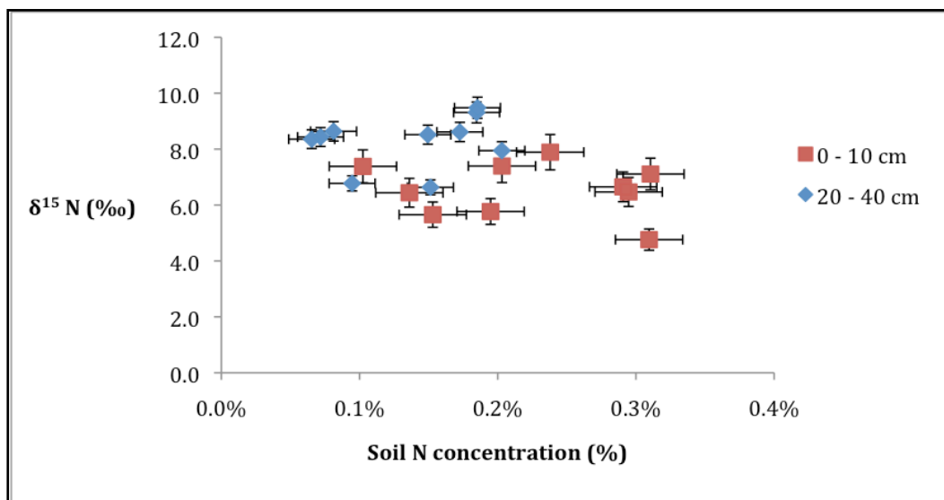
Figure 26. Graph showing mean soil \delta^{15}\text{N} signal versus mean N concentration for both top-soils ( r^2 = 0.026 ) and sub-soil depths ( r^2 = 0.055 ) for Majuba soils.
