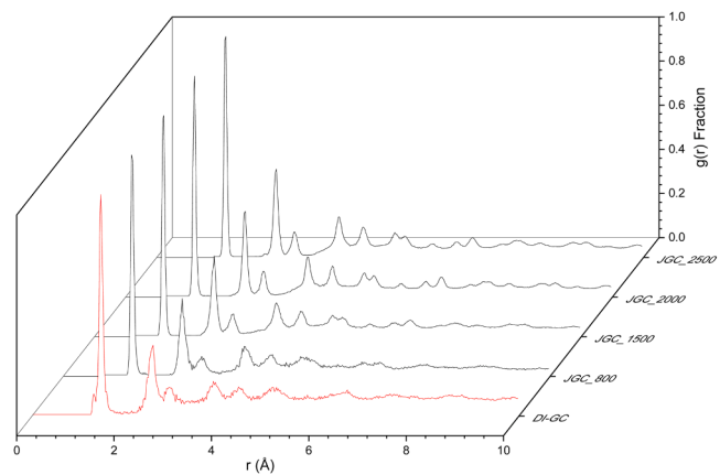
Fig. 10. Radial distribution function of DI-GC (red) and JGC models (black) across the formation temperatures of 800 °C - 2500 °C.
