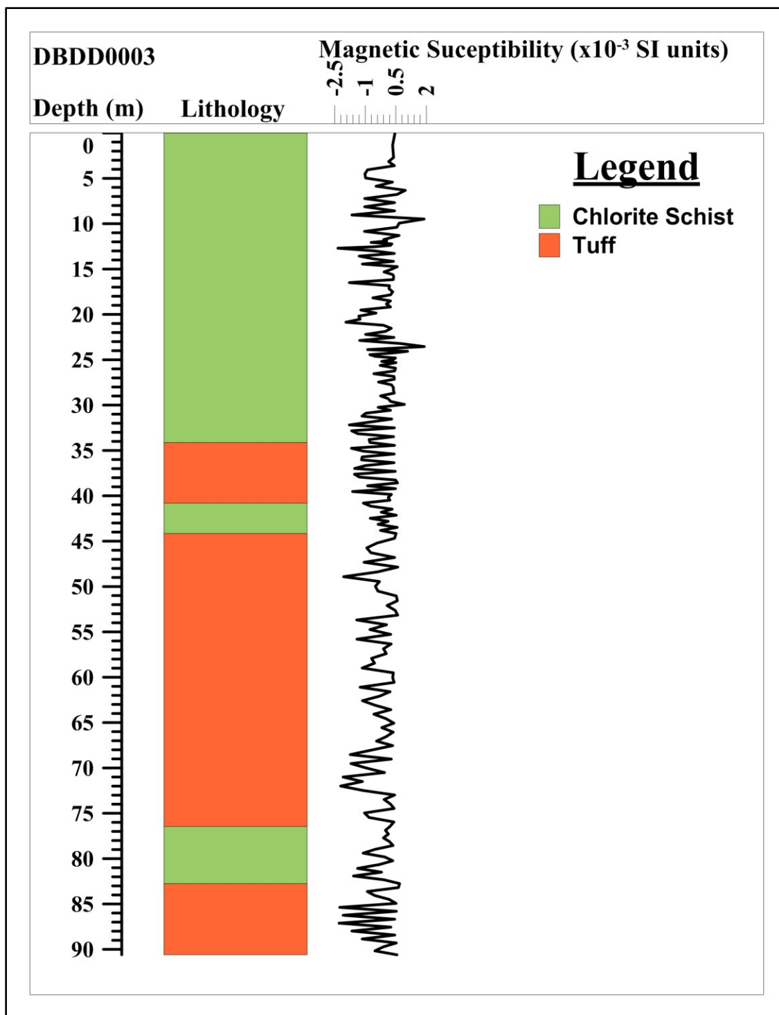
Figure 7.11 Magnetic susceptibility log for drill hole DBDD0003 showing low values.
