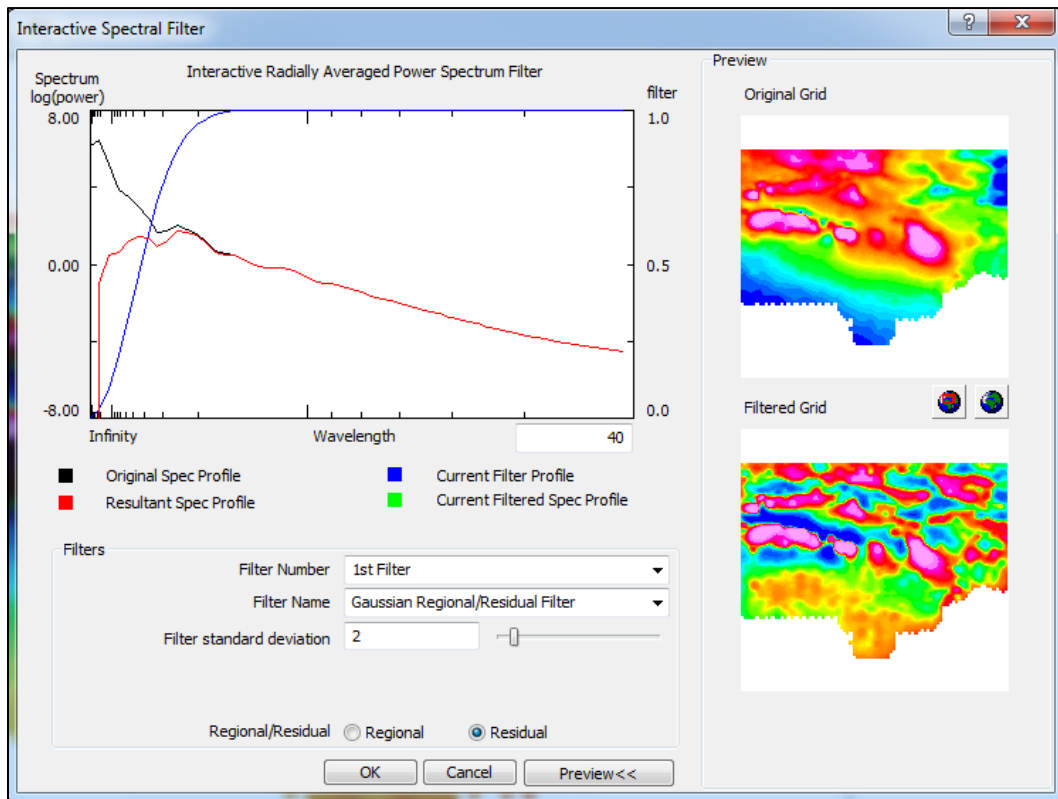
Figure 7.52 Residual filter spectral analysis of the TMI of the Deblin Copper Mine area. Cut-off frequency is 2.0.
