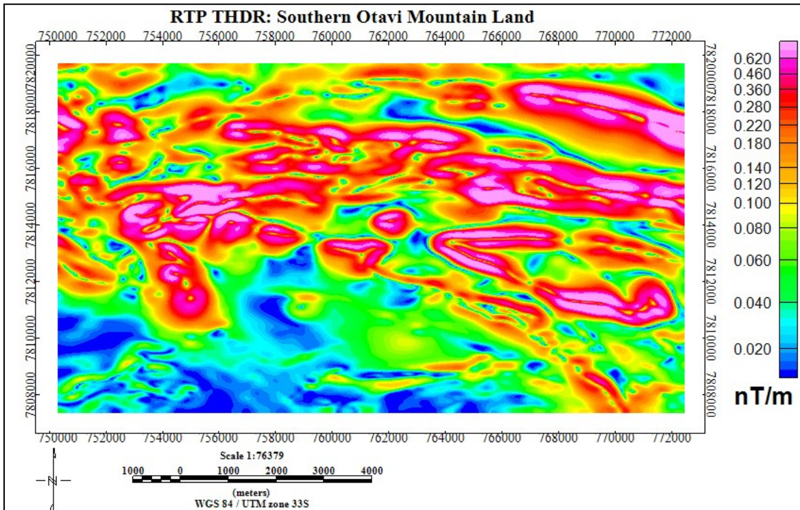
Figure 7.21 Processed THDR showing the edges of the magnetic bodies.
