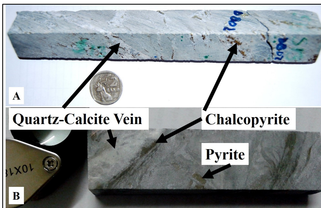
Figure 4.8 Drill core images of silicified dolomite showing vein type mineralization. A) Quartz-calcite vein-hosted chalcopyrite mineralization. DBDD0002: 84.00 m - 84.20 m - DB2S12. B) Convolute chalcopyrite and pyrite bands, discrete euhedral pyrite grains in the matrix and a fabric-parallel quartz-calcite vein with chalcopyrite mineralization along the margin of the vein. DBDD0002: 72.62 m - 72.82 m - DB2S11.
