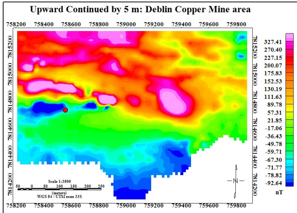
Figure 7.47 The Total Magnetic Intensity (TMI) data upward continued by 5 m. Notice how the TMI data is smoothed. The red dot represents the location of the Deblin Copper Mine shaft.
