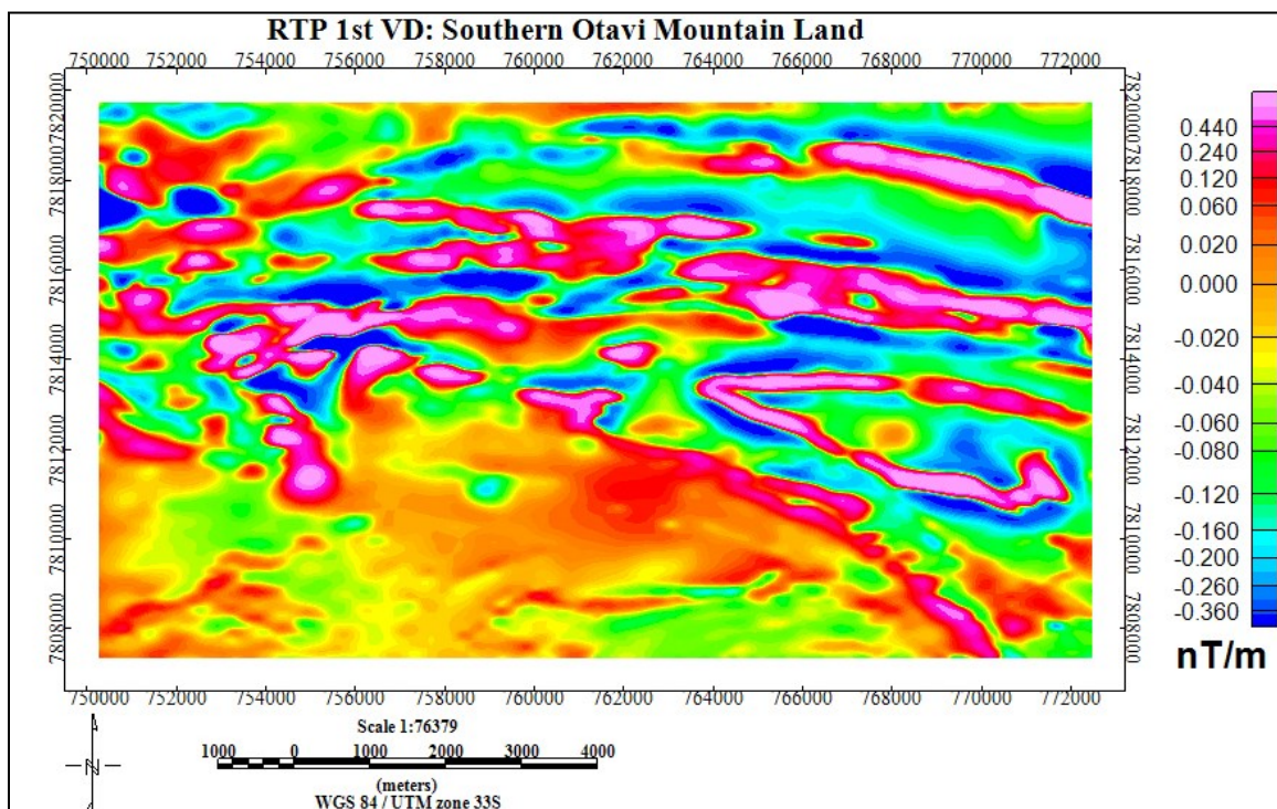
Figure 7.19 1 st VD map with enhanced shallow structures. Note the presence of high frequency noise.
