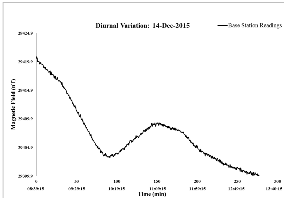
Figure 7.36 Diurnal variation plot for day 4. The Julian day is 348. The survey lasted for 277 minutes.
