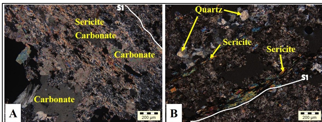
Figure 3.27 Sericite in the silicified dolomite and mineral overgrowths. A) Foliation, S 1 made up of largely sericite (XPL). Additional observations show carbonate overgrowth over sericite in the cleavage domain. DBDD0002: 73.40 m – 73.60 m – DB2S12-D14c. B) Fine-grained quartz in the quartz-calcite vein and minor distinct sericite cleavage domains (XPL). DBDD0001: 82.59 m – 82.59 m – DB1S11-D4b.
