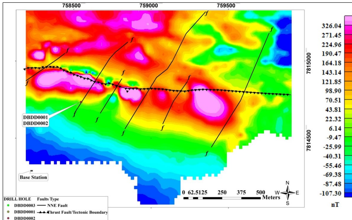
Figure 7.55 Interpreted RTP map showing the magnetic response of the rocks from the Deblin Copper Mine area and positions of the major thrust fault and northeast-oriented faults.
