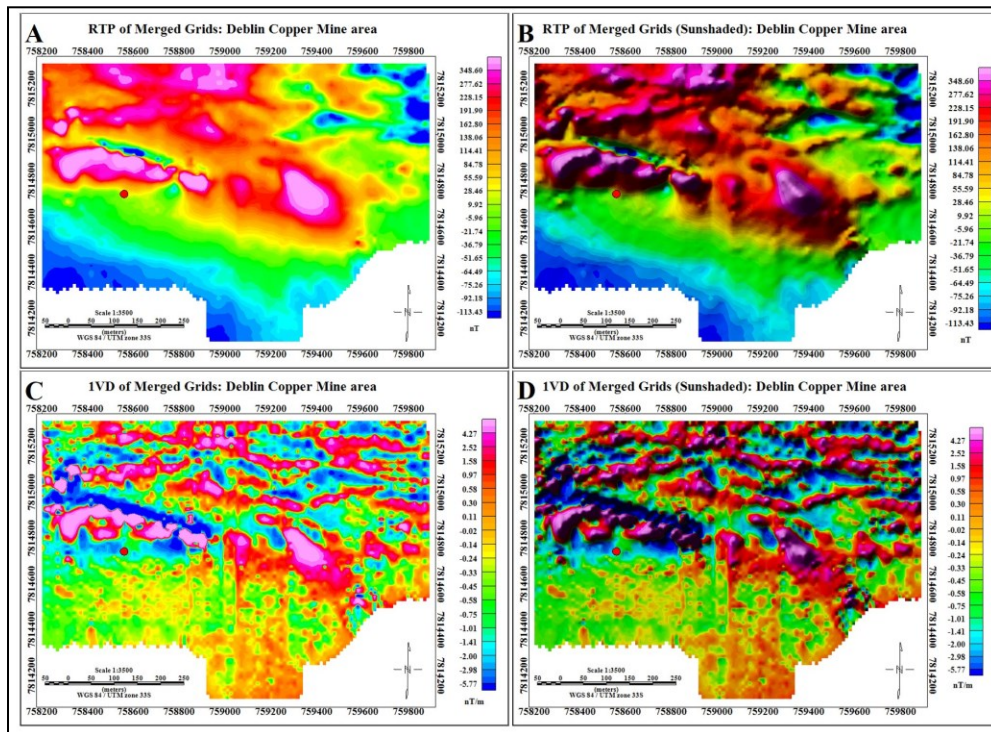
Figure 7.45 Reduced to Pole (RTP) and first vertical derivative (1 st VD) maps of the merged grids with line noise, which is obvious in the sunshaded maps. The red spot in the images represent the Deblin Mine shaft. The inclination and declination for the shaded images are 45° and 45°, respectively.
