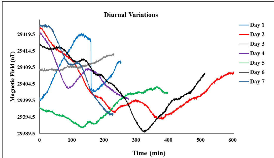
Figure 7.40 Plots for diurnal variations for all the days.
