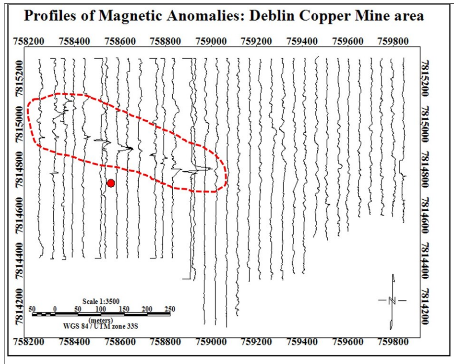
Figure 7.42 2D presentation of magnetic profiles of the 34 infill survey lines. The red dotted line represents the area with a trend of positive anomalies, whereas the red dot represents the location of the Deblin Copper Mine shaft. The trend of the anomalies indicate the strike of magnetic units.
