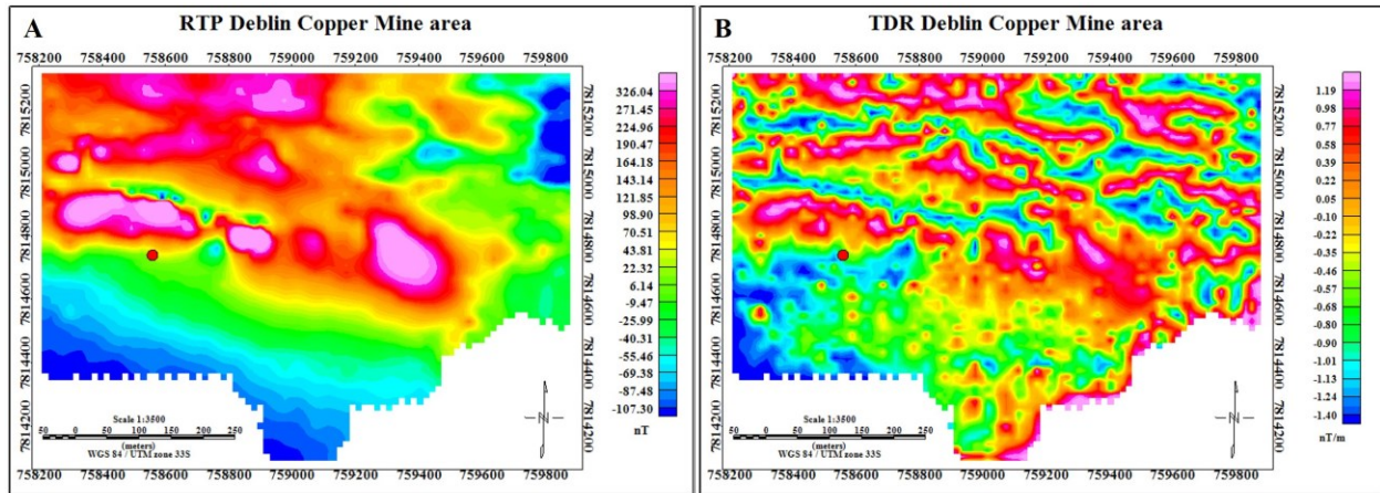
Figure 7.50 The application of the tilt derivative to the ground magnetic of the Deblin Copper Mine area. A) Reduced to Pole (RTP) map and B) the tilt horizontal derivative (TDR) which clearly maps shallow linear structures.
