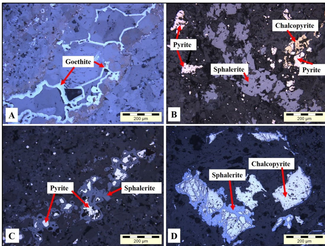
Figure 4.12 Reflected light photomicrographs showing the sphalerite texture and replacements. A) Goethite with colloform texture along the margins of quartz-calcite veins. DBDD0001: 46.80 m – 47 m – DB1S6-D47f (dolomite breccia). B) Sphalerite replacing both pyrite and chalcopyrite, whereas chalcopyrite is replacing pyrite. DBDD0001: 60.70 m – 60.88 m – DB1S9-D50c (dolomite breccia). C) Pyrite enclosed in sphalerite as a consequence of pyrite replacement by sphalerite. DBDD0001: 82.20 m – 82.40 m – DB1S10-D55e (silicified dolomite). D) Chalcopyrite groundmass transected by a network of sphalerite veinlets. Please note that sphalerite in this image appears light bluish because image was taken in the wrong field of light. DBDD0001: 46.80 m – 47 m – DB1S6-D46c (dolomite breccia).
