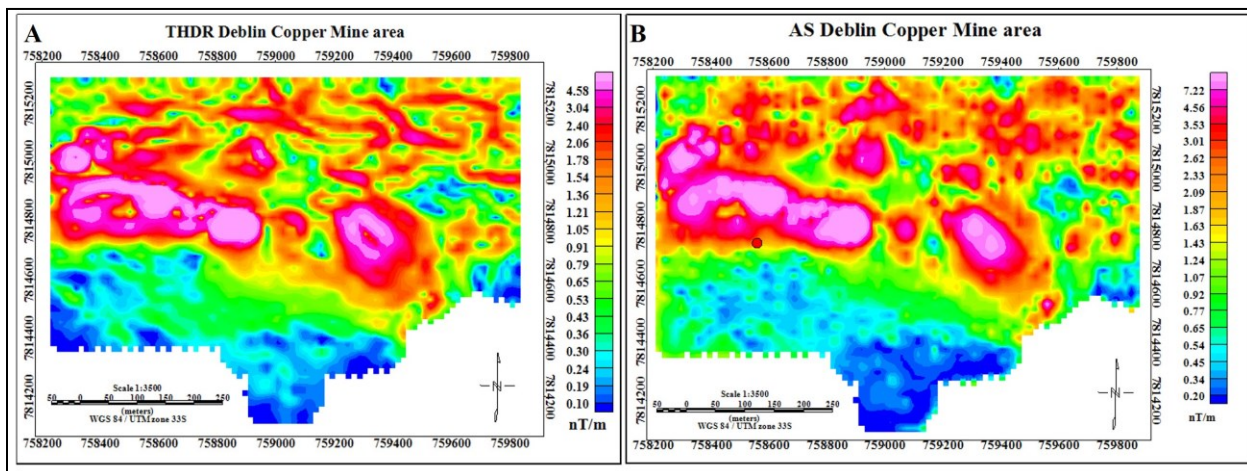
Figure 7.51 Contact mapping of the magnetic units using A) total horizontal derivatives (THDR) and B) analytic signal (AS). The maps show contacts of the magnetic maps. The continuity of the stratigraphy is preserved in the THDR map and destroyed in the AS map.
