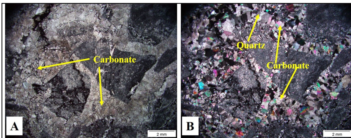
Figure 3.29 Textural characteristics of the dolomite breccia. A) Dilation in the dolomite breccia as a result of the deformation of the quartz and carbonates (PPL) and B) same image shown in crossed-nicols (XPL). DBDD0002: 13.70 m – 13.90 m – DB2S2-D10a.
