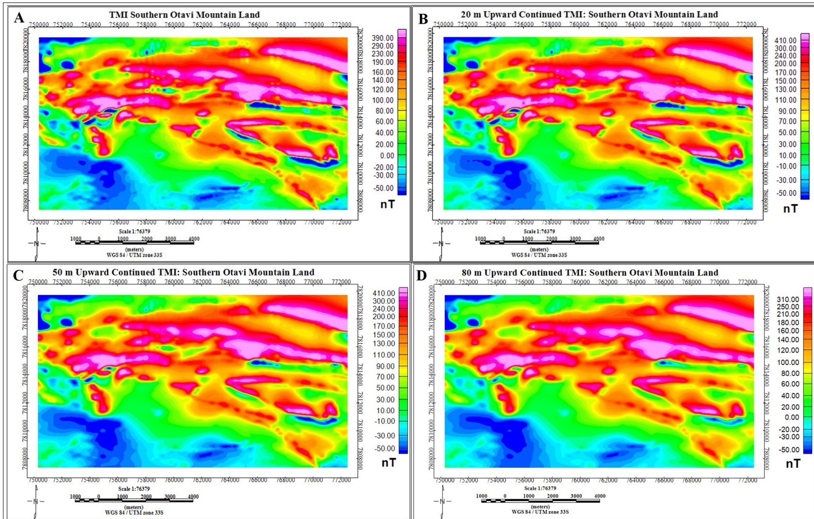
Figure 7.16 The application of upward continuation of the total magnetic intensity (TMI) aeromagnetic data of the southern Otavi Mountain Land by various heights. A) The TMI data shows details of the surface and near surface magnetic sources. B) The TMI data upward continued by 20 m. C) The TMI data upward continued by 50 m. D) The TMI data upward continued by 80 m. Notably, the higher the amount of upward continuation, the smoother the TMI data become.
