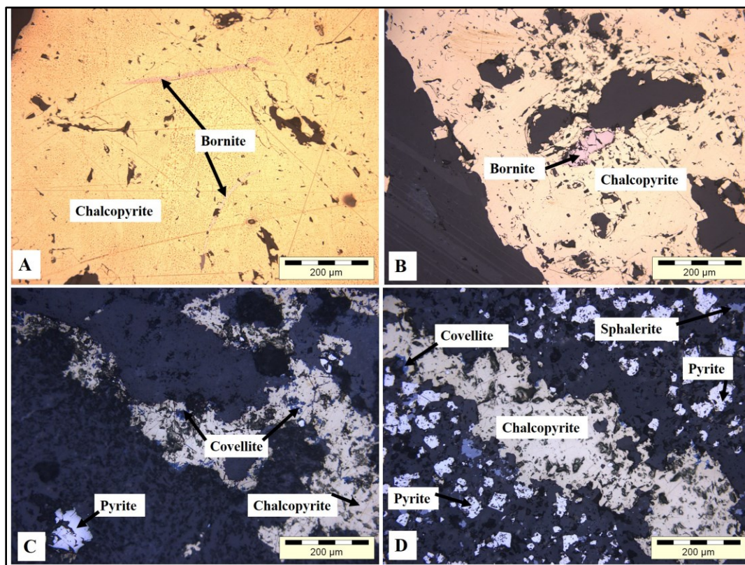
Figure 4.13 Reflected light photomicrographs showing textures and replacement patterns of bornite and covellite. A) Bornite veins cut-across chalcopyrite matrix. DBDD0002: 59.36 m – 59.56 m – DB2S7-D99d (silicified dolomite). B) Fractured bornite replacing chalcopyrite. In addition, the fractures in bornite are infiltrated by gangue minerals. DBDD0002: 59.36 m – 59.56 m – DB2S7-D100b (silicified dolomite). C) Fine-grained covellite replacing tarnished chalcopyrite. DBDD0001: 60.70 m – 60.88 m – DB1S9-D50a (breccia dolomite). D) Sporadic fine-grained covellite replacing chalcopyrite. DBDD0001: 109.67 m – 109.87 m – DB1S15-D61e (silicified dolomite).
