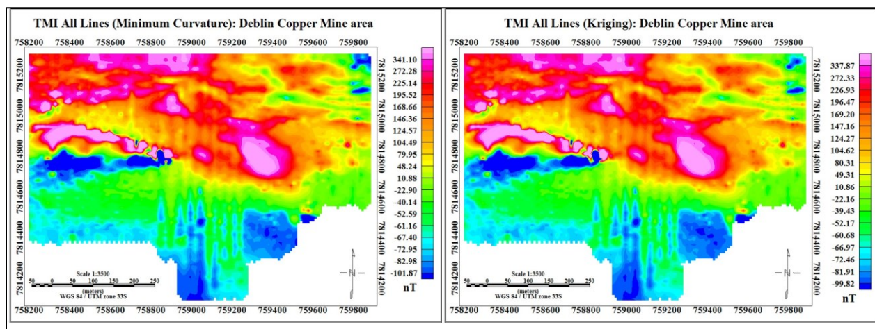
Figure 7.43 Comparison of Total Magnetic Intensity (TMI) maps gridded with A) minimum curvature and B) kriging methods.
