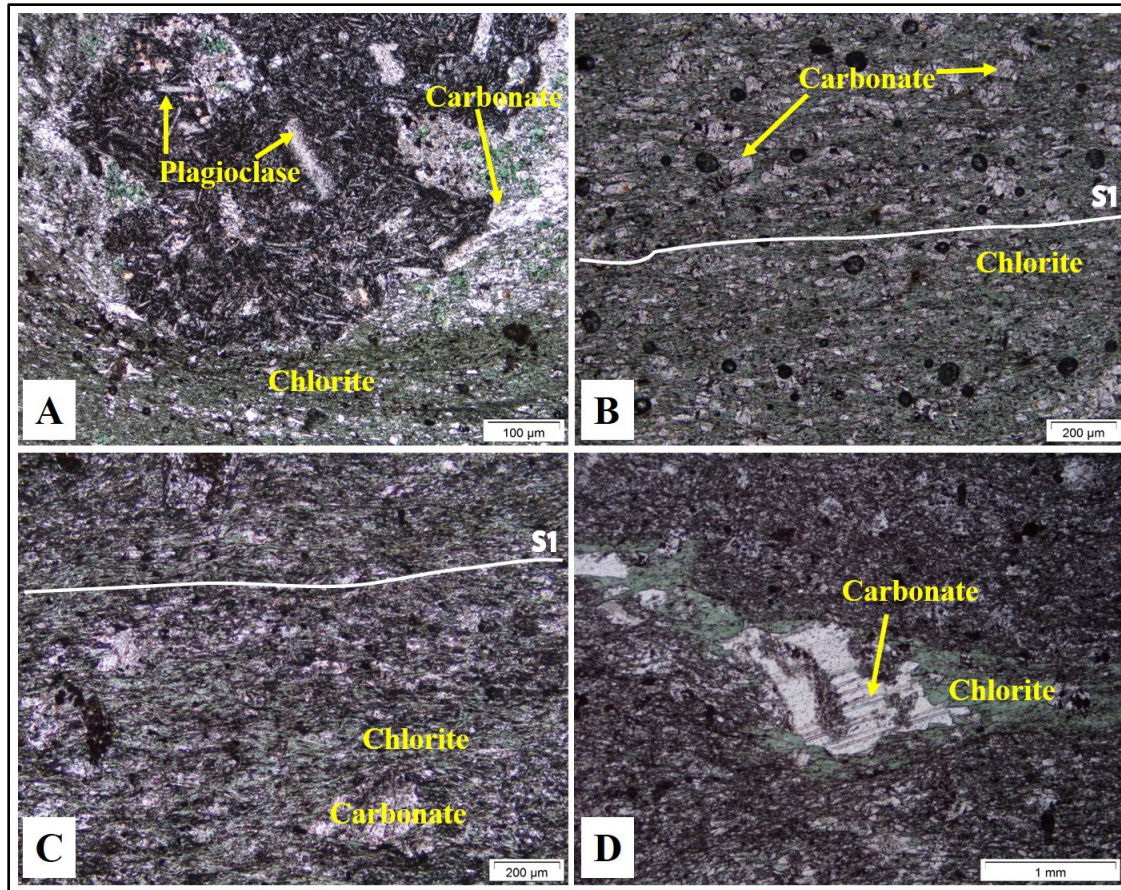
Figure 3.14 Mineral assemblage of the chlorite schist. A) Plagioclase rich pocket surrounded by carbonates and chlorite. Chlorite overgrows the primary minerals (micas) (PPL). DBDD0003: 3.73 m – 3.93 m - DB3S1-D124a. B) Micaceous spaced foliation overgrown by chlorite and fine-grained calcite (PPL). DBDD0003: 4.15 m – 4.35 m - DB3S2-D126a. C) Chlorite overgrowths. Also, the foliation is overgrown by carbonates. (PPL). Grid reference: 758268 mE; 7814999 mN: DB7a-D31a. D) Calcite overgrown by chlorite (PPL). 758268 mE, 7814999 mN: DB7a-D32b. The white line defines S 1 . (XPL= crossed-polarized light; PPL= plane-polarized light).
