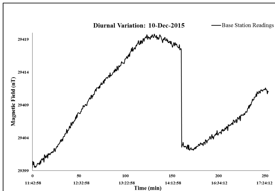
Figure 7.33 Diurnal variation plot for day 1. The Julian day is 344. The survey lasted for 253.5 minutes.
