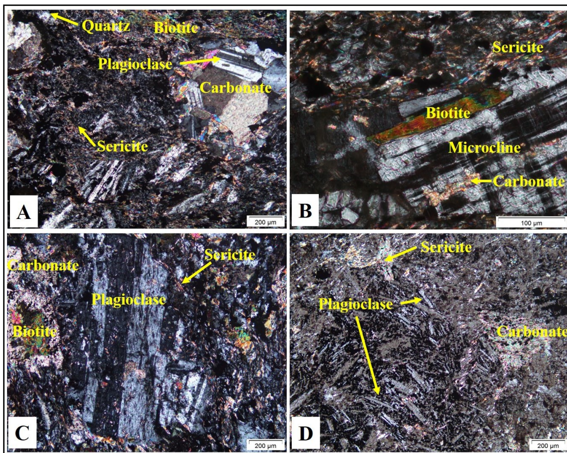
Figure 3.9 The tuff mineralogy, grain size and textural relationships. A) Randomly oriented fine-grained plagioclase, very fine-grained quartz and medium-grained calcite (XPL). DBDD0003: 39.20 m – 39.40 m – DB3S10-D17a. B) Fine-grained microcline overgrown by biotite and fine-grained calcite grains (XPL). DBDD0003: 47.28 m – 47.48 m – DB3S13-D18d. C) Coarse-grained plagioclase replaced by finer-grained calcite and sericite. The biotite grain is replaced by calcite (XPL). DBDD0003: 75.04 m – 75.24 m – DB3S15-D141d. D) Frequent very fine-to fine-grained plagioclase overgrown by calcite (XPL). DBDD0003: 34.20 m – 34.40 m – DB3S9-D131b. (XPL= crossed-polarized light; PPL= plane-polarized light).
