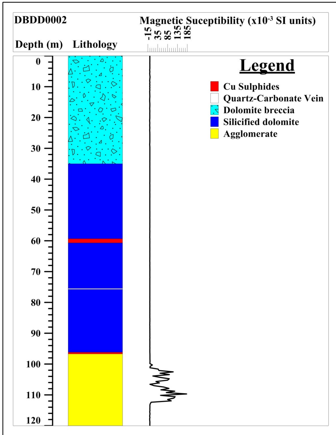
Figure 7.10 Magnetic susceptibility log for drill hole DBDD0002. The high values of the agglomerate suppress the variations in the overlying carbonates.
