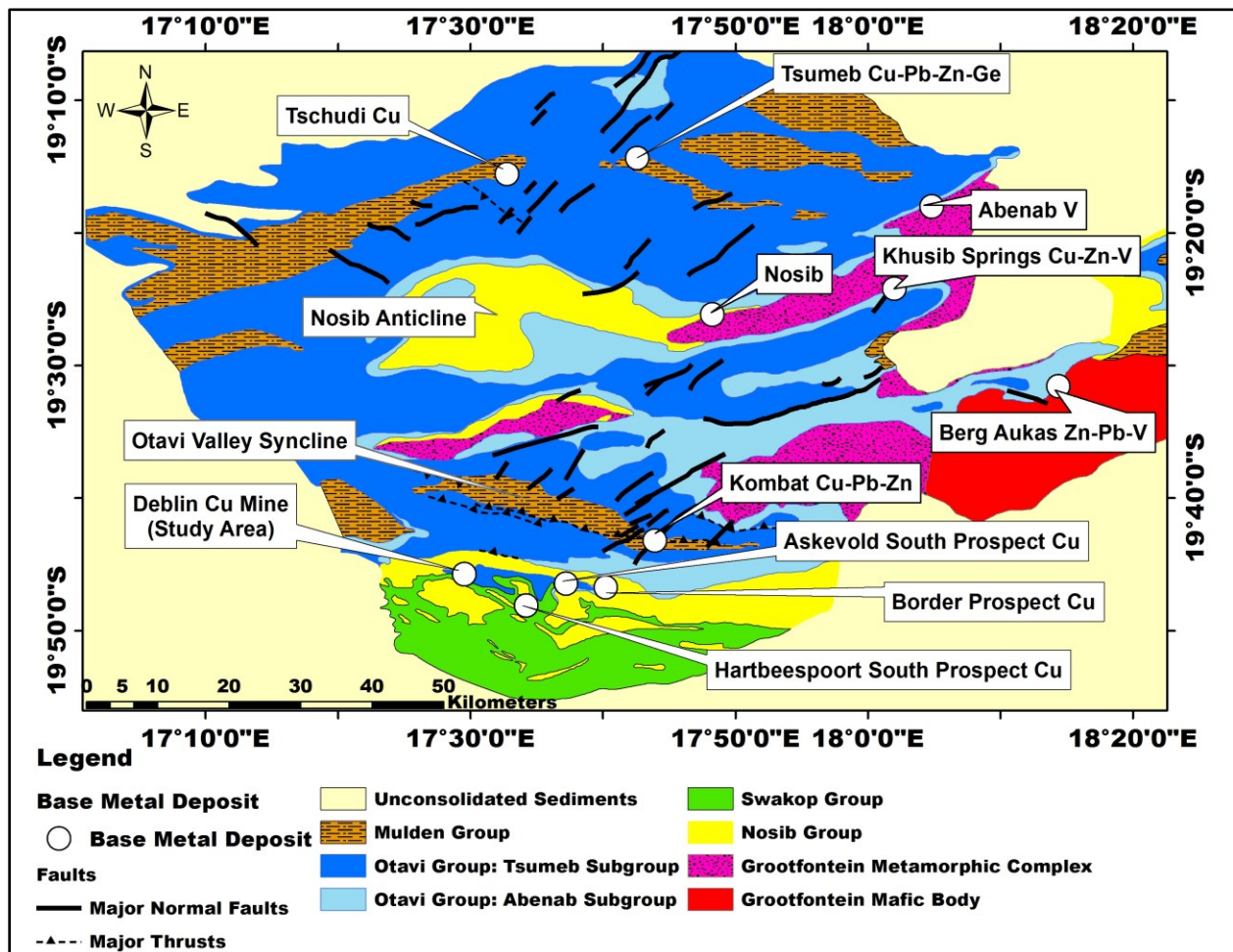
Figure 2.6 Geological map showing the regional architecture of the Otavi Mountain Land metallogenic province, the main base metal deposits (Mississippi Valley Type), the Deblin Cu Mine and other Cu prospects in the southern Otavi Mountain Land (modified after Kamona and Günzel, 2007 and map of 1:250 000 of the Geological Survey of Namibia).
