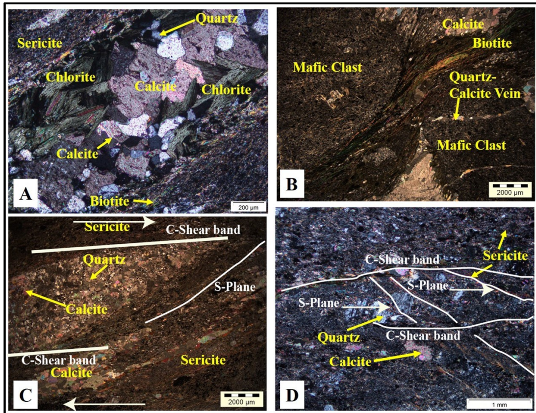
Figure 3.19 Mineral assemblage and textural relationships in the agglomerate unit. A) Chlorite overgrowth on calcite grains (PPL). DBDD0002: 109.70 m – 109.90 m - DB2S19-D26. B) Mafic clasts separated by biotite-rich cleavage domain and cross-cut by quartz-calcite veins (XPL). DBDD0001: 161.30 m – 161.50 m - DB1S23-D9h. C) Lens-shaped quartz-calcite veins with a mica-fish morphology as a result of shearing (XPL). DBDD0001: 145.00 m – 145.20 m – DB1S21-D83a. D) S-C fabric in the agglomerate with the C-plane transecting the main foliation (S-plane). DBDD0001: 161.30 m – 161.50 m - DB1S23-D9e. (XPL= crossed-polarized light; PPL= plane-polarized light). The white line defines the C-shear band and S-plane.
