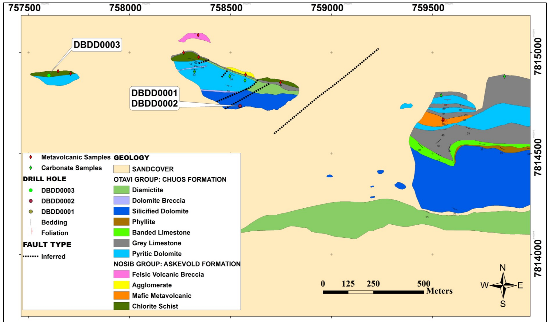
Figure 3.4 Detailed geological map of the area around the Deblin Copper Mine constructed at the scale of 1:2,500. In addition, the map shows the location of the twelve hand samples and three boreholes drilled in the study area. This geological map was constructed from the outcrop geology.
