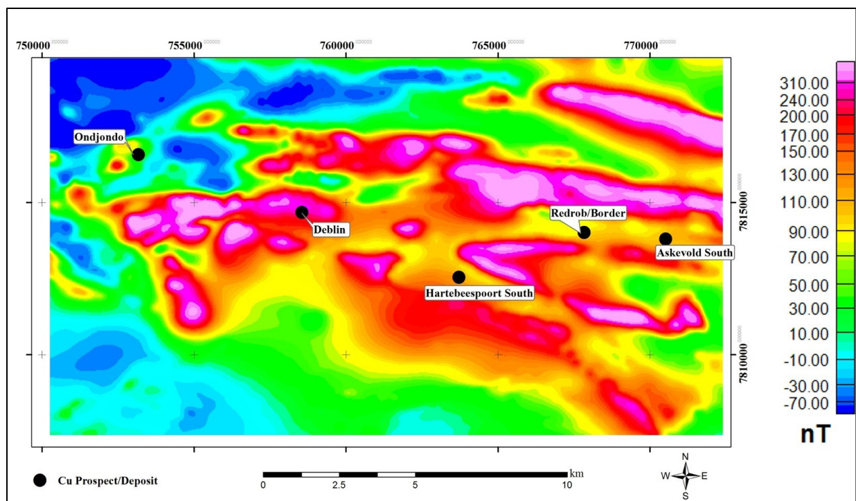
Figure 7.25 RTP map of the southern Otavi Mountain Land showing the magnetic anomalies in relation to copper deposits in the region.
