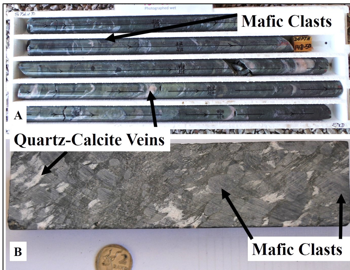
Figure 3.18 Photographs of the agglomerate in drill cores. A) The drill cores exhibit fresh, though chloritized agglomerate with a foliated matrix and fine grained mafic clasts of the agglomerate. The unit is cross-cut by abundant quartz-calcite veins. DBDD0001: 146.60 m – 151.33 m depth. B) Frequent sub-rounded mafic clasts and quartz-calcite veins in the agglomerate. DBDD001: 161.30 m – 161.50 m - DB1S23. The coin for scale in the photograph.
