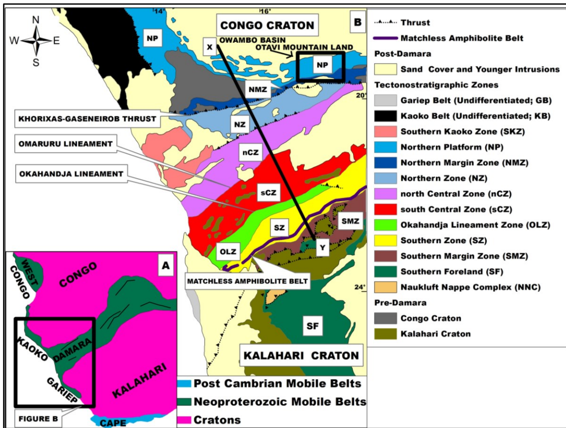
Figure 2.2 The location and architecture of the Damara Belt. (A) Simplified map of the Neoproterozoic Pan-African belt systems in southern and central Africa showing the intracontinental Damara Belt and the coastal Kaoko and Gariep Belts (after Gray et al., 2008; Miller, 2008). (B) Simplified map of the Damara Belt showing the tectonostratigraphic zones (taken from Corner, 2008 and Miller, 2008). The X-Y line represents a cross section shown on Figure 2.4.
