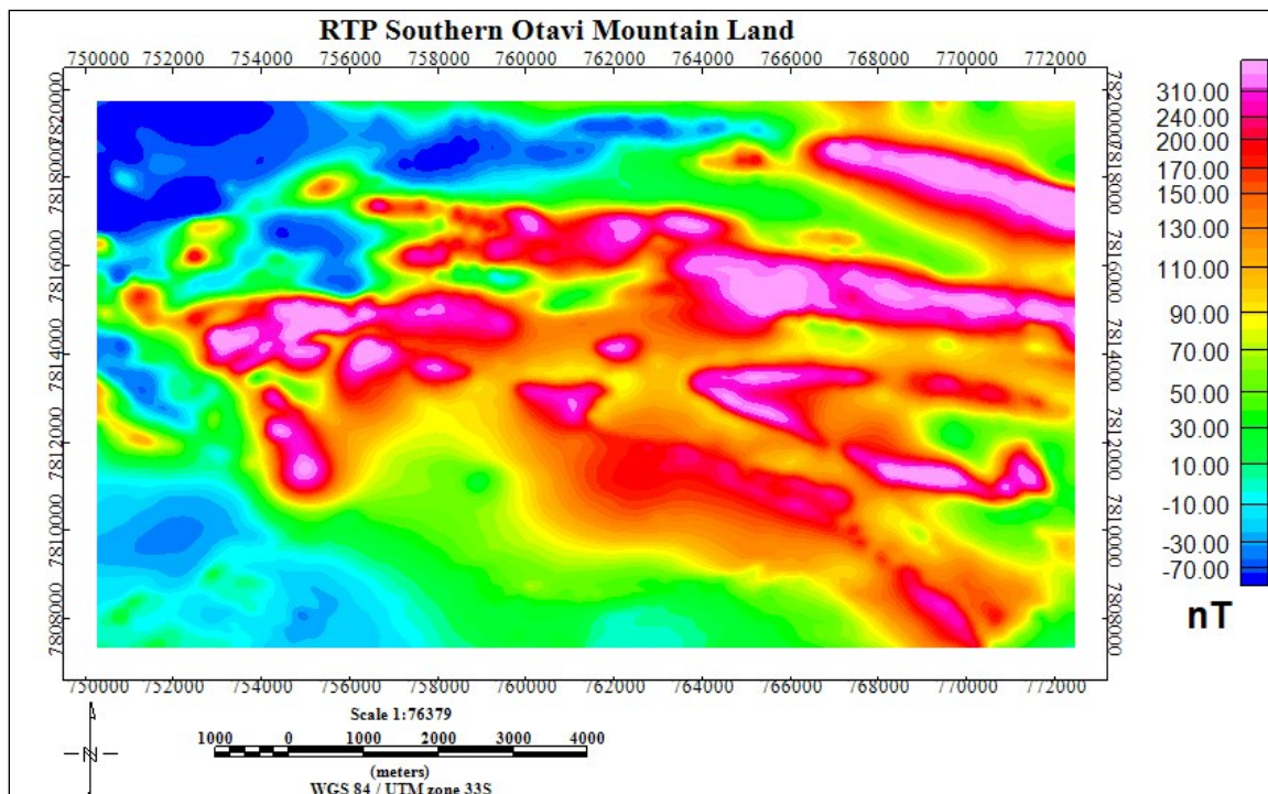
Figure 7.17 Application of the RTP operator to the TMI aeromagnetic data of the southern Otavi Mountain Land. Note that the RTP image has subtle north-south flight line noise (very clear in the sunshaded image). The flight line noise is evident in the northern part of the map.
