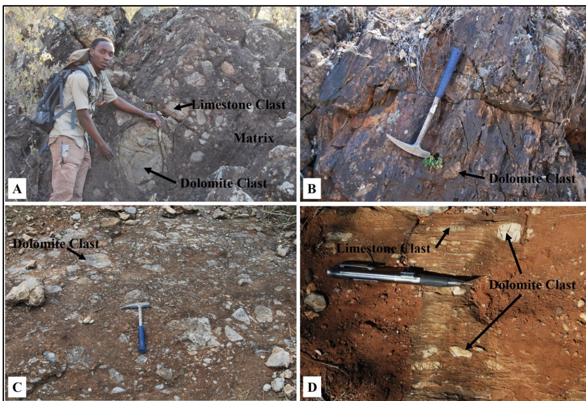
Figure 3.30 Field images of the diamictite: A) Diamictite with large angular carbonate clasts. B) A banded iron-rich layer within the diamictite. The outcrop exhibits a red colour due to ferruginous material. Both A-and B-photographs represent the outcrop in the northwestern part of the study area. Grid reference: 758810 mE, 7814791 mN. C) Diamictite with limestone and dolomite fragments in a brown calcareous matrix. The matrix of the dolomite weathers to brown. Grid reference: 759157 mE, 7814229 mN. D) Poorly exposed diamictite layer (~60 cm) with dolomitic depositional layers intercalated with the pyritic dolomite. Grid reference: 759653 mE, 7814678 mN. The photographs in C and D represent the outcrop in the southern part of the study area. Geological hammer and pen for scale in the photographs.
