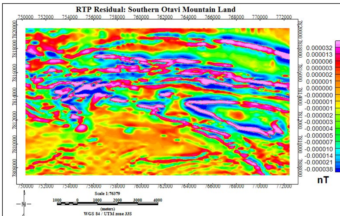
Figure 7.23 Residual filtering are applied to the aeromagnetic data to selectively remove the regional magnetic field. The residual magnetic field map shows magnetic response of the shallower bodies.
