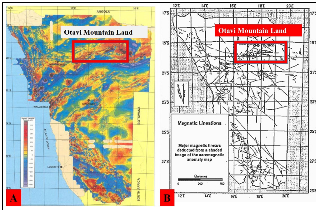
Figure 7.1 Regional aeromagnetic map of Namibia, 1: 1 000 000 scale. A) The airborne magnetic anomaly map (nT) of Namibia, with the International Geomagnetic Reference Field at the time of acquisition removed. B) Pattern of magnetic lineaments representing regional geological features, derived from (A). The red open boxes in both maps show the location of the Otavi Mountain Land. Both maps are modified after Eberle et al. , (1995).
