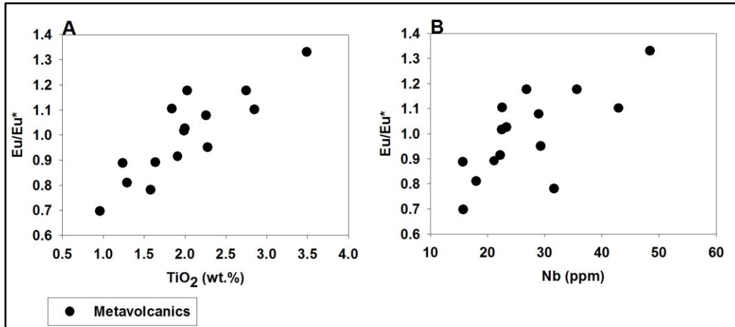
Figure 6.5 Plots of Eu/Eu* vs A) TiO 2 and B) Nb showing positive trends.
