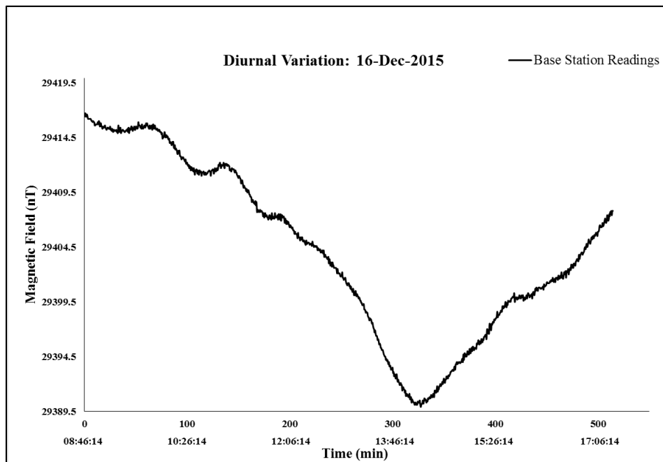
Figure 7.38 Diurnal variation plot for day 6. The Julian day is 350. The survey lasted for 514.5 minutes.
