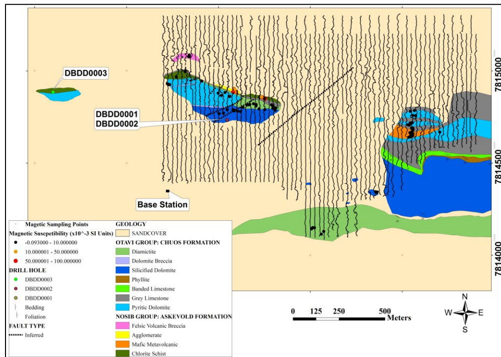
Figure 7.29 Detailed local geological map with survey lines in both areas with known geology and areas with the sand cover.
