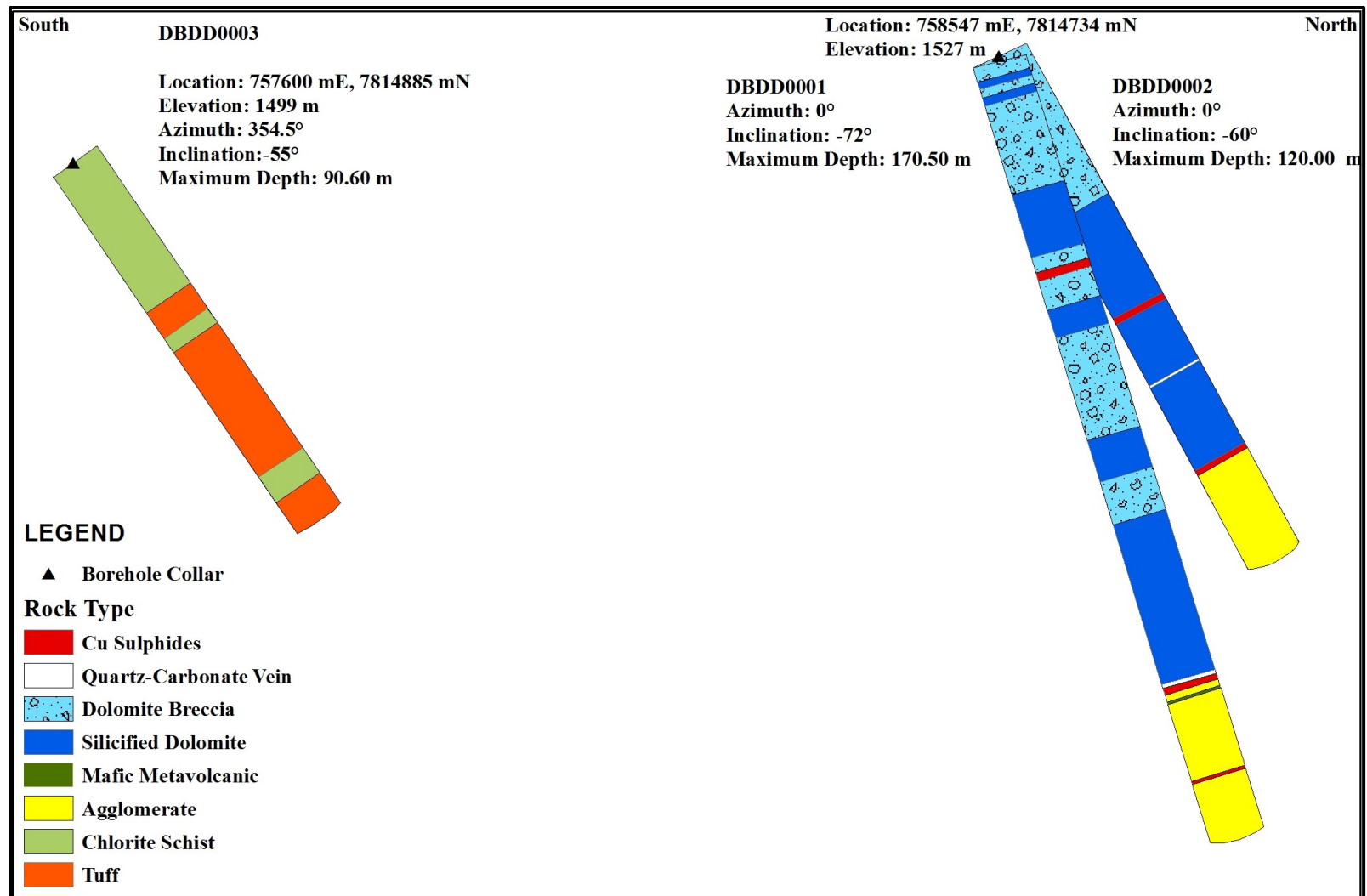
Figure 3.6 Cross-section of the three boreholes from the Deblin Copper Mine area showing their orientations. The drill holes were plotted with Leapfrog Geo 3.1 and digitized in ArcMap 10.2.2.
