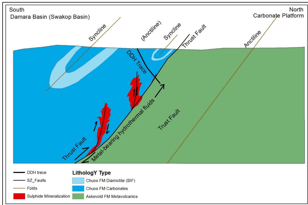
Figure 7.58. A conceptual cross-section model across the Deblin Copper Mine are showing a set of thrust faults along which metal-bearing basinal fluids were introduced into the carbonate host rocks.
