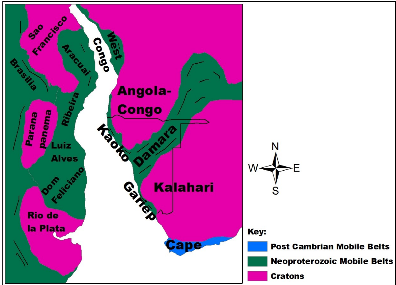
Figure 2.1 Map of the Brasiliano and Pan-African orogens showing the position of the Neoproterozoic Damara Orogen, Kalahari and Congo cratons as well as other orogenic belts (after Gray et al. , 2008, Miller, 2008).
