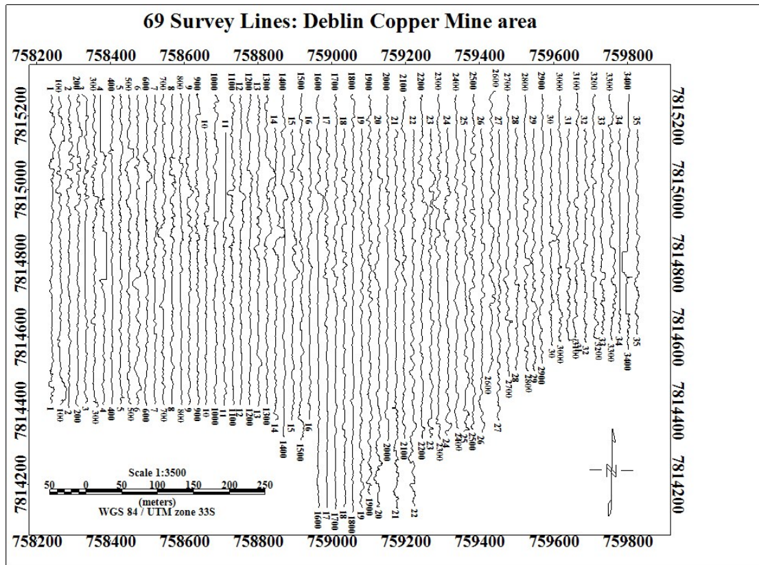
Figure 7.31 The 69 survey lines of the ground magnetic survey with the line spacing of 25 m. The survey lines have different lengths due to limited access of some parts of the survey area.
