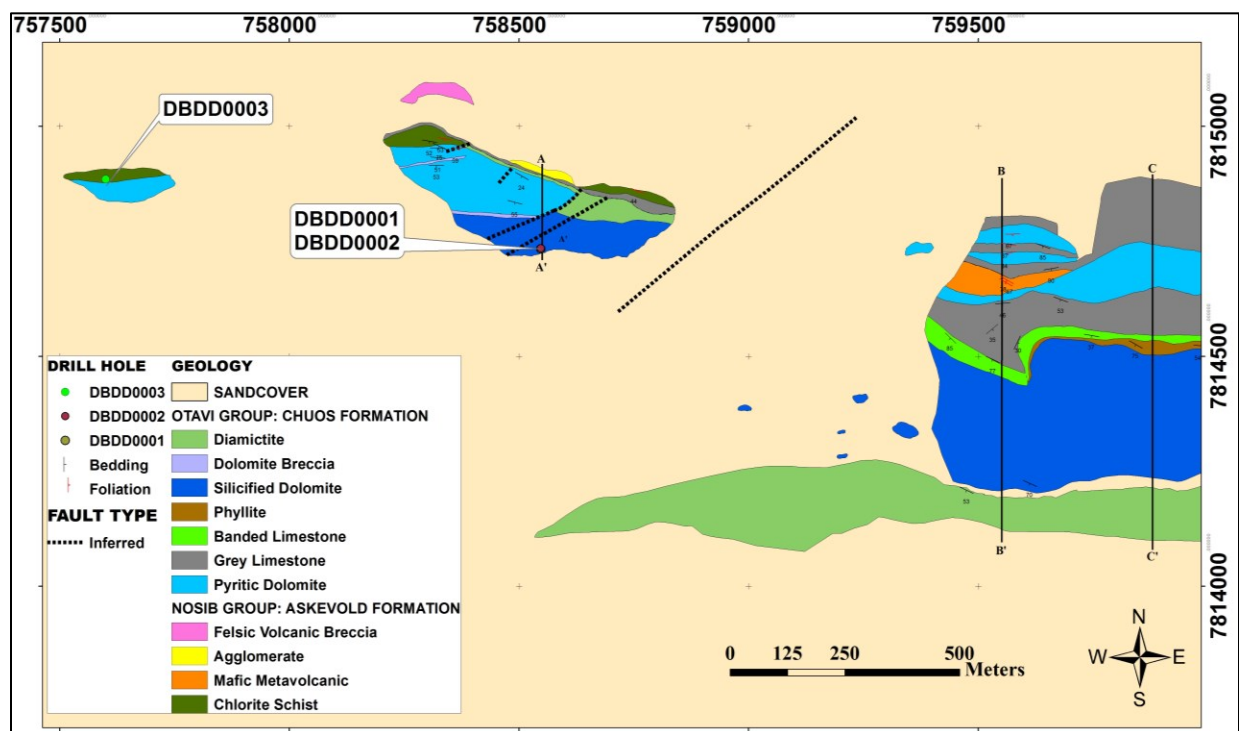
Figure 7.4 Geological map of the Deblin Copper Mine area showing the AA'-CC' lines for the cross-sections shown on Figure 7.5.
