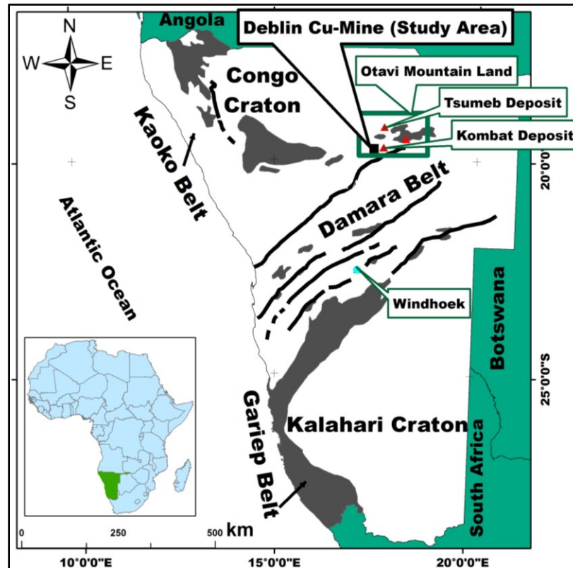
Figure 1.1. Location map of the study area on the northeastern margin of the Damara Belt (taken from Miller, 1983 and Borg, 2000). The open green box represents the Otavi Mountain Land. Bottom left inset shows location of Namibia.
