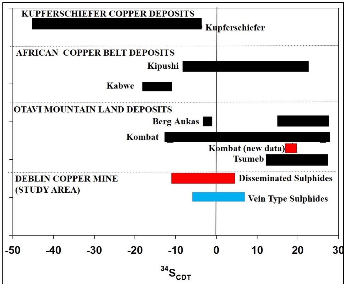
Figure 5.3 Sulphur isotope ratios ( \delta^{34}\text{S}_{\text{CDT}} ) in the major deposits in the Otavi Mountain Land (OML), central African Copper belt and Kupferschiefer. Data taken from Dechow & Jensen (1965), Sawlowicz (1989) and Kamona and Günzel (2007).
