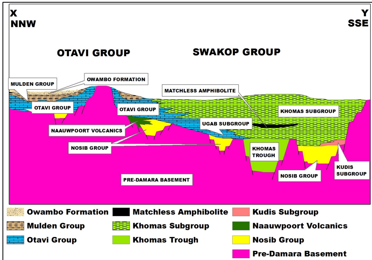
Figure 2.4 Generalized pre-orogenic section across the Damara Belt (from X to Y as shown in Figure 2.2b) with a simplified stratigraphic compilation showing basal, initial rift grabens, the syn-rift Nosib Group and the post-rift units of the Otavi, Swakop and Mulden groups (modified after Borg, 2000).
