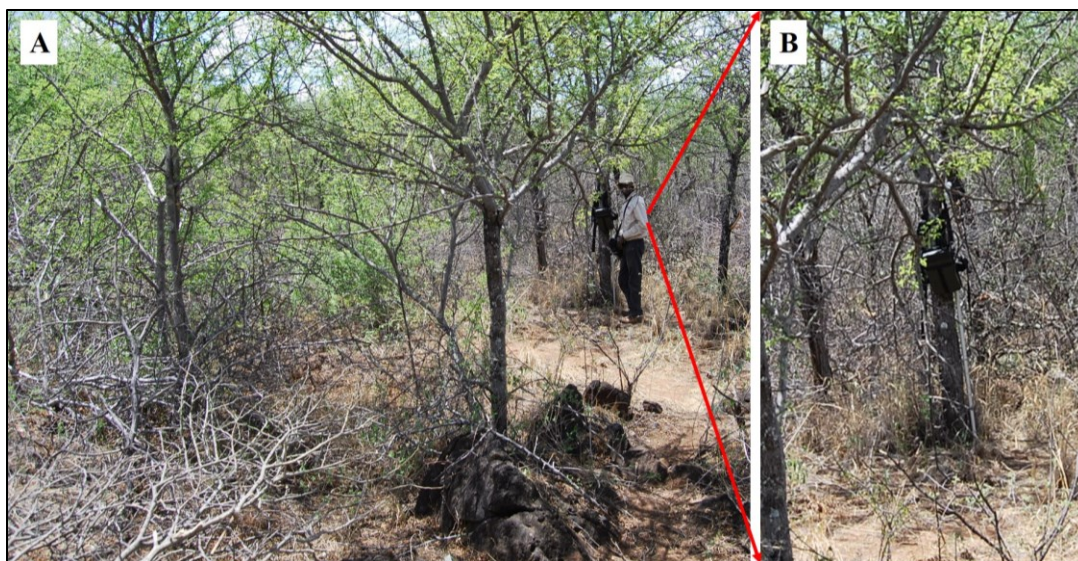
Figure 7.32 Base station. A) The field survey operator setting the base station. B) The base station magnetometer taking readings on an auto cycle mode.
