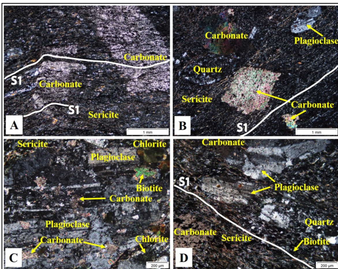
Figure 3.11 Multiple mineral overgrowths in the tuff. A) Calcite grains are cut through by the foliation. While calcite grains exhibit undulose extinction, the micas display kinked microfolds (XPL). DBDD0003: 47.28 m – 47.48 m – DB3S13-D18a. B) Coarse-grained calcite overgrowth over the foliation (sericite). This is the opposite of what is in ‘image A’ (XPL). DBDD0003: 85.60 m – 85.80 m – DB3S18-D19c. C) Medium-grained plagioclase replaced by fine-grained calcite, biotite and chlorite (XPL). DBDD0003: 76.24 m – 76.44 m - DB3S16-D27c. D) Plagioclase overgrown by calcite and sericite. Sericite, in contrast, is overgrown by calcite (XPL). DBDD0003: 85.60 m- 85.80 m – DB3S18-D19d. The white line defines S_1 foliation. (XPL= crossed-polarized light; PPL= plane-polarized light).
