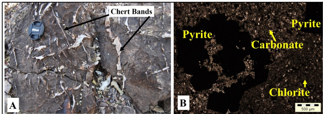
Figure 3.21 Field image and photomicrograph of the pyritic dolomite. A) Pyritic dolomite outcrop with frequent chert bands oriented in different directions. Grid reference: 759899 mE; 7814741 mN. B) Photomicrograph of the chloritized pyritic dolomite with an anhedral pyrite grain (XPL). Grid reference: 758497 mE, 7814882 mN: DB2b-D36e. (XPL=crossed-polarized light). Geological hammer and camera lens cover for scale in the photographs.
