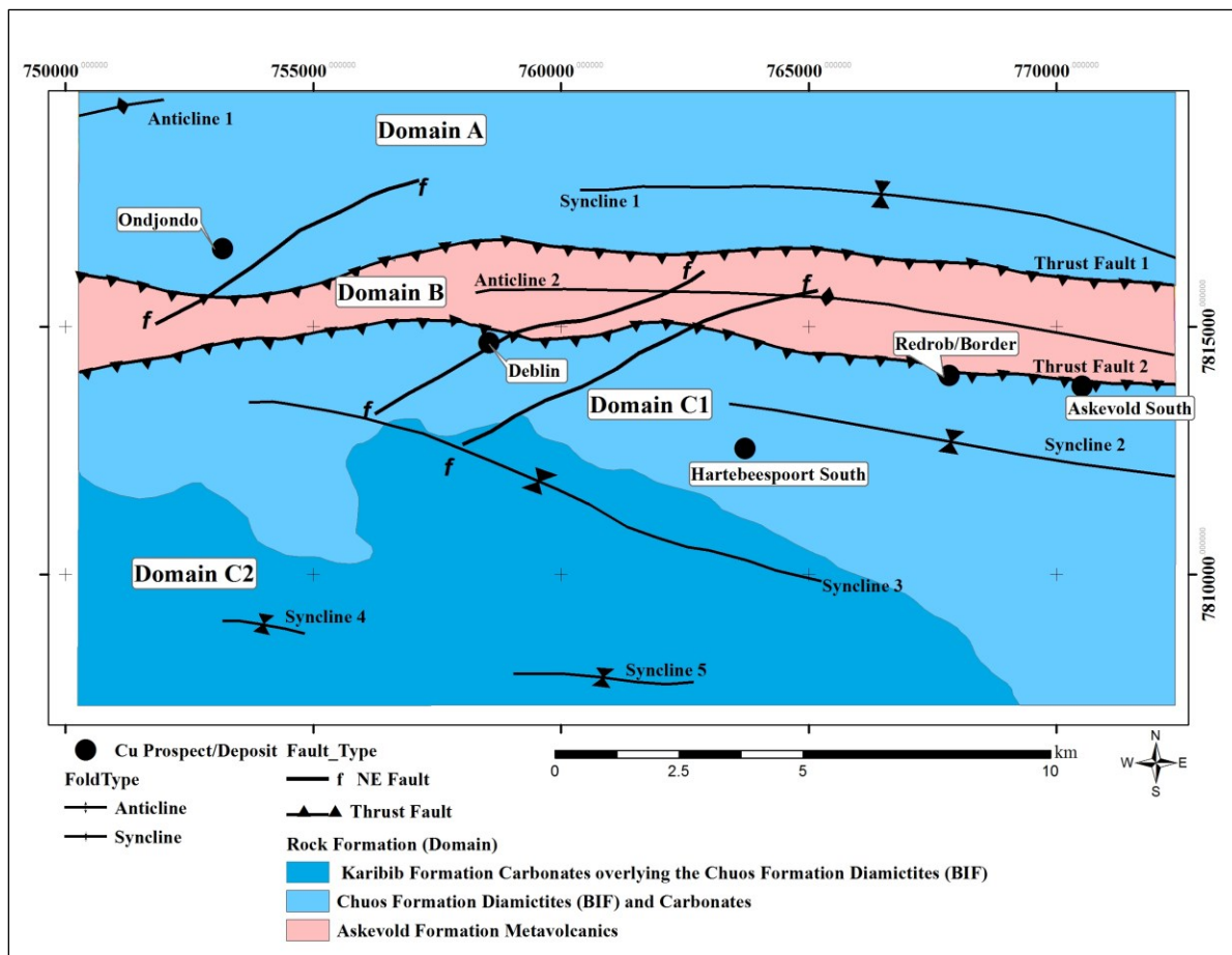
Figure 7.27 Interpreted solid geological map of the southern Otavi Mountain Land with the major east-west-trending thrust faults and shallow structural NE-trending faults as well as folds.
