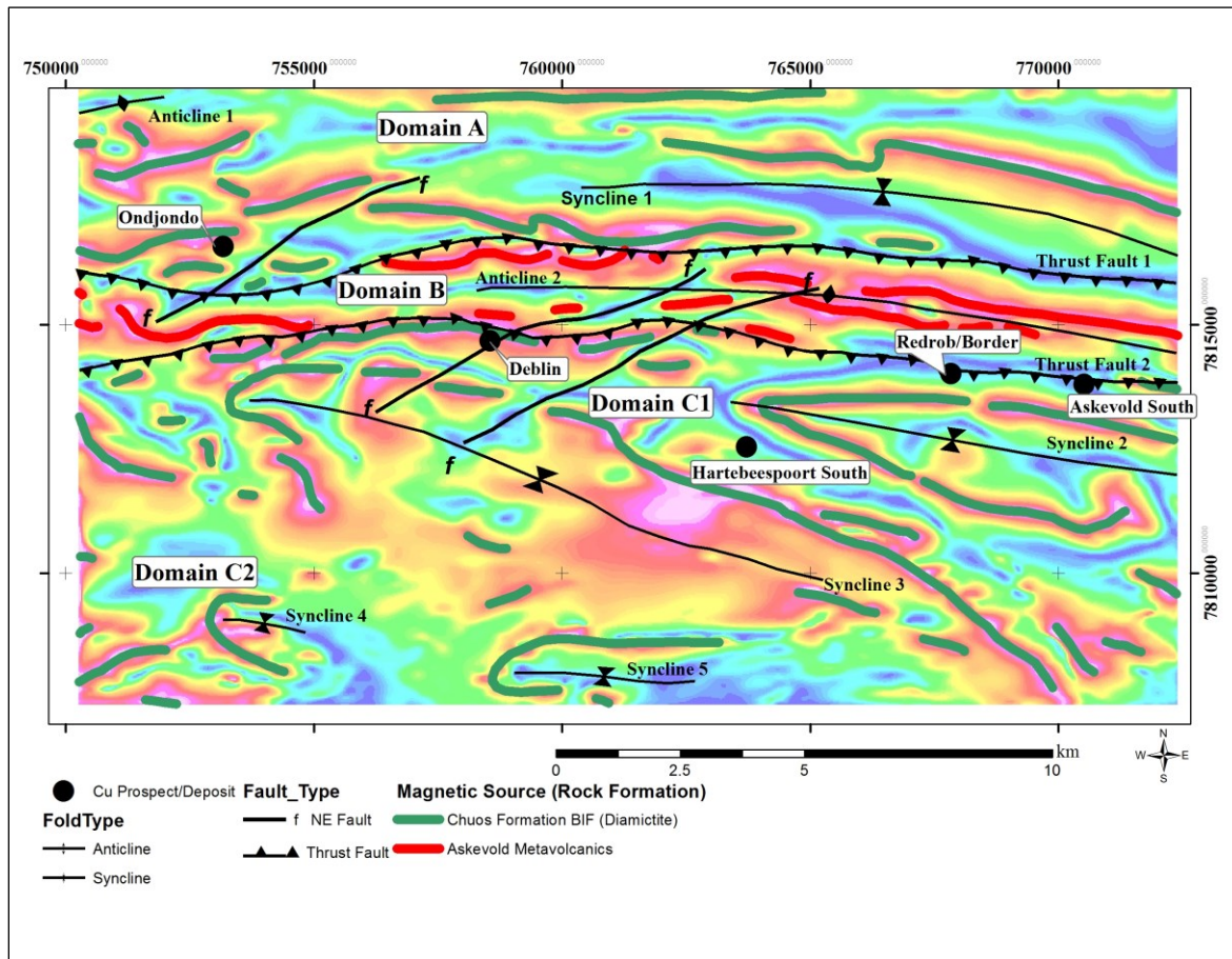
Figure 7.26 TDR map showing the response of different magnetic rock types, shallow regional crustal structures and the three different domains in the southern Otavi Mountain Land.
