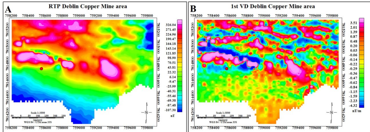
Figure 7.49 The application of the first vertical derivative (1VD) to the Deblin Copper Mine ground magnetic data. A) Reduced to Pole (RTP) map; B) 1VD map showing the shallow linear structures.
