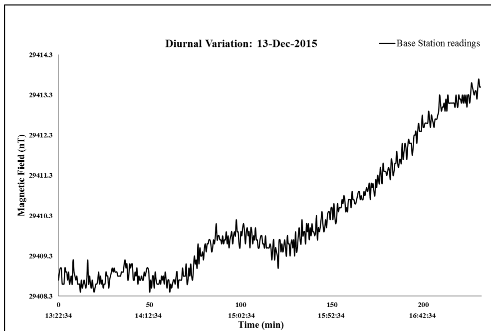
Figure 7.35 Diurnal variation plot for day 3. The Julian day is 347. The survey started after midday and lasted for 231.5 minutes.
