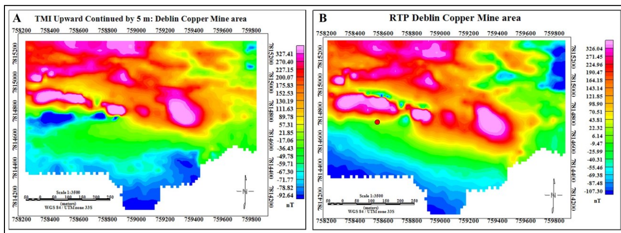
Figure 7.48 Ground magnetic data of the Deblin Copper Mine area. A) Is the Total Magnetic Intensity (TMI) image and B) is the Reduced to Pole (RTP) image of the TMI data with anomalies lying directly on top of their sources.
