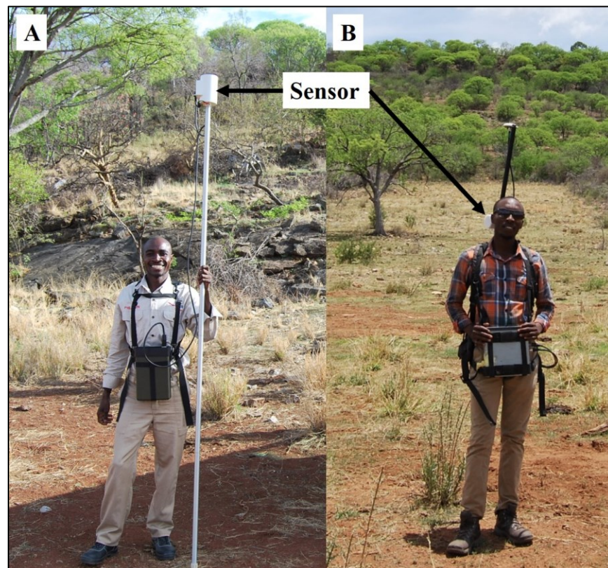
Figure 7.30 Photos of the magnetometers that were used to conduct the ground magnetic survey in the Deblin Copper Mine area. A) The Geometrics 856 proton precession magnetometer (Base station) and B) GSM-19 Overhauser magnetometer (Rover).
