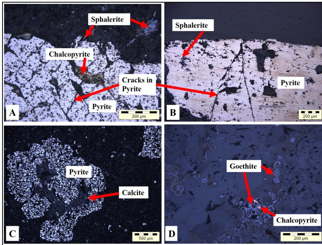
Figure 4.11 Reflected light photomicrographs showing replacement patterns of pyrite A) Fractured pyrite with minor chalcopyrite and sphalerite infills. DBDD0001: 137.73 m – 137.93 m – DB1S18-D75c (agglomerate). B) Outstanding fractures in pyrite with slivers of sphalerite and gangue minerals. DBDD0001: 139.10 m – 139.30 m – DB1S20-D80f (mafic metavolcanic). C) Highly corroded pyrite with cracks invaded by gangue minerals. Grid reference: 758497 mE, 7814882 mN – DB2b-D37 (pyritic dolomite). D) Colloform texture of goethite (formerly pyrite) and replacement of chalcopyrite by goethite. DBDD0001: 46.80 m – 47 m – DB1S6-D47g (dolomite breccia).
