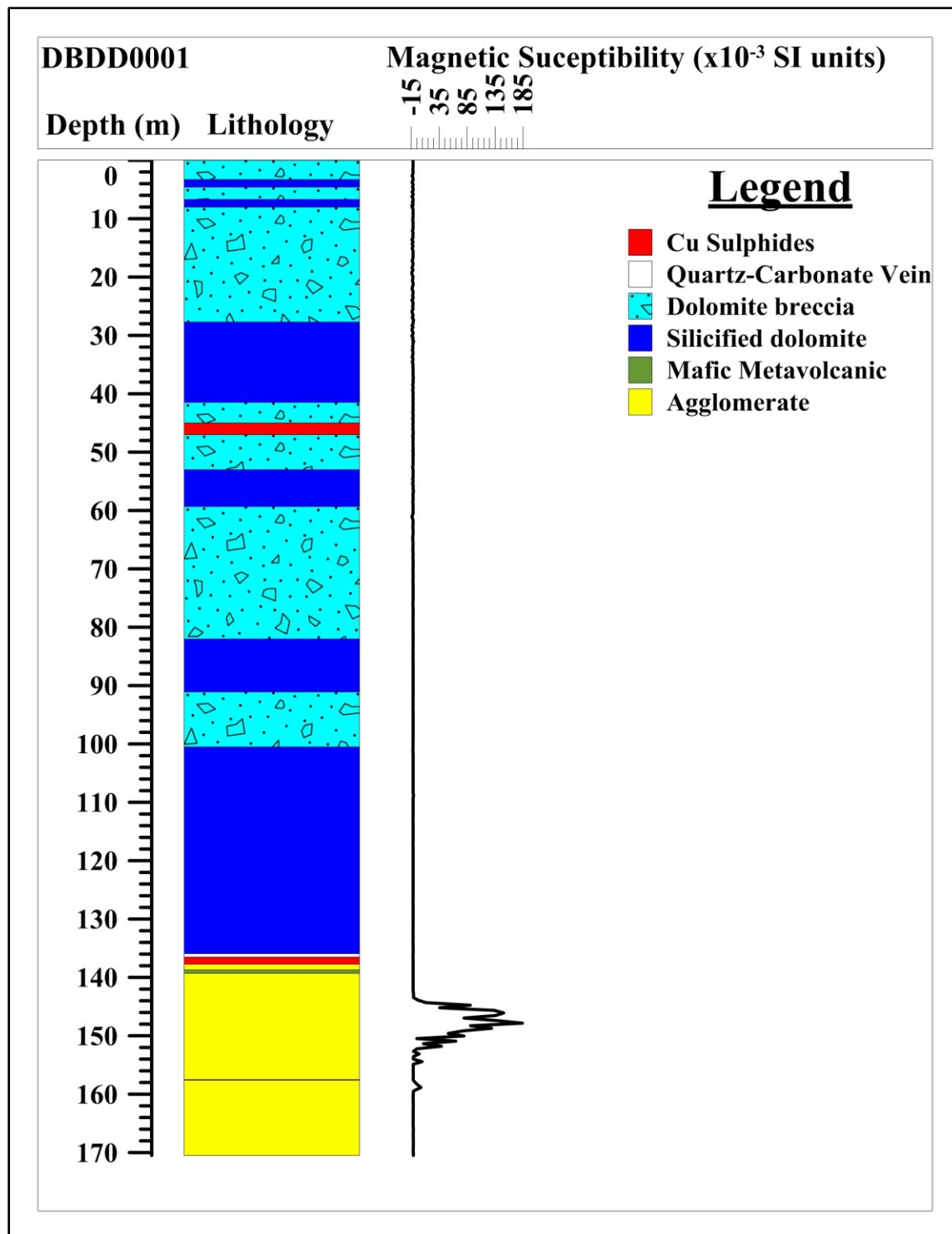
Figure 7.9 Magnetic susceptibility log for drill hole DBDD0001. The high values of the agglomerate suppress the variations in the overlying carbonates.
