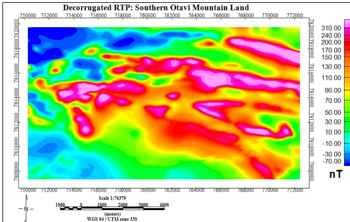
Figure 7.18 Decorrugated RTP map. The flight line noise observed in Figure 7.17 is completely removed and the image appears smooth.
