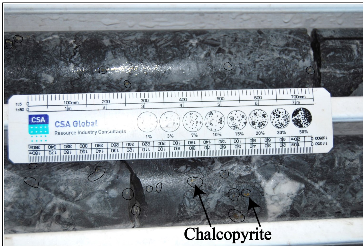
Figure 4.4 Disseminated chalcopyrite grains (enclosed in black circles) in the dolomite breccia. DBDD0001: 45.41 m – 46.20 m.
