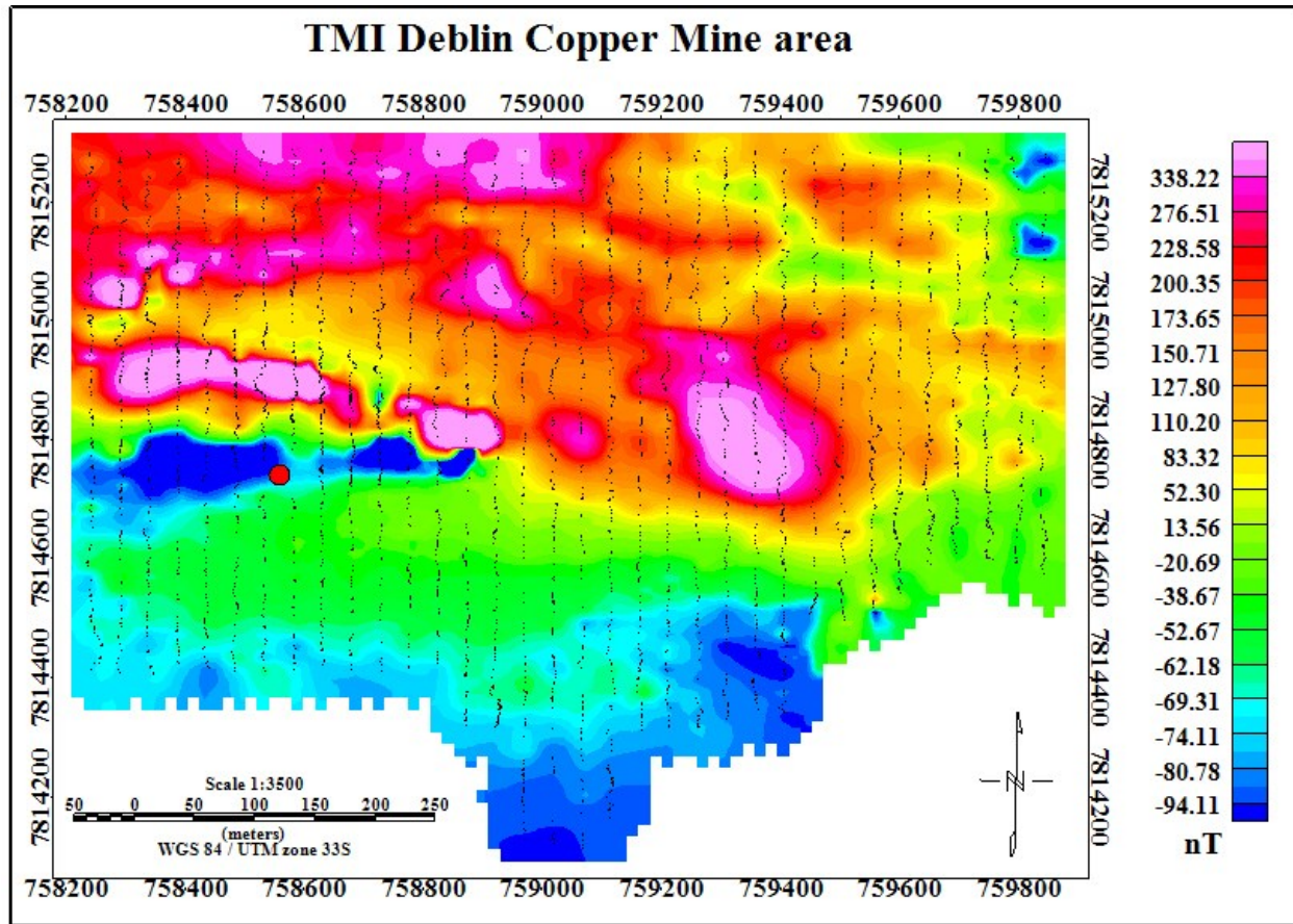
Figure 7.46 Total Magnetic Intensity (TMI) map of the Deblin Mine area with the magnetic data sampling points. The Earth's declination and inclination are -9.4 and -61.9, respectively. The red dot represents the location of the Deblin Copper Mine shaft.
