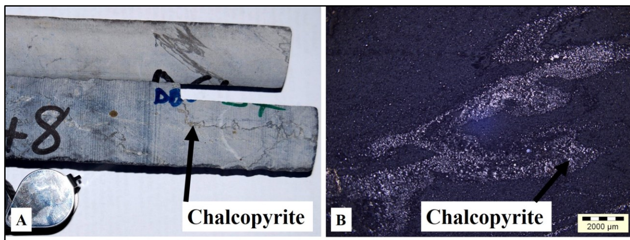
Figure 4.9 Photograph and photomicrograph of the folded sulphides in the silicified dolomite. A) Polydirectional, highly folded fine-grained chalcopyrite and pyrite veinlets. DBDD0001: 54.78 m – 54.98 m – DB1S7 (bottom sample); DBDD0001: 109.67 m – 109.87 m – DB1S15 (top sample). B) Highly folded chalcopyrite. DBDD0001 109.67 m – 109.87 m - DB1S15-D61 (Reflected Light).
