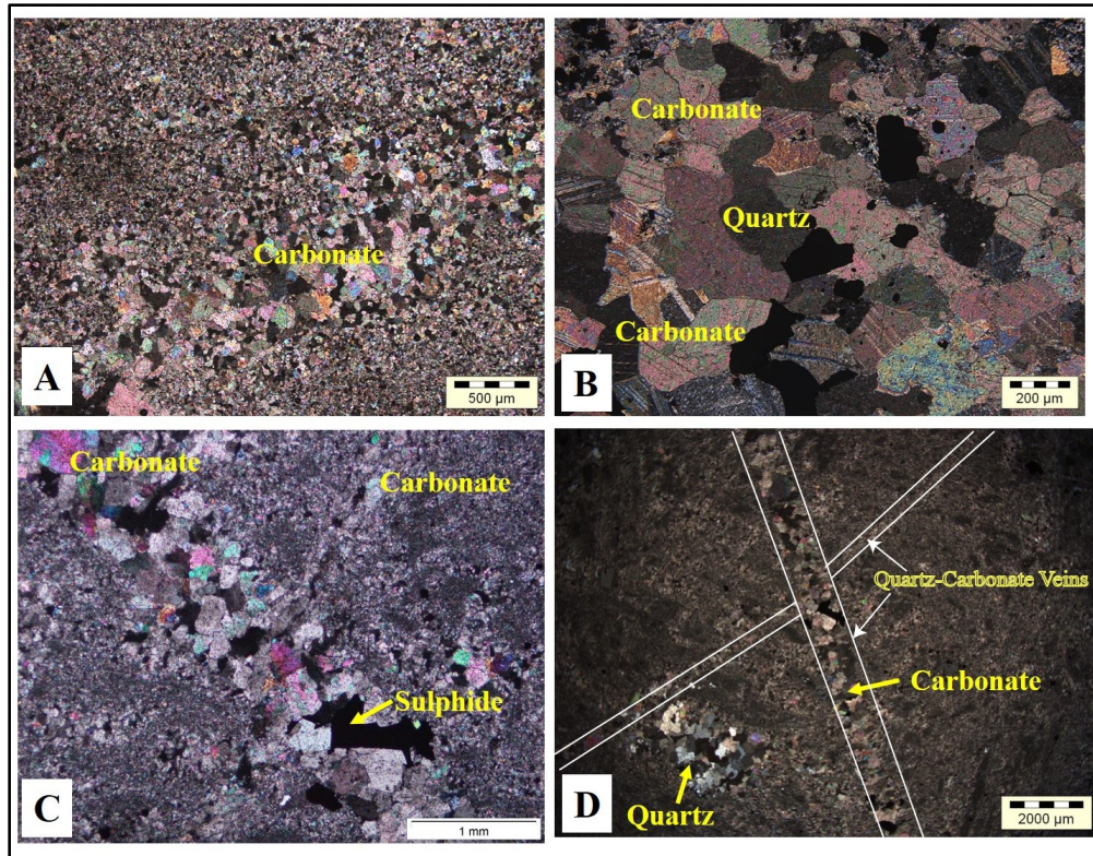
Figure 3.26 Silicified dolomite mineralogy and textures. A) Mosaic texture defined by both fine- and coarse-grained quartz and carbonate minerals (XPL). DBDD0002: 35.27 m – 35.47 m – DB2S4-D11a. B) Carbonate and quartz grains (XPL). DBDD0002: 73.40 m – 73.60 m – DB2S12-D14d. C) Coarse grained quartz-calcite veins with sulphides (XPL). DBDD0001: 3.75 m – 3.95 m – DB1S1-D1b. D) Cross-cutting relation of two quartz-calcite veins. The north-northeast trending vein is displaced by the north-northwest trending vein, which also host sulphides (XPL). DBDD0001: 3.75 m – 3.95 m – DB1S1-D1a. (XPL= crossed-polarized light).
