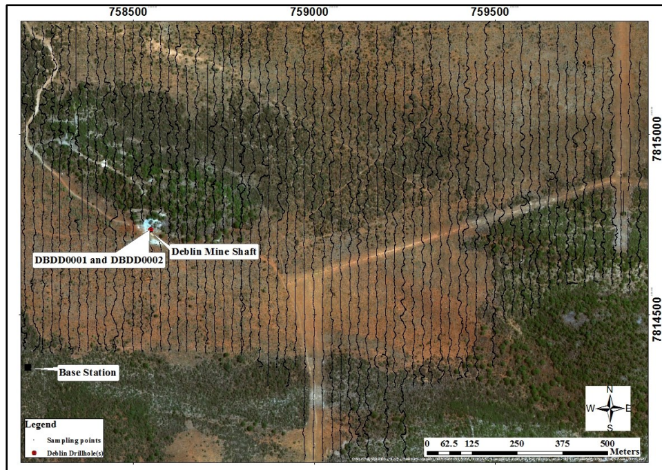
Figure 7.28 Sampling stations along the survey lines on the satellite image. The maps shows the location of the base station and drill holes. DBDD0003 does not appear on this map because it is outside the survey area.
