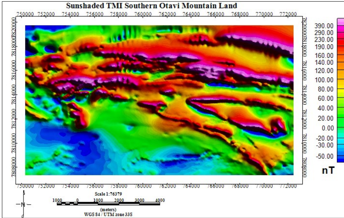
Figure 7.15 Sunshaded TMI map of the aeromagnetic data of the southern Otavi Mountain Land.
