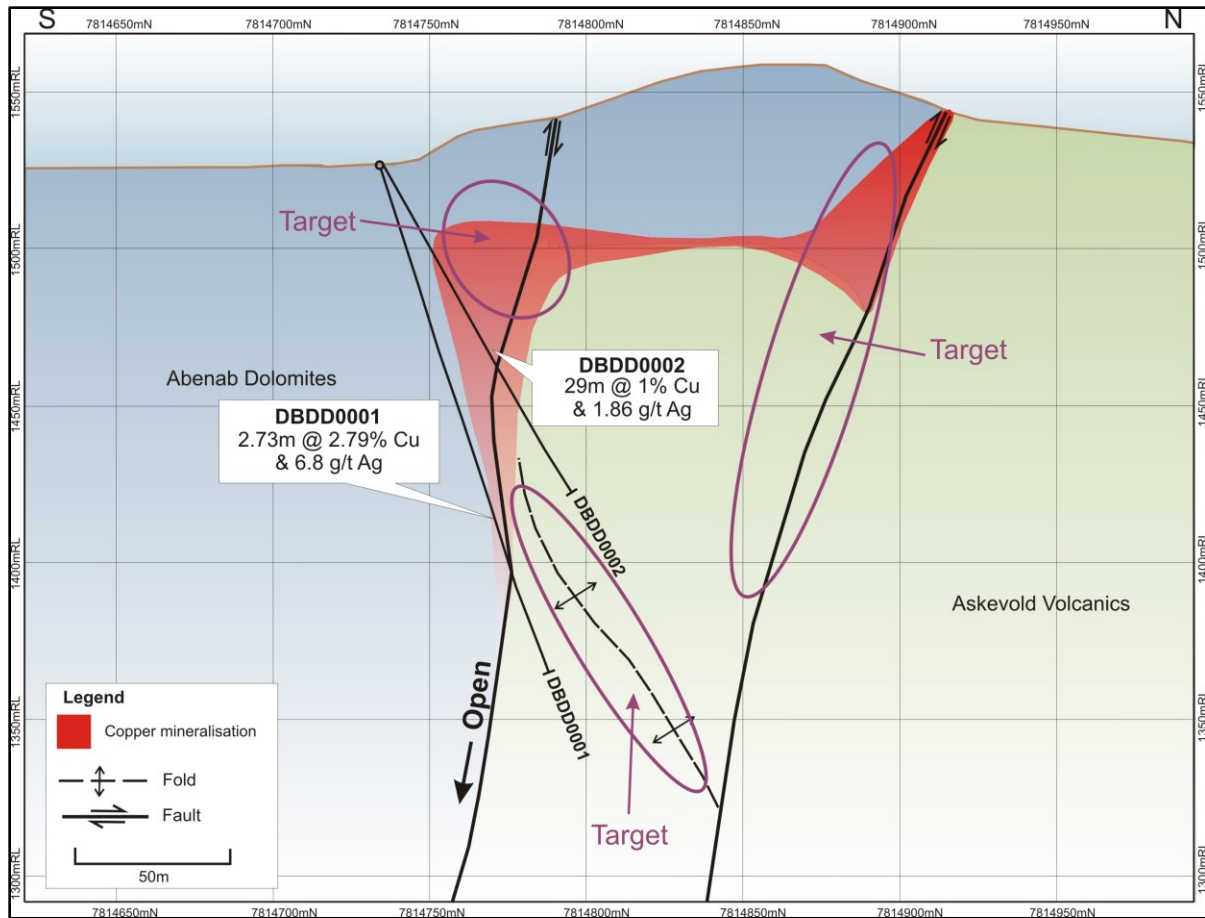
Figure 4.2 Cross section at the Deblin Copper Mine showing the modelled orebody morphology, structural interpretation, orientation of the drill holes DBDD0001 and DBDD0002 and drill targets (Golden Deeps Limited, 2013).
