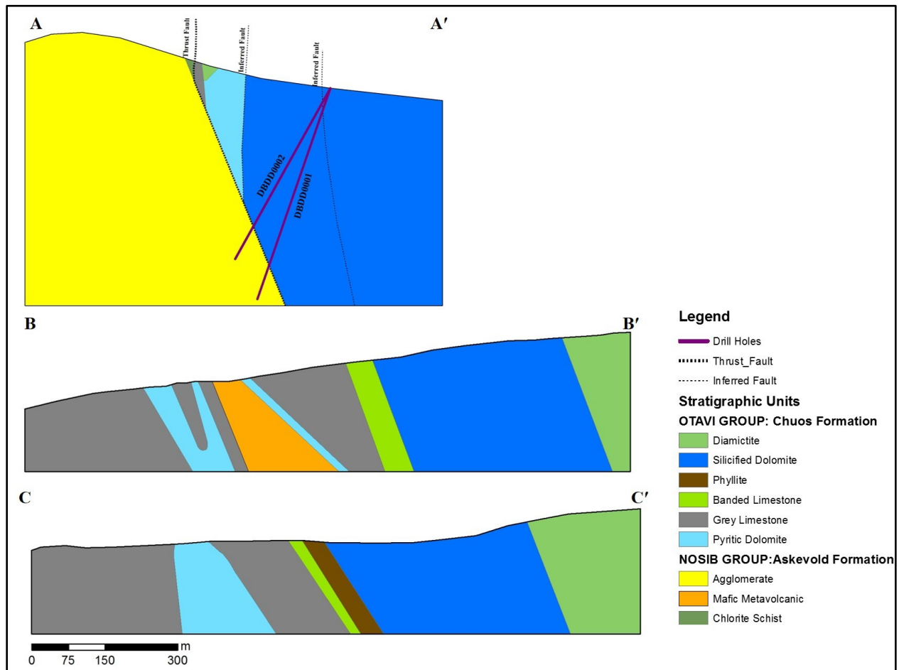
Figure 7.5 Geological cross-sections showing interpreted structural architecture of the Deblin Copper Mine area.
