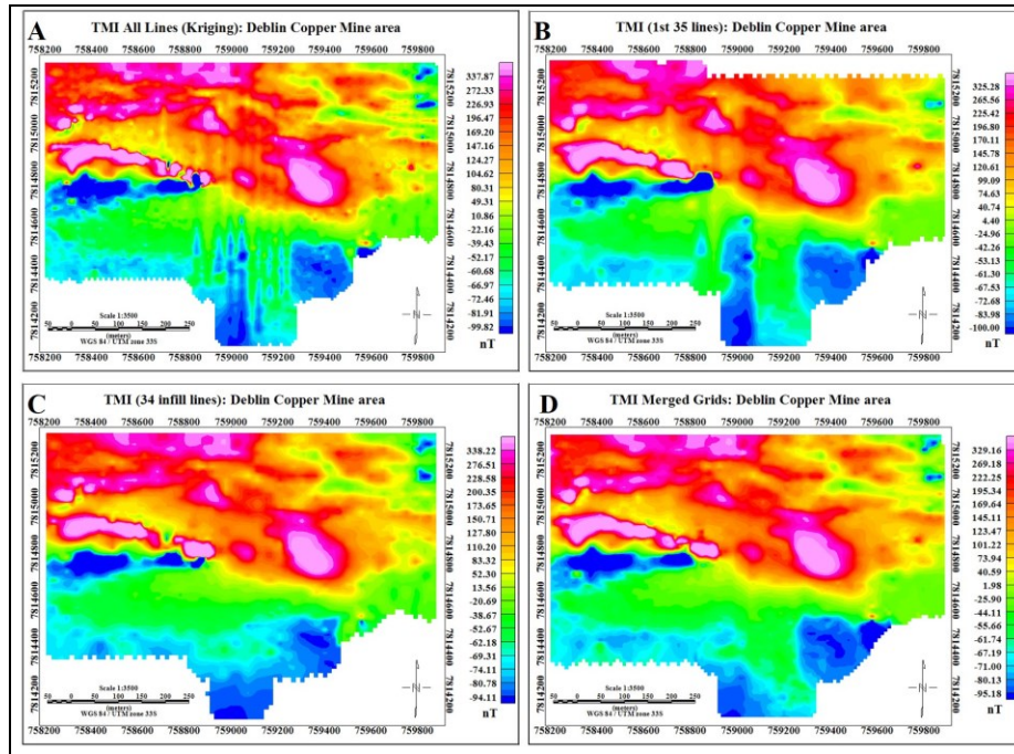
Figure 7.44 TMI maps gridded with different set of lines. A) All survey lines (69 lines). B) The first 35 lines. C) The 34 infill lines. D) A combination of two grids (B and C).
