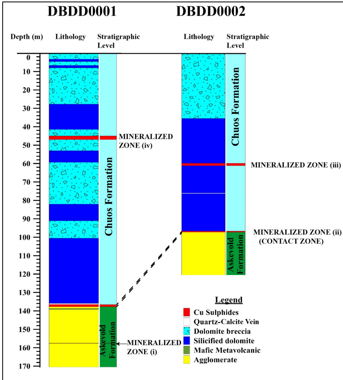
Figure 4.3 Lithostratigraphic logs from the Deblin Mine area showing the four ore-bearing horizons. DBDD0001 has a maximum depth of 170.5 m and intersected three mineralized zones in the agglomerate, silicified dolomite and dolomite breccia. DBDD0002, by contrast, has a maximum depth of 120 m and records two mineralized zones located in the silicified dolomite and dolomite breccia. Drill hole DBDD0001 is located at 758547 mE, 7814734 mN, whereas drill hole DBDD0002 is located at 758547 mE, 7814735 mN.
