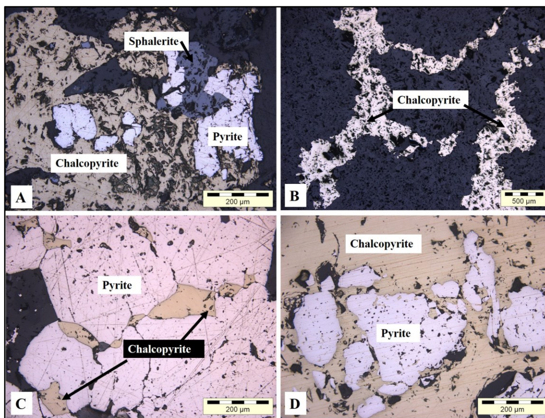
Figure 4.10 Reflected light photomicrographs showing chalcopyrite textures and replacements. A) Successive replacement of pyrite by corroded chalcopyrite. Also shown is both chalcopyrite and chalcopyrite cut by later sphalerite. DBDD0001: 137.22 m – 137.42 m – DB1S17-D69a (silicified dolomite). B) Corroded chalcopyrite veinlets. DBDD0001: 136.61 m – 136.81 m – DB1S16-D63e (silicified dolomite). C) Chalcopyrite veinlets infilling fine cracks of pyrite. DBDD0001: DBDD0002: 96.52 m – 96.71 m – DB2S17-D118c (silicified dolomite). The pinkish color in the pyrite grain is caused by the wrong field of light of the camera. D) Chalcopyrite largely replacing pyrite groundmass. DBDD0002: 59.87 m – 60.07 m – DB2S9-D104d (silicified dolomite).
