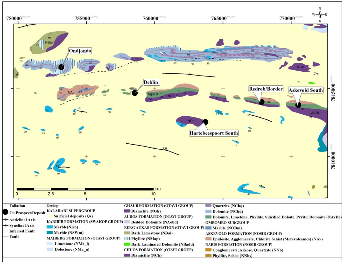
Figure 7.24 Regional geological map of the southern Otavi Mountain Land showing the extensive sand cover and limited rock exposure as well as mappable structural features. Modified after Smit (1959) and the Geological Survey of Namibia (2008).
