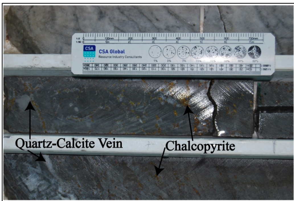
Figure 4.7 Chalcopyrite-bearing quartz-calcite veins, chalcopyrite veinlets and minor chalcopyrite disseminations in the silicified dolomite. DBDD0002: 59.15 m - 59.40 m.
