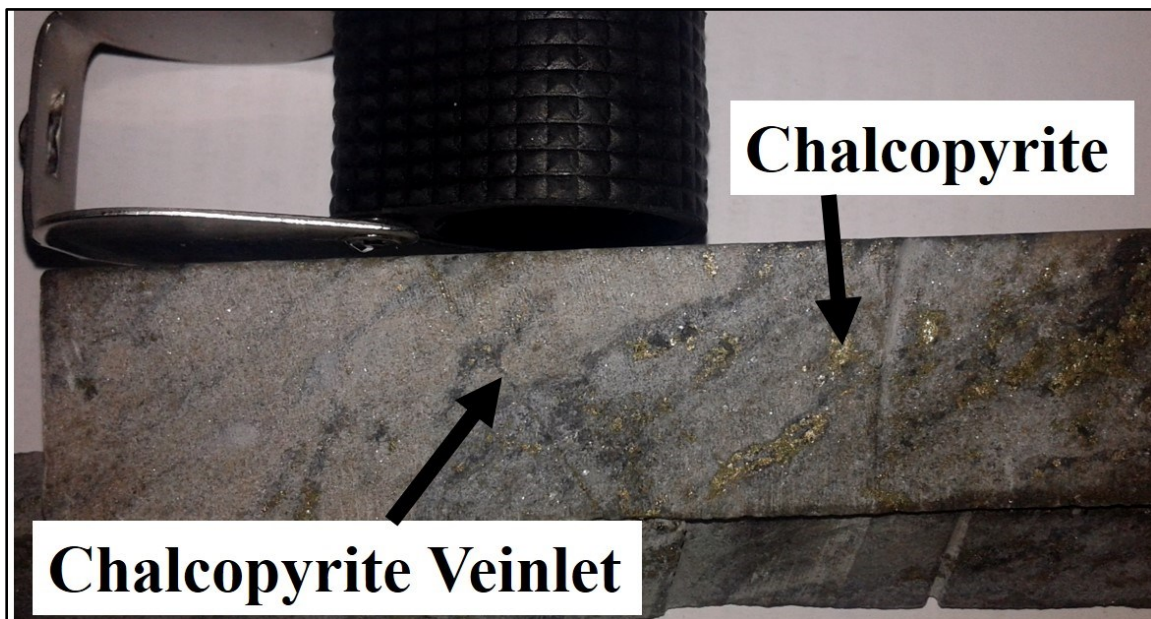
Figure 4.6 Stringer chalcopyrite cross-cut by later chalcopyrite veinlet in the silicified dolomite. DBDD0001: 82.20 m – 82.40 m - DB1S10.
