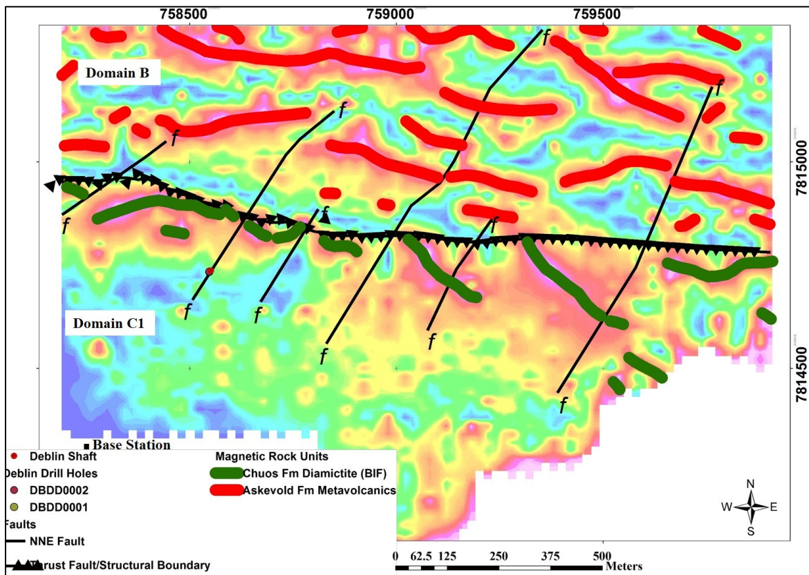
Figure 7.56 Interpreted TDR map showing the magnetic anomalies of the different magnetic units and the locations of the east-west-trending thrust fault and the shallow northeast-trending faults.
