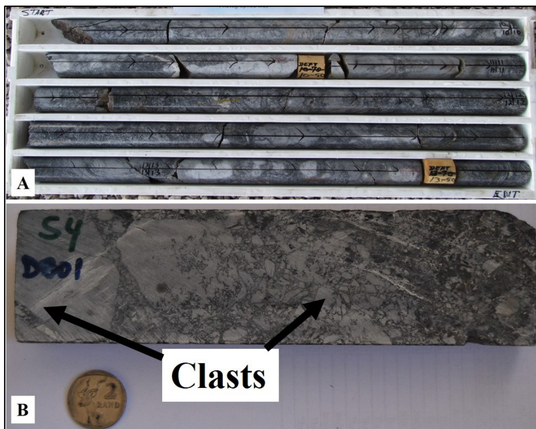
Figure 3.28 Dolomite breccia. A) Dolomite breccia with deformed stromatolites. DBDD0001: 9.14 m – 13.15 m depth. B) Clast-supported dolomite breccia. The clasts are silicified. DBDD0001: 15.84 m – 16.04 m – DB1S4. Coin for scale in the photograph.
