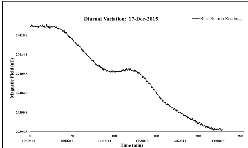
Figure 7.39 Diurnal variation plot for day 7. The Julian day is 351. The survey lasted for 229 minutes.
