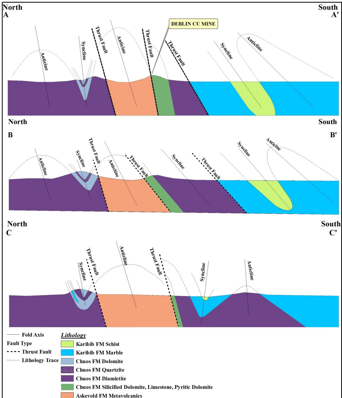
Figure 7.3 Regional geological cross-sections showing interpreted structural architecture of the southern Otavi Mountain Land.
