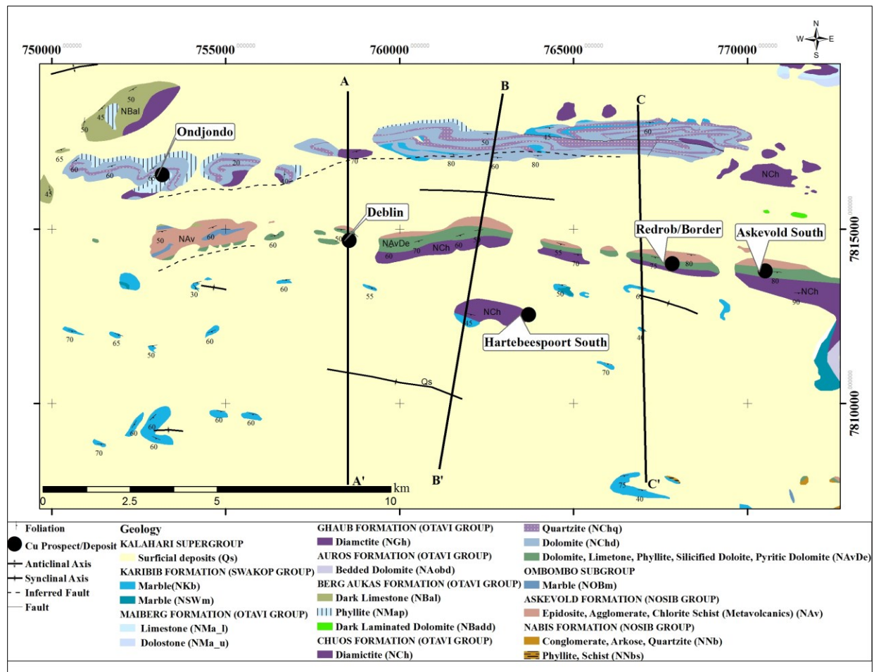
Figure 7.2 Regional geological map of the southern Otavi Mountain Land showing the AA'-CC' lines of the cross-sections shown on Figure 7.3. Modified after Smit (1959) and the Geological Survey of Namibia (2008).
