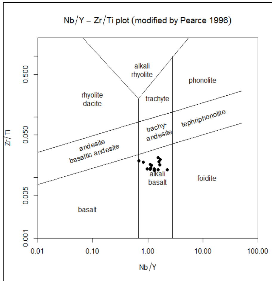
Figure 6.2 Geochemical classification of the metavolcanic rocks of the Askevold Formation using the Nb/Y-Zr/Ti diagram of Pearce (1996). The samples plot within the alkali basalt field, although one sample plots close to the basalt field.
