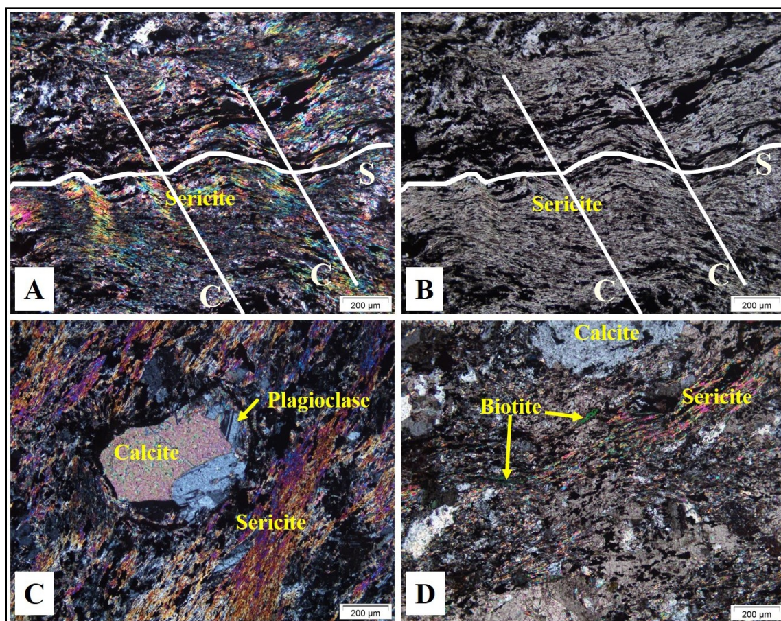
Figure 3.10 Spaced foliation in the tuff. A) S-C fabric with C-shear band foliation transecting the sericite dominated main foliation (S-foliation) during shearing (XPL) and B) same image shown in plane-light (PPL). DBD0003: 39.20 m – 39.40 m - DB3S10-D17c. C) Carbonates and plagioclase constitute the microlithons of the sericite cleavage domain (XPL). DBD0003: 39.20 m – 39.40 m - DB3S10-D17e. D) Sinuous cleavage made up of sericite. Biotite overgrowth on sericite (XPL). Conspicuous calcite overgrowths over the foliation. DBDD0003: 75.04 m – 75.24 m – DB3S15-D140c. The white lines define S and C surfaces. (XPL= crossed-polarized light; PPL= plane-polarized light).
