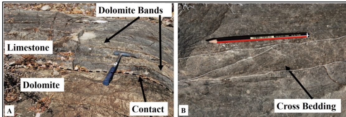
Figure 3.22 Photographs of the grey limestone. A) Contact between the limestone and the underlying pyritic dolomite. The grey limestone has dolomite bands close to its contact with the pyritic dolomite. Grid reference: 760059 mE, 7814656 mN. B) Cross-bedding in the grey limestone. Grid reference: 759832 mE, 7814629 mN. Geological hammer and pencil for scale in the photographs.
