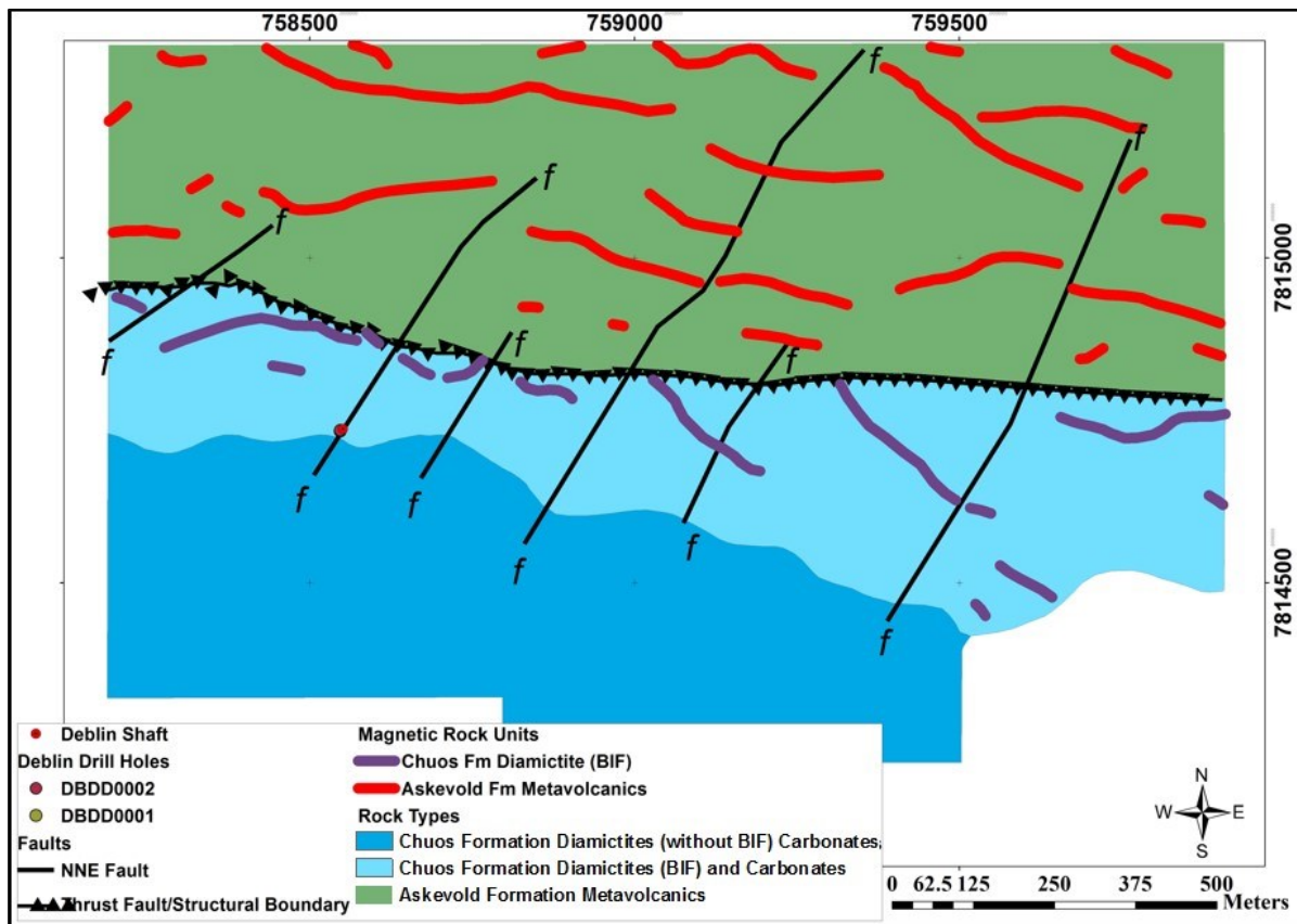
Figure 7.57 Interpreted solid geological map of the Deblin Copper Mine with the major east-west-trending thrust fault and shallow structural NE-trending faults.
