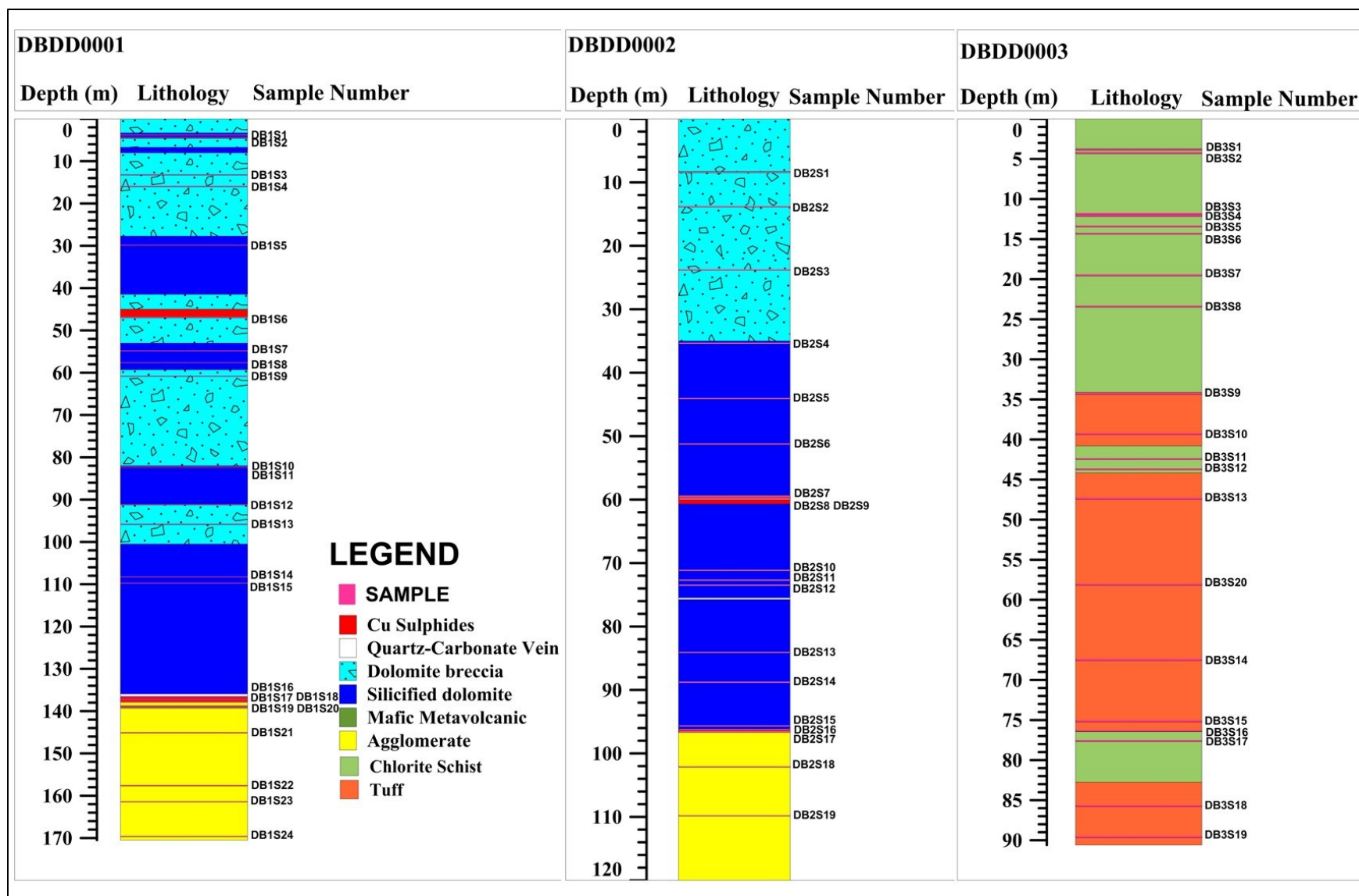
Figure 3.7 Lithological logs of the three boreholes (DBDD0001, DBDD0002 and DBDD0003) from the Deblin Copper Mine area showing sample localities.
