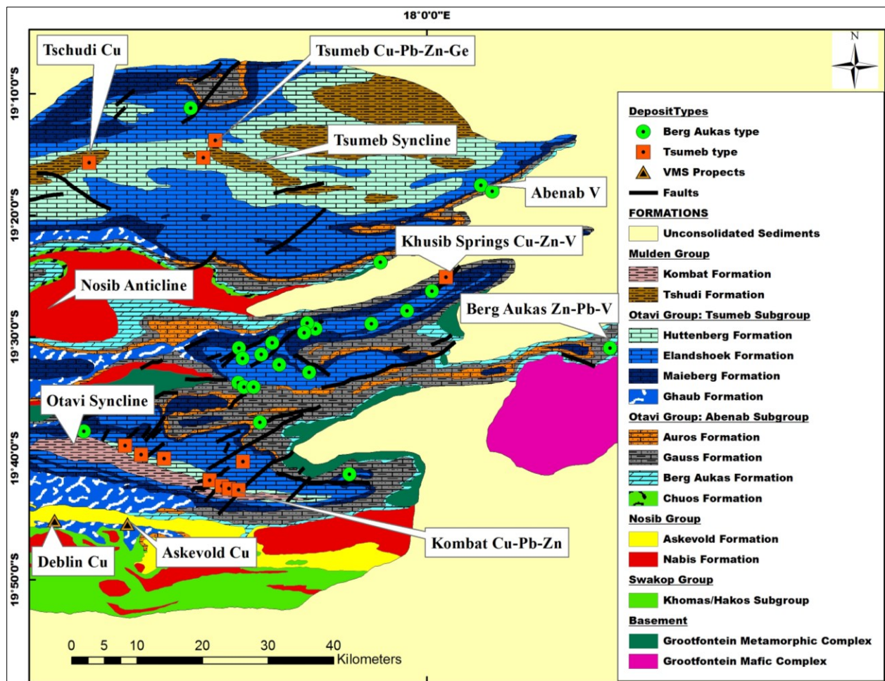
Figure 2.5 Geology of the Otavi Mountain Land with locations of major deposits and some prospects (modified after Söhnge, 1957; Kamona and Günzel, 2007 and map of 1:250,000 of the Geological Survey of Namibia). Generally, the Tsumeb type consists of sulphide ores containing Cu, Pb, Zn, Ag, As, Ge, Cd and Ga, whereas the Berg Aukas type contains primarily Pb-Zn and V sulphide ores with little Cu.
