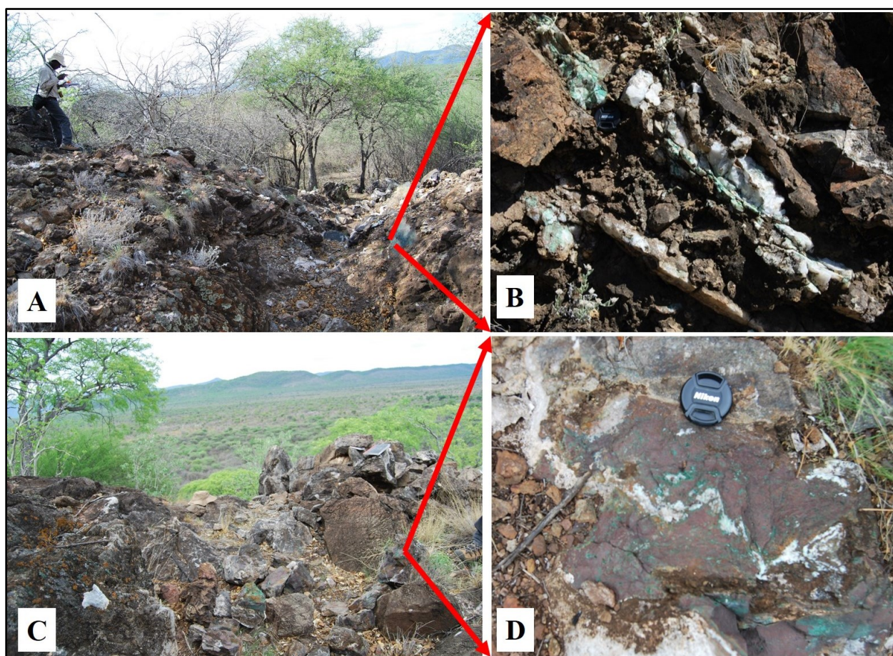
Figure 4.14 Field images of the exploration trenches showing supergene enrichment of malachite. A) A 20 m long, 4m wide and 1.5 to 2 m deep pink volcanic breccia exploration trench. B) Volcanic breccia outcrop with malachite in cross-cutting quartz veins. Grid reference: 758342 mE, 7815085 mN. C) A 12 m long, 5 m wide and ~8 m deep silicified dolomite exploration trench. D) Malachite and quartz-calcite veins hosted in a highly oxidized silicified dolomite. Grid reference 758747 mE, 7814817 mN.
