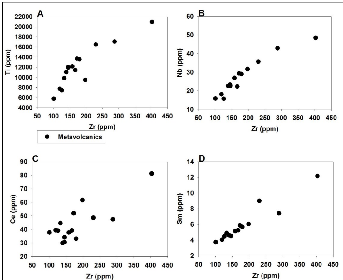
Figure 6.3 Bivariate graphs of Zr versus selected HFSE and REE showing positive correlations. A) The Zr vs Ti plot. B) The Zr vs Nb plot. C) The Zr vs Ce plot. D) The Zr vs Sm plot.
