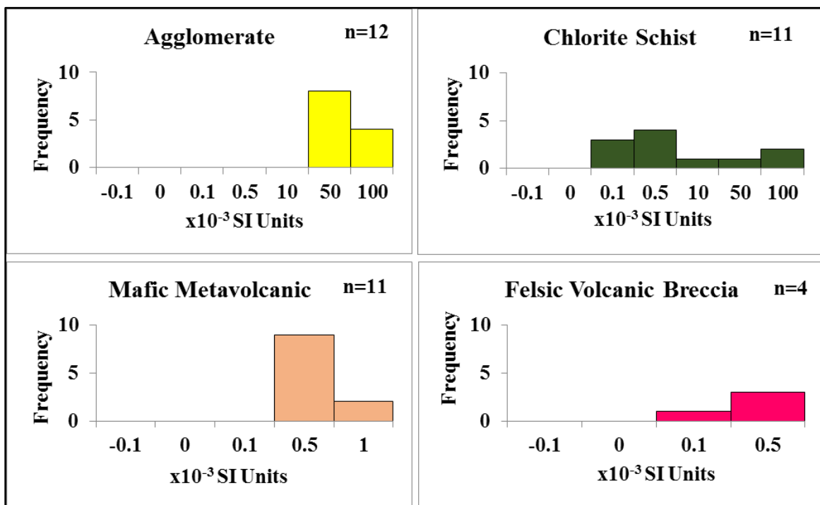
Figure 7.8 Histograms of in situ measured magnetic susceptibility data of the Askevold Formation lithologies.
