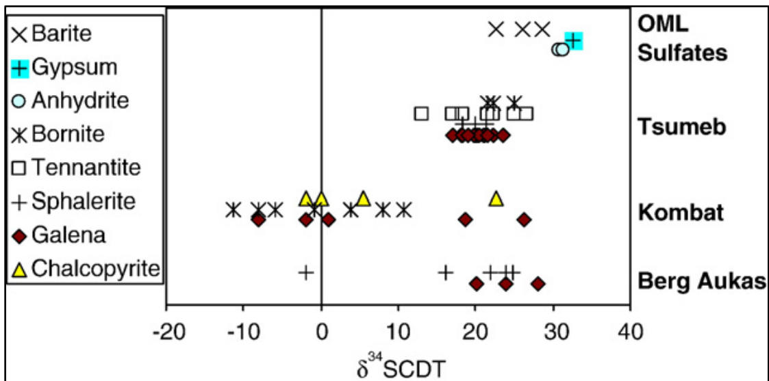
Figure 5.1 Sulphur isotope ratios ( \delta^{34}\text{S}_{\text{CDT}} ) in sulphides and sulphate of the major deposits in the Otavi Mountain Land (OML). Taken from Kamona and Günzel (2007).
