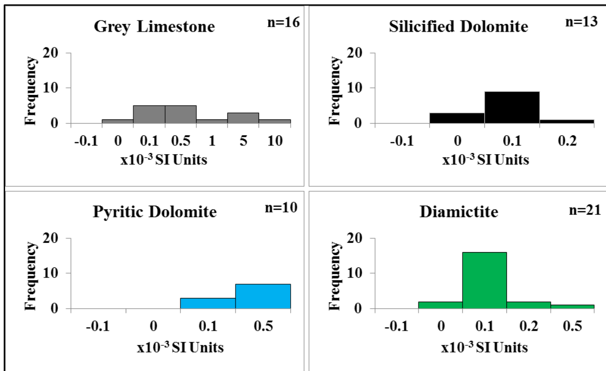
Figure 7.12 Histograms of in situ measured magnetic susceptibility data of the Chuos Formation lithologies.
