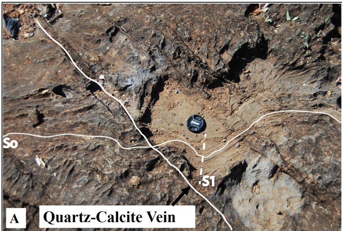
Figure 3.23 Banded limestone outcrop showing microfolds cross-cut by quartz-calcite veins. Grid reference: 759548 mE; 7814447 mN. Camera lens cover used for scale in the photograph.
