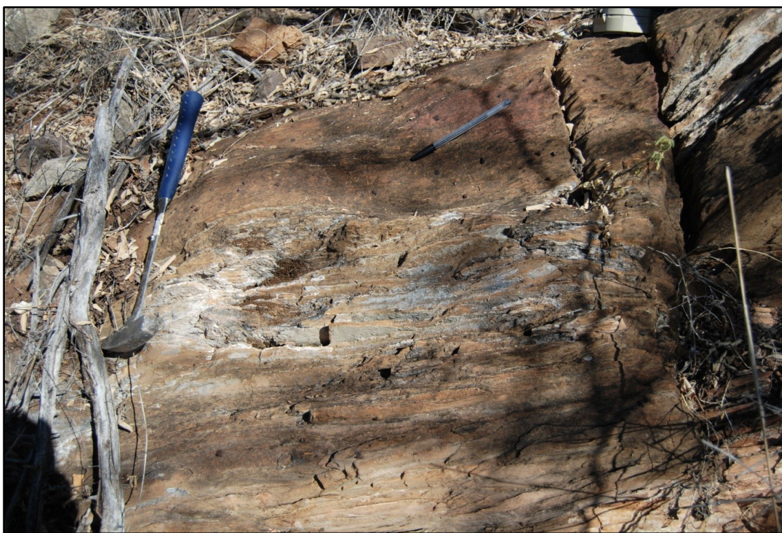
Figure 3.24 Intensely-weathered calcareous phyllite with brown oxidized idiomorphic cubic pyrite grains. Grid reference: 759985mE; 7814520mN. Geological hammer for scale in the photograph.
