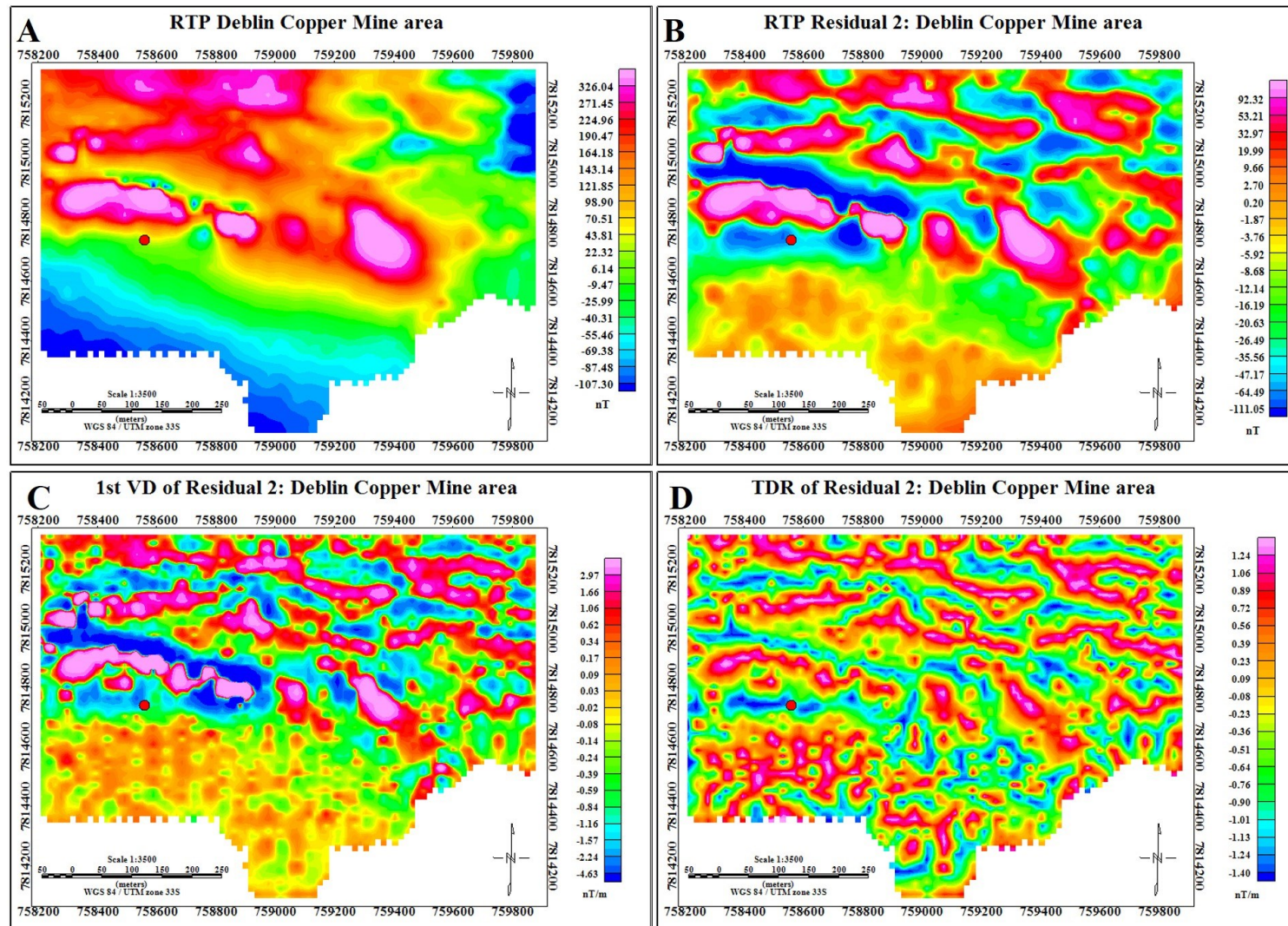
Figure 7.53 Residual filter applied to the ground magnetic data of the Deblin Copper Mine area. A) RTP map showing the total magnetic field of all the shallow and deep underground magnetic sources; B) Residual magnetic field map showing magnetic response of shallow seated sources; C) 1 st VD of the residual magnetic field showing shallow linear structures; D) TDR of the residual magnetic field showing shallow linear structures with a high resolution.
