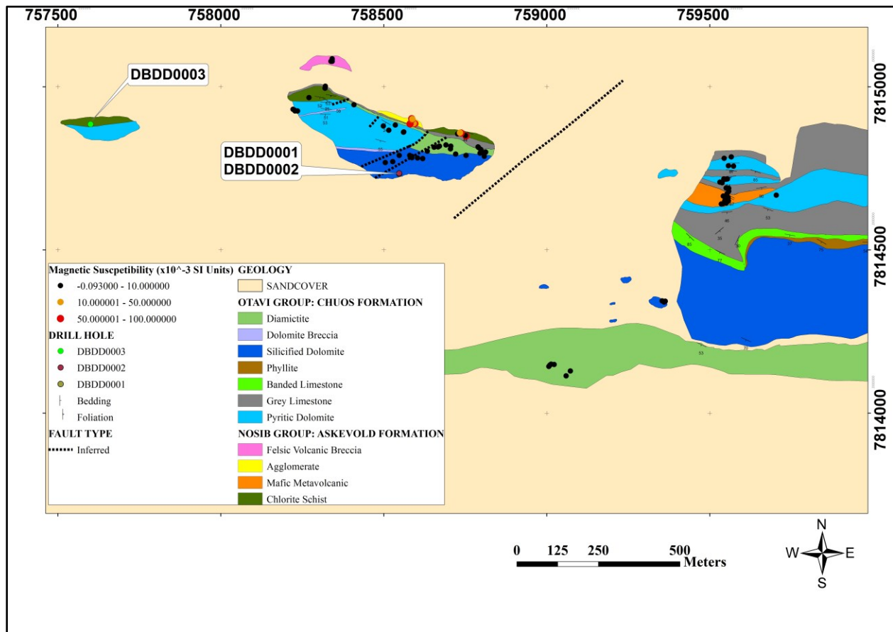
Figure 7.7 Detailed geological map of the Deblin Copper Mine area showing the distribution of the magnetic susceptibility values of different rock types.
