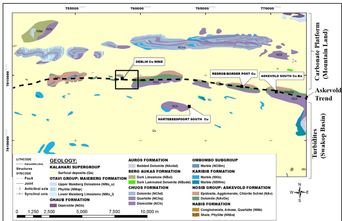
Figure 3.1 Regional geological map of the southern Otavi Mountain Land with the Askevold Trend defined by Cu prospects closely related to the Askevold Formation volcanics. Taken from the 1: 250,000 of the Geological Survey of Namibia (2008). The black dotted line indicates the Askevold Trend. The black box shows the local study area (Figure 3.4).
