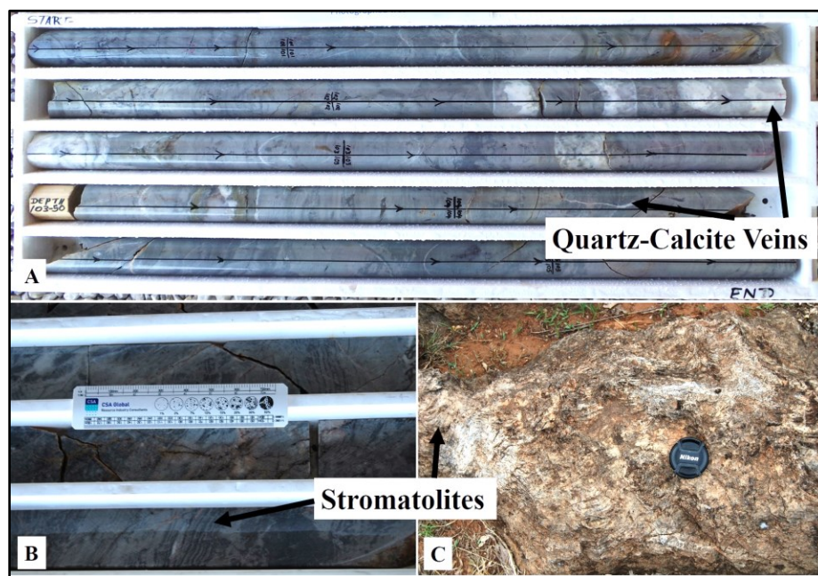
Figure 3.25 Images of the silicified dolomite in drill cores and outcrop. A) Silicified dolomite with outstanding thin and thick quartz-calcite veins. DBDD0001: 100.65 m – 105.31 m depth. B) Stromatolites in the silicified dolomite drill cores. DBDD0001: 117.00 m – 119.00 m depth. C) Silicified dolomite outcrop with deformed stromatolites and brown weathering colour. Grid reference: 759363 mE, 7814342 mN. Camera lens cover and ruler for scale in the photograph.
