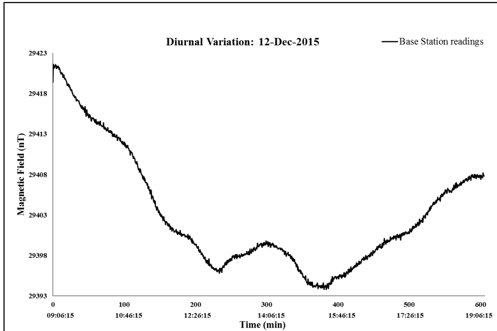
Figure 7.34 Diurnal variation plot for day 2. The Julian day is 346. The survey lasted for 605 minutes.
