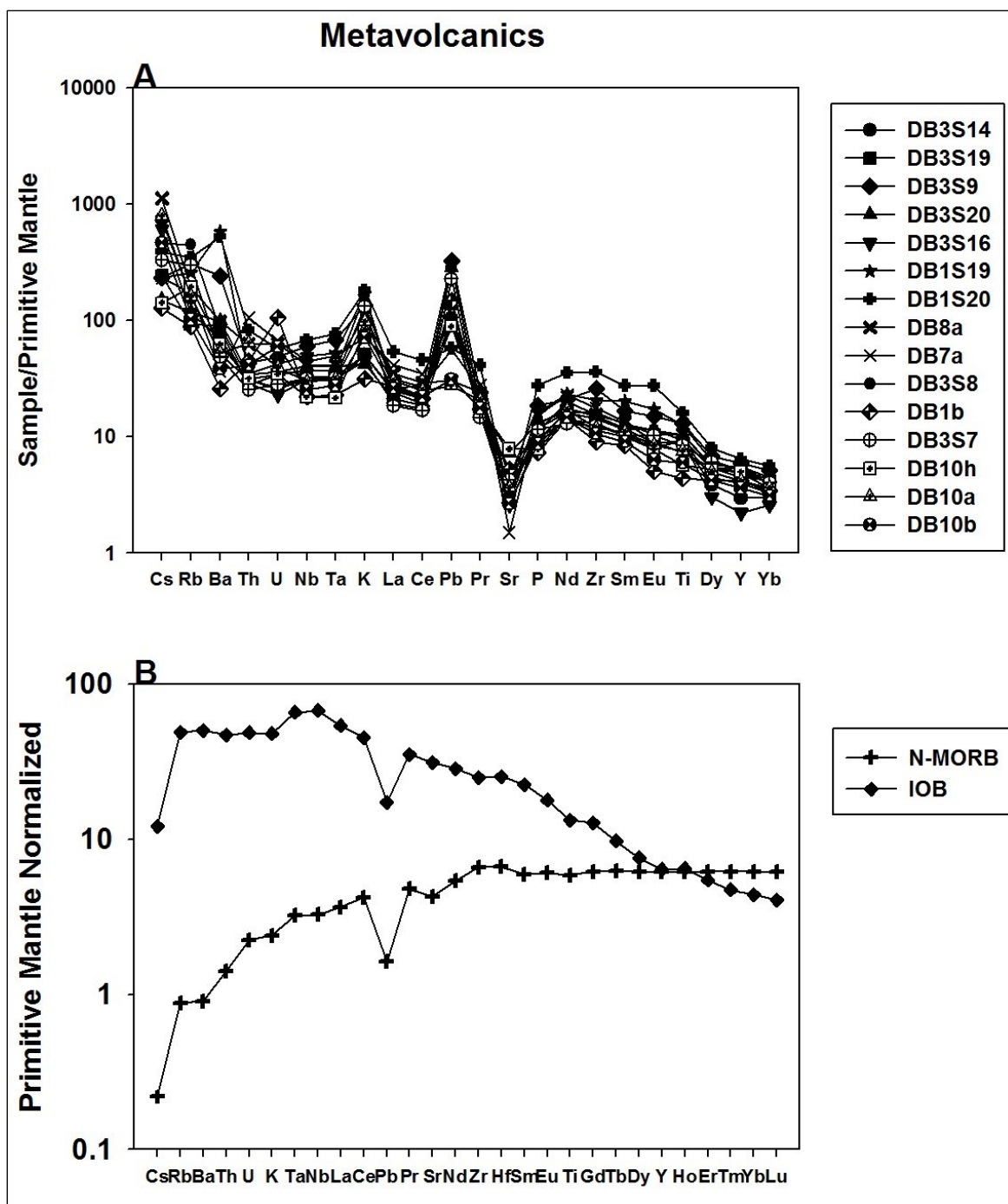
Figure 6.6 Primitive mantle-normalized spider diagrams. A) Primitive mantle-normalized multi-element patterns of the metavolcanic samples from the area around the Deblin Copper Mine. B) A comparison of the primitive mantle-normalized spider diagrams of the N-MORB and Oceanic Island Basalts (OIB) average values. All normalization values and the order of the elements are taken from Sun and McDonough (1989).
