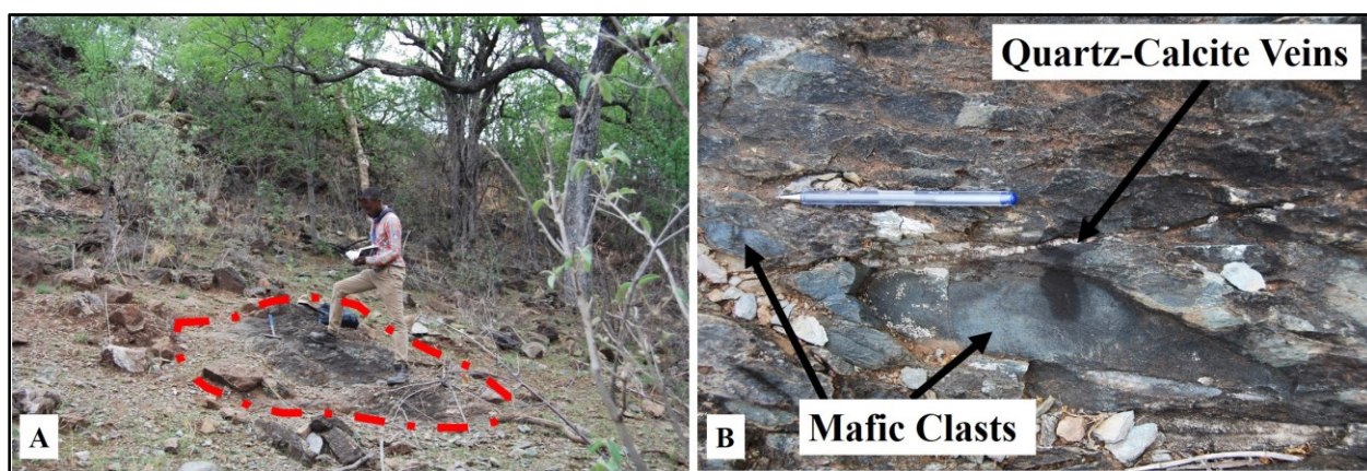
Figure 3.17 Field photographs of the agglomerate outcrop (5 x 4 m). Grid reference: 758747 mE, 7814817 mN. A) Poorly exposed agglomerate outlined in red. This unit is concealed by younger sediments. B) Deformed mafic clasts of the agglomerate that are elongated along strike. The pen for scale in the centre of the photograph.
