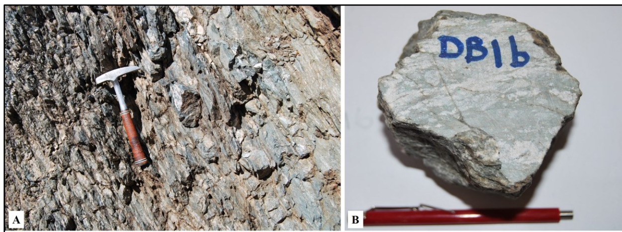
Figure 3.13 Photographs of the chlorite schist. Grid reference: 758343 mE; 781477 mN. A) Chlorite schist exposed in the exploration trench. Geological hammer for scale in the photograph. B) Hand specimen of the chlorite schist with flecks of malachite and ubiquitous quartz-calcite veins, DB1b. Magnetic pen for scale in the photograph.
