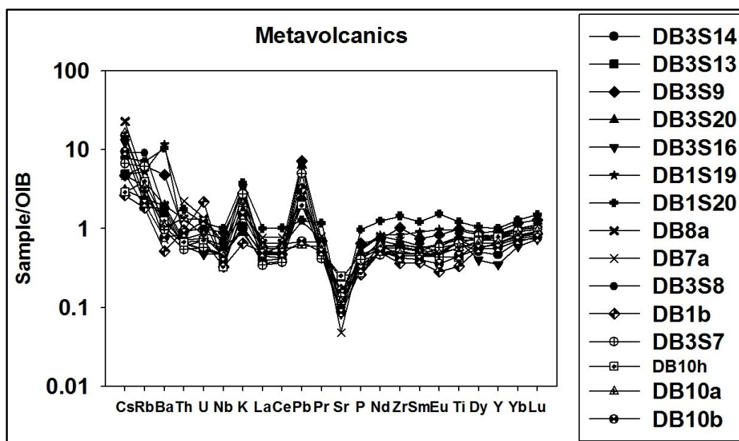
Figure 6.7 Oceanic Island Basalt (OIB)-normalized multi-element patterns of the metavolcanic samples from the area around the Deblin Copper Mine. Normalization values and the order of the elements are taken from Sun and McDonough (1989).
