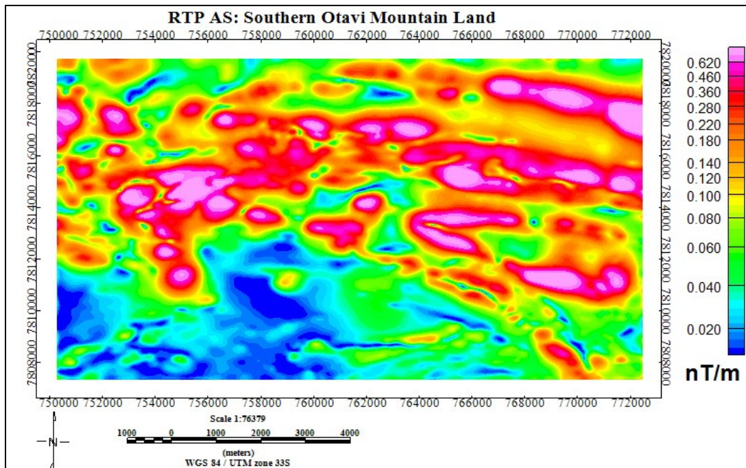
Figure 7.22 Processed AS map showing the edges of the magnetic bodies. Please note that the geological continuity is destroyed.
