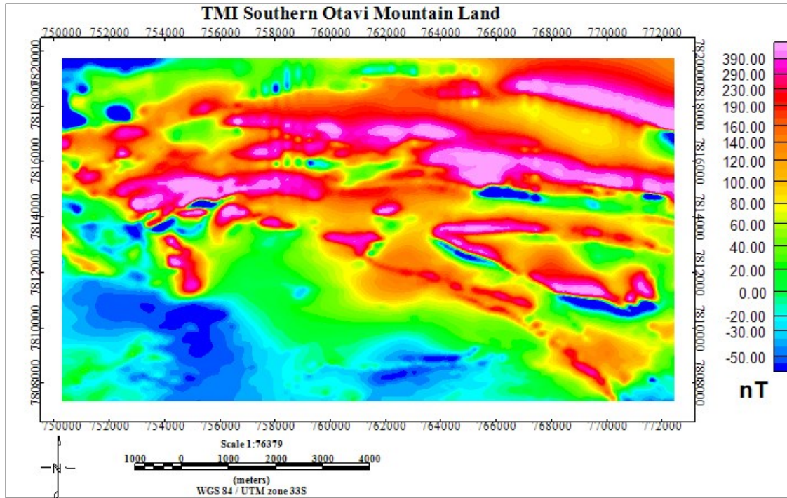
Figure 7.14 TMI map of the aeromagnetic data of the southern Otavi Mountain Land (OML).
