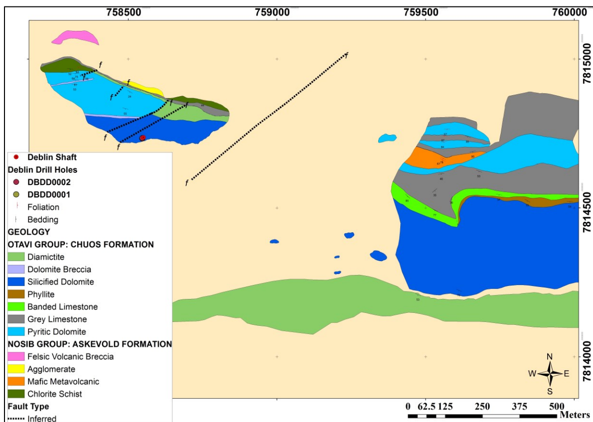
Figure 7.54 Detailed geological map of the Deblin Copper Mine showing the extensive sand cover, rock outcrops and inferred structures.
