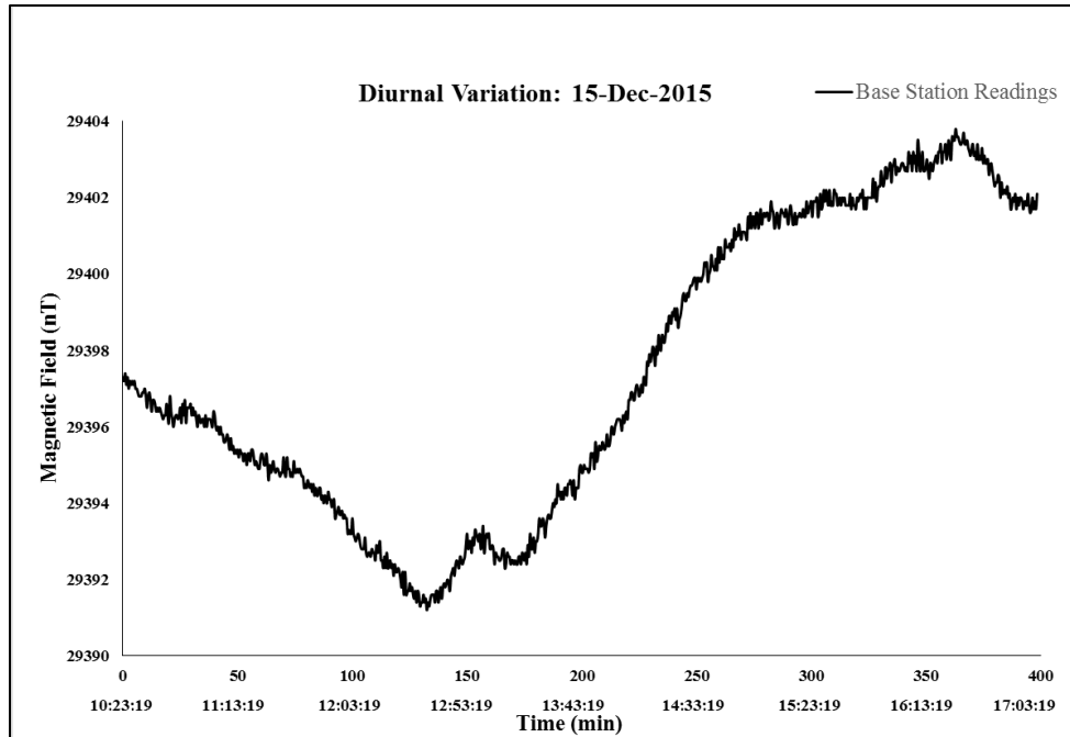
Figure 7.37 Diurnal variation plot for day 5. The Julian day is 349. The survey lasted for 398.5 minutes.
