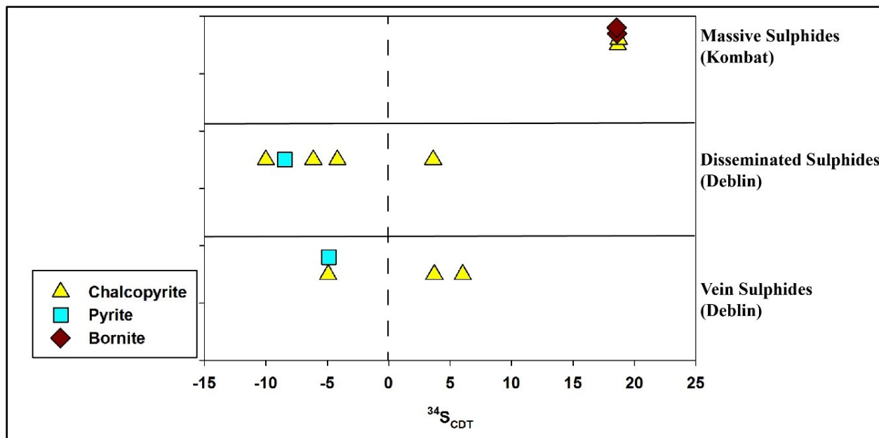
Figure 5.2 Variation of sulphur isotope ratios ( \delta^{34}\text{S}_{\text{CDT}} ) in sulphides of the Deblin Copper Mine and Kombat deposit.
