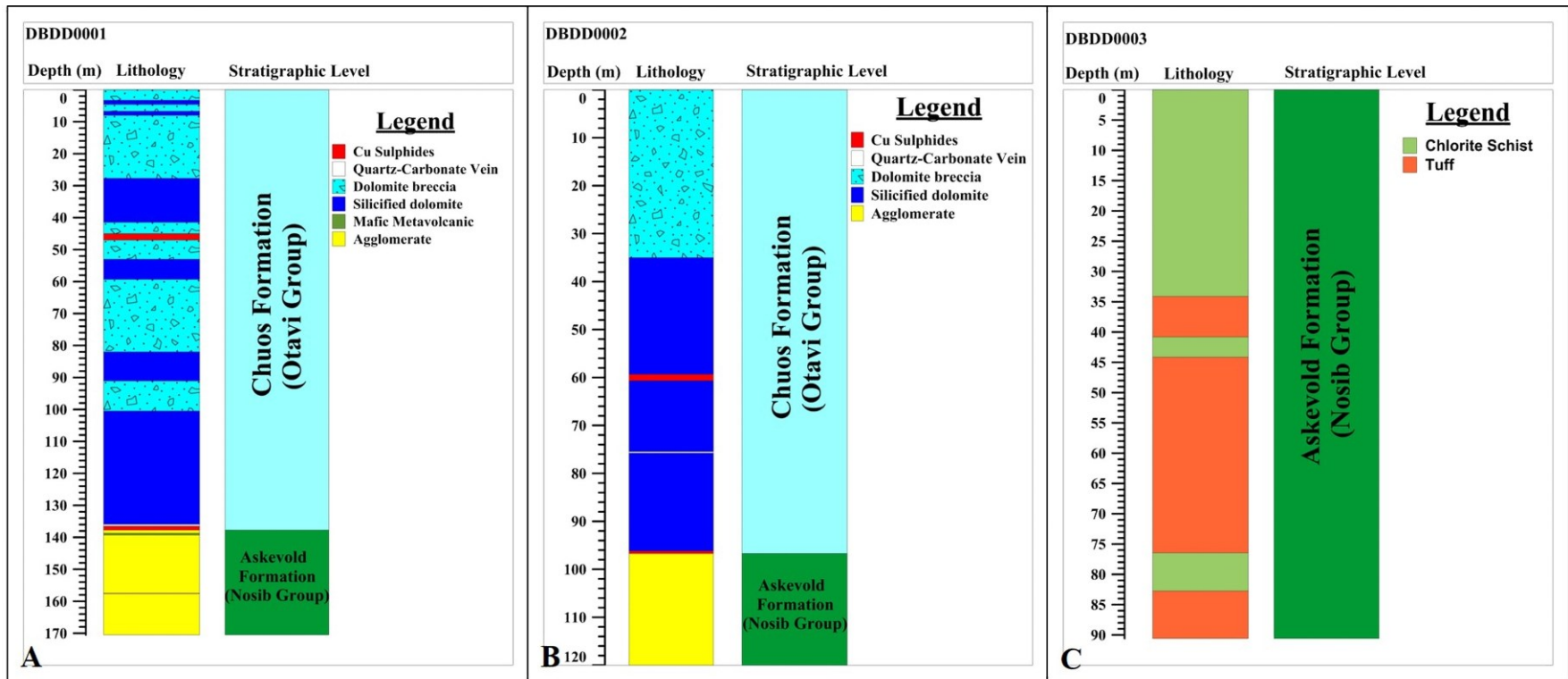
Figure 3.5 Lithological logs of the three boreholes from the Deblin Copper Mine area. A) DBDD0001 lithological log showing the succession of both the Nosib Group metavolcanic rocks and Otavi Group dolomites, and the location of the copper sulphide mineralization in the stratigraphy. Grid reference: 758547 mE, 7814734 mN. B) DBDD0002 lithological log showing the succession of both the Nosib Group metavolcanic rocks and Otavi Group dolomites, and the location of the copper sulphide mineralization in the stratigraphy. Grid reference: 758547 mE, 7814735 mN. C) DBDD0002 lithological log. This borehole intersected solely the Nosib Group metavolcanic rocks. Note the lack of a mineralized unit. Grid reference: 757600 mE, 7814885 mN.
