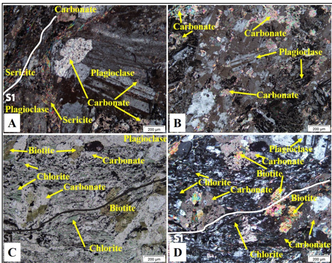
Figure 3.12 More observations of calcite overgrowths over other mineral phases. A) Plagioclase overgrown by calcite and sericite (XPL). DBDD0003: 58.00 m – 58.20 m – DB3S20-D139a. B) Ubiquitous plagioclase replacement by calcite (XPL). DBDD0003: 34.20 m – 34.40 m – DB3S9-D130b. C) Chlorite overgrowth over the foliation, whereas biotite enclosed in a calcite grain is not altered (PPL) and D) same image in crossed-nicols (XPL) DBDD0003: 75.04 m – 75.24 m – DB3S15-D142c. The white and black lines defines S_1 . (XPL= crossed-polarized light; PPL= plane-polarized light).
