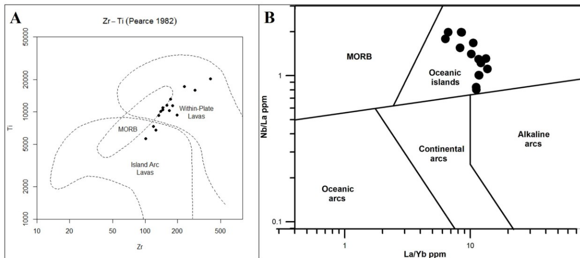
Figure 6.8 Basalt tectonic discrimination diagrams. A) The majority of the metavolcanic samples plot in the within-plate lavas field. B) Metavolcanic samples plot within the oceanic islands field on the La/Yb-Nb/La diagram of Hollocher et al. (2012).
