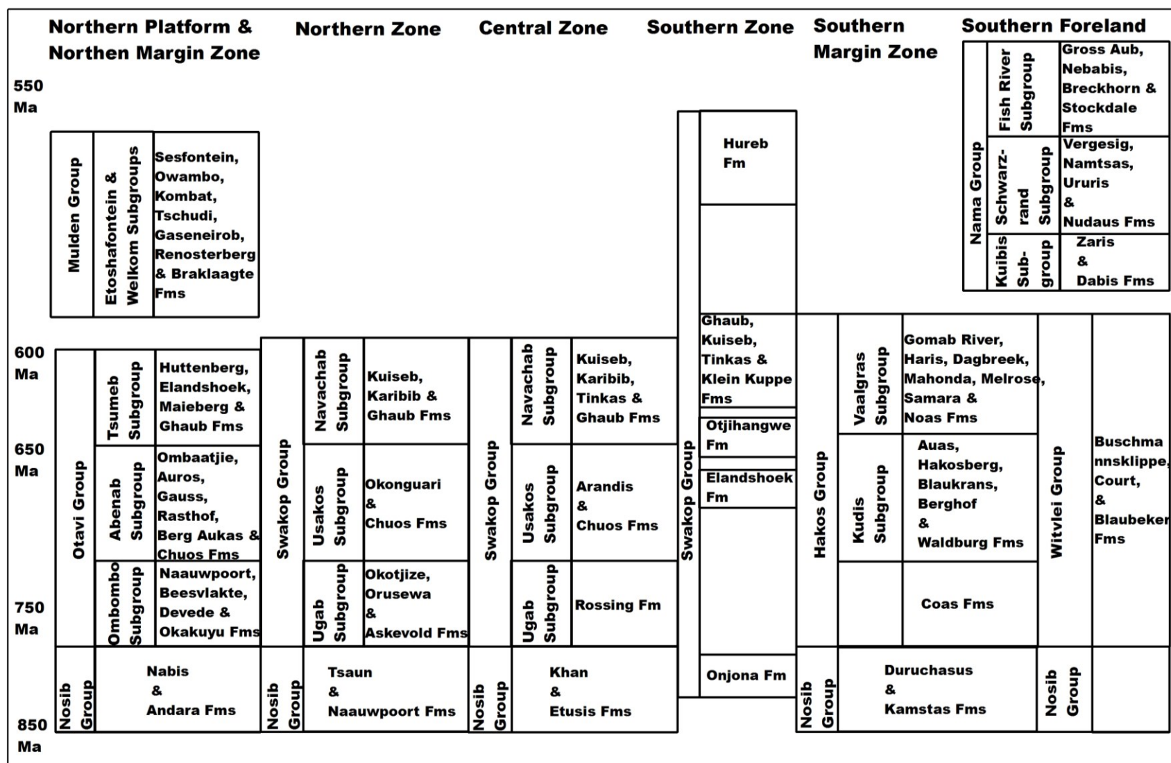
Figure 2.3 Lithostratigraphy and correlation across the Damara Belt with approximate deposition age for the Damara Sequence (modified after Miller, 2008). The vertical thickness of the sequence is not to scale.
