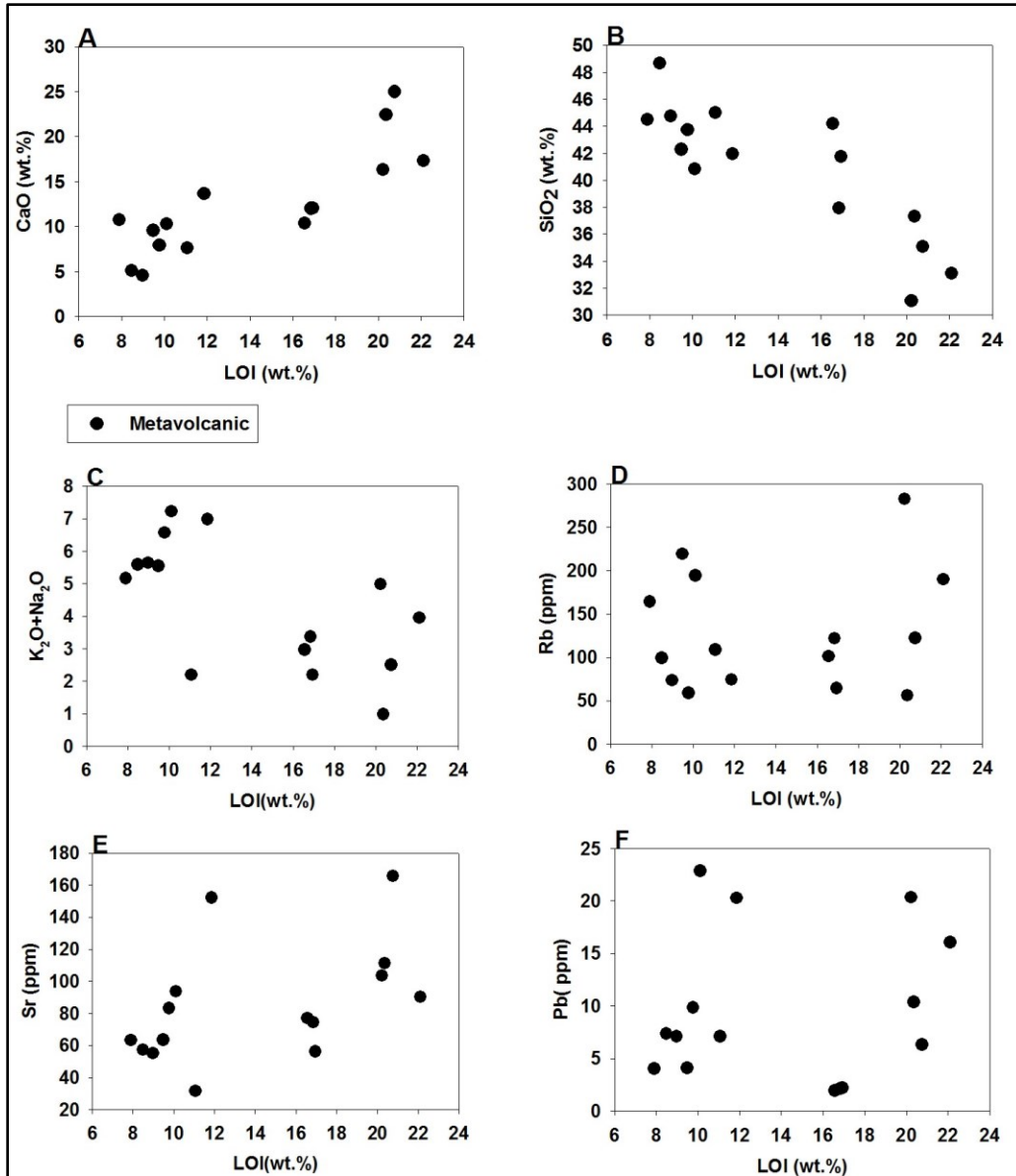
Figure 6.1 Bivariate plots of Loss on Ignition (LOI) versus selected major elements and Large Ion Lithophile Elements (LILE). The Rb, Sr and Pb plots do not show any correlations. A) The plot of the Loss on Ignition with CaO displays a positive trend. B) The Loss on Ignition vs SiO 2 exhibits a negative trend. C) The LOI vs total alkali content (K 2 O+Na 2 O) plot. D) The LOI vs Rb plot. E) The LOI vs Sr plot. F) The LOI vs Pb plot.
