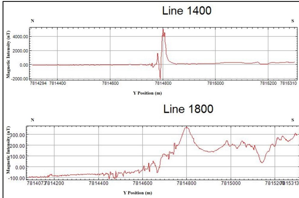
Figure 7.41 Profiles of the selected survey lines: Line 1400 and 1800.
