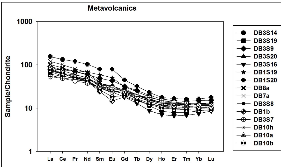
Figure 6.4 Chondrite-normalized REE patterns of the metavolcanic samples from the area around the Deblin Copper Mine, with subtle positive and negative Eu anomalies. Normalization values and the order of the elements are taken from Sun and McDonough (1989).
