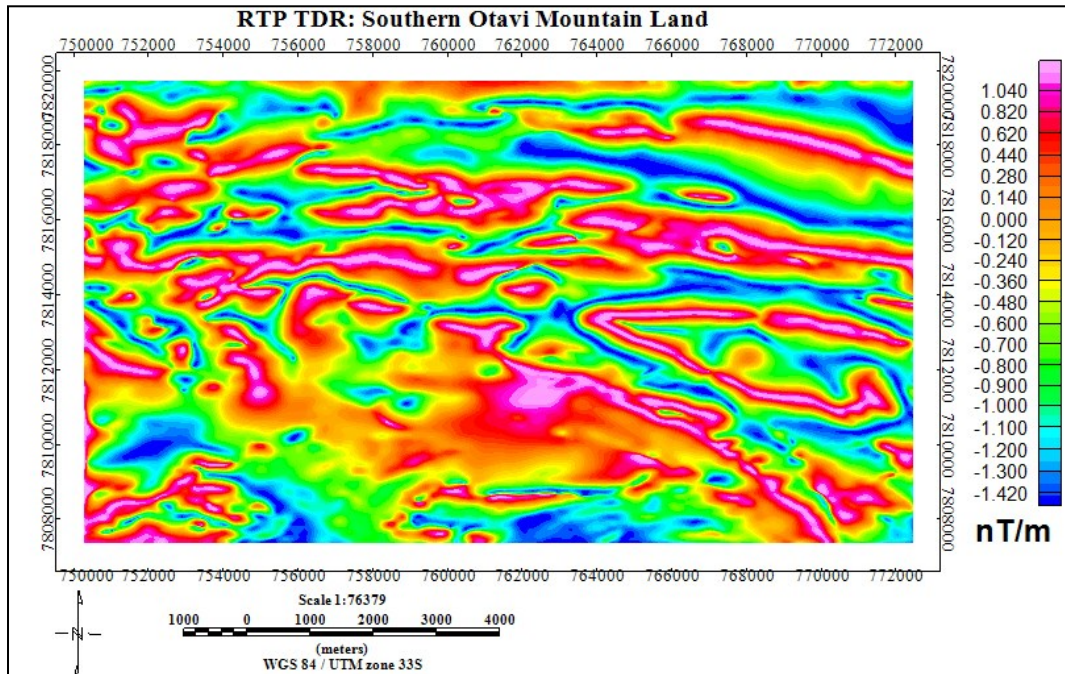
Figure 7.20 Processed TDR map showing shallow crustal features.
