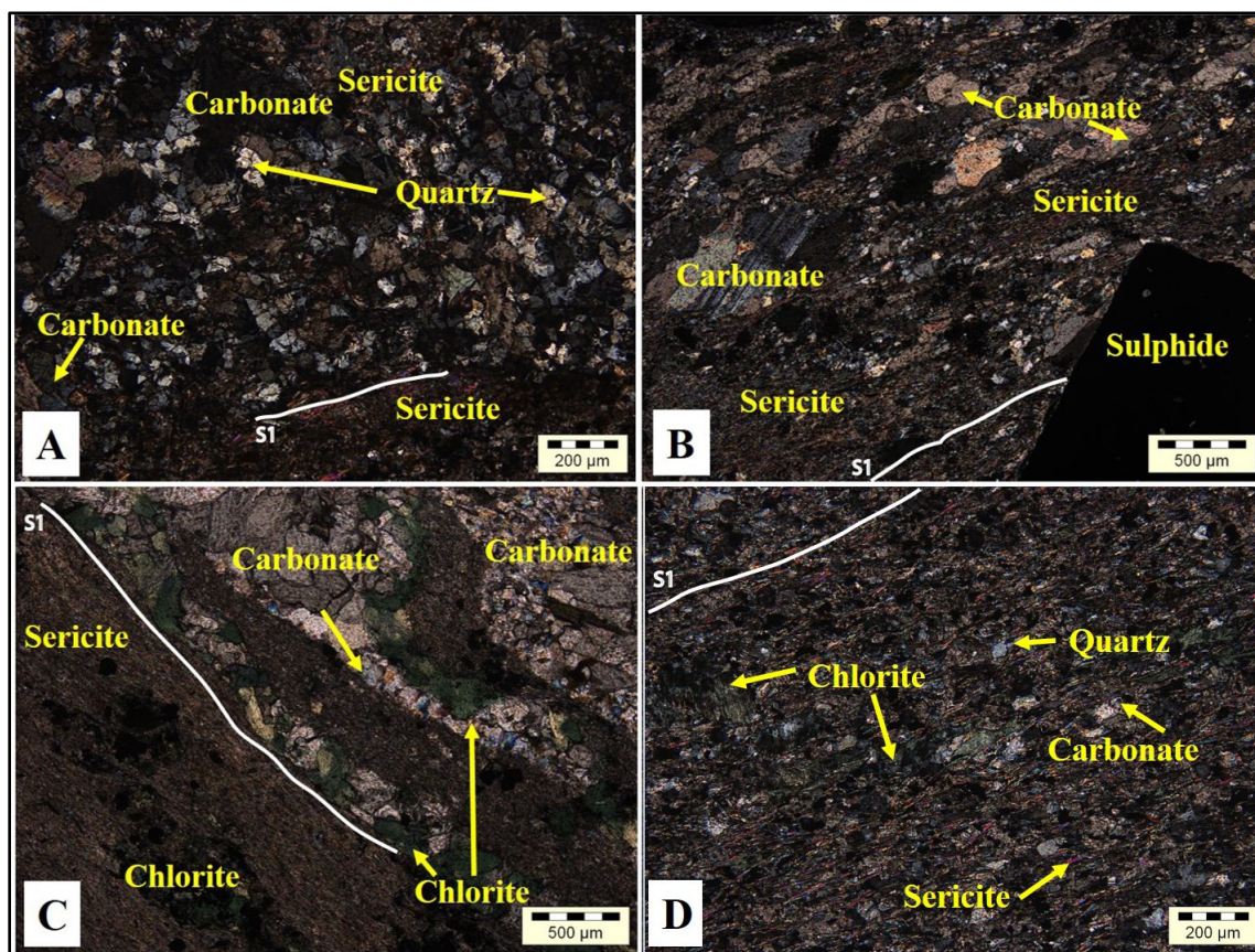
Figure 3.16 Mineral assemblage of the mafic metavolcanic rock. A) Fine-grained carbonate and quartz grains constitute the microlithon, whereas sericite makes up the cleavage domain of the foliation observed in this sample (XPL). Grid reference: 759552 mE; 7814663 mN – DB8a-D33b. B) Carbonate overgrowth on sericite in the cleavage domain (XPL). DBDD0001: 138.10 m – 138.30 m - DB1S20-D30a. C) Chlorite overgrows both the disjunctive foliation (sericite) and quartz-calcite veins (XPL). DBDD0001: 138.10 m – 138.30 m - DB1S20-D80a. D) Chlorite overprinting the foliation ( S_1 ) and other mineral phases (XPL). DB10a-40a. The white line defines S_1 . (XPL= crossed-polarized light; PPL= plane-polarized light).
