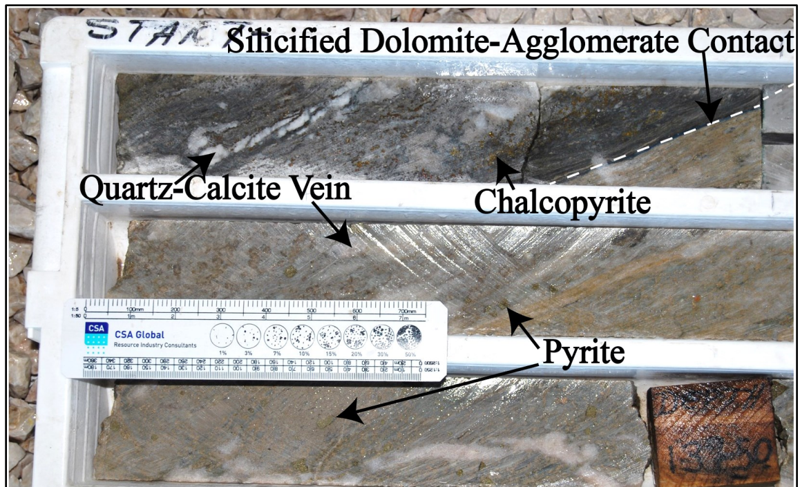
Figure 4.5 Pyrite disseminations in the agglomerate below the contact and vein type mineralization with chalcopyrite in the silicified dolomite above the contact. DBDD0001: 137.41 m – 139.50 m. The quartz-calcite veins in the agglomerate are not mineralized.
