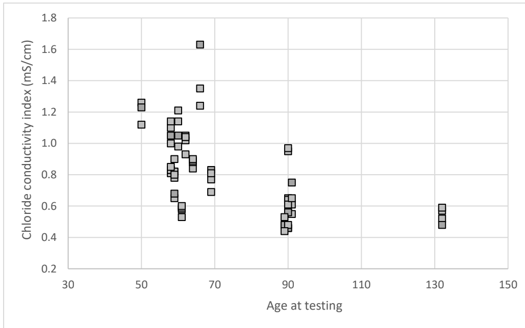
Figure 4-14 - Effect of age at testing in CCI
