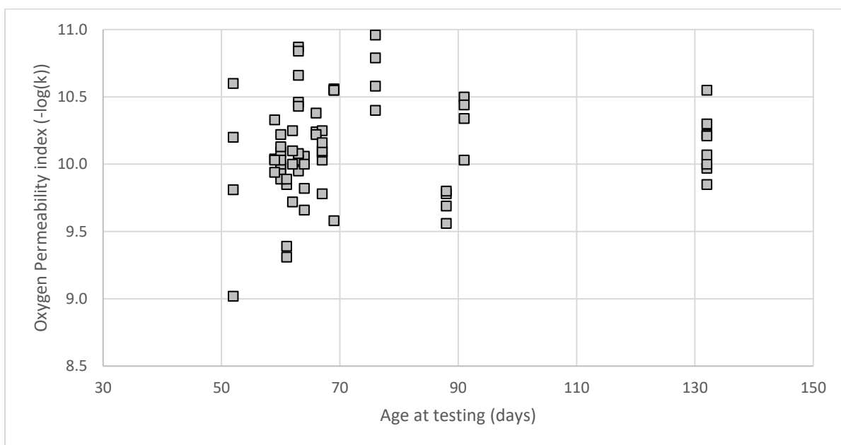
Figure 4-6 - Effect of age at testing on OPI
