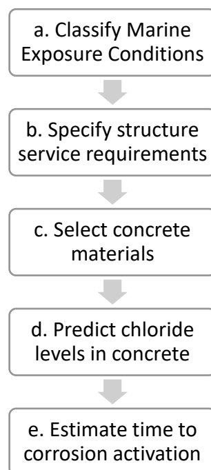
Figure 2-23- Flow diagram of design steps using the South African Chloride Ingress Model
