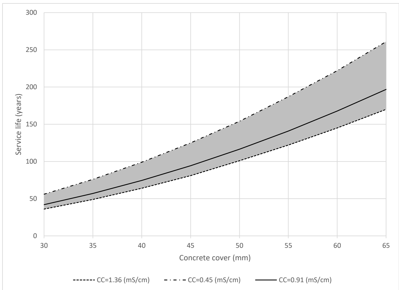
Figure 4-23 - Effect of concrete cover on service life
