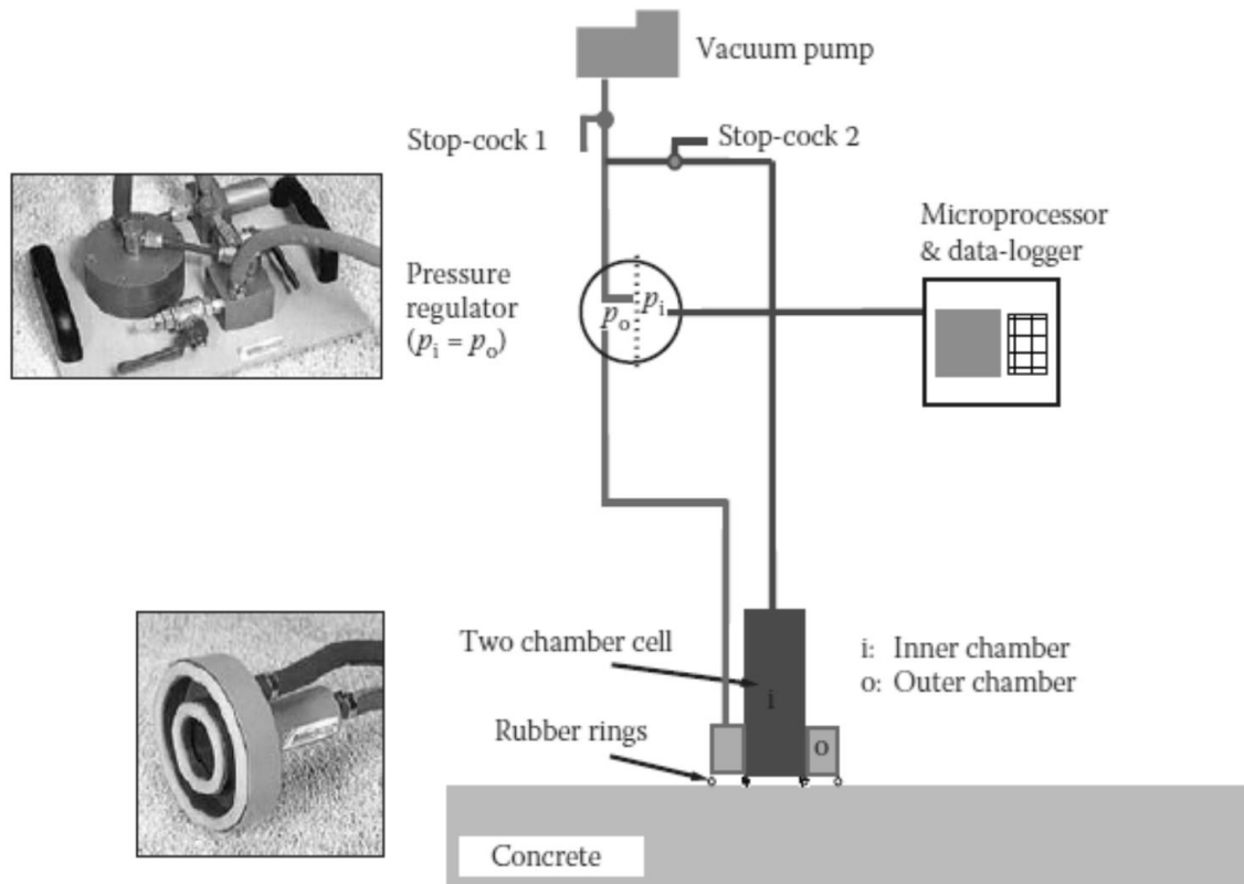
Figure 2-16 – Line Diagram of Torrent Permeability Test (Torrent, 1992)
