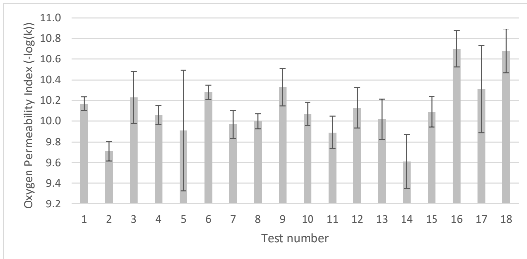
Figure 4-3 - Graphical summary of OPI results
