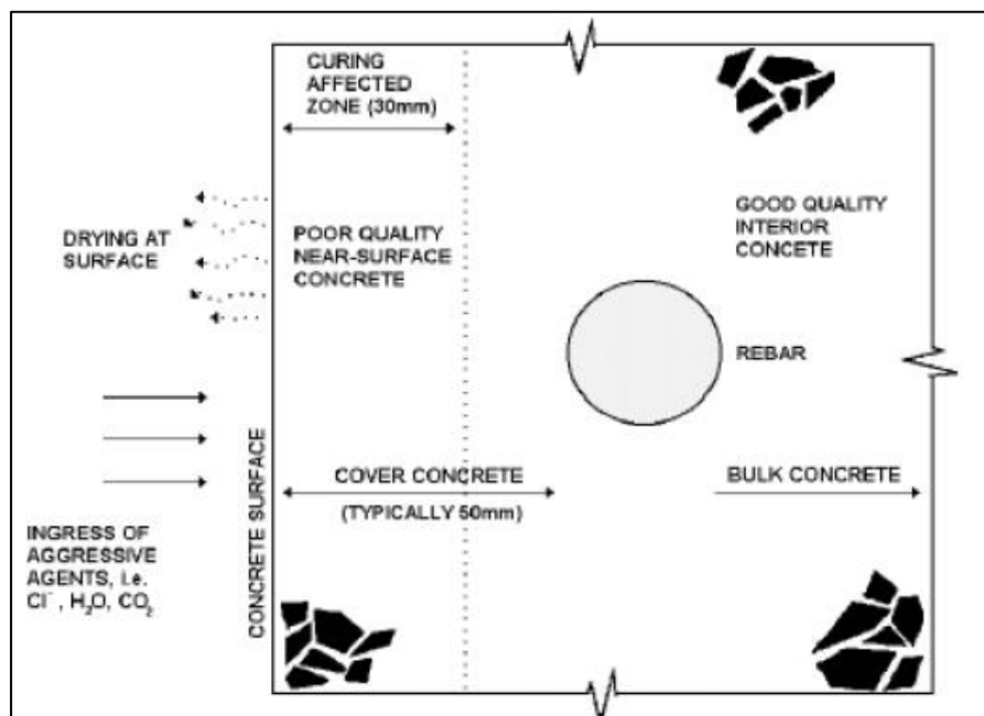
Figure 2-5 - Schematic of concrete cover layer (Alexander, 2004)
