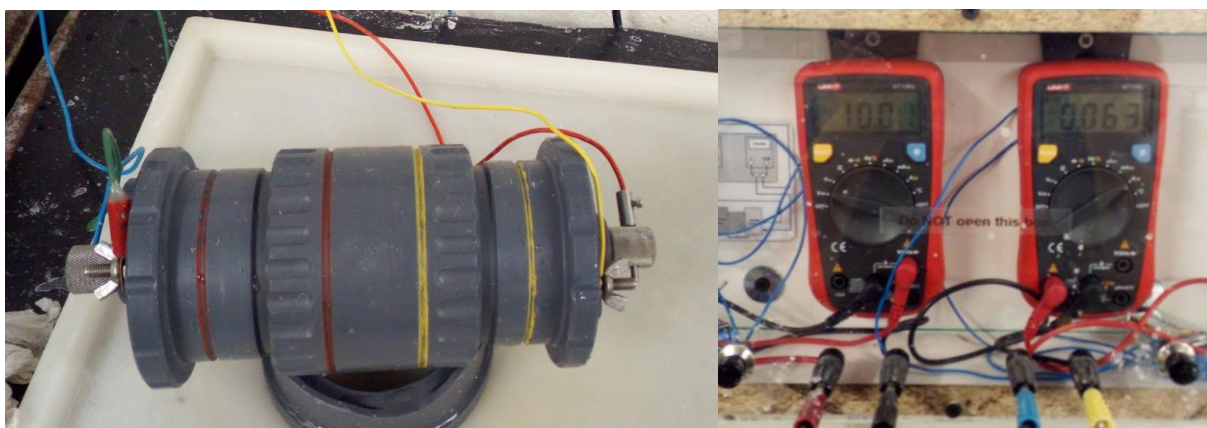
Figure 3-27 - CCI test set-up
