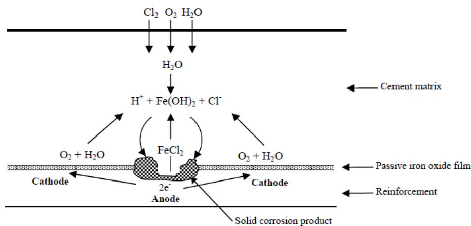
Figure 2-11 - Corrosion of reinforcement in concrete exposed to chloride ions (Broomfield, 2007)
