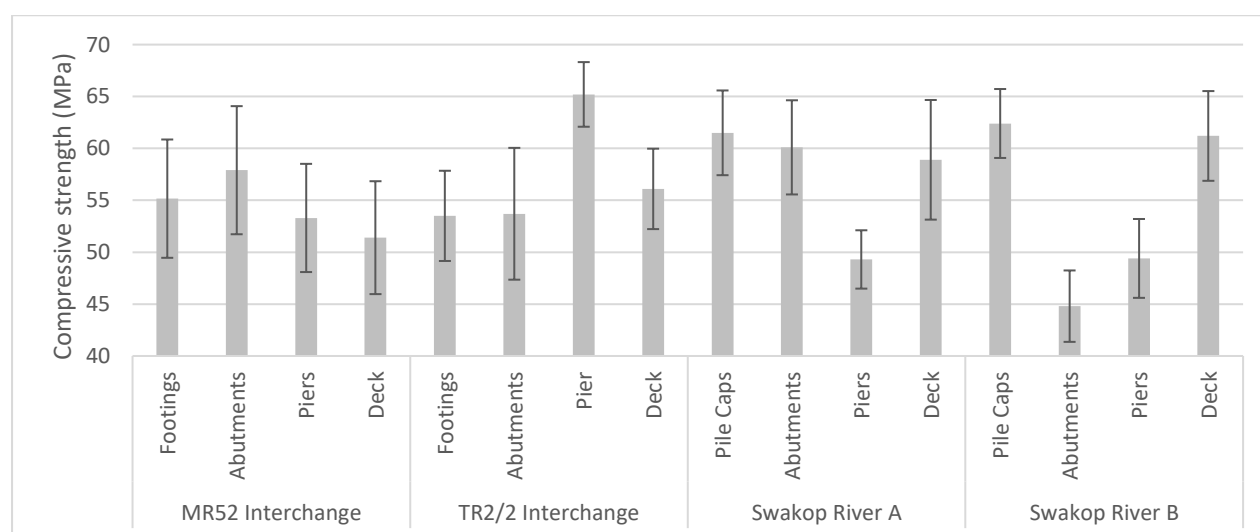
Figure 4-1 – Graphical summary of 28-day concrete strength results
