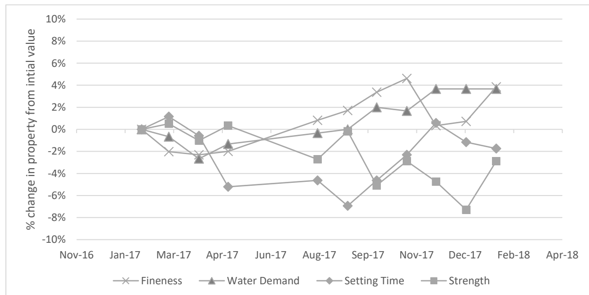
Figure 3-14 - Variation in cement properties over a year
