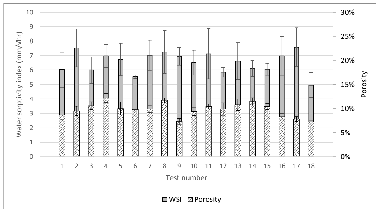
Figure 4-7 - Graphical summary of WSI and porosity result
