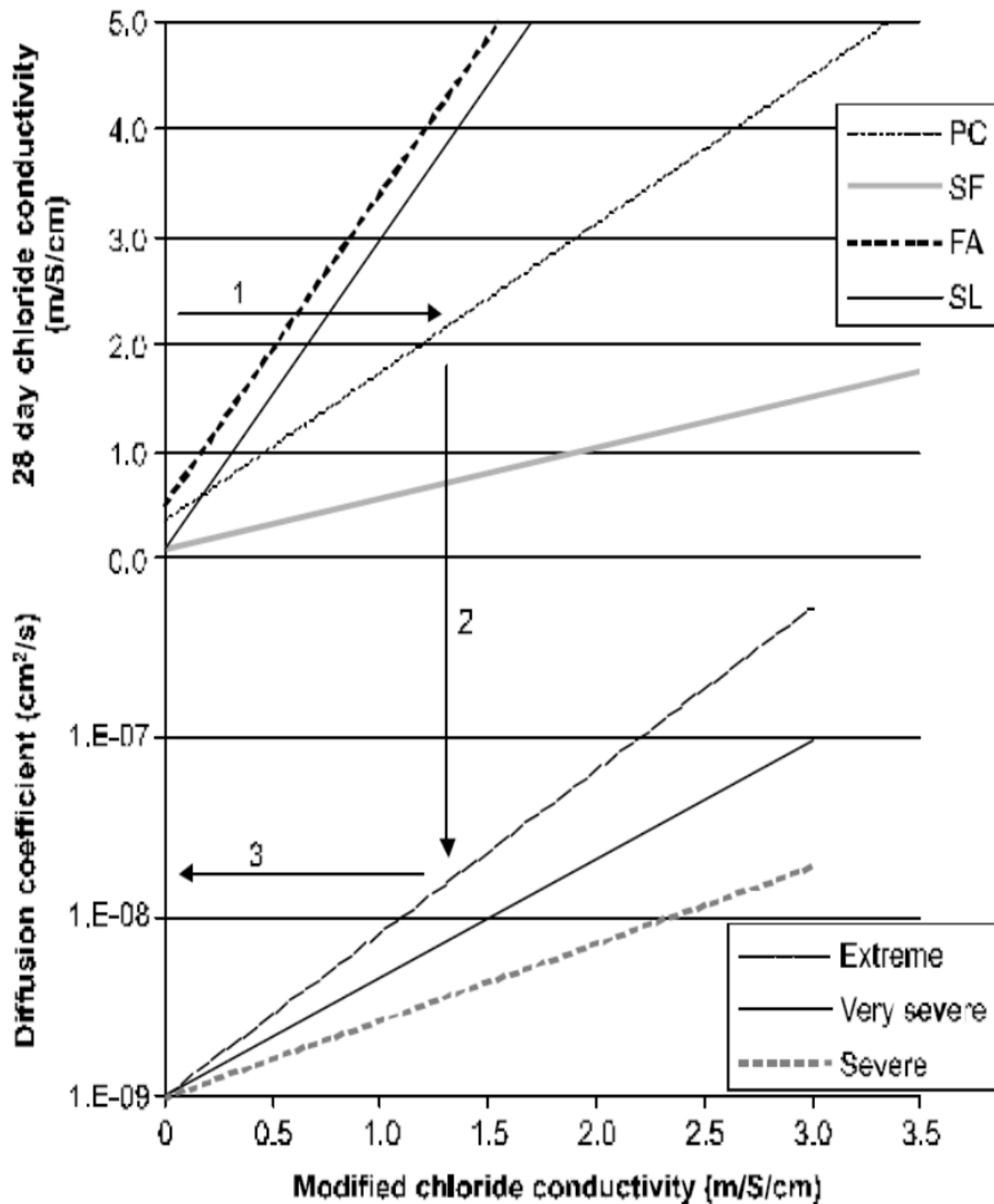
Figure 4-21 - Nomogram for the prediction of 50-year diffusion coefficient from chloride conductivity index
