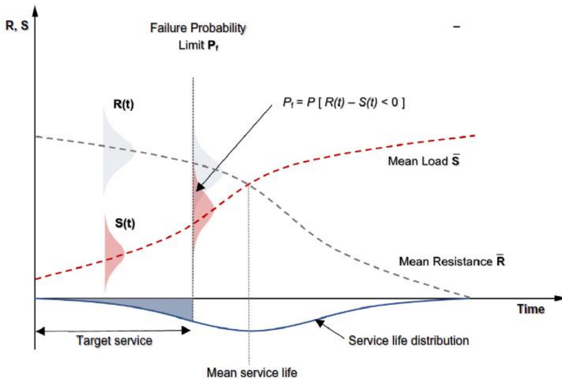
Figure 2-22 - Schematic representation of probabilistic service life design (Alexander & Beushausen, 2019)
