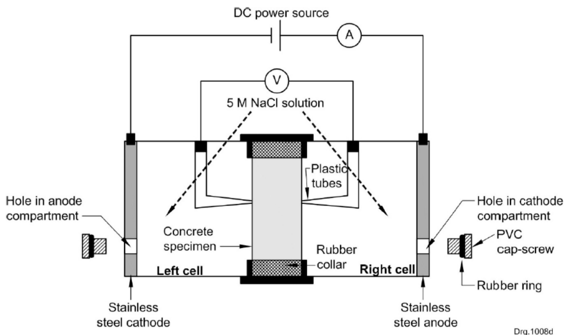
Figure 2-21 - Schematic of chloride conductivity cell (DI Testing Manual, 2018)
