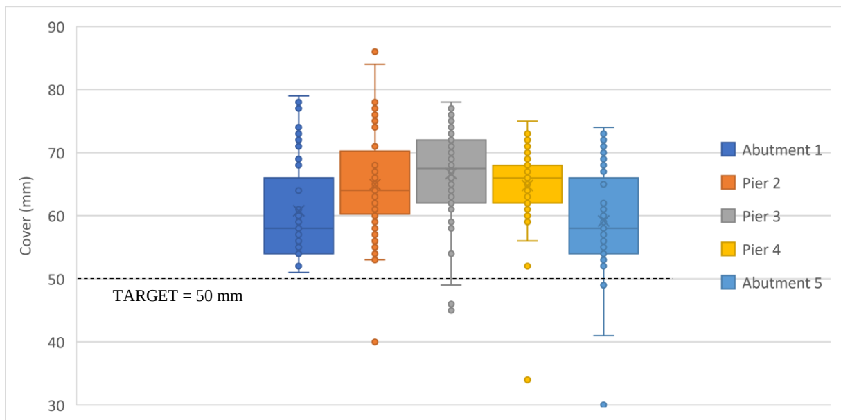
Figure 4-18 - Swakop River Bridge A cover readings - boxplot per element
