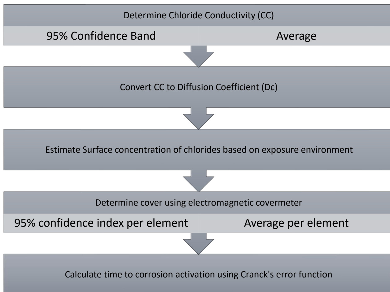
Figure 3-30 - Calculation of service life of structures
