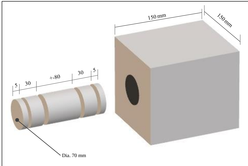
Figure 3-21 - Details of cores from 150 mm concrete cube
