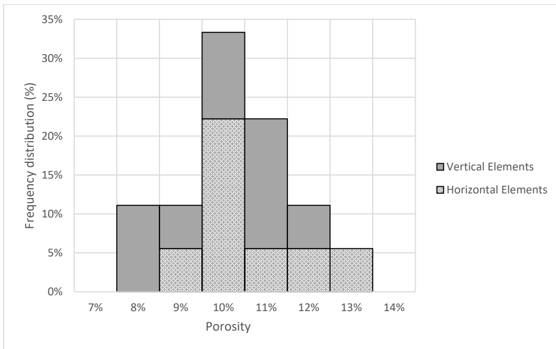
Figure 4-8 - Frequency distribution histogram for porosity results
