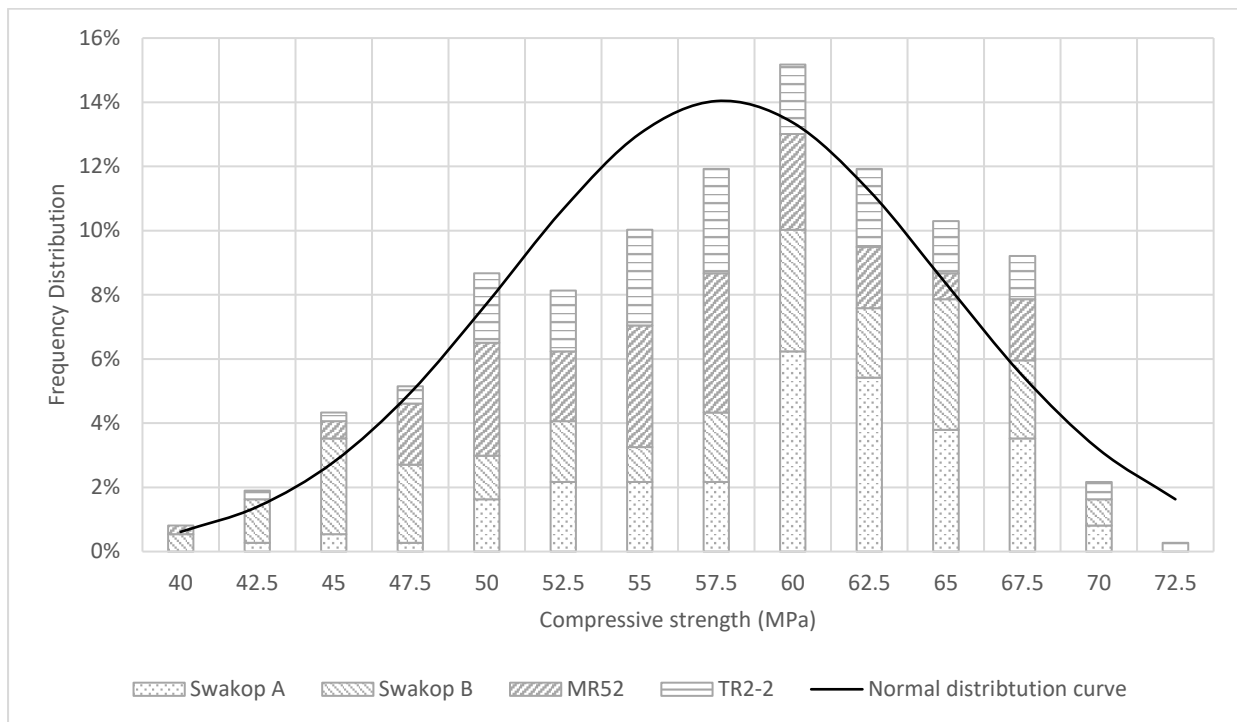
Figure 4-2 – Frequency distribution histogram of compressive strength for all bridges
