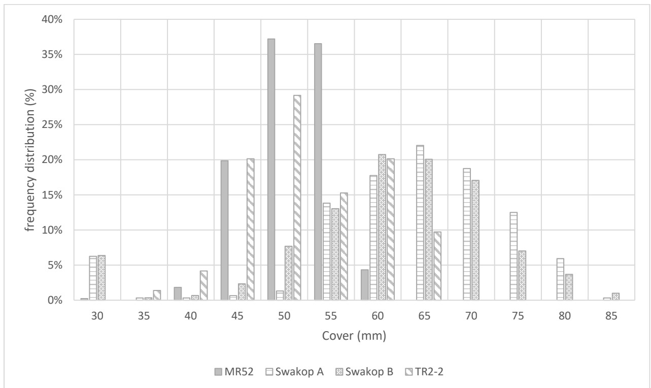
Figure 4-16 - Frequency distribution of cover readings for all bridges
