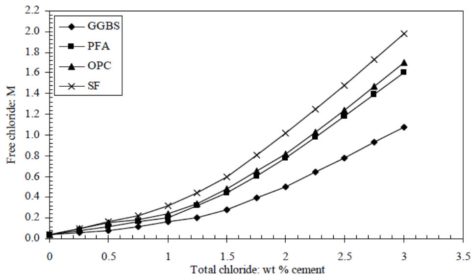
Figure 2-12 - Chloride binding relationships dependant on binder type and total concentration (Glass & Buenfield, 1997)
