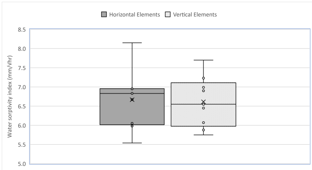
Figure 4-9 - Boxplot comparison of horizontal and vertical element WSI test results
