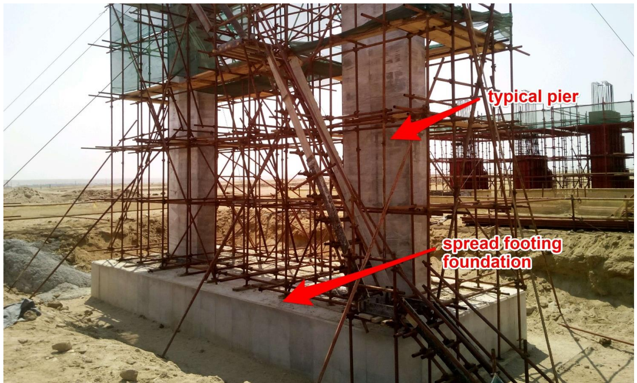
Figure 3-4 -Photograph of typical spread-footing foundations for interchange bridges
