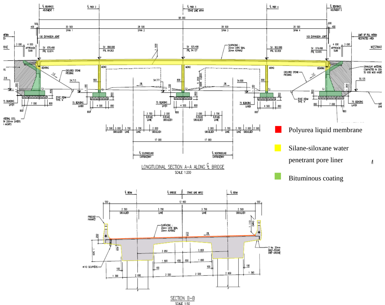
Figure 3-11 - Illustration of concrete protective coatings
