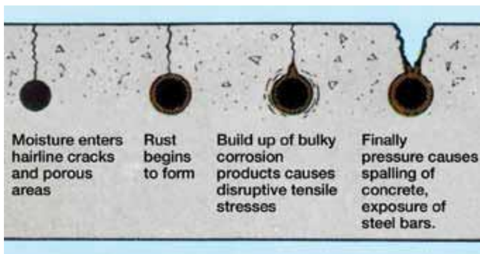
Figure 2-6 - The progress of corrosion-induced damage in concrete (Yeomans, 2017)
