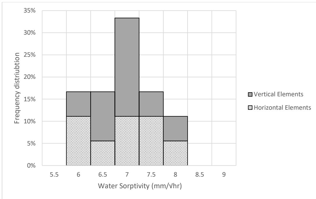
Figure 4-7 - Frequency distribution histogram for WSI results
