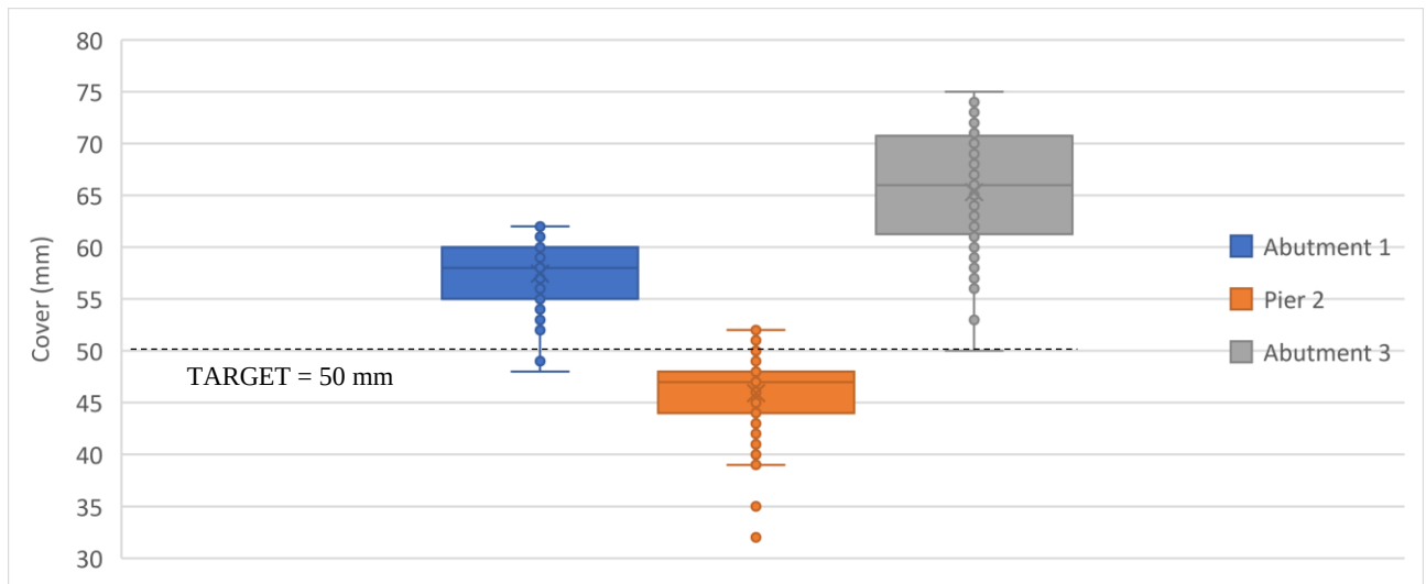
Figure 4-20 - TR2/2 Bridge cover readings - boxplot per element
