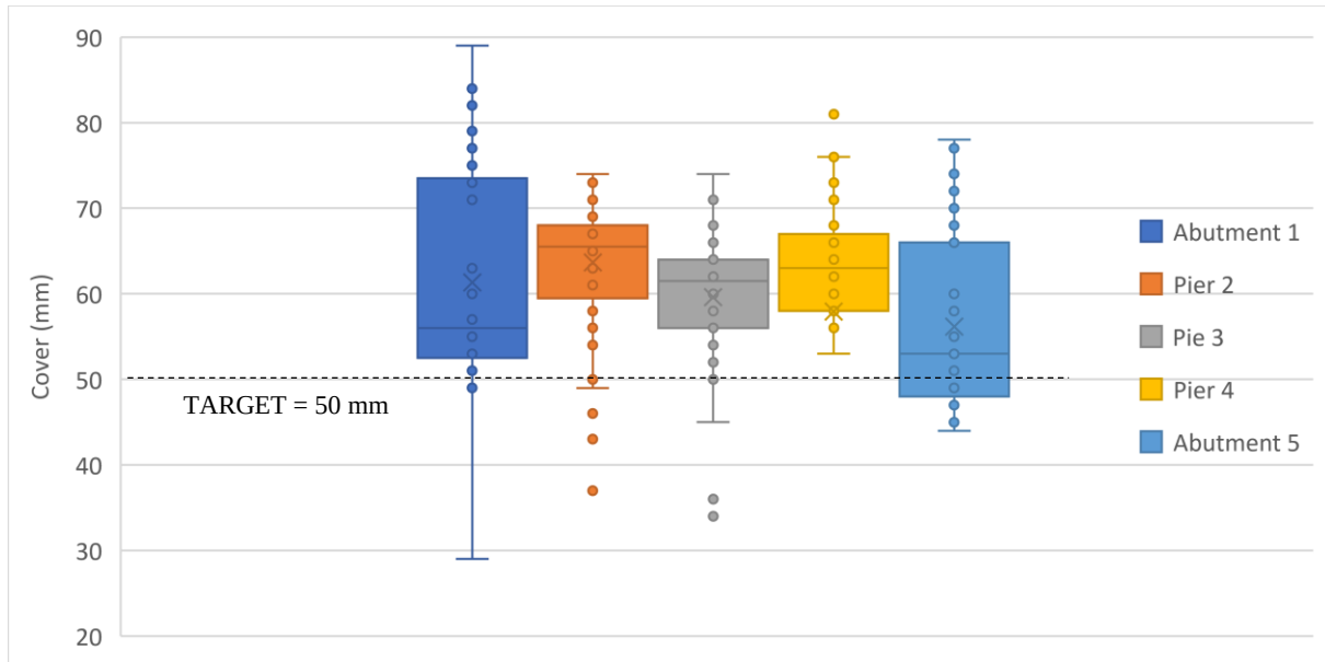
Figure 4-19 - Swakop River Bridge B cover readings - boxplot per element
