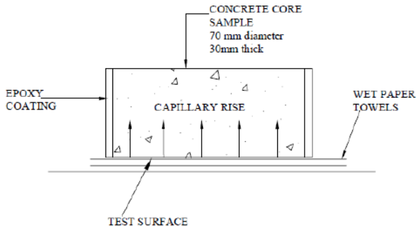
Figure 2-20 - Schematic of Water Sorptivity Test Arrangement (Alexander & Mackechnie, 2001)
