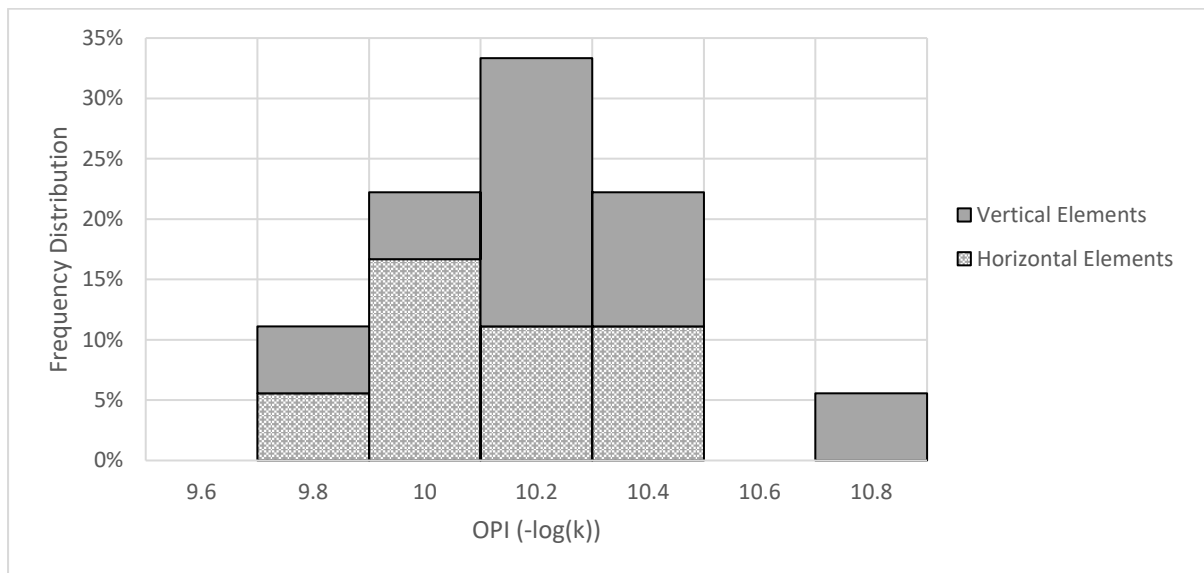
Figure 4-4 - Frequency distribution histogram for OPI test results
