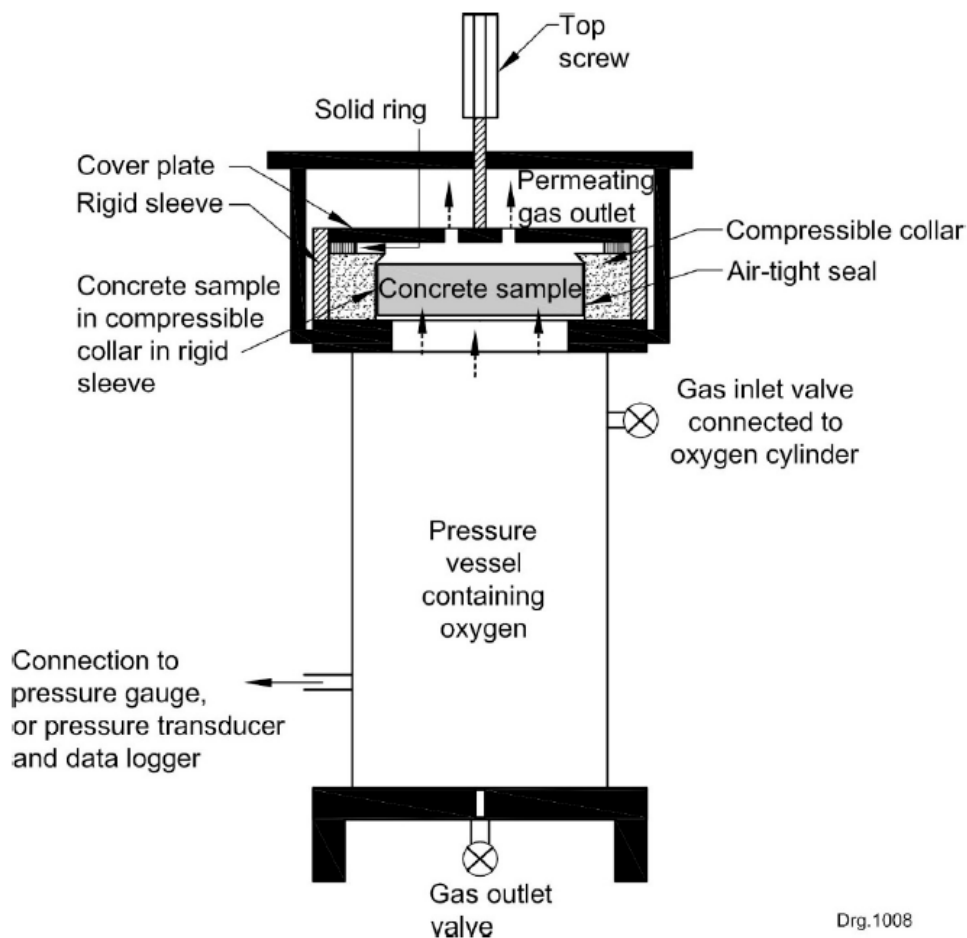
Figure 2-19 - Schematic of an oxygen permeameter (DI Testing Manual, 2018)
