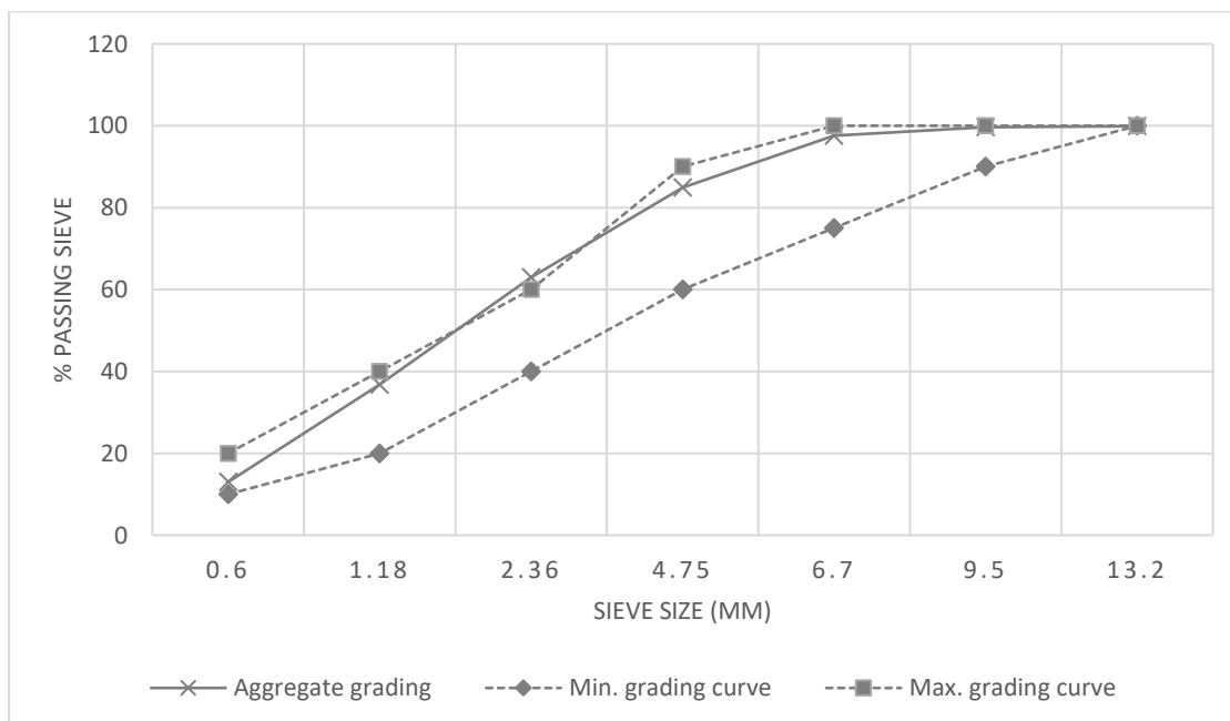
Figure 3-13 -Fine aggregate grading curve
