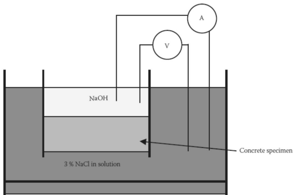
Figure 2-18 - Schematic of rapid chloride permeability test (ASTM C1202-19, 2019)
