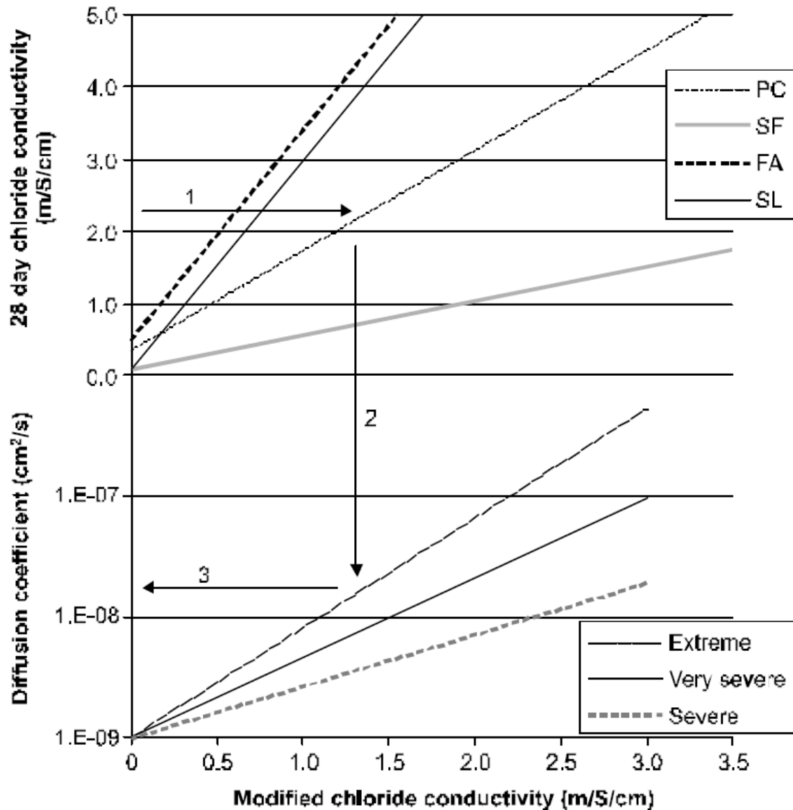
Figure 2: Predicting 50-year diffusion coefficients for marine concrete
