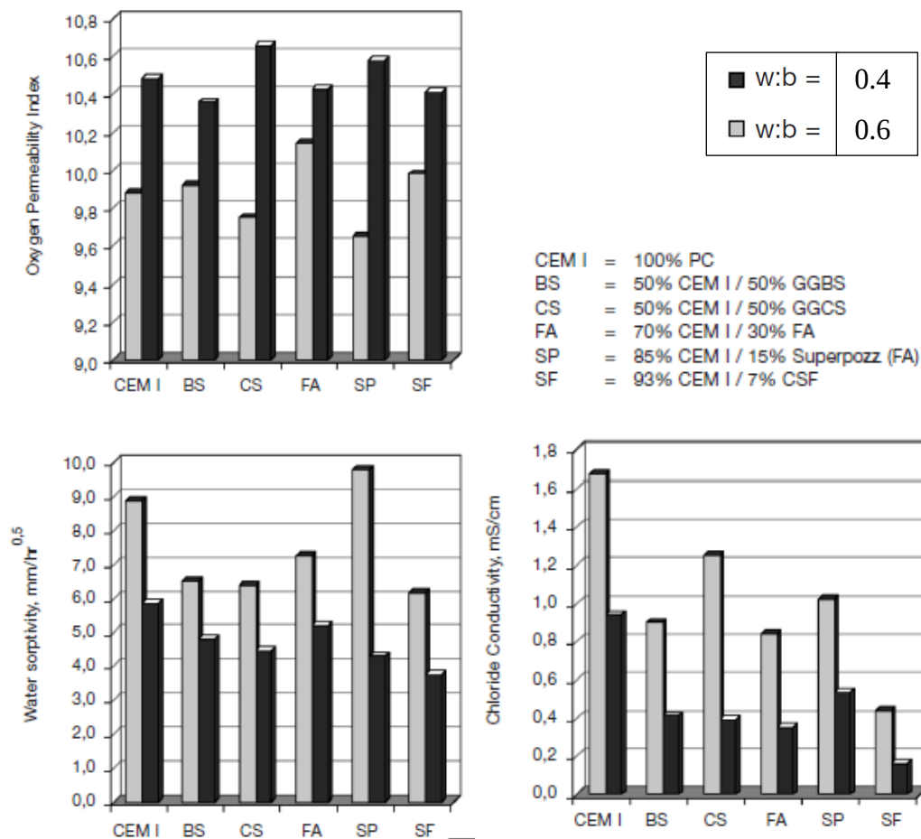
Figure 2-3 - Typical test results for Durability Index values, measured on water-cured samples at 28 days of age, in relation to w:b ratio and binder type (Ballim, et al., 2009)
