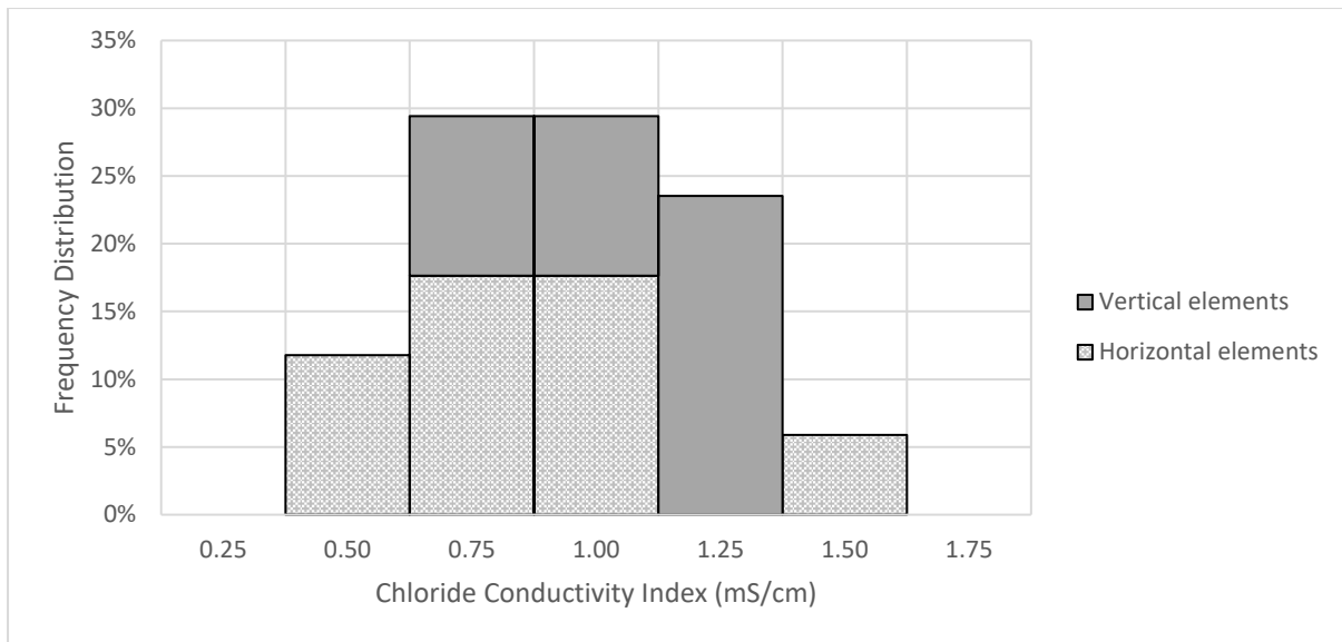
Figure 4-12 - Frequency distribution histogram for CCI results
