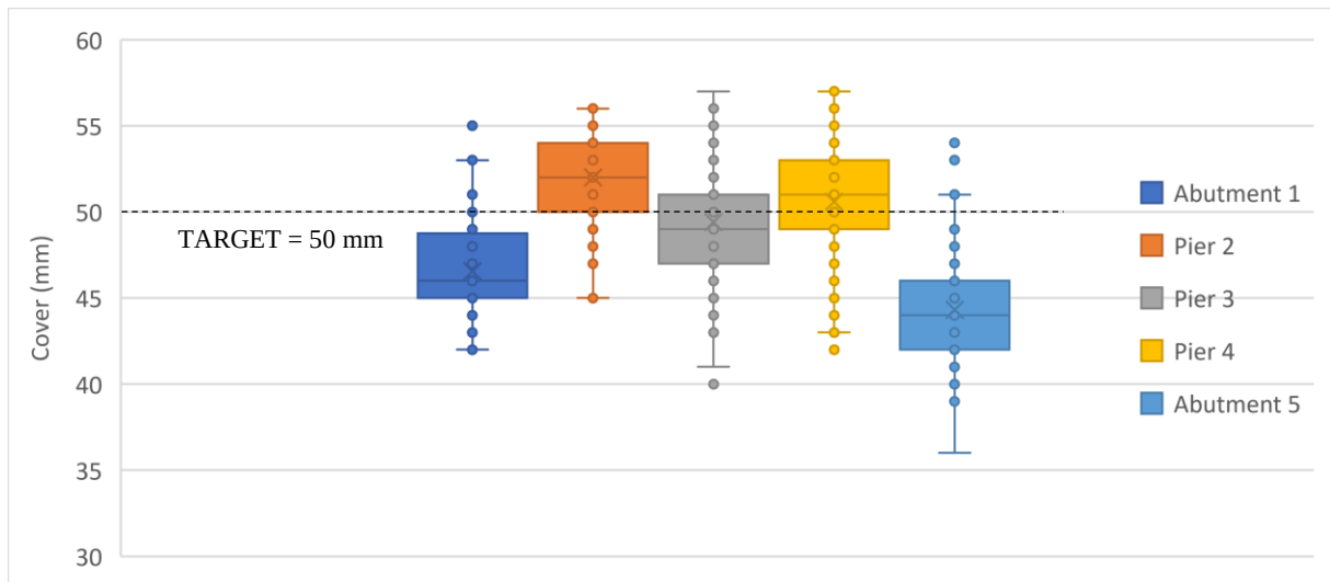
Figure 4-17 - MR52 Bridge cover readings - boxplot per element
