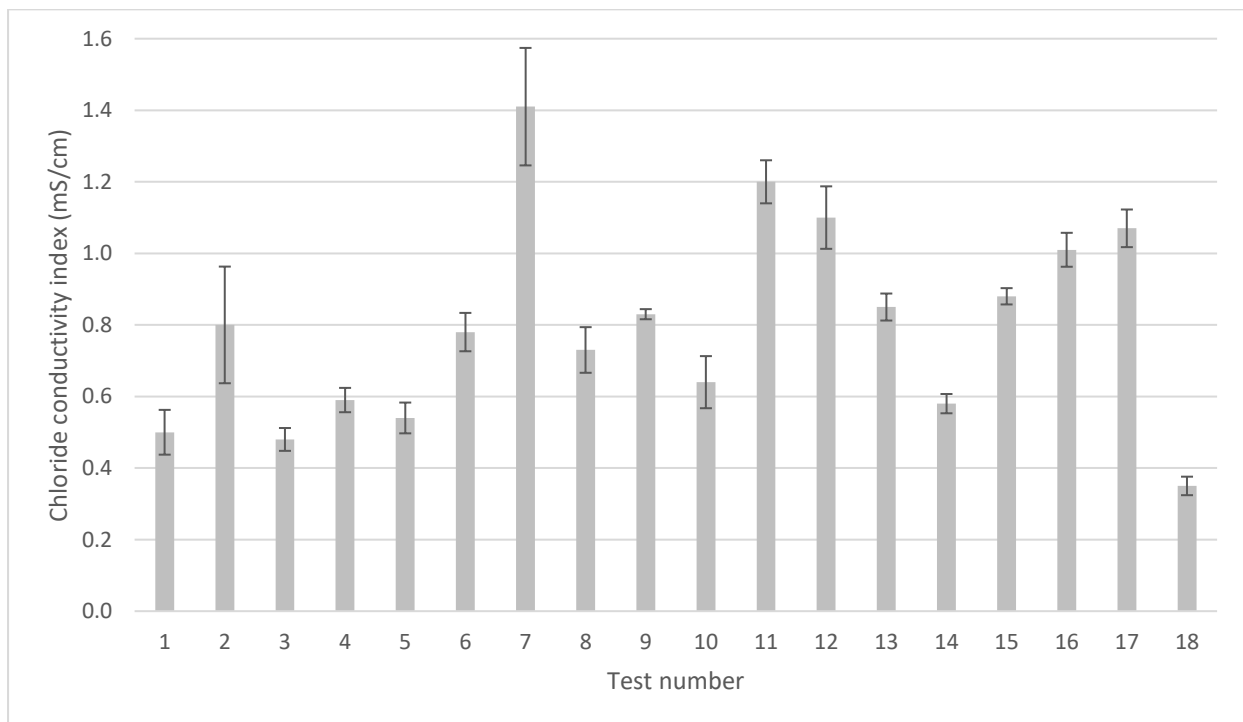
Figure 4-11 - Graphical summary of CCI results
