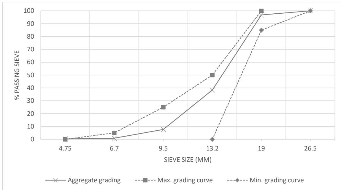
Figure 3-12 - Coarse aggregate grading curve
