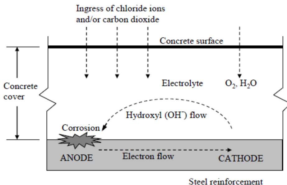
Figure 2-7 - A schematic illustration of the corrosion process in concrete (Alexander, et al., 2012)
