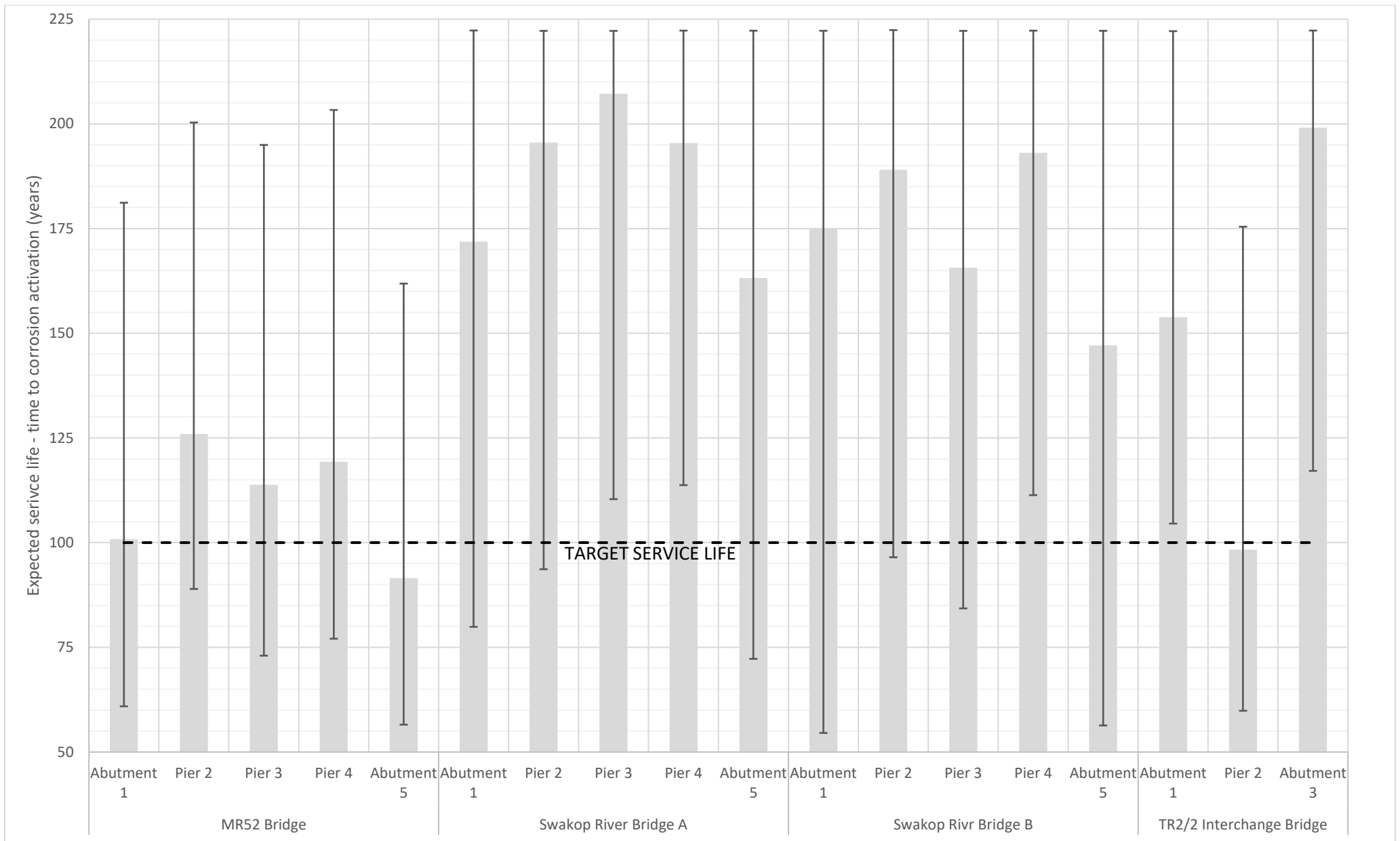
Figure 4-22 - Expected service life of bridge elements
