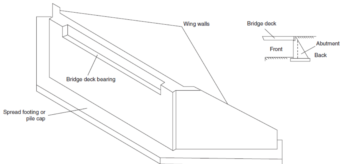
Figure 3-7 - Typical solid wall abutment (Lindsell, et al., 2008)
