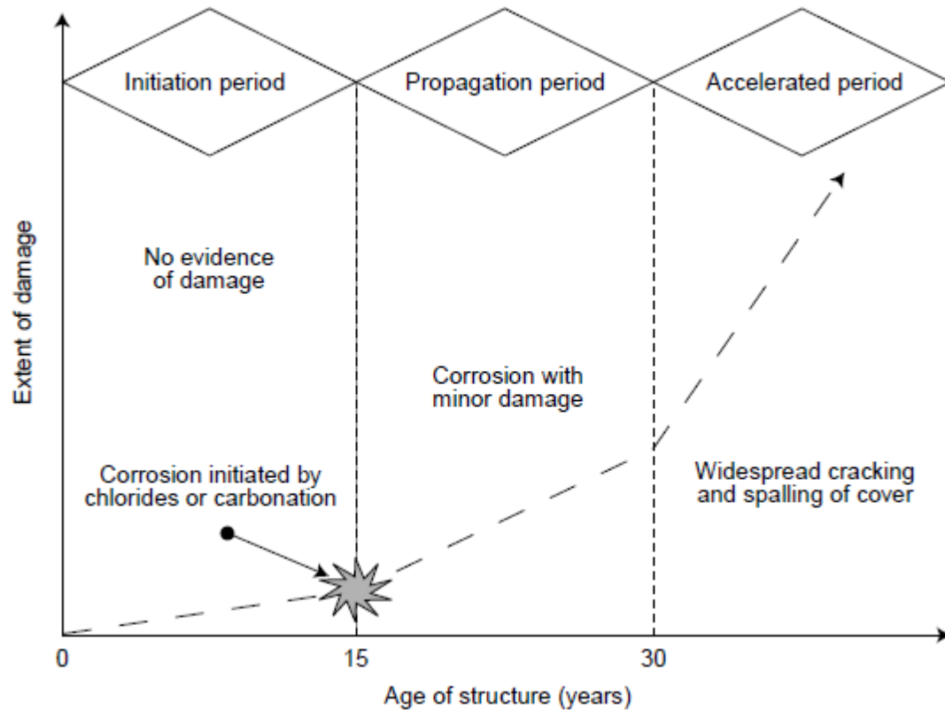
Figure 2-9 - Three stage corrosion damage model (Heckroodt, 2002)
