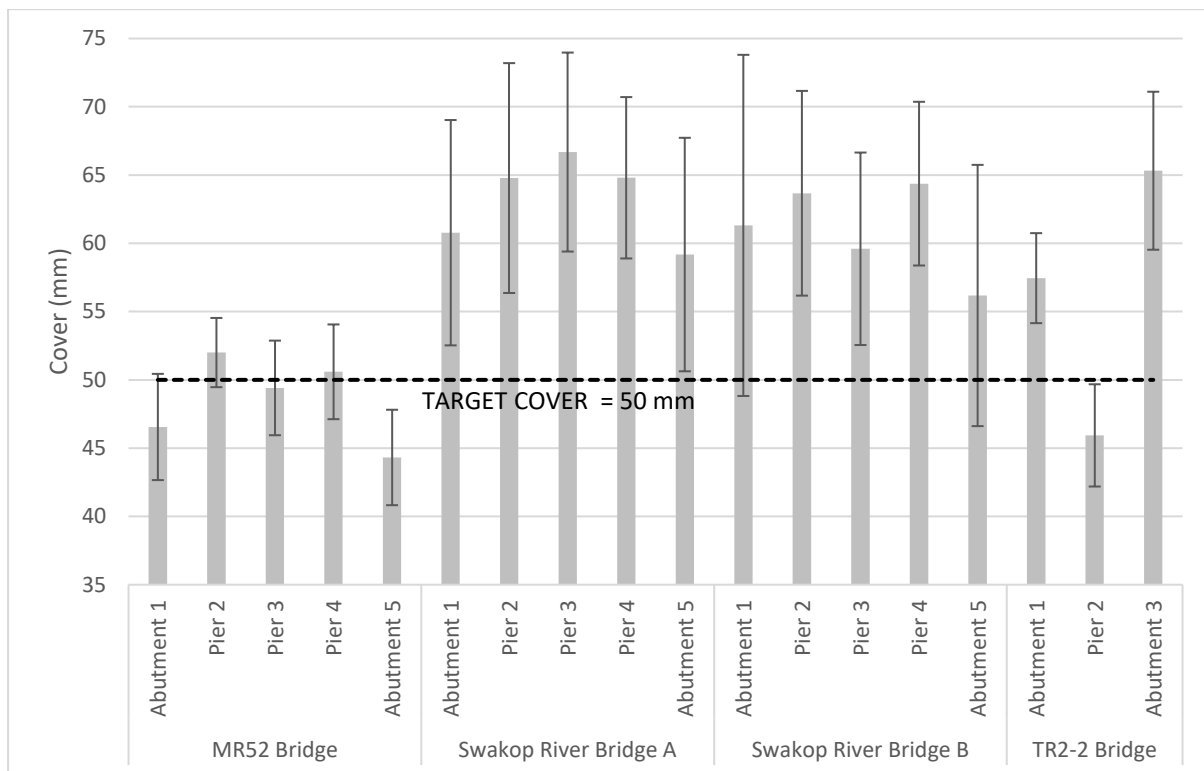
Figure 4-15 - Graphical summary of cover depth readings
