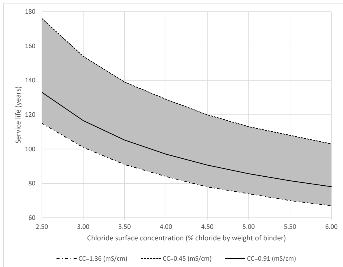
Figure 4-25 - Effect of surface concentration of chlorides on service life
