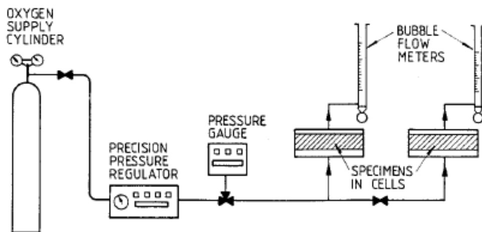
Figure 2-15 - Line diagram of Cembureau oxygen permeability apparatus (Kollek, 1989)
