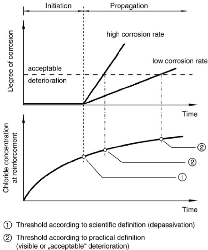
Figure 2-13 - Definitions of chloride threshold levels (Angst, et al., 2009)
