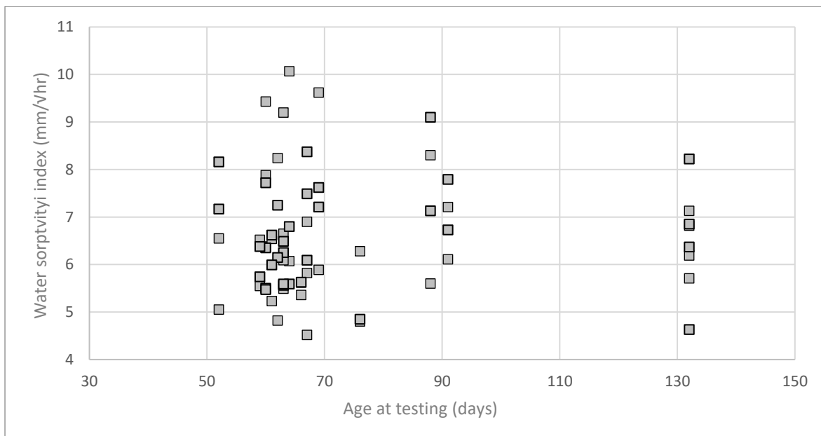
Figure 4-10 - Effect of age at testing on WSI
