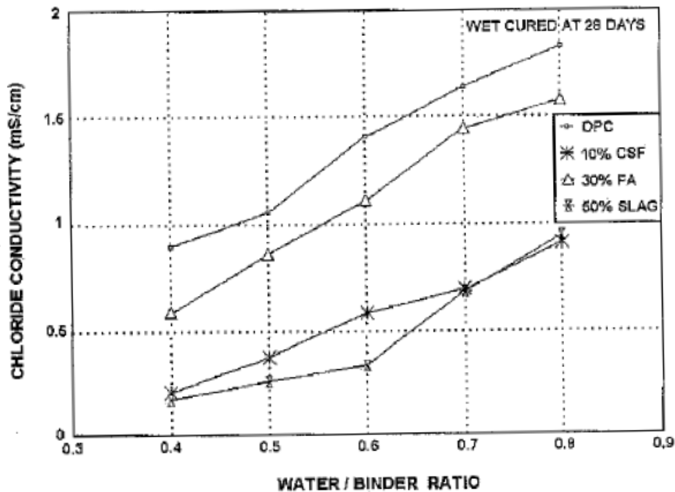
Figure 2-4 - Chloride conductivity versus water-binder ratio (Alexander, et al., 1999)
