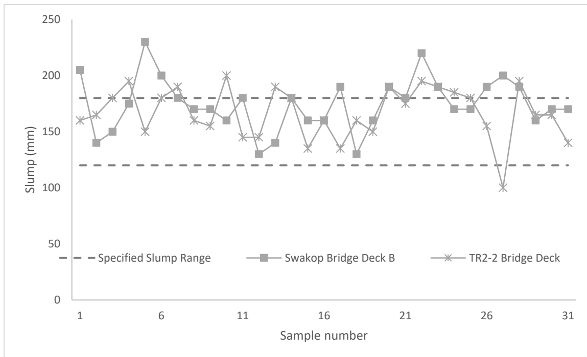
Figure 3-15 - Typical Variation in concrete slumps across several samples
