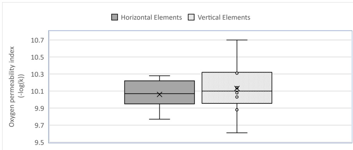
Figure 4-5 - Box plot comparison of OPI values for vertical and horizontal elements
