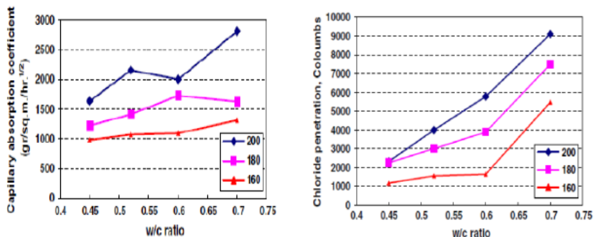
Figure 2-2 - Effect of cement content on absorption and chloride penetration (Wasserman, et al., 2009)
