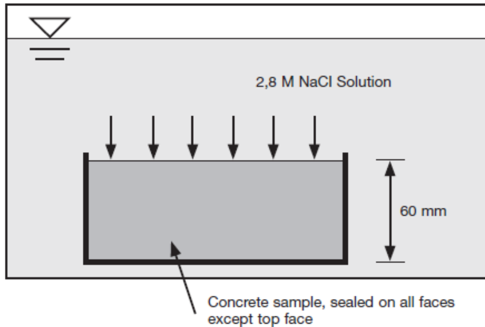
Figure 2-17 - Schematic of bulk diffusion test (ASTM C1556 - 04, 2004)
