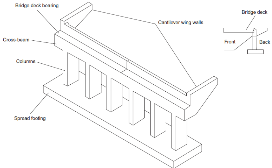
Figure 3-6 - Typical spill-through abutment (Lindsell, et al., 2008)
