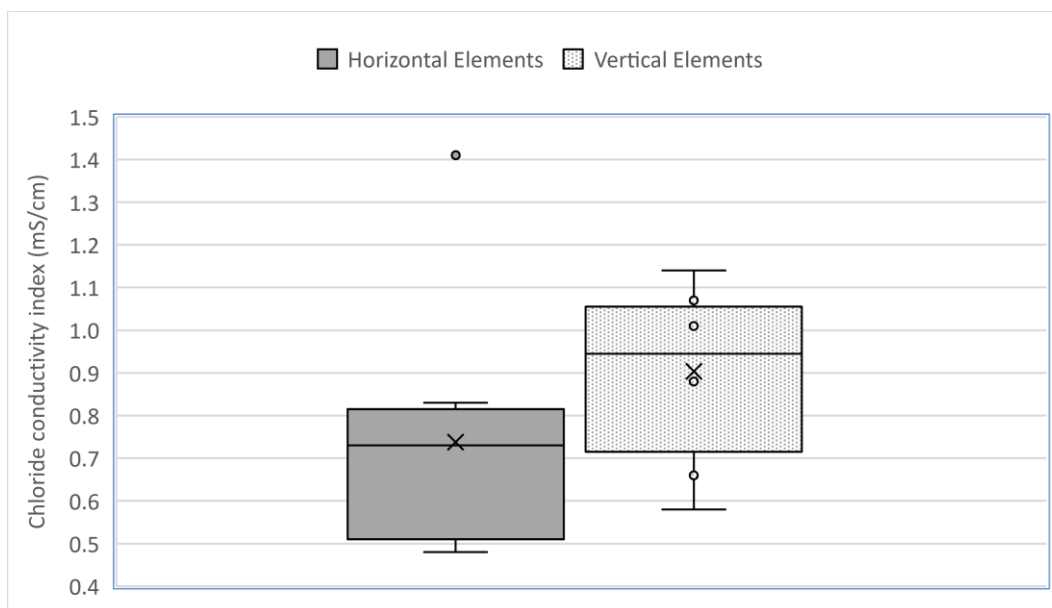
Figure 4-13 - Boxplot comparison of horizontal and vertical element CCI test results
