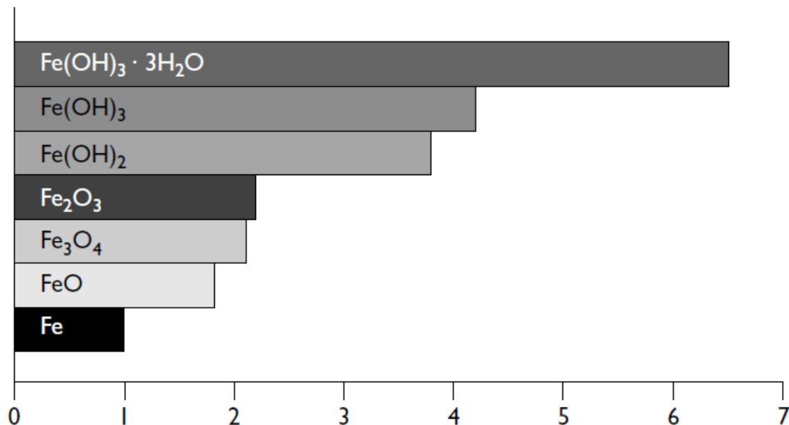
Figure 2-8- Relative volume of iron and its oxides (Corrosion1981mansfield) – (See Broomfield corrosion of steel in concrete page 9)
