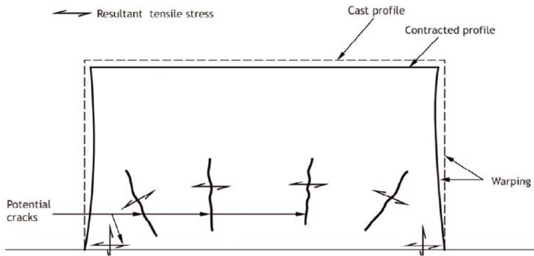
Figure 3-10 - Early thermal contraction cracks in concrete walls (The Concrete Centre, 2015)
