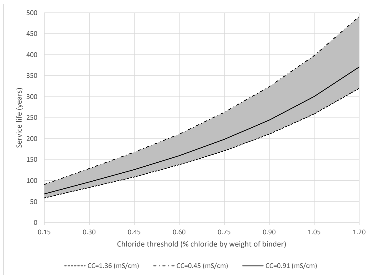
Figure 4-24 - Effect of chloride threshold on service life
