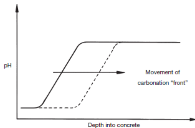
Figure 2-10 - pH reduction due to carbonation movement as a front from the concrete surface (Ballim, et al., 2009)
