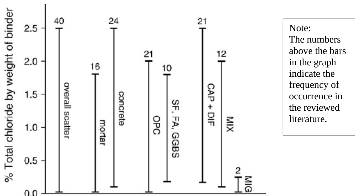
Figure 2-14 - Scatter of chloride threshold values sorted by selected parameters (Angst, et al., 2009)
