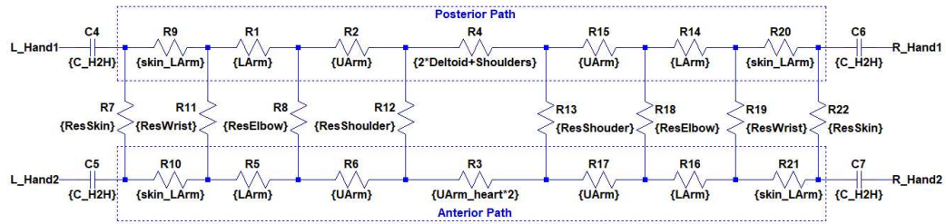
Figure 18 – Modification 3 of Hand-to-hand Human Body Impedance Model
