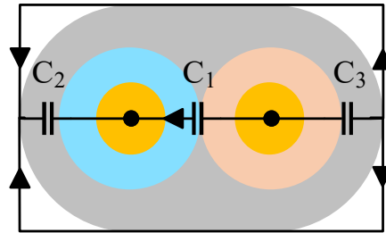
Figure 12 – Simplified current paths in a cross-section of a flat power cable
