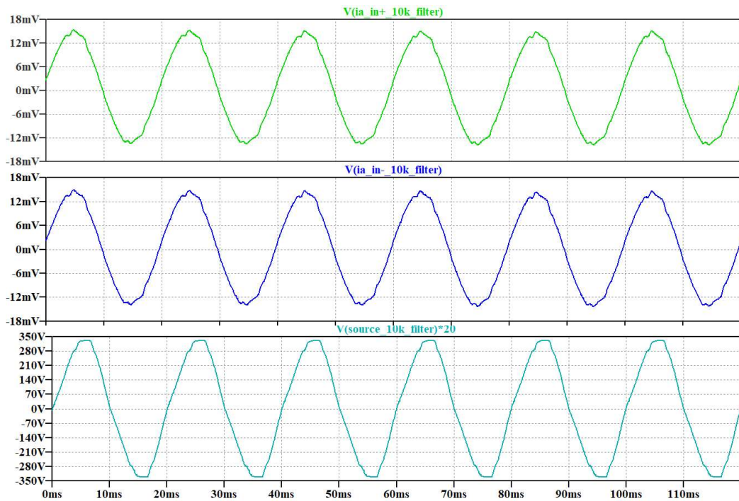
Figure 41 – Case 4 Measurements of Participant C. Measurements taken from the Voltage Follower Outputs for Electrode A and B; and Plug point source with 20:1 Step Down Transformer.
