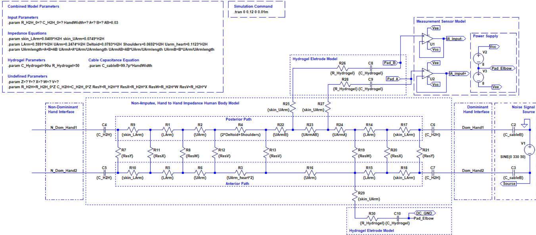
Figure A4 – Model of Experiment for Case 4 Measurements
