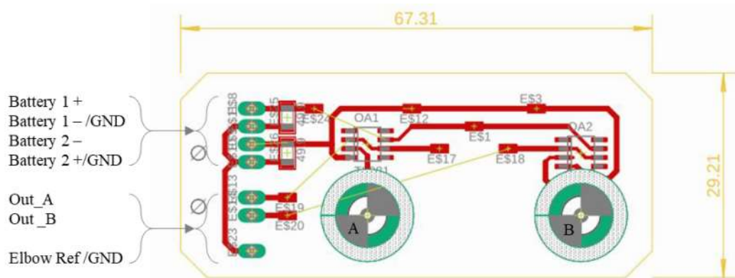
Figure 28 – PCB design for the Measurement sensor
