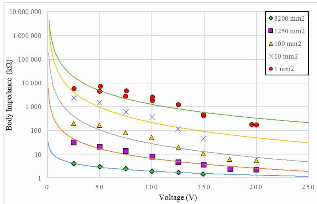
Figure 7 – Total body impedance as a function of applied voltage for various contact areas; dry hand-to-hand electrodes measured by Beigelmeier [44]. The image was extracted from Reilly [47] and the various curves illustrated are identified by the contact area on each hand.
