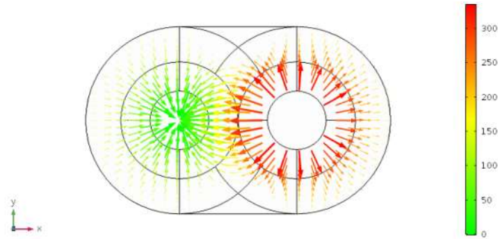
Figure 10 – Simulated Electric Potential of a flat power cable with a floating potential boundary surrounding sheath. The legend indicates the arrow potentials in V/m. Live and neutral conductors are on the right and the left, respectively.
