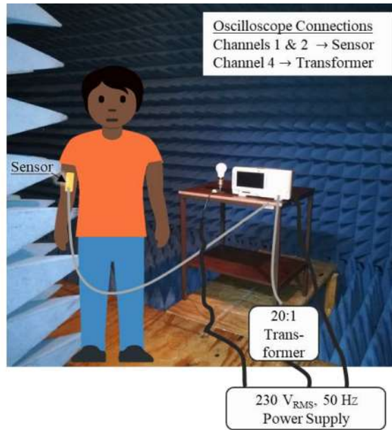
Figure 32 – Simplified setup for the experiment in the Anechoic Chamber. Participant does not hold any surfaces during baseline measurements. Figure of person was available through Creative Commons Licence [63]
