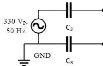
Figure 14 – Capacitive-Coupling Model, where magnitudes of C_2 and C_3 are determined using Equation (4)
