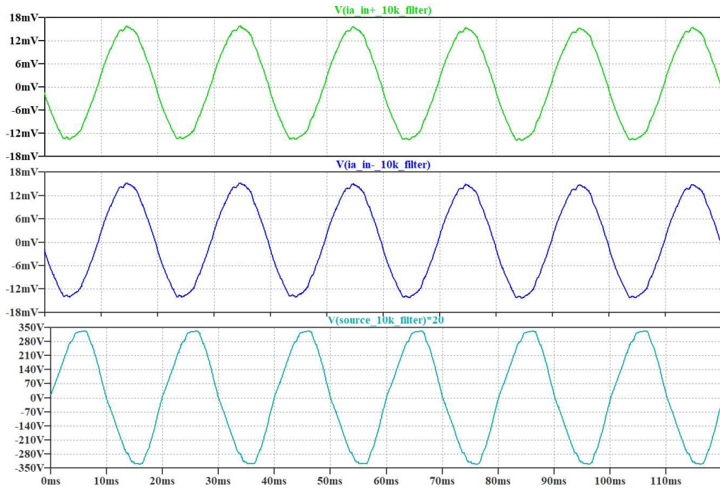
Figure 40 – Case 3 Measurements of Participant C. Measurements taken from the Voltage Follower Outputs for Electrode A and B; and Plug point source with 20:1 Step Down Transformer.
