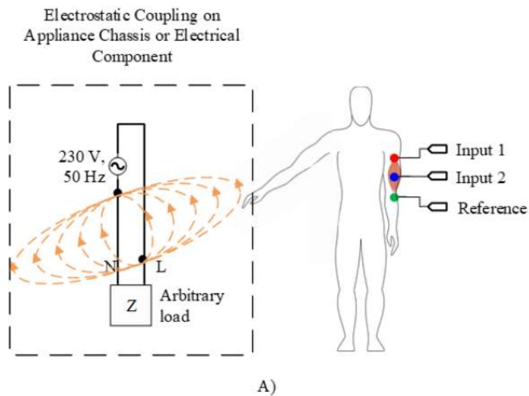
Figure 2 – Electrostatic Coupling between Powered Cables and the subject describing the inherent electric field coupling between the subject and power cables. Electric field direction indicates the positive half cycle. The negative half cycle will reverse the field direction.
