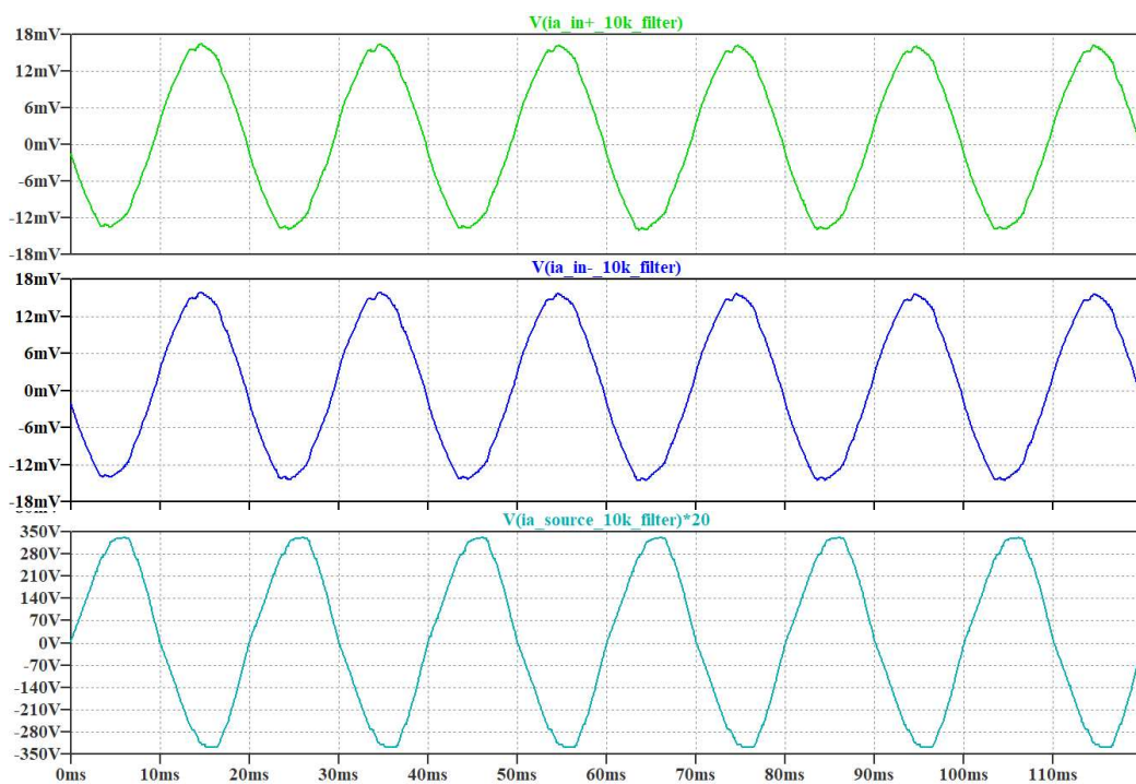
Figure 38 – Case 1 Measurement of Participant C. Measurements taken from the Voltage Follower Outputs for Electrode A and B; and Plug point source with 20:1 Step Down Transformer.
