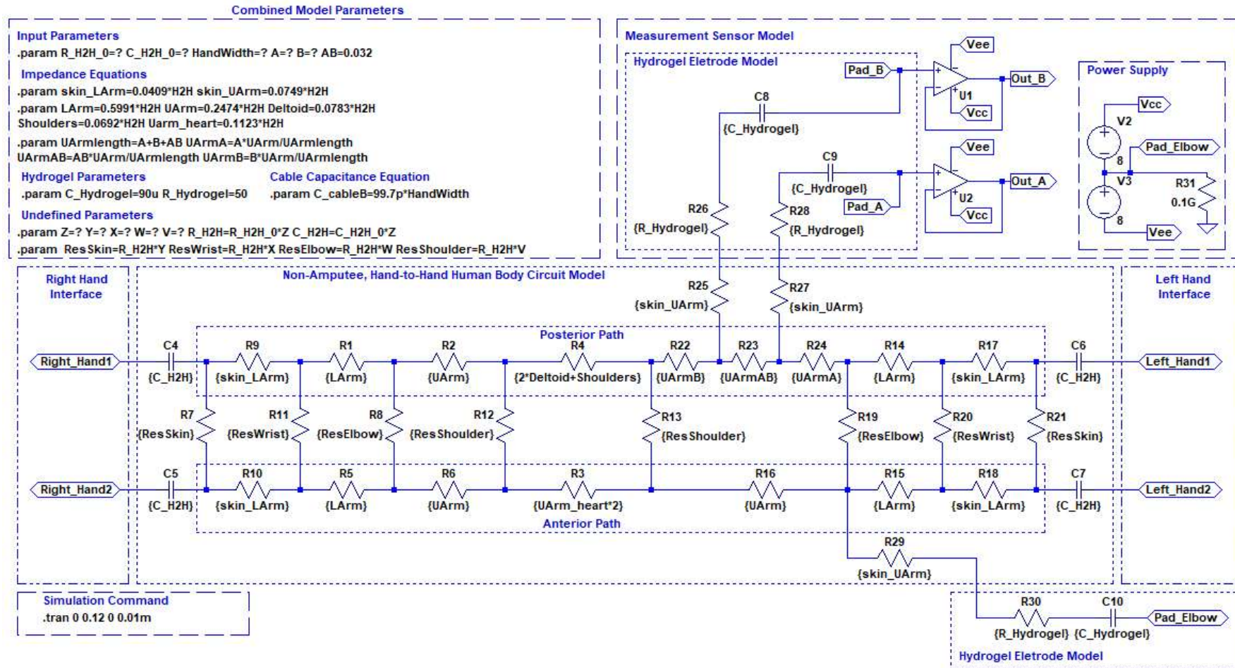
Figure 47 – Unified Model of Validation Experiment, with the Noise Source connection shown in Figure 46
