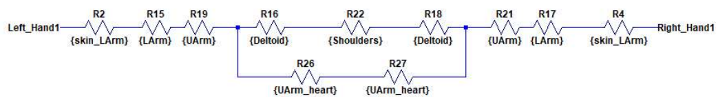
Figure 16 – Hand-to-hand Section of Freiberger Model
