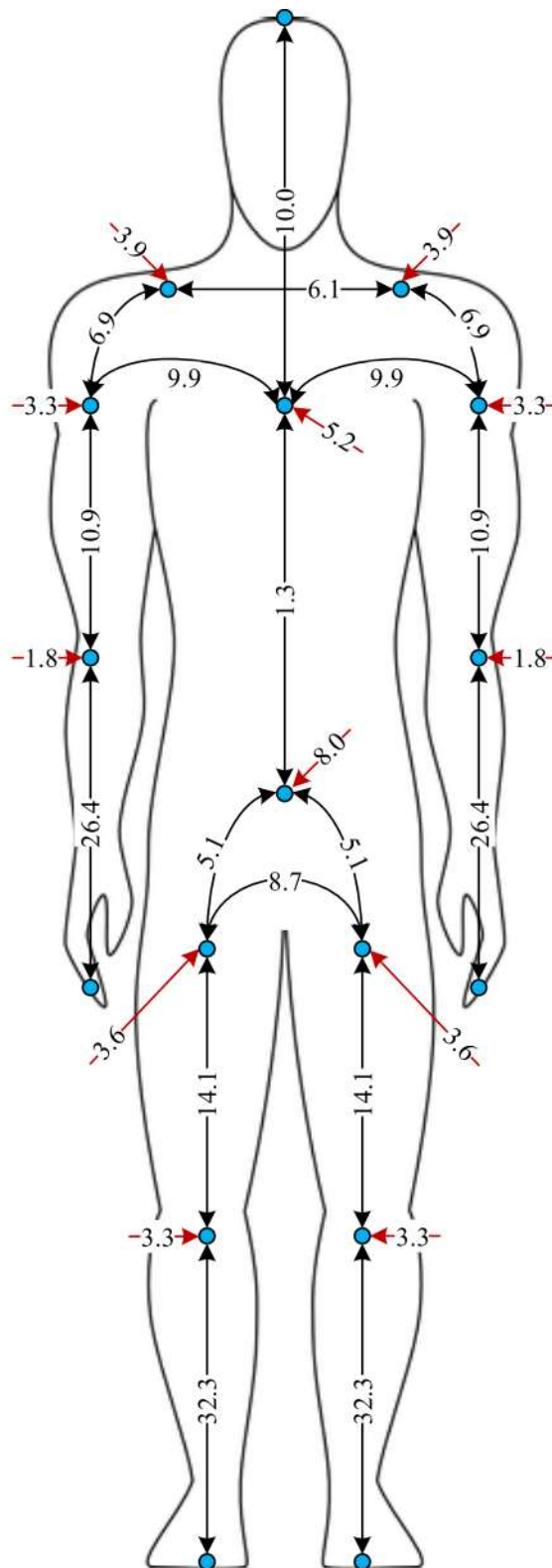
Figure 8 – Internal Partial Impedances of the Human body. The numbers indicate the percentage of the internal impedance of the human body for the part of the body concerned, in proportion to the ‘hand-to-foot’ path. (Red arrows indicate skin impedances from the top layer to the nodes in the body). i
