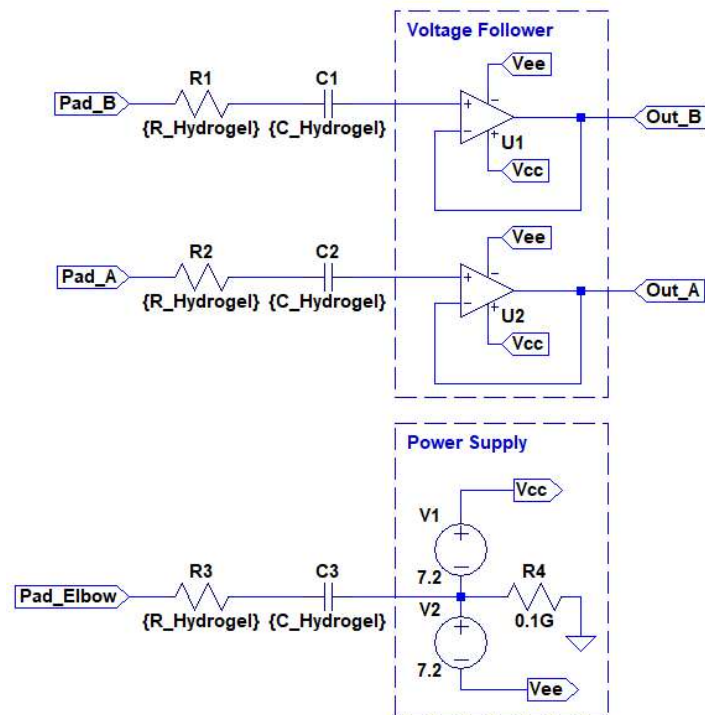
Figure 26 – EMI Measurement System Circuit Model. V_{CC} and V_{EE} are powered by the lithium batteries
