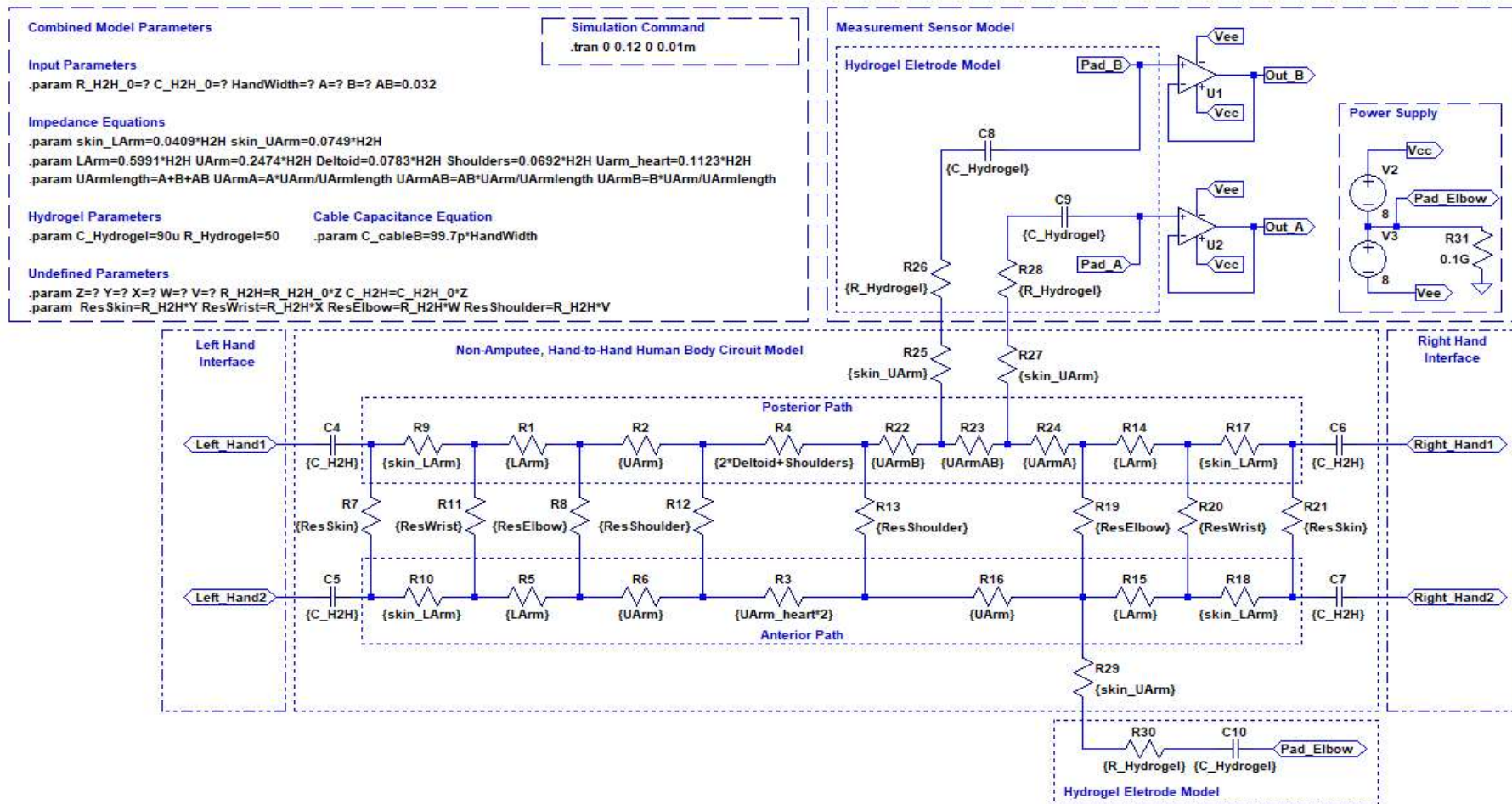
Figure 43 – Unified Model of Experiment, with the Noise Source connection shown in Figure 44
