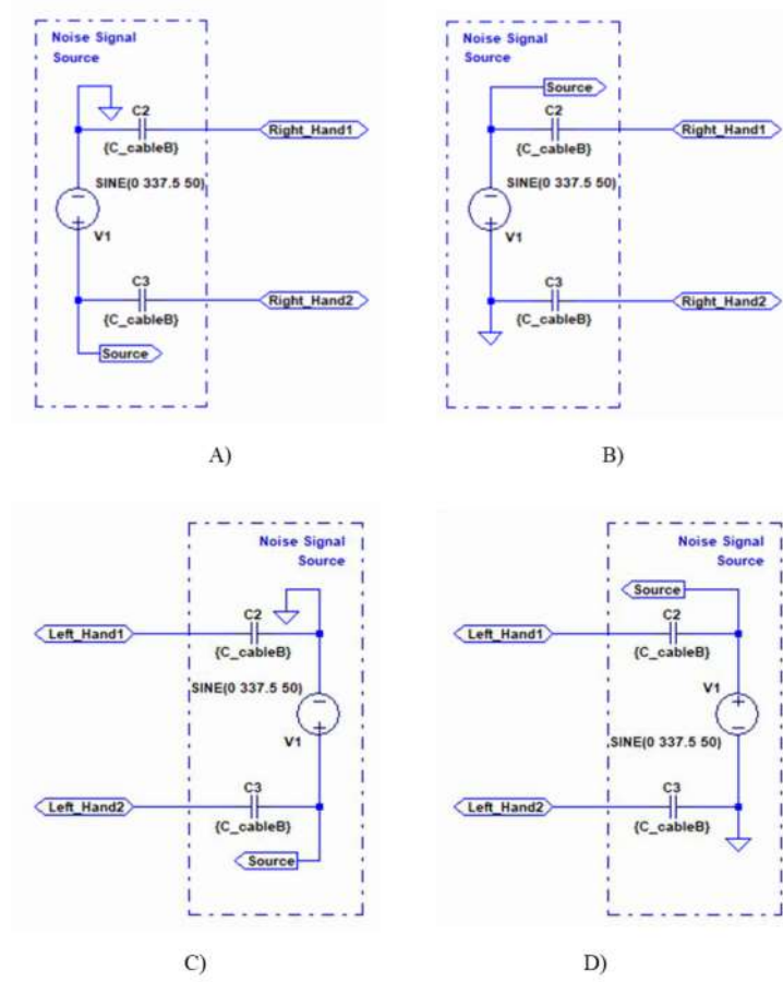
Figure 46 – Noise Source Connection Diagram for the Four Different Cases. A) Case 1, B) Case 2, C) Case3, and D) Case 4
