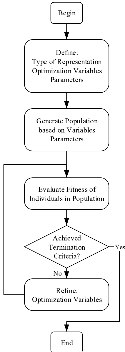
Figure 50 – Flowchart of the Pseudo-code for the desired Genetic Algorithm [66]
