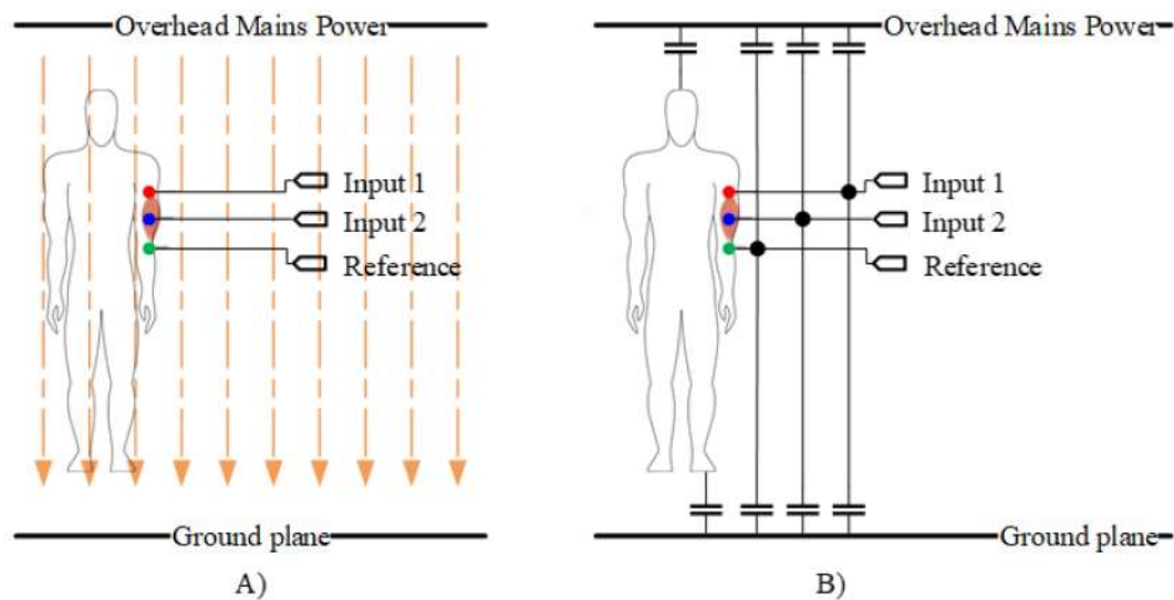
Figure 1 – Electrostatic Coupling between the Overhead Cables and EMG system. A) Describes the inherent electric field coupling between the EMG electrode wires and overhead power cables. B) Describes the parasitic capacitances that exist between the subject, electrode wires and power cables.
