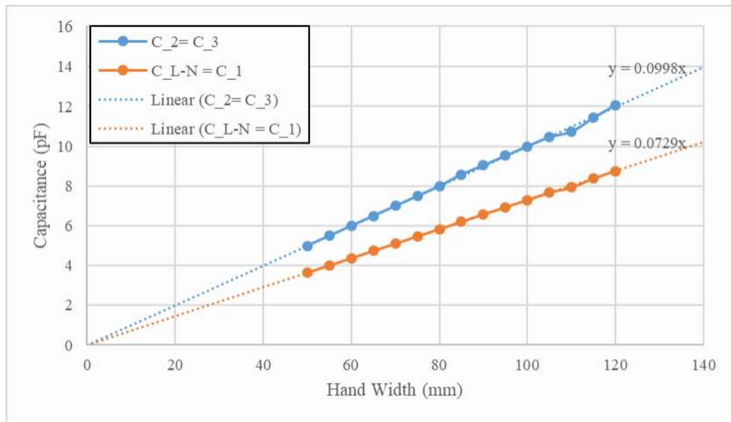
Figure 13 – Simulated Capacitance C_1 and Calculated Capacitances C_2 and C_3 for Various Hand Widths Between 50 mm And 120 mm
