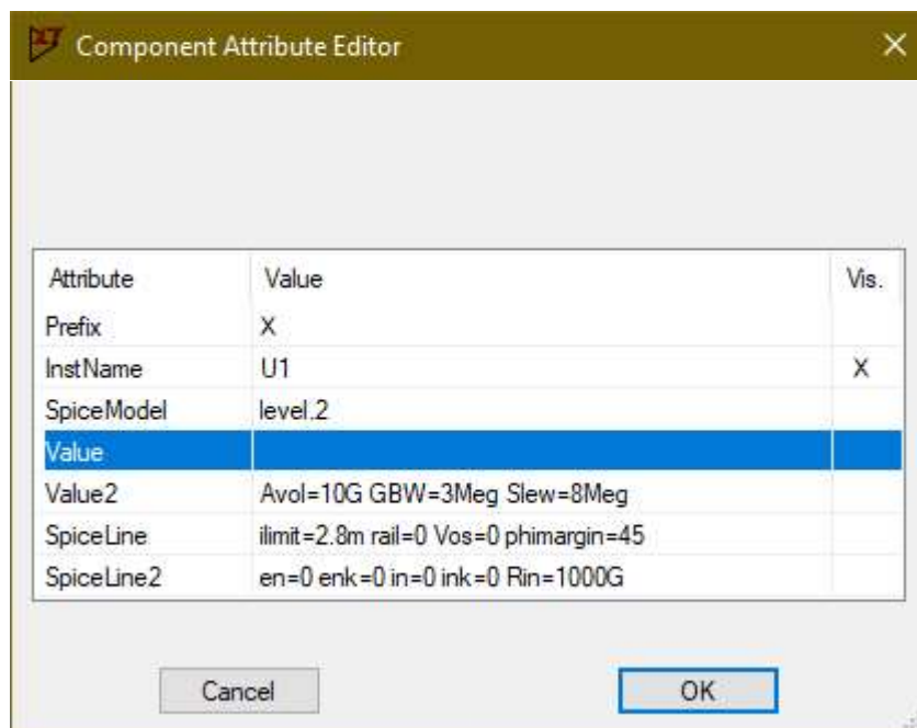
Figure 27 – Virtual Op-Amp Settings
