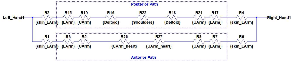
Figure 17 – Modification 2 of Hand-to-hand Human Body Impedance Model
