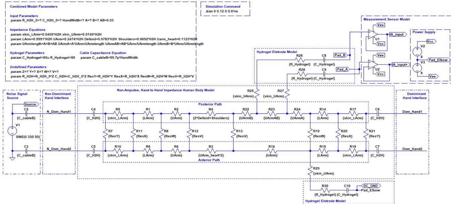
Figure A2 – Model of Experiment for Case 2 Measurements
