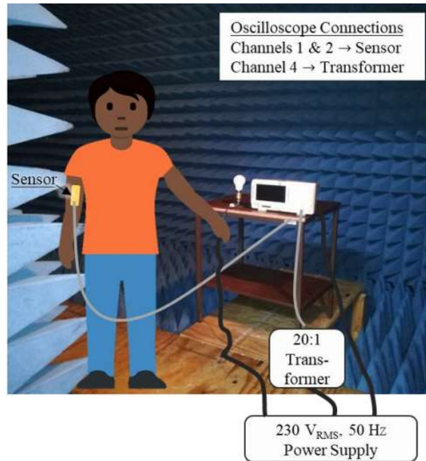
Figure 34 – Simplified setup for the Case 1 and Case 2 experiment in the Anechoic Chamber. Figure of person was available through Creative Commons Licence [63]
