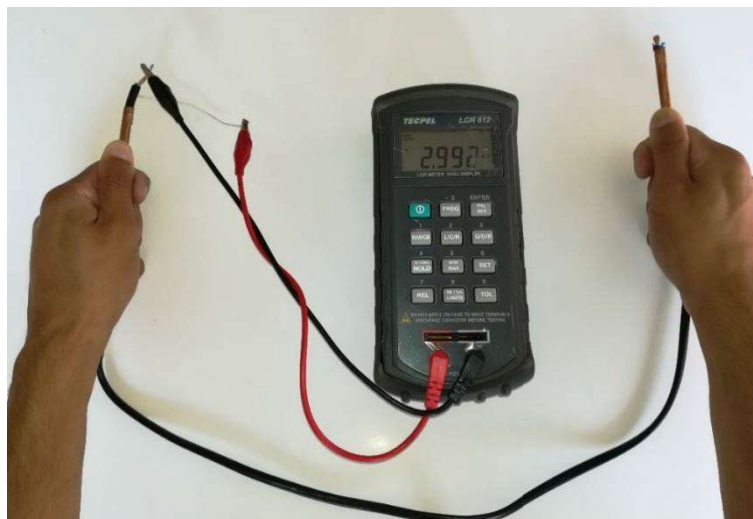
Figure 31 – Grasping the Hand-to-hand Impedance measurement setup
