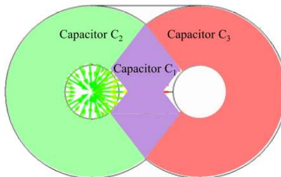
Figure 11 – Segmenting Cross-section of type flat power cable into three capacitance regions
