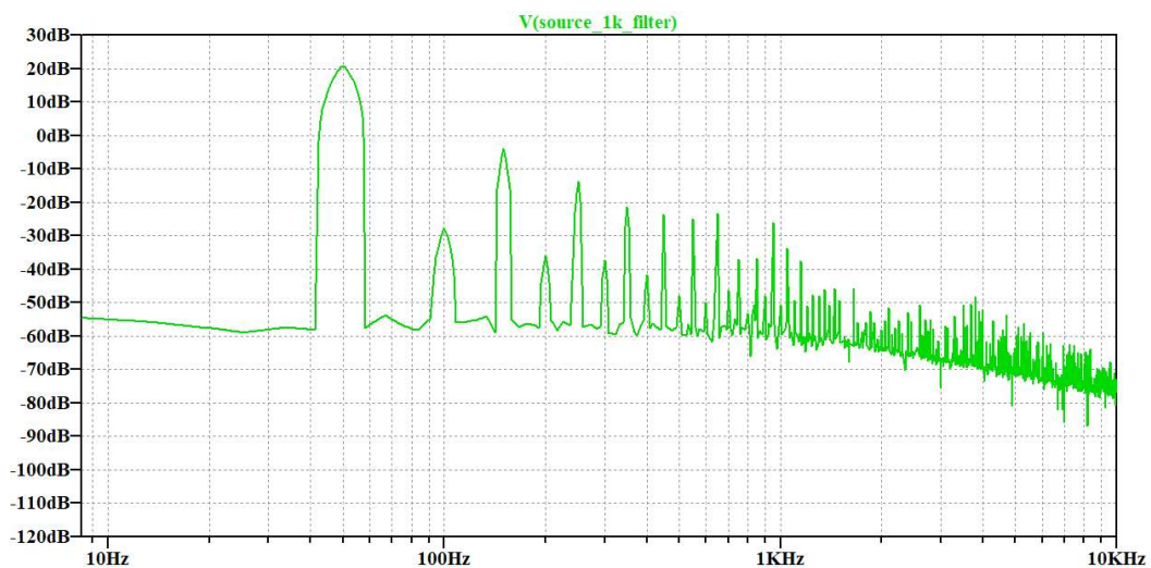
Figure 23 – FFT of Sample measurement of the 230V rms power supply found in the Anechoic Chamber
