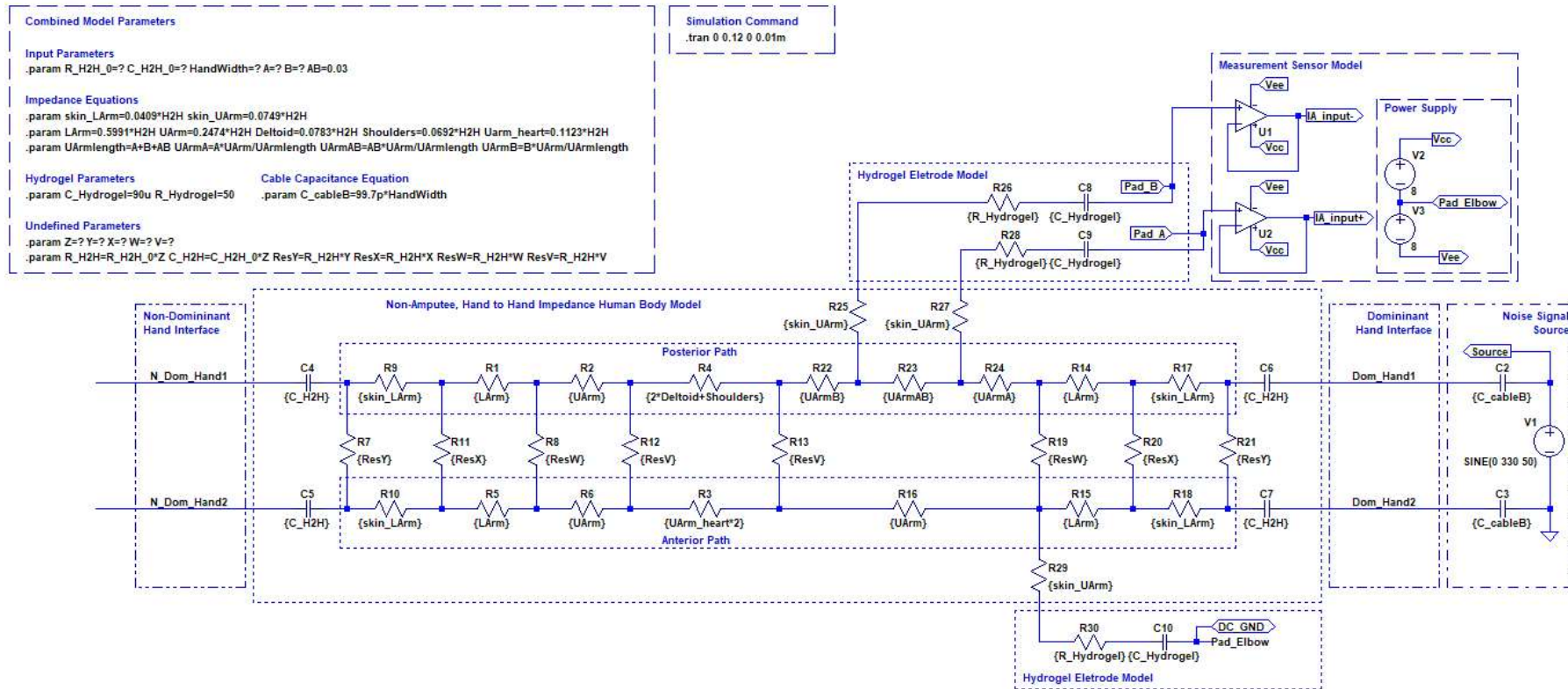
Figure A3 – Model of Experiment for Case 3 Measurements
