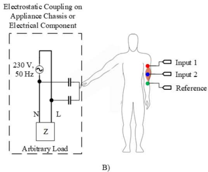
Figure 3 – Describing the parasitic capacitances that exist between the subject and appliance or electrical component chassis.
