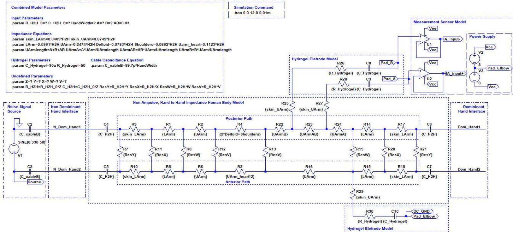
Figure A1 – Model of Experiment for Case 1 Measurement
