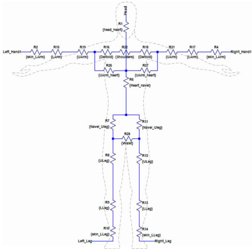
Figure 15 – Original Freiberger Model with human body outline.
