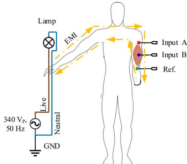
Figure 4 – Electrostatic Coupling between Powered Cables and the Amputee subject. The subject is grasping a lamp's insulated power cable with their un amputated hand. The flow of EMI induced current conducting through the body is indicated with orange dashed lines (arrows' pointing direction is arbitrary). The negative half cycle will reverse the field direction.
