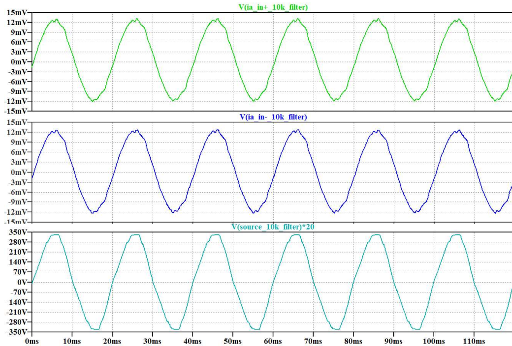
Figure 38 – Case 1 Measurement of Participant C. Measurements taken from the Voltage Follower Outputs for Electrode A and B; and Plug point source with 20:1 Step Down Transformer.
