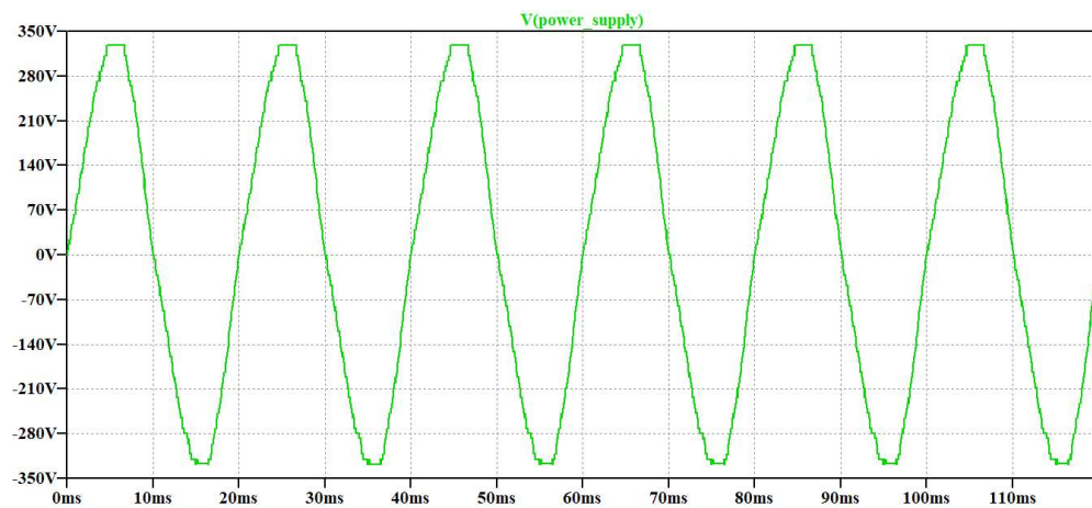
Figure 22 – Sample measurement of the 230 V rms power supply found in the Anechoic Chamber
