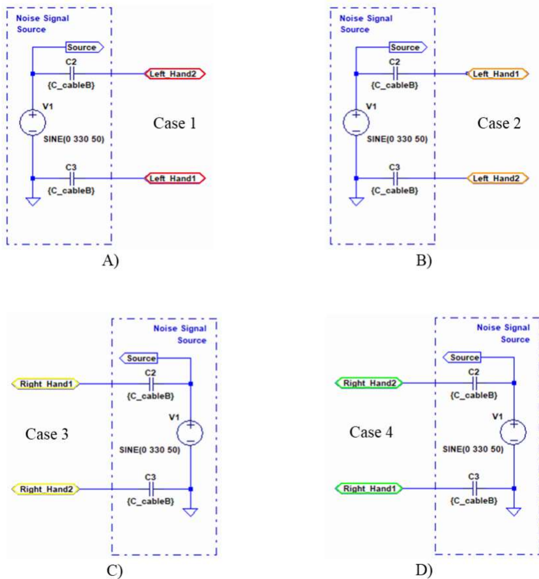
Figure 44 – Noise Source Connection Diagram for the Four Different Cases. A) Case 1, B) Case 2, C) Case3, and D) Case 4
