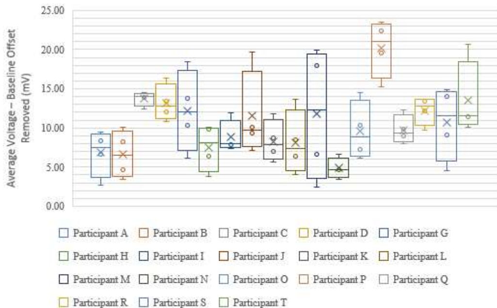
Figure 42 – Box and Whisker Diagram of Averaged Voltage Follower Output Voltages, Baseline Offset Removed, for all Four Cases.
