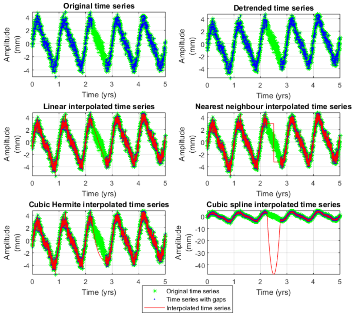
Figure 9.3: Synthetic time series T3 (with 10% missing data points), used in the variance test in chapter 4.2 and the response of the interpolation methods when applied to the noise contaminated time series. (a) Noise-contaminated synthetic time series without gaps (green) and with gaps (blue). (b) Detrended time series. (c) Linear interpolated time series. (d) Nearest neighbour interpolated time series). (e) Piecewise cubic Hermite interpolated time series. (f) Piecewise cubic spline interpolated time series.
