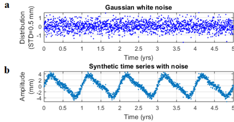
Figure 4.3: (a) Random Gaussian noise with a mean of 0 and a standard deviation of 0.5. (b) Noisy time series obtained by adding the noise time series in (a) and the noise-free-time series in Figure 4.2.
