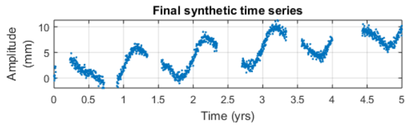
Figure 4.5: Synthetic signal with missing data points.
