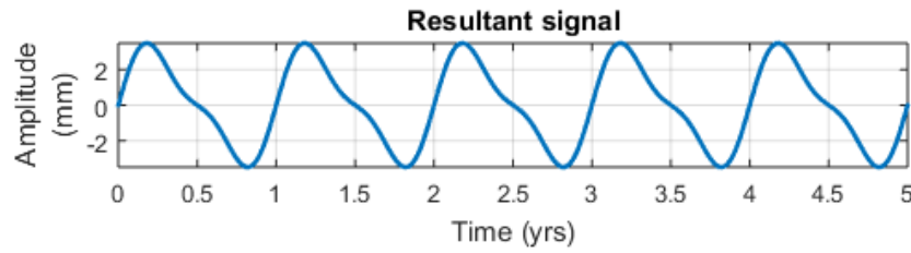
Figure 4.2: Noise-free synthetic time series obtained by adding the annual and semi-annual signals in Figure 4.1.
