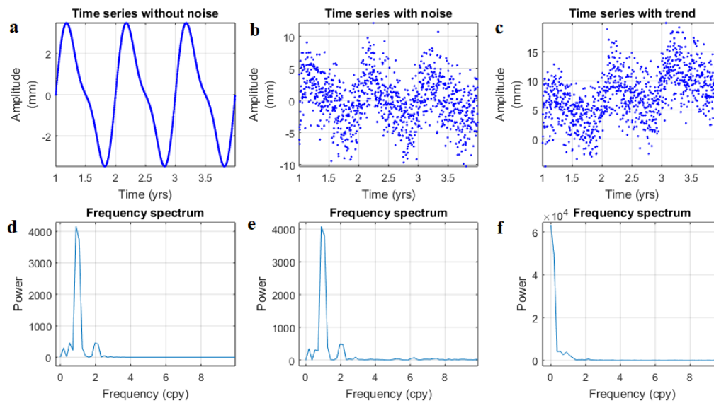
Figure 4.9: Fast Fourier Transform (FFT) decomposition of a time series without noise, with noise and with a trend. (a) Time series composed of an annual and semi-annual signal (i.e., signals of frequency 1 and 2 cpy), without noise. The annual signal has an amplitude of 3 mm, while the semi-annual signal has an amplitude of 1 mm. (b) Time series in (a) contaminated by white Gaussian noise with a standard deviation of 3 mm. (c) Time series in (b) with noise and a trend. (d) FFT spectrum of the time series in (a). (e) FFT spectrum of the time series in (b). (f) FFT spectrum of the time series in (c).
