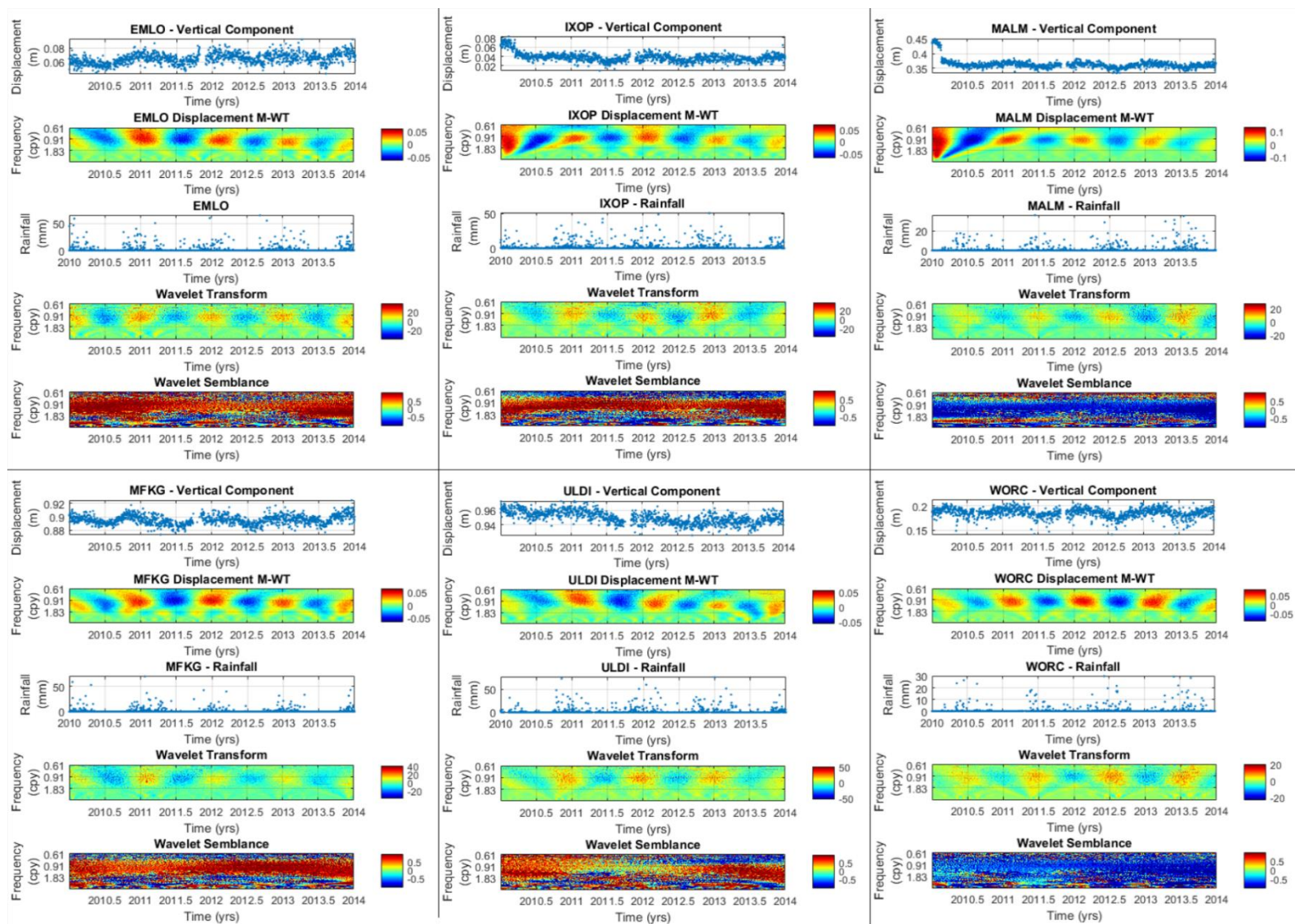
Figure 5.24: Sembance correlation plots of cGPS displacement time series (m) vs rainfall time series (mm).
