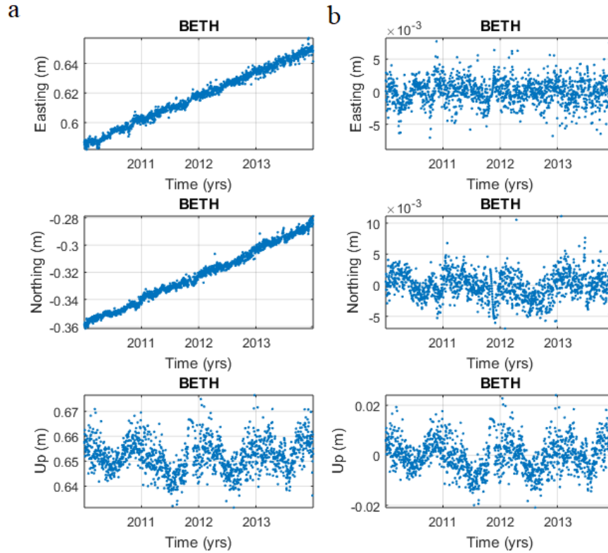
Figure 1.1: cGPS daily position time series of station BETH located in Bethlehem, South Africa. BETH represents Bethlehem. (a) Interpolated original time series. (b) Interpolated and detrended original time series; which shows the seasonal displacement of the easting and northing components with respect to that of the up (vertical) component.
