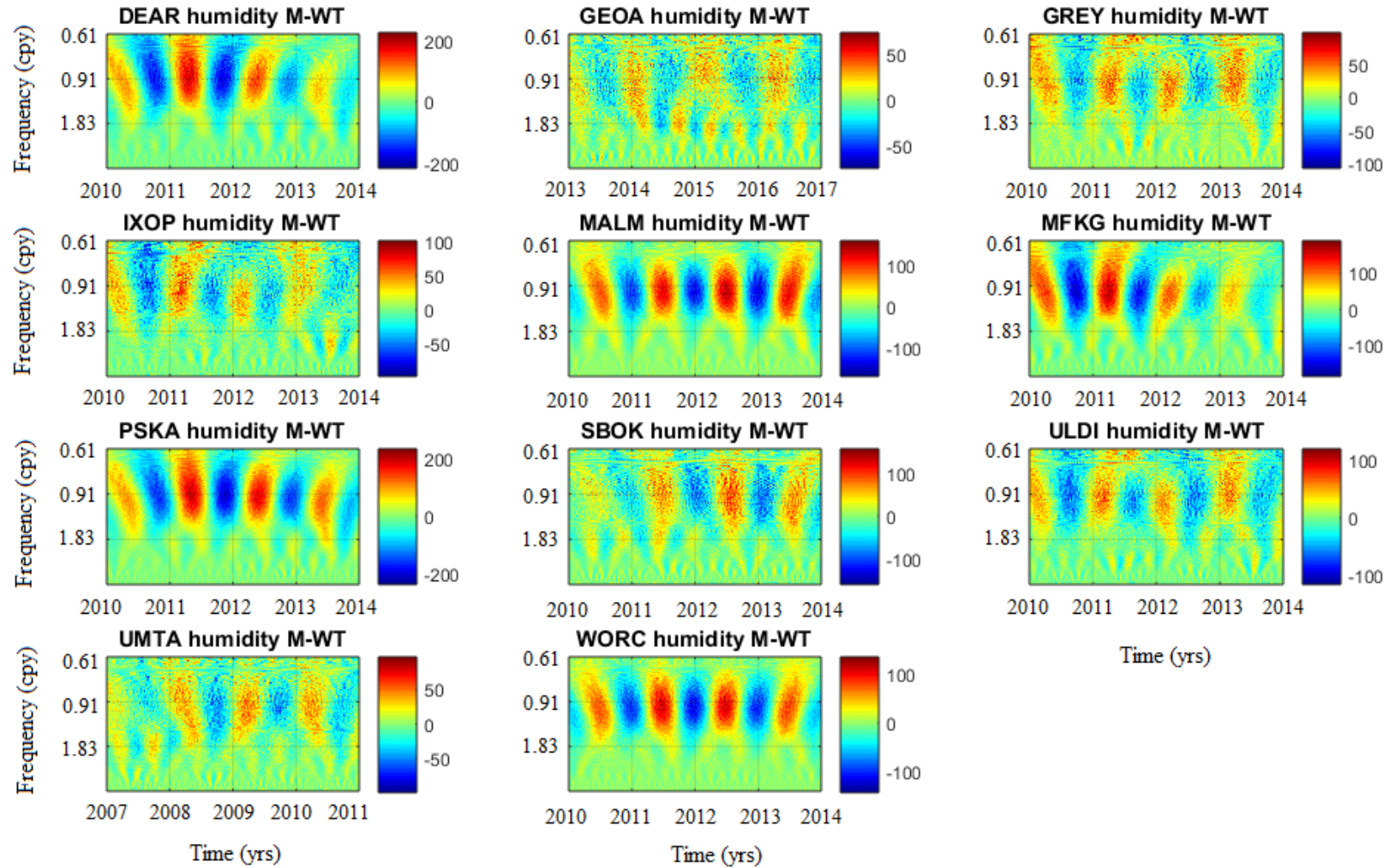
Figure 5.16: Humidity time series Morlet continuous wavelet transform (CWT) of the time series in Figure 5.8. The colour bar shows the variation of the CWT coefficients as a function of frequency and time. The bright red indicates a positive amplitude and the dark blue indicates a negative amplitude.
