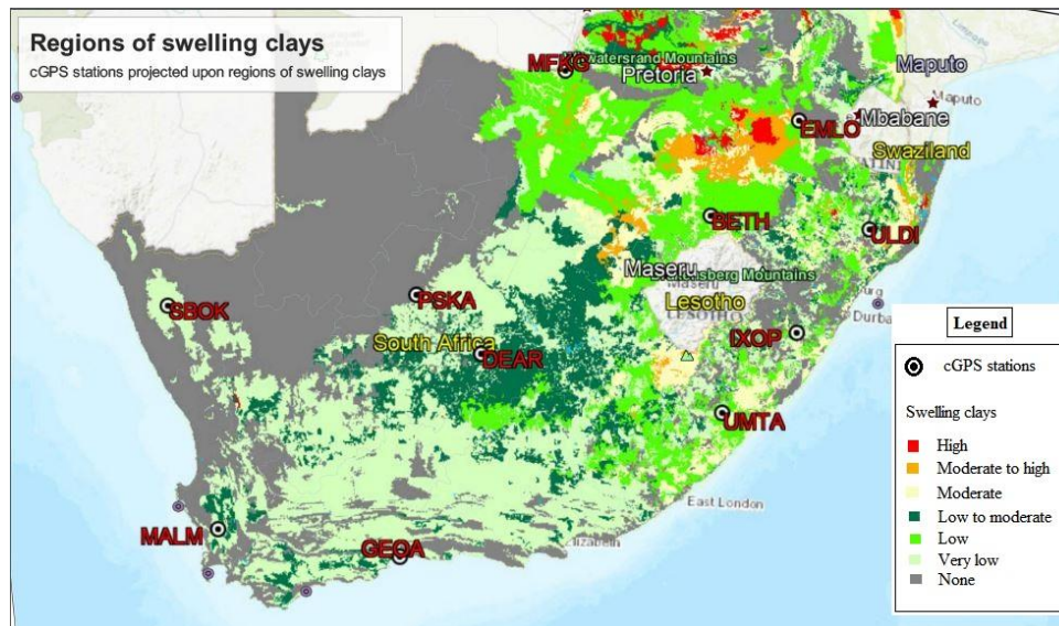
Figure 6.3: cGPS station locations projected upon regions of swelling clays across South Africa ( http://197.96.144.125/jsviewer/Geohazards/index.html , accessed on the 02-03-2019).
