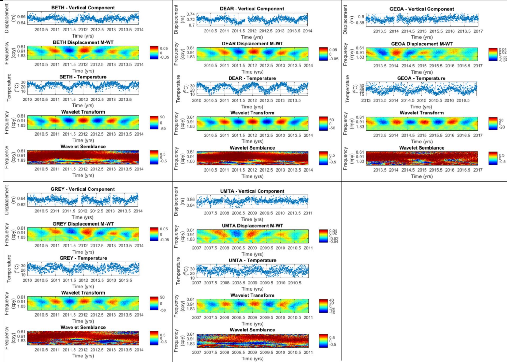
Figure 9.10: Additional semblance correlation plots of cGPS displacement time series (m) vs average temperature time series (°C).
