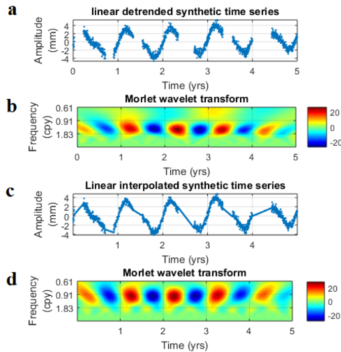
Figure 4.14: Effects of missing data (gaps) on the complex continuous wavelet transform (CWT). (a) Time series with the same properties as that in Figure 4.11c, but with missing values. (b) Real part of the complex CWT of time series in (a). The bright red indicates a positive amplitude and the dark blue indicates a negative amplitude. (c) Linear interpolated time series with the same parameters as the time series in (a). (d) Real part of the complex CWT of time series in (c). The colour bar shows the variation of the CWT coefficients as a function of frequency and time. The bright red indicates a positive amplitude and the dark blue indicates a negative amplitude.
