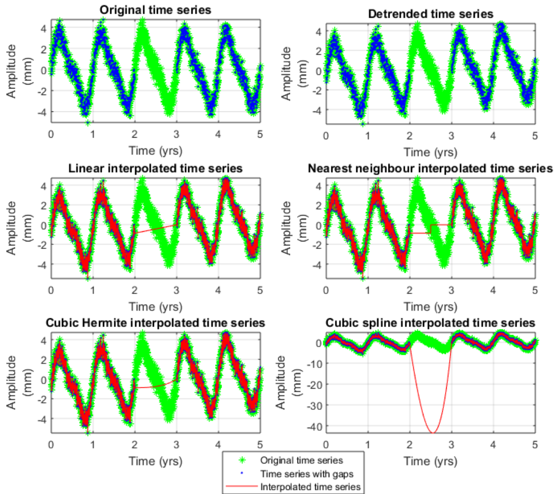
Figure 9.5: Synthetic time series T5 (with 20% missing data points), used in the variance test in chapter 4.2 and the response of the interpolation methods when applied to the noise contaminated time series. (a) Noise-contaminated synthetic time series without gaps (green) and with gaps (blue). (b) Detrended time series. (c) Linear interpolated time series. (d) Nearest neighbour interpolated time series). (e) Piecewise cubic Hermite interpolated time series. (f) Piecewise cubic spline interpolated time series.
