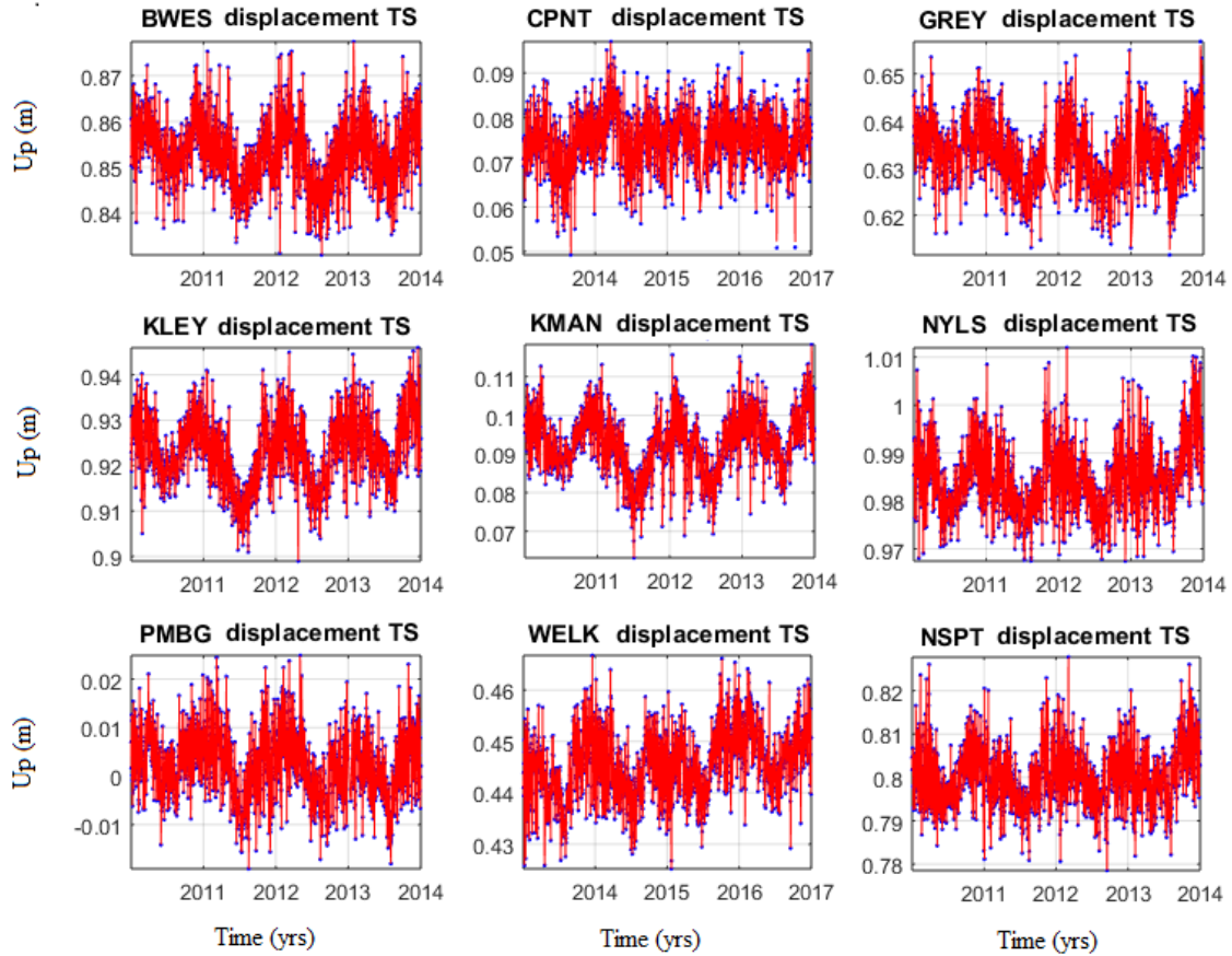
Figure 9.14: Time domain plots of the addition displacement time series
