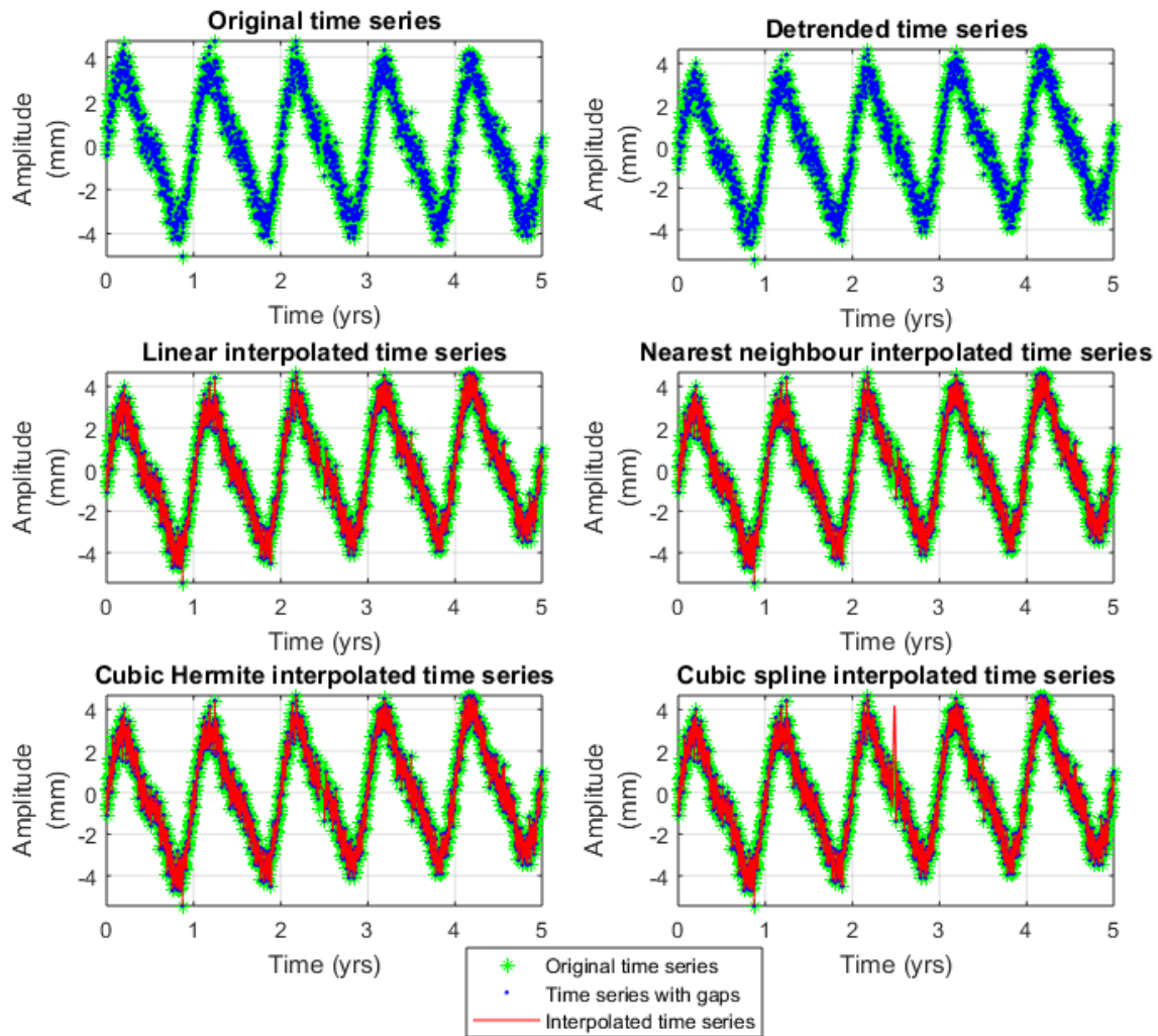
Figure 9.1: Synthetic time series T1 (with 2% missing data points), used in the variance test in chapter 4.2 and the response of the interpolation methods when applied to the noise contaminated time series. (a) Noise-contaminated synthetic time series without gaps (green) and with gaps (blue). (b) Detrended time series. (c) Linear interpolated time series. (d) Nearest neighbour interpolated time series. (e) Piecewise cubic Hermite interpolated time series. (f) Piecewise cubic spline interpolated time series.
