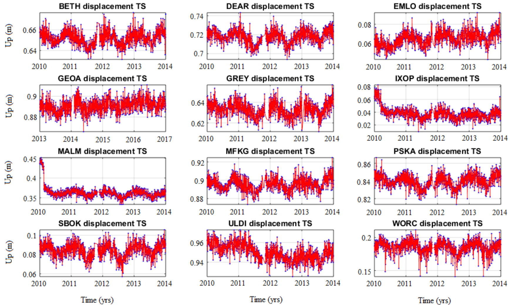
Figure 5.2: Daily position vertical component cGPS surface displacement time series. The blue points in the cGPS time series plots are the original data points and the red continuous line is the cubic Hermite interpolated time series.
