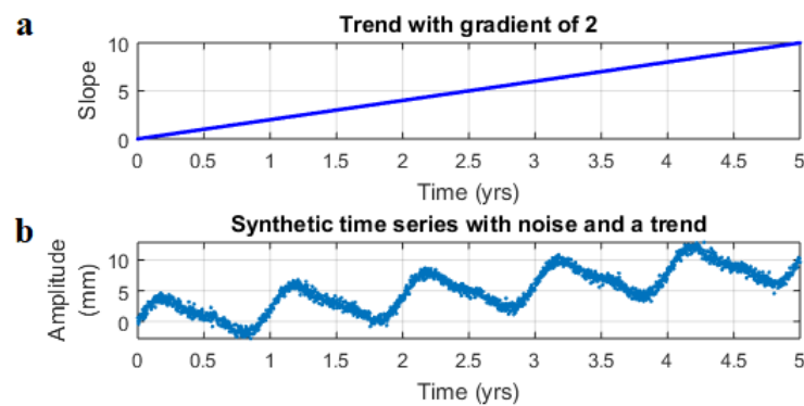
Figure 4.4: (a) Trend with a slope of 2 and a y-intercept of zero. (b) Time series obtained by adding the noise contaminated time series in Figure 4.3 and the trend in (a).
