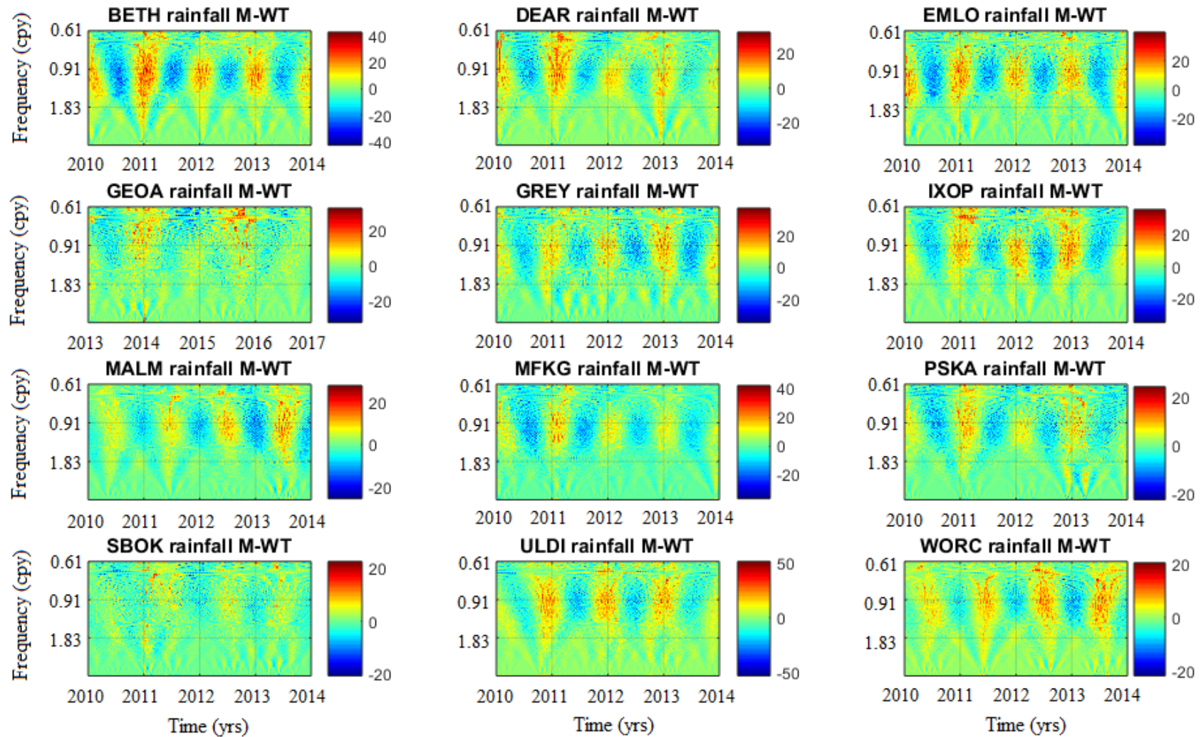
Figure 5.15: Rainfall time series Morlet continuous wavelet transform (CWT) of the time series in Figure 5.7. The colour bar shows the variation of the CWT coefficients as a function of frequency and time. The bright red indicates a positive amplitude and the dark blue indicates a negative amplitude.
