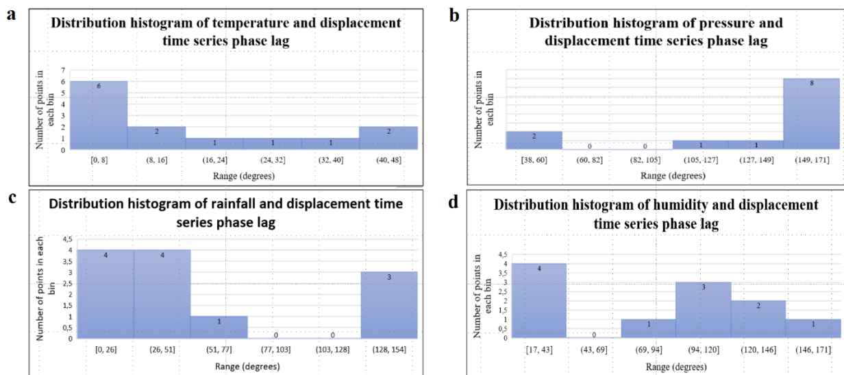
Figure 5.21: Phase lag distribution histograms for the considered meteorological processes.
