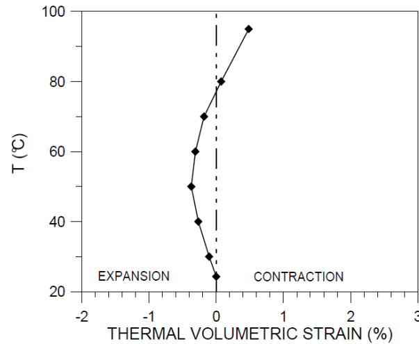
Figure 6.1: Thermal expansion curve of expansive Boom clay soil with an OCR of 2 (Delage et al., 2000)
