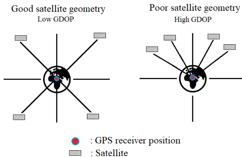
Figure 2.6: The effect of satellite configuration on position calculations. Evaluating the Geometric Dilution of Precision (GDOP).
