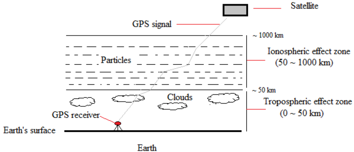
Figure 2.3: Tropospheric and ionospheric error sources and zones.
