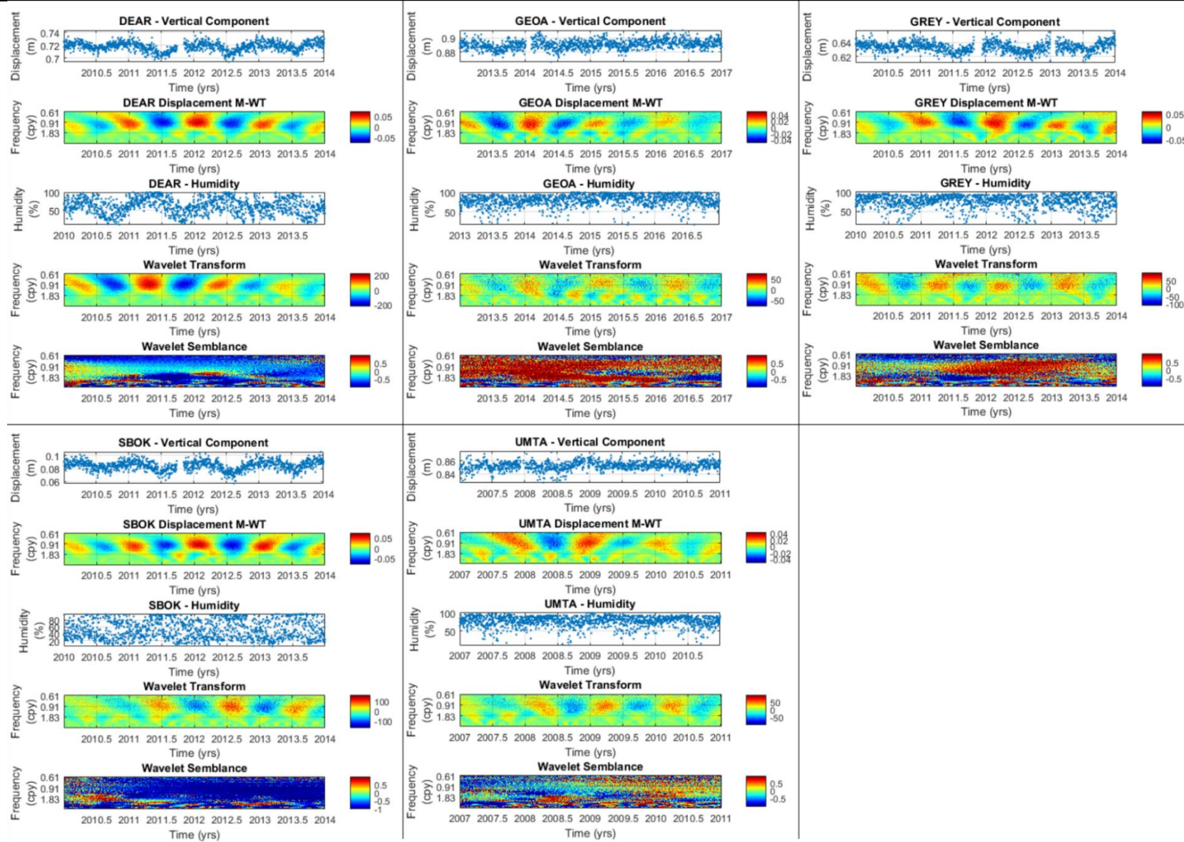
Figure 9.13: Additional semblance correlation plots of cGPS displacement time series (m) vs humidity time series (%).
