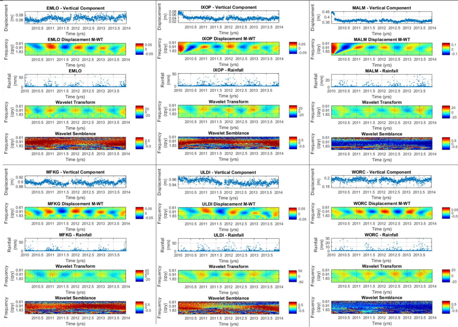
Figure 9.12: Additional semblance correlation plots of cGPS displacement time series (m) vs rainfall time series (mm).
