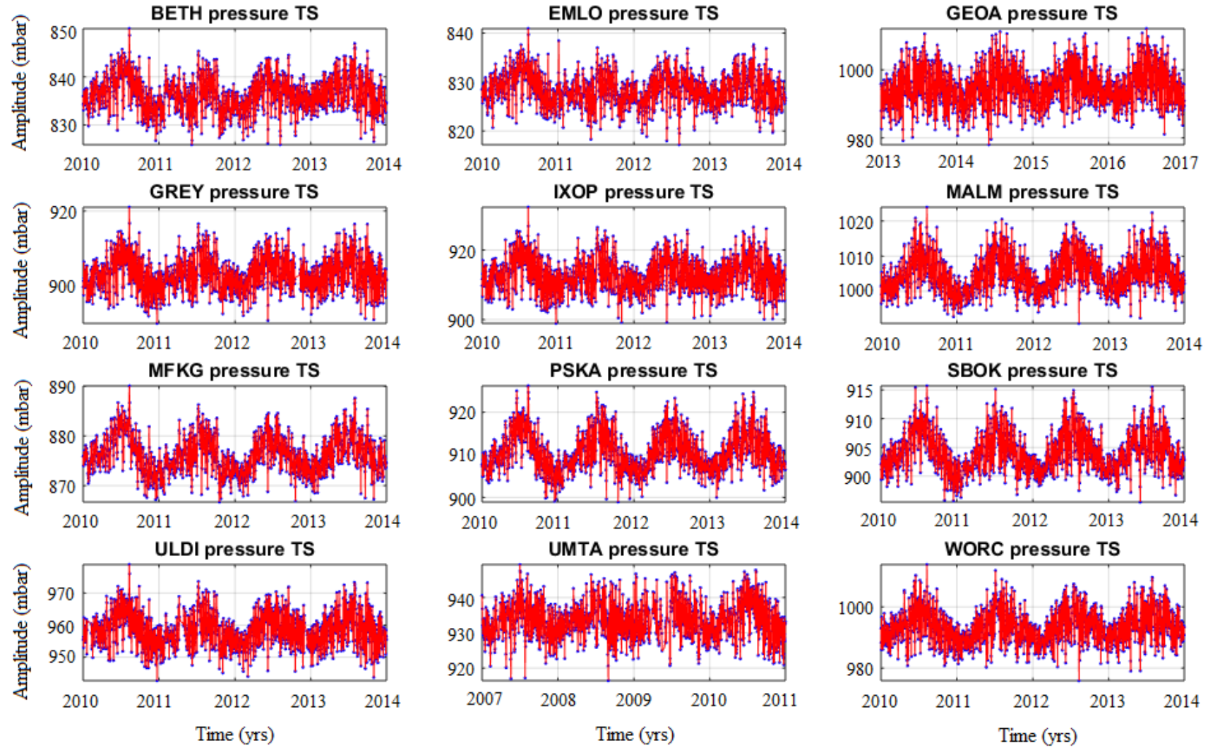
Figure 5.6: Atmospheric pressure time series. The blue points in the cGPS time series plots are the original data points and the red continuous line is the cubic Hermite interpolated time series.
