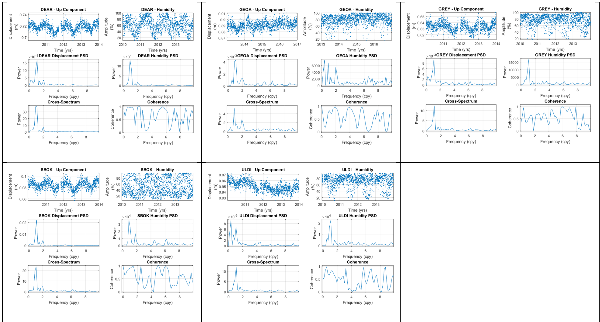
Figure 9.9: Additional cross-spectrum and coherence correlation plots of cGPS displacement (m) vs humidity (%) time series.
