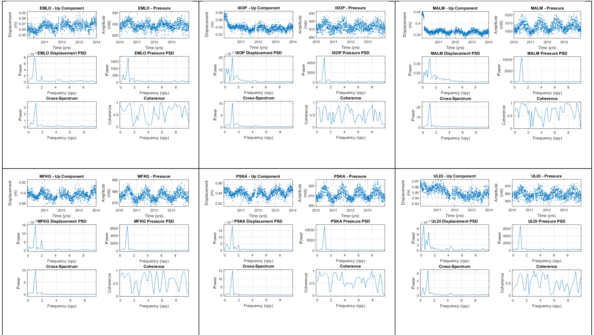
Figure 5.18: Cross-spectrum and coherence correlation plots of cGPS displacement (m) vs pressure (mbar) time series.
