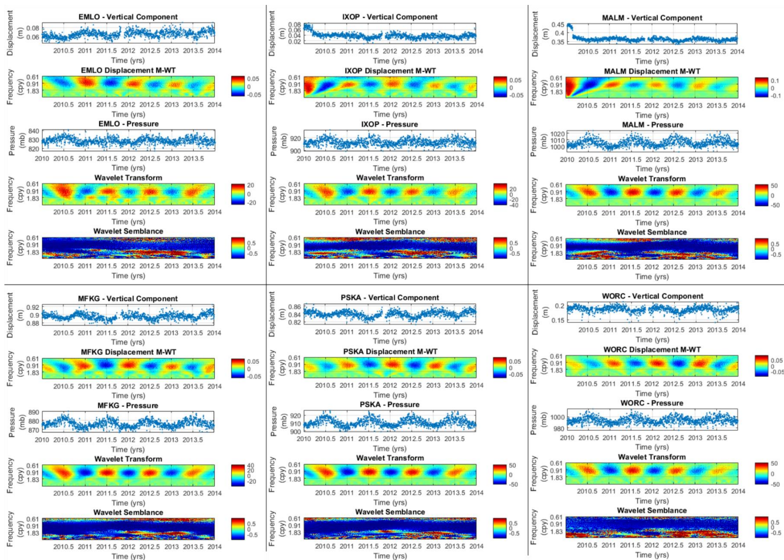
Figure 5.23: Semblance correlation plots of cGPS displacement time series (m) vs atmospheric pressure time series (mbar).
