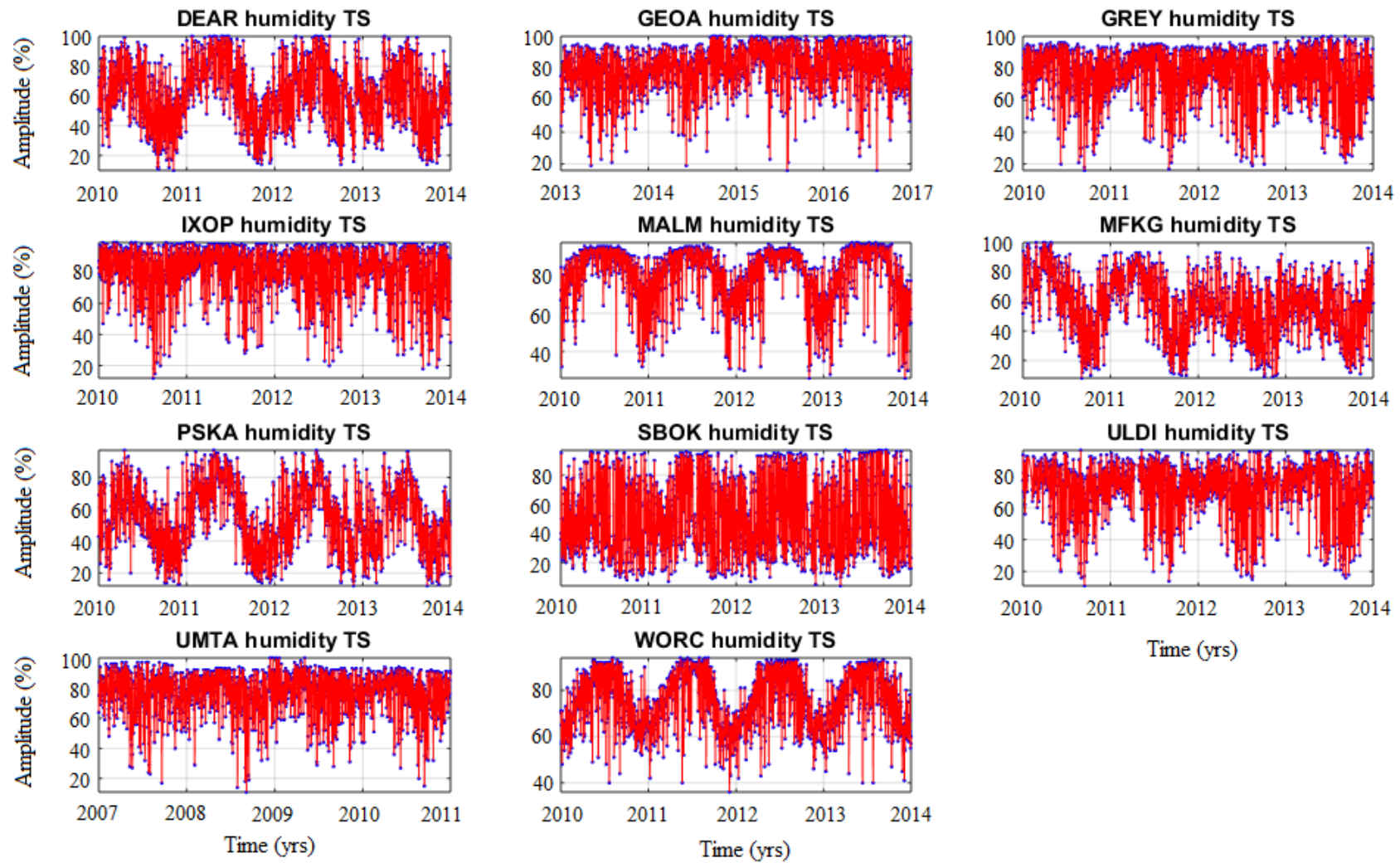
Figure 5.8: Humidity time series. The blue points in the cGPS time series plots are the original data points and the red continuous line is the cubic Hermite interpolated time series.
