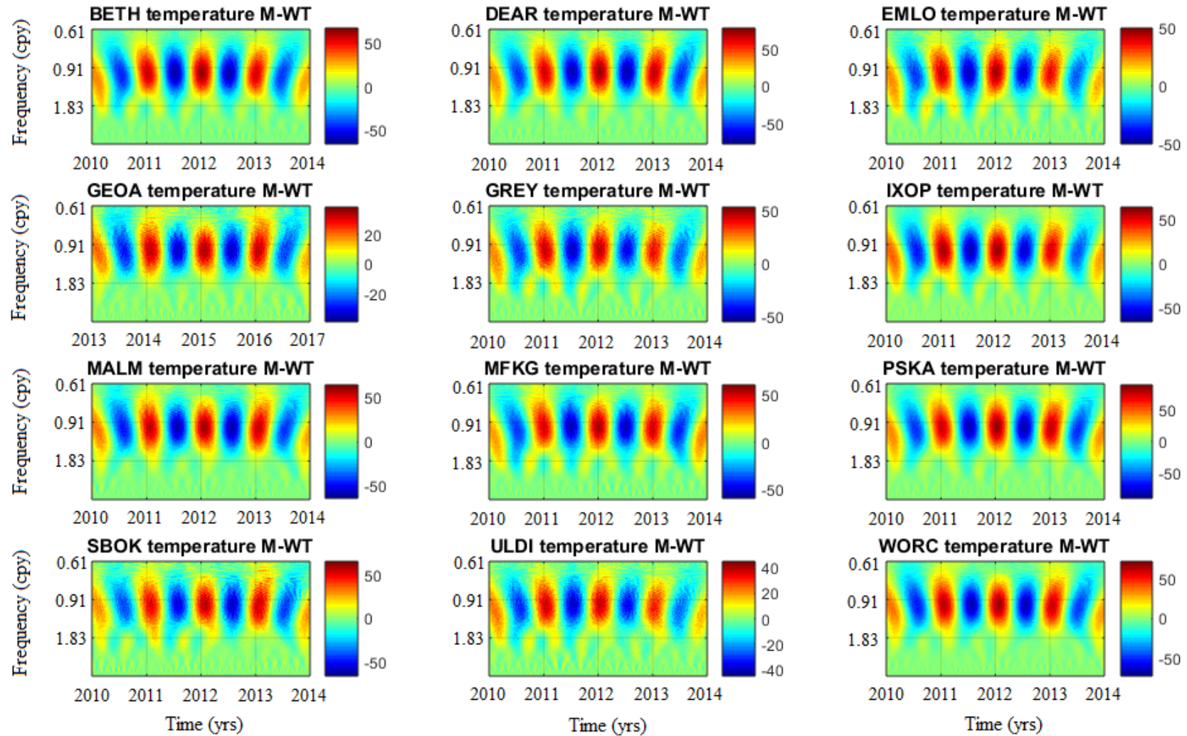
Figure 5.13: Surface air temperature time series Morlet continuous wavelet transform (CWT) of the time series in Figure 5.5. The colour bar shows the variation of the CWT coefficients as a function of frequency and time. The bright red indicates a positive amplitude and the dark blue indicates a negative amplitude.
