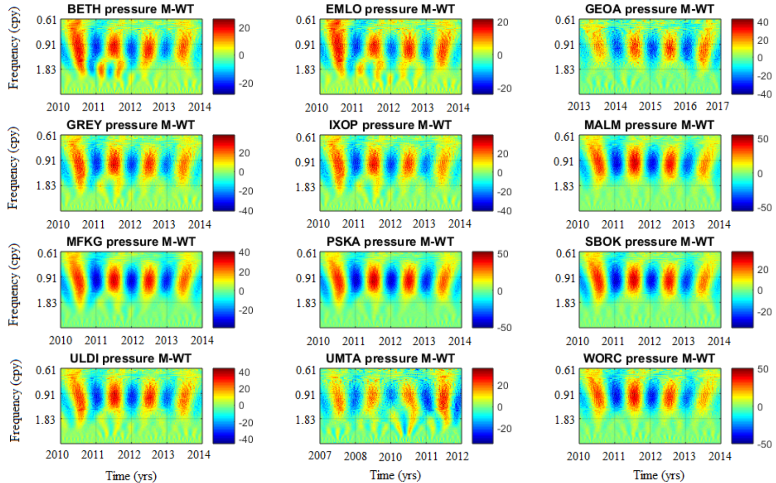
Figure 5.14: Atmospheric pressure time series Morlet continuous wavelet transform (CWT) of the time series in Figure 5.6. The colour bar shows the variation of the CWT coefficients as a function of frequency and time. The bright red indicates a positive amplitude and the dark blue indicates a negative amplitude.
