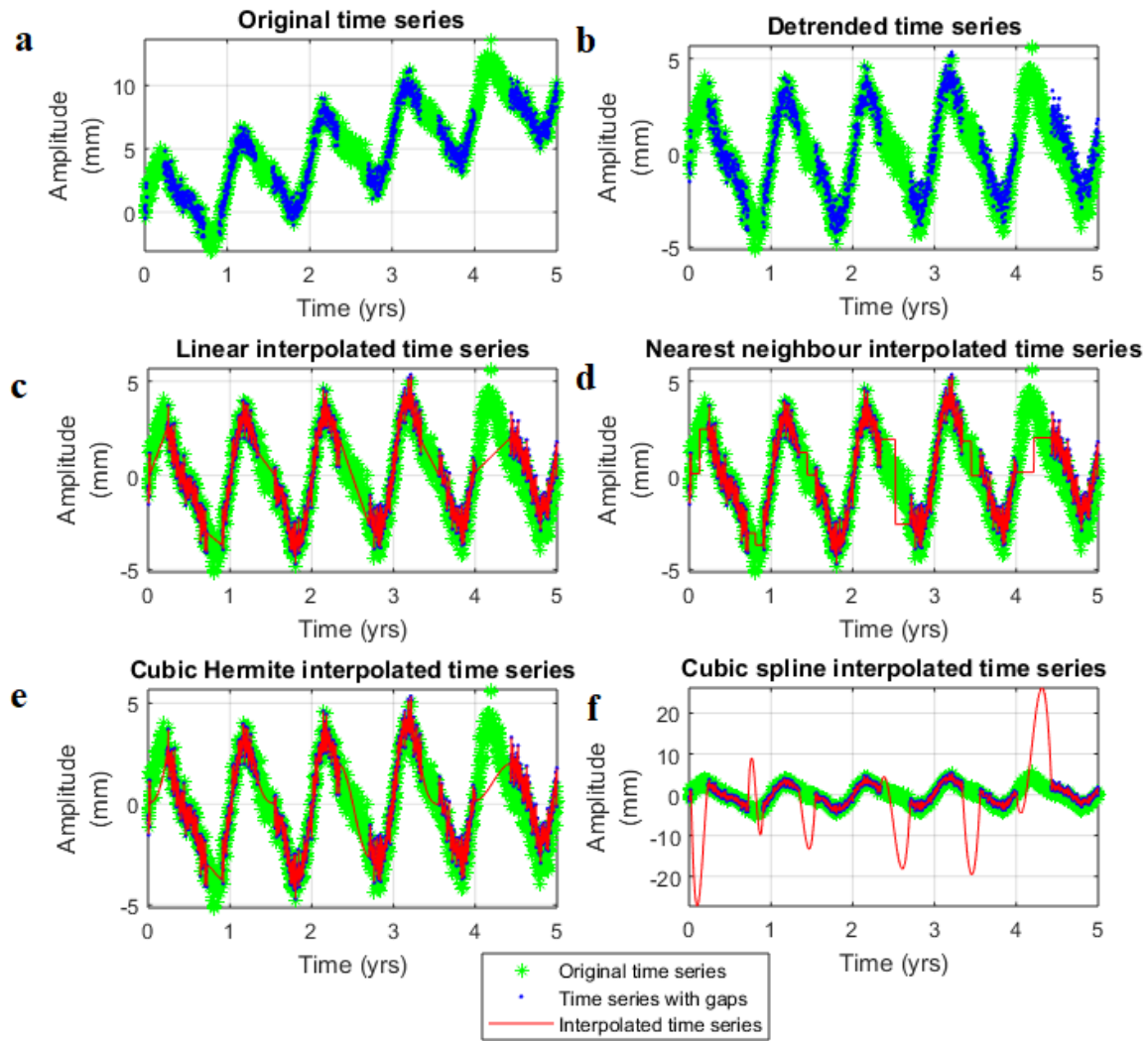
Figure 4.8: Response of the interpolation methods when applied to a noise-contaminated synthetic time series. (a) Noise-contaminated synthetic time series without gaps (green) and with gaps (blue). (b) Detrended time series. (c) Linear interpolated time series. (d) Nearest neighbour interpolated time series. (e) Piecewise cubic Hermite interpolated time series. (f) Piecewise cubic spline interpolated time series.
