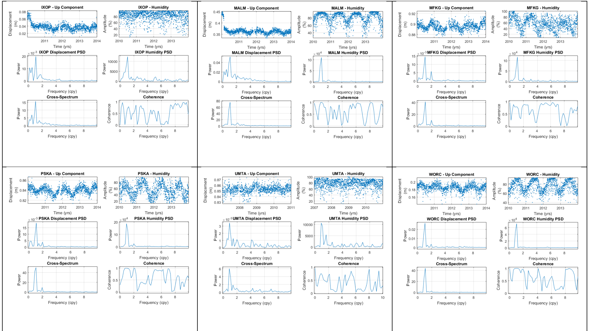
Figure 5.20: Cross-spectrum and coherence correlation plots of cGPS displacement (m) vs humidity (%) time series.
