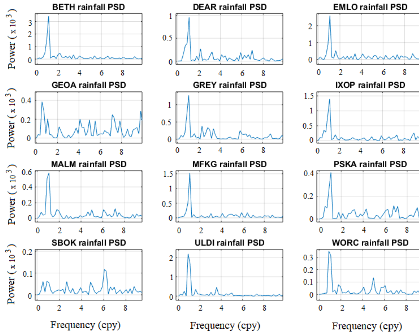
Figure 5.11: Rainfall time series Fast Fourier Transforms (FFT) Power Spectral Density (PSD) spectra of the time series in Figure 5.7.
