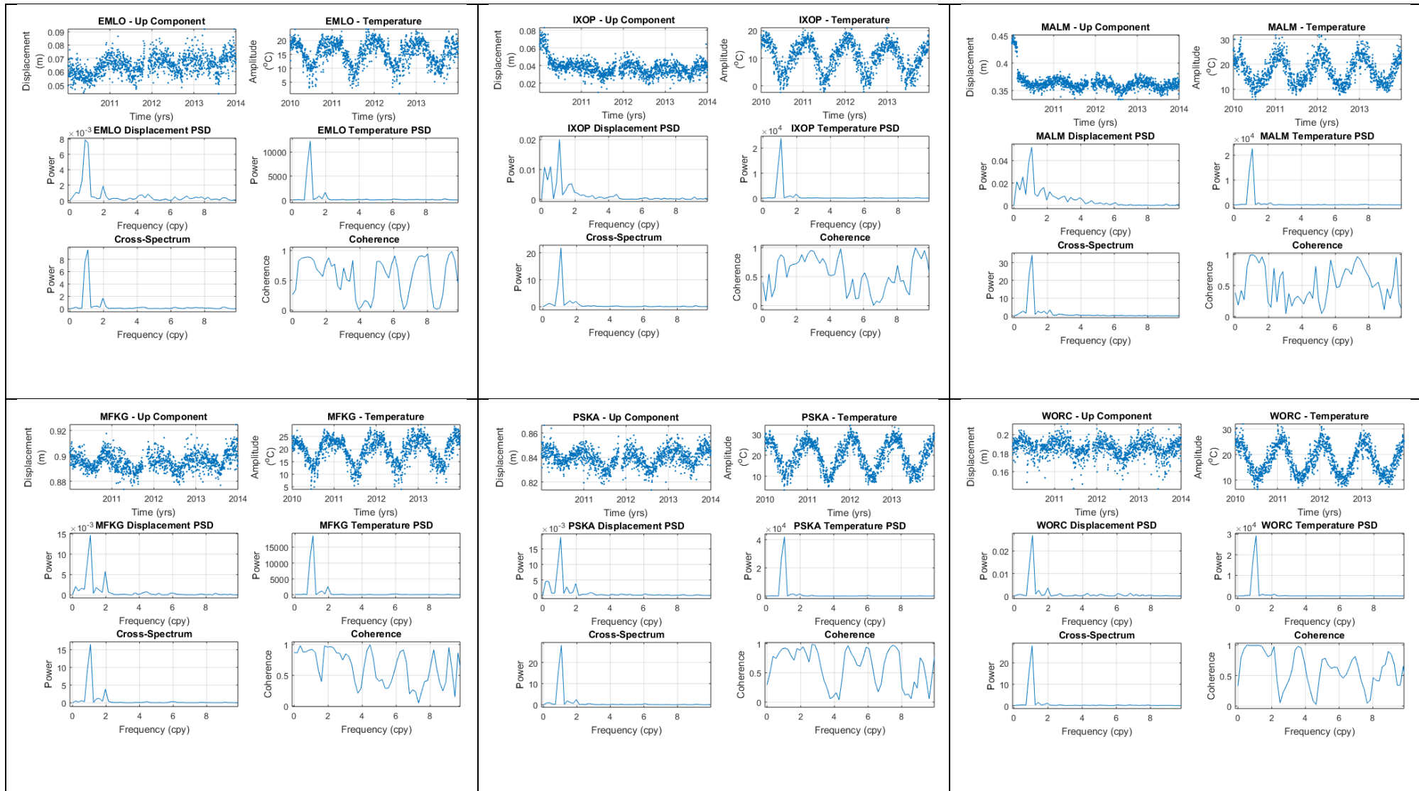
Figure 9.6: Additional Cross-spectrum and coherence correlation plots of cGPS displacement (m) vs average temperature (°C) time series.
