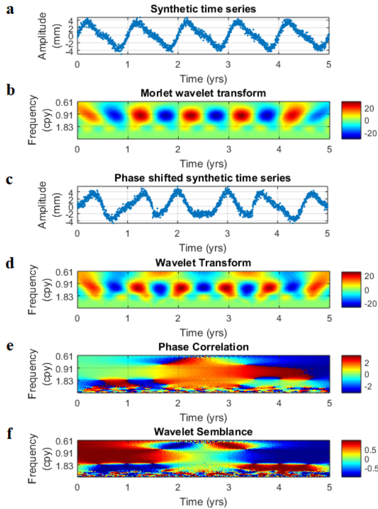
Figure 4.16: Wavelet transform, phase and semblance correlation spectrums. (a) Time series in Figure 4.11c. (b) Real part of the complex continuous wavelet transform (CWT) of the time series in (a). The bright red indicates a positive amplitude and the dark blue indicates a negative amplitude. (c) Time series in (a) with phase variations between the intervals at 0 - 1.5 yrs, 1.5 – 3.5 yrs and 3.5 - 5 yrs. (d) Real part of the complex CWT of time series in (c). (e) Phase correlation spectrum. (f) Wavelet semblance spectrum. The colour bar shows the variation of the CWT coefficients as a function of frequency and time. The bright red indicates a positive amplitude and the dark blue indicates a negative amplitude
