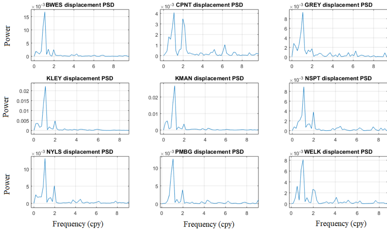
Figure 9.15: FFT transform of the addition displacement time series
