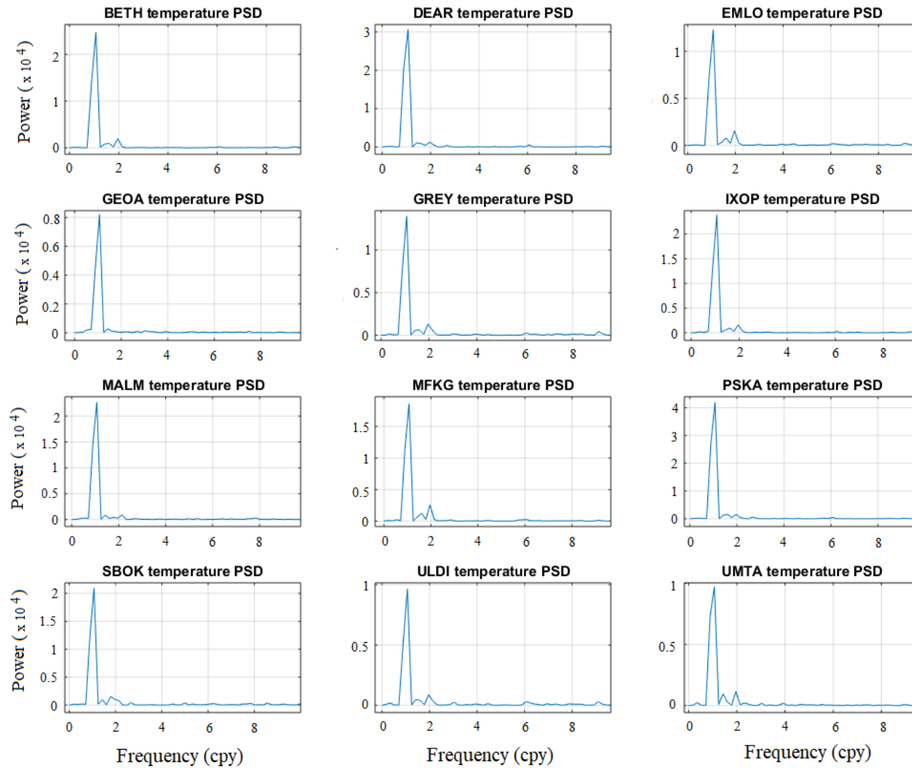
Figure 5.9: Surface air temperature Fast Fourier Transforms (FFT) Power Spectral Density (PSD) spectra of the time series in Figure 5.5.
