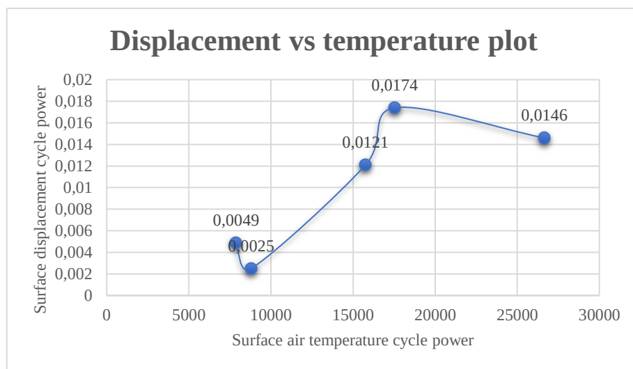
Figure 7.1: Surface air temperature cycle power vs surface displacement cycle power.
