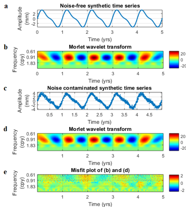
Figure 4.11: Synthetic data decomposition using the complex continuous wavelet transform (CWT). (a) Noise-free time series composed of an annual and semi-annual signal. The annual signal has an amplitude of 3 mm, while the semi-annual signal has an amplitude of 1 mm. (b) Real part of the complex CWT of the time series in (a). (c) Time series with the same signals as those in (a) but contaminated with a Gaussian noise of standard deviation of 0.5 mm. (d) Real part of the complex CWT of time series in (c). (e) Misfit plot of (b) and (d). The colour bar shows the variation of the CWT coefficients as a function of frequency and time. The colour bar shows the variation of the CWT coefficients as a function of frequency and time. The bright red bands indicate a positive amplitude and the dark blue bands indicates a negative amplitude.
