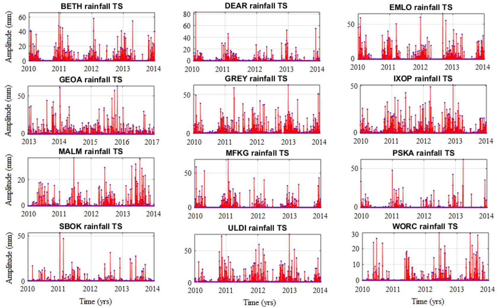
Figure 5.7: Rainfall time series. The blue points in the cGPS time series plots are the original data points and the red continuous line is the cubic Hermite interpolated time series.
