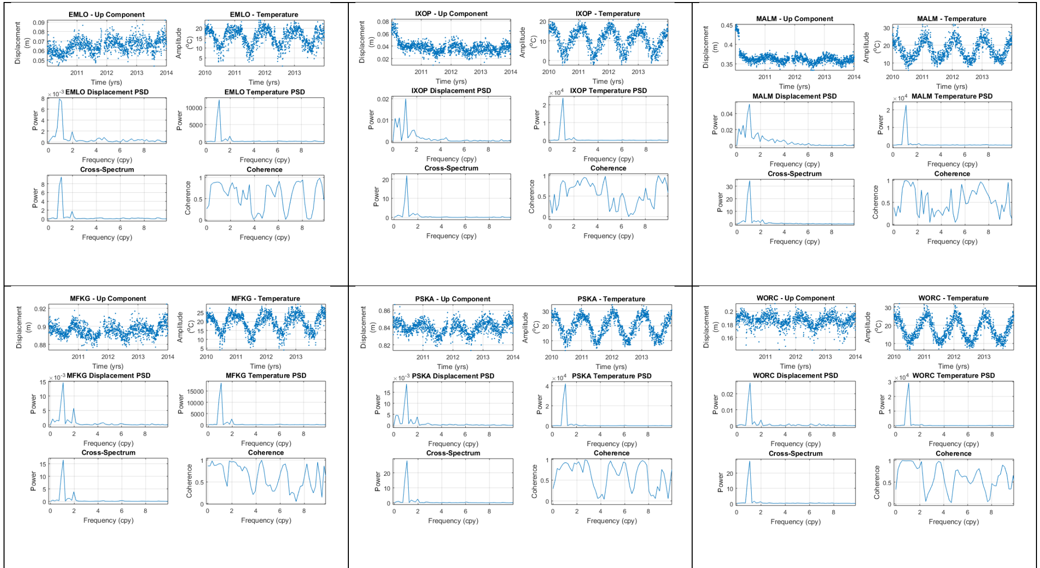
Figure 5.17: Cross-spectrum and coherence correlation plots of cGPS displacement (m) vs average temperature (°C) time series.
