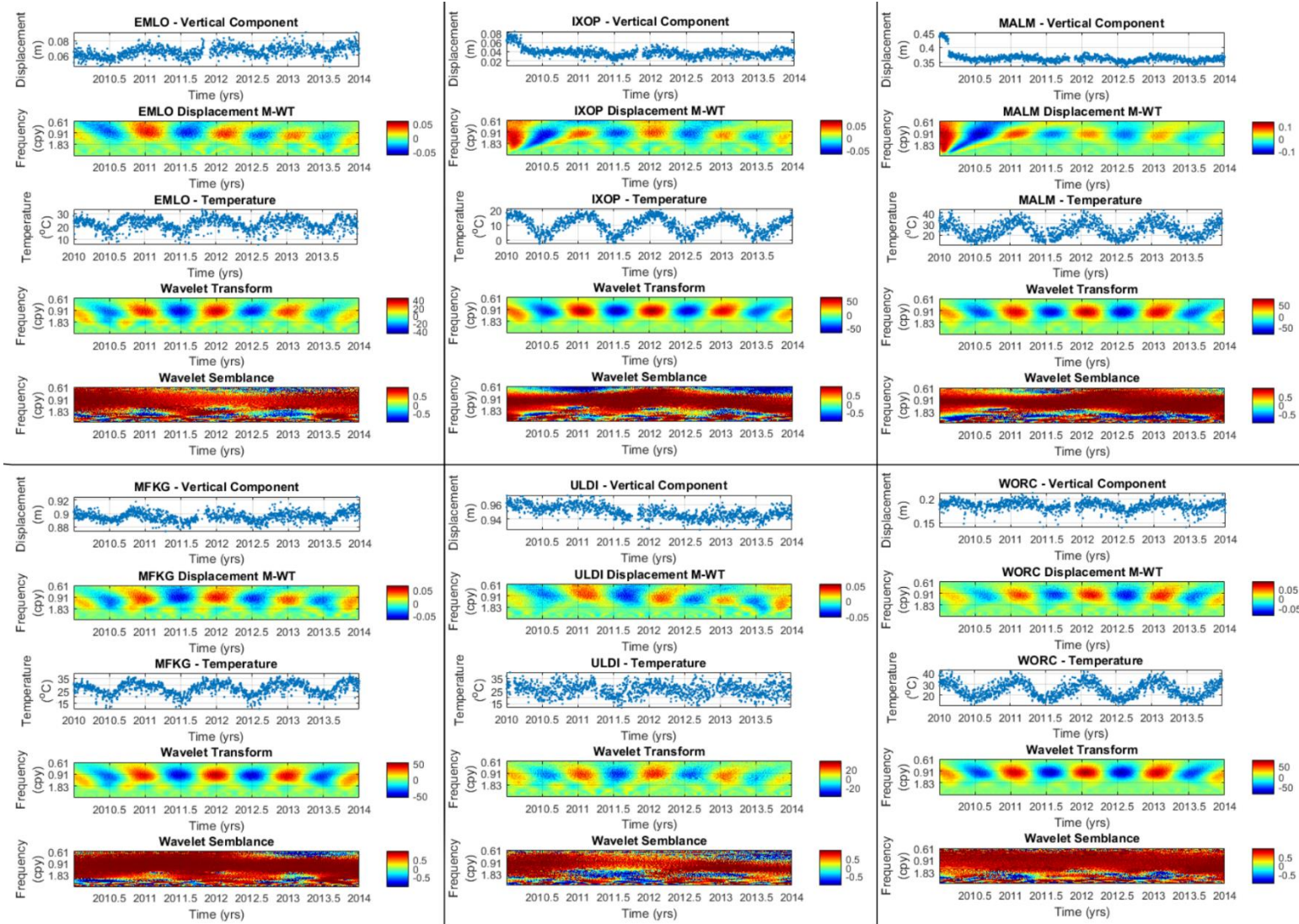
Figure 5.22: Sembance correlation plots of cGPS displacement time series (m) vs average temperature time series (°C)
