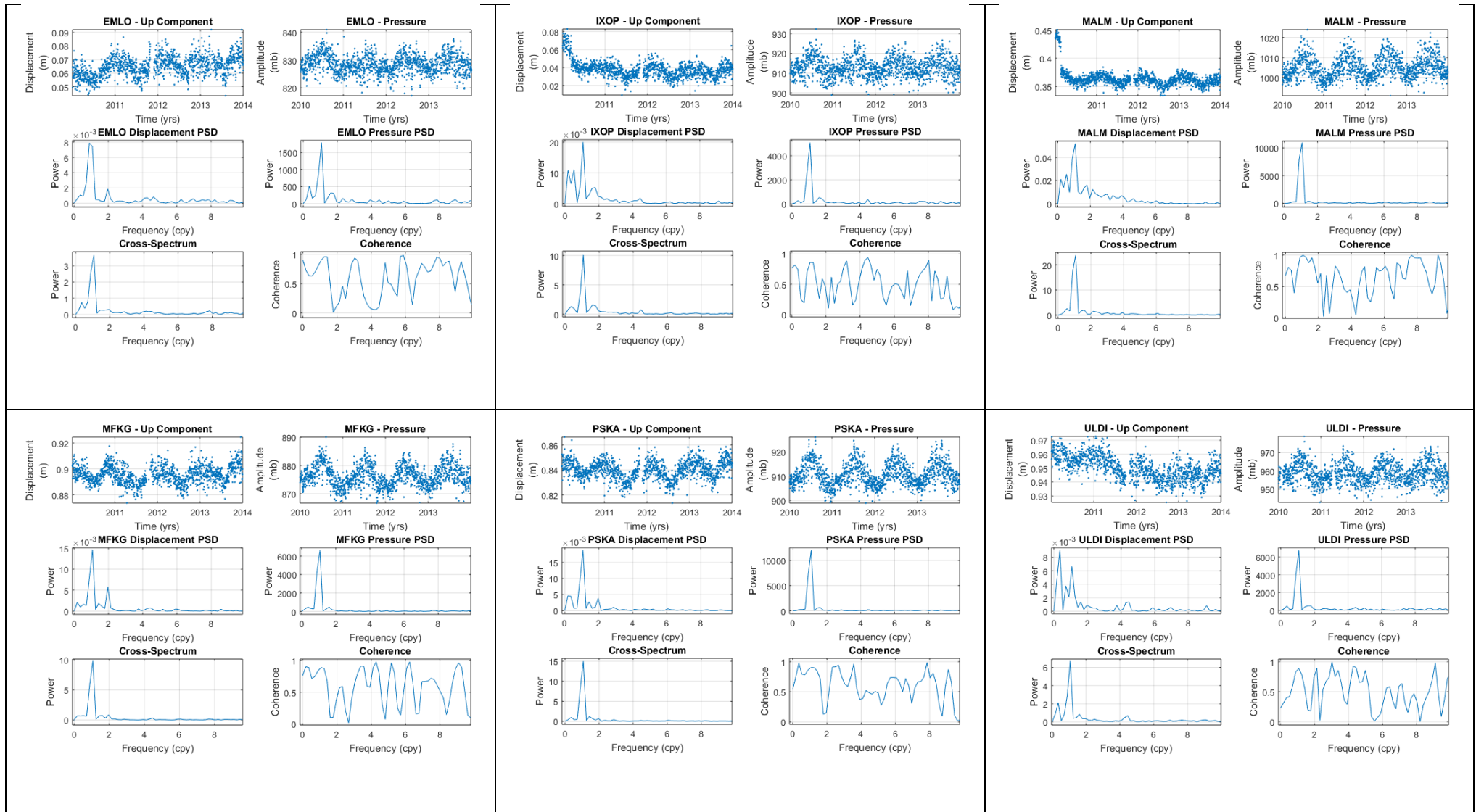
Figure 9.7: Additional cross-spectrum and coherence correlation plots of cGPS displacement (m) vs pressure (mbar) time series.
