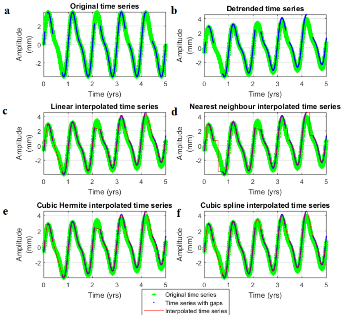
Figure 4.7: Response of the interpolation methods when applied to noise-free synthetic time series. (a) Noise-free synthetic time series without gaps (green) and with gaps (blue). (b) Detrended time series. (c) Linear interpolated time series. (d) Nearest neighbour interpolated time series. (e) Piecewise cubic Hermite interpolated time series. (f) Piecewise cubic spline interpolated time series.
