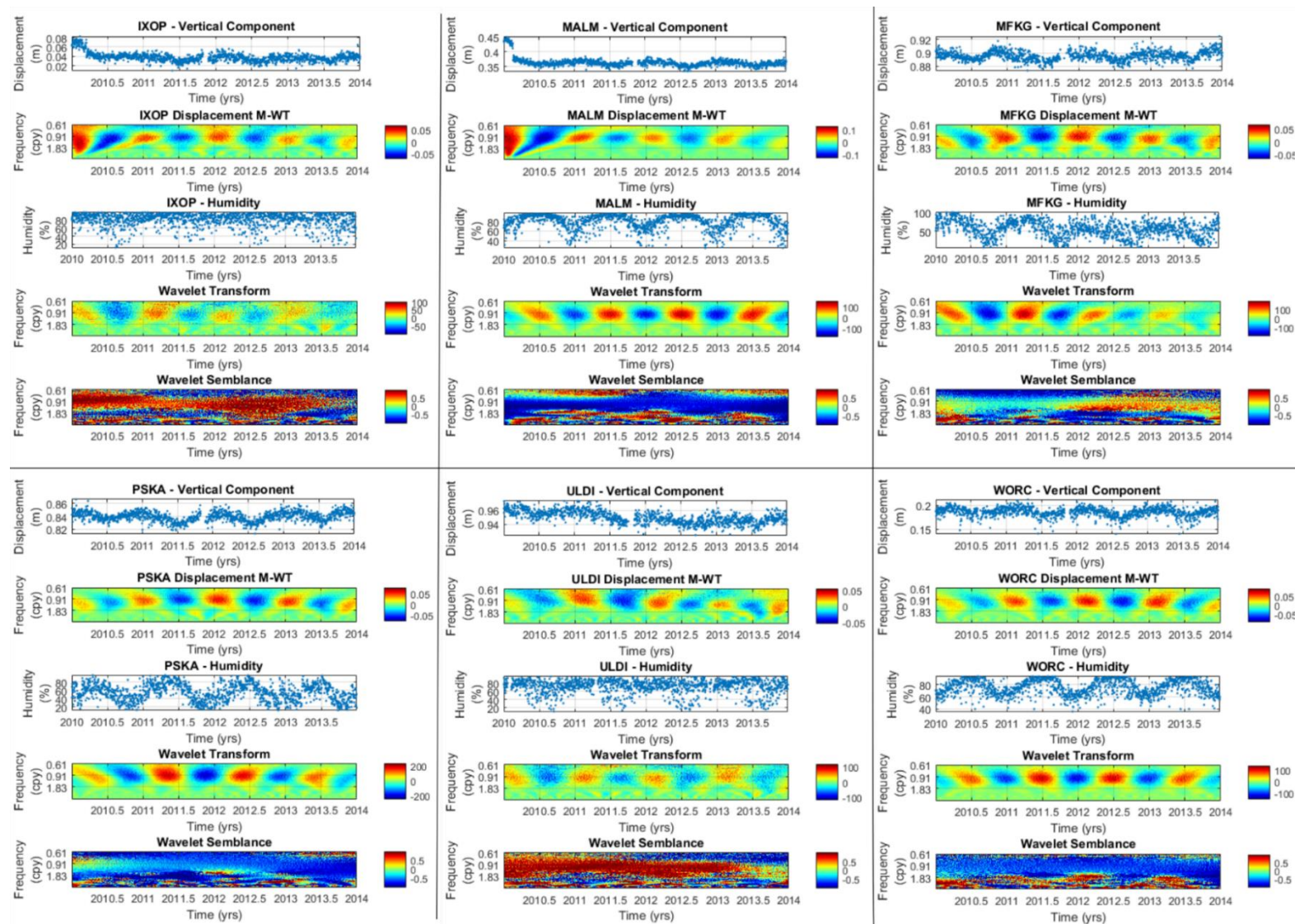
Figure 5.25: Semblance correlation plots of cGPS displacement time series (m) vs humidity time series (%).
