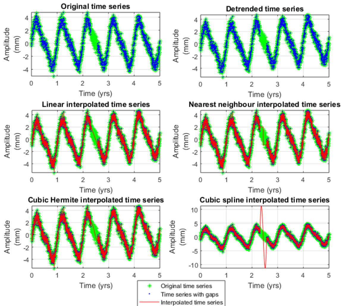
Figure 9.2: Synthetic time series T2 (with 5% missing data points), used in the variance test in chapter 4.2 and the response of the interpolation methods when applied to the noise contaminated time series. (a) Noise-contaminated synthetic time series without gaps (green) and with gaps (blue). (b) Detrended time series. (c) Linear interpolated time series. (d) Nearest neighbour interpolated time series). (e) Piecewise cubic Hermite interpolated time series. (f) Piecewise cubic spline interpolated time series.
