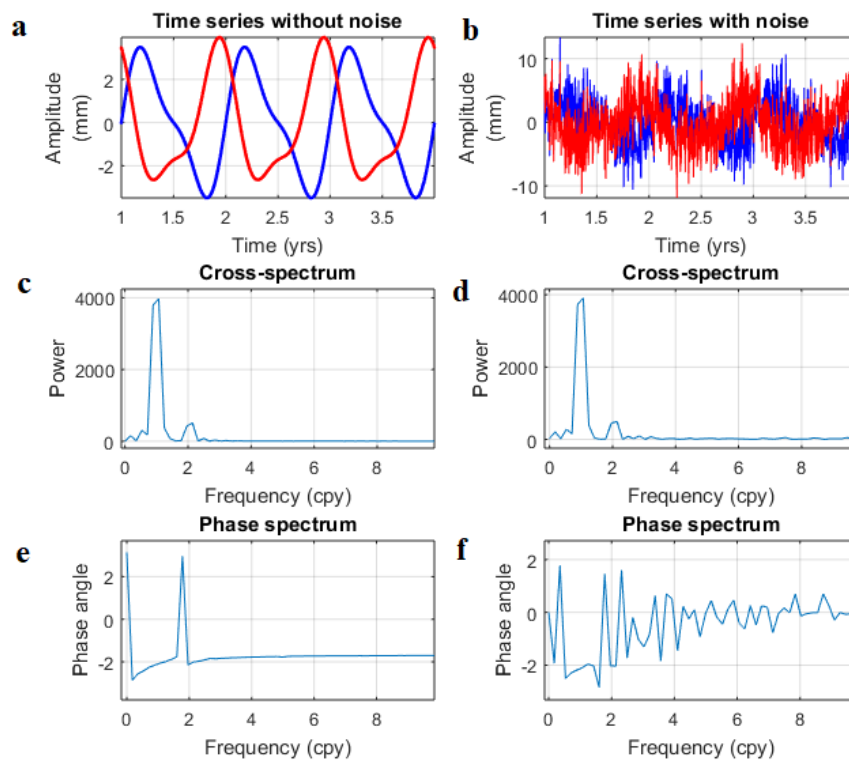
Figure 4.10: Cross-spectrum and phase tests. (a) Identical time series with a phase difference of 120 degrees (2.1 radians), both (blue and red) time series are composed of an annual and semi-annual signal. The annual signal has an amplitude of 3 mm, while the semi-annual signal has an amplitude of 1 mm. (b) Time series in (a) contaminated by Gaussian noise with a STD of 3 mm. (c) Cross-spectrum of the time series in (a). (d) Cross-spectrum of the time series in (b). (e) Phase spectrum of the time series in (a). (f) Phase spectrum of the time series in (d). The phase is given in radians.
