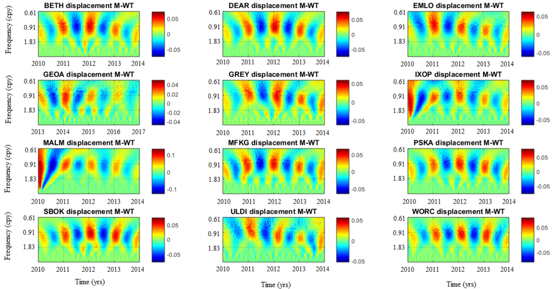
Figure 5.4: Morlet continuous wavelet transform (CWT) spectra of the daily position cGPS vertical displacement component time series in Figure 5.2. The colour bar shows the variation of the CWT coefficients as a function of frequency and time. The bright red indicates a positive amplitude and the dark blue indicates a negative amplitude.
