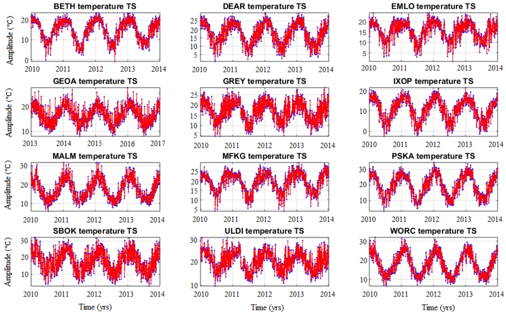
Figure 5.5: Average surface air temperature time series. The blue points in the cGPS time series plots are the original data points and the red continuous line is the cubic Hermite interpolated time series.
