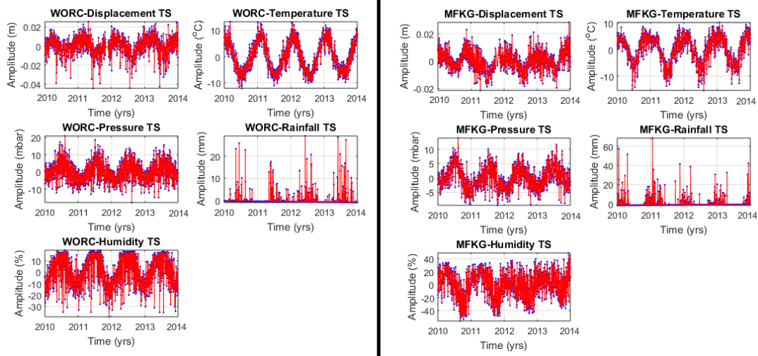
Figure 5.1: On the left-hand side of the black line are displacement and meteorology time series from Worcester (WORC), a town located in the south-western part of southern Africa, a winter rainfall region. On the right are displacement and meteorology time series at in Mafikeng (MFKG). Mafikeng is a summer rainfall region, located in the north-central part of South Africa. The displacement, temperature, pressure and humidity time series are zero centred so as to be able to easily see approximate amplitudes of the different datasets.
