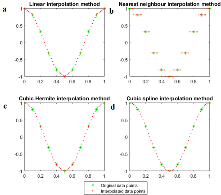
Figure 4.6: The green dots are known points of the original time series and the red dots are interpolation points obtained using different interpolation methods. The plots display how each of the considered interpolation methods interpolate for unknown data points.
