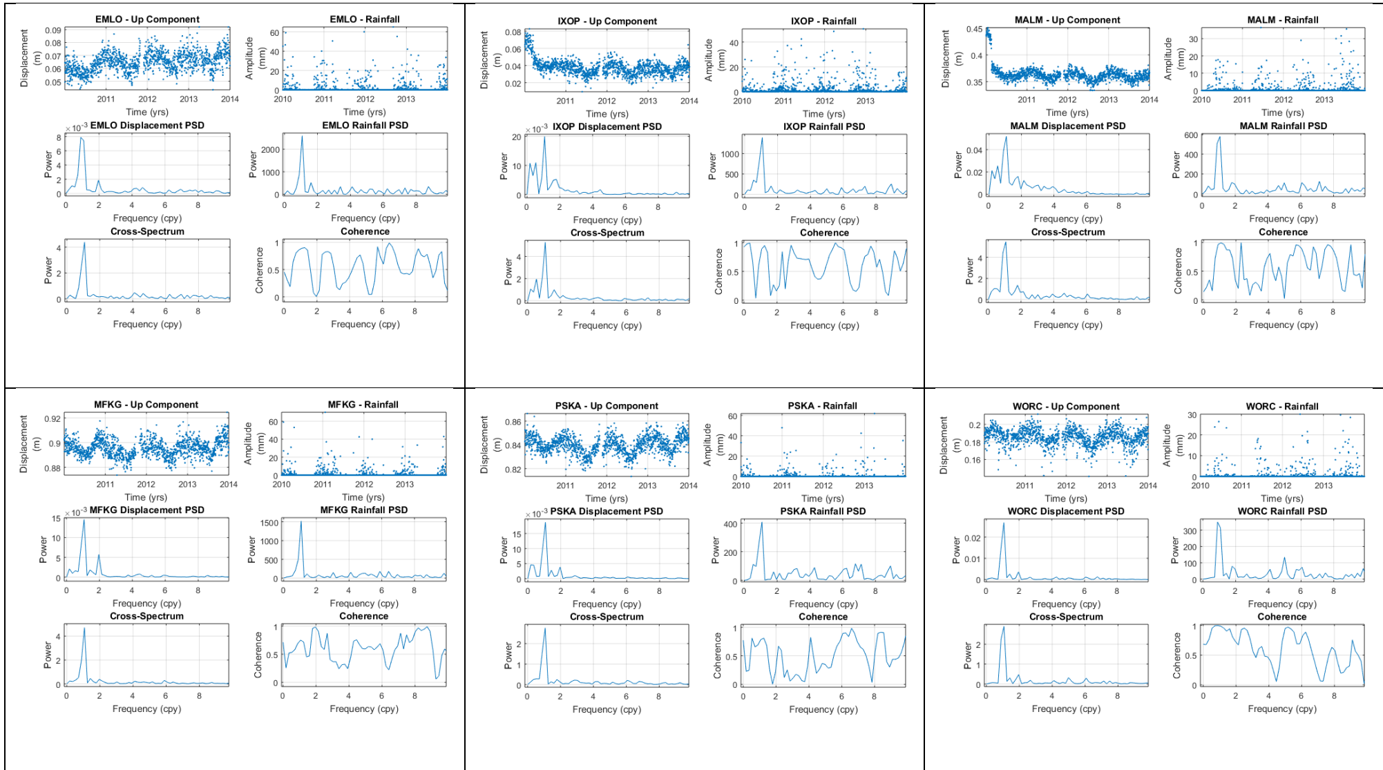
Figure 9.8: Additional cross-spectrum and coherence correlation plots of cGPS displacement (m) vs rainfall (mm) time series.
