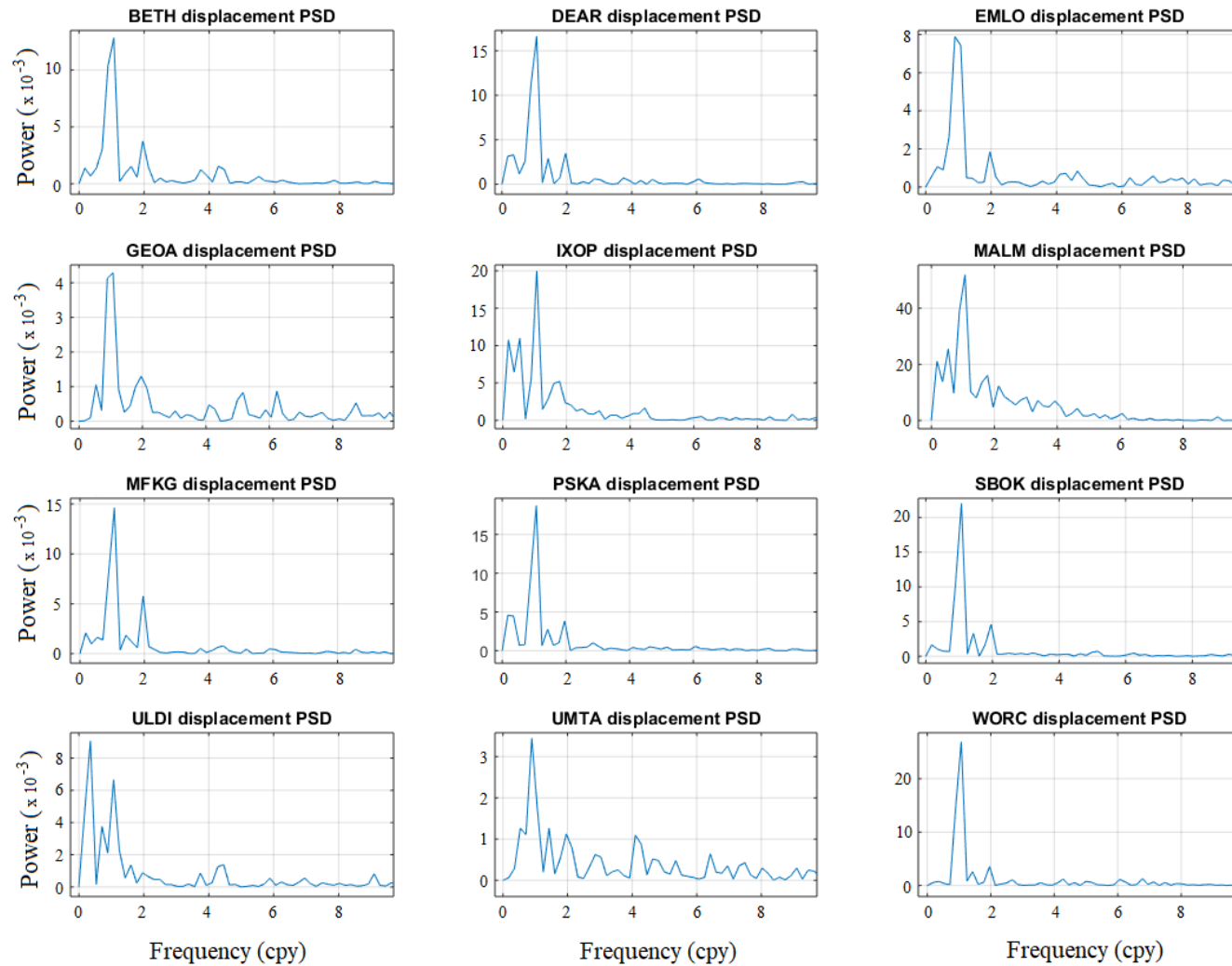
Figure 5.3: Daily position cGPS vertical (up) displacement component time series Fast Fourier Transforms (FFT) Power Spectral Density (PSD) spectra of the time series in Figure 5.2.
