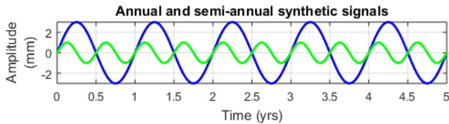
Figure 4.1: Annual (in blue) and semi-annual (in green) signals. Each year is composed of 365.2422 samples which are equivalent to the number of days. The annual signal is defined by a period of 1 year and the semi-annual signal is defined by a period of 6 months.
