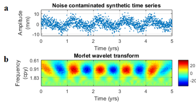
Figure 4.12: (a) Time series in Figure 4.11a contaminated with Gaussian noise of higher standard deviation, i.e., 3 mm. (b) Real part of the complex continuous wavelet transform (CWT) of time series in (a). The colour bar shows the variation of the CWT coefficients as a function of frequency and time. The colour bar shows the variation of the CWT coefficients as a function of frequency and time. The bright red indicates a positive amplitude and the dark blue indicates a negative amplitude.
