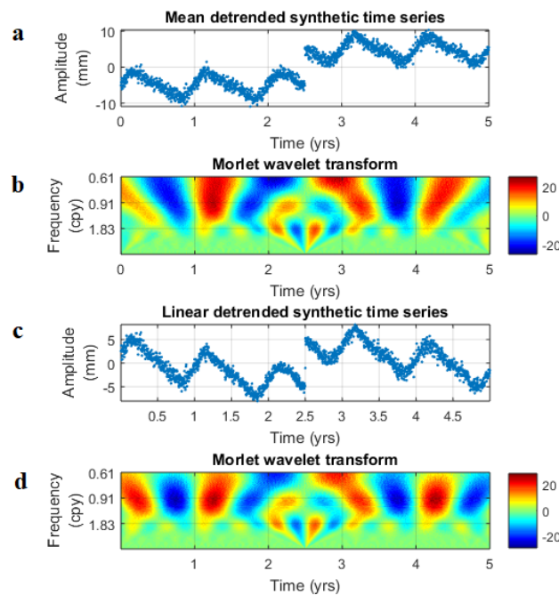
Figure 4.15: Morlet wavelet transform of mean shifted time series. (a) Time series in Figure 4.11c with a mean shift, the time series is detrended using a constant mean. (b) Real part of the complex continuous wavelet transform (CWT) of time series in (a). (c) Time series in Figure 4.11c detrended using a first order linear trend. (d) Real part of the complex CWT of the time series in (c). The colour bar shows the variation of the CWT coefficients as a function of frequency and time. The bright red indicates a positive amplitude and the dark blue indicates a negative amplitude.
