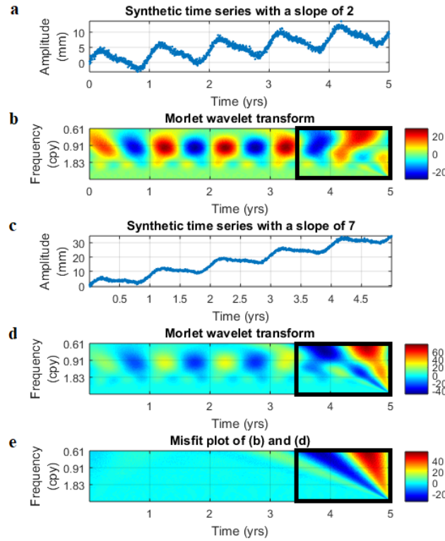
Figure 4.13: Effects of a trend when transforming data into the time-frequency domain using the complex continuous wavelet transform (CWT). (a) Time series with the same properties as that in Figure 4.11c plus a trend with a slope of 2 units. (b) Real part of the complex CWT of time series in (a). The bright red indicates a positive amplitude and the dark blue indicates a negative amplitude. (c) Time series with the same parameters as the time series in (a), but with a trend of higher slope (7 units). (d) Real part of the complex CWT of time series in (c). (e) Misfit plot of (b) and (d). The colour bar shows the variation of the CWT coefficients as a function of frequency and time. The bright red indicates a positive amplitude and the dark blue indicates a negative amplitude. The black boxes at approximately 3.4 to 5 yrs highlight the edge effects, regions of higher than normal CWT coefficients, induced by the presence of a trend.
