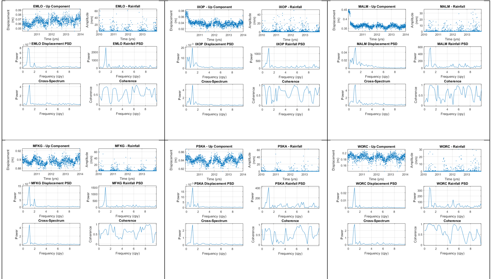
Figure 5.19: Cross-spectrum and coherence correlation plots of cGPS displacement (m) vs rainfall (mm) time series.
