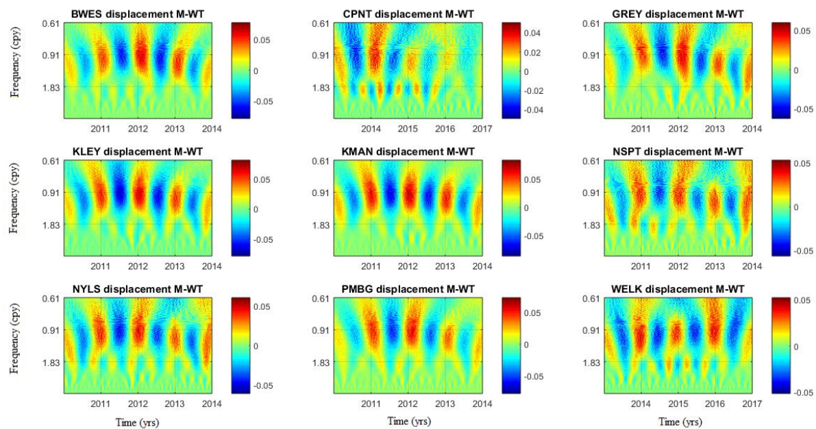
Figure 9.16: Morlet wavelet transform of the addition displacement time series.
