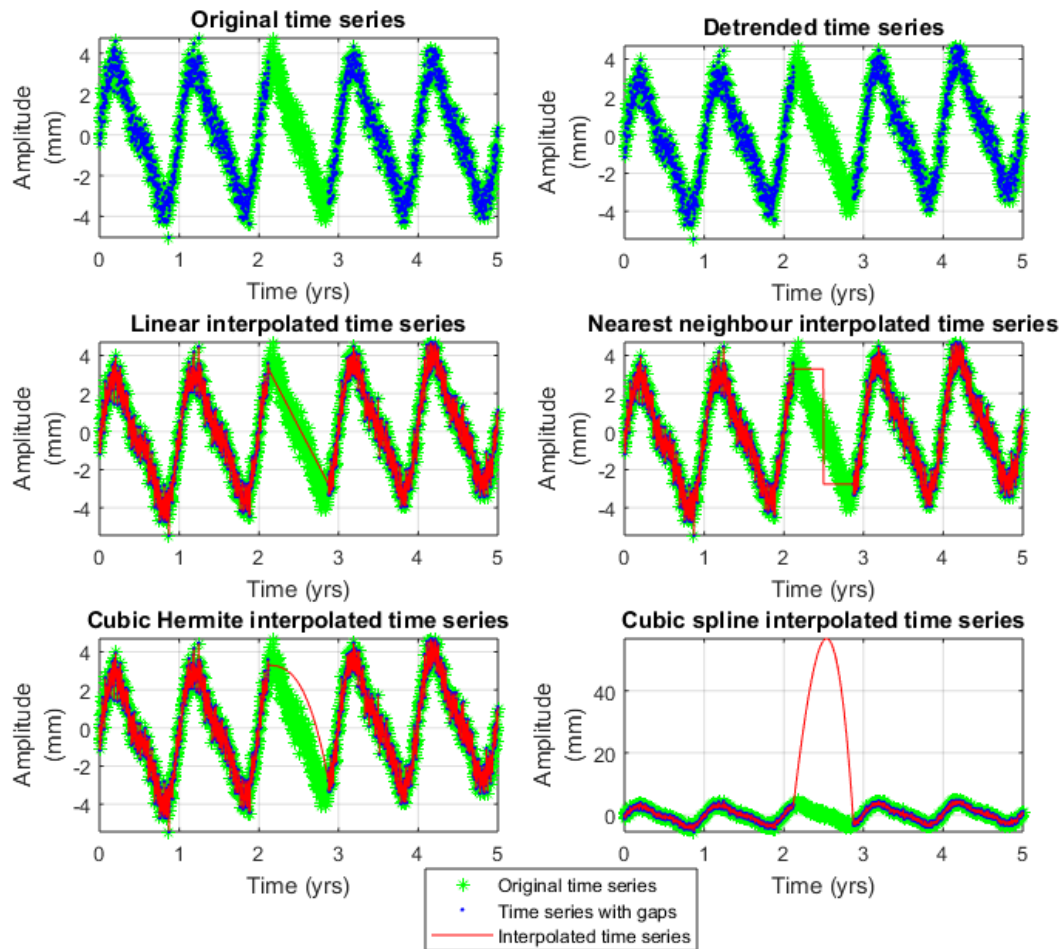
Figure 9.4: Synthetic time series T4 (with 15% missing data points), used in the variance test in chapter 4.2 and the response of the interpolation methods when applied to the noise contaminated time series. (a) Noise-contaminated synthetic time series without gaps (green) and with gaps (blue). (b) Detrended time series. (c) Linear interpolated time series. (d) Nearest neighbour interpolated time series). (e) Piecewise cubic Hermite interpolated time series. (f) Piecewise cubic spline interpolated time series.
