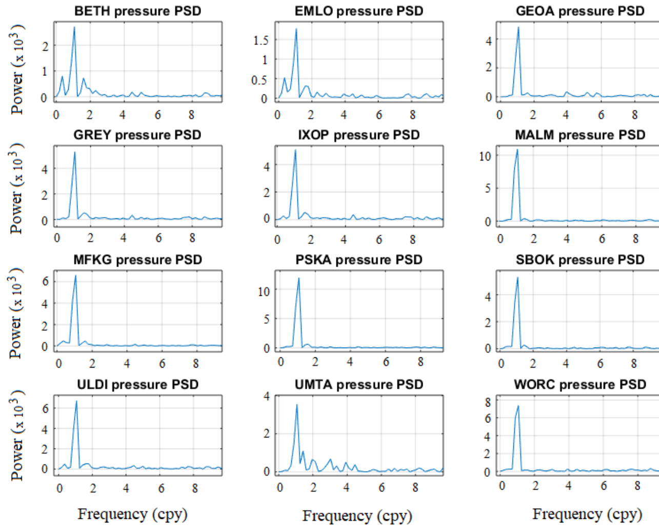
Figure 5.10: Atmospheric pressure time series Fast Fourier Transforms (FFT) Power Spectral Density (PSD) spectra of the time series in Figure 5.6.
