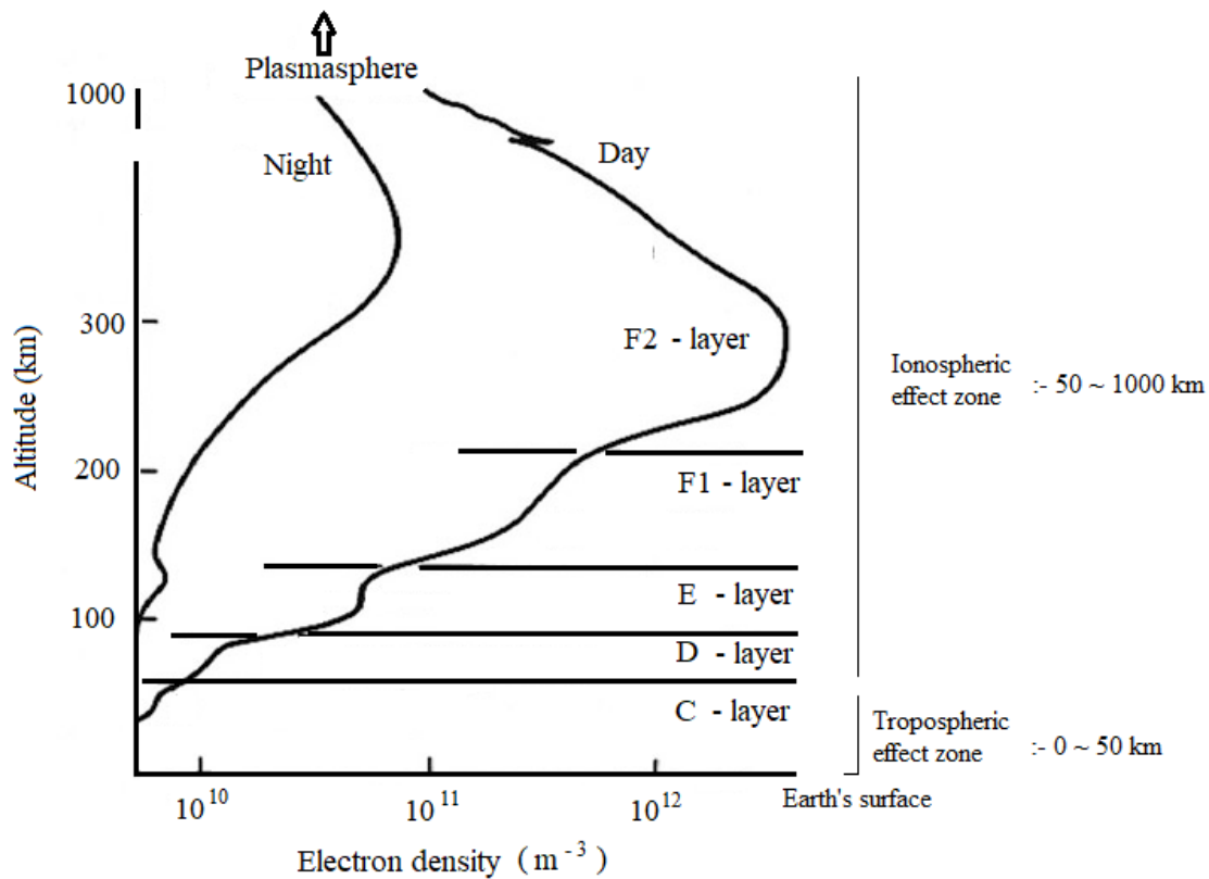
Figure 2.4: Variation of the electron density with altitude from the Earth's surface in summer (modified after Pulinets and Boyarchuk, 2004 ).
