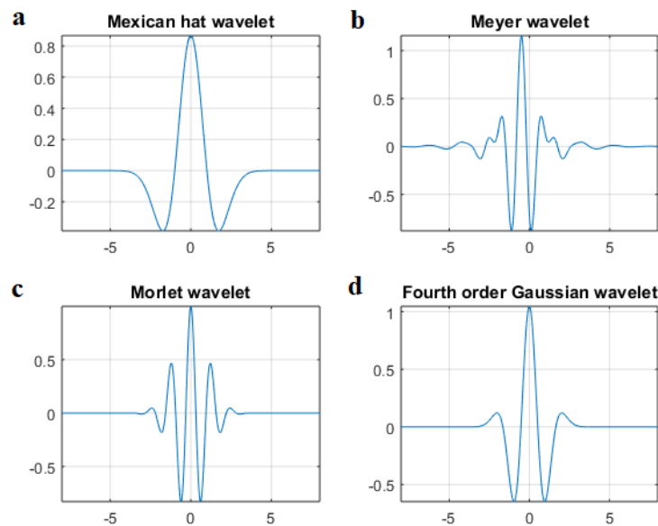
Figure 3.1: (a) Mexican hat wavelet, (b) Meyer wavelet, (c) Morlet wavelet, and (d) Fourth order Gaussian wavelet.
