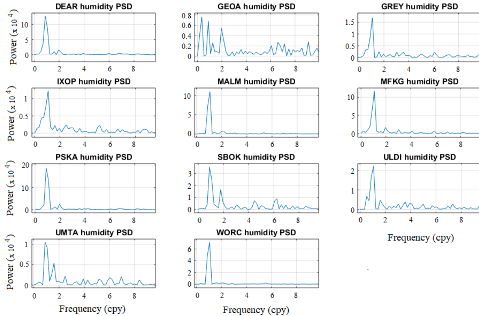
Figure 5.12: Humidity time series Fast Fourier Transforms (FFT) Power Spectral Density (PSD) spectra of the time series in Figure 5.8.
