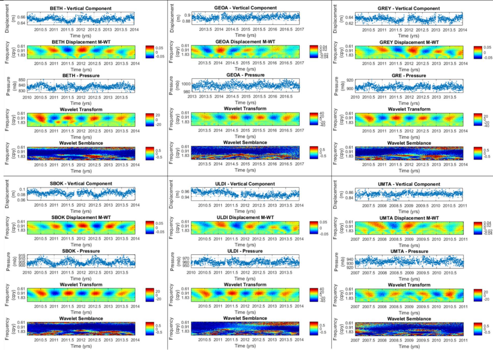
Figure 9.11: Additional semblance correlation plots of cGPS displacement time series (m) vs atmospheric pressure time series (mb).
