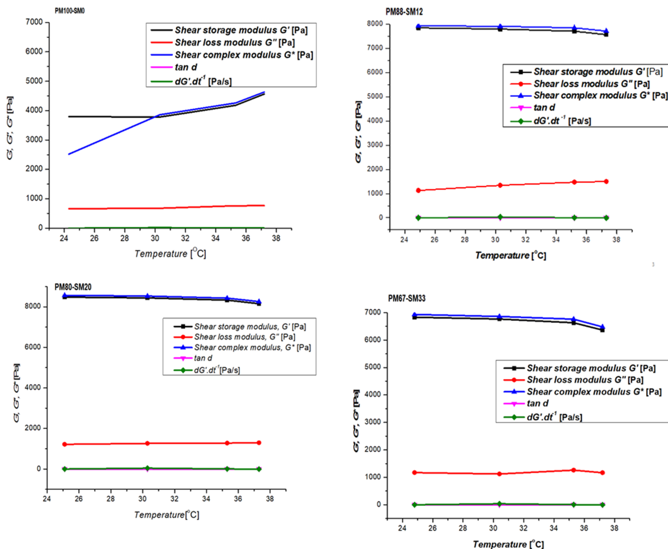
Figure 3. Graphical illustration of the G' , G'' , G^* , and \tan \delta of hydrogels PM100-SM0, PM88-SM12, PM80-SM20, and PM67-SM33.
