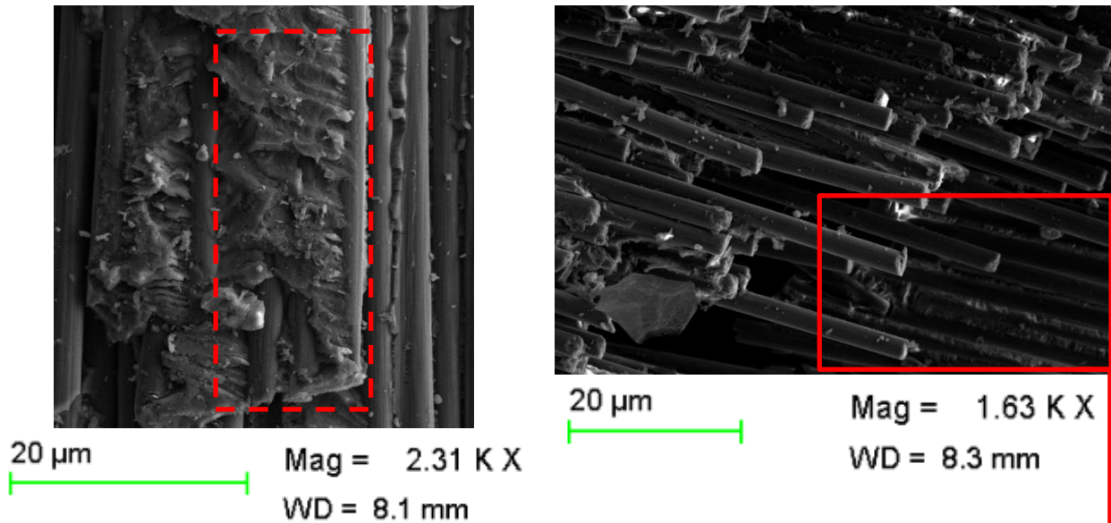
(a) Matrix cusps formed by repeated loading
