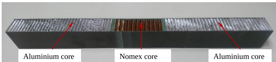
b) Manufactured sandwich specimen
