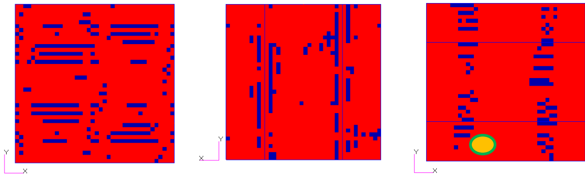
Matrix elements at 8.02 kN Weft tows elements at 8.02 kN Warp tows elements at 8.02 kN
