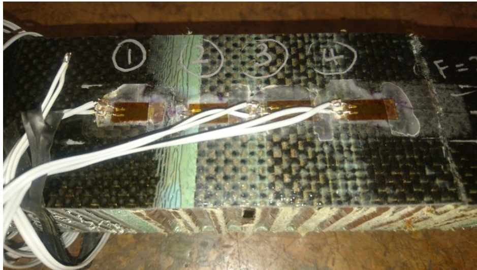
Figure 3.8 Strain gauge positions for E1,E2,E3 and E4 positions over the repair area
