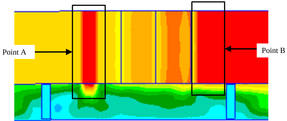
Figure 4.34 Tool facing sheet failure areas for MsM and experimental specimens
