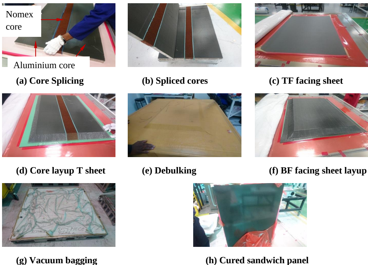
Figure 3.4 Manufacturing process of core layups and bag facing sheet
