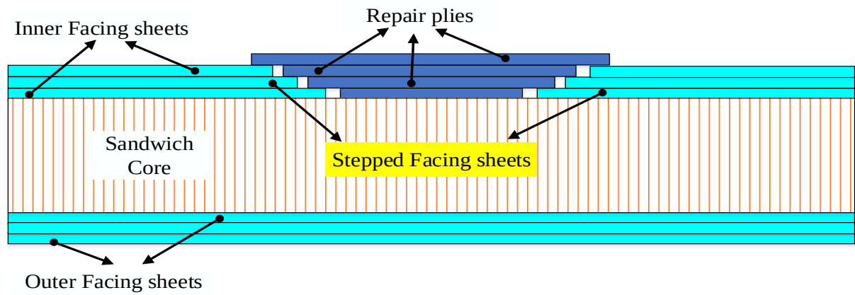
(c) Stepped Repair
