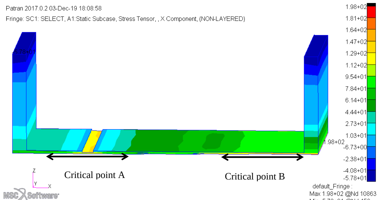
Figure 4.35 Element list positions on a stress plot of the macro model (critical point A)
