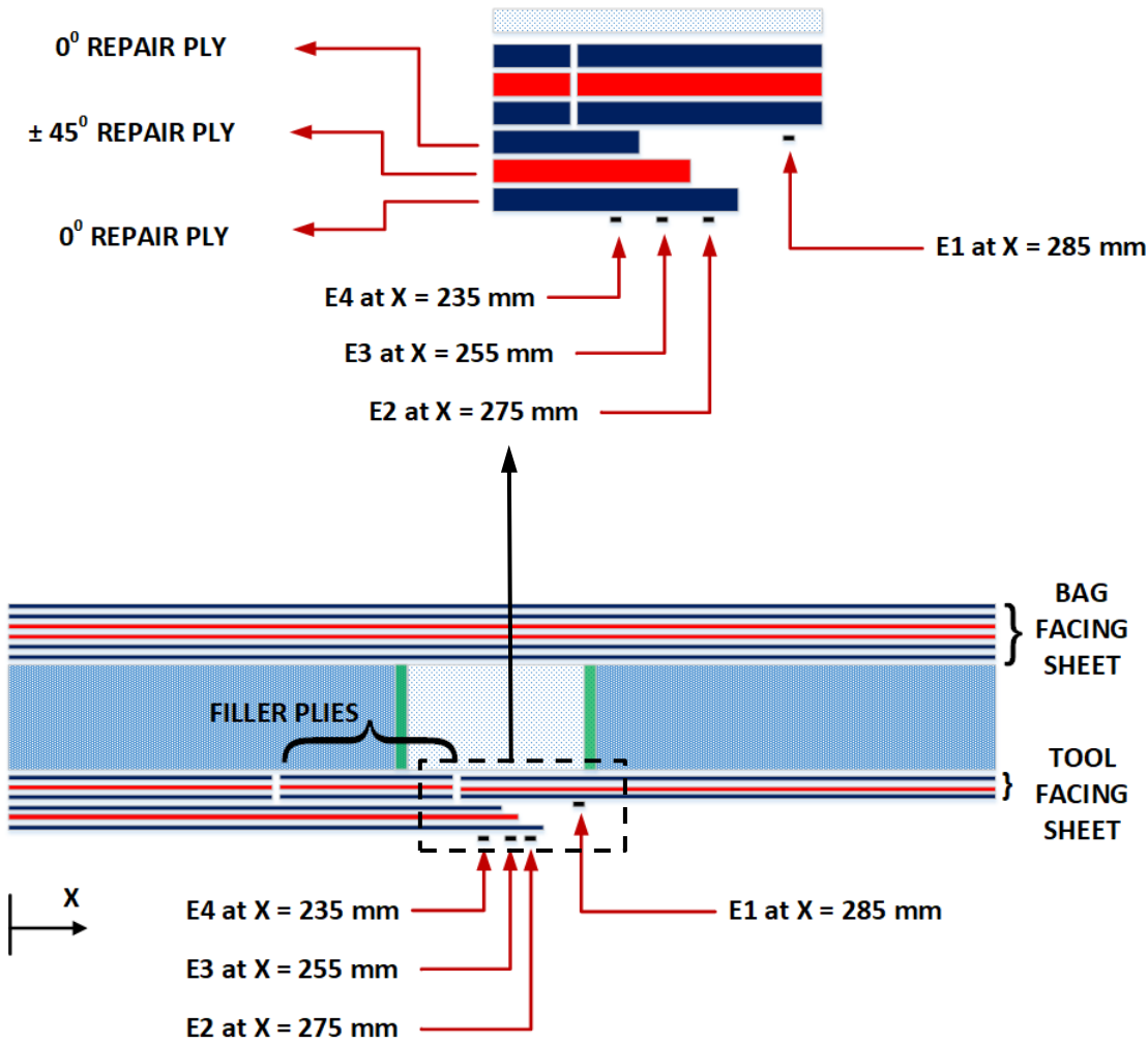
Figure 4.3 Strain gauge positions on the repaired facing sheet
