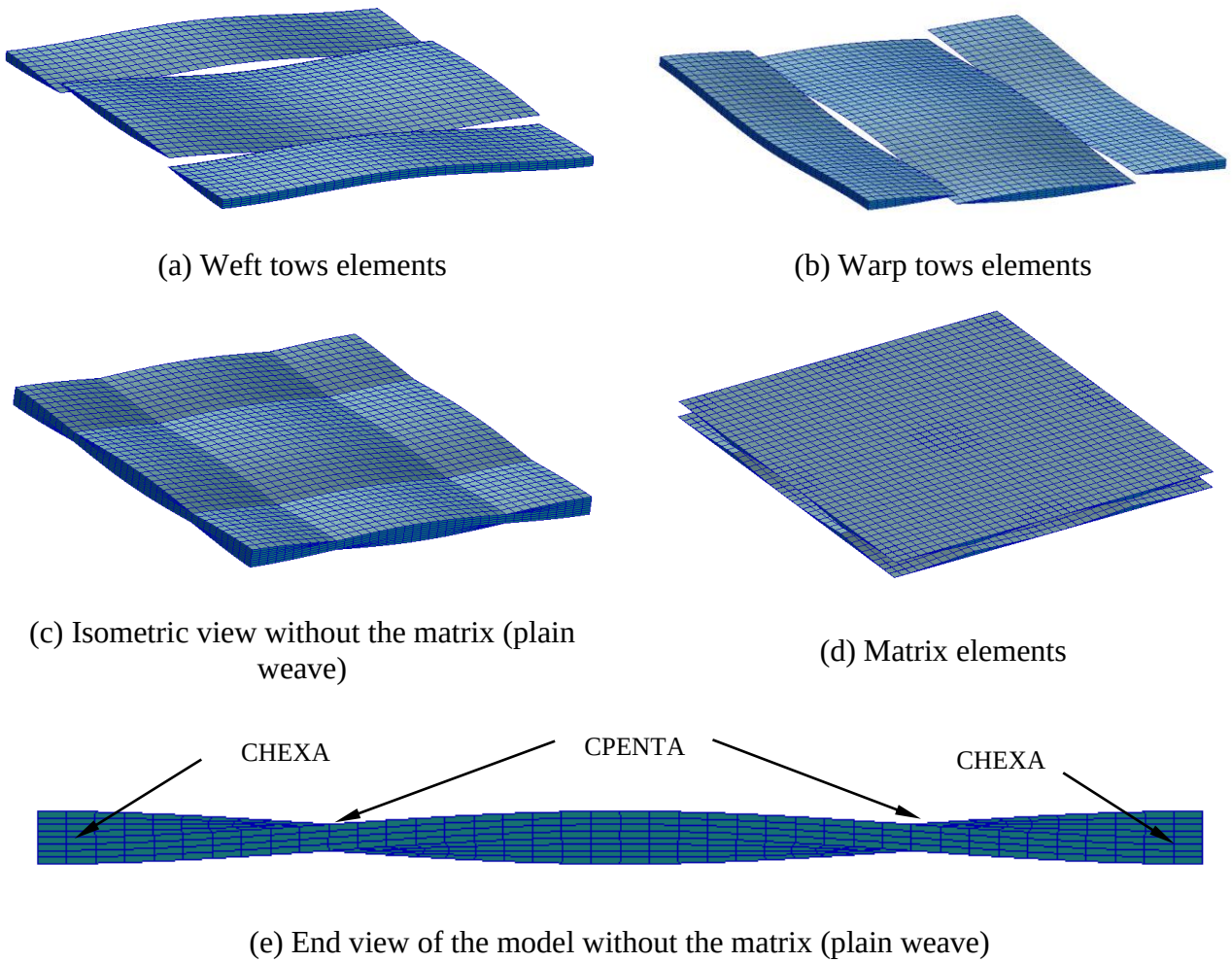
Figure 3.22 Meso model element groups for a plain weave
