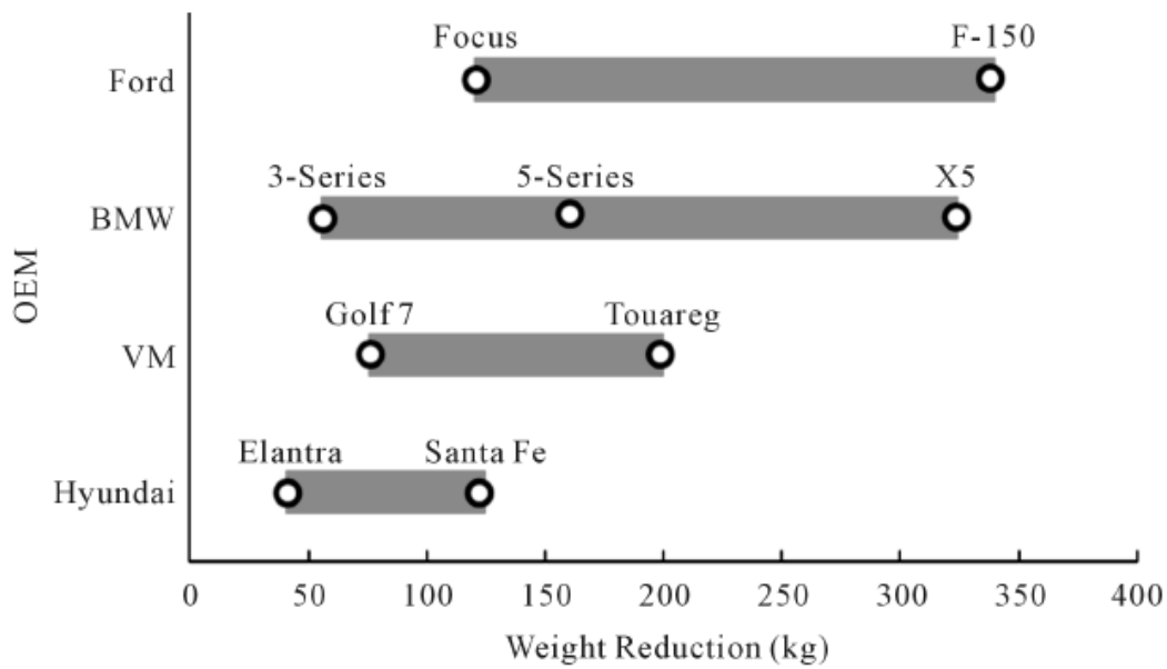
Figure 2.2 Auto light-weighting agenda of major global Original Equipment Manufacturers (OEMs) and their models from 2013 to 2020 [20]
