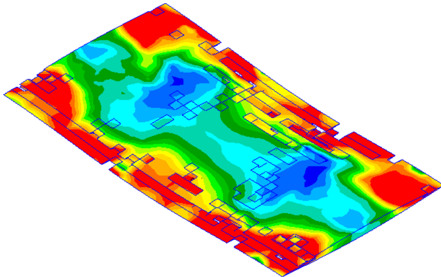
Figure 4.30 Meso scale weft tow failure morphology for MsM and experimental specimens
