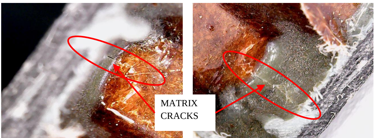
(c) Macro matrix cracking at 8 kN
