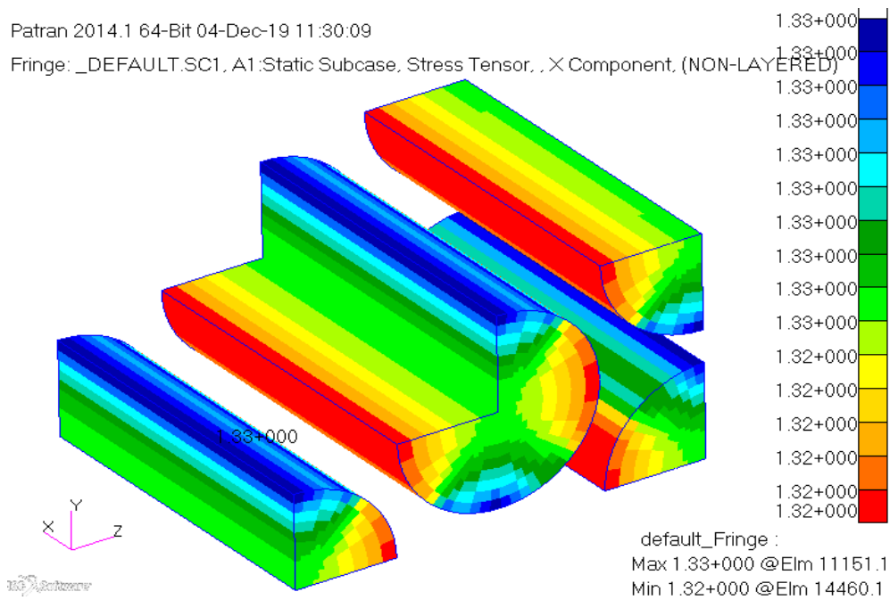
[b] Tensile stress plot of the matrix
