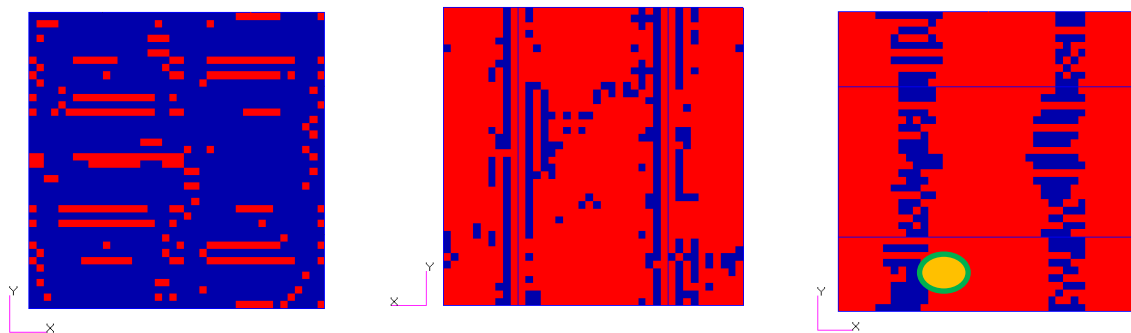
Matrix elements at 8.76 kN Weft tows elements at 8.76 kN Warp tows elements at 8.76 kN
