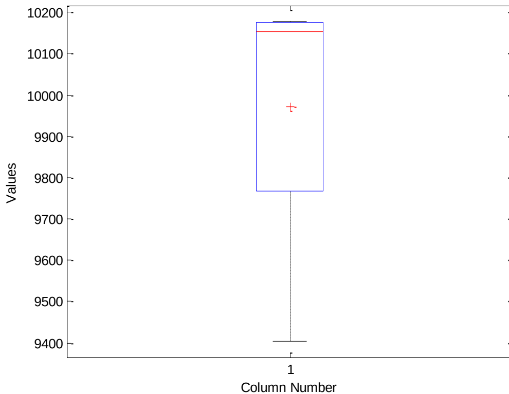
Figure 4.2 Box and whiskers plot of repaired facing sheet failure loads
