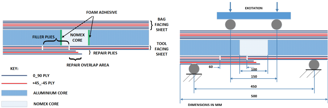
(a) Section view of the sandwich specimen
