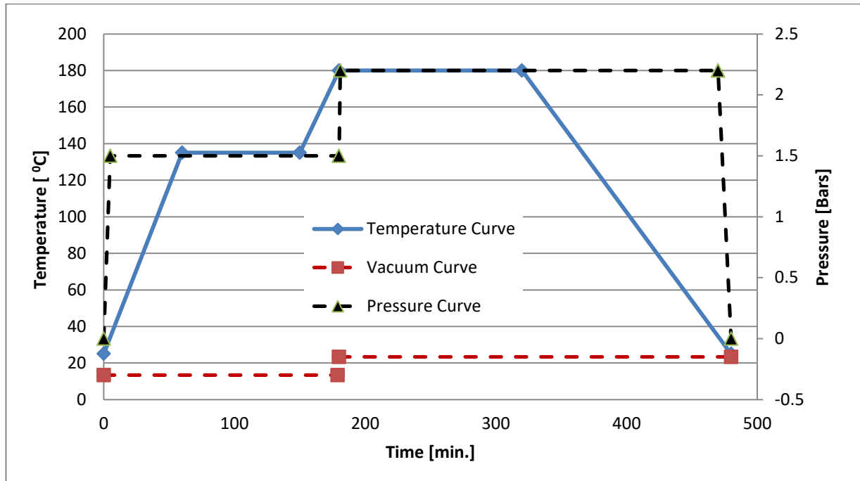
Figure 3.5 Bag Facing sheet cure cycle for the tool side facing sheets
