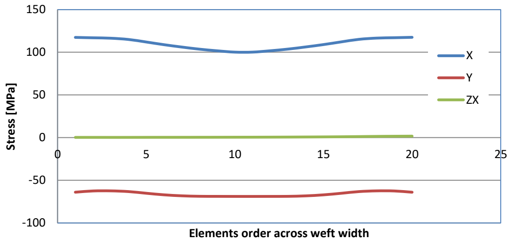
Figure 4.24 Element centroid stress components across the weft width
