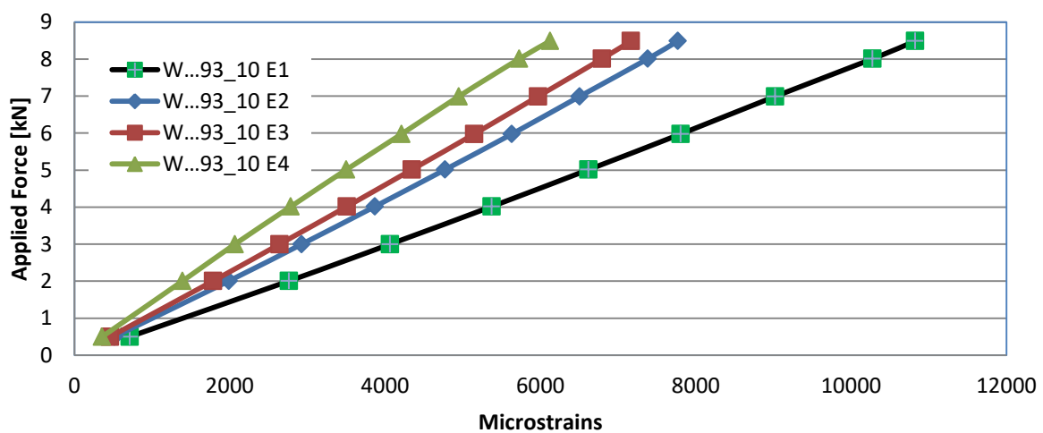
b) Strain measurements from specimens from W94_6
