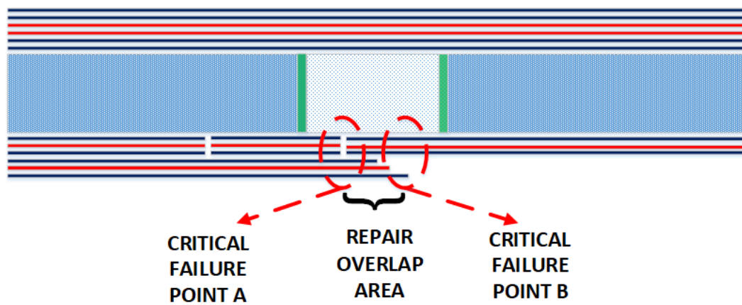
(b) Critical failure points on the repaired tool facing sheet
