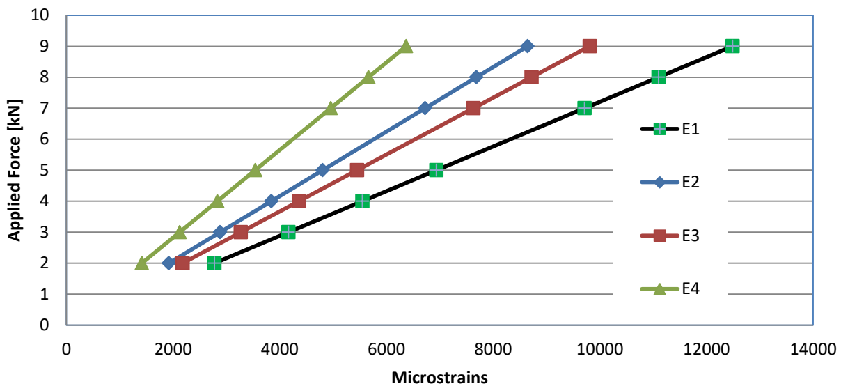
Figure 4.7 Load versus strains from macro model (MsM)
