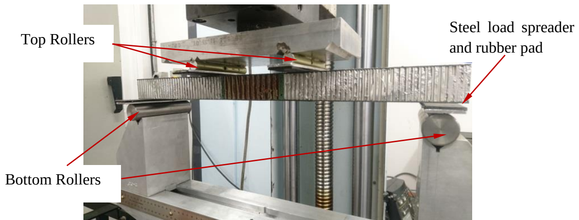
(a) Specimen positioning with pads at loading points for the static test
