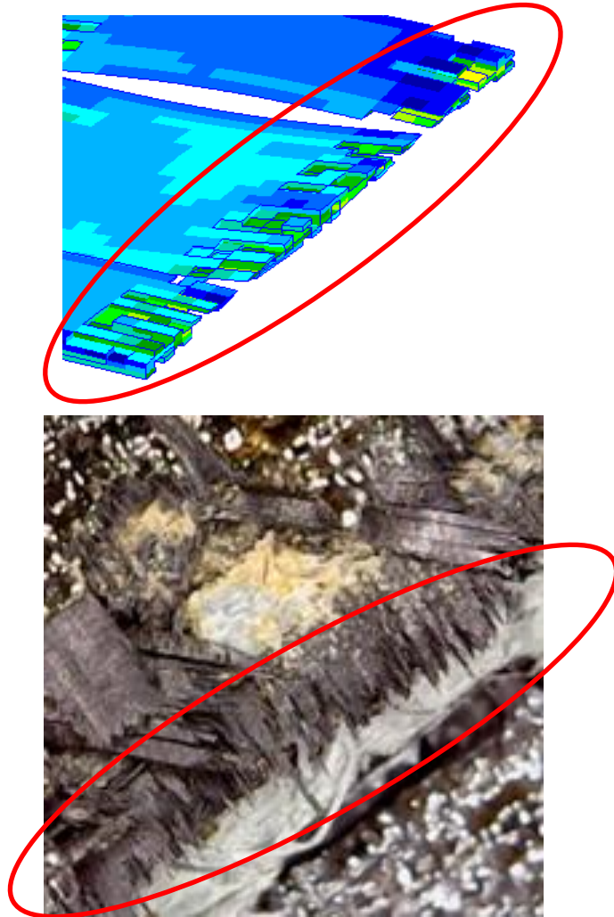
Figure 4.29 Meso scale warp tow failure edge for MsM and experimental specimens
