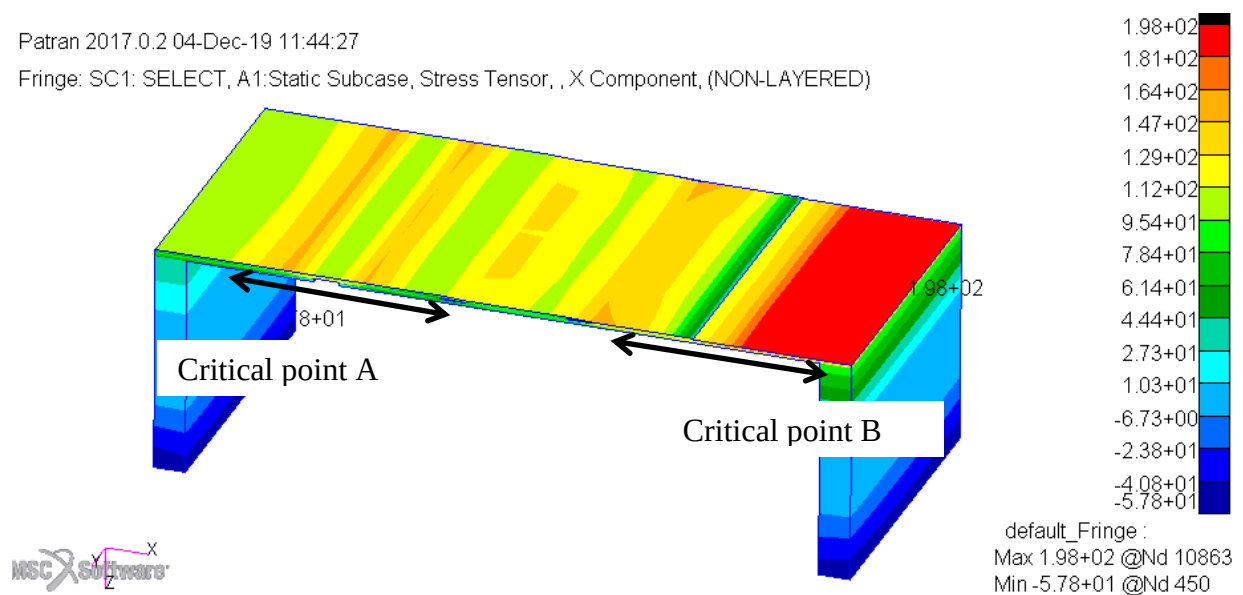
Figure 4.36 Element list positions on a stress plot of the macro model (critical point B)
