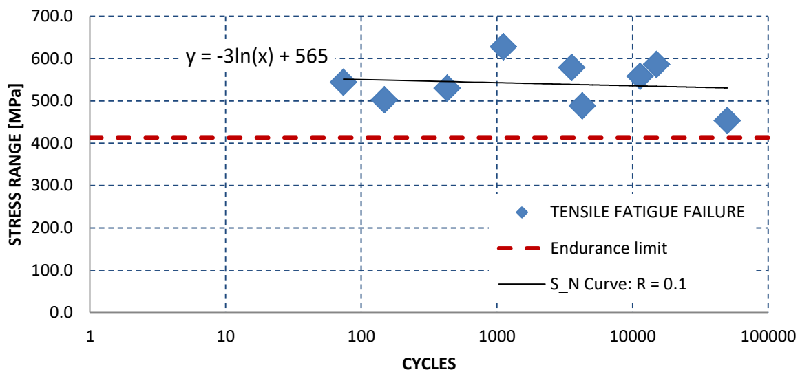
Figure 4.39 Experimental fatigue loading cycles against tool facing sheet stresses: S-N curve
