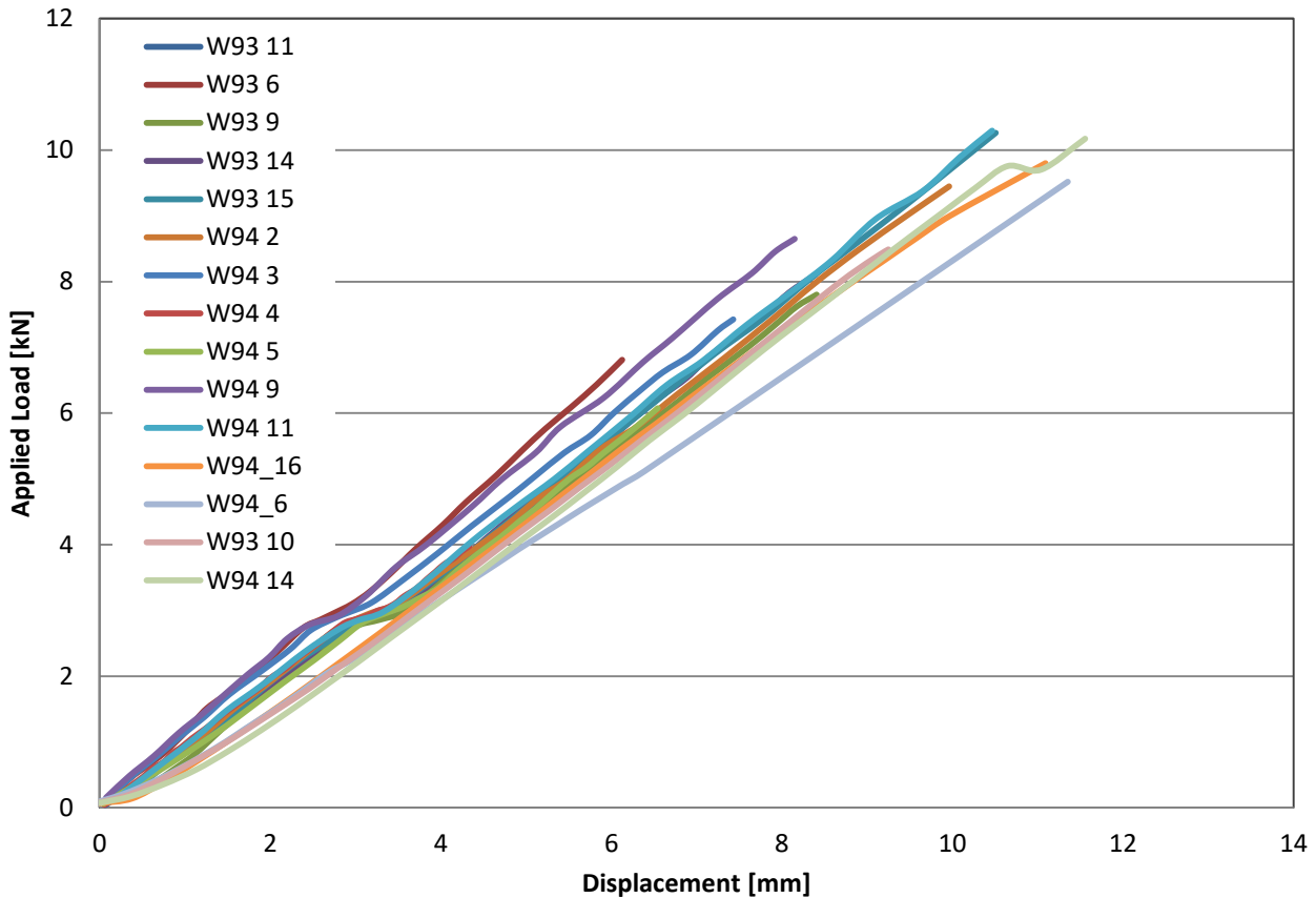
Figure 4.1 Displacement versus applied transverse load
