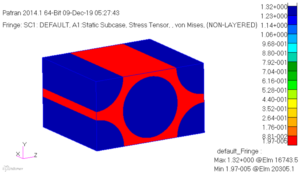
Figure 4.12 Von Mises stress plot of the micro model (GPa)
