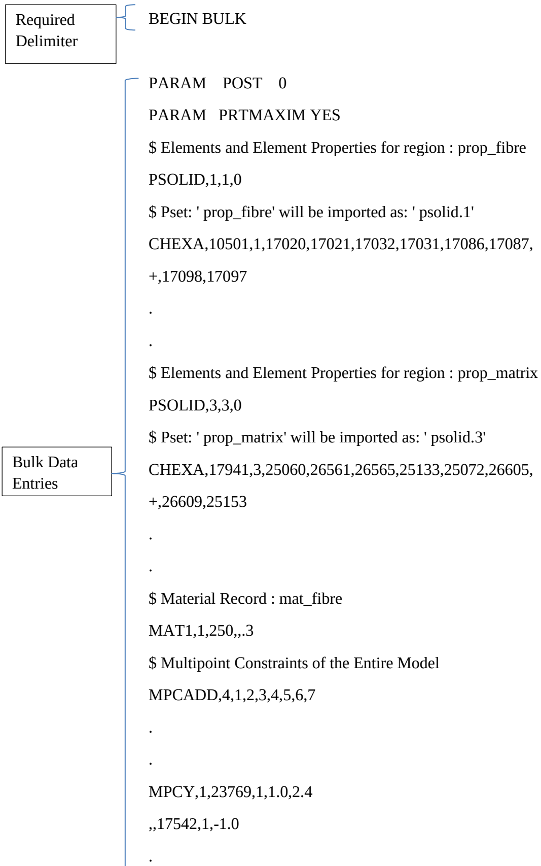
Figure 3.16 Micro model input file sample Bulk Data Entries
