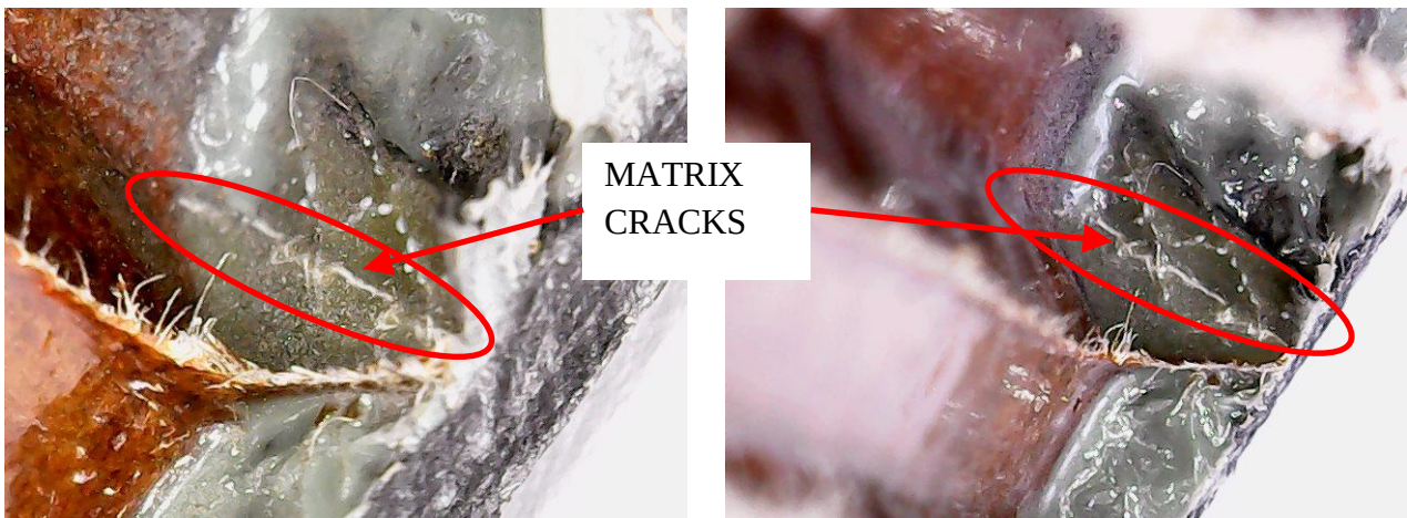
(a) Macro matrix cracking at 6 kN
