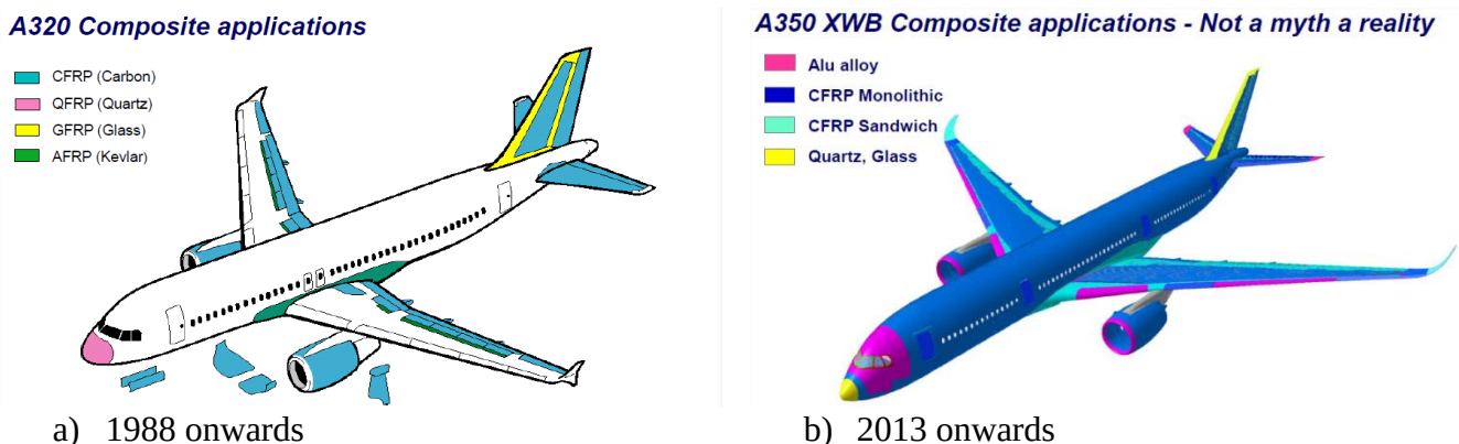
Figure 1.2 Composite application trends for Airbus aircraft [Roland] [2]
