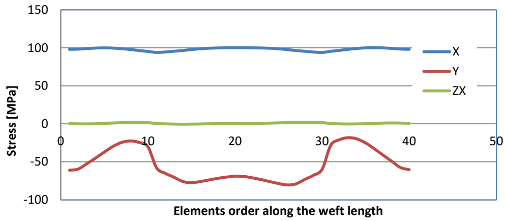
Figure 4.23 Element centroid stress components along weft length
