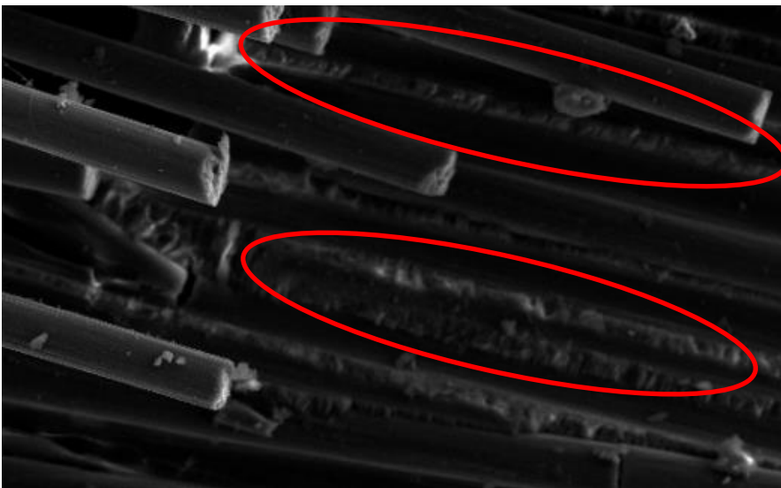
(c) Matrix flaking failure also caused by repeated loading
