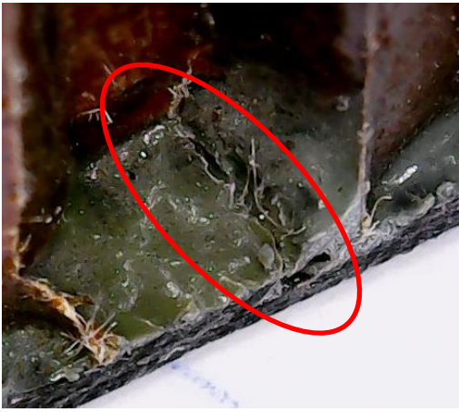
(c) Bond line matrix cracking at CP-A
