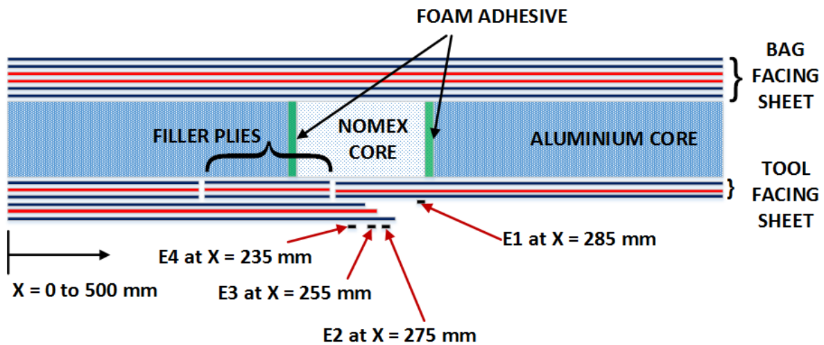
(a) Strain gauge positions on the tapered area of the repaired tool facing sheet
