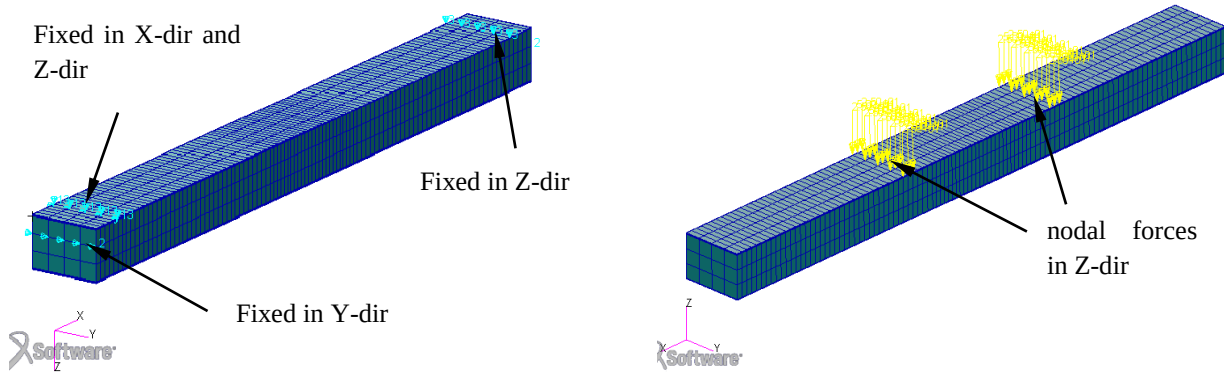
(e) Boundary constraints of the macro model (f) Nodal forces on the macro model
