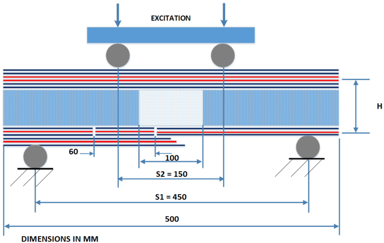
Figure 3.11 Roller positions on the specimen
