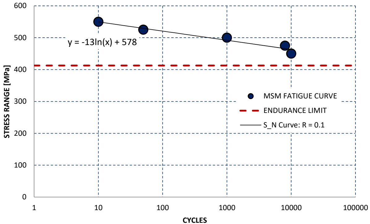
Figure 4.40 MsM fatigue loading cycles against tool facing sheet stresses: S-N curve
