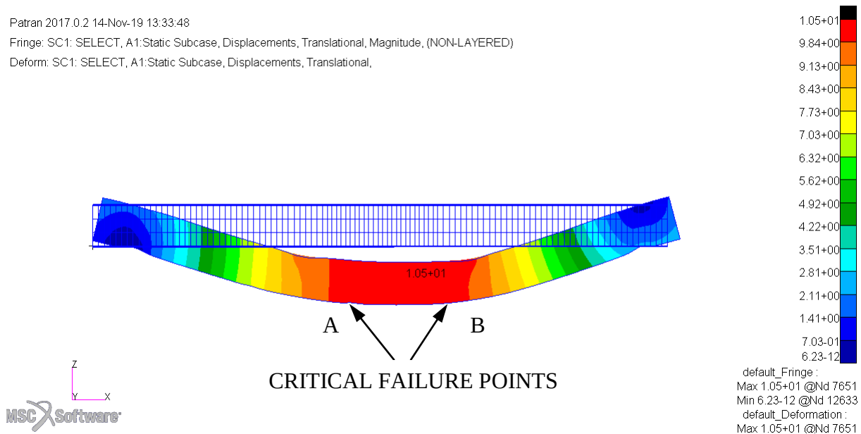
Figure 4.9 Critical points A and B on the repaired facing sheet
