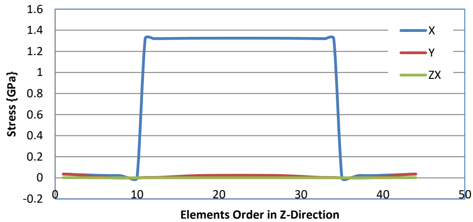
Figure 4.14 Element centroid stress components along Z-dir arrow
