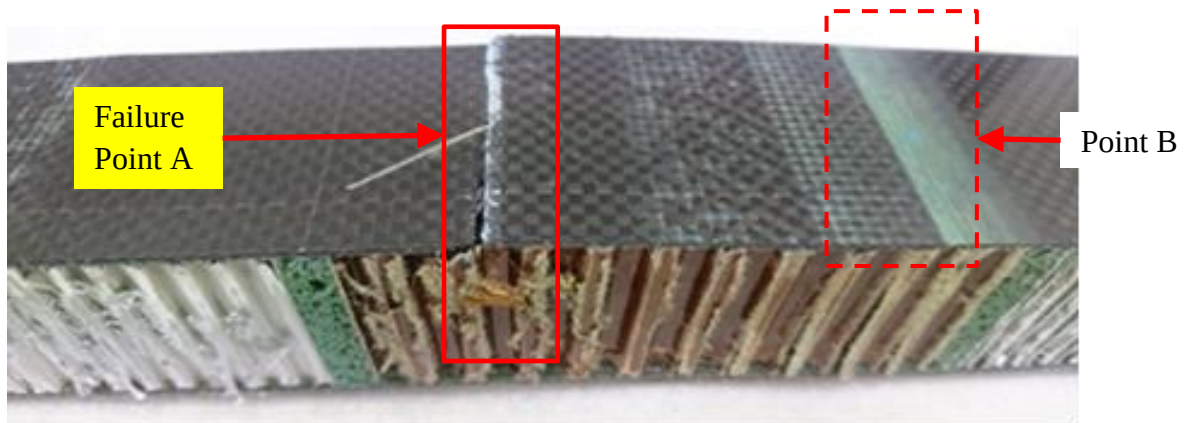
Figure 4.32 Macroscale: Tool facing sheet (repair plies) rupture line ( Critical Point A )
