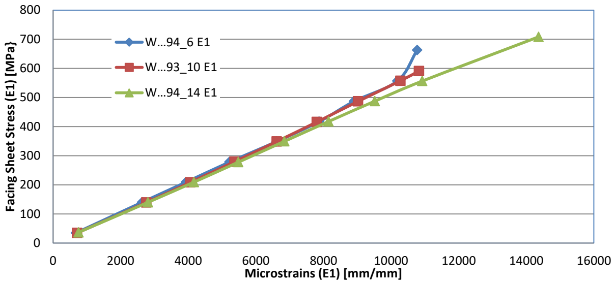
Figure 4.5 Experimental strains versus parent laminate stress at position E1
