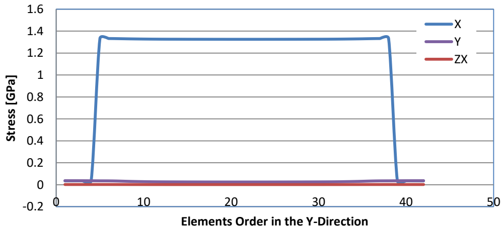
Figure 4.15 Element centroid stress components along Y-dir arrow
