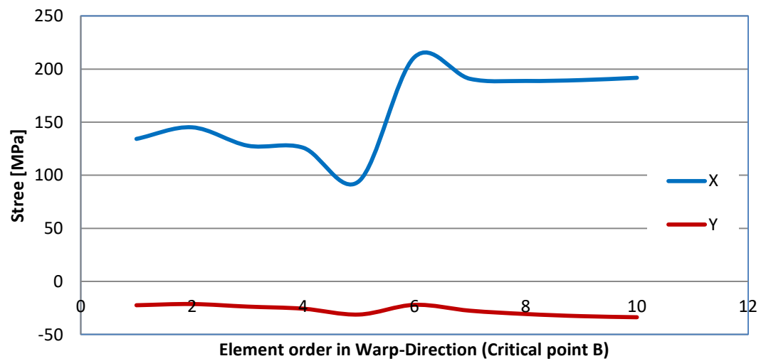
Figure 4.38 Element centroid stress components for critical point B
