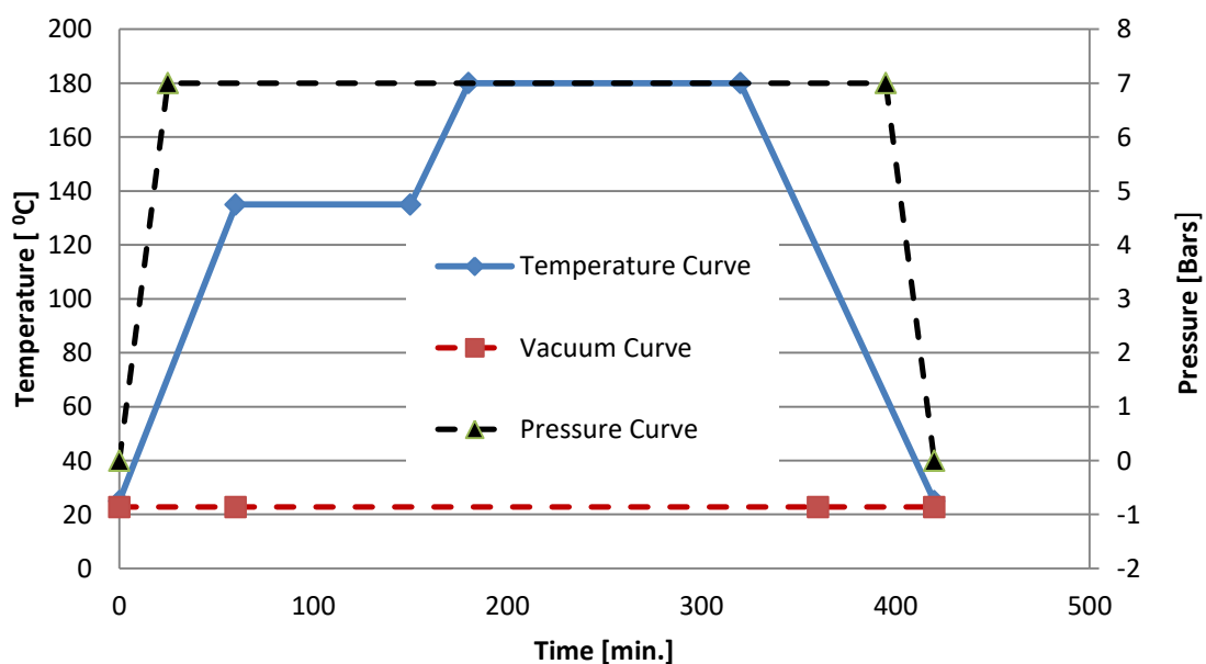
Figure 3.3 Tool Facing sheet cure cycle for the tool side facing sheets
