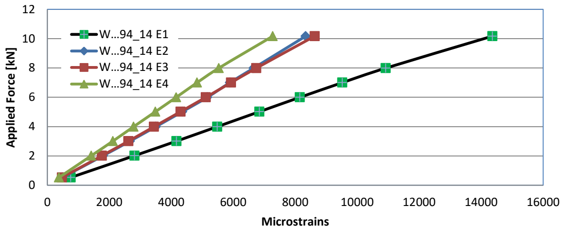
a) Strain measurements from specimens from W94_14
