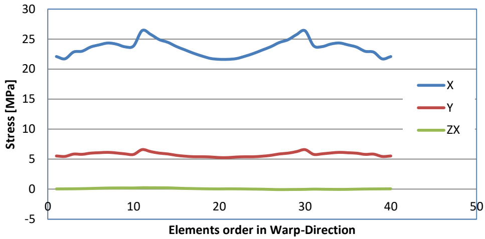
Figure 4.26 Element centroid stress components along warp length
