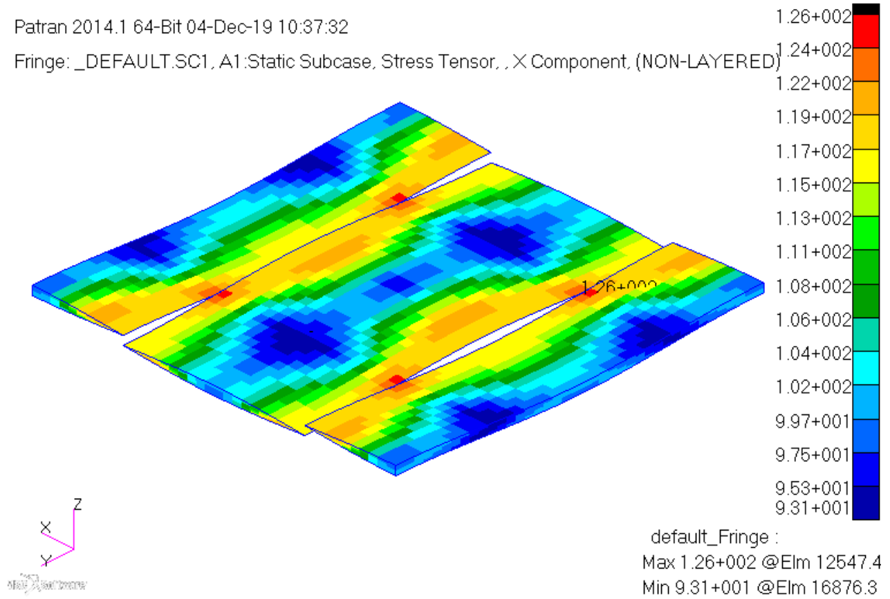
Figure 4.22 Element list positions on a stress plot of the meso model weft tows
