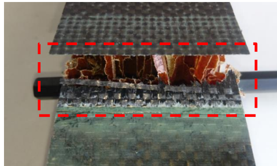
(b) Wide failure strip across the original tool facing sheet at CP B
