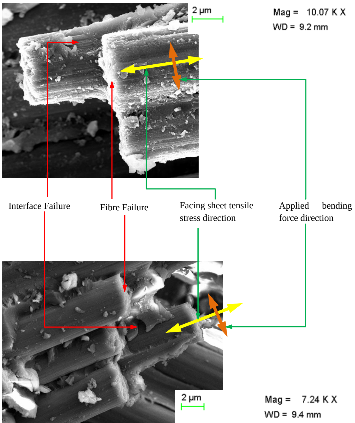
Figure 4.10 SEM pictures of static micro scale failure at critical points A (Warp Tows)
