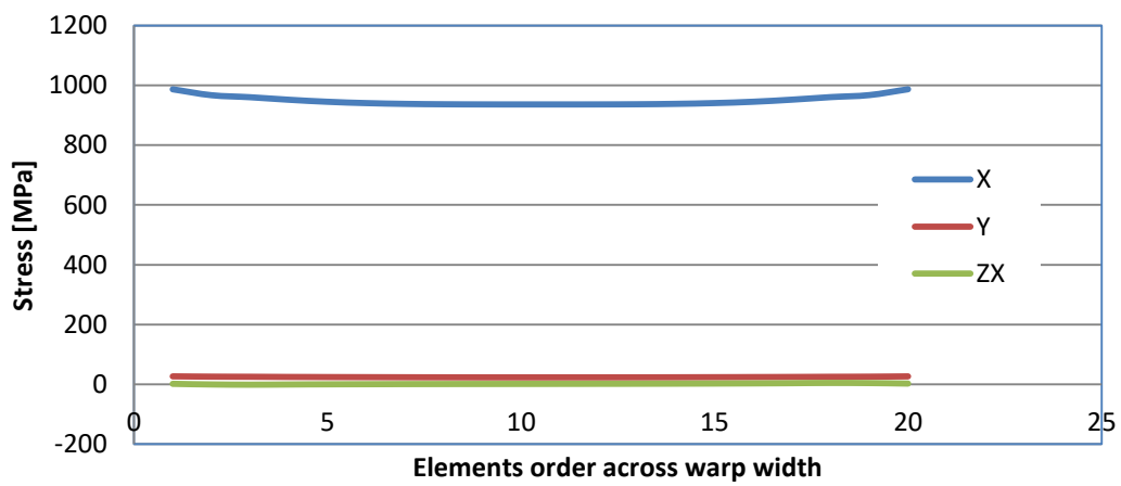
Figure 4.21 Element centroid stress components across the warp width
