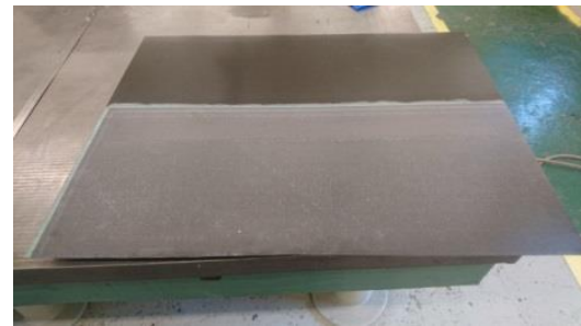
(e) Cured repair
