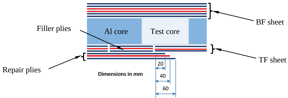
(f) Tool facing sheet filler and repair plies
