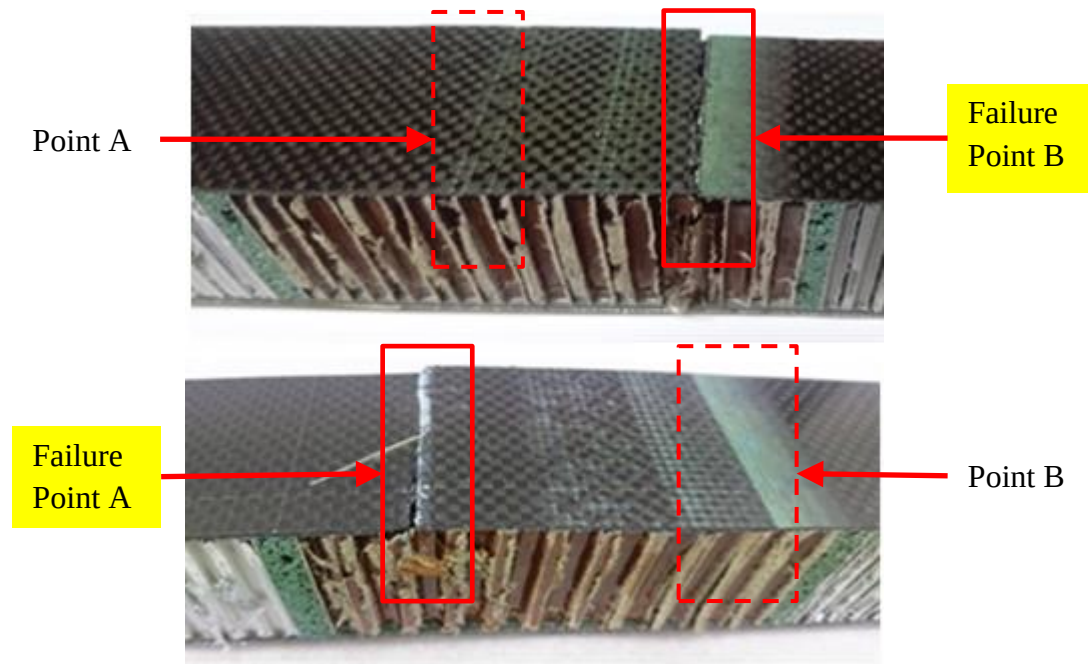
Figure 4.6 Tool facing sheet failure areas for experimental specimens
