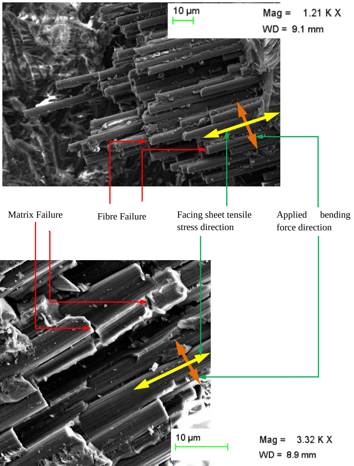
Figure 4.11 SEM pictures of static micro scale failure at critical points B (Warp Tows)
