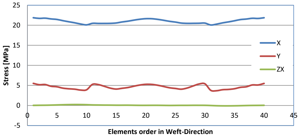
Figure 4.27 Element centroid stress components along weft length
