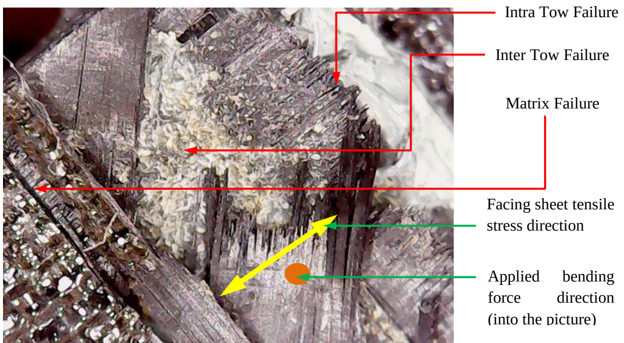
(b) Inter-tow and matrix failure
