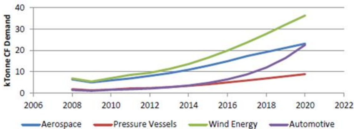
Figure 2.1 Carbon Fibre demand projections by weight for the four major applications analysed [16]
