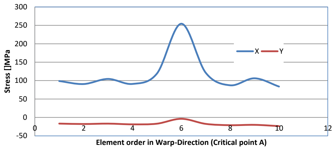
Figure 4.37 Element centroid stress components for critical point A
