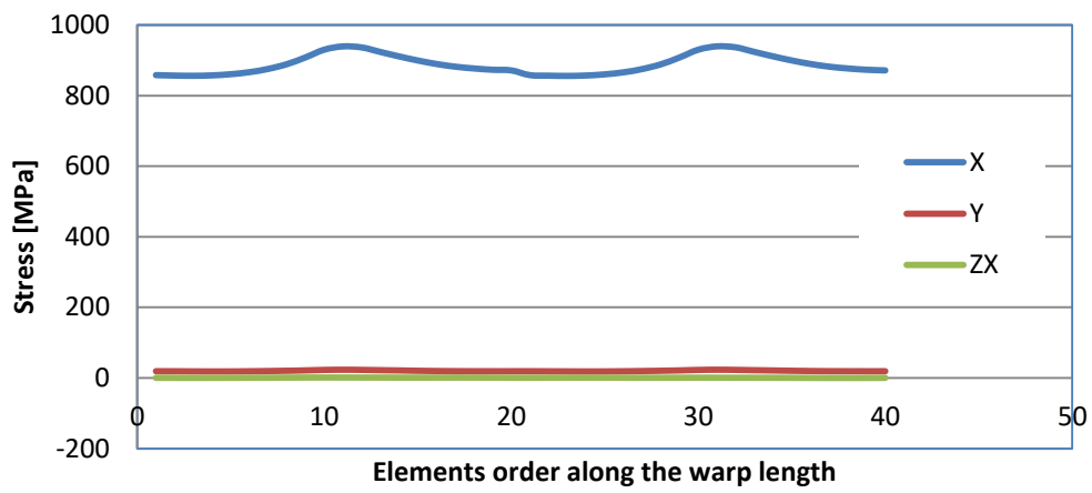
Figure 4.20 Element centroid stress components along the warp length
