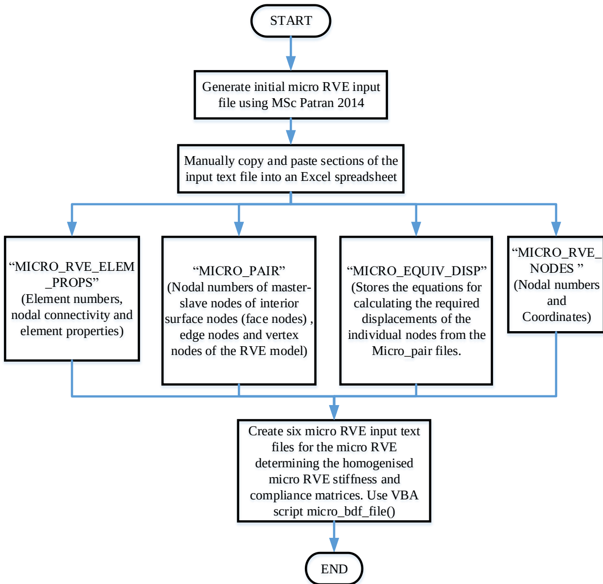
Figure 3.19 Generating the micro RVE input files
