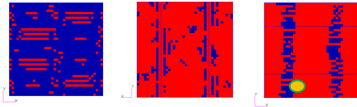
Matrix elements at 8.52 kN Weft tows elements at 8.52 kN Warp tows elements at 8.52 kN
