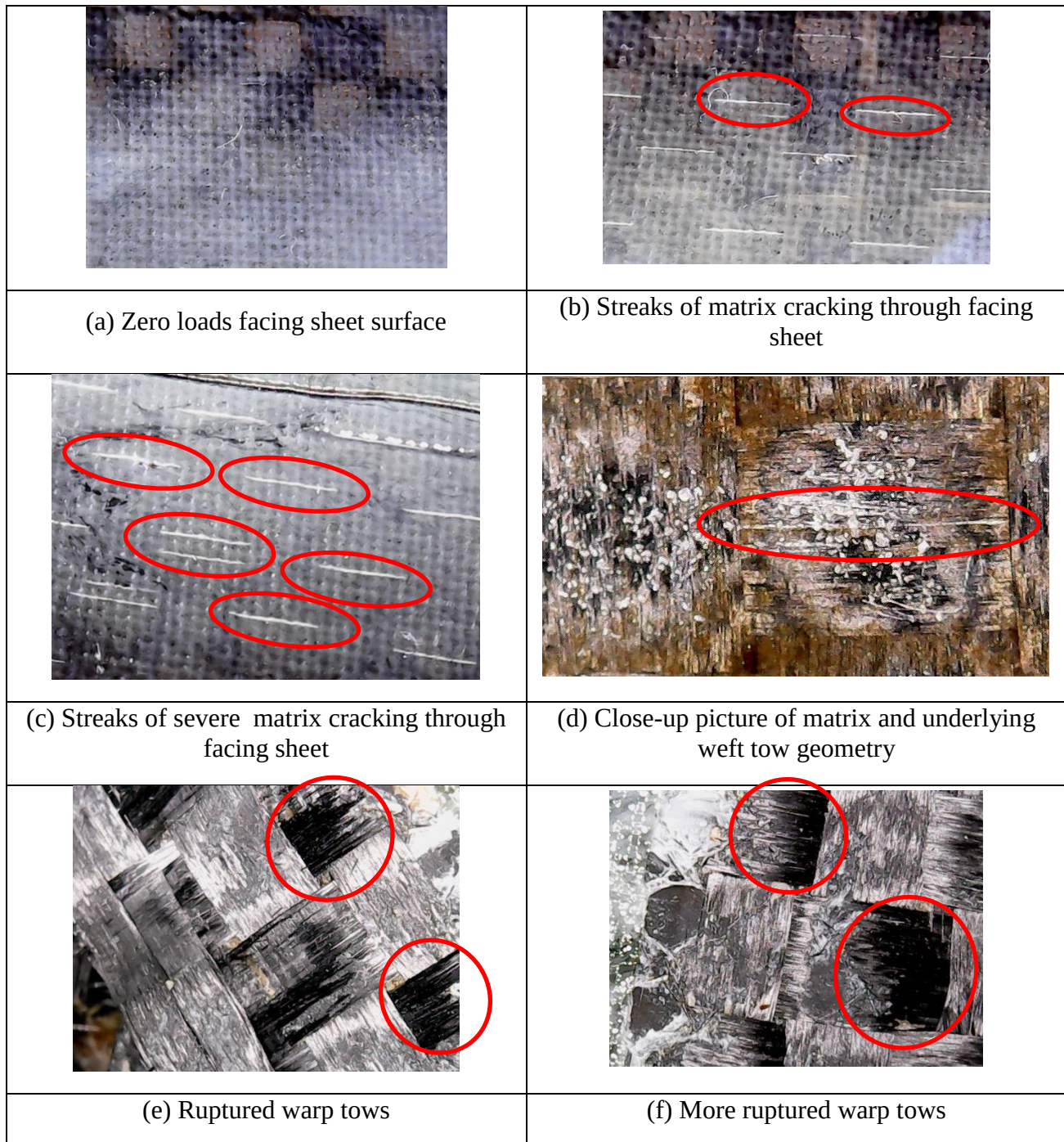
Figure 4.43 Meso scale failure observations at CP B
