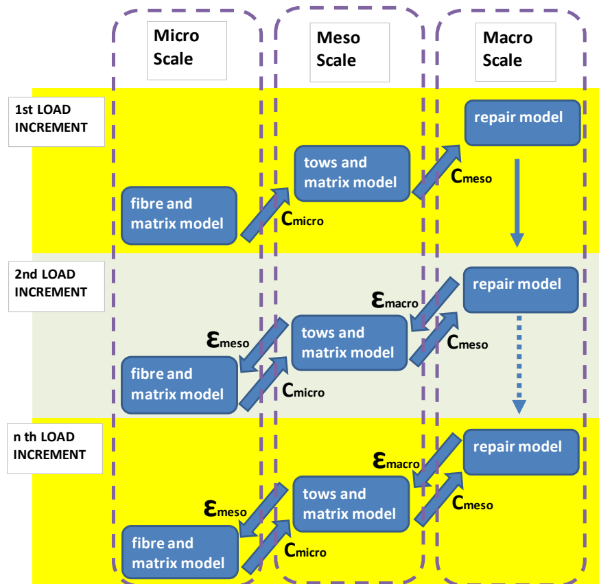
Figure 3.26 General MsM progressive failure analysis flow diagram
