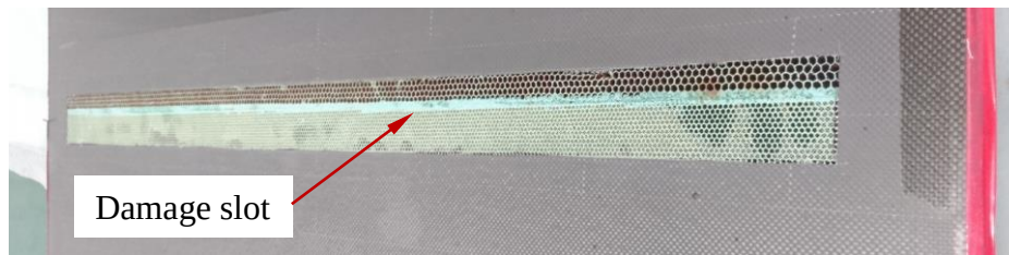
(a) Create damage slot and clean surface
