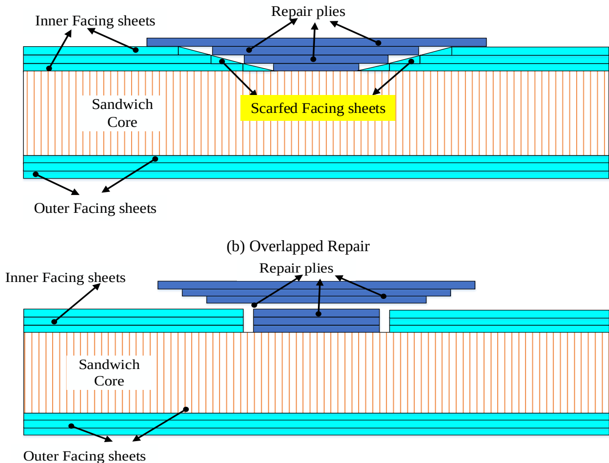
(b) Overlapped Repair
