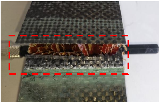
(a) Wide failure strip across the original tool facing sheet at CP B
