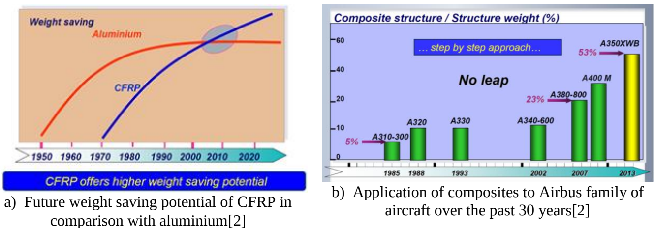
Figure 1.1 Composite weight saving and historical application
