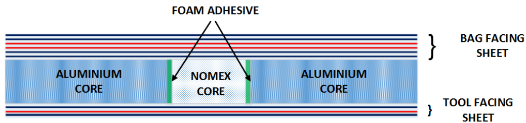
a) Schematic of the sandwich panel
