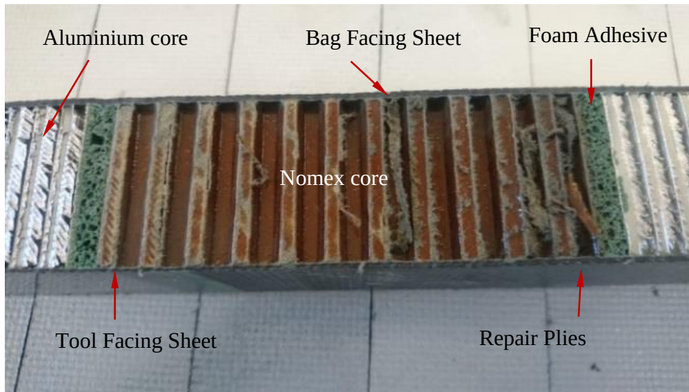
(b) Specimen test section
