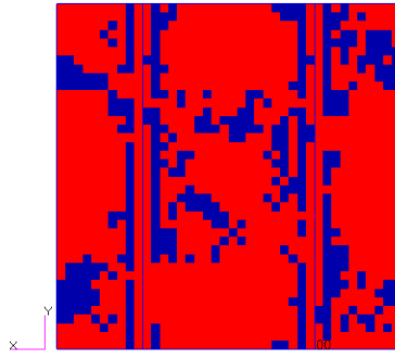
Weft elements at 9000 cycles
