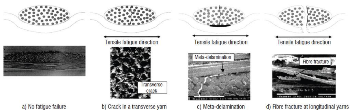
Figure 2.4 Progressive failure characterisation of fibre reinforced composites [39]
