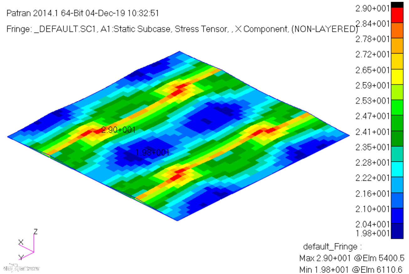
Figure 4.25 Element list positions on a stress plot of the meso model matrix
