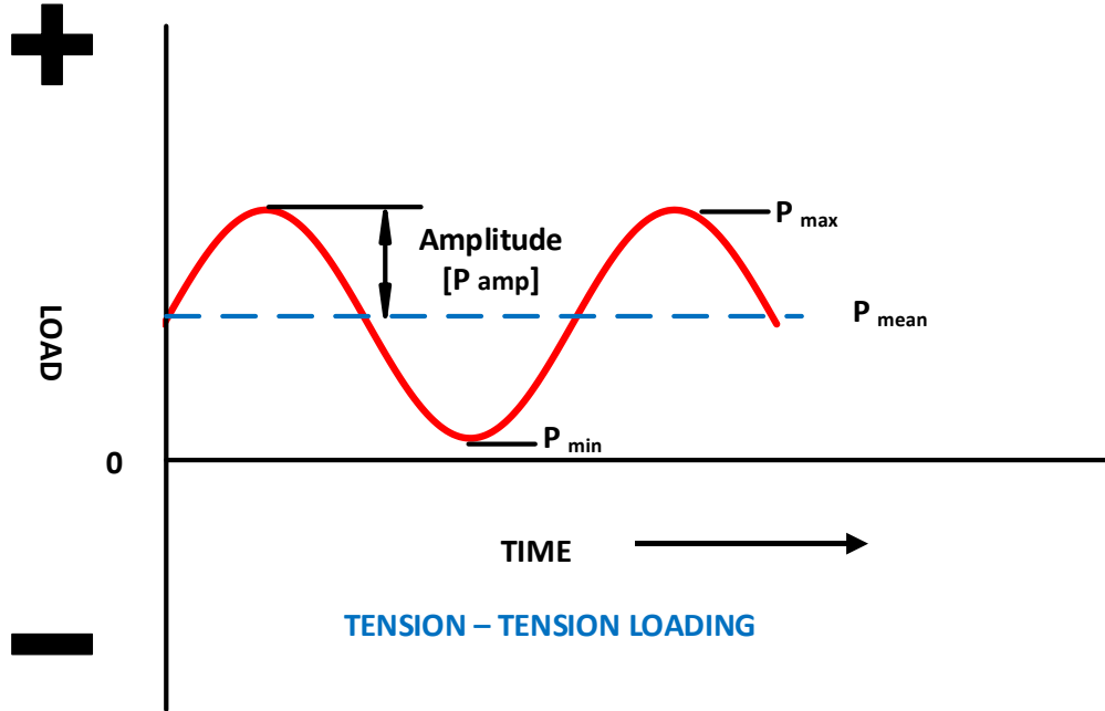
Figure 3.10 Sine wave loading applied to fatigue specimens
