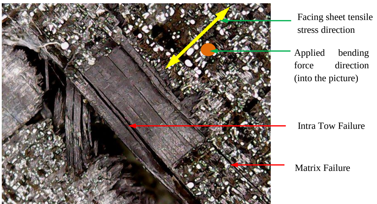
(a) Warp-tow rupturing across its cross-section
