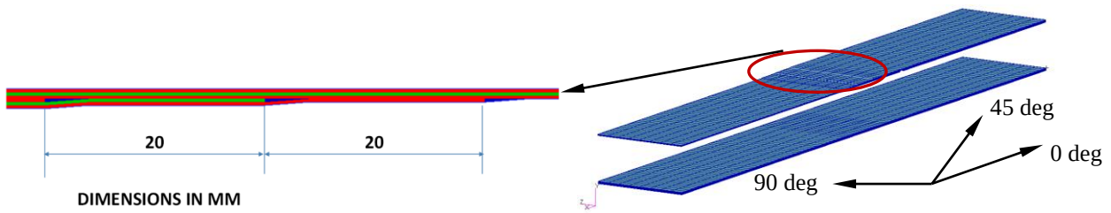
(a) Repair ply drops-offs and overlap distances (b) Facing sheet elements for the macro model
