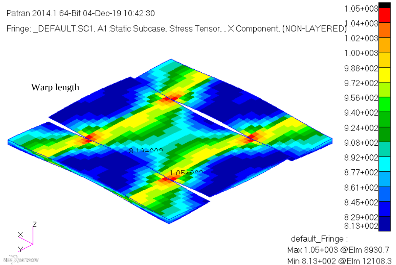
Figure 4.19 Element list positions on a stress plot of the meso model warp tows
