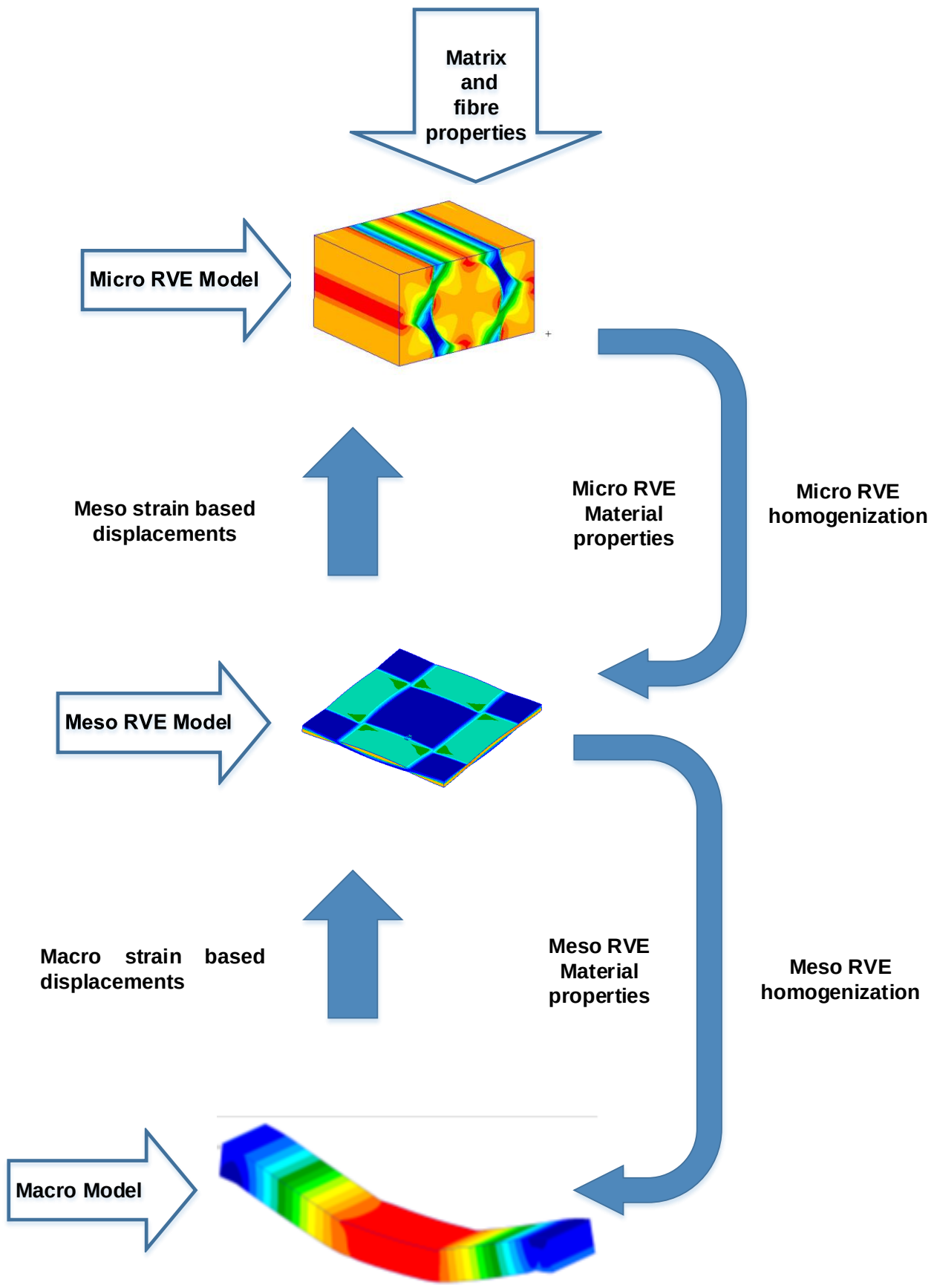
Figure 3.13 Multiscale modelling strategy framework
