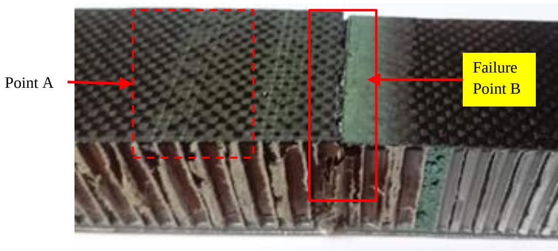
Figure 4.33 Macro scale: Tool facing sheet (parent laminate) rupture line ( Critical Point B )
