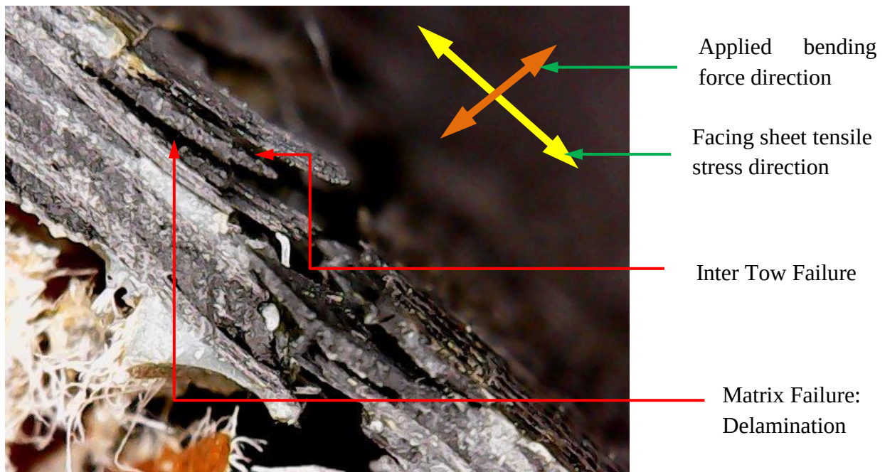
(a) Ruptured laminate delamination and inter-tow failure
