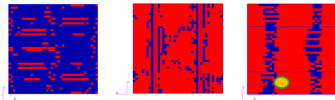
Matrix elements at 9.02 kN Weft tows elements at 9.02 kN Warp tows elements at 9.02 kN
