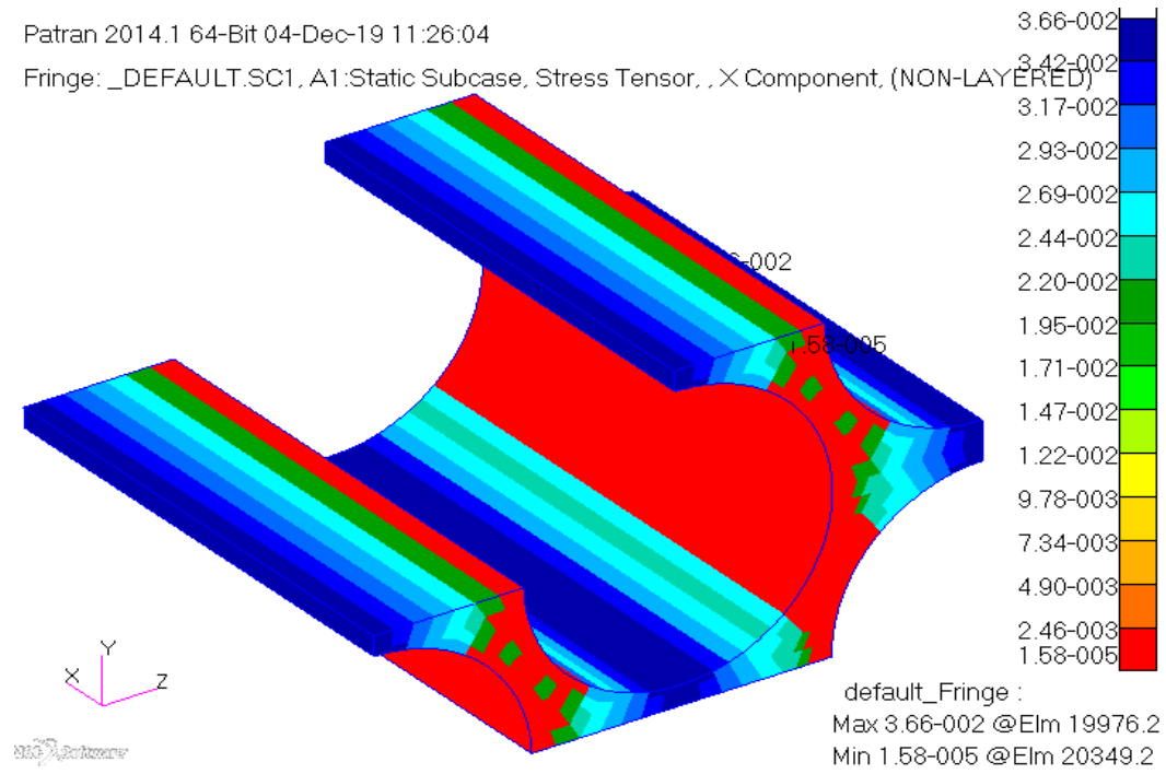
[a] Tensile stress plot of the matrix
