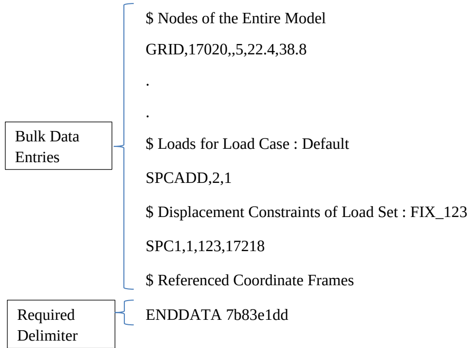
Figure 3.17 Micro model input file sample bulk entries continued
