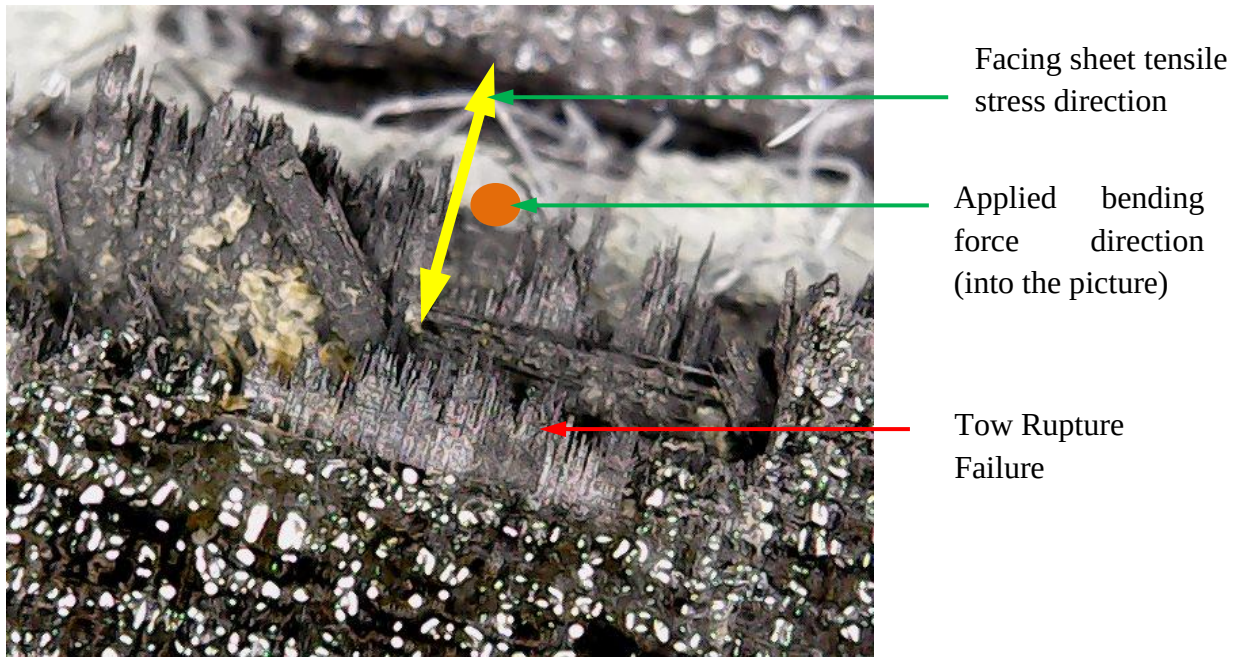
(a) Warp-tow rupturing across its cross-section
