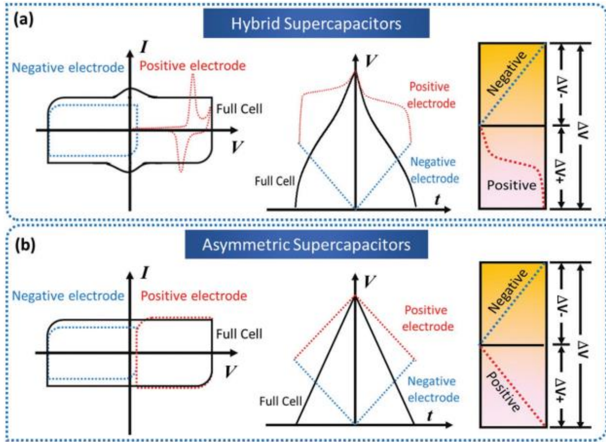
Figure 2.8: Electrochemical signatures of typical (a) hybrid and (b) asymmetric supercapacitors [39].
