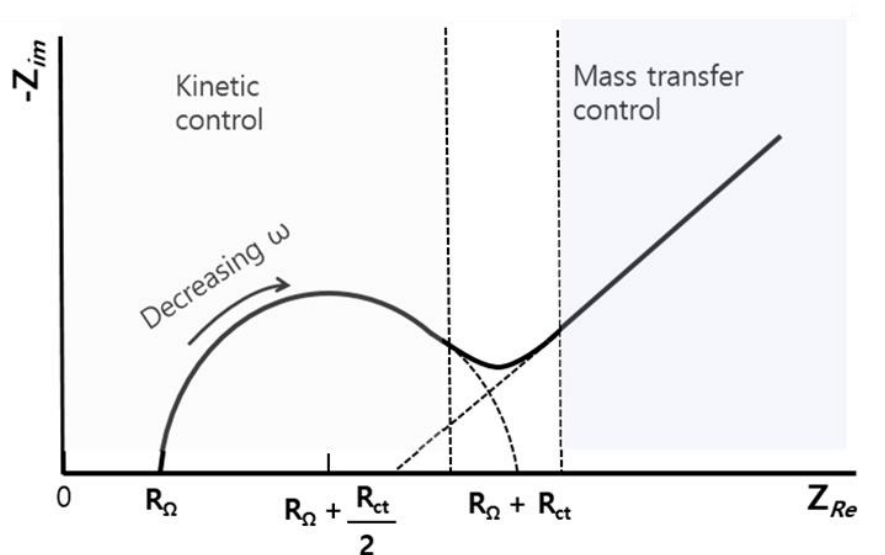
Figure 2.18: Nyquist plot with R_{ct} and R_{\Omega} [168].
