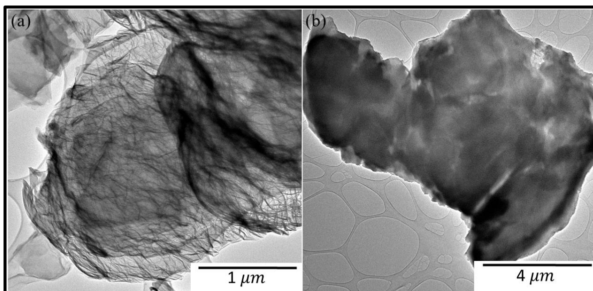
Figure 7.4: TEM images of (a) GO and (b) N-rGO.
