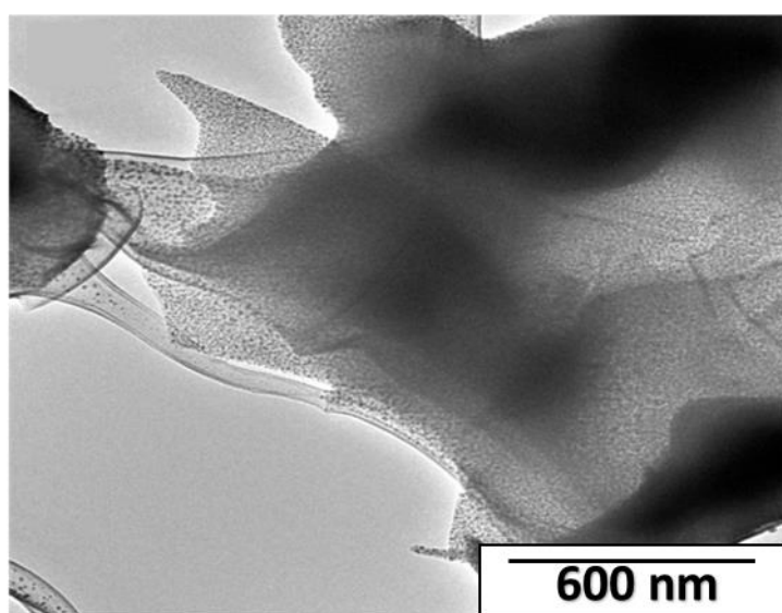
Figure S2: Typical TEM micrograph of as-prepared Ni-MOF in this work shows interconnecting pores distributed over the surface.
