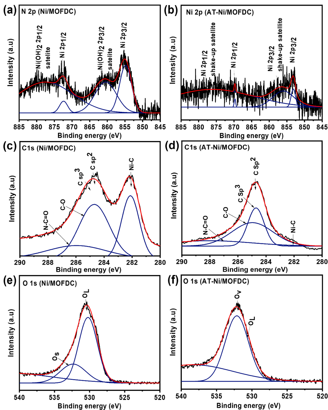
Figure 5.2: Deconvoluted XPS scan of the electrocatalysts (a, b) Ni 2p, (c,d) C 1s and (e, f) O 1s.
