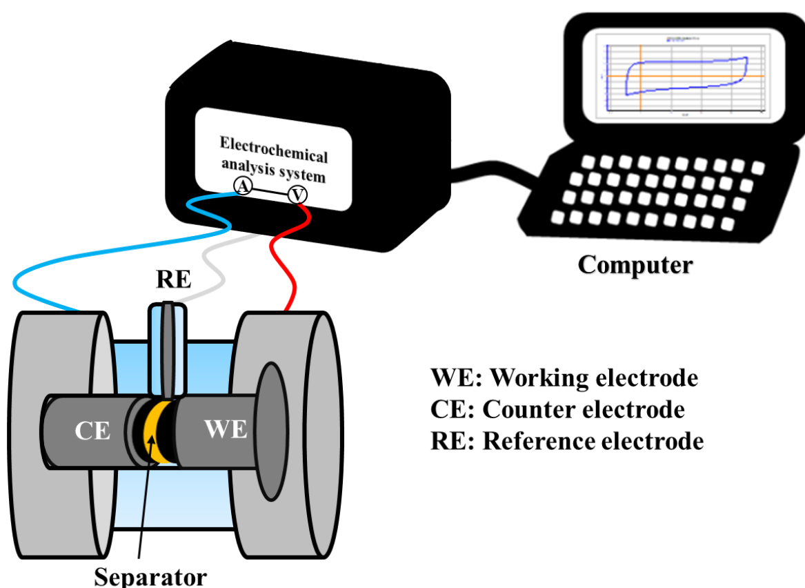
Figure 2.13: A three-electrode configuration using a battery-type Swagelok cell.
