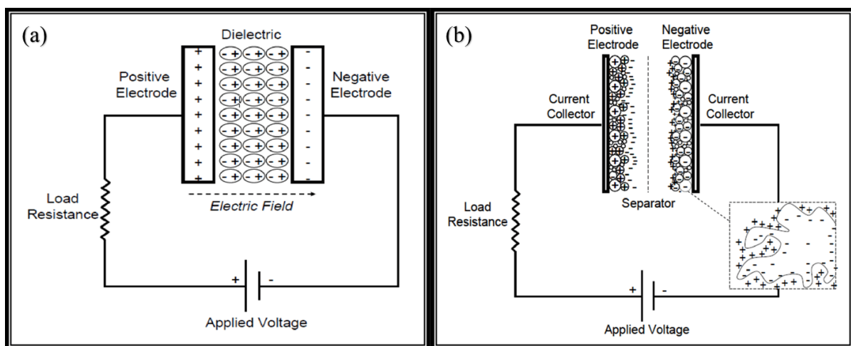
Figure 2.2: Schematic of (a) conventional capacitor and (b) supercapacitor [26].
