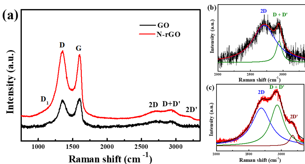
Figure 7.2: (a) Raman spectrum of GO and N-rGO (b) deconvoluted 2D peaks of GO and (c) deconvoluted 2D peaks of N-rGO.
