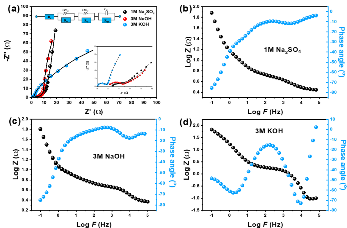
Figure 6.5: Presents (a) Nyquist plots and (b-d) Bode plots of \text{Na}_{0.44}\text{MnO}_2 in 1M \text{Na}_2\text{SO}_4 , 3M NaOH and 3M KOH. The inset of (a) shows the magnified high-frequency region of Nyquist plots and the electrical circuit used in the fitting of the impedance data.
