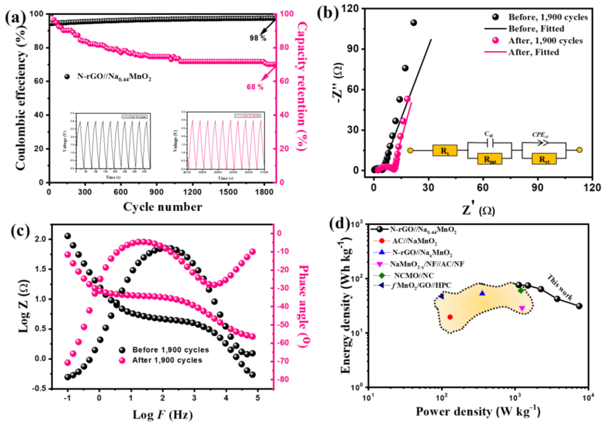
Figure 7.8: (a) Coulombic efficiency and capacity retention for 1,900 GCD cycles carried out at a current density of 5 \text{ A g}^{-1} , (b) EIS measurement before and after 1,900 cycles, (c) Bode plots before and after 1,900 cycles of the N-rGO//Na 0.44 MnO 2 device and (d) Ragone plot of the supercapacitor (energy density vs. power density).
