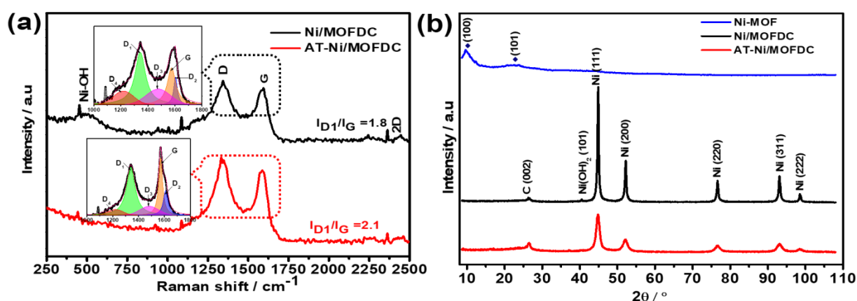
Figure 5.1: (a) Raman spectra of Ni/MOFDC and AT-Ni/MOFDC (the insert show typical deconvoluted Raman signal of carbon) and (b) XRD of the Ni-MOF, Ni/MOFDC and AT-Ni/MOFDC.
