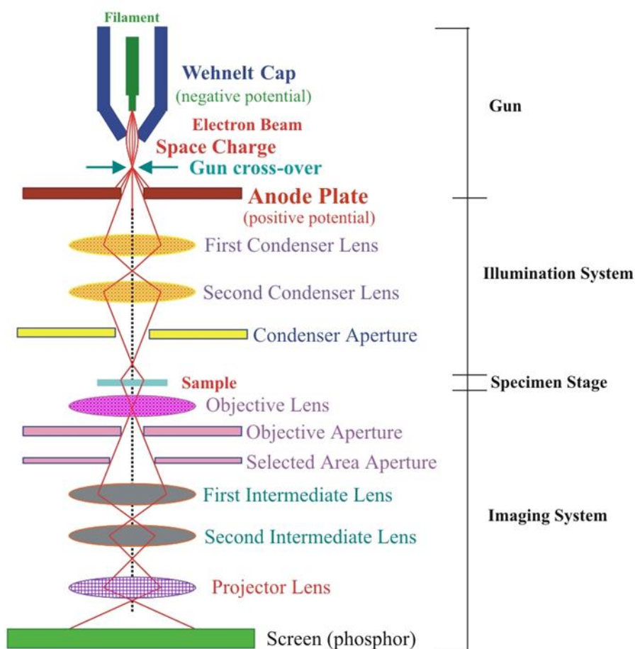
Figure 3.2: Schematic diagram of a typical TEM [6].
