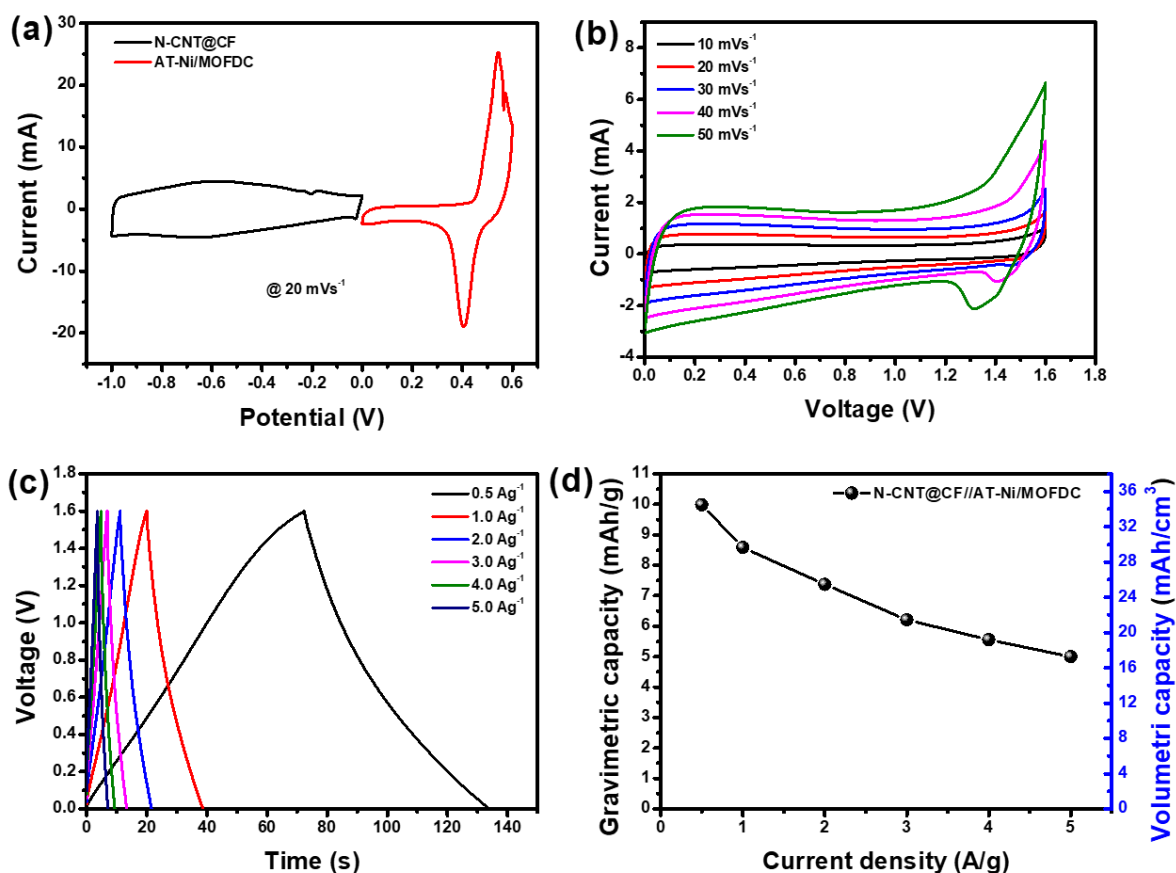
Figure 5.6: (a) CV curves of N-CNT@CF and AT-Ni/MOFDC, (b) CV curves of N-CNT@CF//AT-Ni/MOFDC at different scan rates, (c) typical GCD curves of N-CNT@CF//AT-Ni/MOFDC at different current densities and (d) capacity versus current density plot.
