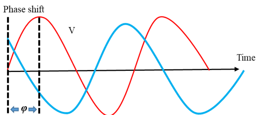
Figure 2.17: Phase shift \phi in the current I as a response to a sinusoidal perturbation-potential V in a pseudo-linear system (Adapted from Ref [167]).
