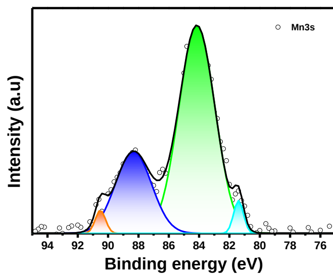
Figure S2: X-ray photoelectron spectroscopy (XPS) analysis, narrow scan of Mn3s.
