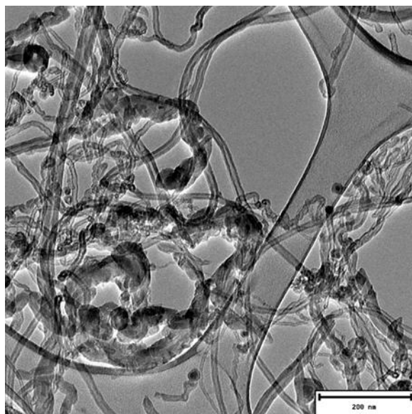
Figure S1: TEM image of reference CNTs.
