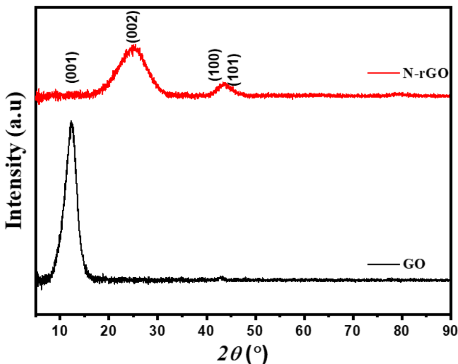
Figure 7.1: XRD spectrum of GO and N-rGO.
