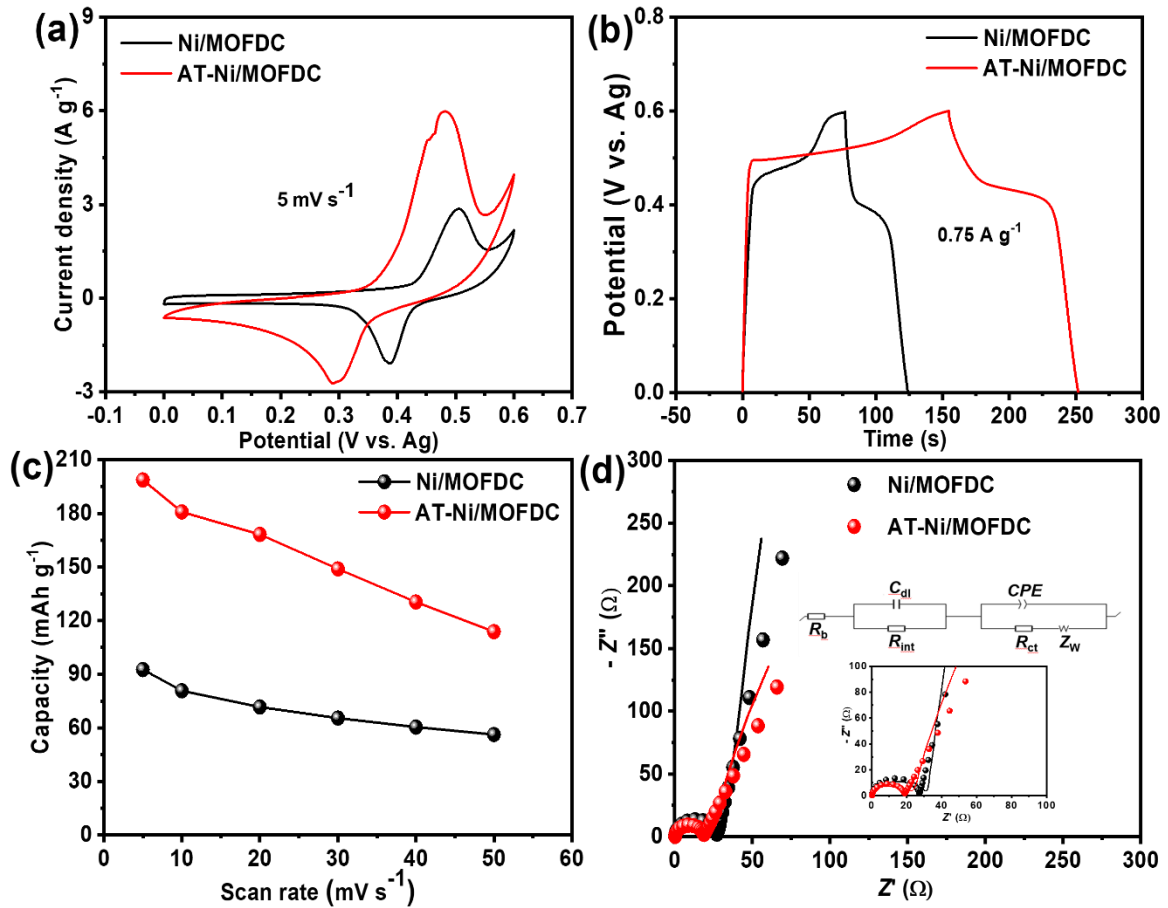
Figure 5.4: (a) CV curves, (b) GCD curves, (c) gravimetric specific capacity and (d) Nyquist plots of the Ni/MOFDC and AT-Ni/MOFDC for the three-electrode system.
