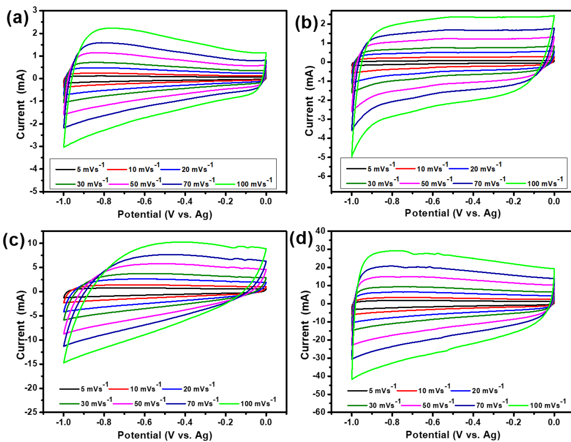
Figure S2: CV curves of (a) CFs, (b) CNTs, (c) CNT@CF and (d) N-CNT@CF network.
