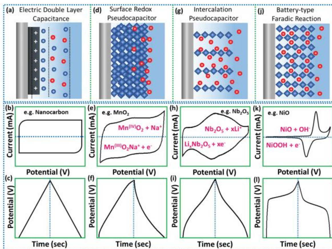
Figure 2.6: Energy storage mechanisms along with their electrochemical signatures: (a–c) electrical double layer capacitance, (d–f) surface redox capacitance, (g–i) intercalation capacitance and (j–l) faradic battery-type [39].
