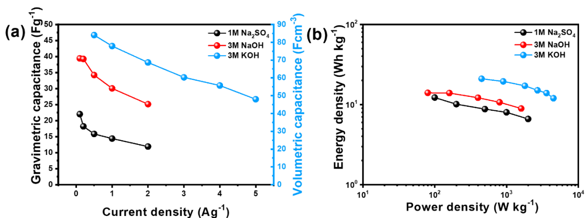
Figure S4: Capacitance and Ragone plot of asymmetric capacitors on N-CNT@CF//Na 0.44 MnO 2 in 1M Na 2 SO 4 , 3M NaOH, and (c) 3M KOH.
