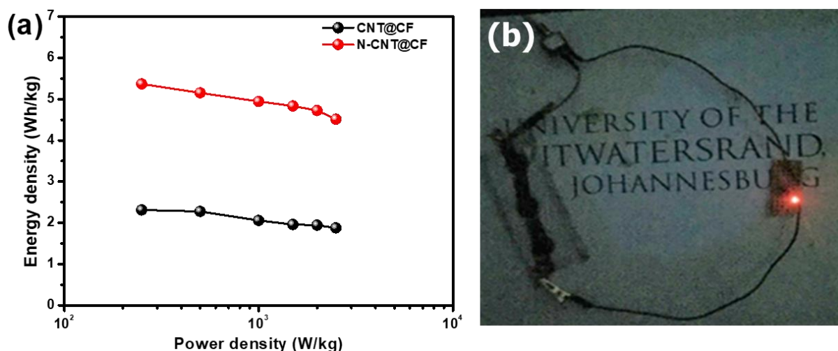
Figure 4.10: (a) Ragone plot and (b) image of 1.6 V red LED bulb lit up by N-CNT@CF supercapacitor.
