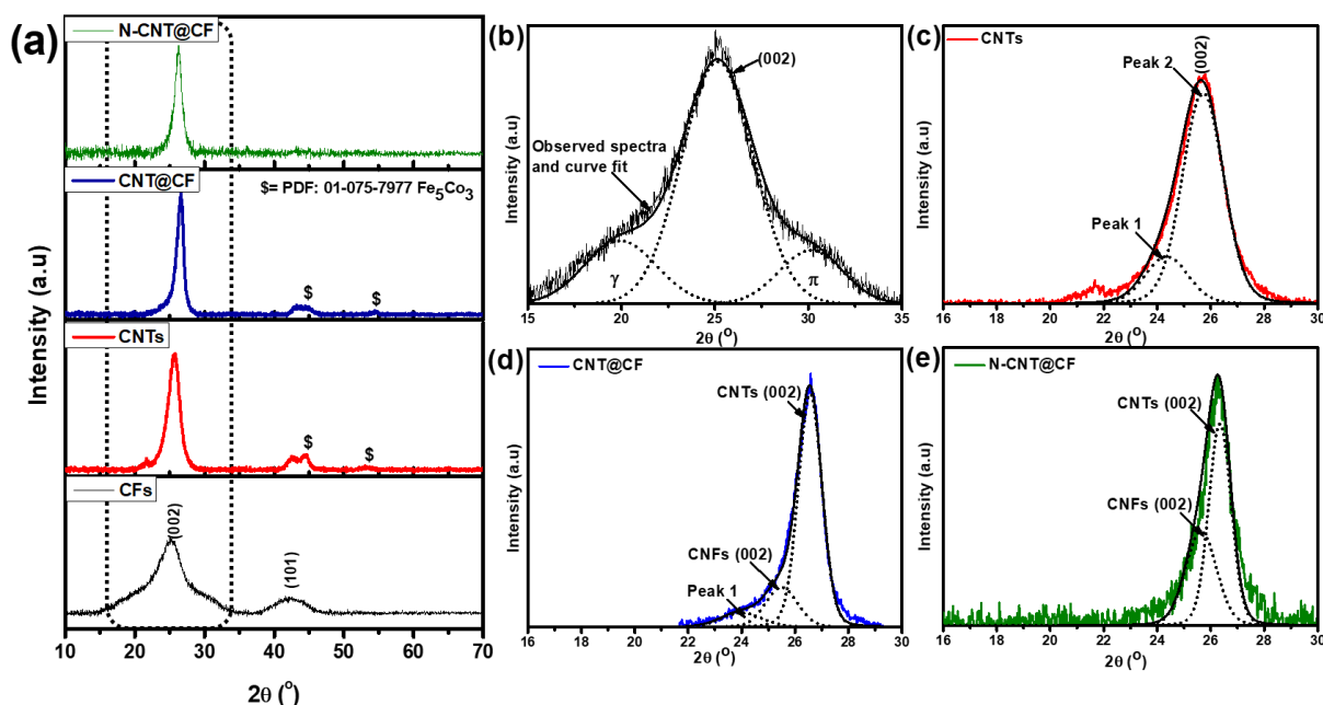
Figure 4.2: P-XRD patterns of (a) CFs, CNTs, CNT@CF network and N-CNT@CF network, and (b, c, d, e) deconvoluted (002) diffraction peak of all materials.
