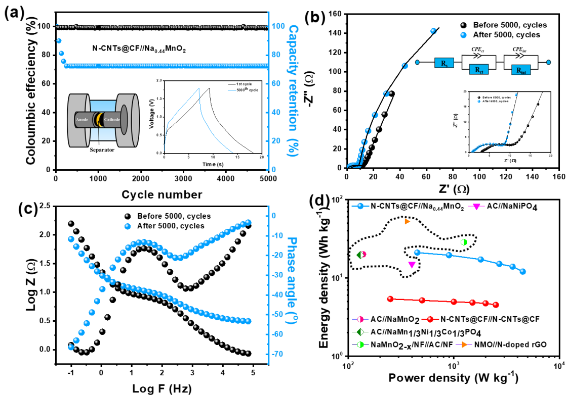
Figure 6.8: Electrochemical performance of the N-CNT@CF// \text{Na}_{0.44}\text{MnO}_2 asymmetric device: (a) cycling stability and coulombic efficiency of N-CNT@CF// \text{Na}_{0.44}\text{MnO}_2 asymmetric device at 5 \text{ A g}^{-1} , (b) Nyquist plots obtained before and after 5,000 charge-discharge cycles, (c) Bode plots before and after 5,000 cycles of the N-CNT@CF// \text{Na}_{0.44}\text{MnO}_2 device and (e) comparative Ragone plot of this work with recent literature.
