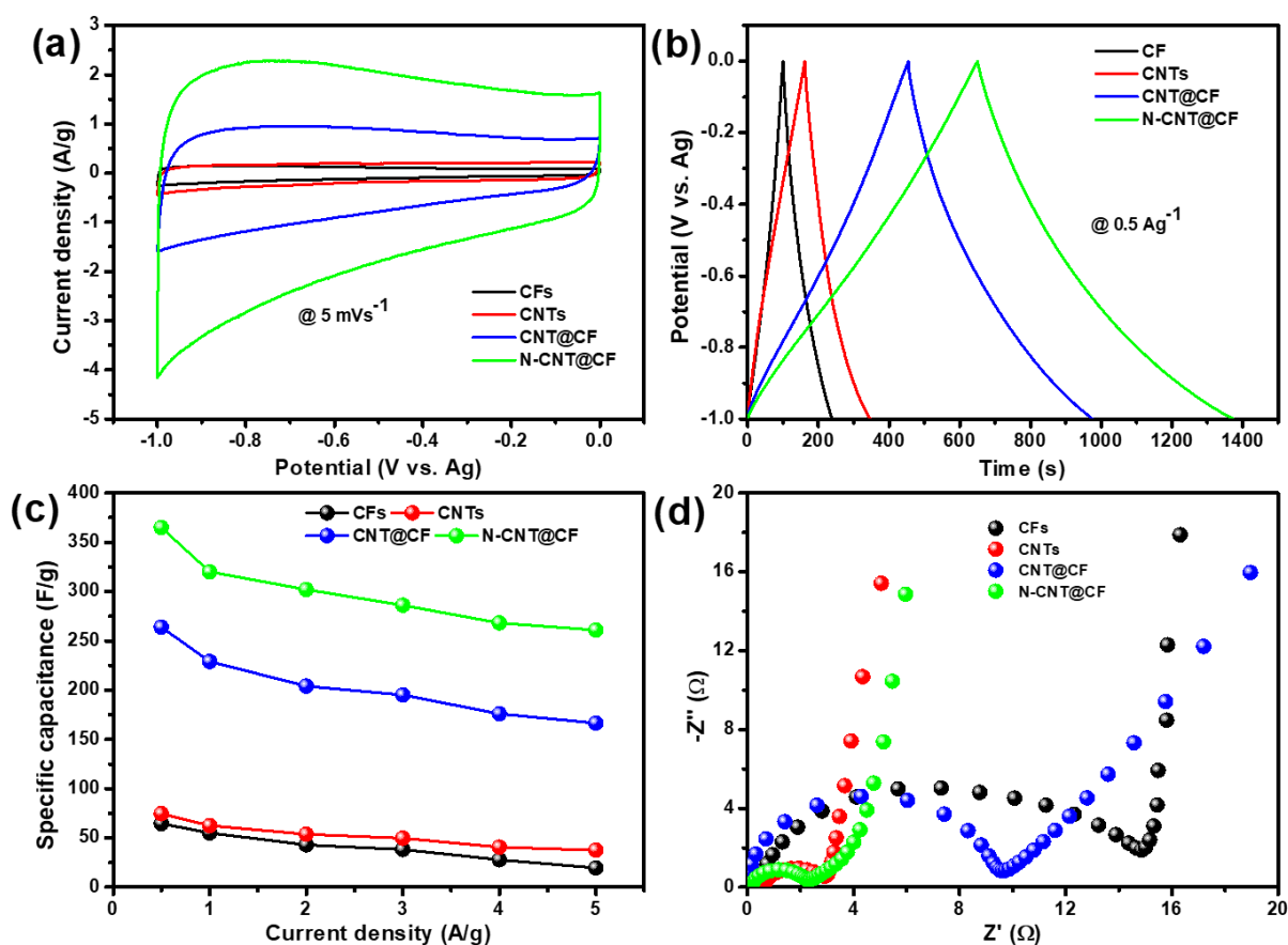
Figure 4.7: CV curves of (a) CFs, CNTs, CNT@CF and N-CNT@CF at 5 \text{ mVs}^{-1} scan rates (b) GCD comparison of CFs, CNTs, CNT@CF and N-CNT@CF at 0.5 \text{ Ag}^{-1} , (c) Comparison of specific capacitance of at different current densities, (d) EIS measurements of all electrode materials.
