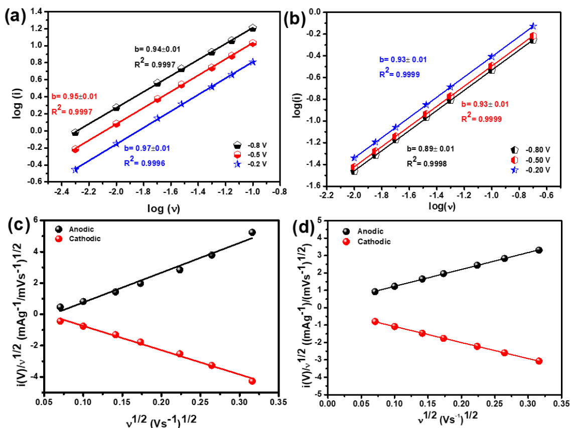
Figure S4: (a) Log peak current vs log scan rate for CNT@CF network anodic, (b) Log peak current vs log scan rate for N-CNT@CF network anodic, (c) i/v^{1/2} vs. v^{1/2} for CNT@CF network and (d) i/v^{1/2} vs. v^{1/2} N-CNT@CF network.
