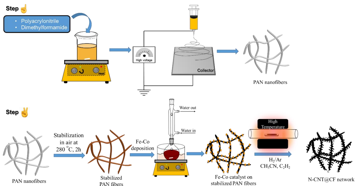
Scheme 3.1: Fabrication of N-CNF@CF network by electrospinning and CVD method.
