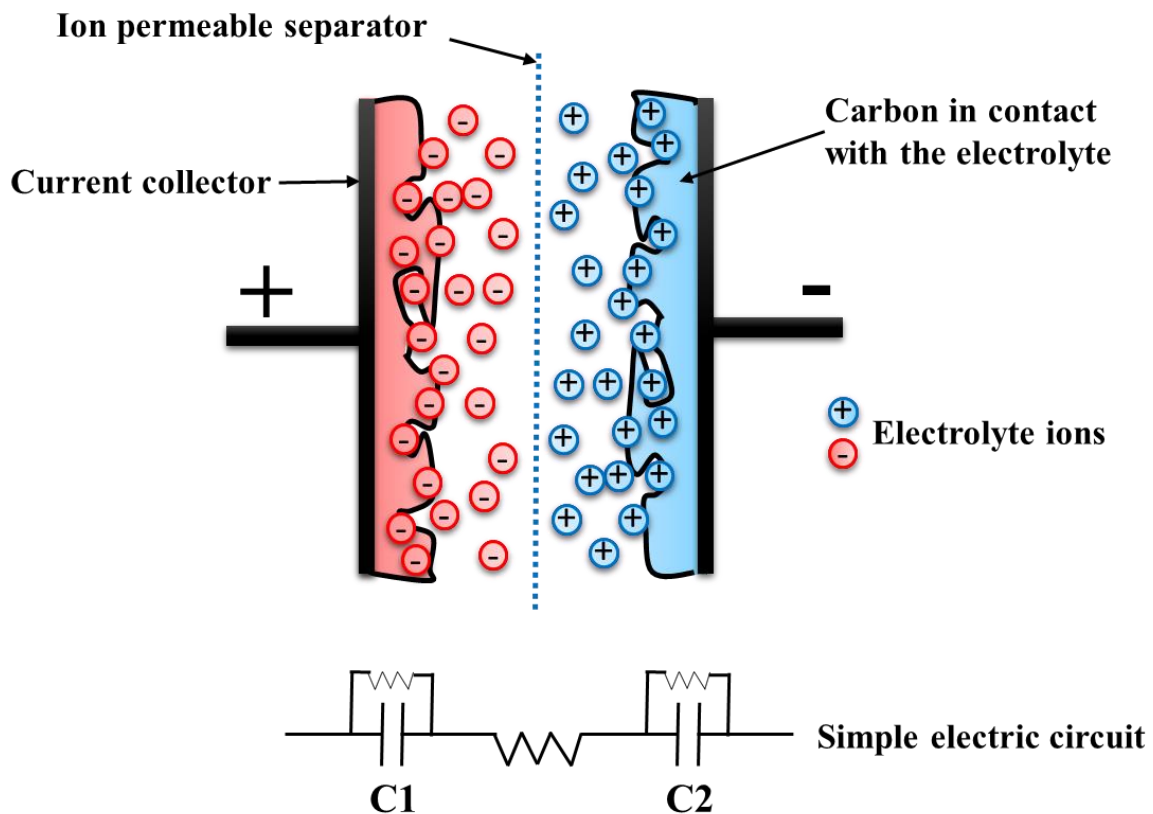
Figure 2.5: EDLC with porous electrodes in a charged state with equivalent circuit (Adapted from [34]).
