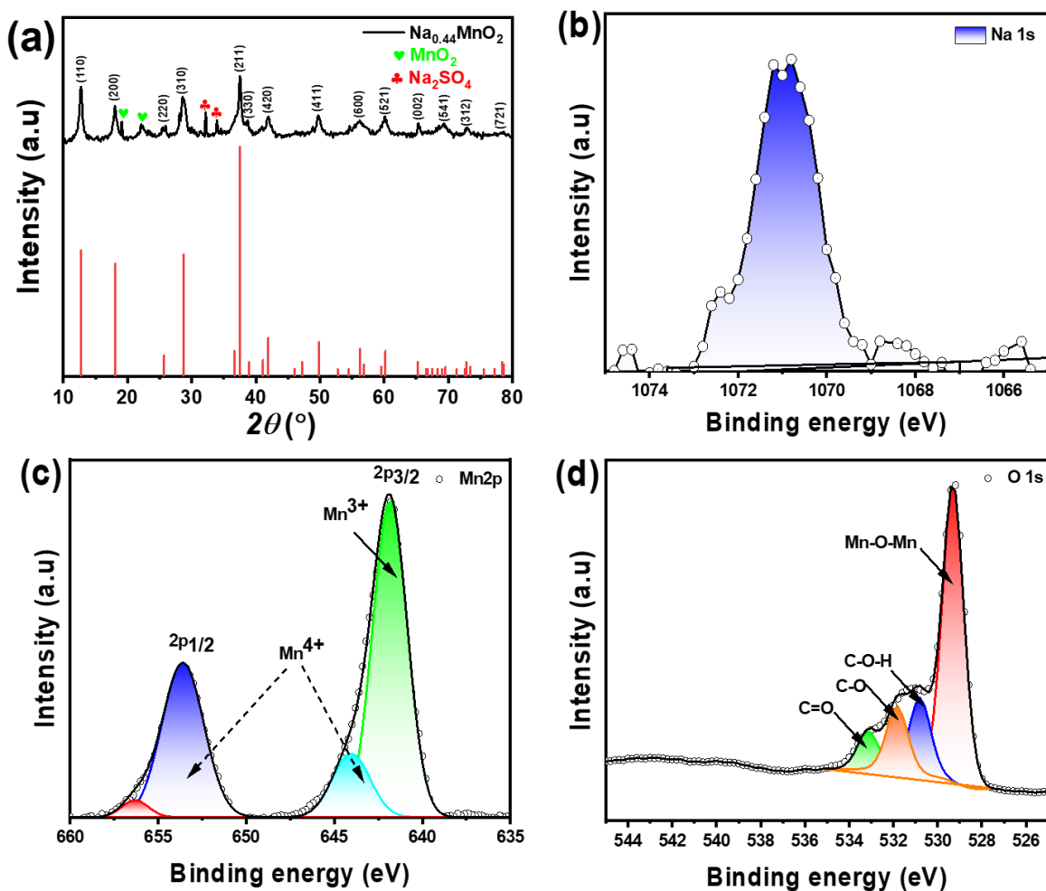
Figure 6.2: (a) X-ray diffraction (XRD) pattern of \text{Na}_{0.44}\text{MnO}_2 , (b) X-ray photoelectron spectroscopy (XPS) analysis, (b) narrow scan of Na, (c) Mn 2p and (d) O 1s.
