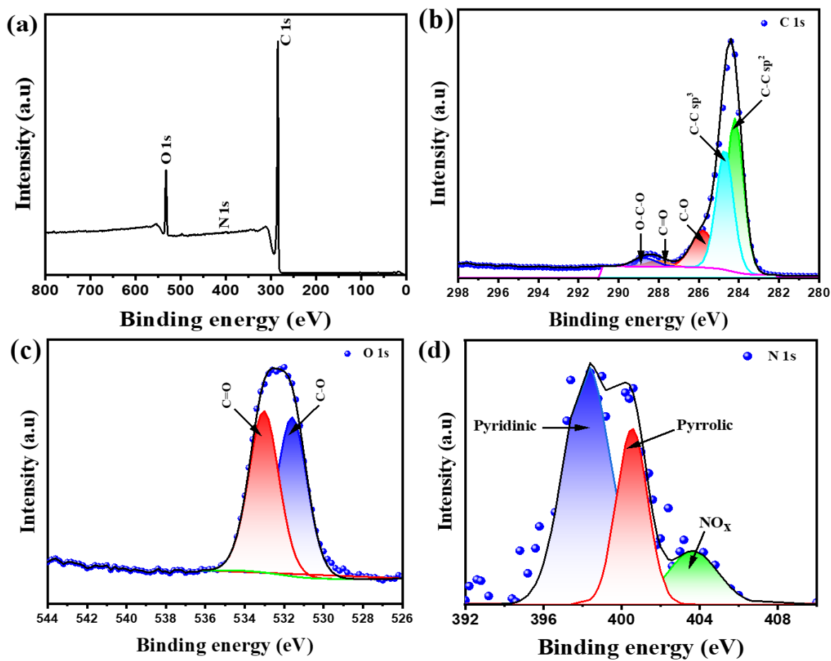
Figure 7.3: (a) XPS survey spectra of the N-rGO, (b) high resolution C 1s XPS spectra, (c) high resolution O 1s XPS spectra, (d) high resolution N 1s XPS spectra.
