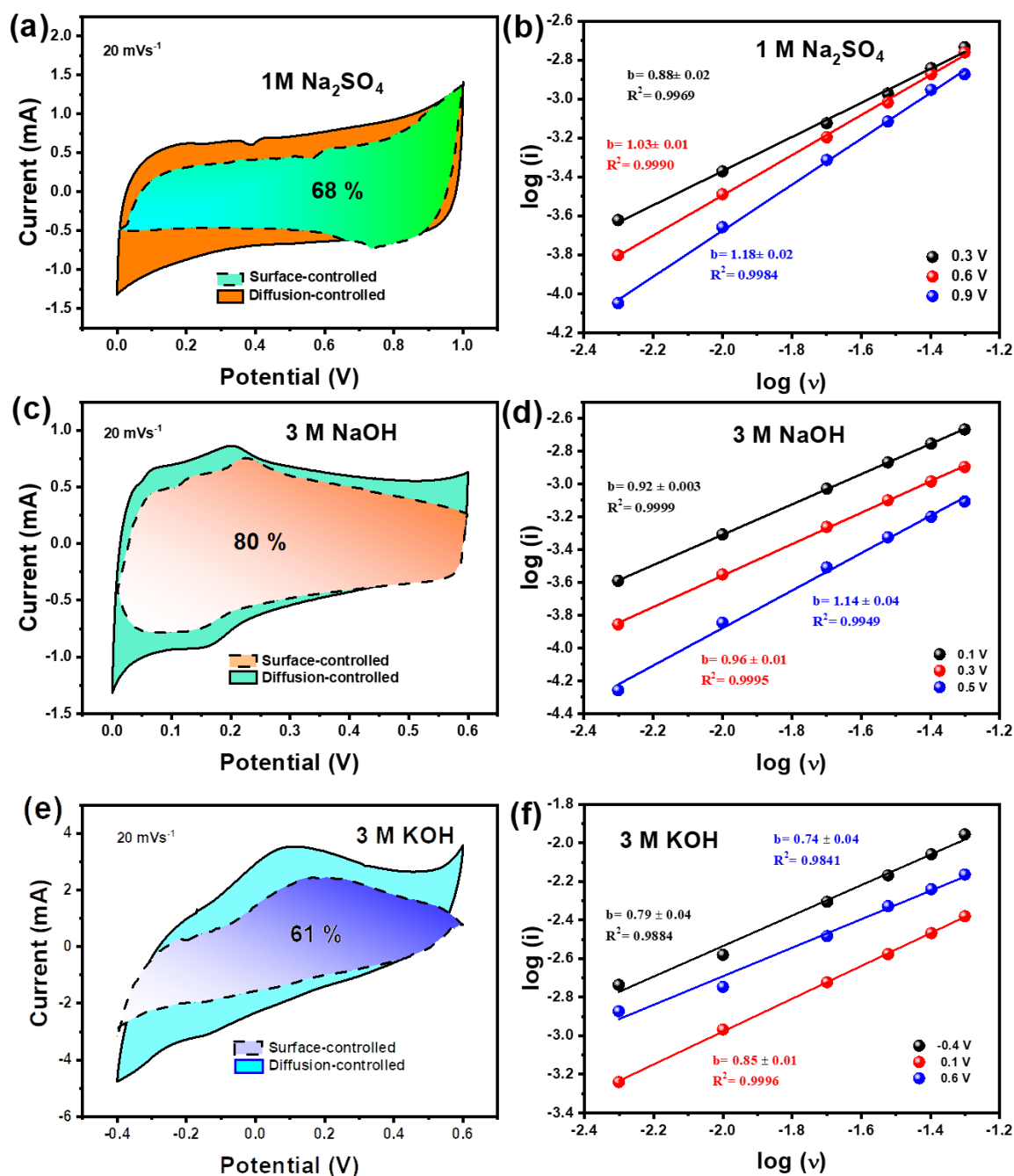
Figure 6.6: (a, c & e) Comparison of the capacitive and diffusion-controlled contributions fraction for \text{Na}_{0.44}\text{MnO}_2 at 20 \text{ mV s}^{-1} in different electrolytes, (b, d & f) log peak current vs. log scan rate for \text{Na}_{0.44}\text{MnO}_2 in different electrolytes.
