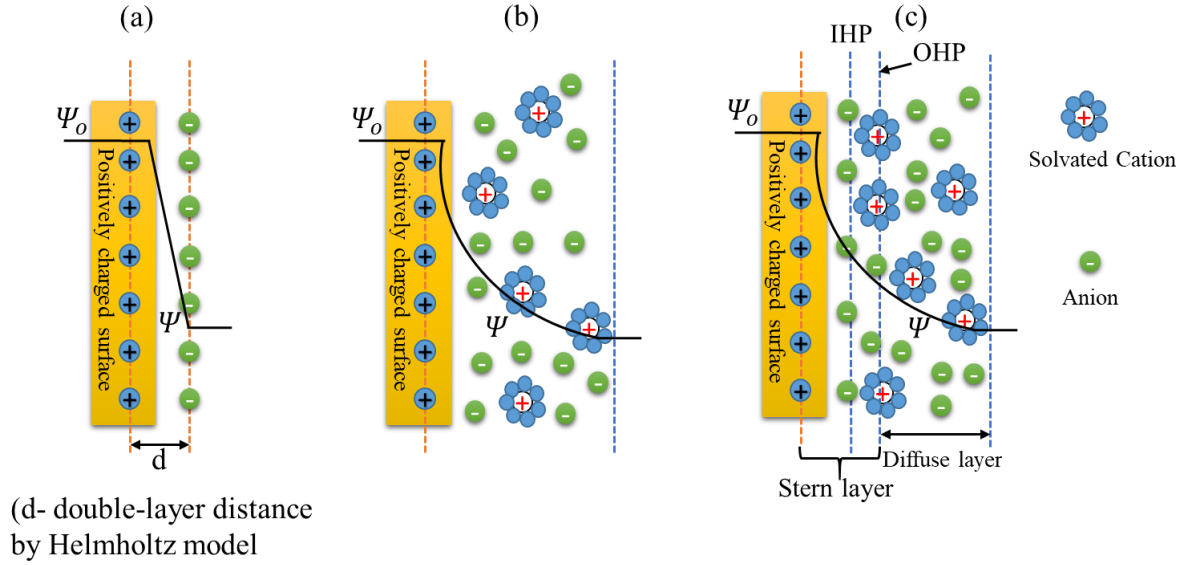
Figure 2.4: Models of the electrical double layer at a positively charged surface: (a) the Helmholtz model, (b) the Gouy–Chapman model and (c) the Stern model (Adapted from Ref [32]).
