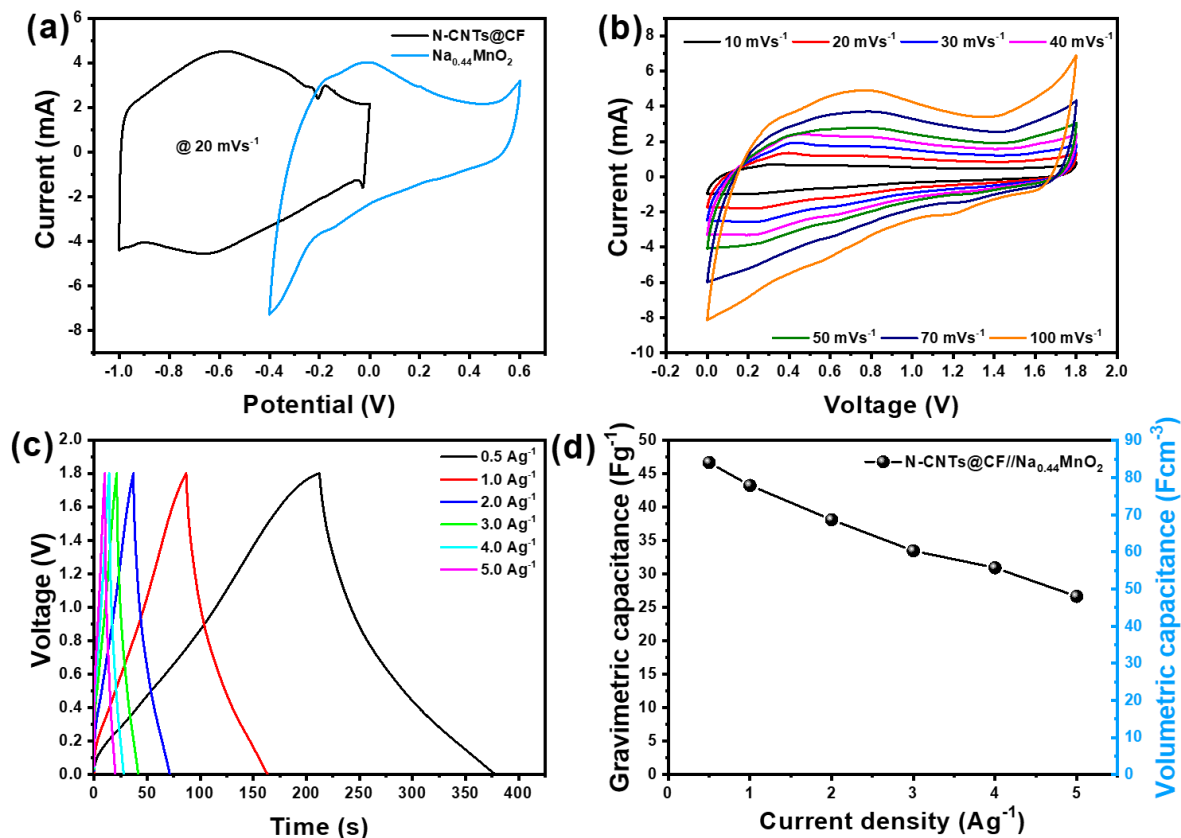
Figure 6.7: (a) CV curves of N-CNT@CF and Na 0.44 MnO 2 , (b) CV curves of N-CNT@CF//Na 0.44 MnO 2 at different scan rates, (c) typical GCD curves of N-
