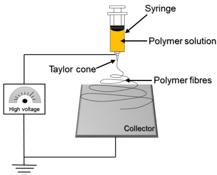
Figure 2.11: Schematic diagram of electrospinning PAN including basic electrospinning setup, Taylor cone and bending instability.
