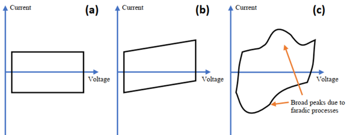
Figure 2.15: A representation of cyclic voltammograms of (a) an ideal capacitor, (b) a capacitor with resistivity and (c) pseudocapacitors [166].
