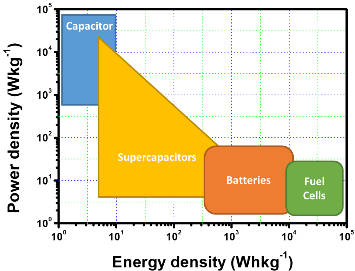
Figure 2.1: Ragone plot depicting specific energy versus specific power for various energy storage and conversion devices [11].
