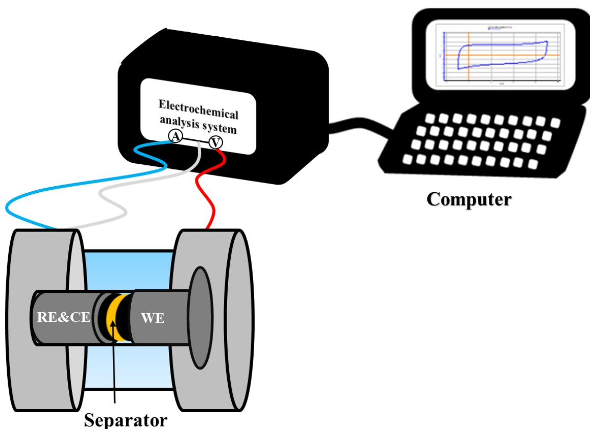
Figure 2.14: A two-electrode configuration using a battery-type Swagelok cell.
