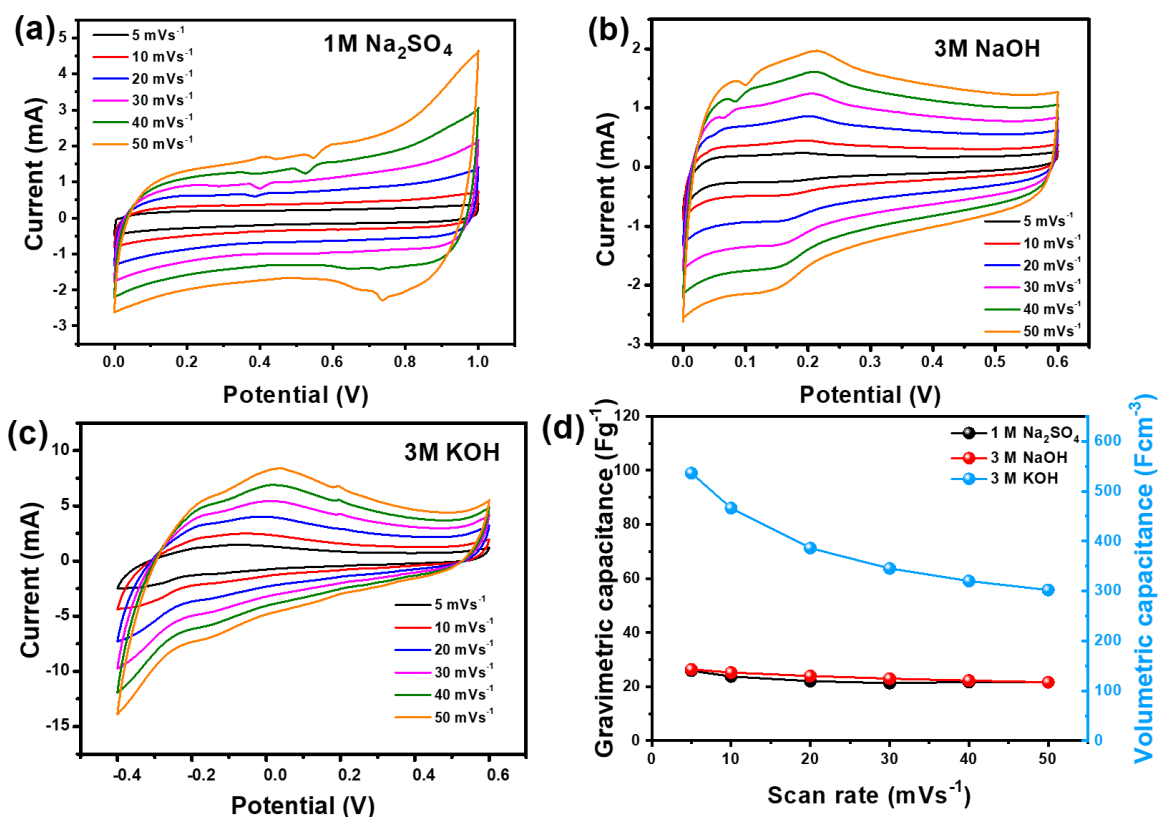
Figure 6.3: The CV curves of \text{Na}_{0.44}\text{MnO}_2 in (a) 1M \text{Na}_2\text{SO}_4 , (b) 3M \text{NaOH} and (c) 3M \text{KOH} medium at scan rate ranging from 5 to 50 \text{mV s}^{-1} , (d) Specific gravimetric and volumetric capacitance versus scan rate of \text{Na}_{0.44}\text{MnO}_2 under different aqueous electrolytes.
