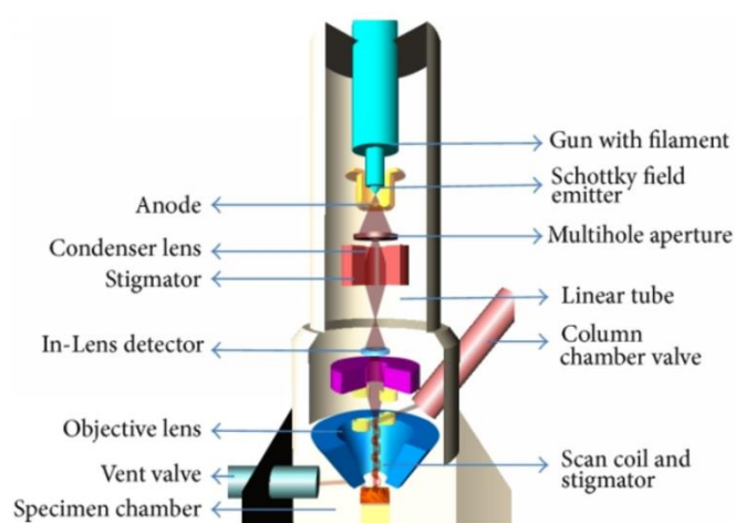
Figure 3.1: Schematic representation of an SEM operation [4].
