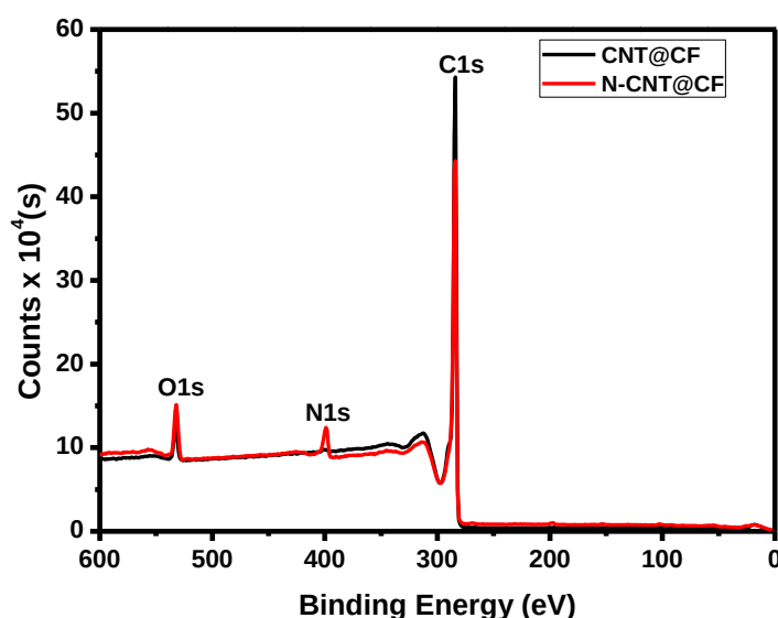
Figure 4.5: XPS survey spectra of CNT@CF network and N-CNT@CF network.
