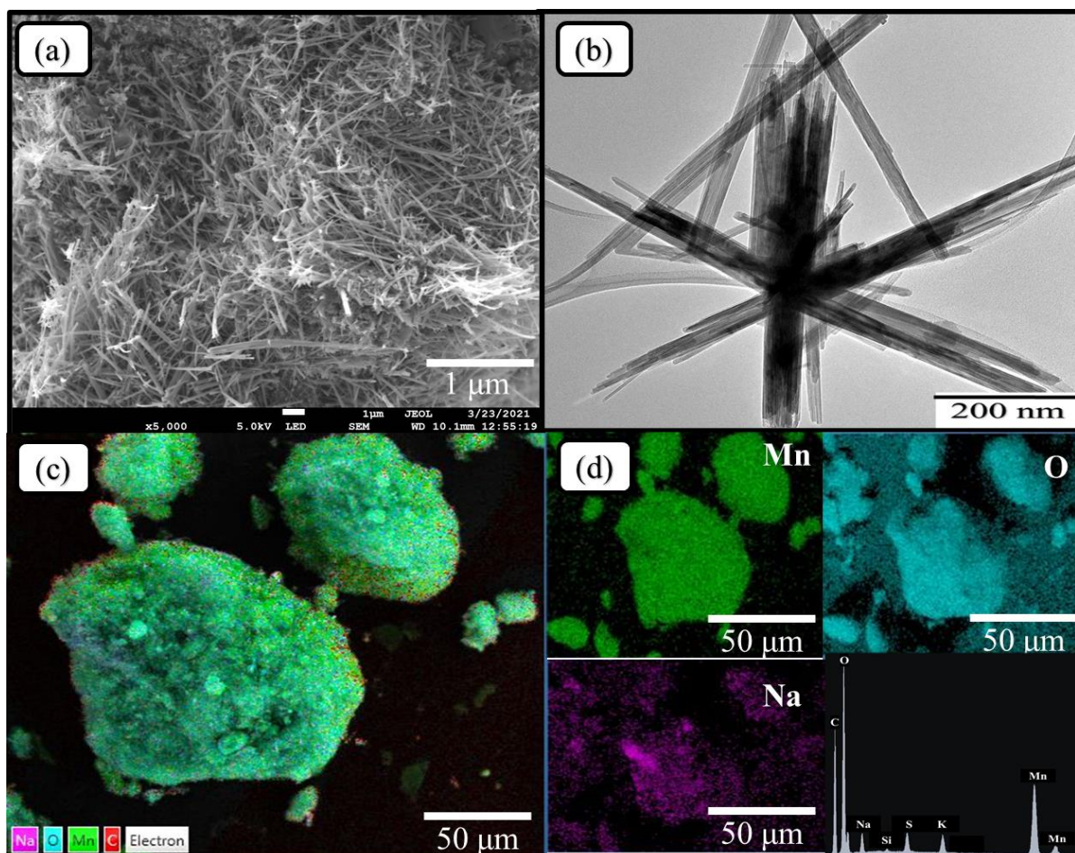
Figure 6.1: (a) SEM image of \text{Na}_{0.44}\text{MnO}_2 , (b) TEM image of \text{Na}_{0.44}\text{MnO}_2 , (c) EDS mapping images of \text{Na}_{0.44}\text{MnO}_2 and (d) elemental mapping of Mn, O and Na together with the corresponding EDS spectrum.
