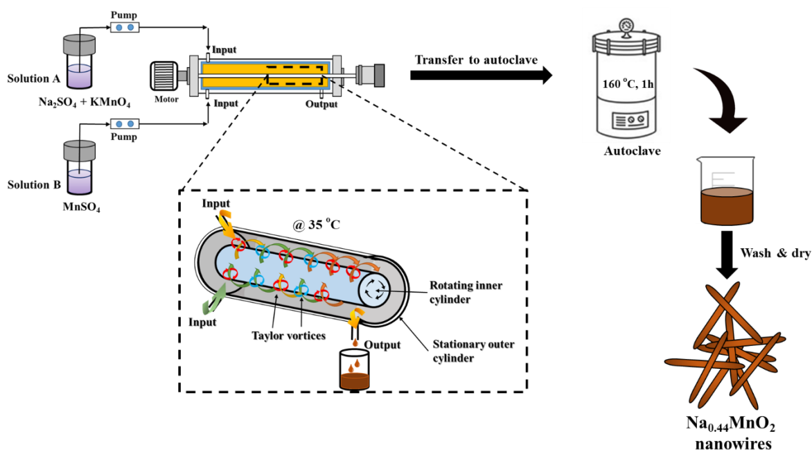
Scheme 3.3: Schematic illustrations of the synthesis of the \text{Na}_{0.44}\text{MnO}_2 .
