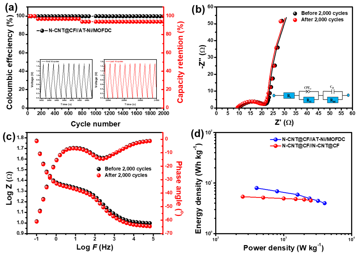
Figure 5.7: Electrochemical performance of the N-CNT@CF//AT-Ni/MOFDC hybrid device: (a) typical cycling performance at 5 \text{ A g}^{-1} , (b) Nyquist plots obtained before and after 2,000 charge-discharge cycles, (c) Bode plots before and after 2,000 cycles of the N-CNT@CF//AT-Ni/MOFDC device and (d) comparative Ragone plot of this work with a symmetric N-CNT@CF//N-CNT@CF.
