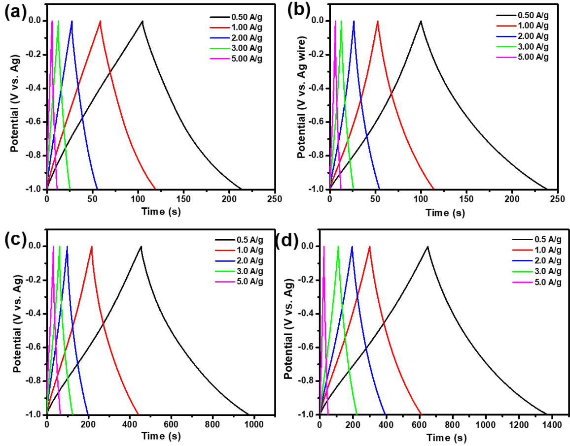
Figure S3: GCD curves of (a) CFs, (b) CNTs, (c) CNT@CF and (d) N-CNT@CF network.
