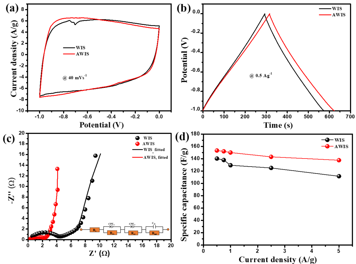
Figure 7.6: Half-cell electrochemical characterization of N-rGO anode material (a) CV plots of N-rGO in different electrolytes collected at scan rates of 40 mV s -1 , (b) galvanostatic charging-discharging plots collected at the current density of 0.5 A g -1 , (c) EIS measurements of N-rGO electrode in different electrolytes and (d) variation of specific capacitance as a function of current density.
