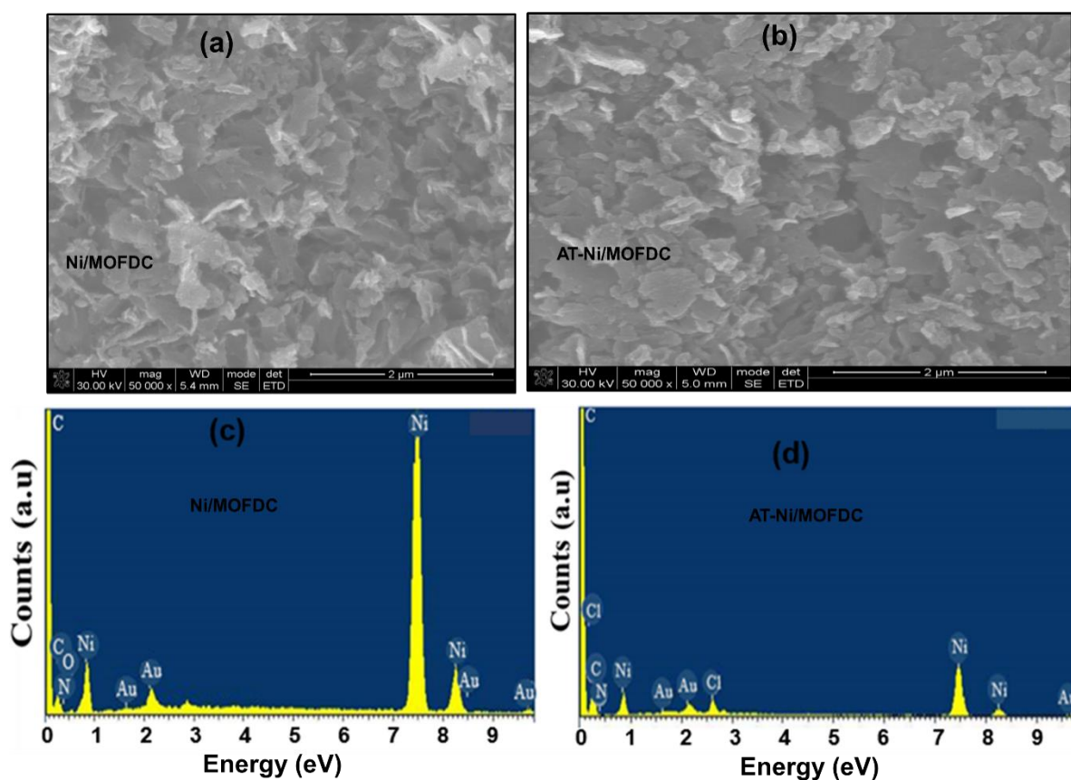
Figure S3: SEM images of the (a) Ni/MOFDC, (b) AT-Ni/MOFDC, EDS spectra of the (c) Ni/MOFDC, and (d) AT-Ni/MOFDC.
