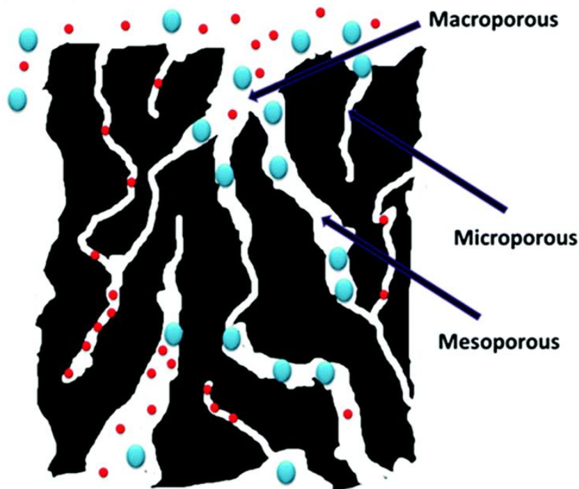
Figure 2.9: An illustration of a typical activated carbon structure with strongly disordered macropores ( >50 nm), mesopores (2–50 nm) and micropores (less than 2 nm) (Adapted from [64]).
