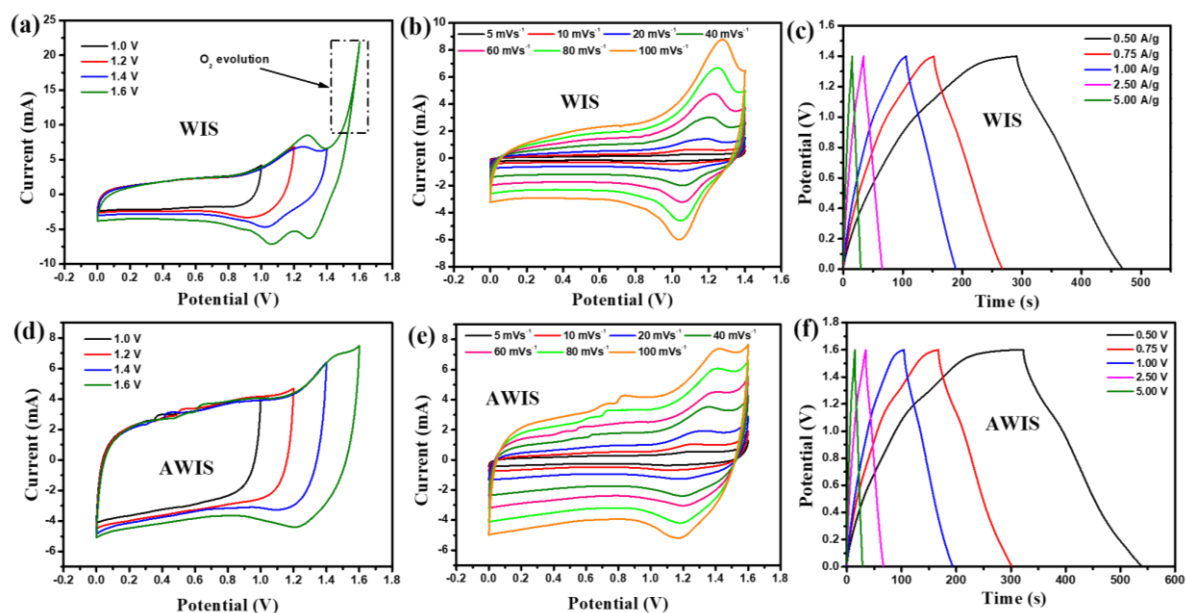
Figure S1: (a, d) Electrochemical stable window, (b, e) CV at various scan rates and (c, f) GCD at various current densities of \text{Na}_{0.44}\text{MnO}_2 in WIS and AWIS electrolytes.
