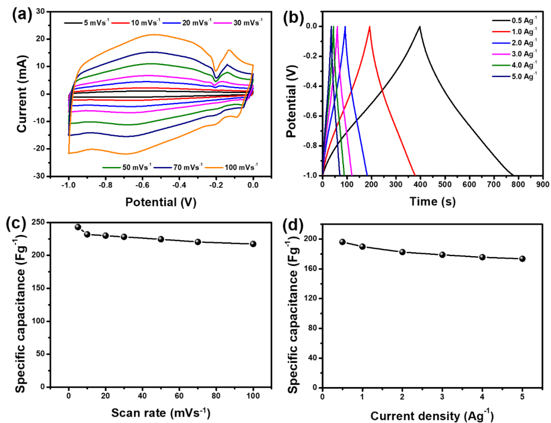
Figure S7: (a) CV curves of N-CNT@CF, (b) GCD curves of N-CNT@CF, (c) specific capacitance from CV, and (d) specific capacitance from GCD in 3M KOH.
