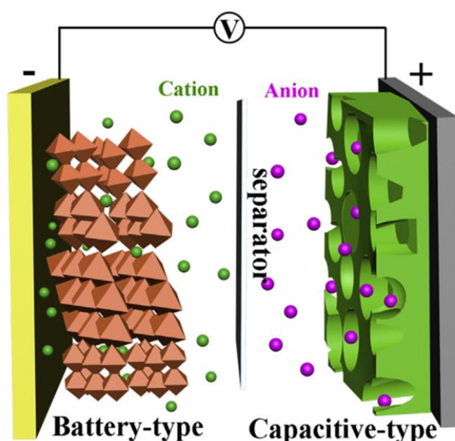
Figure 2.7: The fundamental configuration of the HSCs [49].
