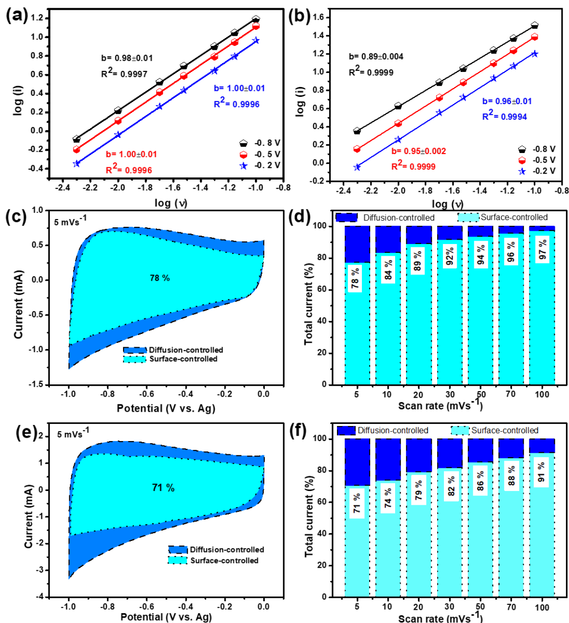
Figure 4.8: Log peak current vs log scan rate for (a) CNT@CF and (b) N-CNT@CF obtained at the cathodic directions; Typical charge storage contributions from capacitive and diffusive processes from cyclic voltammetry at 5 \text{ mVs}^{-1} for (c) CNT@CF and (e) N-CNTs/CF; Comparative histograms of the percentage charge storage contributions from capacitive and diffusive processes from 5-100 \text{mVs}^{-1} for (d) CNT@CF and (f) N-CNTs/CF.
