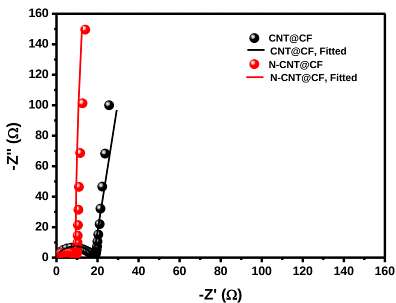
Figure S4: EIS measurements of CNT@CF and N-CNT@CF electrodes, before 10,000 cycles.
