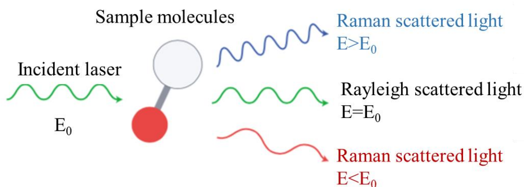
Figure 3.3: Rayleigh and Raman light scattering by molecules [10].
