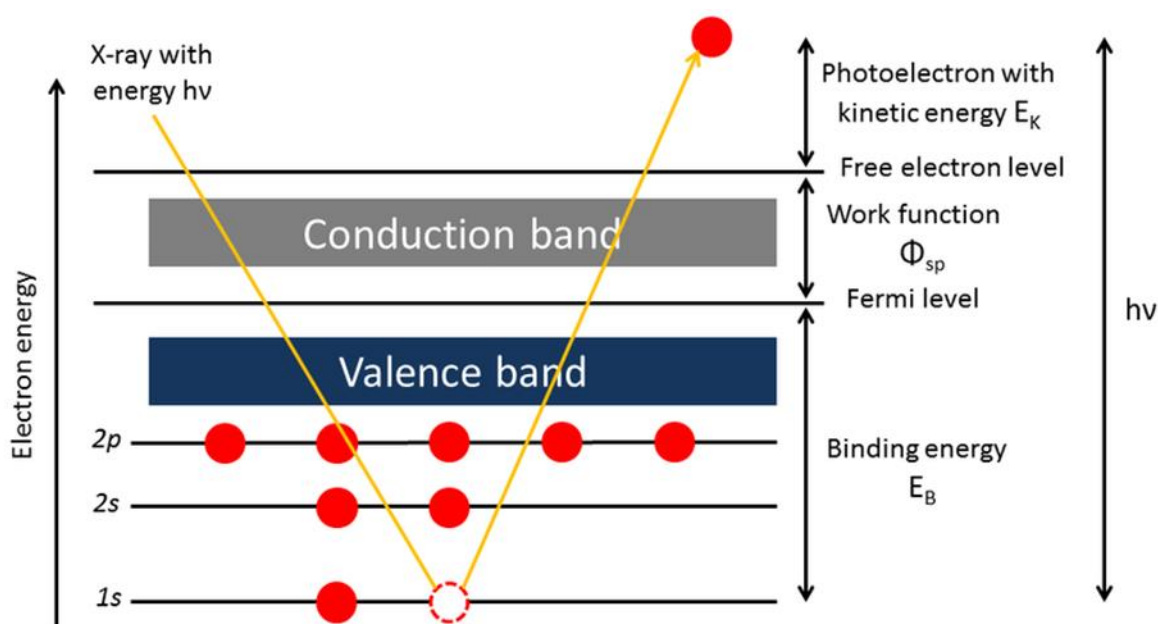
Figure 3.4: Schematic diagram of XPS operation [14].
