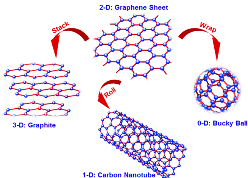
Figure 2.12: The 2D hexagonal nanosheets of graphene as a building block of other forms. An illustration of different allotropes of carbon arising from a graphene sheet (Adapted from Ref [99]).
