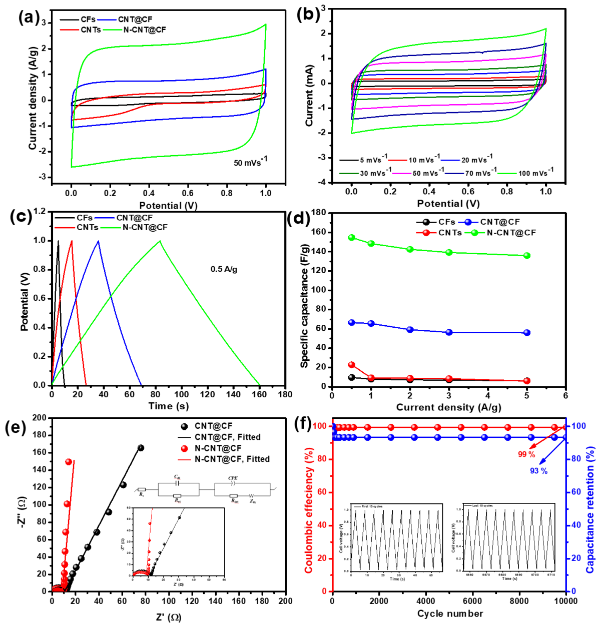
Figure 4.9: CV curves of (a) CFs, CNTs, CNT@CF and N-CNT@CF at 50 mV s -1 scan rates (b): CV curves of N-CNT@CF at different scan rates, (c) GCD comparison of CFs, CNTs, CNT@CF and N-CNT@CF at 0.5 A g -1 ; (d) Comparison of specific capacitance of at different current densities, (e) EIS measurements of CNT@CF and N-CNT@CF electrodes and (f) coulombic efficiency and capacitance retention of N-CNT@CF.
