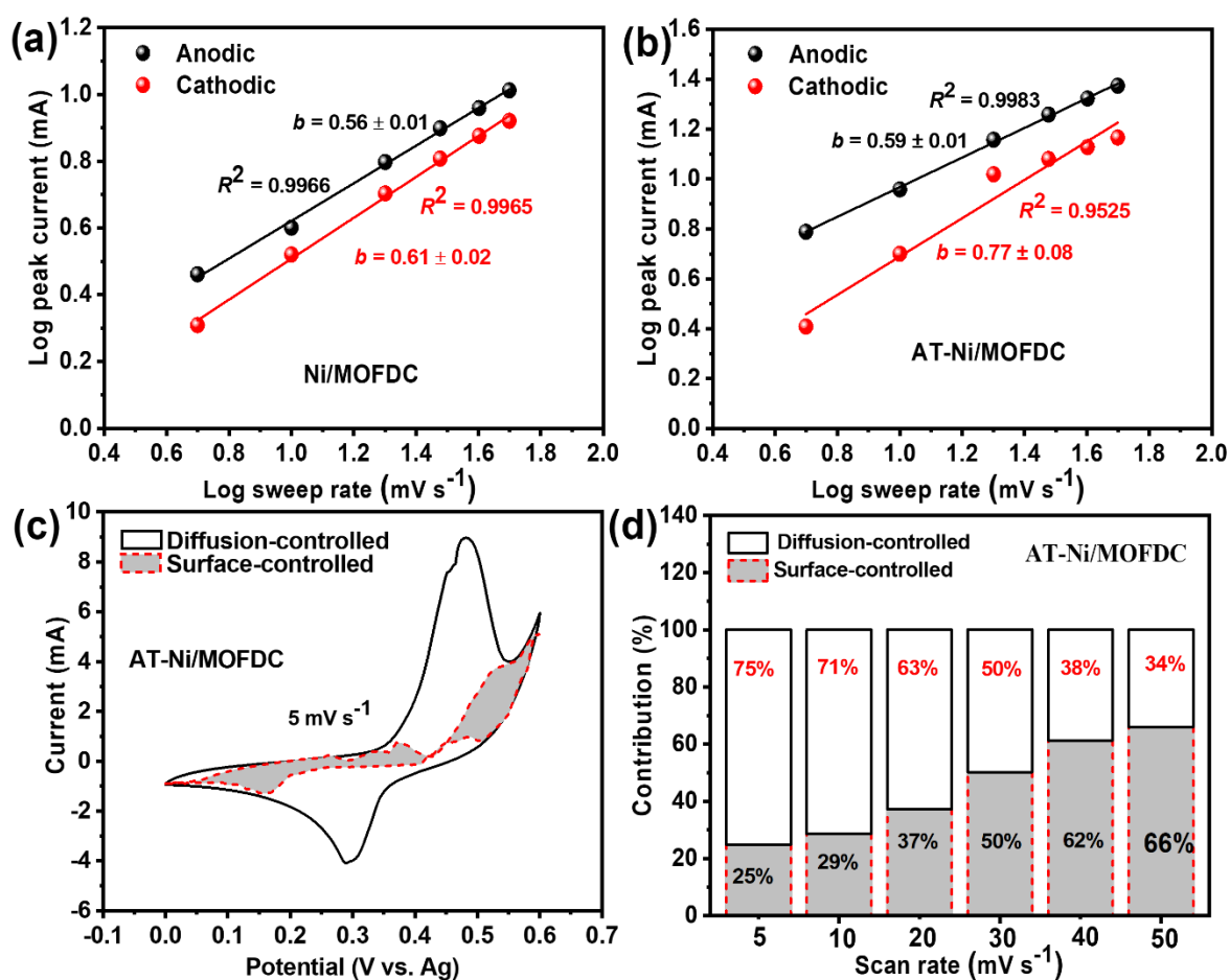
Figure 5.5: (a) Log peak current vs log scan rate for Ni/MOF, (b) Log peak current vs Log scan rate for AT-Ni/MOF, (c) Comparison of the capacitive and diffusion-controlled contributions fraction for the AT-Ni/MOFDC at 5 \text{ mV s}^{-1} and (d) histograms of the percentage contributions at 5–50 \text{mV s}^{-1} .
