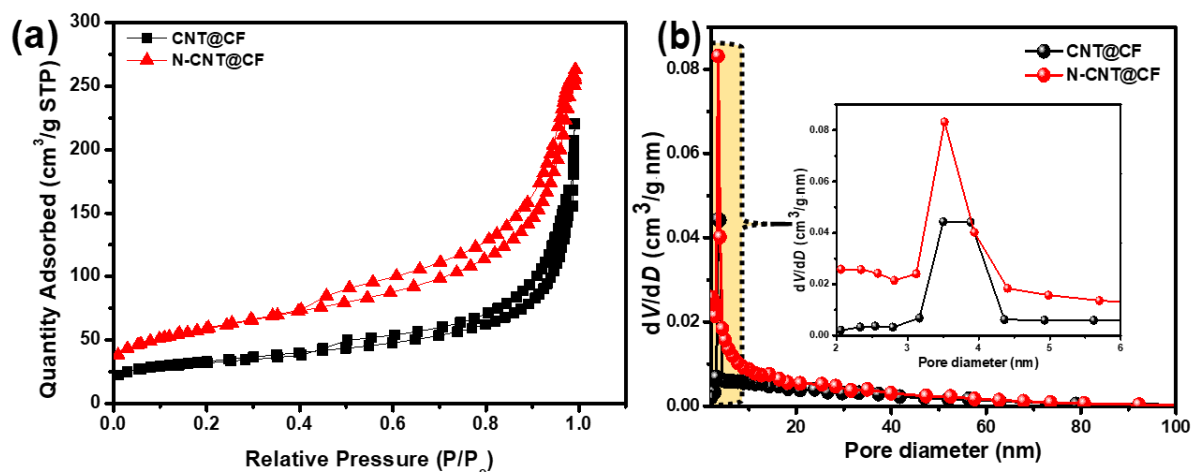
Figure 4.4: a) BET adsorption desorption curve and (b) pore size distribution curve of the CNT@CF network and the N-CNT@CF network (insert pore diameter between 2-6 nm).
