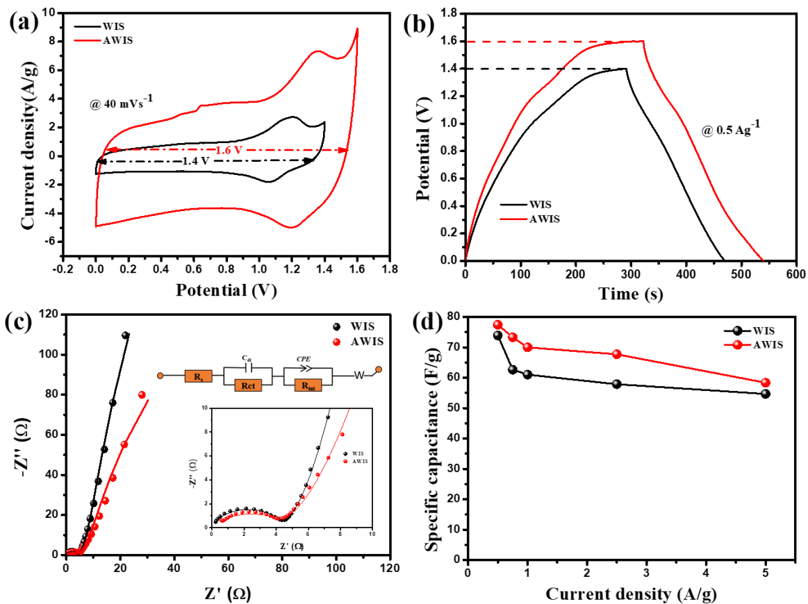
Figure 7.5: Half-cell electrochemical characterization of \text{Na}_{0.44}\text{MnO}_2 cathode material (a) CV plots of \text{Na}_{0.44}\text{MnO}_2 in different electrolytes collected at scan rates of 40 \text{ mV s}^{-1} , (b) galvanostatic charging-discharging plots collected at the current density of 0.5 \text{ A g}^{-1} , (c) EIS
