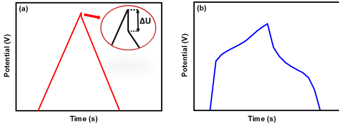
Figure 2.16: GCD plot of (a) an EDLC (the figure inset illustrates the IR drop) and (b) a redox active pseudocapacitor or faradaic [166].
