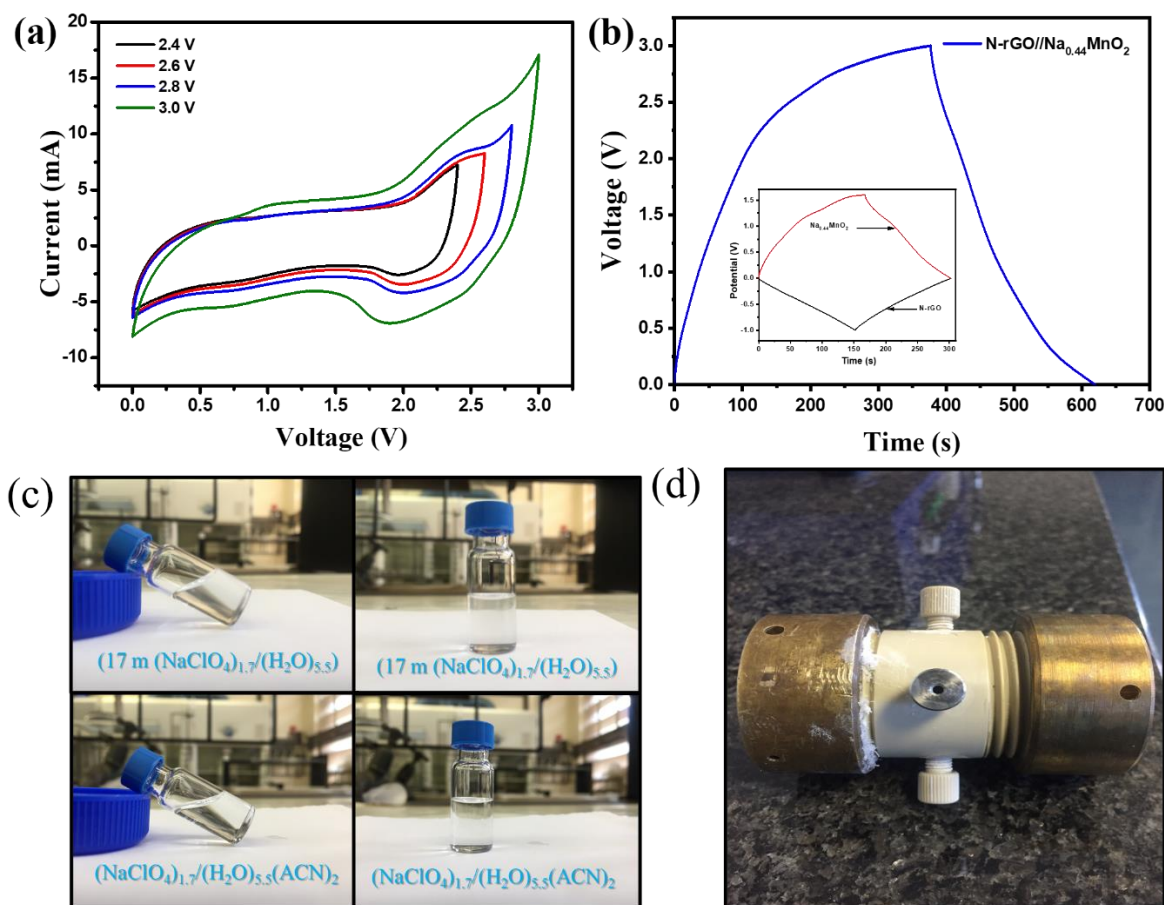
Figure S3: (a) electrochemical window of ASC device, (b) GCD of ASC device (insert GCD of N-rGO and Na 0.44 MnO 2 ), (c) images of WIS and AWIS electrolytes and (d) T-type Swagelok after 1,900 cycles (re-crystallization of the electrolyte).
