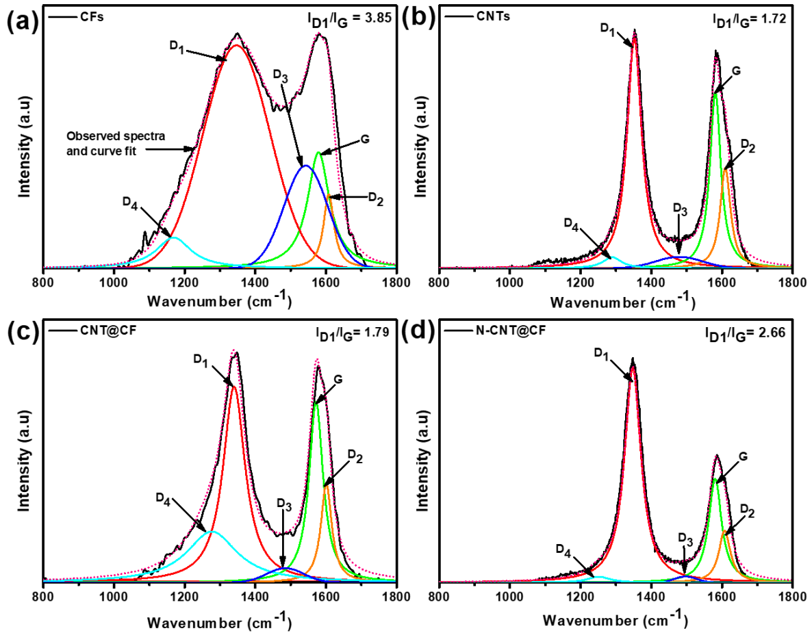
Figure 4.3: Raman spectra of (a) CFs, (b) CNTs, (c) CNT@CF network and (d) N-CNT@CF network.
