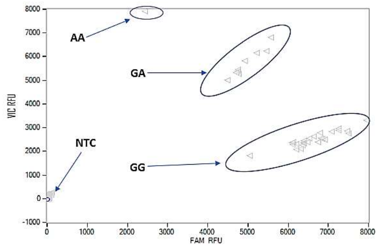
Figure 3.17: Two parameter amplification graph demonstrating the different genotype populations and NTC (No DNA) for AGT (rs699) polymorphism. FAM and VIC flourophores are represented by alleles G and A, respectively.
