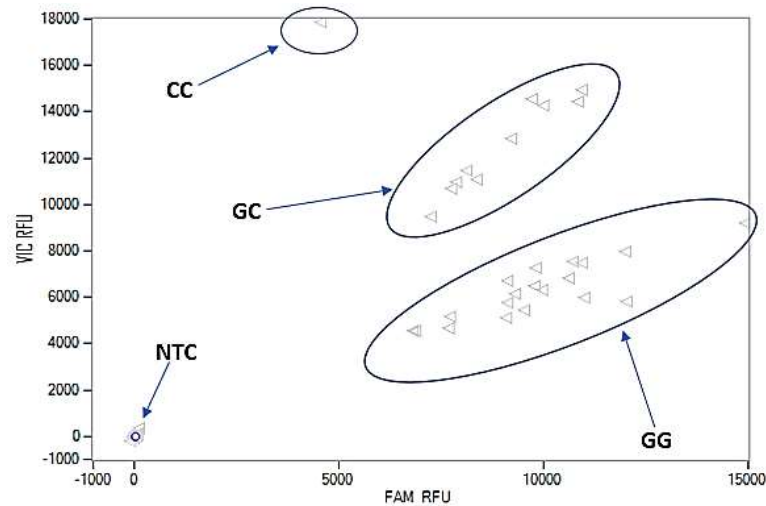
Figure 3.5: Two parameter amplification plots demonstrating the separation of the three genotype populations and NTC- No template controls (lower left population) for IL-6 (rs1800796) polymorphism. FAM and VIC are represented by allele G and C, respectively.
