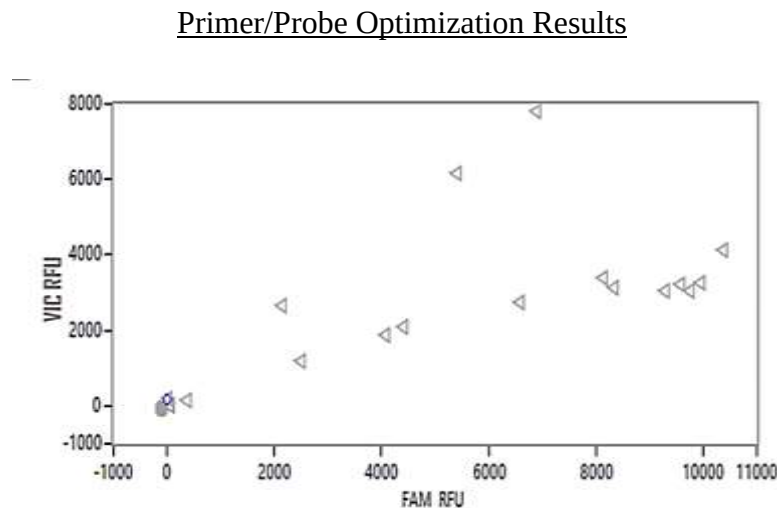
Figure 3.16: Allelic discrimination plot demonstrating sample amplification for the AGT SNP.
