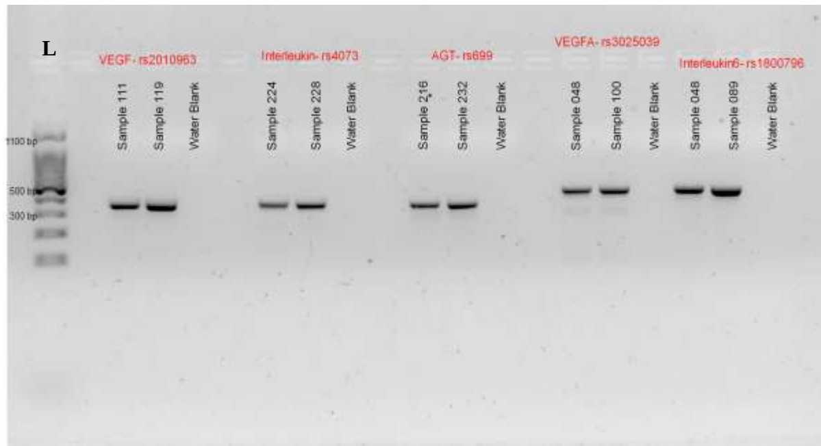
Figure 3.3: Gel photograph illustrating DNA products of various control samples that amplified for SNPs rs2010963, rs4073, rs699, rs3025039, and rs1800796. The PCR products were run on a 1% agarose gel containing ethidium bromide. L-DNA ladder (100 bp); water blanks- negative controls (no DNA).
