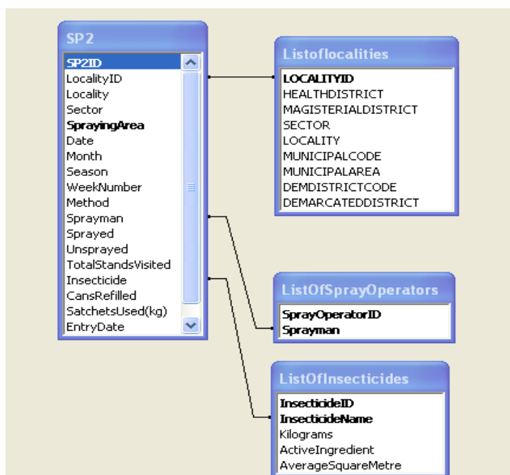
Figure 3.4 Entity relationship diagram
