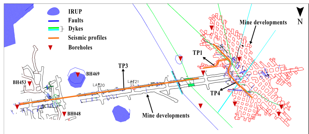
Figure 2. Underground mine plan, showing the location of the seismic profiles (orange) and geological structures such as faults (blue) and dolerite dyke (green) for in-mine seismic experiments.
