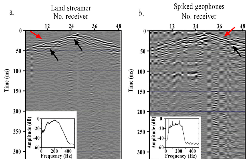
Figure 3. Shot gather examples with frequency spectrum from planted and landstreamer receivers. Shot 45 and shot 73. (a) Shows landstreamer shot gathers; (b) shows planted geophone shot gathers. Red arrows show first breaks, black arrows show reflections.
