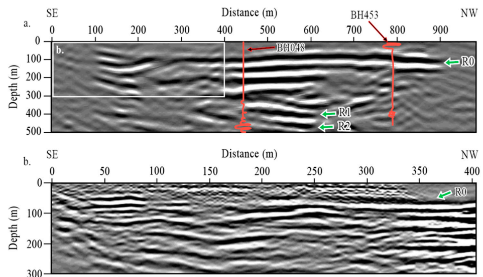
Figure 13. Migrated depth stack section of (a) SP2, with projected synthetic traces from the BH048, a depth discrepancy of ~25 m is a result of the borehole being ~50 m away from the seismic profile, and (b) SP3 shows clear reflections in the first 200 m. Green arrows mark different reflections detailed in the text.
