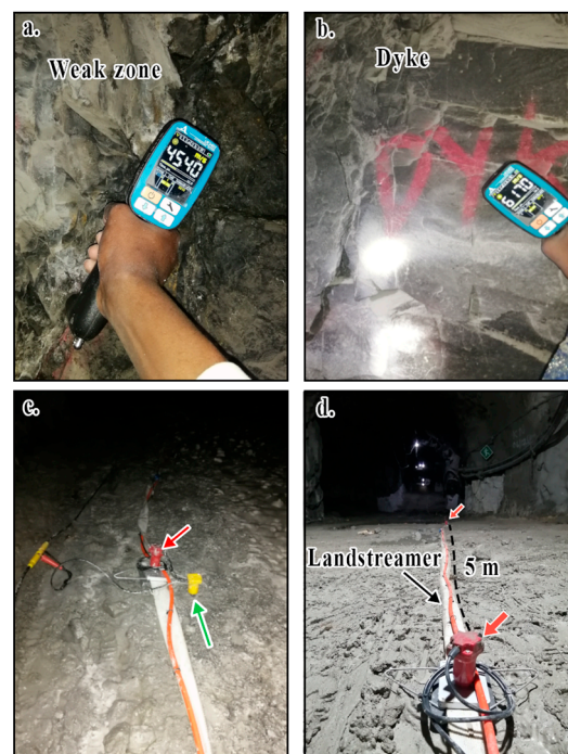
Figure 4. Measurements of the seismic velocities underground using an ultrasonic pulse meter over a (a) weak zone and (b) dyke. (c,d) Shows the setup inside the tunnel of the seismic survey using the seismic landstreamer (red arrows) and planted geophone (green arrows).
