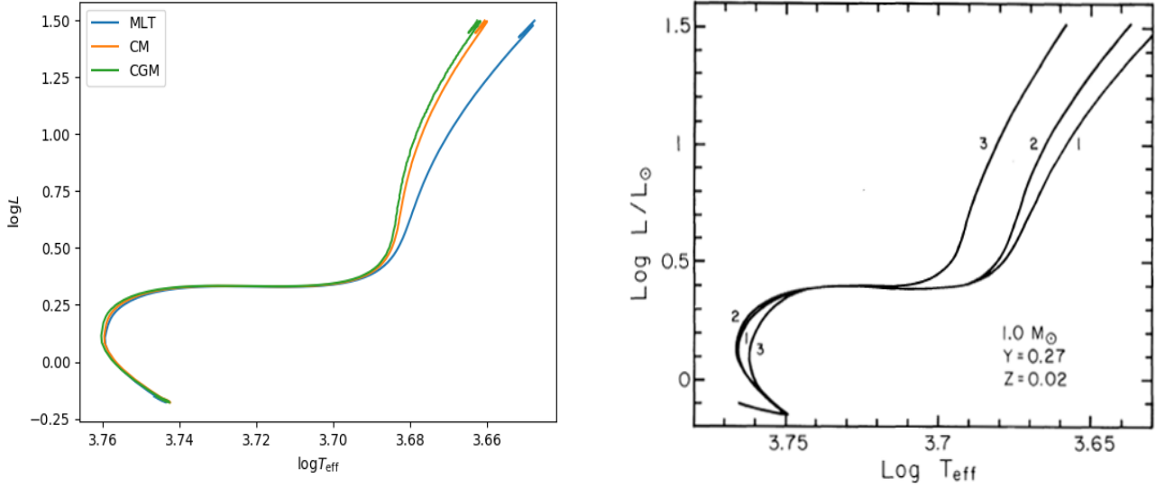
Figure 7.2: Comparison of the MESA implementation of the FST models for a 1 M_{\odot} star with Y = 0.28 and Z = 0.02 ( left panel ), against figure 6 of Canuto and Mazzitelli (1991) [22] ( right panel ) which considers the same evolution, but with Y = 0.27 , within the context of the ATON code . Note that the curves labelled ‘1’ and ‘2’ correspond to the solar calibrated MLT and CM models respectively, whereas the curve labelled ‘3’ corresponds to the CM model with l = z (which I have not implemented).
