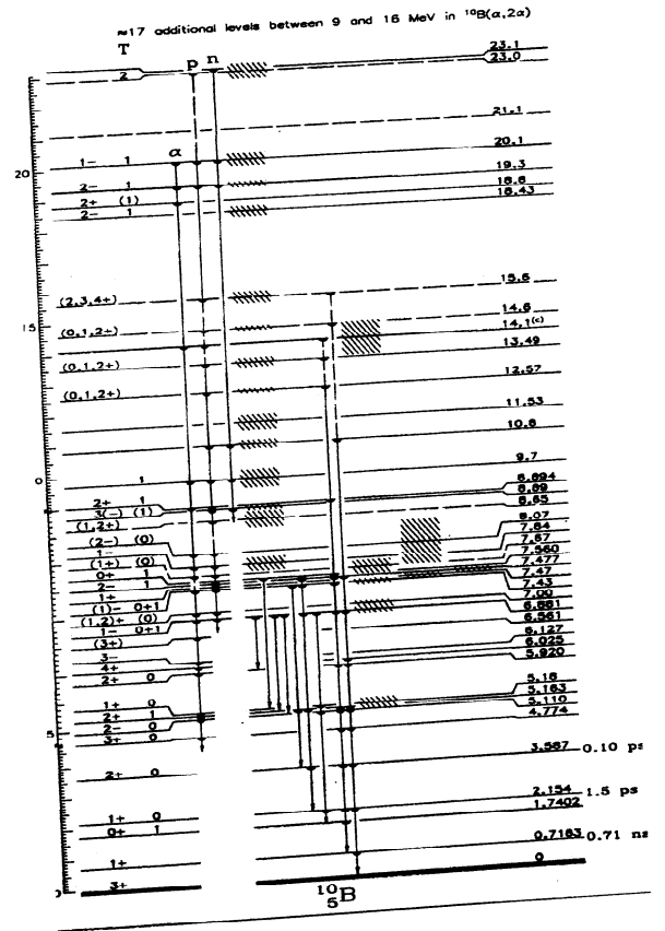
Figure 5. Nuclear level structure of ^{10}\text{B} [80].
