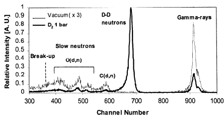
Figure 40. Gated TOF spectra obtained in the bombardment of evacuated target and target charged with deuterium gas at 1 bar at room temperature, with a 5 MeV deuteron beam.
