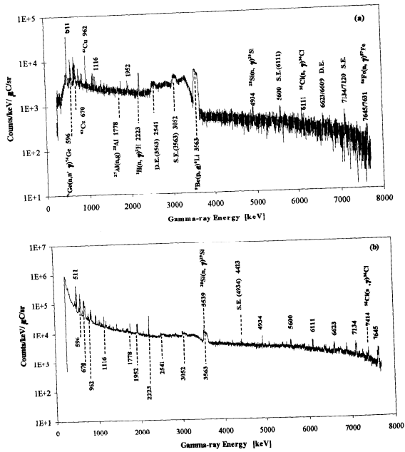
Figure 21. TOF-gated (a) and ungated (b) gamma-ray spectra at 40°, obtained in the bombardment of a thick Be target with 4.0 MeV protons. The major gamma-ray lines are identified in keV.
