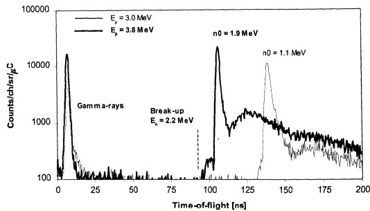
Figure 15. Time-of-flight spectra obtained in the bombardment of a 7.5 \mu\text{m} thick Be target with 3.0 MeV and 3.8 MeV protons. Flight path = 2 m, timing resolution \sim 2 ns. Ground state neutrons are labelled n0 and maximum energy of break-up neutrons is also marked ( E_n = 2.2 MeV for E_p = 3.8 MeV).
