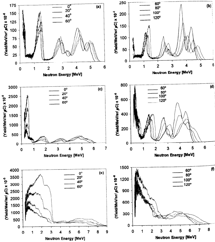
Figure 6. Neutron spectra at a range of laboratory angles of 0°–120° produced in bombardment of a thick Be target with deuterons of energy 0.9 MeV (a,b), 1.5 MeV (c,d), 4.0 MeV (e,f).
