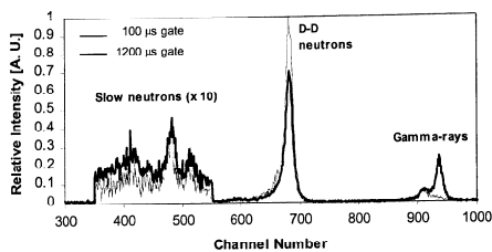
Figure 39. Gated TOF spectra obtained in the bombardment of the target charged with deuterium gas at 1 bar at room temperature, with 5 MeV deuteron beam. Gates of two different widths and delays were applied.
