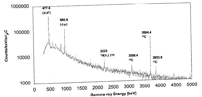
Figure 14. TOF-gated gamma-ray spectrum at 40° obtained in the bombardment of a thick Li target with 4.0 MeV deuterons. The major gamma-ray lines are identified in keV.
