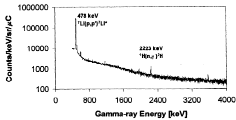
Figure 28. TOF-gated gamma-ray spectrum obtained in the bombardment of a thick natural lithium target with a 2.32 MeV proton beam.
