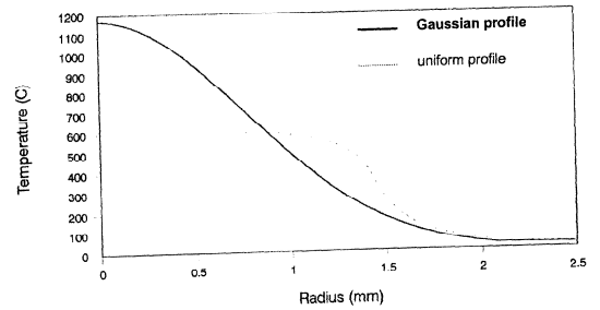
Figure 31. Calculated temperature profiles for Gaussian and uniform beam distribution of 4.5 MeV ions at 50 \mu\text{A} passing through 2.5 \mu\text{m} of Havar. Beam spot size was 3 mm in diameter, foil size was 5 mm in diameter.
