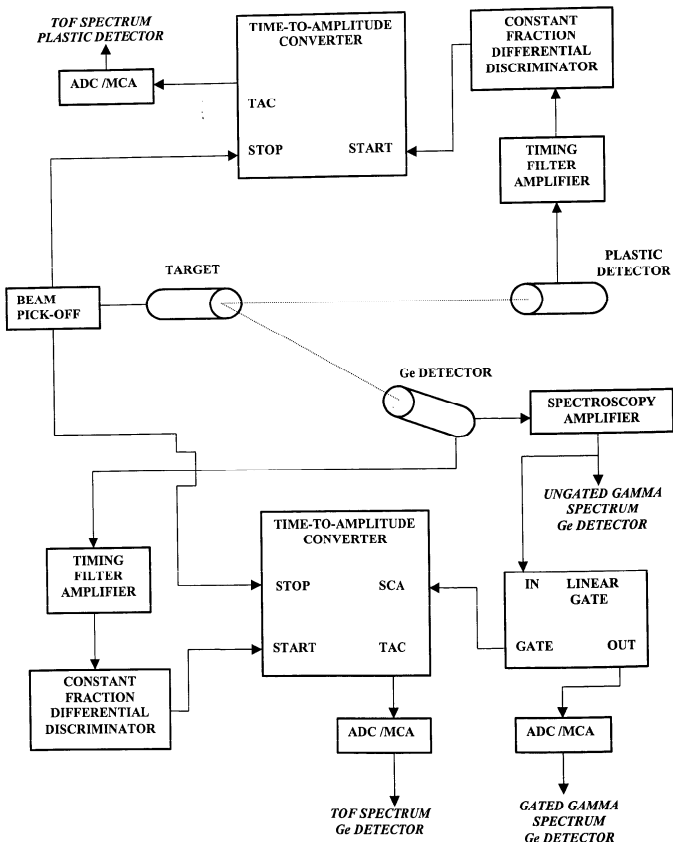
Figure 1. Block diagram of electronics set-up used in time-of-flight experiments.
