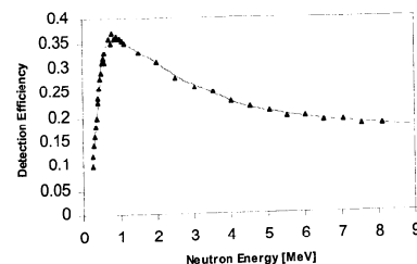
Figure 2. The experimental neutron detection efficiency for the plastic scintillator used in this work. The detector was biased at \sim 250 keV of proton recoil energy. Moving average 2-point best fit line is superimposed on a set of experimental data points.
