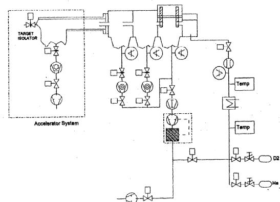
Figure 37. Schematic of the differentially pumped gas target vacuum system.
