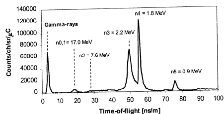
Figure 11. Time-of-flight spectrum obtained in bombardment of a thin Li target with a 4 MeV deuteron beam at 0^\circ . Neutron groups corresponding to different final states of the residual {}^8\text{Be} nucleus are indicated.
