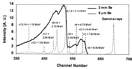
Figure 4. Time-of-flight spectra of the ^9\text{Be}(d,n)^{10}\text{B} reaction at incident deuteron energy of 4.0 MeV, at 0^\circ , obtained with targets of 2 mm and 5 \mu\text{m} thickness. Neutron groups corresponding to different final states of the residual ^{10}\text{B} nucleus are indicated.
