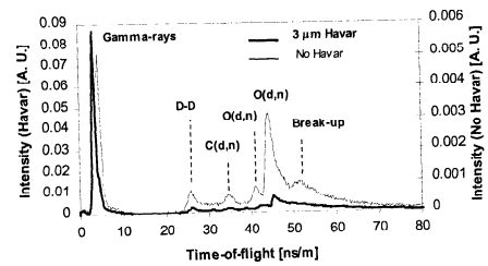
Figure 33. TOF spectra obtained at 0^\circ in the bombardment of an evacuated reference cell with and without Havar entrance foil present. Spectra normalized as in Figure 32.
