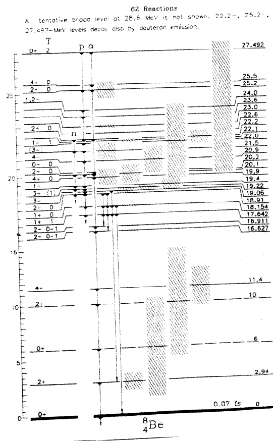
Figure 12. Nuclear level structure of {}^8\text{Be} [80].
