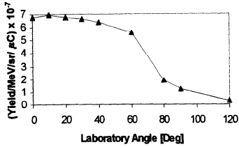
Figure 26. The total neutron yield (for E_n > 0.25 MeV) in the bombardment of a thick Li target with 2.32 MeV proton beam.
