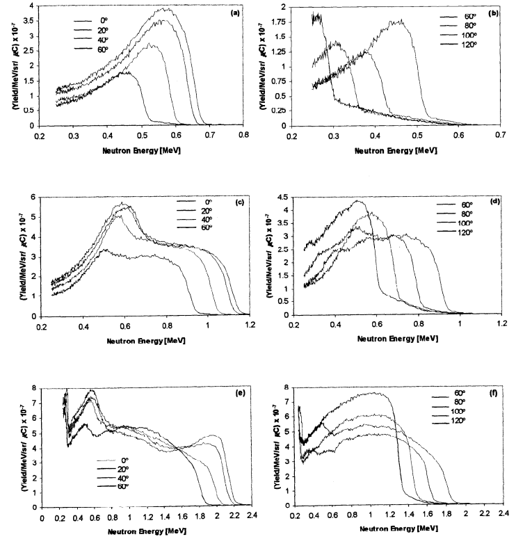
Figure 19. Neutron spectra in the laboratory angle range of 0^\circ - 120^\circ obtained in the bombardment of a thick Be target with 2.57 (a,b), 3.0 (c,d) and 4.0 MeV (e,f) protons.
