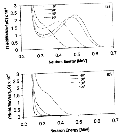
Figure 24. Neutron energy spectra obtained in the bombardment of a thick natural Li target with protons of energy of 2.32 MeV in a range of laboratory angles of 0^\circ - 120^\circ .
