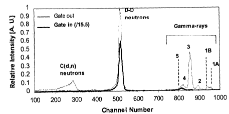
Figure 38. Gated and ungated TOF spectra obtained during the bombardment of the target charged with 1 bar of deuterium gas at room temperature, with 2.1 MeV deuteron beam. Flight distance = 2 m, timing calibration = 0.186 ns ch^{-1} .
