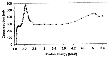
Figure 25. The cross-section for the {}^7\text{Li}(p,n){}^7\text{Be} reaction [88].
