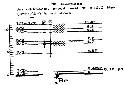
Figure 23. Nuclear level structure of {}^7\text{Li} [80].
