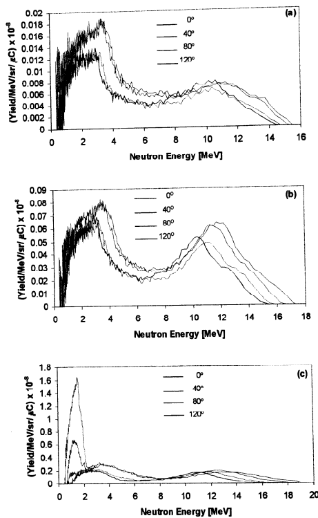
Figure 13. Neutron spectra obtained in bombardment of thick Li target with 0.9 (a), 1.5 (b) and 4.0 (c) MeV deuterons, for various laboratory angles.
