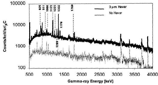
Figure 34. TOF-gated gamma-ray spectra at 0^\circ obtained in the bombardment of evacuated reference gas cell, with and without Havar entrance foil present, with a 5 MeV deuteron beam.
