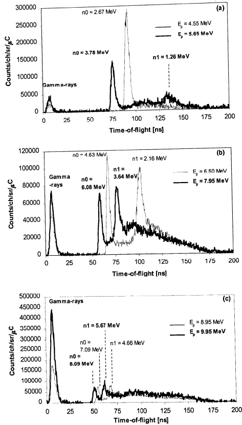
Figure 16. Time-of-flight spectra obtained in the bombardment of a 15 \mu\text{m} thick Be target with protons in the energy range of 4.55 – 9.95 MeV (a – E_p = 4.55 and 5.65 MeV, b – E_p = 6.50 and 7.95 MeV and c – E_p = 8.95 and 9.95 MeV). Flight path = 2 m, timing resolution \sim 3 ns. Ground state and the first excited state neutron groups are indicated by n0 and n1 , respectively.
