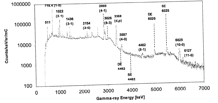
Figure 10. Thick target Be(d,n) reaction TOF-gated gamma-ray spectrum at a deuteron energy of 4.0 MeV obtained at a laboratory angle of 80^\circ . The numbers indicate the energies of the gamma-ray lines in keV, and transitions corresponding to ^{10}\text{B} excitation levels are given in brackets; SE and DE stand for single escape and double escape, respectively and (d,p) indicates the gamma-ray lines resulting from the ^9\text{Be}(d,p)^{10}\text{B} reaction.
