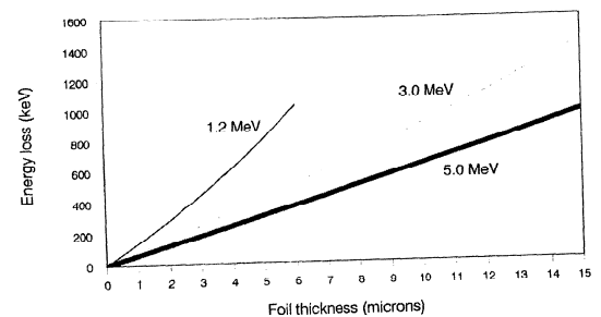
Figure 29. Energy loss of deuteron ions traversing Havar foil as evaluated using TRIM [84].
