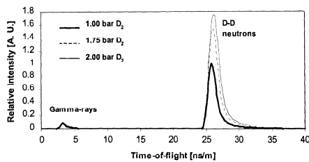
Figure 32. TOF spectra at 0^\circ obtained from the bombardment of the reference gas cell (10 cm long, 3 \mu\text{m} Havar foil, deuterium at room temperature) at different static pressures of deuterium gas, with a 5 MeV deuteron beam. The maximum value in the neutron peak in the spectrum for 1 bar deuterium pressure was normalized to unity.
