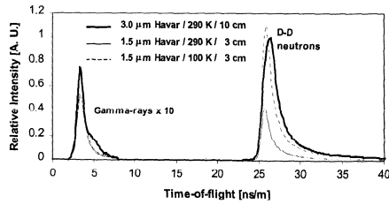
Figure 35. TOF spectra at 0^\circ obtained in the bombardment of the reference cell and newly developed target cell (3 cm long, 1.5 \mu\text{m} Havar foil), filled with deuterium gas at room temperature and cooled-down to 100 K, with a 5 MeV deuteron beam. Spectra normalized as in Figure 32.
