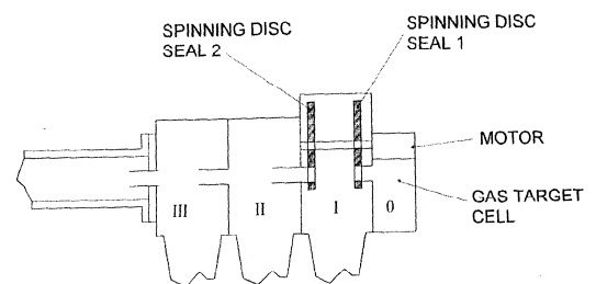
Figure 36. Schematic of the differentially pumped gas target arrangement.
