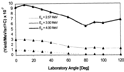
Figure 20. Neutron yield ( E_n \geq 0.25 MeV) for the thick target \text{Be}(p,n) reaction for E_p = 2.57 MeV, 3.0 MeV and 4.0 MeV.
