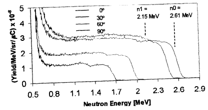
Figure 27. Neutron energy spectra obtained in the bombardment of a thick natural Li target with 4.28 MeV protons in the laboratory angle range of 0^\circ - 90^\circ . The onset energy of the ground state (n0) and the first excited state (n1) neutrons at 0^\circ are indicated in MeV.
