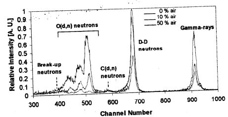
Figure 41. Gated TOF spectra obtained in the bombardment of the target charged with deuterium gas contaminated with air, with a 5 MeV deuteron beam.
