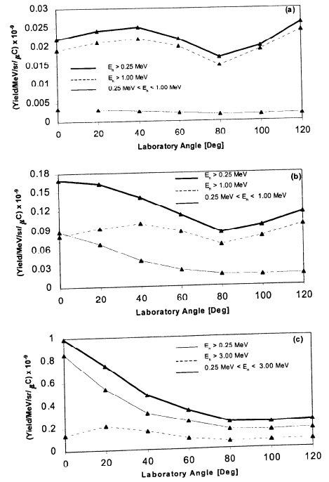
Figure 7. Neutron yield angular distributions for thick target Be(d,n) reaction at deuteron energy of 0.9 MeV (a), 1.5 MeV (b) and 4.0 MeV (c).
