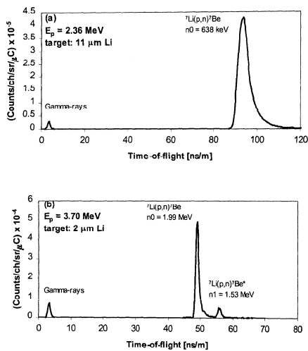
Figure 22. TOF spectra obtained at 0^\circ in the bombardment of a thin natural lithium targets with 2.36 MeV (a) and 3.70 MeV (b) protons.
