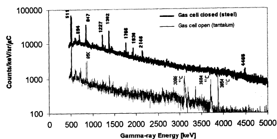
Figure 42. TOF-gated gamma-ray spectra obtained in the bombardment of the evacuated target with stationary disc seal, with a 5 MeV deuteron beam. Positions of the disc seal correspond to the full opening of the gas cell (the beam dumped on Ta end-stop) and to the fully obscured gas cell by the disc seal (the beam dumped on steel).
