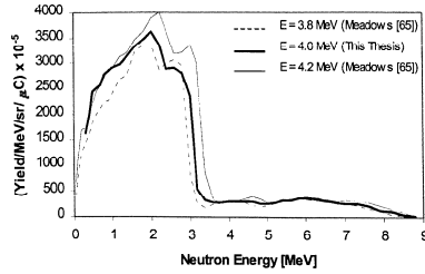
Figure 9. Comparison of spectral shapes between Meadows [65] and the present study.
