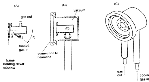
Figure 30. Schematic of the gas cell system.
