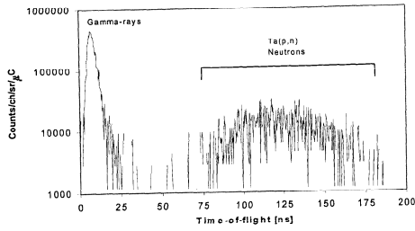
Figure 18. TOF spectrum obtained in the bombardment of thick Ta target with 9.95 MeV protons. Flight path = 2 m, timing resolution ~ 3 ns
