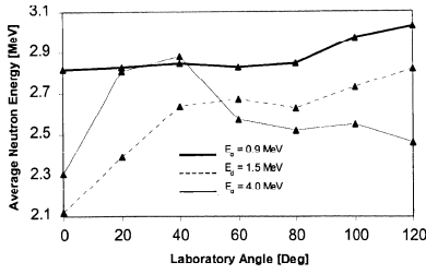
Figure 8. Average neutron energies for thick target Be(d,n) reaction spectra at deuteron energies of 0.9 MeV, 1.5 MeV and 4.0 MeV.
