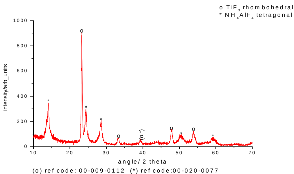
Figure 4. 9: XRD Analysis of product after decomposing precursor at 400°C in UHP Argon
