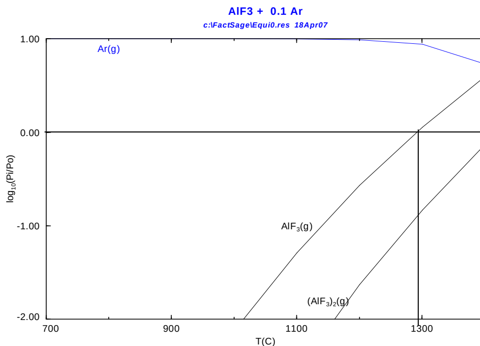
Figure 5. 17: Vapour pressure over \text{AlF}_3 as a function of temperature
