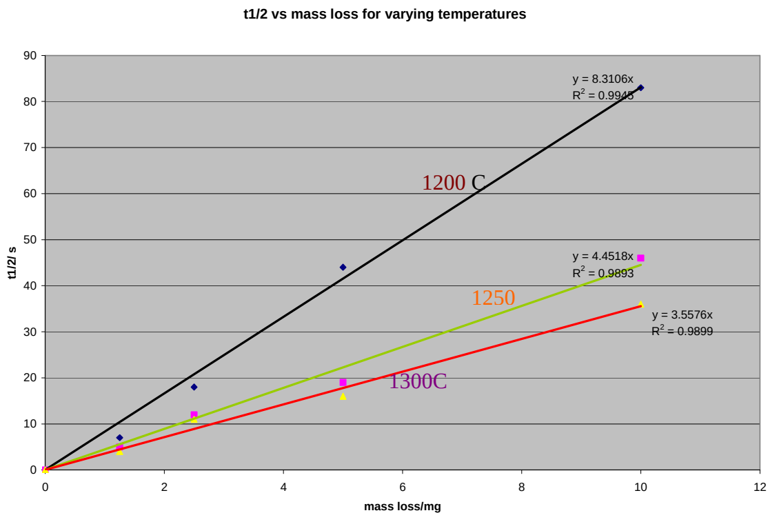
Figure 5. 15: t_{1/2} vs. mass loss for varying temperatures
