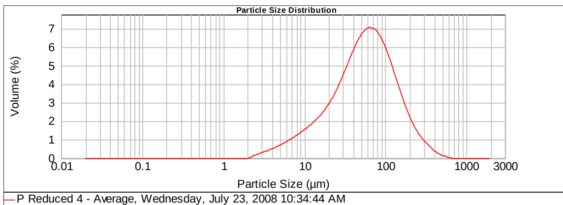
Figure 4. 2: Particle size distribution of the final titanium product
