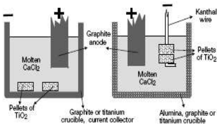
Figure 2. 9: Schematic of the FFC electrolytic cell
