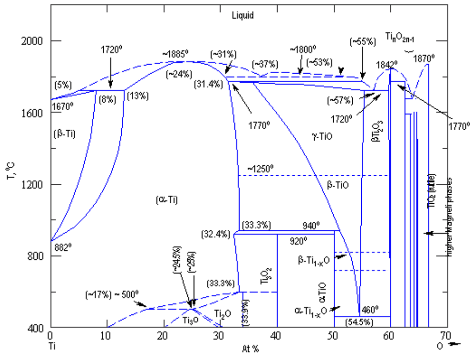
Figure 2. 3: The Ti-O phase diagram [41]
