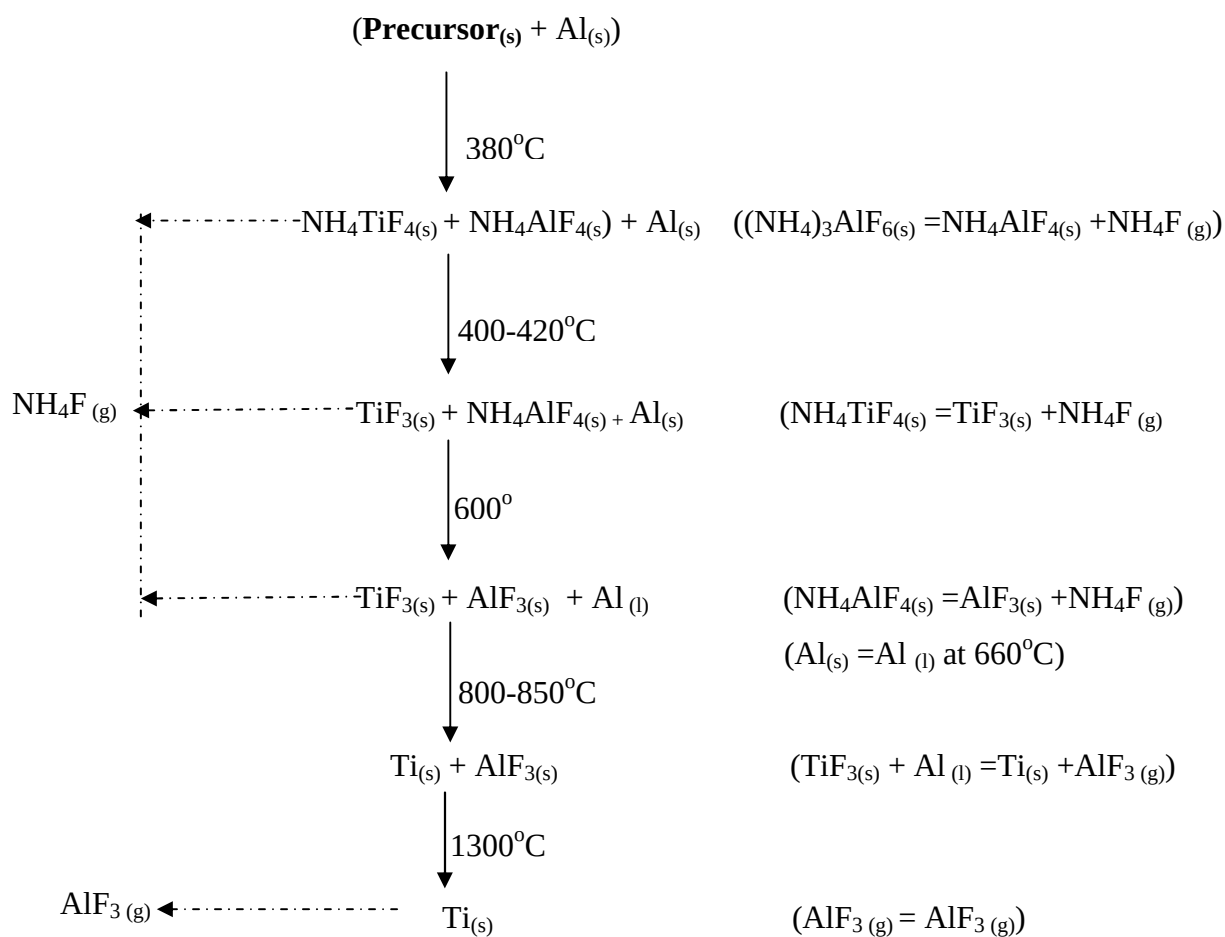
Figure 5. 19: Flow sheet of the process with the precursor premixed with Aluminium
