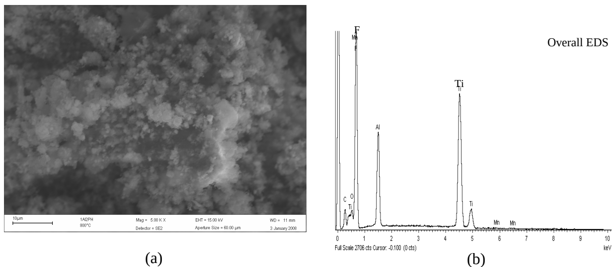
Figure 4. 12: SEM analysis of product after decomposing precursor at 800°C and soaking for 2 hours (a) SEM (b) Overall EDX spectrum
