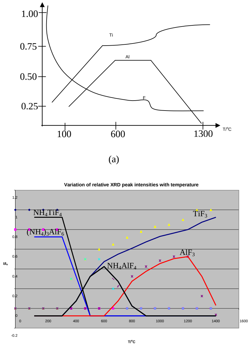
Figure 5. 6 (a) Variation of EDS peak intensities (b) Variation of XRD peak intensities with Temperature
