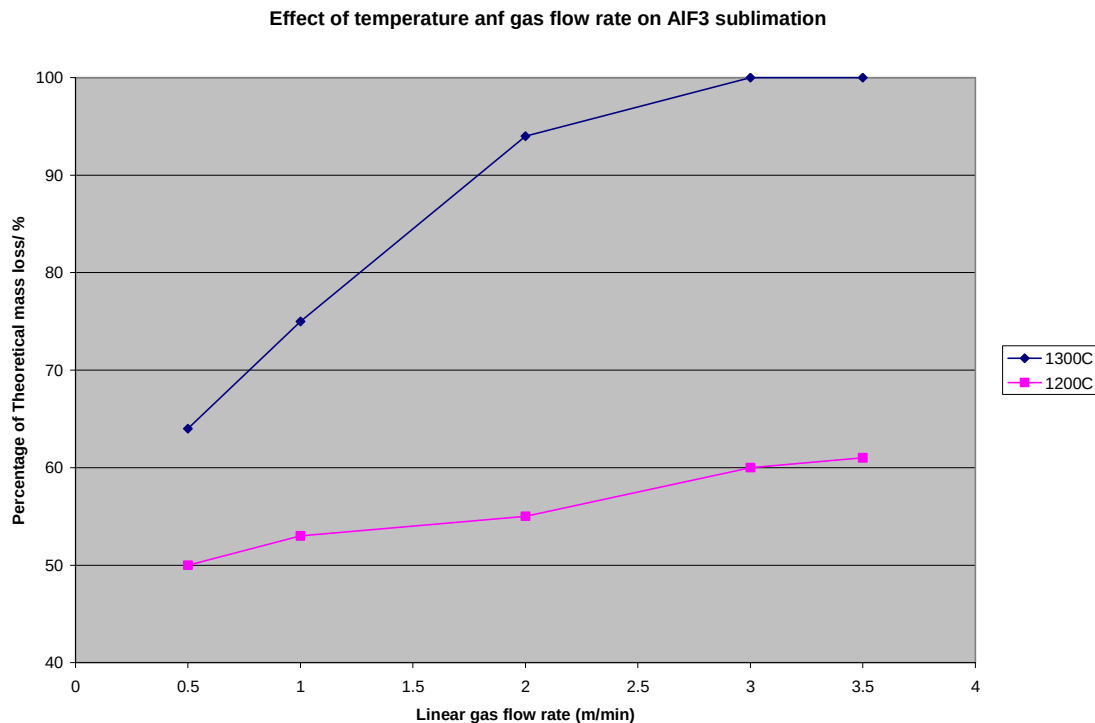
Figure 5.10 (b): Effect of temperature and gas flow rates on the sublimation of \text{AlF}_3
