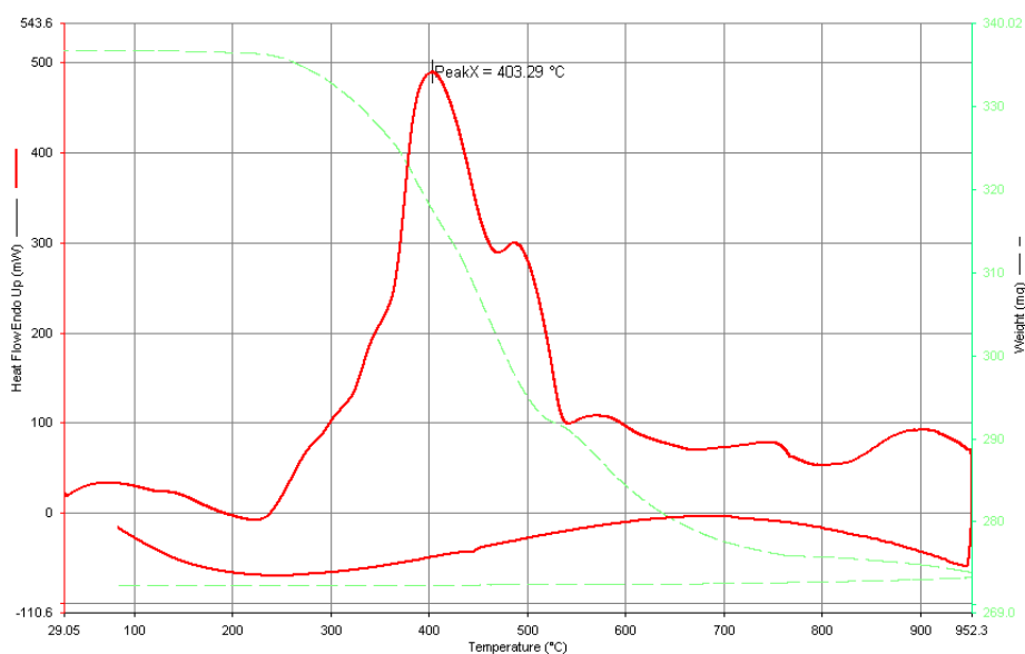
Figure 4. 25: TGA-DSC trace of precursor in UHP Argon
