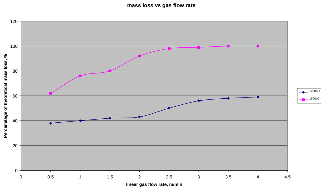
Figure 5. 7: Variation of mass loss with gas flow rate at 1300°C after soaking for 2 hrs
