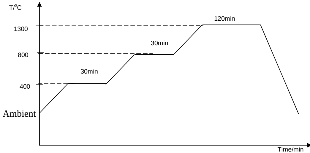
Figure 3. 2: Heat treatment cycle during precursor reduction trials
