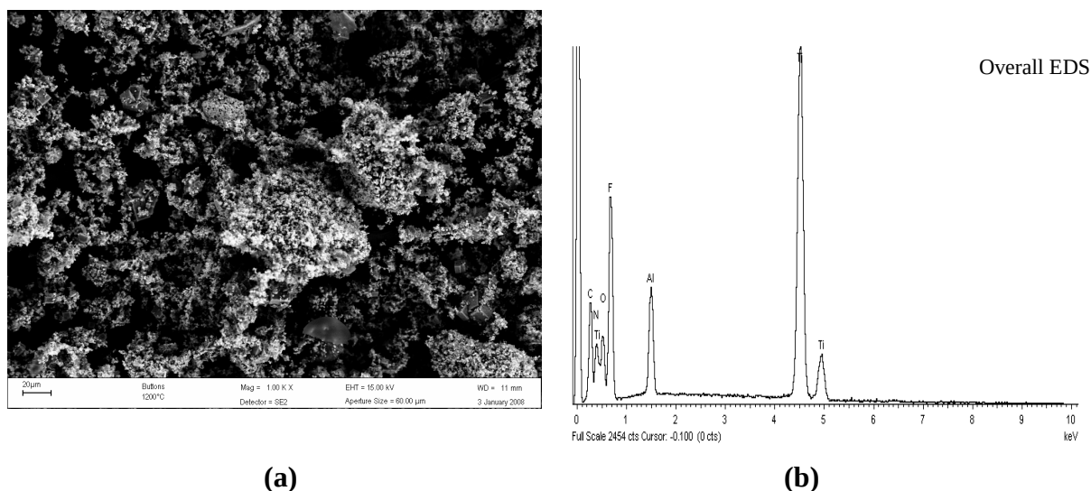
Figure 4. 16: SEM analysis of product after decomposing precursor at 1200°C for 2 hours
