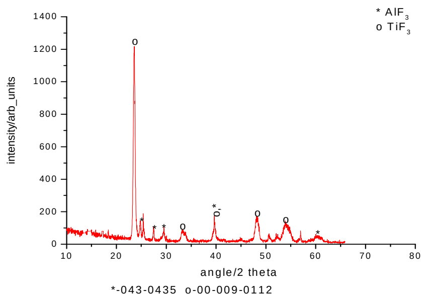
Figure 4. 19: XRD Analysis of product after decomposing precursor at 1300°C in UHP Ar
