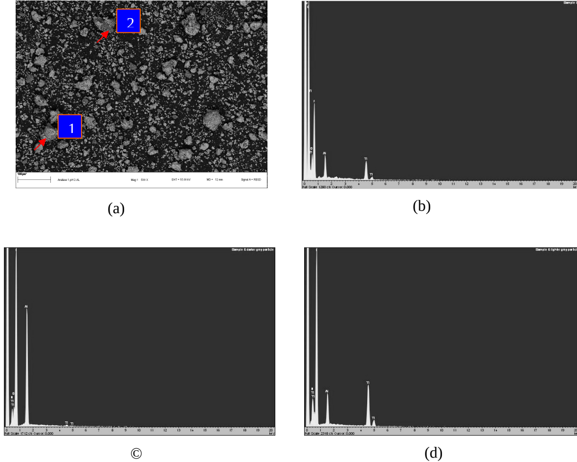
Figure 4. 3: SEM analysis of the precursor (a) SEM micrograph (b) Overall EDS spectrum (c) EDS for spot 1 (d) EDS for spot 2.
