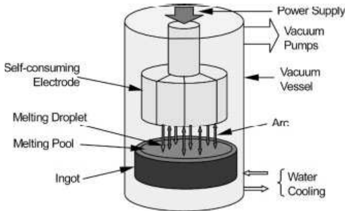
Figure 2. 7: Schematic of a vacuum arc melter (after H.Sibum [5] .)
