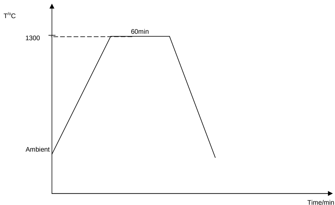
Figure 3. 3: Heat treatment cycle during CVD trials
