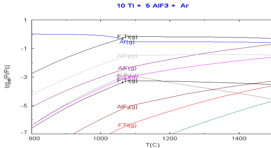
Figure 5. 13: Variation of vapour pressure of Ti fluorides and Aluminium fluorides with Temperature (computer generated using an SGTE database)
