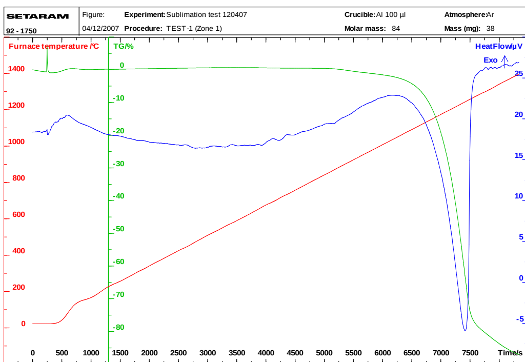
Figure 5. 14: TGA-DTA trace of pure \text{AlF}_3
