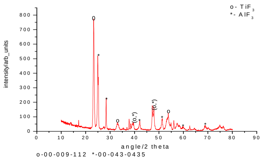
Figure 4. 15: XRD Analysis of product after decomposing precursor at 1000°C for 2 hours
