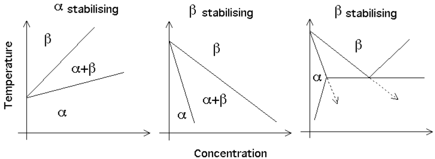
Figure 2. 6: Effect of alloying elements on the phase fields of the constitutional diagram [42]
