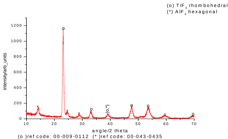
Figure 4. 13: XRD of product after decomposing precursor at 800°C and soaking for 2 hours
