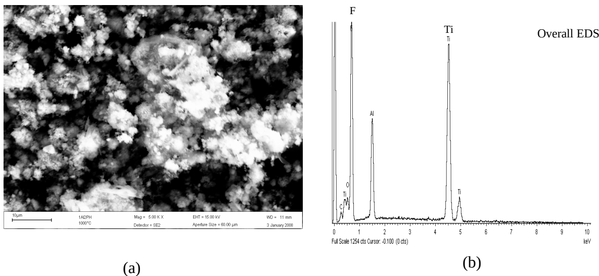
Figure 4. 14: SEM analysis of product after decomposing precursor at 1000°C for 2 hours (a) SEM (b) Overall EDS spectrum
