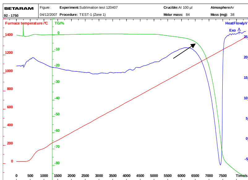
Figure 4. 26: TGA/DTA trace of AlF 3
