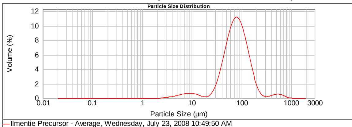
Figure 4. 1: Particle size distribution of raw precursor
