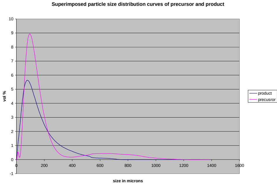
Figure 5. 1: Superimposed particle size distributions of the precursor and Ti product
