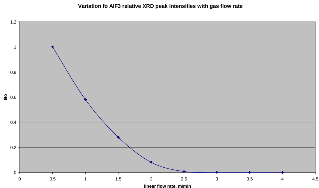
Figure 5. 8: Variation of \text{AlF}_3 XRD intensities normalised to its value at 0.5m/min with gas flow rate at 1300°C
