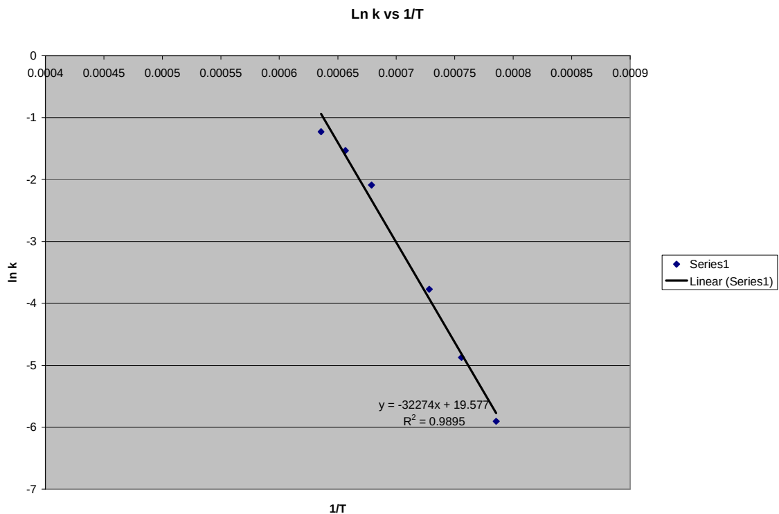
Figure 5. 16: A plot of natural log of rate constants versus the inverse absolute T/K
