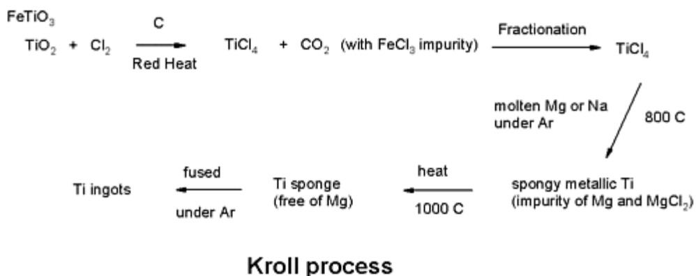
Figure 2. 2: Flowchart for titanium production by the Kroll or Hunter process [44] .
