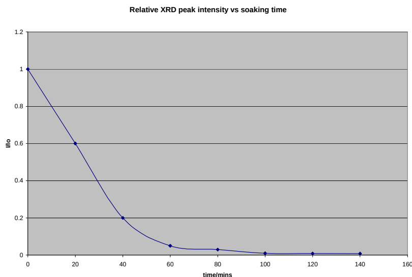
Figure 5. 10 (a): Variation of \text{AlF}_3 relative peak intensities with soaking time at 1300°C and 2.6m/min gas linear flow rate.
