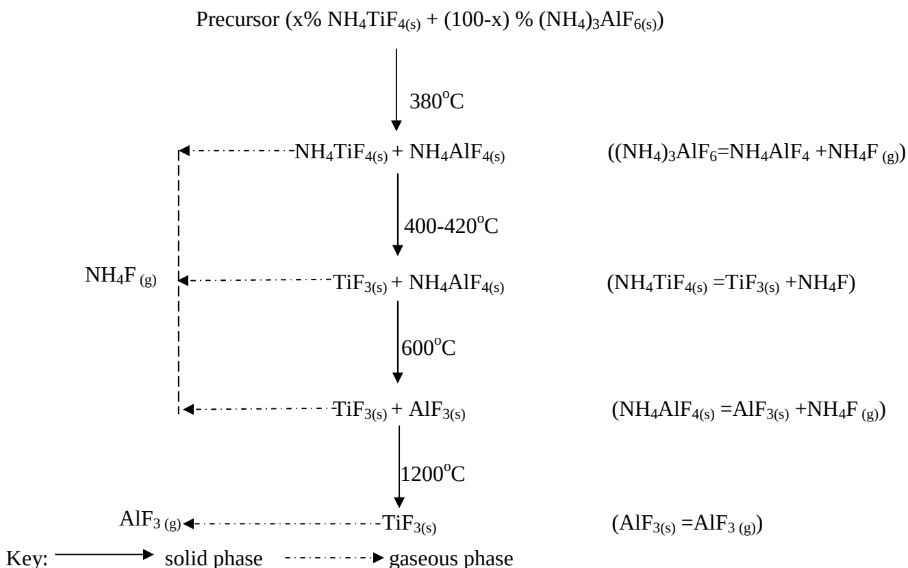
Figure 5. 188: Flow sheet for the pyrolysis of the titanium precursor
