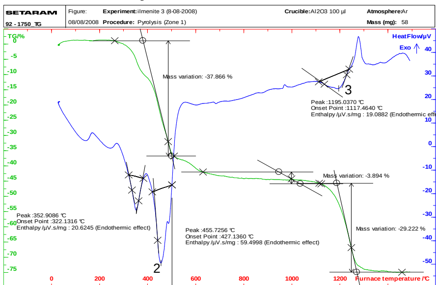
Figure 4. 5: TGA/DTA trace of precursor in UHP argon
