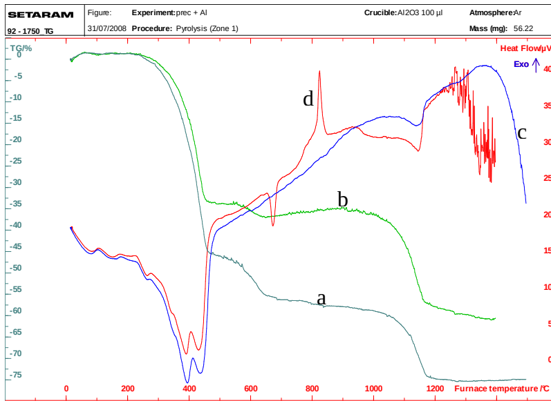
Figure 5. 11: Superimposed TG/DTA traces of precursor and premixed with Al
