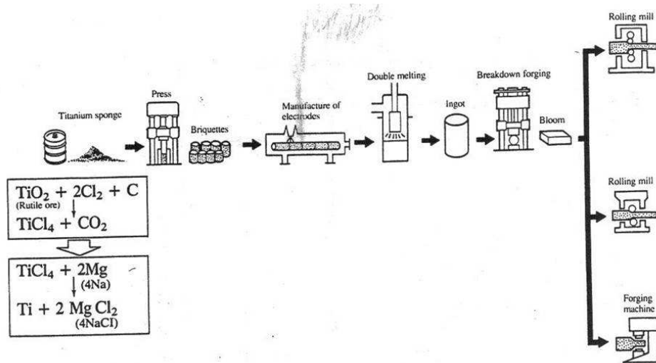
Figure 2. 8: Process flow chart for titanium sponge [40]
