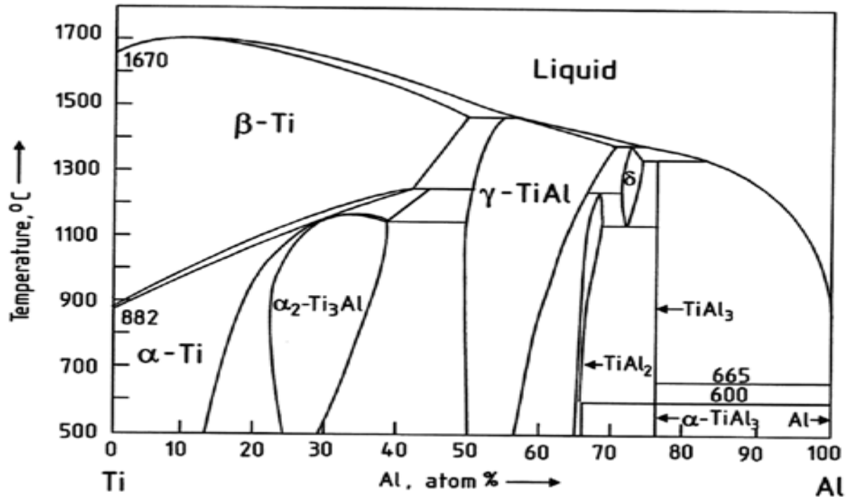
Figure 2. 4: Phase diagram of the Ti-Al system [41] .
