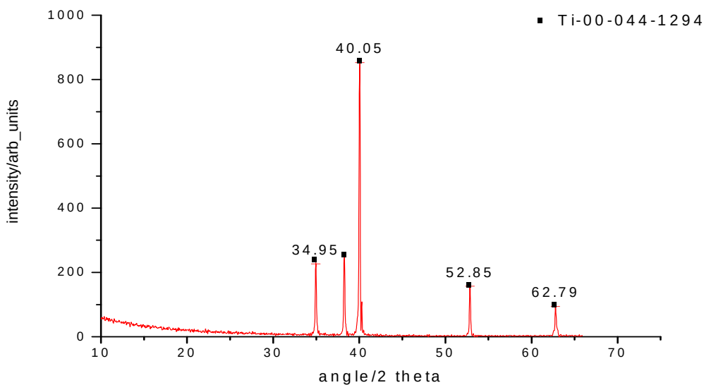
Figure 4. 23: XRD pattern of product after reduction and soaking at 1300°C for 2 hours
