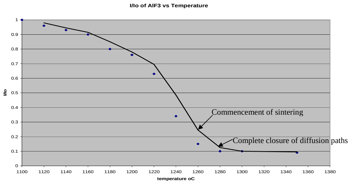
Figure 5.12c: Variation of \text{AlF}_3 XRD relative peak intensities with soaking temperature
