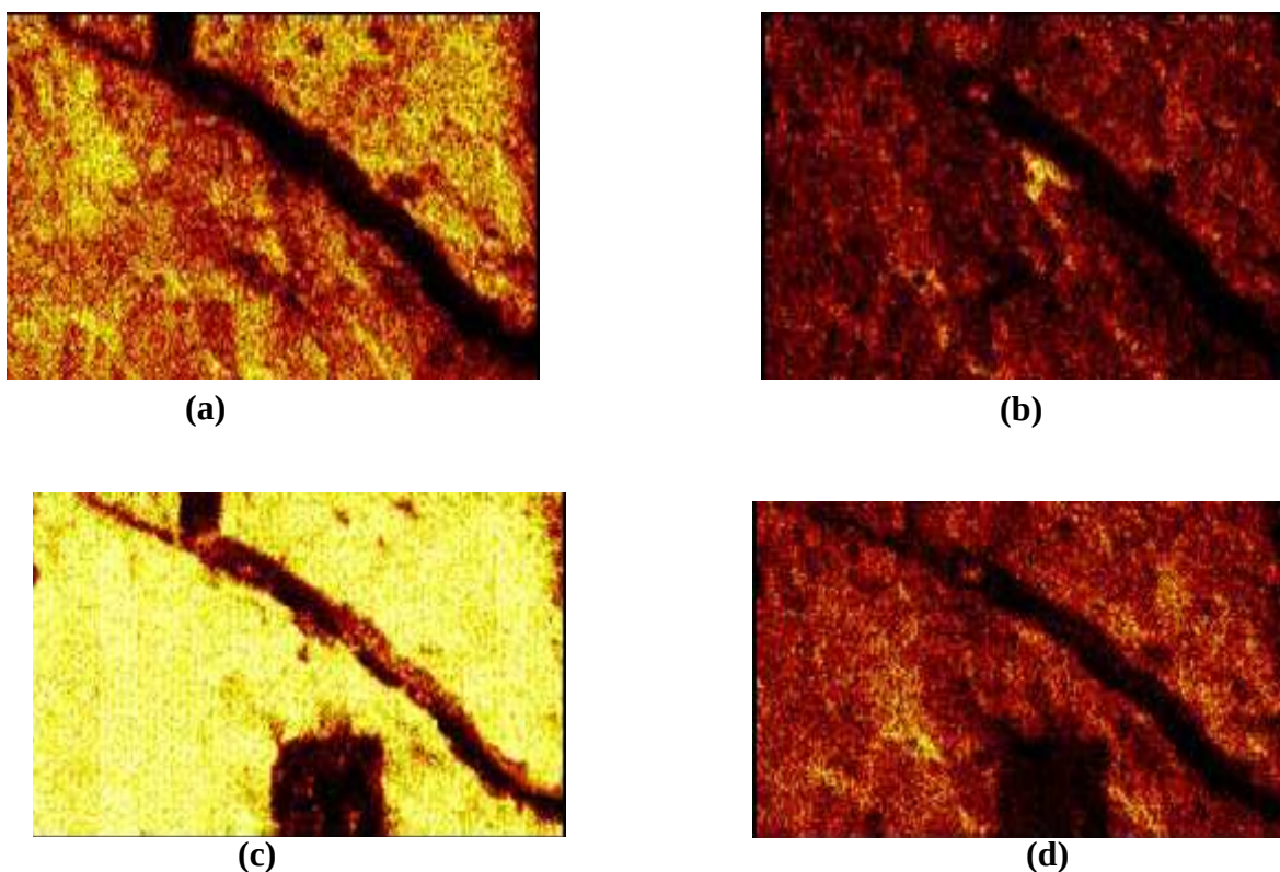
Figure 4. 24: ToF-SIMS images of passivated product (a) Al ion image before sputtering (b) Ti ion Image before sputtering (c) Al ion image after sputtering (d) Ti ion image after sputtering
