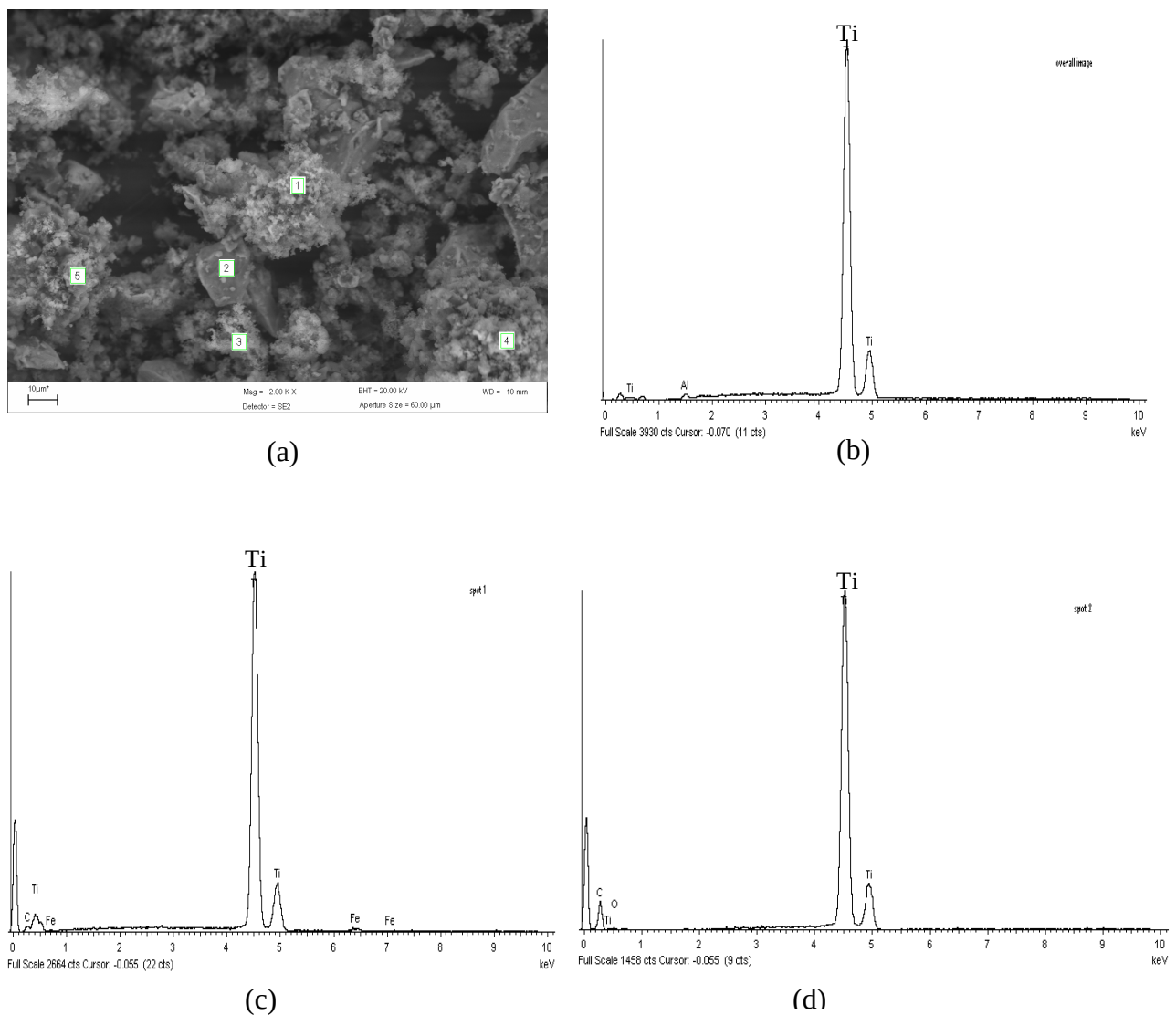
Figure 4. 22: SEM analysis of product after reduction of precursor with aluminium at 1300°C for 2 hours (a) SEM micrograph (b) Overall EDX spectrum (c) EDS spot 1 and (d) EDS spot 2
