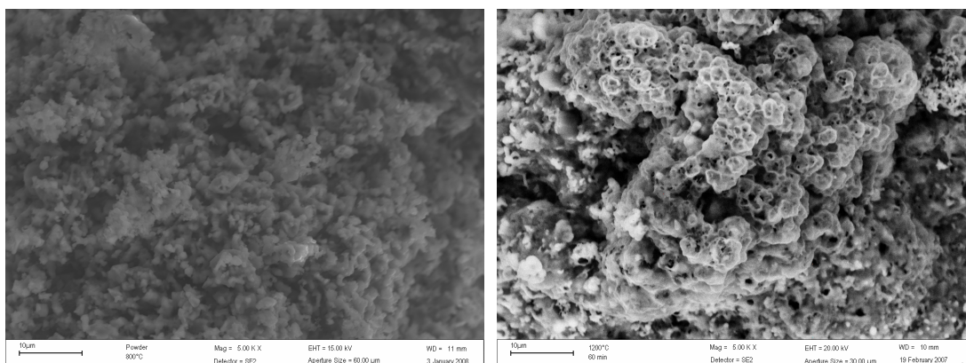
Figure 5. 4: SEM Analysis (a) 800°C (b) 1200°C after sublimation of \text{AlF}_3
