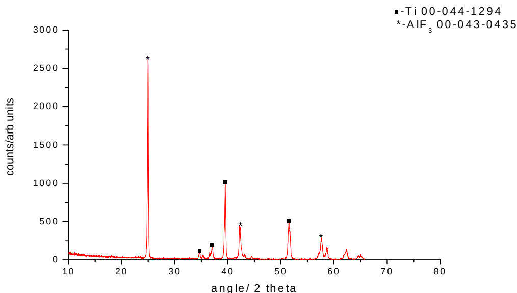
Figure 4. 21: XRD pattern after reduction of precursor with aluminium at 800°C
