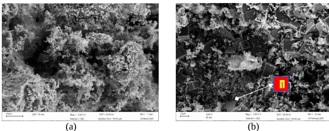
Figure 5. 9: SEM micrographs of product (a) 1.3m/min 10 minutes (b) 1.3 m/min 60 minutes at 1300°C
