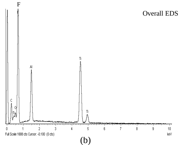
Figure 4. 10: SEM analysis of product after decomposing precursor at 600°C (a) SEM (b) overall EDS
