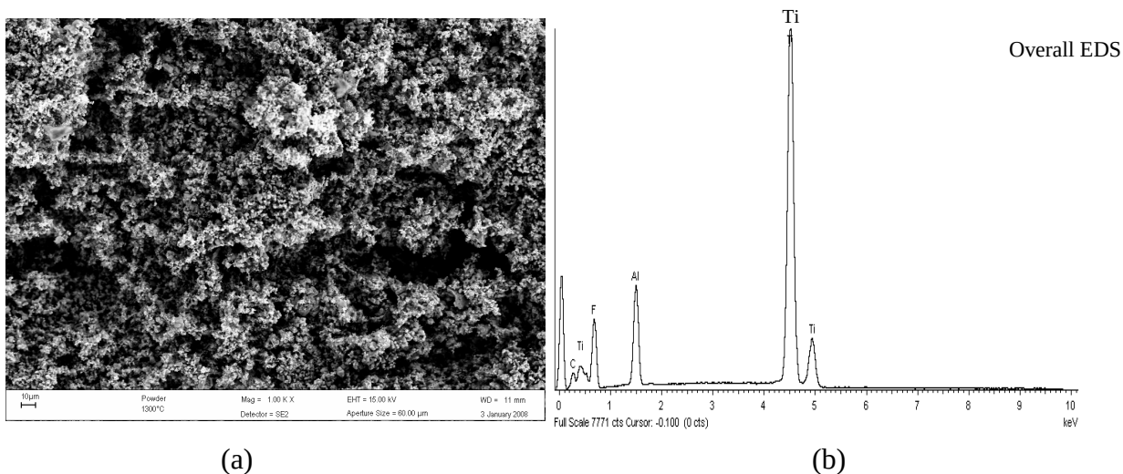
Figure 4. 18: SEM analysis of product after decomposing precursor at 1300°C (a) SEM (b) Overall EDX spectrum
