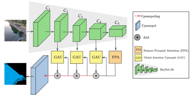
FIGURE 7. Architecture of PAN (ResNet50), adopted from [33].
