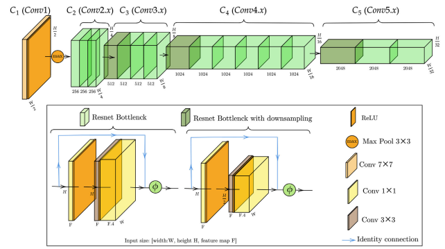
FIGURE 2. The ResNet50 backbone adopted from the PyTorch implementation and [38].
