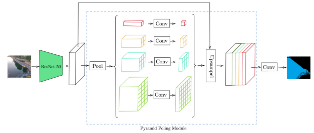
FIGURE 6. Architecture of PSPNet (ResNet50), adopted from [32].
