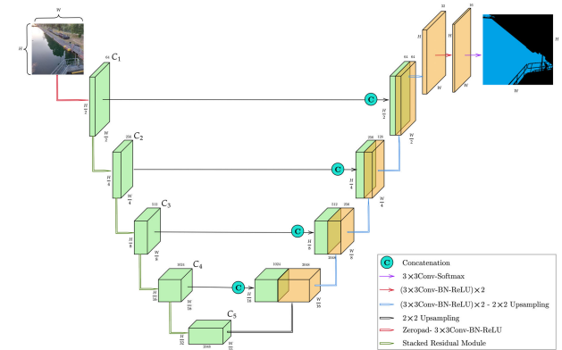
FIGURE 3. Architecture of U-Net(ResNet50), adopted from [39].
