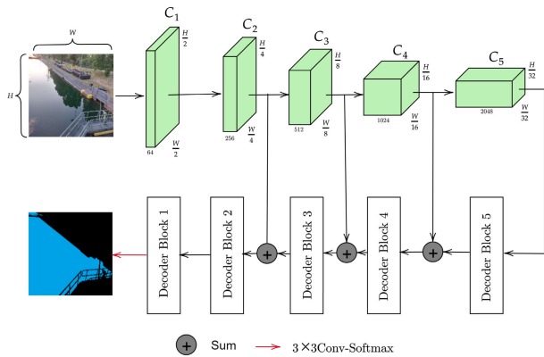
FIGURE 5. Architecture of LinkNet (ResNet50), adopted from [34].
