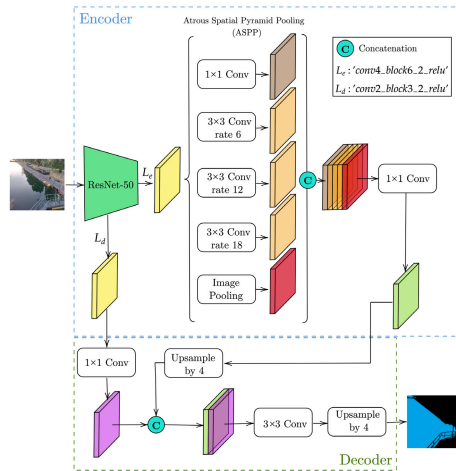
FIGURE 4. Architecture of DeepLabV3+ (ResNet50), adopted from [29].
