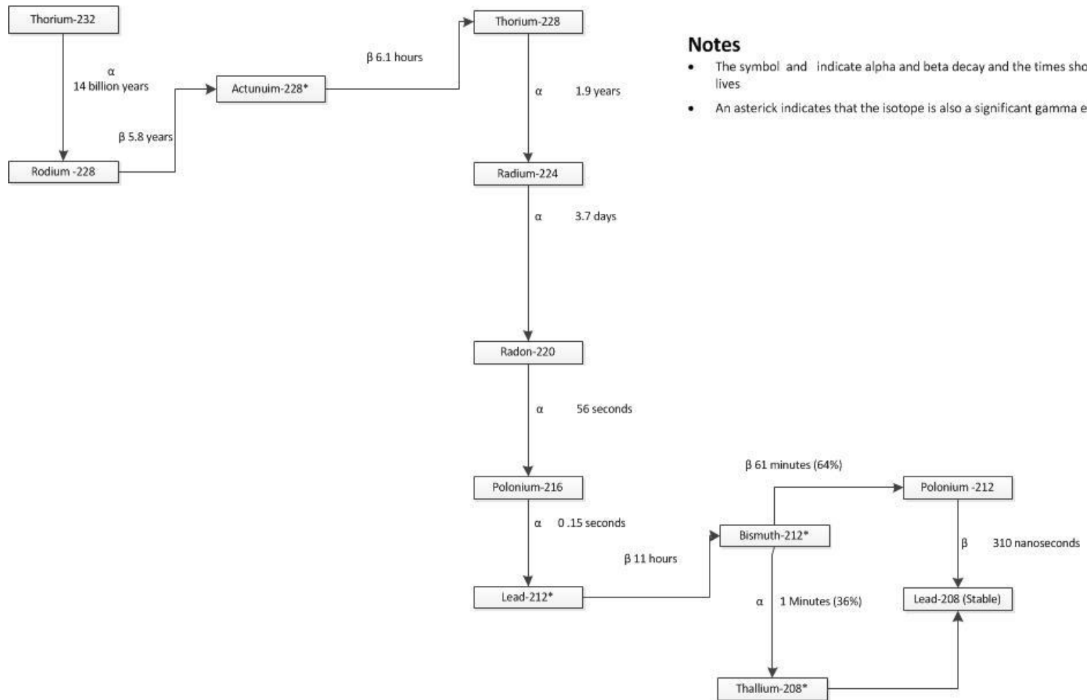
Figure 2.6: Natural decay series of Thorium-232 showing the modes of decay ( \alpha = alpha; \beta =beta) and the half-lives of the daughter nuclides (Coles et al. , 1978).
