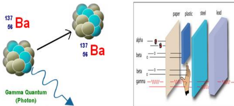
Figure 2.3: The mechanism of \gamma radiation, the matter penetration ability by \alpha , \beta and \gamma radiation.
