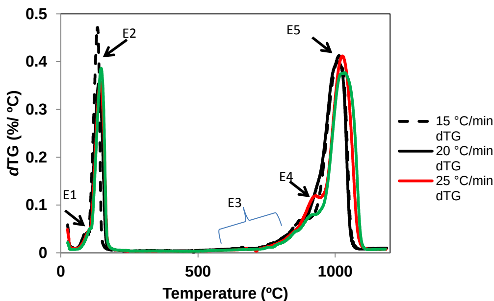
Figure 5.14: First derivatives of the thermographs of phosphogypsum + carbonaceous material (1:3 molar ratio)
