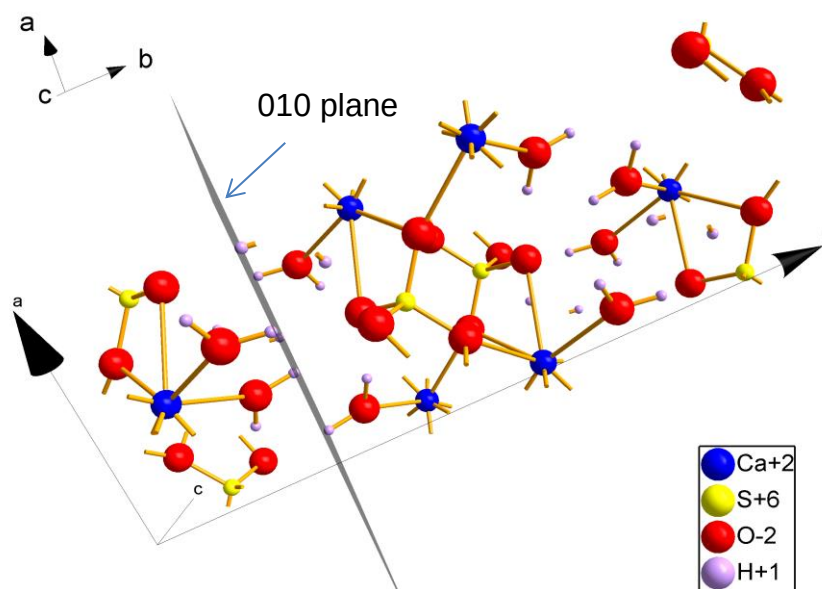
Figure 5.3: Ball and stick model of Gypsum showing the water layer in the 010 plane
