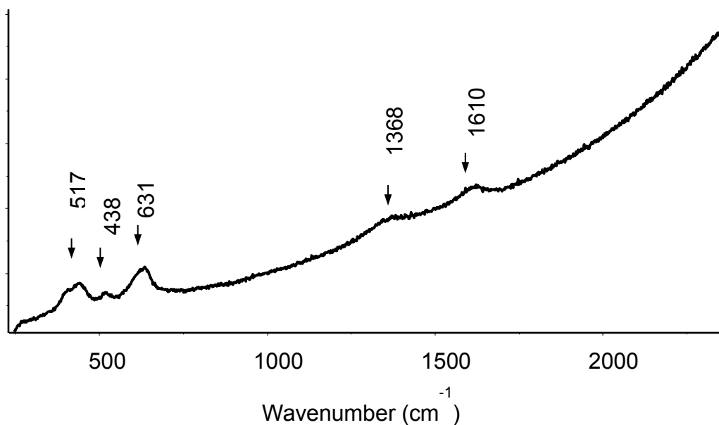
Figure 5.13: Room temperature Raman spectrum of graphite heated under continuous N 2 flow to 1080 °C
