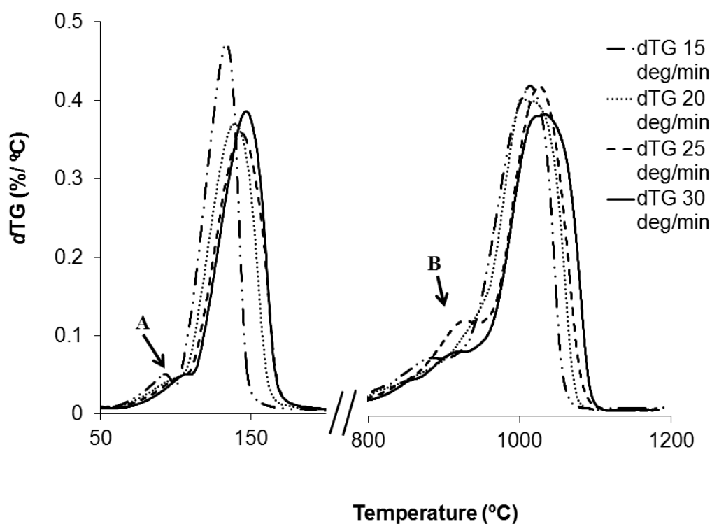
Figure 5.8: First derivative of the thermographs of phosphogypsum reduction with graphite at heating rates 15, 20, 25 and 30 °C/min; A indicates the dehydration of gypsum to hemihydrate and B indicates the formation of an intermediate compound
