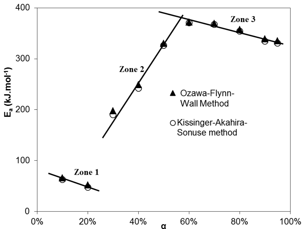
Figure 5.11: Activation energies calculated according to the OFW and KAS methods
