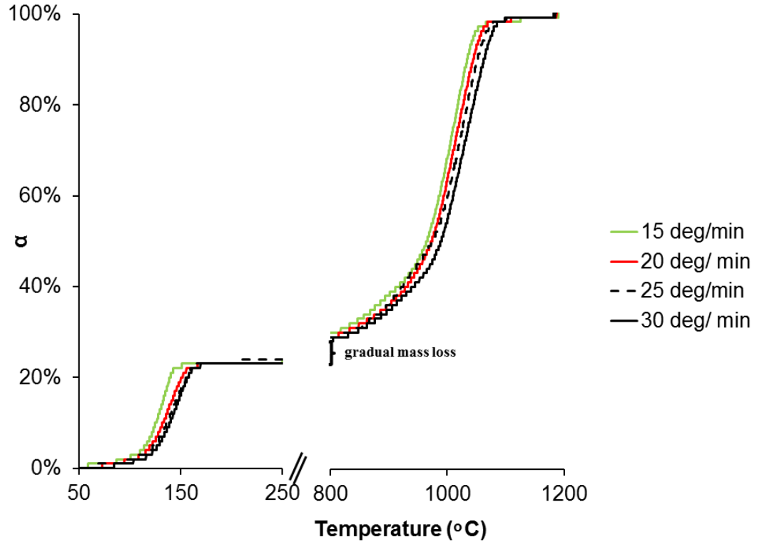
Figure 5.7: Normalised mass loss for the reaction between phosphogypsum and graphite
