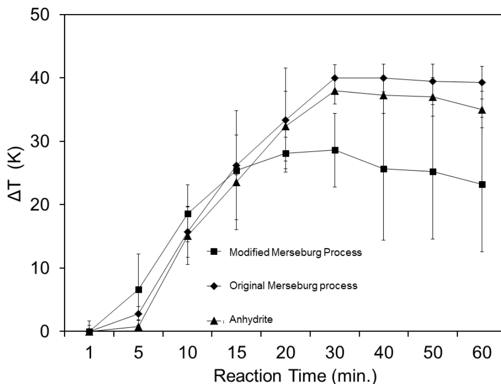
Figure 4.2: Temperature profile of ammonium carbonate formation in the original Merseburg; modified Merseburg and modified Merseburg and gypsum replaced with anhydrite
