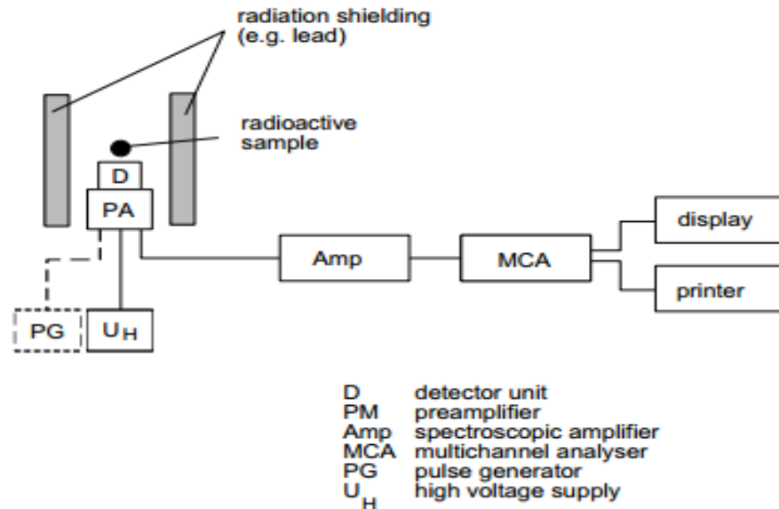
Figure 2.8: Schematic diagram of a gamma spectrometer ( https://tu-dresden.de )
