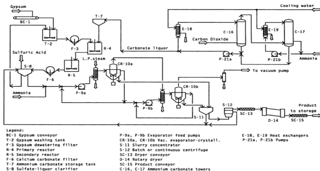
Figure 1.3: Gypsum - Ammonium Carbonate (Merseburg) process (reproduced from Alienov, 1998)
