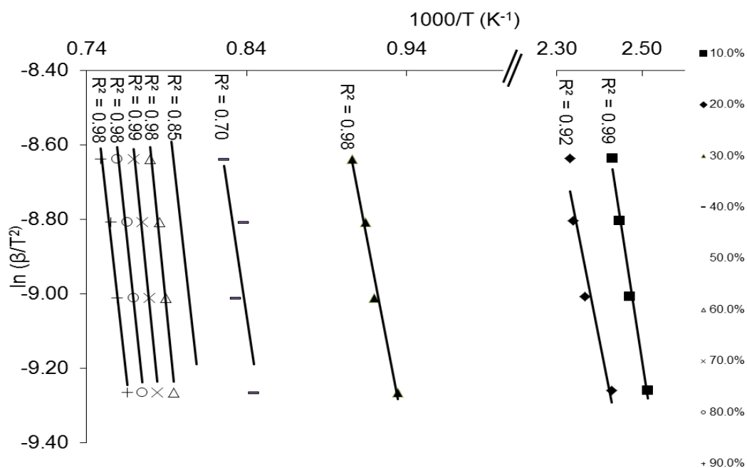
Figure 5.10: Plot according to Kissinger-Akahira-Sunose Method (KAS)
