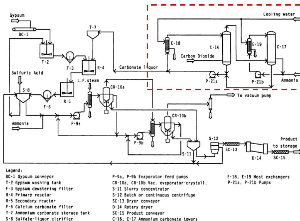
Figure 4.1: PFD of the Merseburg process with modification/omission highlighted in red
