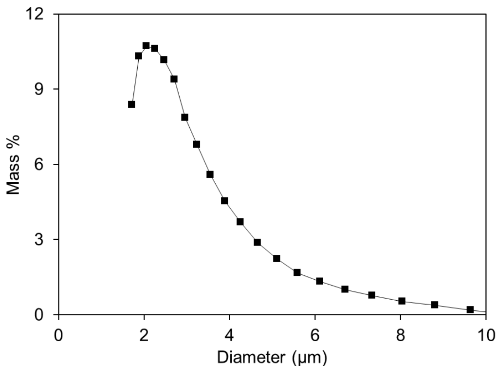
Figure 4.4: PSD of the Merseburg PCC
