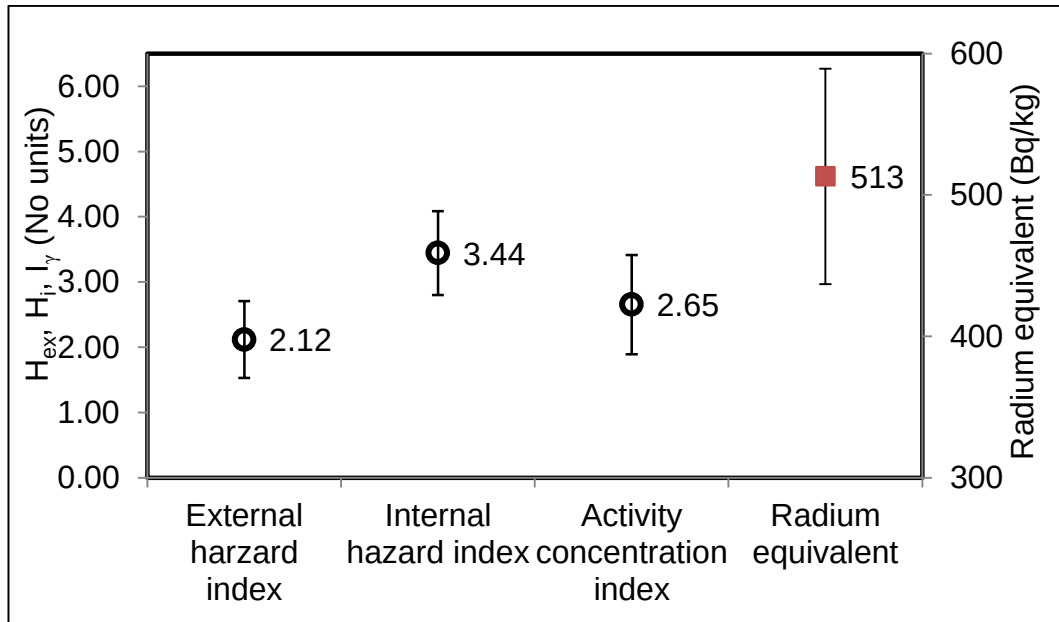
Figure 3.1: The calculated H_{ex} , H_{in} , I_\gamma and Ra_{eq} in the LSA phosphogypsum- error lines indicate the standard deviation
