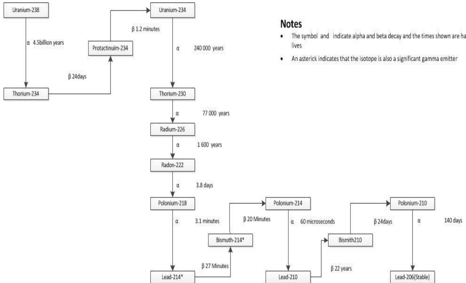
Figure 2.4: Natural decay series of Uranium-238 showing the modes of decay ( \alpha = alpha; \beta =beta) and the half-lives of the daughter nuclides (Coles et al. , 1978)
