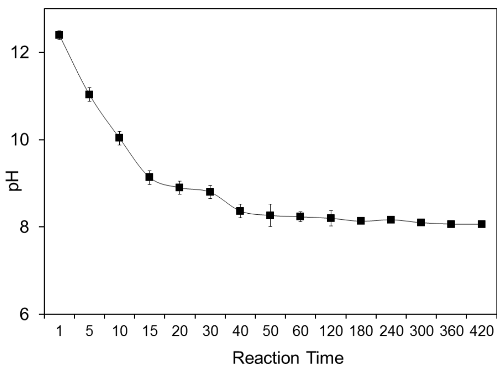
Figure 4.3: Average pH during modified Merseburg reaction
