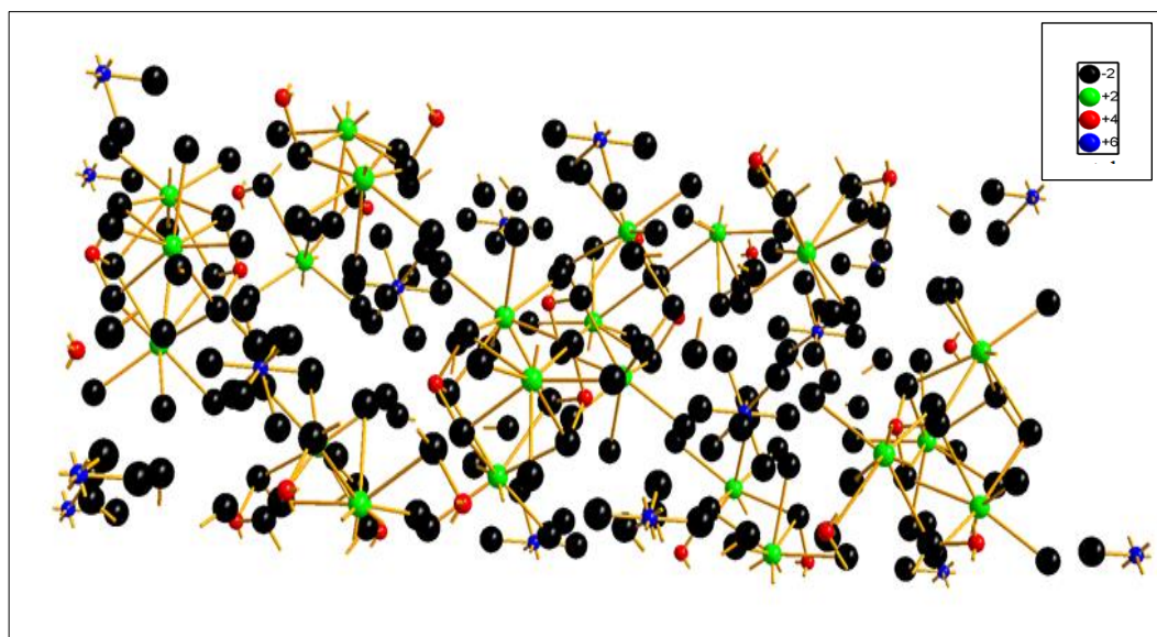
Figure 5.17: Wire or sticks model of Orschallite ( \text{Ca}_3[\text{SO}_4][\text{SO}_3]_2 \cdot 12\text{H}_2\text{O} ) from Diamond crystal visualisation software [black - \text{O}^{2-} ; green - \text{Ca}^{2+} ; red - \text{S}^{4+} ; blue - \text{S}^{6+} ]
