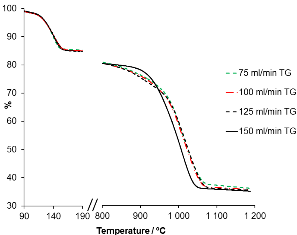
Figure 5.5: TG analysis of the reaction between phosphogypsum and graphite at molar ratio (1:2) at varying N 2 flow rates
