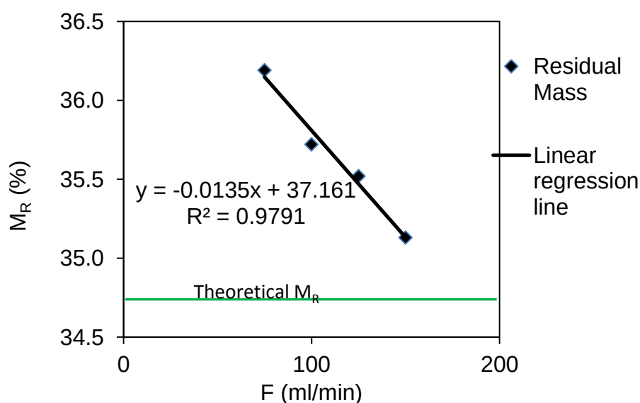
Figure 5.6: Dependency of residual mass ( M_R ) on the N_2 Flow rate ( F )
