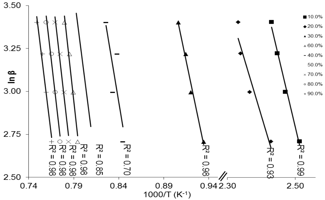
Figure 5.9: Plot according to Ozawa-Flynn-Wall method (OFW)
