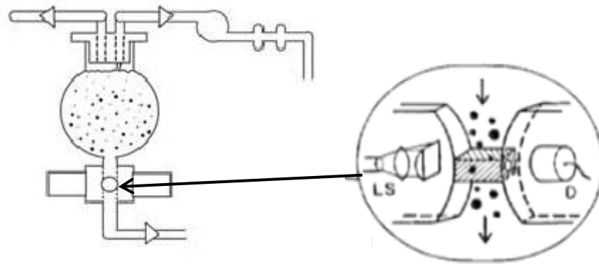
Figure 2.9: Schematic diagram of the Auto dilution system of the Nicomp 780 Accusizer system
