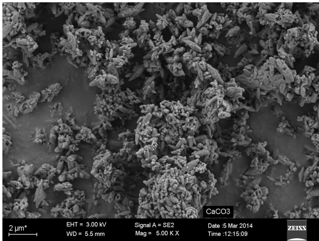
Figure 4.6: SEM image of the modified Merseburg PCC
