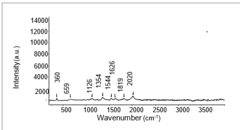
Figure 5.15: Raman spectrum of \text{CaO}
