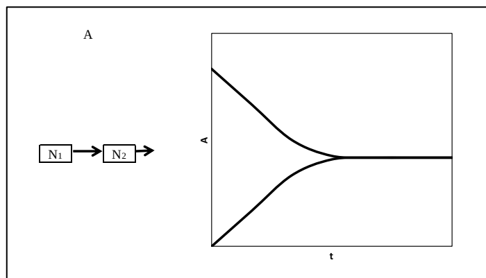
Figure 2.7: Depiction of decay rates (A) of arbitrary parent nuclides N_1 and daughter nuclide N_2 and the state of secular equilibrium
