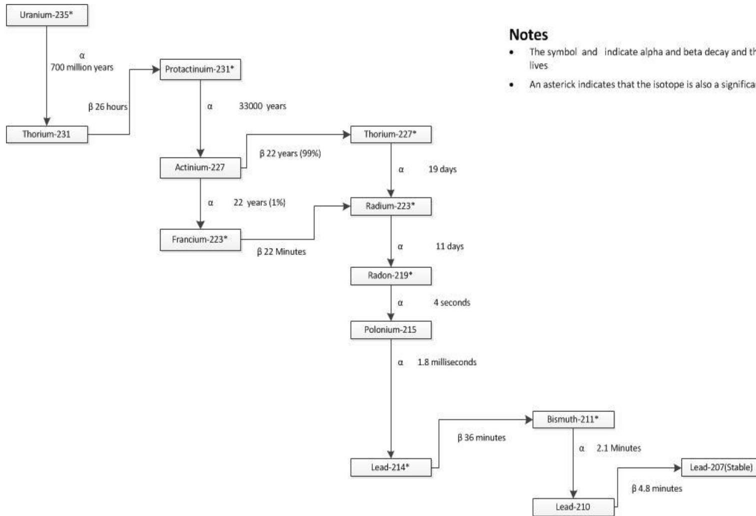
Figure 2.5: Natural decay series of Uranium-235 showing the modes of decay ( \alpha = alpha; \beta =beta) and the half-lives of the daughter nuclides (Coles et al. , 1978)
