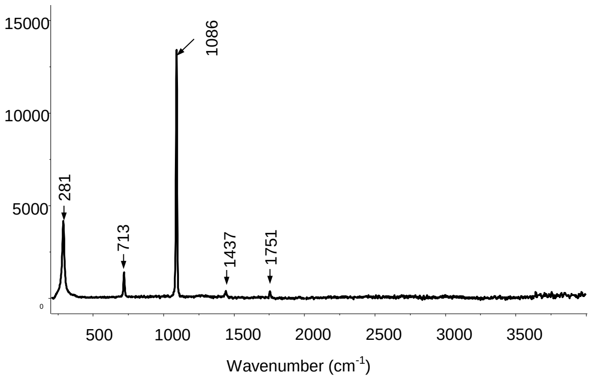
Figure 4.5: Raman spectrum of the modified Merseburg process PCC
