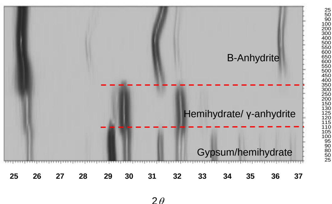
Figure 5.1: Reaction between gypsum and carbonaceous material 25-650 °C under nitrogen flow
