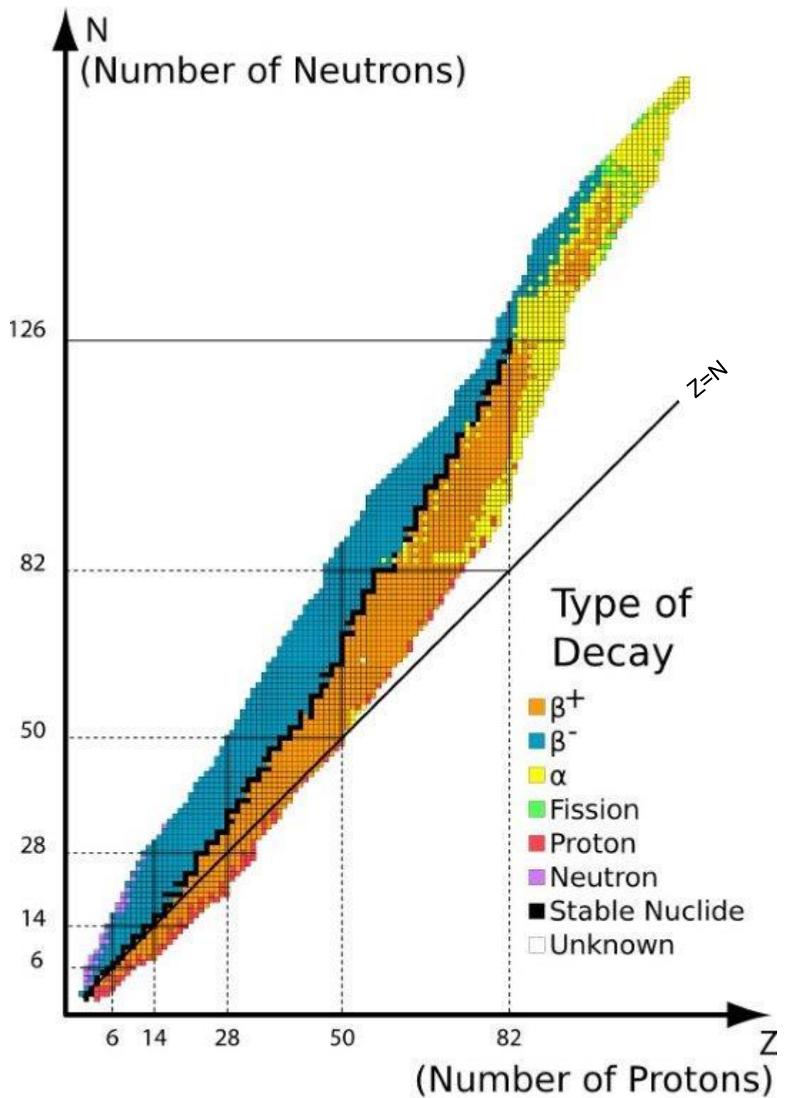
Figure 2.1: Chart of radionuclides in a plot of Z versus N ( www.nndc.bnl.gov/chart/ )
