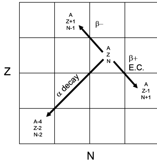
Figure 2.2: Transition diagram for decay modes of a radioactive nuclide, with mass number A and atomic number Z (shown are \alpha , \beta^\pm , emissions, EC denotes electron capture). http://www2.lbl.gov/abc/
