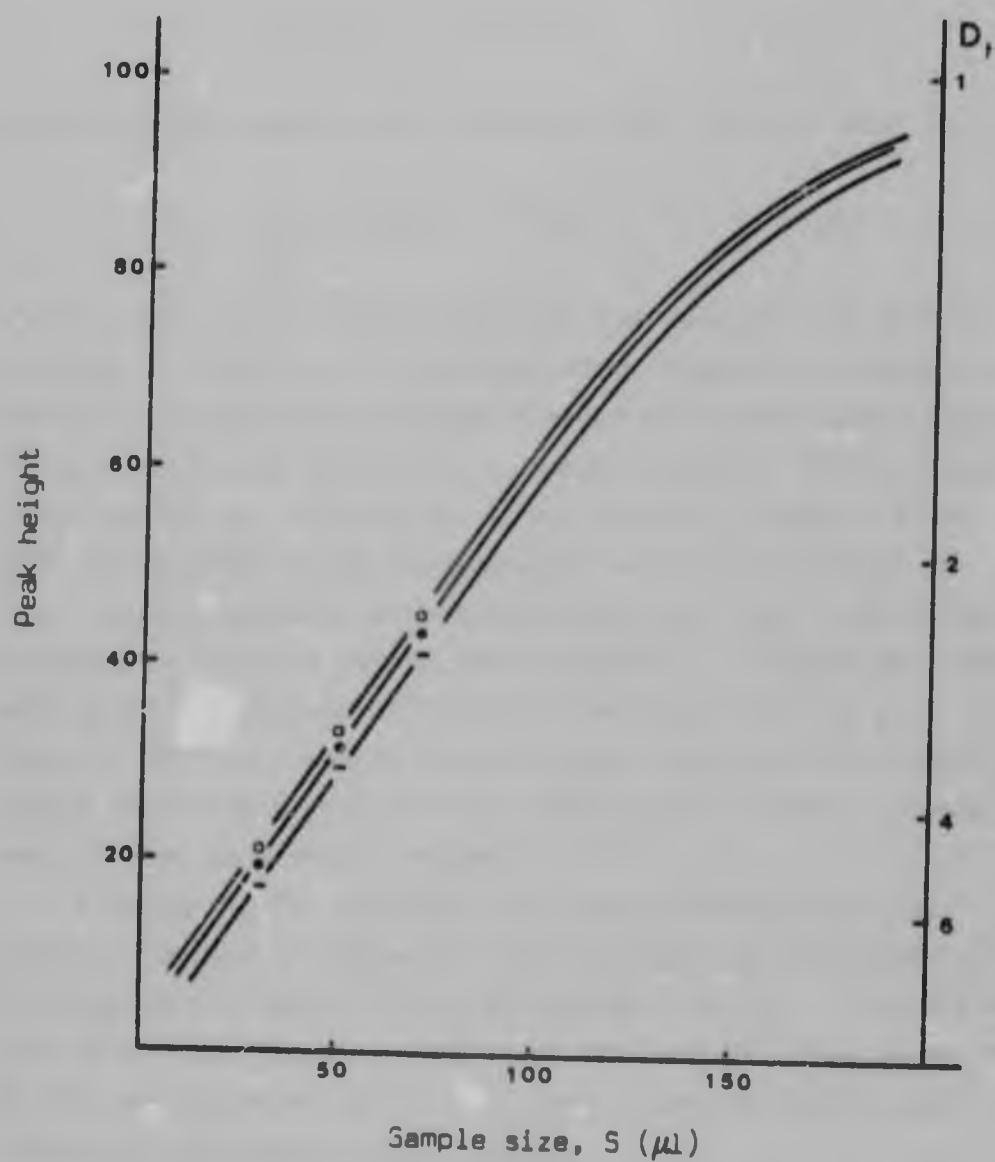
Figure 3.7 Effect of coil length and sample size on peak height
