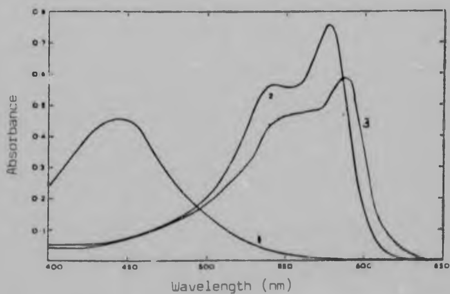
Figure 2.1 Wavelength absorbance curves
