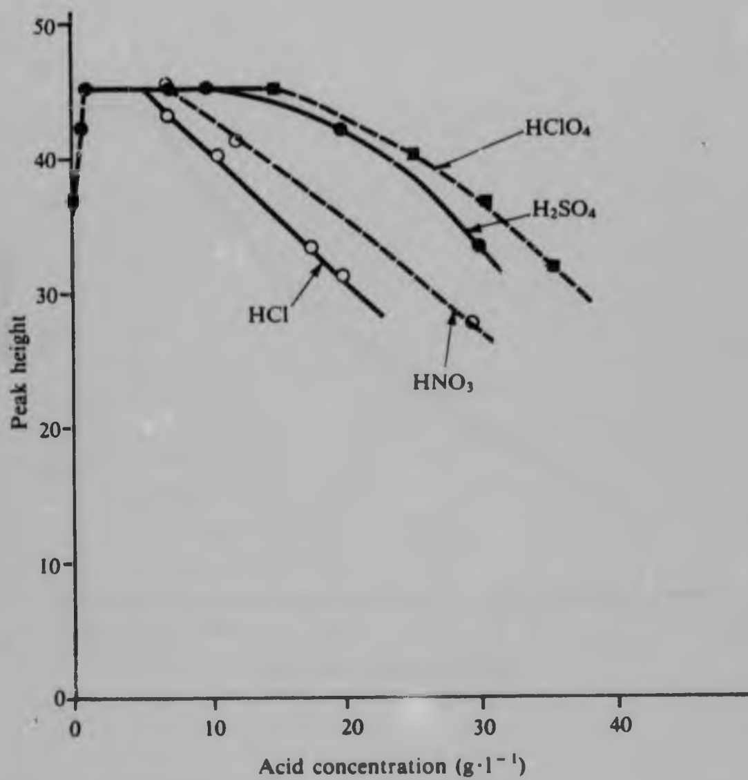
Figure 4.2 Interference from inorganic acids
