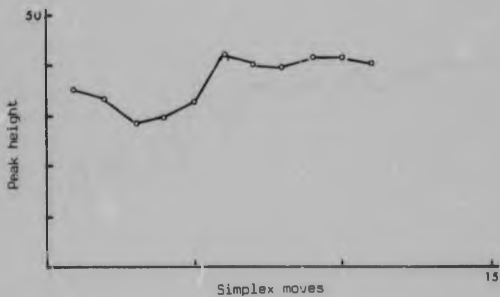
Figure 3.18 Optimization using a Modified Simplex approach with two variables
