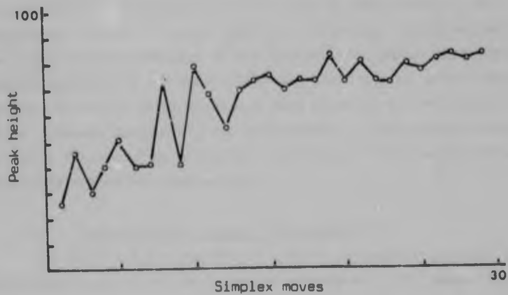
Figure 3.20 Optimization using a Modified Simplex approach with three variables
