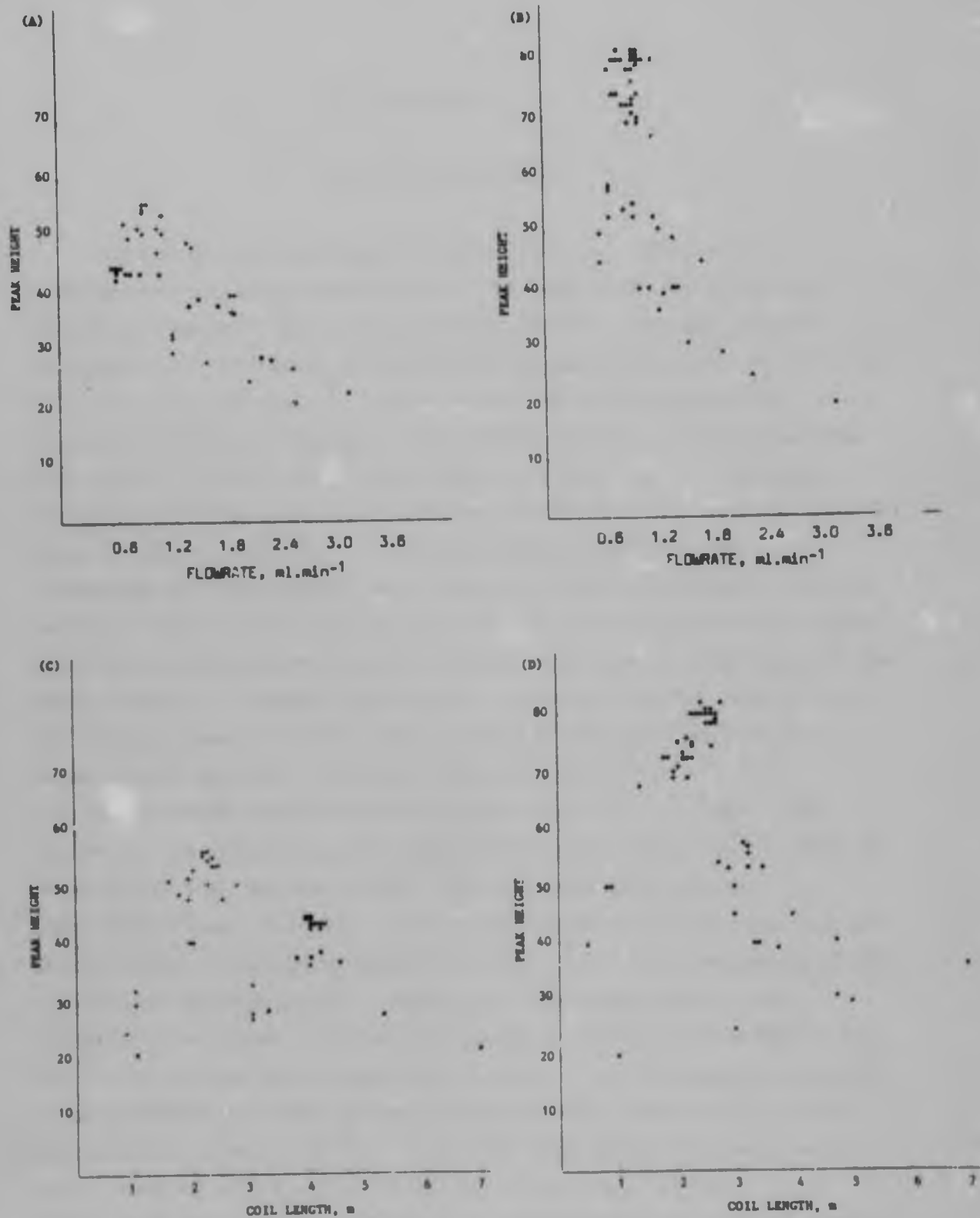
Figure 3.21 Scatter diagrams of peak heights vs. variable values for the Modified Simplex optimizations
