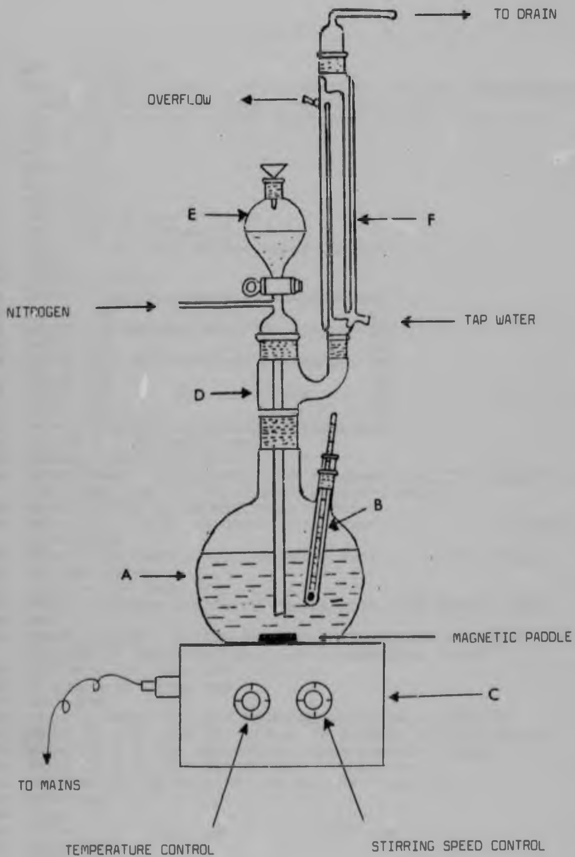
Figure I-1 The apparatus (Diagrammatic - not to scale)
