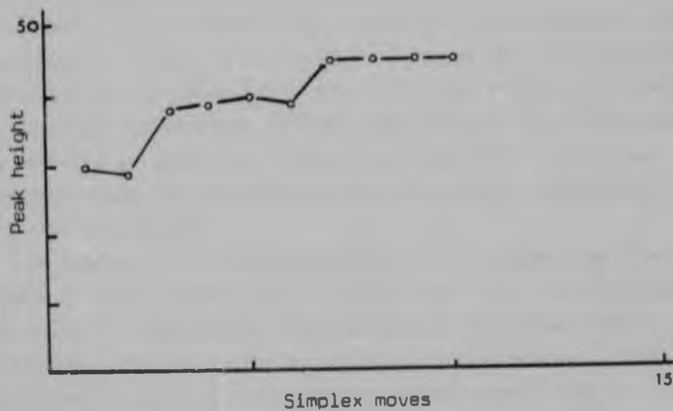
Figure 3.19 Optimization using a Modified Simplex approach with two variables
