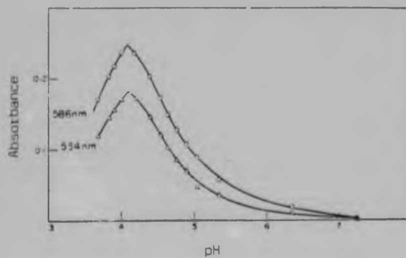
Figure 2.2 pH absorbance curves
