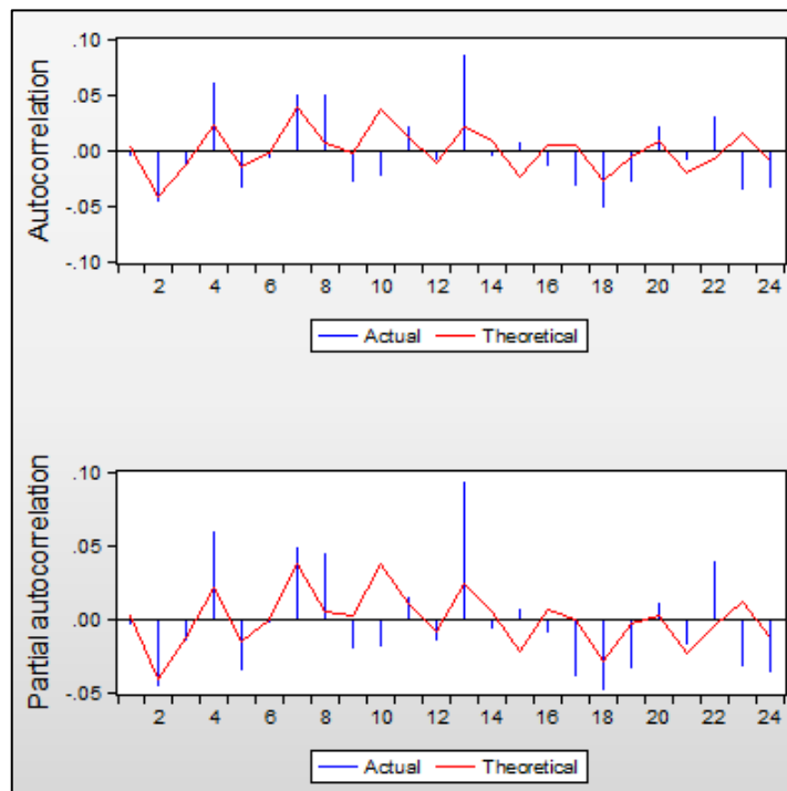
Figure 12: Graphical view of the actual and ARMA model correlogram
