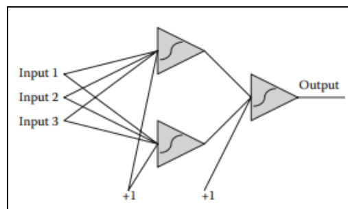
Figure C1: Three neurons in multilayer perceptron network (Source: Wilamowski and Yu (2011))
