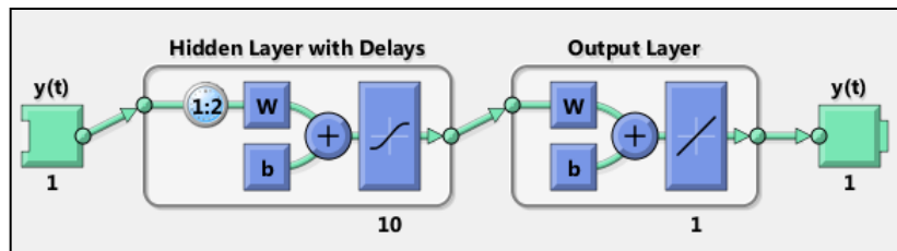
Figure 14 : Graphical representation of TDNN
