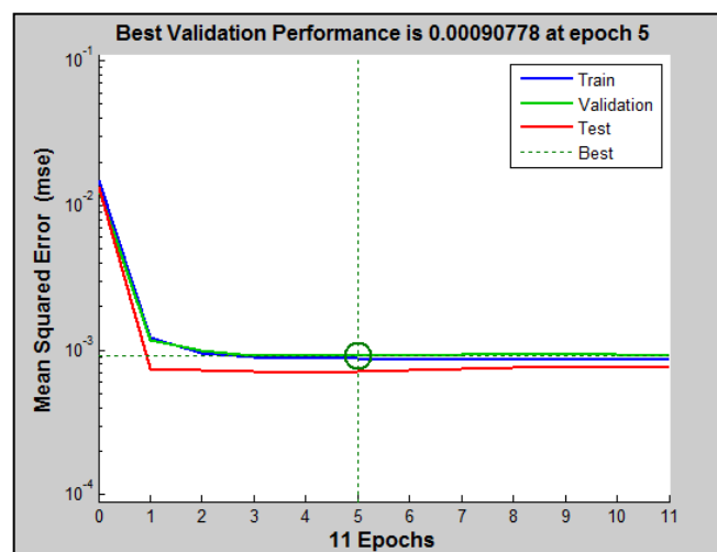
Figure 16: Best validation performance
