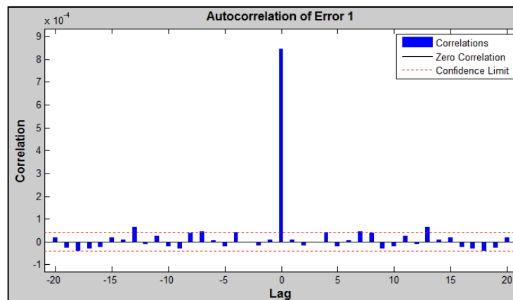
Figure 17: Plot of the error autocorrelation function
