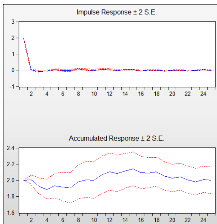
Figure 13: Impulse response function of ARMA model
