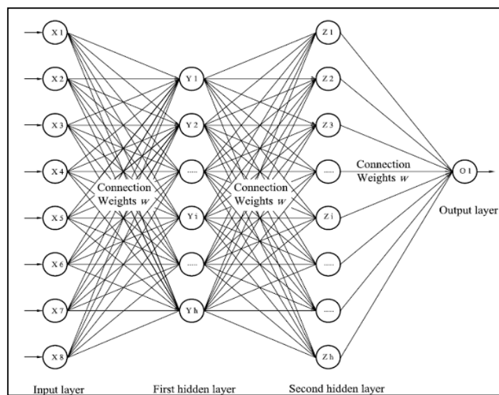
Figure 3: Typical architecture of a multilayer perceptron
