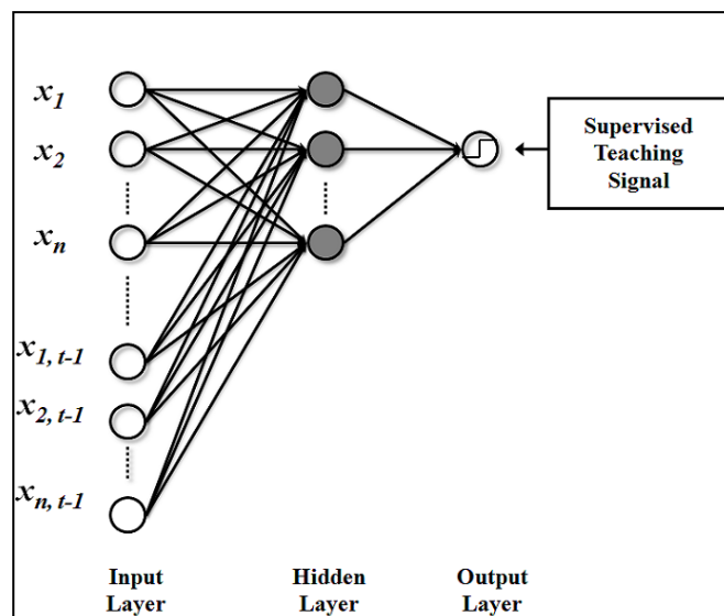
Figure 4: Typical architecture of a time delay neural network (Source: Versace & Wong, 2009, p, 14)
