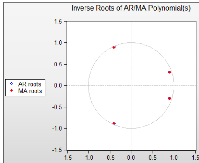
Figure 11: Graphical view of the inverse roots of the AR and MA characteristic polynomial
