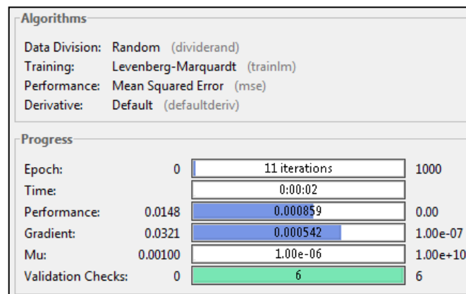
Figure 15: Algorithm and progress of TDNN
