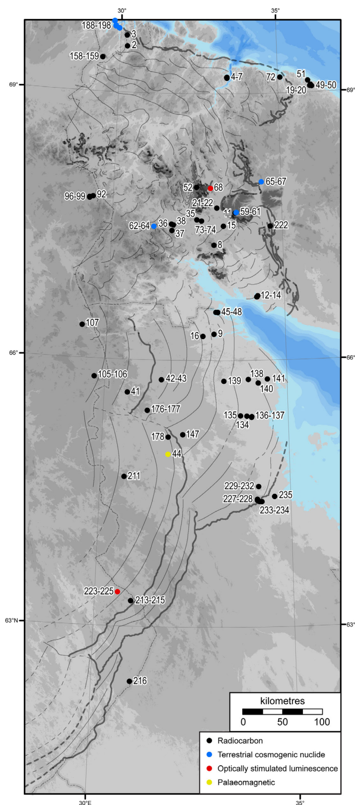
Fig. 5. Locations of numerical ages within the study area that are included in the numerical age database. Numerical ages outside of, and beyond, the study area are not shown for clarity, but the locations of all numerical ages can be viewed in the Supporting Information as Data S1 and S2.
