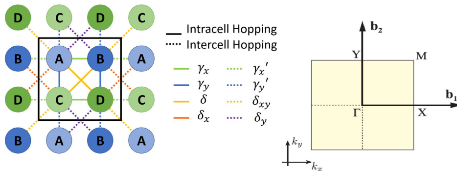
Figure 1. (Left) Construction of a 2D system using two different 1D SSH chains coupled together in the y -direction. Lattice sites A, B, C, and D represent one unit cell (outlined in black). Dashed and solid lines show all the possible nearest and next-nearest-neighbor hoppings from each unit cell. (Right) The typical 2D Brillouin zone for the unit cell in reciprocal space. \Gamma , M, X, and Y represent the high-symmetry points of the cell.
