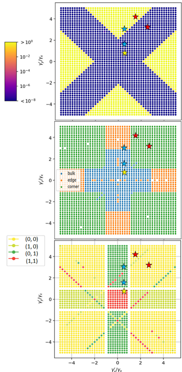
Figure 2. (Top) Bulk bandgap where the color bar on the left tracks the size of the bandgap, from blue (zero bandgap) to yellow (gap size > 1 ). (Middle) VBM localization type for a system with 80 \times 80 unit cells with open-boundary conditions, where blue, orange, and green represent a bulk, edge, and corner localization, respectively. (Bottom) Parity invariant for a nearly isotropic 2D SSH system, where 0 corresponds to a topological phase and 1 corresponds to a trivial phase. The stars represent the five different sample points used to study the different phases possible for the system.
