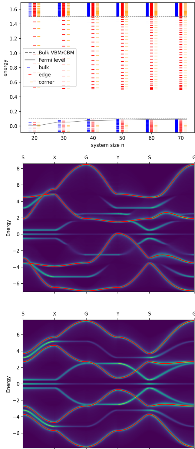
Figure 4. Fully topological nonmetallic phase, where \gamma_x = \gamma_y = 1 , \gamma'_x = 1.5 , and \gamma'_y = 4.2 with \delta = -0.8 . Top: Eigenvalues and state localization for different system sizes and open-boundary conditions. Opacity indicates strength of bulk, edge, and corner contributions to the wave functions. Center: Fourier transform of n = 70 wave functions. Red curves represent the corresponding bulk band structure. Bottom: Reference band structure without SNN interaction.
