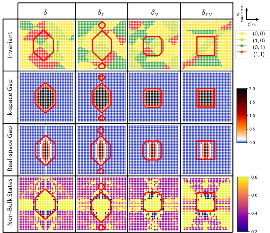
Figure 3. (Top row) Bulk invariant, (second row) reciprocal space gap size, (third row) real space gap size, and (bottom row) VBM state localization for a nonperiodic real system. The plots are made for \gamma'_x = 4.1 and consider the relationship between each of the different SNN parameters as a function of \gamma'_y . Parameters are varied in interval [-5, 5] . An invariant value of 1 or 0 refers to a trivial or topological phase, respectively. The first color bar runs from blue to black, indicating gaps from 0.0 to 2.0. The last color bar represents the magnitude of the VBM localization.
