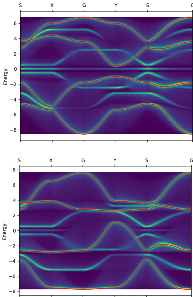
Figure 6. Fourier transforms of the open-boundary wave functions plotted over reciprocal space, with the bulk wave functions indicated in red for a NM_{11} system, where the bulk bandgap is less than the open-boundary bandgap, with (top) \delta = 0.6 and \delta_{xy} = 0.3 , that is, a fully topological phase, and (bottom) \delta = -0.9 and \delta_{xy} = \pm 0.95 , that is, a partially topological phase. A system size of n = 60 was used.
