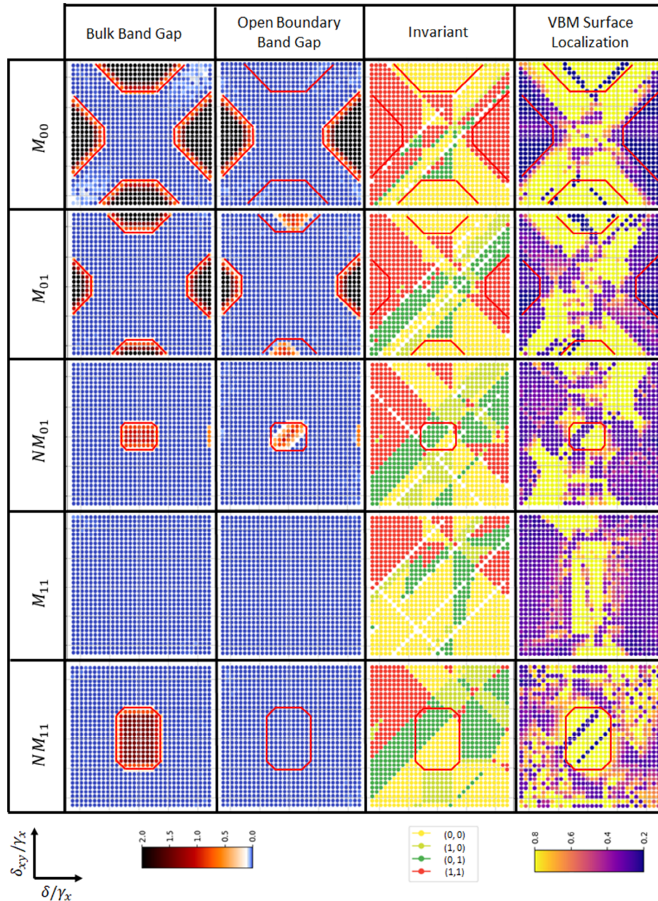
Figure 5. The bulk bandgap, open-boundary bandgap, invariant, and VBM localization for an initially metallic trivial and partially topological phase and a nonmetallic trivial, partially and completely topological phase for varying \delta and \delta_{xy} . The left color bar represents a gap running from 0 (blue) to 2.0 (black). The right color bar represents the magnitude of the VBM localization.
