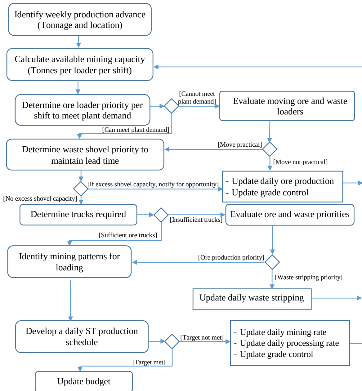
Figure 2.5: A typical planning activity diagram for daily short-term production scheduling
