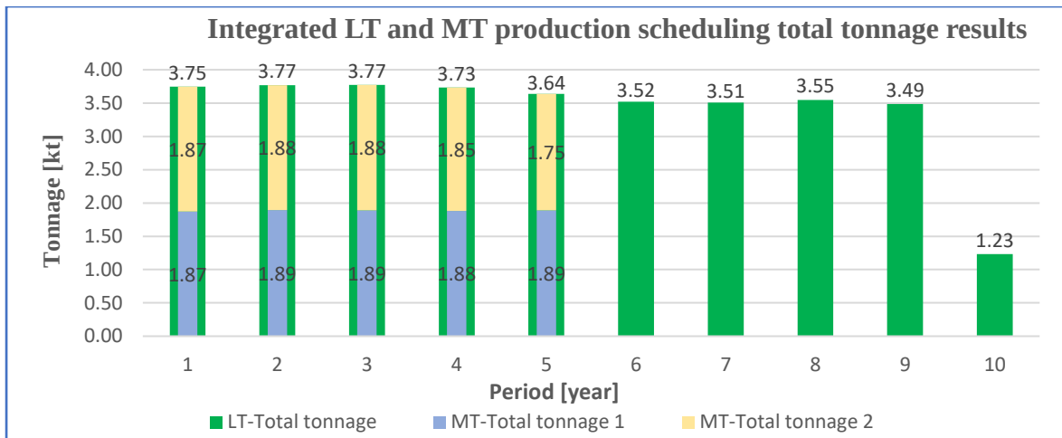
Figure 5.37: Total tonnage achieved for the integrated LT and MT production schedule
