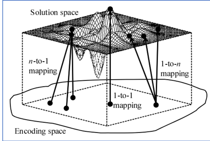
Figure 2.8: Mapping from chromosomes to feasible solutions in a solution space (Source: Gen, et al. , 2008)
