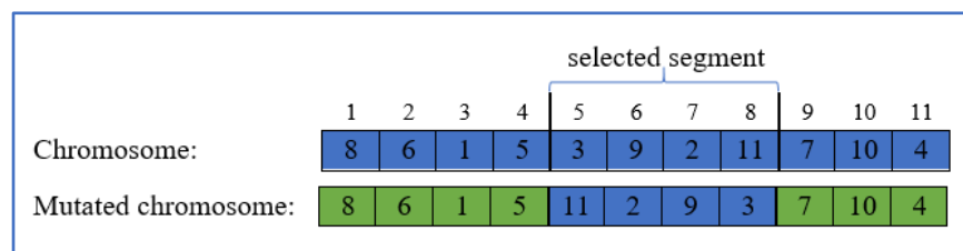
Figure 2.12: Illustration of an inversion mutation genetic procedure
