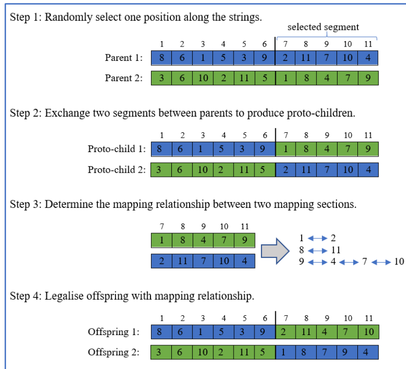
Figure 2.9: Illustration of a single-point crossover genetic procedure (Source: adapted from Gen et al. , 2008)
