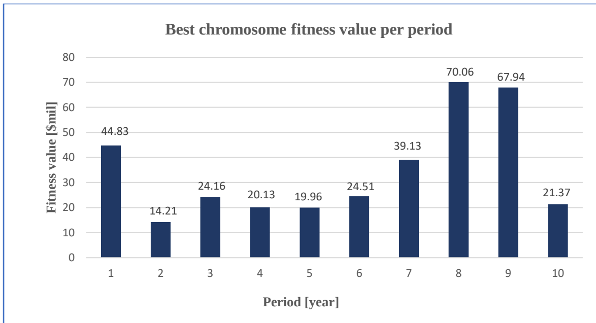
Figure 5.34: Fitness value of the best chromosome per period for the optimisation of the integrated LT and MT production schedule
