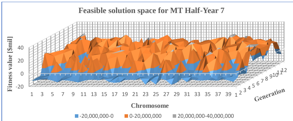
Figure 5.23: Feasible solution space for the optimisation of the MT production schedule in Period 7
