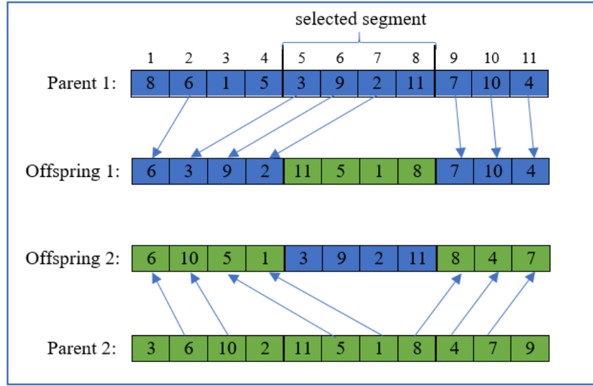
Figure 2.11: Illustration of an order crossover genetic procedure (Source: adapted from Gen et al. , 2008)
