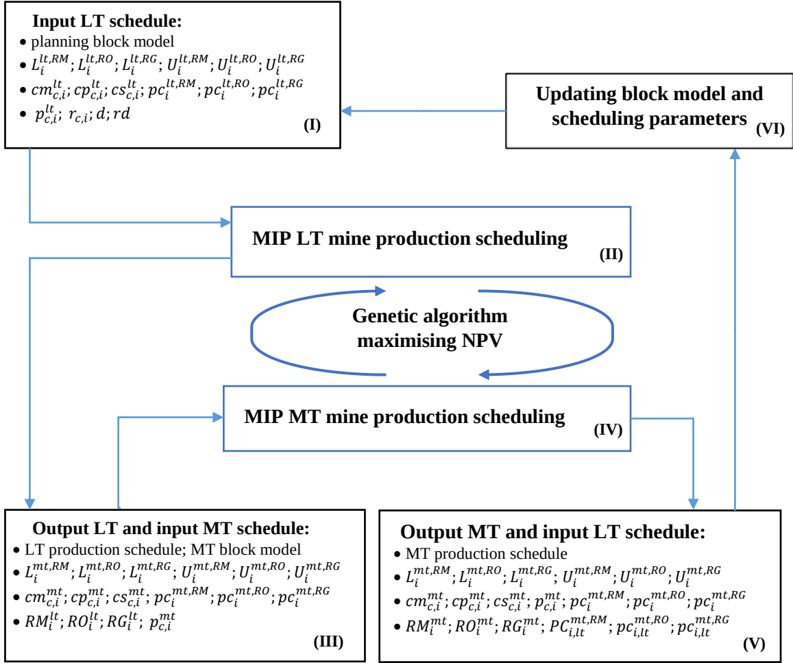
Figure 3.2: A framework for a dynamic integrated long-term and medium-term mine production scheduling model (Muke et al., 2025a)
