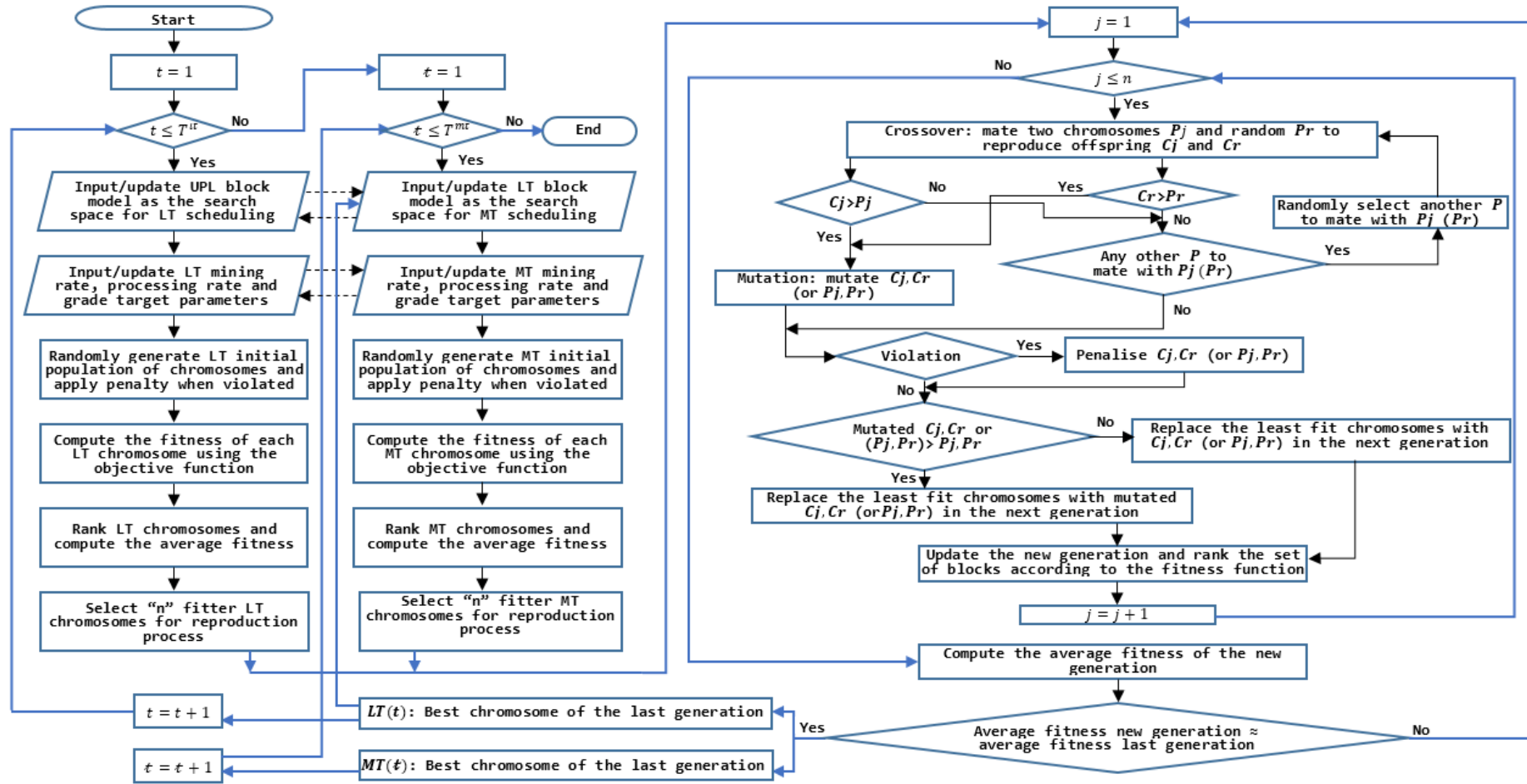
Figure 4.1: Framework of the GA methodology for solving the MIP model (Muke et al., 2025a)
