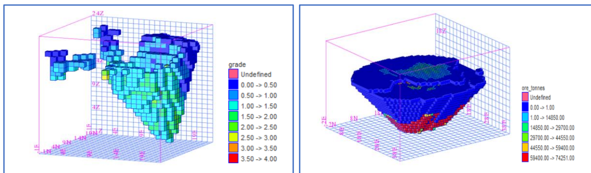
Figure 5.1: Spatial view of the Newman (left) model with grade variation and Zuck Small (right) model with ore tonnage variation per block
