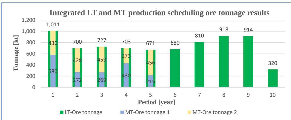
Figure 5.38: Ore tonnage achieved for the integrated LT and MT production schedule
