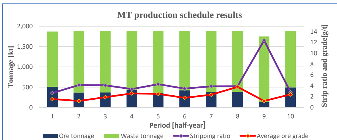
Figure 5.31: Ore and waste tonnages, stripping ratio and average grade in each period of the MT production schedule
