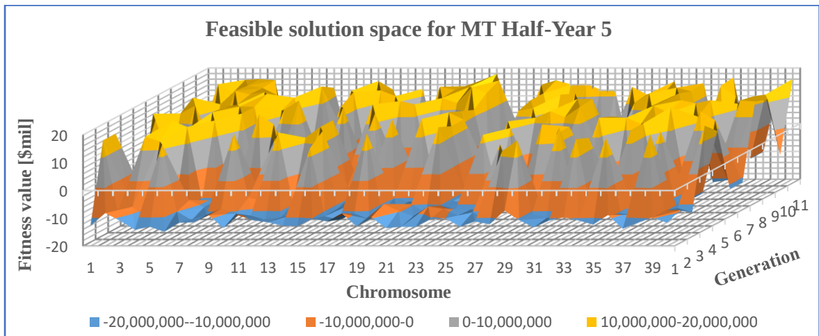
Figure 5.21: Feasible solution space for the optimisation of the MT production schedule in Period 5
