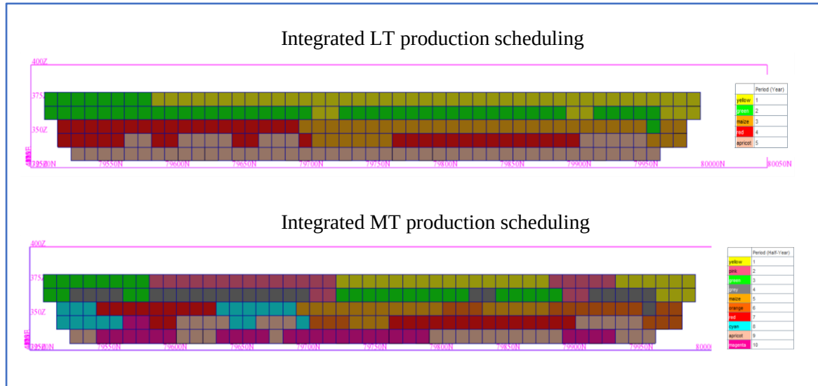
Figure 5.36: 4250E cross-sections spatial compliance between LT and MT production scheduling integrally optimised
