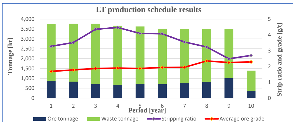
Figure 5.16: Ore and waste tonnages, stripping ratio and average grade in each period of the LT production schedule
