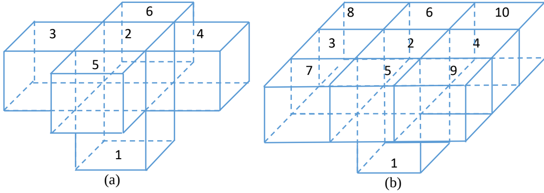
Figure 3.1: Graphical views of block predecessors, 1:5 pattern (a) and 1:9 pattern (b) (Muke et al. , 2025a)
