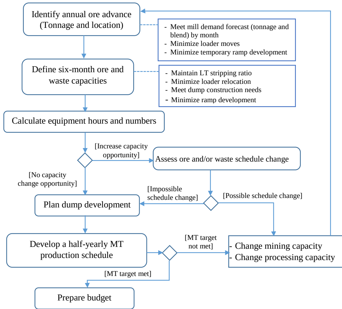
Figure 2.2: A typical planning activity diagram for medium-term six-month production scheduling (Source: adapted from Thorley, 2012)
