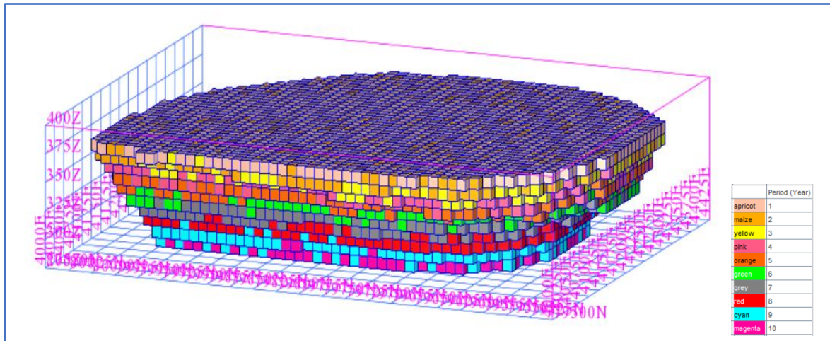
Figure 5.14: A 3D view of the LT production schedule for the Surpac block model
