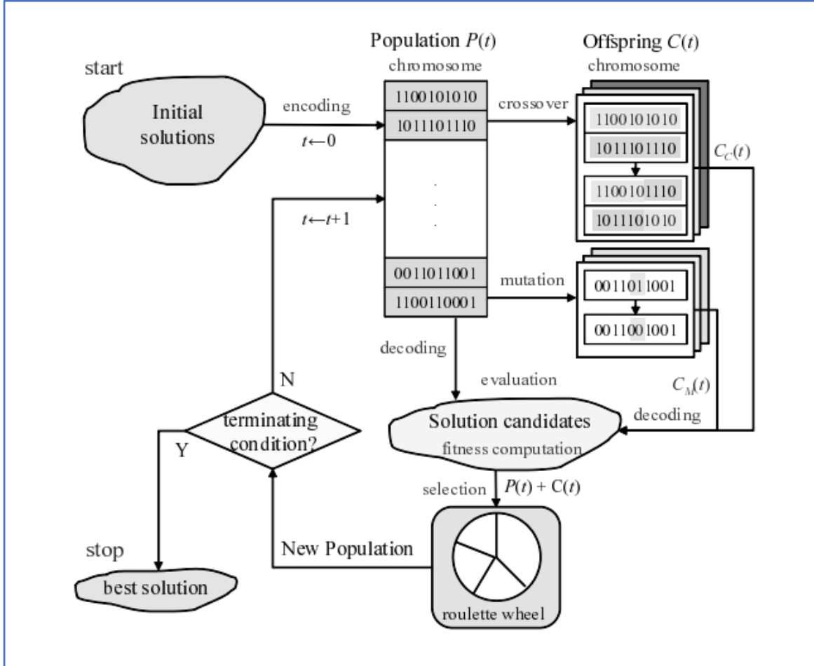
Figure 2.7: General structure of the genetic algorithm (Source: Gen, et al., 2008)
