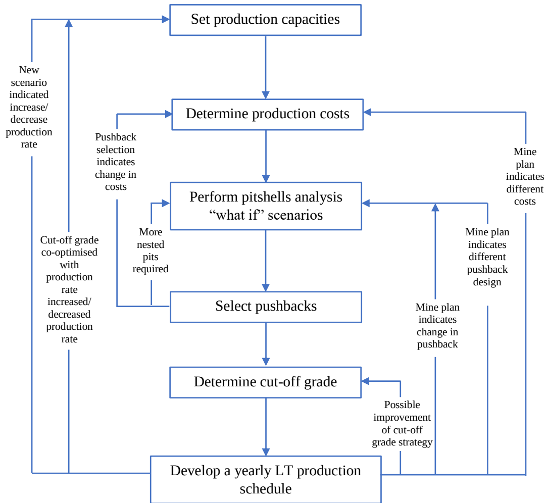
Figure 2.1: A typical activity diagram for long-term production scheduling (Source: adapted from Thorley, 2012)
