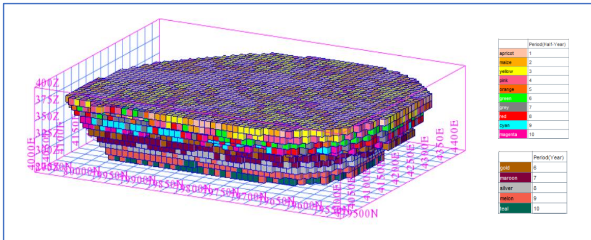
Figure 5.35: A 3D view of the integrated LT and MT production schedule for the Surpac block model
