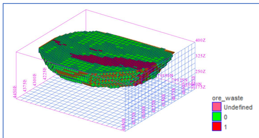
Figure 5.2: Spatial view of Surpac block model showing ore (1) and waste (0) blocks
