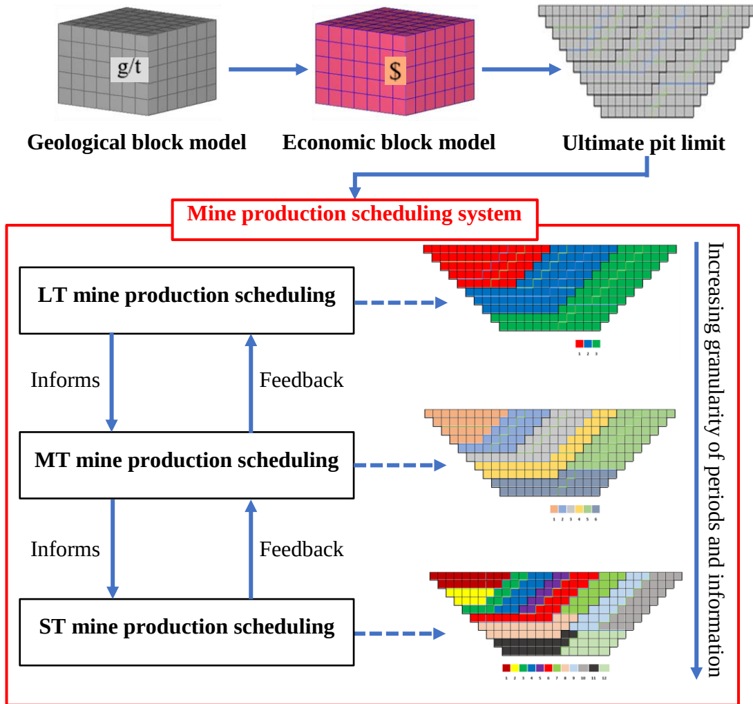
Figure 1.2: Open-pit mine production scheduling system highlighting the link between long-term, medium-term and short-term production schedules (Muke et al. , 2025a)
