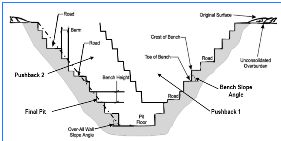
Figure 1.1: A generic cross-sectional view of an open-pit mine design
