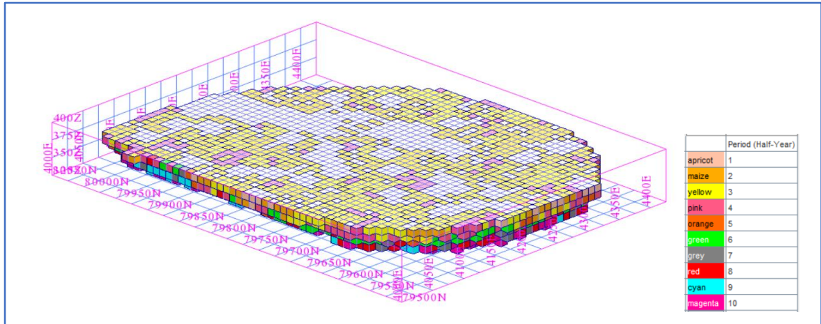
Figure 5.29: A 3D view of the MT production schedule for the Surpac block model
