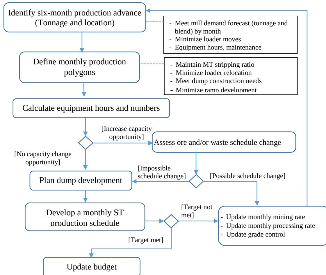
Figure 2.3: A typical planning activity diagram for monthly short-term production scheduling
