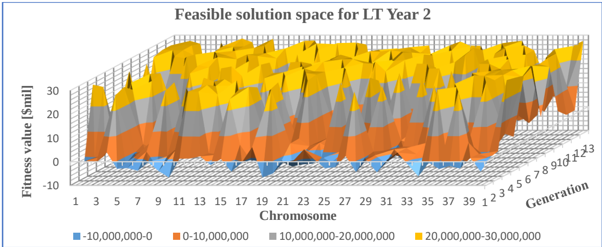
Figure 5.4: Feasible solution space for the optimisation of the LT production schedule in Period 2
