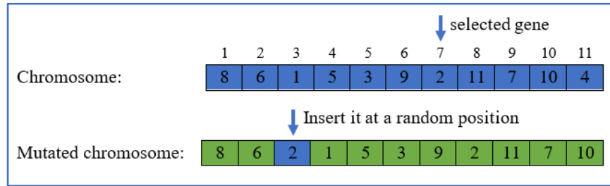
Figure 2.13: Illustration of an insertion mutation genetic procedure (Source: adapted from Gen et al. , 2008)
