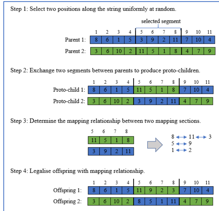
Figure 2.10: Illustration of a partial-mapped crossover genetic procedure (Source: adapted from Gen et al. , 2008)
