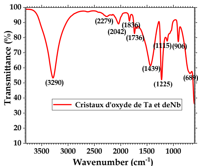
Fig. 12. FTIR of Ta and Nb crystals after precipitation-crystallization process of solution
