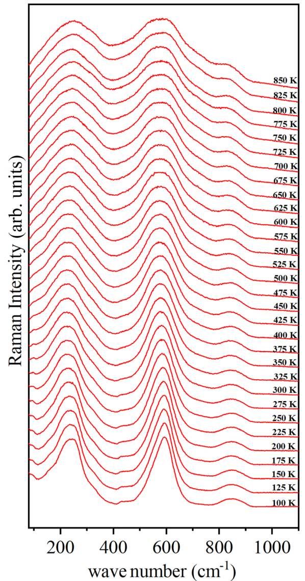
FIG. 5. Variable-temperature Raman spectra of NN-25BCT in the temperature range 100 \text{ K} \leq T \leq 850 \text{ K} . The Raman spectra shown here have been taken during the heating cycle using the protocol described in the experimental section.
