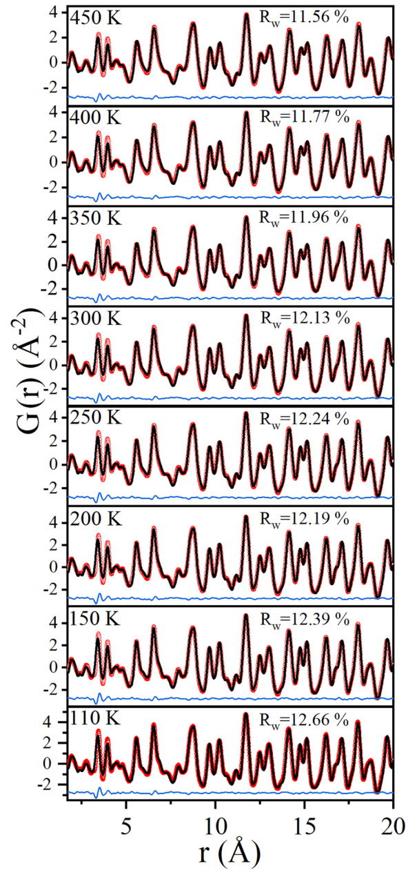
FIG. 8. The experimental (red dots) and calculated (black continuous line) pair distribution functions (PDFs) and their difference (blue line at the bottom) using the tetragonal space group ( P4bm ) in the temperature range 110–450 K obtained by refinement using the PDFGUI program.
