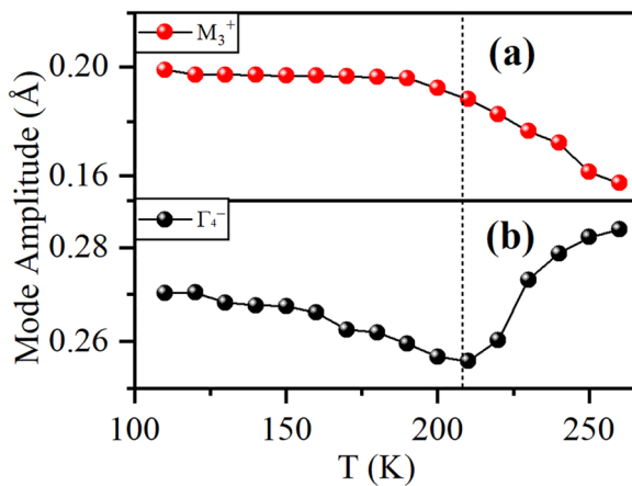
FIG. 3. Temperature-dependent evolution of (a) M_3^+ and (b) \Gamma_4^- modes in the stability region of long-range ferroelectric phase with P4bm space group calculated using the information obtained from the refinement of SXRD patterns.
