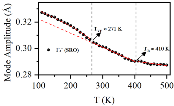
FIG. 9. Temperature dependent evolution of \Gamma_4^- mode calculated for short-range ordering (SRO) using the information obtained from refinement of PDF patterns.
