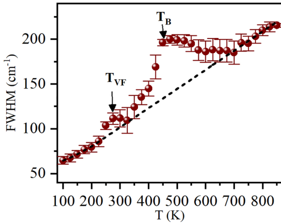
FIG. 6. Temperature-dependent variation of the FWHM of the Raman mode located near 250\text{ cm}^{-1} . The black dashed line is a polynomial baseline to account for the trivial increase in phonon widths on heating.
