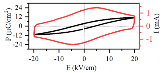
FIG. 4. Room-temperature polarization vs electric field ( P - E ) and associated current vs electric field ( I - E ) loops of NN-25BCT measured at a maximum electric field of 20 kV/cm. The slim hysteresis loop is characteristic of a relaxor-like behavior.
