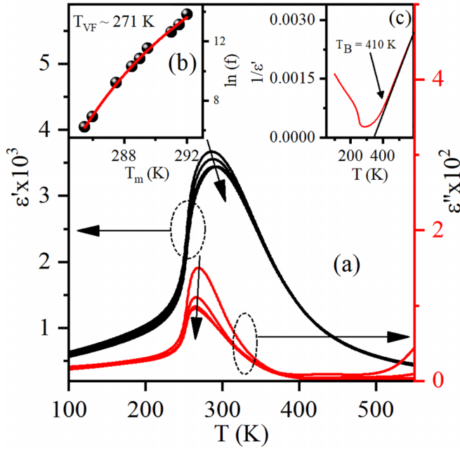
FIG. 1. (a) Temperature-dependent evolution of real and imaginary part of dielectric permittivity. (b) Vogel-Fulcher fitting of the temperatures corresponding to the dielectric to estimate the freezing temperature. (c) The inverse of dielectric permittivity as a function of temperature, marking the Burns temperature.
