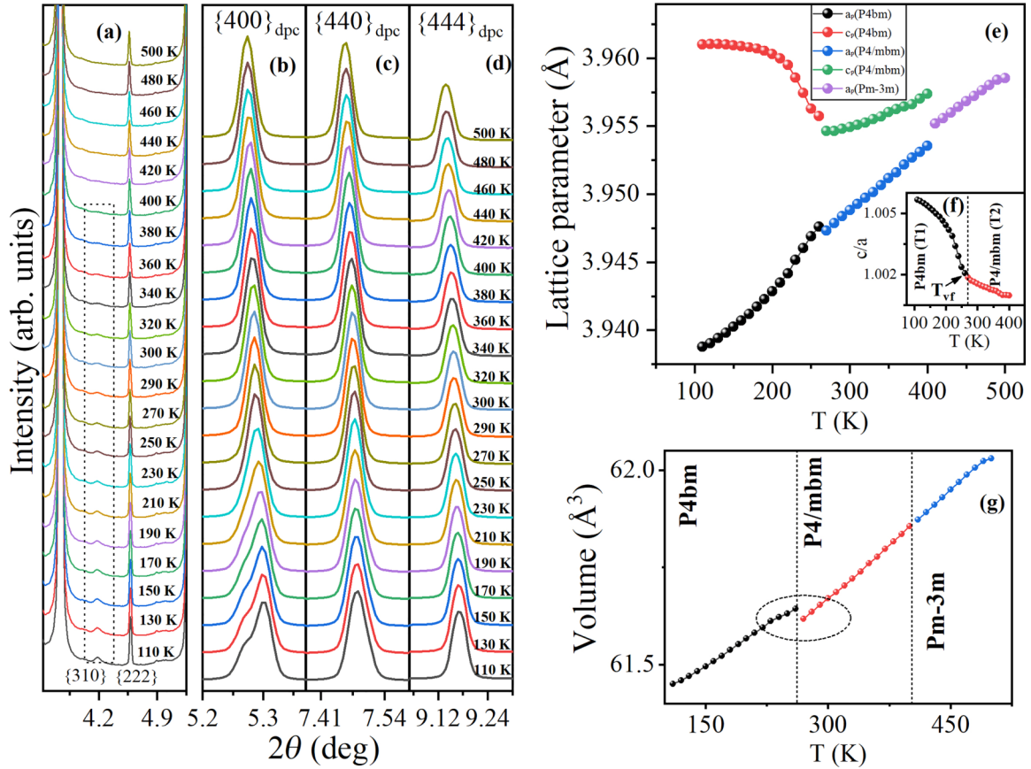
FIG. 2. Temperature-dependent evolution of some representative (a) superlattice reflections, (b)–(d) main perovskite reflections. Evolution of (e) lattice parameters, (f) tetragonality, and (g) volume of the elementary cell as a function of temperature.
