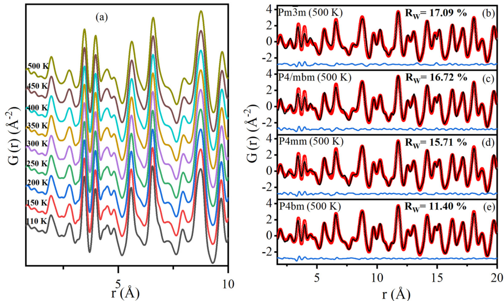
FIG. 7. (a) Temperature dependent evolution of PDF profiles of NN-25BCT. Atomic PDF fitting at 500 K using different plausible models viz., (b) Pm\bar{3}m (c) P4/mbm , (d) P4mm , (e) P4bm . The goodness of fit parameter suggests that the P4bm model produces the best fit to the data.
