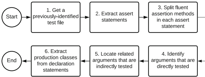
Fig. 2. Flow diagram of the statement-based matching algorithm.
