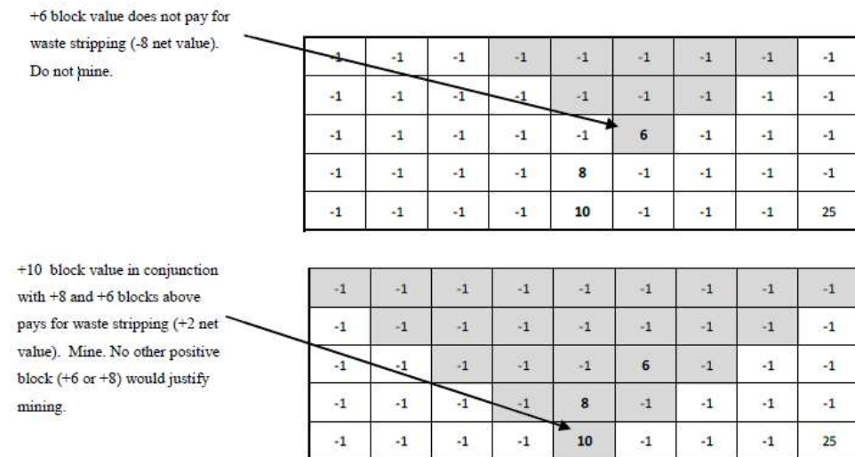
Figure 2-3 A simple 2D pit limit analysis (after Thorley, 2012)
