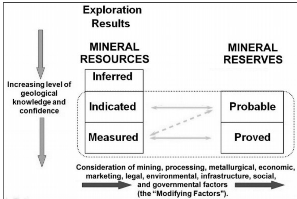
Figure 2-2 Mineral Resource and Mineral Reserve classifications (after Committee for Mineral Reserves International Reporting Standards, 2012)
