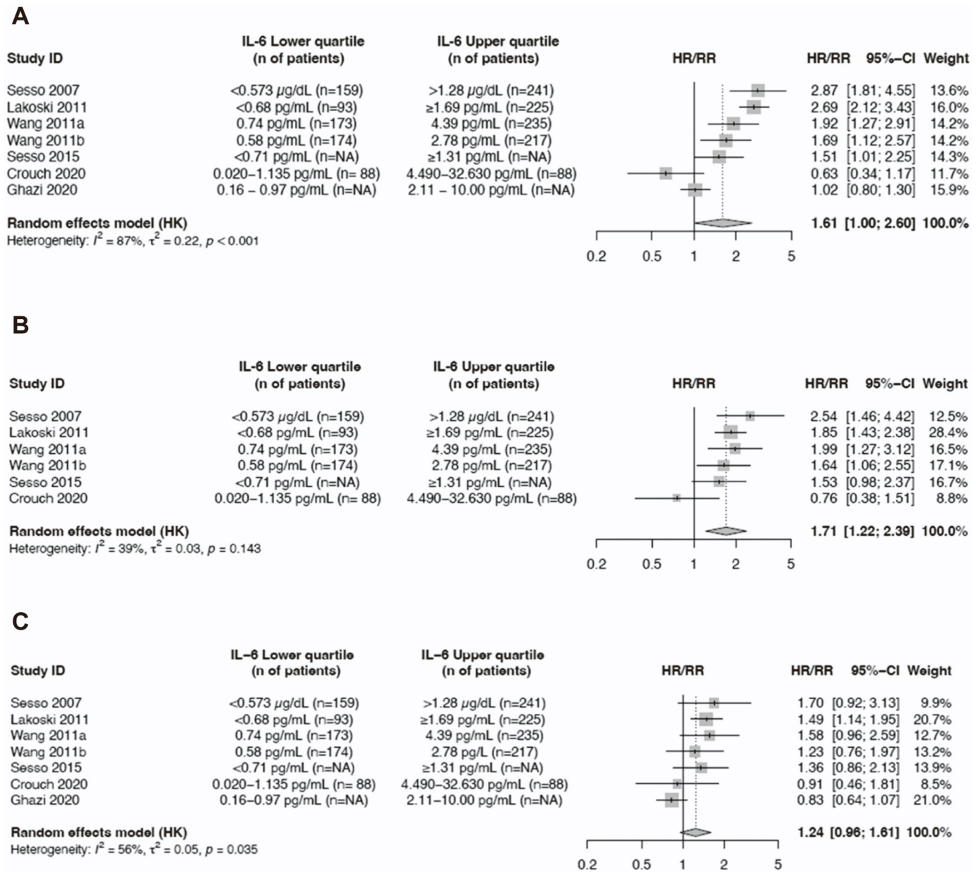
Fig. 2. Forest plots of pooled HR/RR of hypertension for the highest versus lowest quartile of IL-6. Hazard ratio (HR)/Risk ratio (RR) and 95% confidence interval (CI) from the eligible studies of the association between IL-6 circulating levels and incident hypertension estimates in a random effects model with crude RR/HR pooled in (A), adjusted RR/HR pooled in (B) without BMI and adjusted RR/HR pooled in (C) including BMI.
