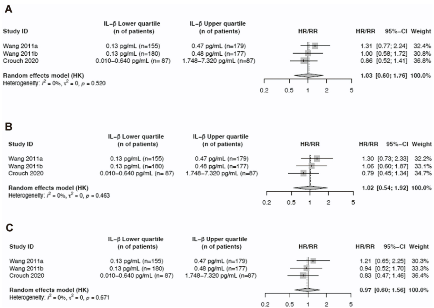
Fig. 3. Forest plots of pooled HR/RR of hypertension for the highest versus lowest quartile of IL-1 \beta . Hazard ratio (HR)/Risk ratio (RR) and 95% confidence interval (CI) from the eligible studies of the association between IL-1 \beta circulating levels and incident hypertension estimates in a random effects model with crude RR/HR pooled in (A), adjusted RR/HR pooled in (B) without BMI and adjusted RR/HR pooled in (C) including BMI.
