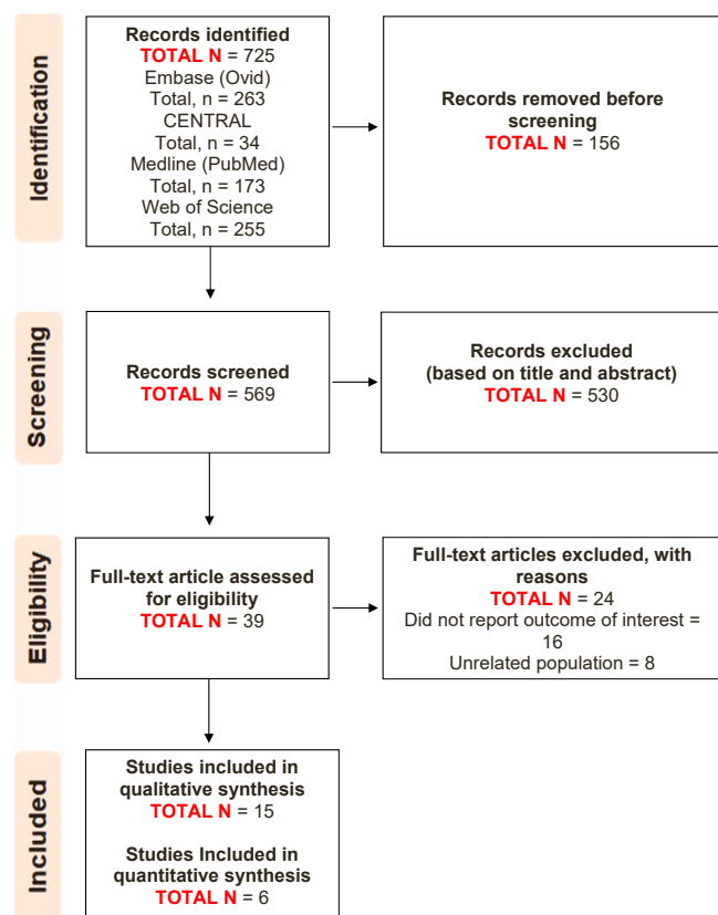
Fig. 1. Flow chart reporting the search strategy according to PRISMA.
