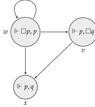
FIGURE 2.2: A Kripke model, with highlighted wffs, whose underlying Kripke frame is taken from Figure 2.1.
