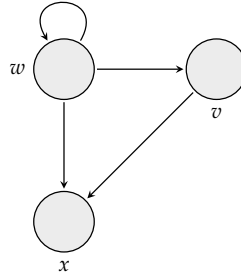
FIGURE 2.1: A Kripke frame defined by W = \{w, v, x\} , R = \{(w, w), (w, v), (w, x), (v, x)\} .
