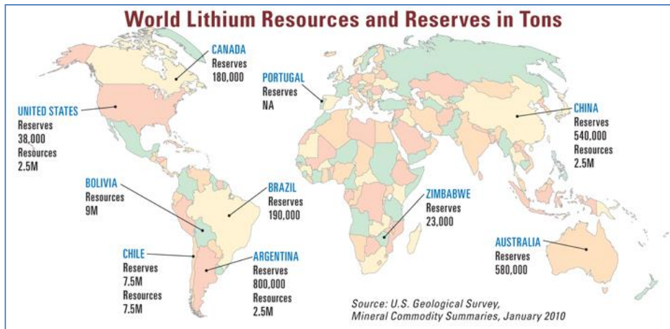
Figure 17: World Lithium Resources
