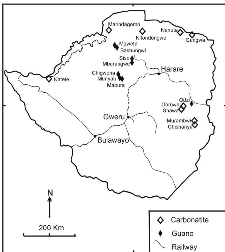
Figure 46: Carbonatite and Guano (cave) Deposits of Zimbabwe
