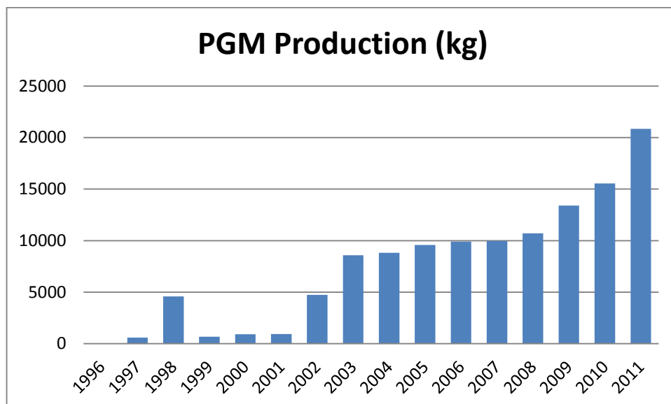
Figure 8: PGM Production (1996-2011)
