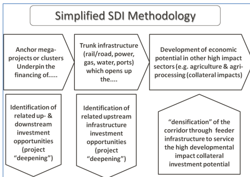
Figure 51: SDI Methodology
