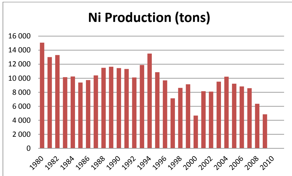
Figure 11: Nickel Production
