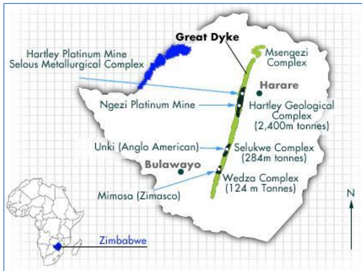
Figure 7: The Great Dyke
