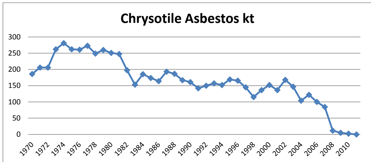
Figure 10: Asbestos Production (1970-2011)
