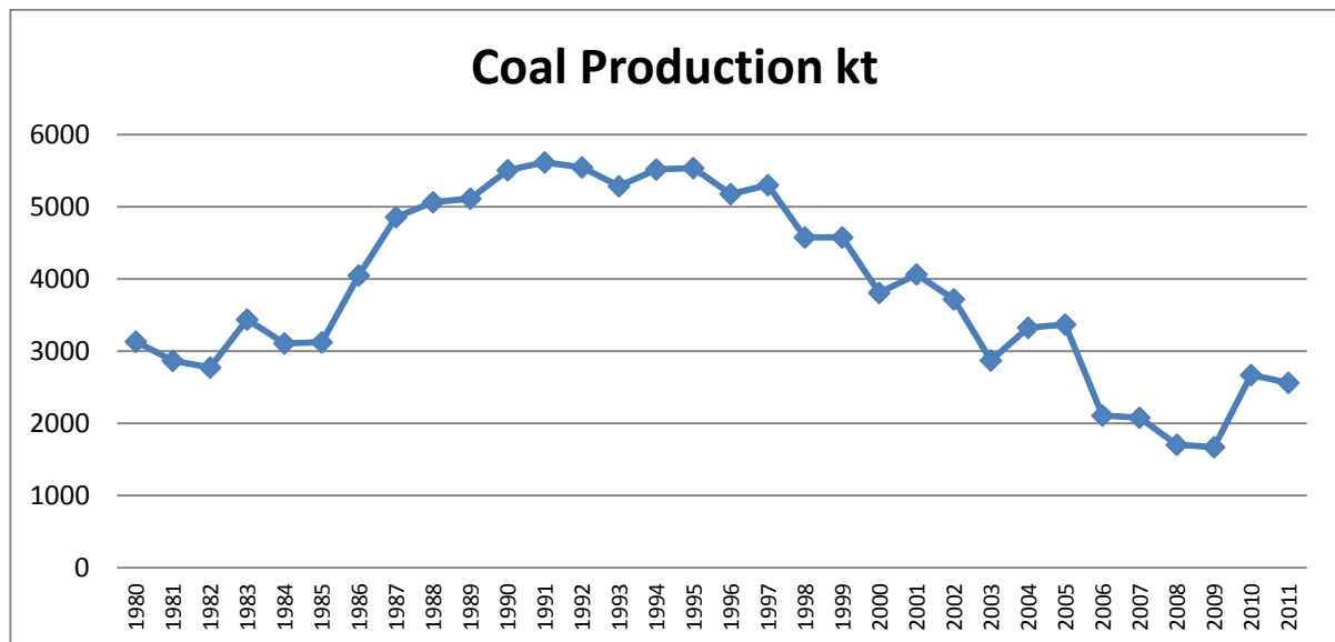
Figure 9: Coal Production (1980-2011)
