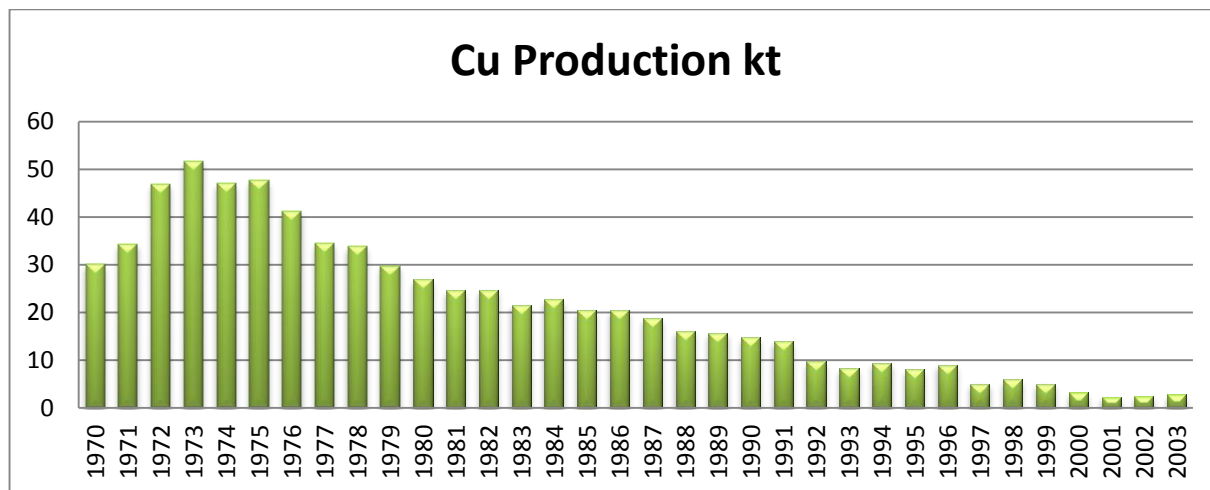
Figure 12: Copper Production (1970-2003)
