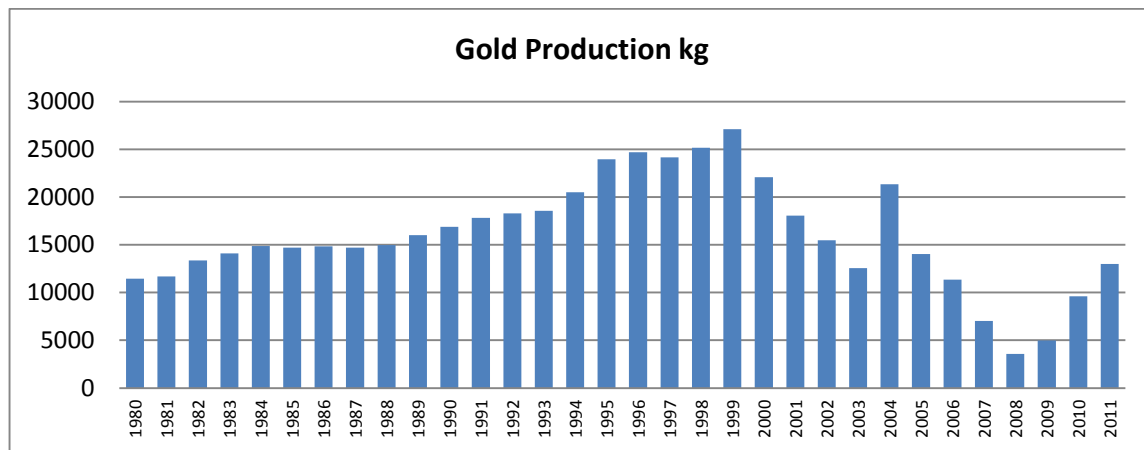
Figure 6: Gold Production
