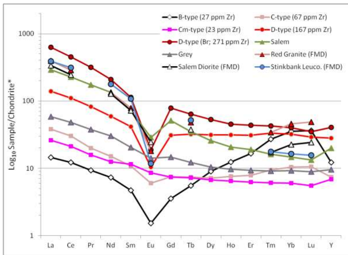
Figure 9.4 Average REE abundances of selected Central and Southern Zone granite groups. The pre-D 3 , B- and C-type samples have contrasting HREE enrichment; where the C-type is weakly depleted and the B-type is strongly enriched. The post-D 3 leucogranites have been split into two varieties; one with uraninite dominated mineralisation, and the other brannerite-dominated (D-type, Br). HREE and LREE fractionation are comparable, as is the -ve Eu anomaly, but the overall REE abundance is consistently enriched in the brannerite-bearing type. Samples with (FMD) are sourced from McDermott et al. (1989) and McDermott et al. (1996). All data normalised to McDonough and Sun (1995).
