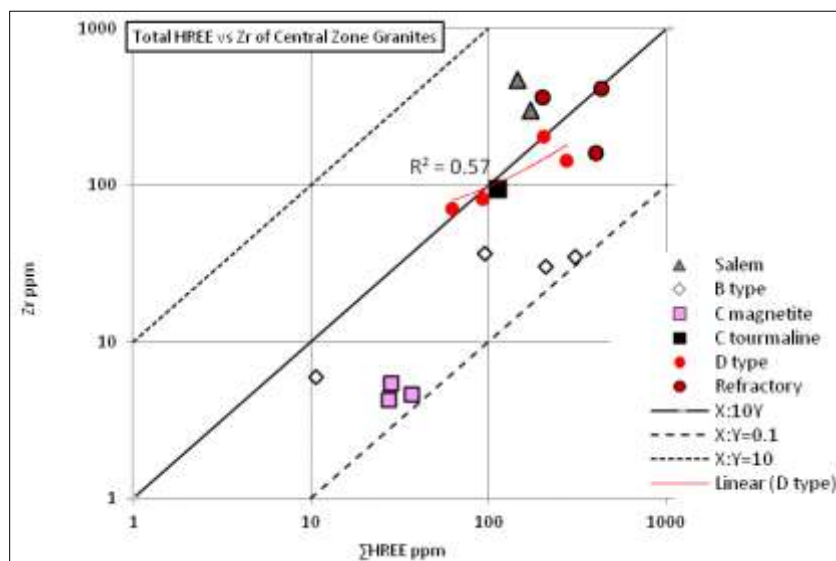
Figure 6.15 X-Y plot illustrating systematic behaviour of HREE abundances vs. Zr. There is a weak positive relationship between Zr and total HREE of the D-type sheets; however, none of the other leucogranite populations, or equigranular granites are similar. The high HREE content of the B-type is concentrated in garnet, while in the brannerite-bearing leucogranites, phosphates and brannerite may host the HREE and Y.
