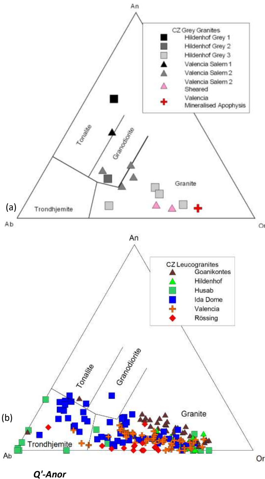
Figure 5.3 Or-An-Ab normative plots (after Barker, 1979) of Salem, Grey, and leucogranite suites of the Central Zone uranium deposits. (a) Or-An-Ab normative plots of Grey granites from Hildenhof and Salem Suite samples from Valencia. The diagram illustrates a compositional trend with age (type-1 are old and types 2 and 3 are successively younger, shearing and partial melting of Salem type-2 samples has resulted in higher normative Or proportions. The mineralised apophysis is a sample of mineralised leucogranite (alaskite) that intrudes megacrystic Salem granite near the Valencia deposit.
