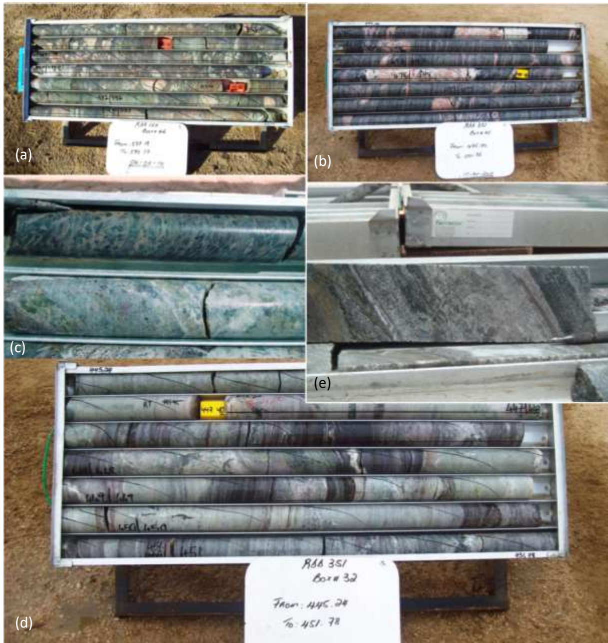
Figure 3.33 Typical Khan - Rössing transition succession lithologies observed in Zone 1 core specimens. (a-b) The upper Khan Formation meta-conglomerate (a) and banded gneiss becomes progressively less calcareous and retains pronounced compositional banding with depth (b). The banded gneiss is invaded by granitic leucosomes and veins (C-type of Nex, 1997). Core trays from drill holes RDD164 and RDD373, respectively. (c) Biotite is typically black and shows localised chloritic alteration, RDD373. (d) The lower Rössing carbonate package in RDD351 (southern section of Zone 1) is an intercalated package of green serpentine marbles which reach considerable thicknesses in some parts of Zone 1 and Zone 2. RDD351 (e) Close-up of the serpentine marble, showing fine banding, RDD373.
