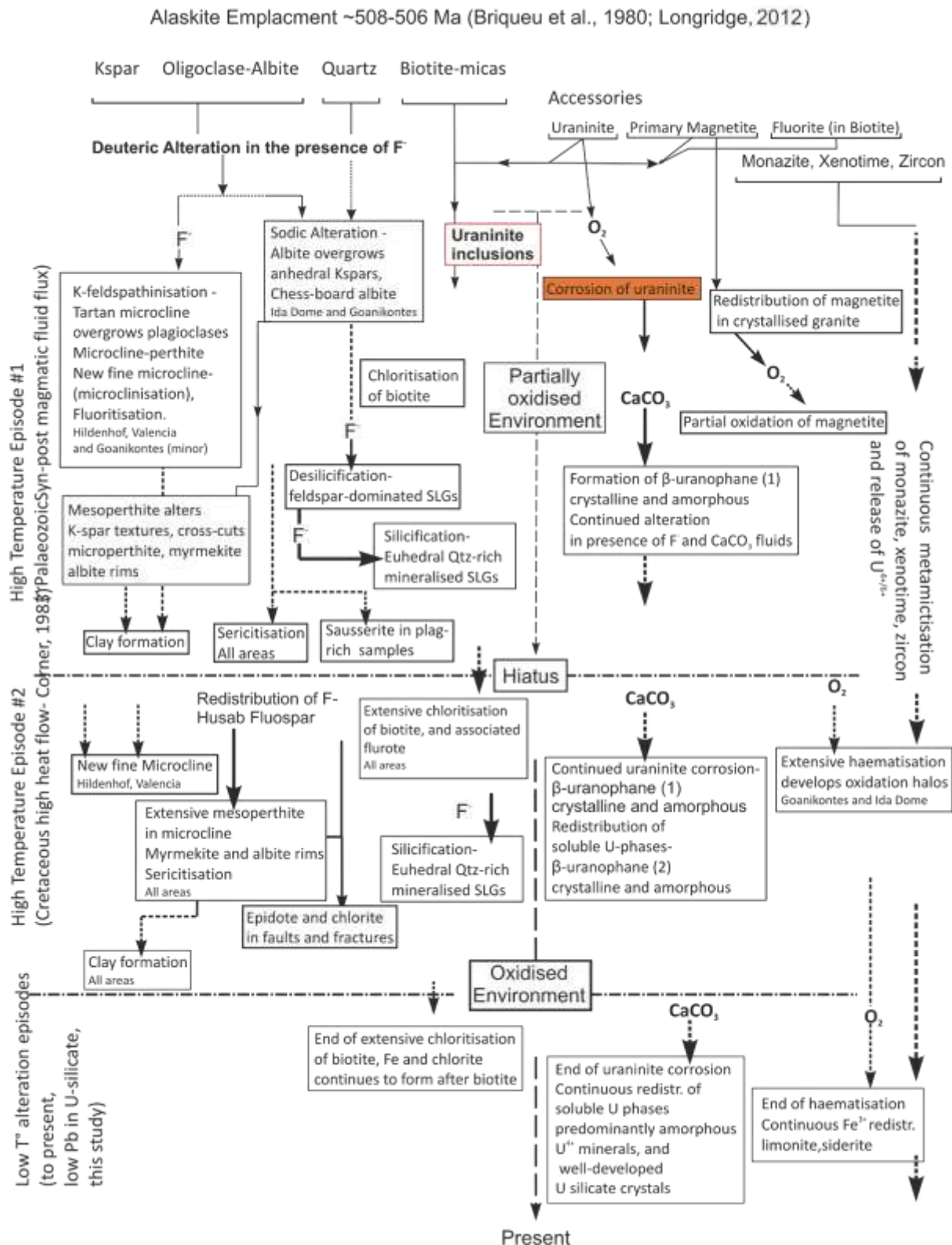
Figure 8.33 Simplified mineralisation sequence for the primary uranium deposits. The scheme splits the sequence into three episodes, the first is initial formation, the intermediate is a period of high heat flow in the Cretaceous and the third is the last period which includes recent geologic time where deposits exposed at the surface are perceived to be altered by oxidising meteoric fluids.
