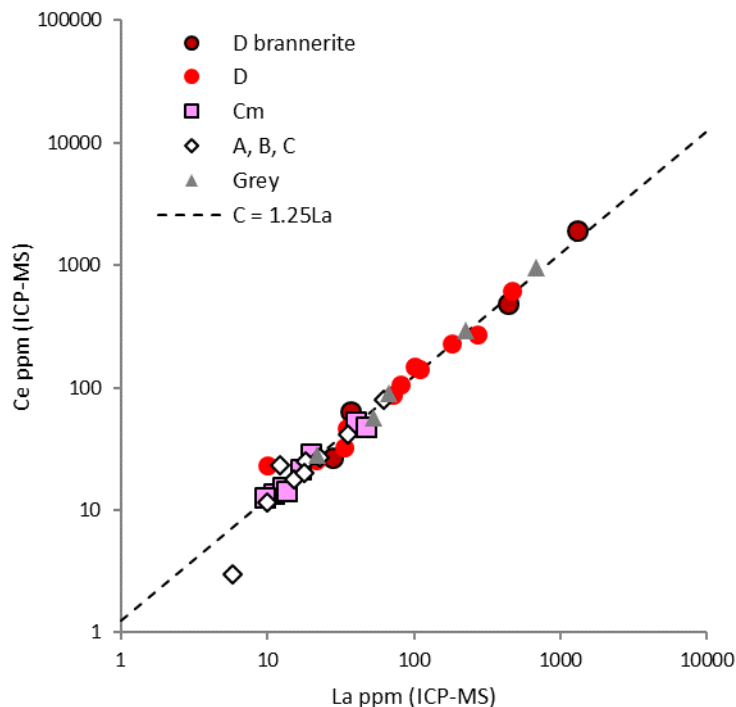
Figure 5.36 Ce vs La of 41 samples analysed by ICP-MS. Ce is consistently 1.25 x La, which is inconsistent with the average of 2:1 in the XRF dataset. A, B, and C types have low HFS abundance, as do the Cm types. The D-type SLGs show a range of HFS abundance but tend to be greater than in the pre-D3 leucogranites.
