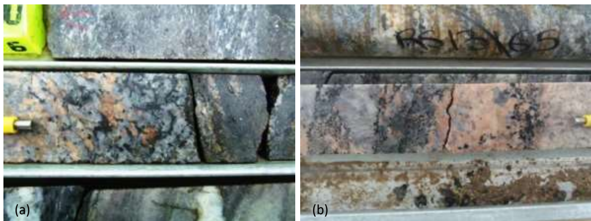
Figure 3.3 Examples of wall rock assimilation in Husab granites. (a) Alaskite contact with Rössing schist, where the contact is characterised by quartz and coarse biotite and elevated CPS, RDD051 - 440 m. (b) Streaks of remnant metasediments in leucogranite, RDD113 - 404 m.
