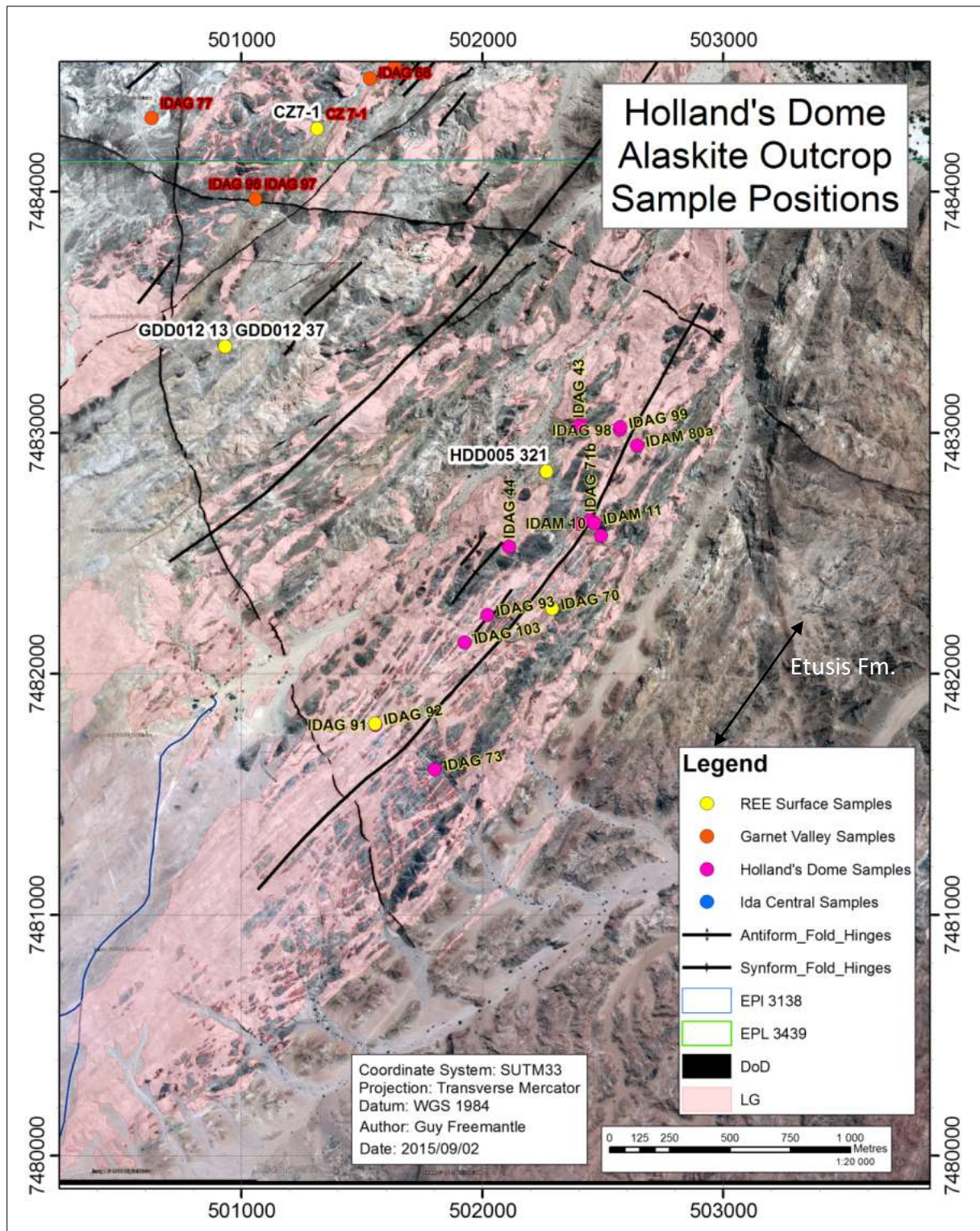
Figure 3.27 Aerial view of the Holland's Dome deposit. The Holland's Dome structure is an antiform, immediately adjacent to the Garnet Valley deposit on the south-eastern flank of the Ida Dome. The Garnet Valley deposit occupies a synform between the Ida Dome and Holland's Dome. The structure is bound by discontinuous marbles of the Rössing Formation at the limbs. Mineralisation occurs above and below the marble units and occurs in association with the calcsilicate-garnet-diopside-amphibole skarn pods. The axial planar-parallel leucogranite sheets (code LG) are conventional, but had to have intruded after folding. Late, Cretaceous dolerite dykes criss-cross the area (code DoD). Drill core samples come from the 'GDD' and HDD prefix samples.
