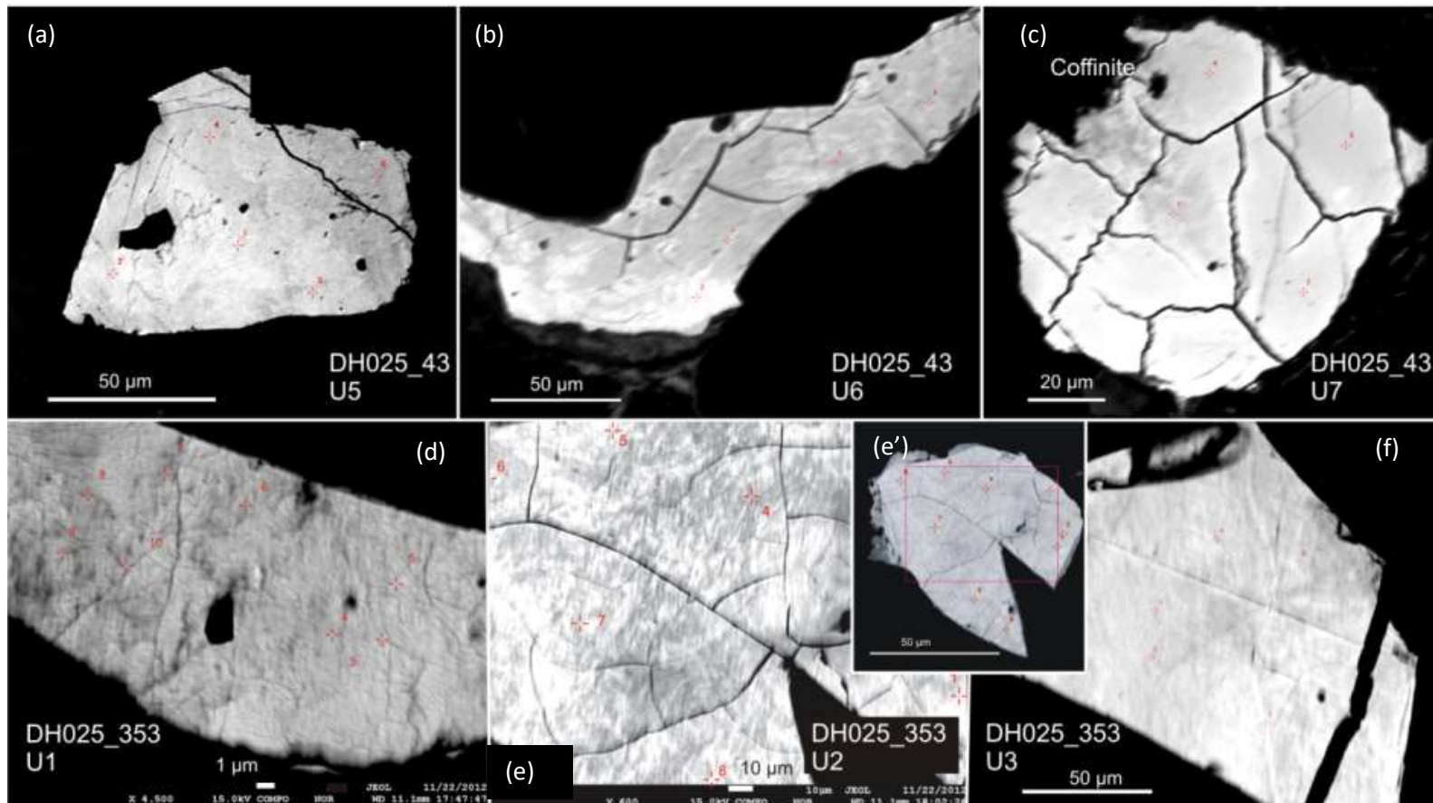
Figure 8.4 Uraninite and coffinite in sample DH025-43m and DH025-353m. (a) Secondary uraninite fills a fracture and is itself altered at one of the edges (bottom). The uraninite is less uniformly dense than U7 DH25-43m: (b) U6 shows fairly uniform density, and is slightly brighter surrounding a void (left). Hairline fractures surround the void, suggesting a metamict, radioactive mineral occupied it and expanded and fractured the host. (c) U7 is an anhedral uraninite, completely replaced by coffinite. It has conchoidal cleavage linked by radial pattern fractures. The grain has particularly uniform reflectance. Backscatter images of selected Etango deposit uraninites. DH025-353m: (d) U1 has a relatively uniform reflectance and is crosscut by a network of hairline fractures. QEMSCAN studies show that calcite predominantly replaces the voids within the Valencia uraninite crystals. (e and e') U2 displays well-developed conchoidal cleavage, typical of crystalline, magmatic uraninite. The grain is coffinitised throughout (dark grey). The missing segment was likely lost during sample preparation. (f) U3 is a euhedral uraninite, which appears to have been octahedral. The reflectance is uniform, with some metal-dense patches showing bright.
