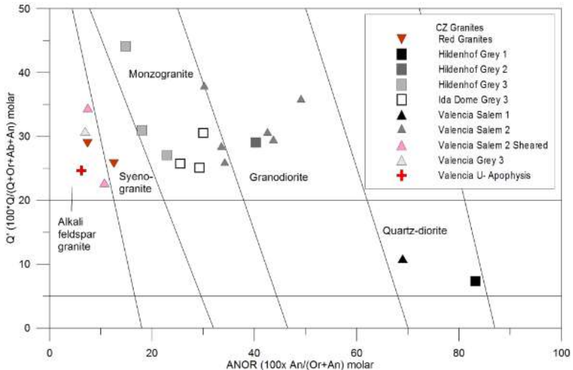
Figure 5.4 Q'-ANOR diagrams of Central Zone uranium deposit granites. Salem and equigranular (Grey and Red) granites at the Central Zone uranium deposits at Hildenhof, Ida Dome and Valencia. The trend from diorite to monzogranite is reflected in successively decreasing mafic content, and increasing K-feldspar proportion observed in petrographic and study.
