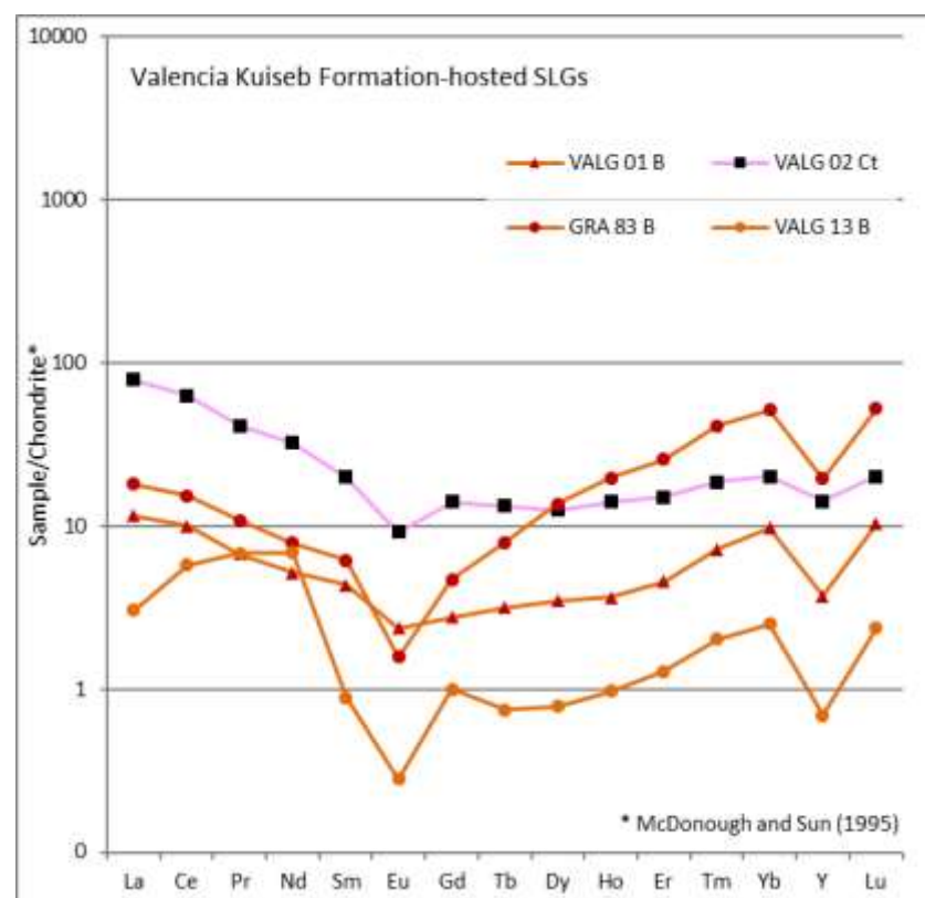
Figure 6.13 The Kuiseb Formation-hosted sheeted leucogranites at Valencia. Garnet- and tourmaline-bearing varieties have enriched HREE abundances, relative to the Khan Formation-hosted leucogranites. The garnet-bearing samples have distinct convex HREE curves, reflecting the garnet abundances in a given sample. The tourmaline sample has -ve slope, relatively enriched LREE and a weak -ve Eu anomaly. The low LREE and Y abundance, in comparison to the Salem granite, reflects low phosphate abundance.
