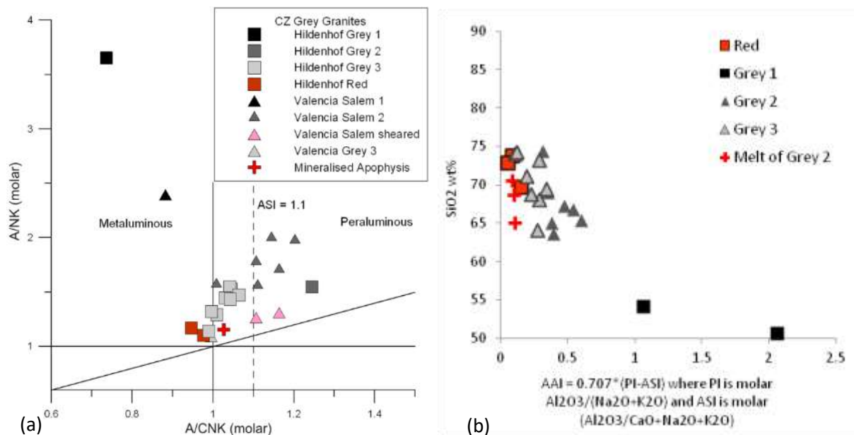
Figure 5.14 Aluminium saturation diagrams of the granite suites at the Central Zone primary uranium deposits. (a) The Grey and Salem type granites plot with successively decreasing peraluminosity between type 2 and type 3 generations. The diorite composition type 1 Grey and type 1 Salem samples plot within the metaluminous field; petrographic observation of abundant plagioclase with >20 % An is reflected in high A/NK and low A/CNK. (b) Alkali-alumina index vs. silica for the Grey and Salem suite samples. The diagram shows the successive decrease in AAI as silica saturation increases. Partial melt in the Salem granites comprise almost entirely K-feldspar and quartz, and plot with correspondingly low AAI.
