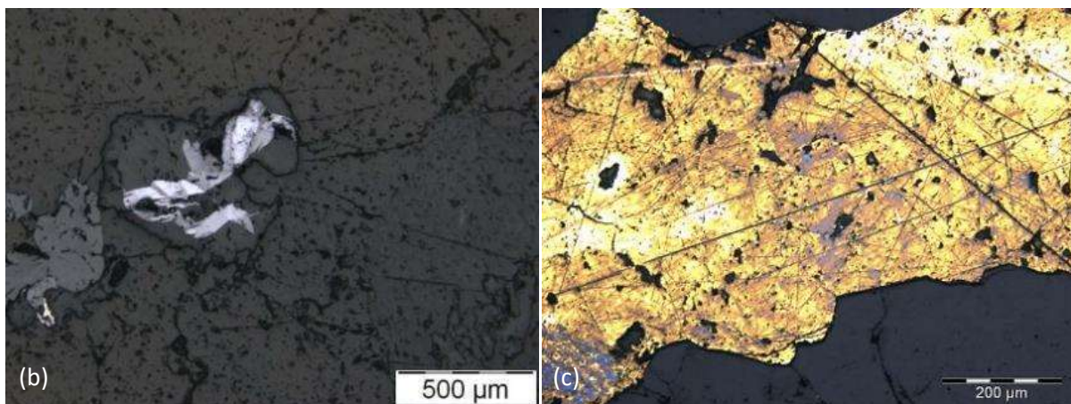
Figure 5.45 (b) Molybdenite surrounds uraninite in Husab leucogranite and (c) chalcopyrite is altered to bornite in an Ida Dome leucogranite. Rössing sample data: Freemantle (2006).
