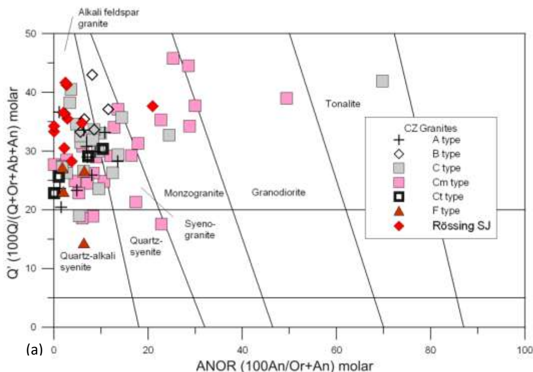
Figure 5.5 Q'-ANOR of the pre- and post-D3 leucogranite type populations of the Central Zone U deposits. (a) Q'-ANOR diagram of pre-D3 sheeted leucogranite from the Central Zone U-deposits. The plot also includes late pegmatite F-type sheets. The majority of the samples are alkali-feldspar granite in composition, exceptions that plot in the monzogranite to tonalite fields are predominantly Ida Dome samples. Rössing sample data: Freemantle (2006).
