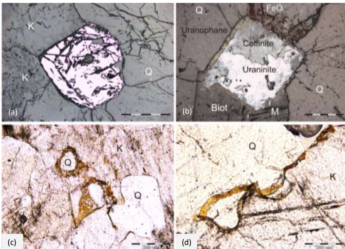
Figure 4.38 Uraninite and uranophane in Ida Dome Leucogranites. (a) Uraninite with radiating cracks in sample IDAG 08. (b) Pyrite/uraninite in an E-type sample IDAG 05; the sample may be pyrite or uraninite or a combination of both. Note FeO denotes a variety of potential hydrated iron oxides, uranophane occurs in the surrounding metamict halo and radiating fractures. (c) Uranophane surrounding globular quartz crystals within altered K-feldspar. (d) Uranophane in a sample from depth (HDD027 104.36-104.70); the secondary mineral permeates along grain boundaries where quartz has intergrown with K-feldspar.
