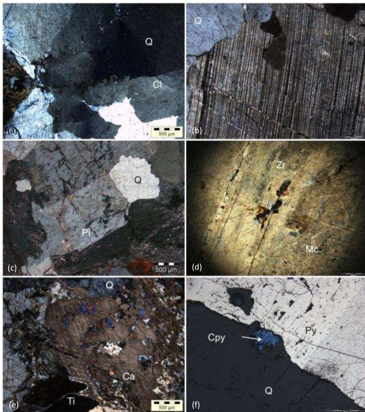
Figure 4.43 Petrographic features of brannerite- and betafite-hosting sheeted leucogranites. (a) Coarse-grained quartz grains with chloritised biotite (left) and chlorite veins along a suture. The worm - like suture and chessboard extinction in the quartz reflect solid - state strain (from deformation). (b) Plagioclase twins with displacement along micro fractures and a quartz rune comprised of multiple crystals (scale bar is 500 \mu\text{m} ). (c) A euhedral plagioclase (Pl) with irregular, sutured boundaries shared with later quartz (Q). (d) Hydrothermal alteration of tartan - twinned microcline, (e) Accessory titanite (Ti) in quartz, with later calcite that has filled a void. The high interference minerals are clinopyroxene. (f) Sulphides are present in coarse pyrite (millimetric) and subordinate chalcopyrite/bornite.
