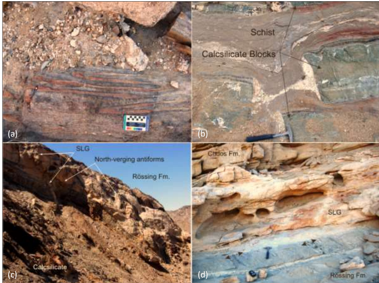
Figure 3.16 Stratigraphic and structural features of the Hildenhof area. (a) Tight folding within ductile carbonates of the Rössing Formation. (b) Brittle and ductile deformation in Khan Formation diopside gneiss. (c) North verging secondary folds in Rössing Formation marble, with bedding parallel SLG. A SLG has also intruded along the axial plane of the antiform. (d) SLG intruding between the Rössing (lower) and Chuos Formations (upper). Note the SLG sheet is at an oblique angle to the dilatational features in the Rössing calcsilicate. Locations: (a) and (c) 489331E 7489434N and (b) and (d) 488824E 7489479N.
