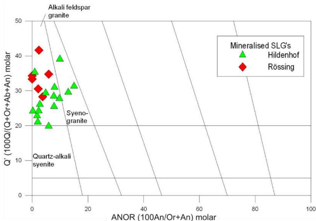
Figure 5.8 Q'-ANOR diagram of Hildenhof mineralised sheeted leucogranite. The majority of the Hildenhof samples are alkali – feldspar granite in composition, quartz content is slightly lower than those sampled at Rössing.
