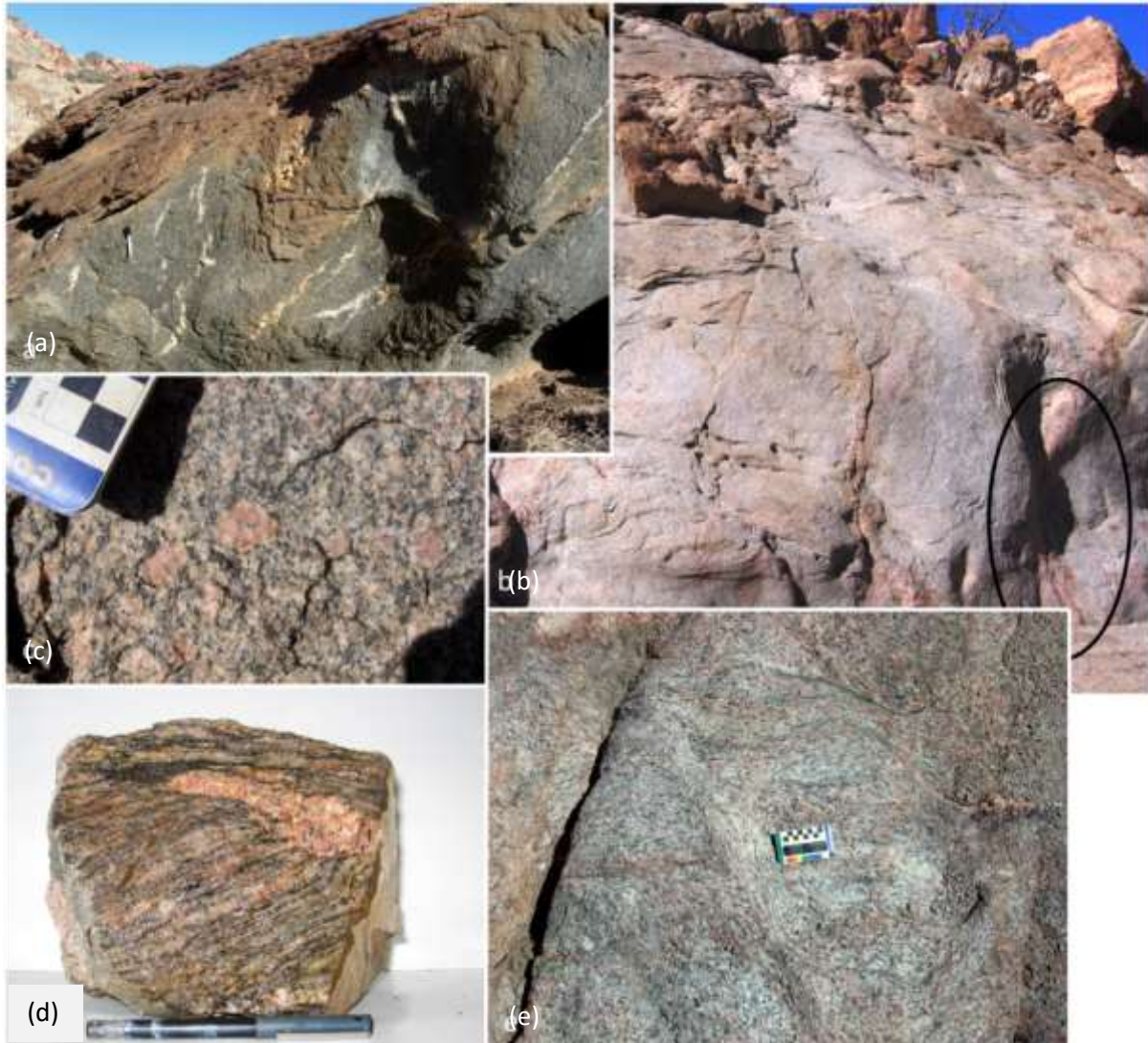
Figure 3.44 Salem Suite granites at Valencia. (a) The first generation of Salem-type granite is characterised by high biotite content and strong foliation. Subsequent quartz-feldspar leucosomes developed sub-parallel to the foliation. Position 524549E 7530330N. (b and c) Salem type-2 with characteristic K-feldspar megacrysts, U-mineralised melt apophyses, circled in (b). Position: 524002E 7528840N. (d) Partial melt vein oblique to foliation in Salem type-2, the sample in picture has elevated U concentrations. Position: 523092E 7530183N. (e) Conjugate shear bands in Salem type-2, the megacrystic granite has been strained to the extent that it has an augen gneiss texture. Note that some of the shear bands are oblique to the gneissic texture. The partial melts tend to have elevated U values. Position: 523113E 7530125N.
