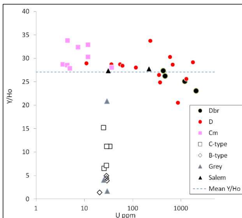
Figure 6.20 U in ppm vs. Non-chondritic Y/Ho of CZ granites. The Cm types plot above the mean for the sample group, while the D-type show considerable scatter, there appears to be a negative trend with respect to U. The brannerite-bearing samples (D br ) plot with a systematic negative Y/Ho relationship with respect to increasing U, with 3 of 4 samples below the mean. The Grey granites, B-type and the C-type SLGs are considerably different to the Cm and D-type SLGs.
