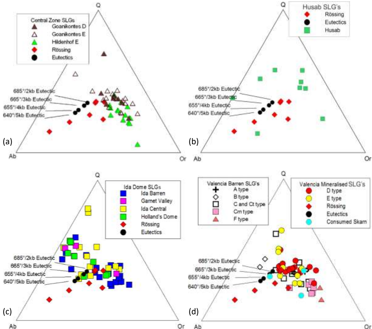
Figure 5.13 Normative orthoclase-quartz-albite ternary plots of sheeted leucogranites of the CZ uranium deposits. (a) Granite ternary system diagram of the Etango (Goanikontes) and Hildenhof mineralised sheeted leucogranites. Q is higher than the Rössing samples and oxidised (open triangles) samples, on average have higher, Q proportions. (b) Granite ternary system diagram of Husab alaskites. Q proportions are higher than the Rössing samples and plot with a broad range of Or. The poor correlation with the expected eutectics compares with the scattered plotting seen on the granite classification diagrams. (c) The granite ternary system diagram of the Ida Dome deposits; mineralised sheeted leucogranites are in colour and weakly mineralised varieties are in blue. The majority of the weakly mineralised samples plot below the eutectics (in terms of Q) with a relatively narrow Ab-Or range. The mineralised sample plot roughly into two groups; one group varies along Ab-Or with a narrow Q range, the other reflects inconsistent composition with very low Or, and have the highest Q content. (d) The granite ternary system diagram of Valencia granitoids. Trends in the successive sheeted leucogranite generations are not clear cut, but the F-type and Cm-type have the highest Or component and the mineralised varieties have higher quartz content overall.
