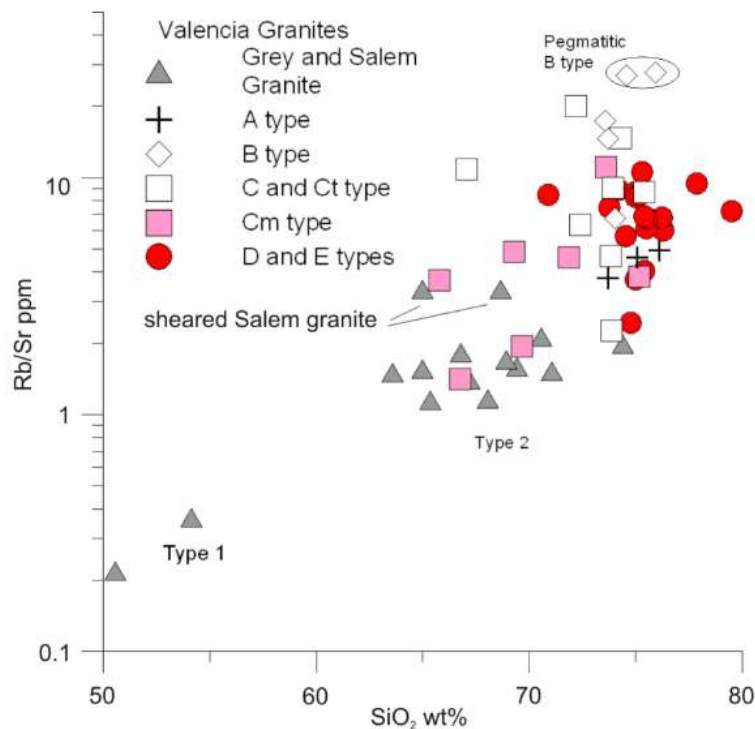
Figure 5.32 Plot of \text{SiO}_2 vs. \text{Rb/Sr} ppm of Valencia and Goanikontes granites. (a) \text{Rb/Sr} plotted against Si content of the Valencia granite suites shows a systematic increase in \text{Rb/Sr} from Salem type syenogranite through Cm-type leucogranites to mineralised varieties. The garnet-bearing types within the Kuiseb Formation have high K-feldspar proportions and a correspondingly high \text{Rb/Sr} , overall the ratio increases with stratigraphic level of intrusion.
