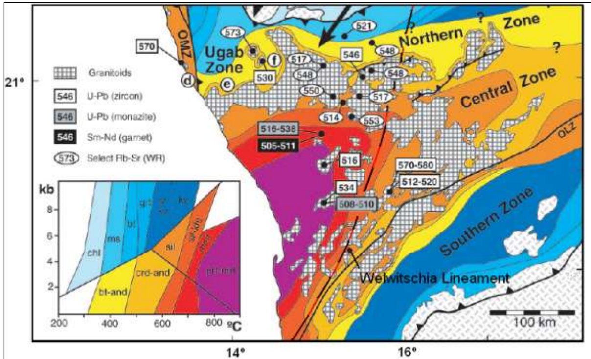
Figure 2.4 Map of metamorphic grades and age date distribution of the western part of the Damara Orogen. The map is a summarised interpretation of Central Zone metamorphic conditions by Goscombe et al. (2003a) after Hoernes and Hoffer (1979). Rb-Sr (whole-rock) and U-Pb zircon ages are magmatic. The Welwitschia Lineament is added, and shows that the majority of metamorphic assemblages west of it are in the upper amphibolite to granulite facies.
