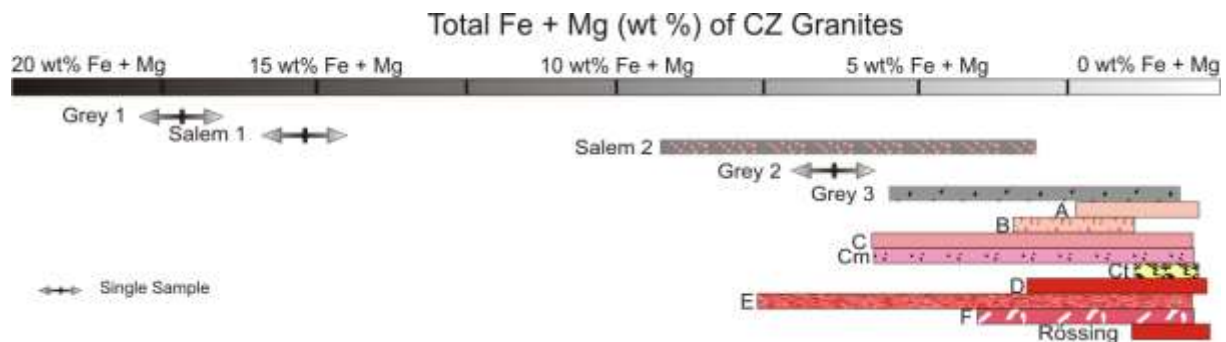
Figure 5.22 Total \text{Fe}_2\text{O}_3 + \text{MgO} (wt.%) of Central Zone granites. The Grey and Salem granites show a decrease in Fe and Mg with decreasing age. C type (except Ct varieties) and E-type (oxidised and haematite stained) sheets, have the broadest range of total Fe + Mg content.
