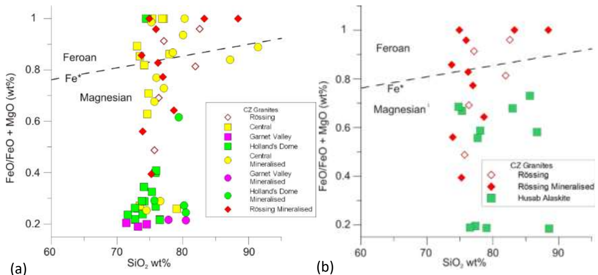
Figure 5.21 \text{Fe}^* vs. \text{SiO}_2 diagrams of the leucogranite suite at the Ida Dome and Husab. (a) \text{Fe}^* vs. \text{SiO}_2 diagram of mineralised and weakly mineralised Ida Dome sheeted leucogranites. There is a clear difference between the Ida Central, Garnet Valley and Holland's Dome samples; Ida Central samples plot close to Rössing samples with high \text{Fe} - \text{Mg} ratios. Holland's Dome samples have higher \text{Fe} - \text{Mg} ratios due to greater interaction with \text{Fe} and \text{Mg} skarn minerals. (b) \text{Fe}^* vs. \text{SiO}_2 diagram of Husab alaskites. The Husab data set has a range of \text{Fe}^* from <0.2 to \sim 0.7 and plots in two distinct populations, with no apparent relationship to \text{U} content.
