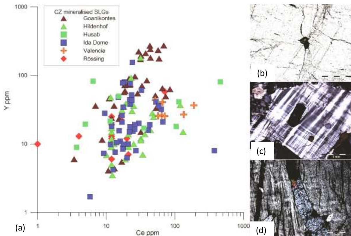
Figure 5.37 Ce and Y content of mineralised sheeted leucogranite and photomicrographs of phosphate minerals. (a) Y and Ce ratios are only weakly systematic, illustrating a variable abundance of monazite and xenotime. The relatively high Y/Ce ratio of the Goanikontes samples for example suggests xenotime is the dominant phosphate, in addition to apatite. Valencia contrasts with comparatively few samples hosting Y above 5 ppm. The weakly linear trend in the Ida Dome samples indicates that xenotime and monazite are present. (b) Xenotime and zircon between quartz and microcline, ppl, DH25 334.99-355.45. (c) Apatite is a prominent P-bearing phase and does not hold significant lanthanides or Y, xpl, HILG 22. (d) The Valencia deposit has samples of apatite >3 mm long but relatively little xenotime.
