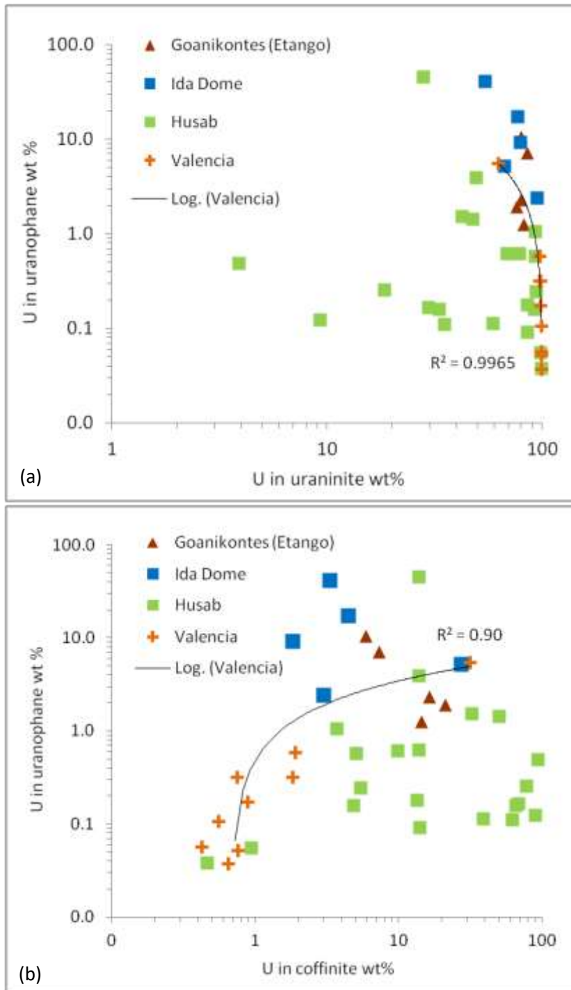
Figure 7.28 Uraninite, coffinite, and uranophane phase distribution and relationships of the Central zone primary deposits. (a) U-deportment in
