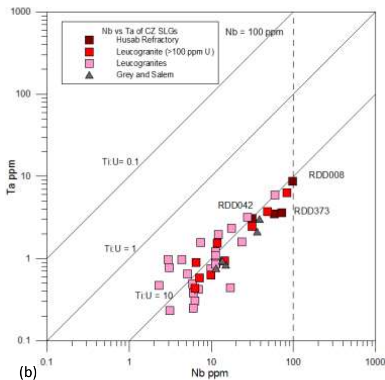
Figure 5.51 (b) Ta vs. U shows that four of the seven most Ta-enriched samples are refractory mineral-bearing. Th
