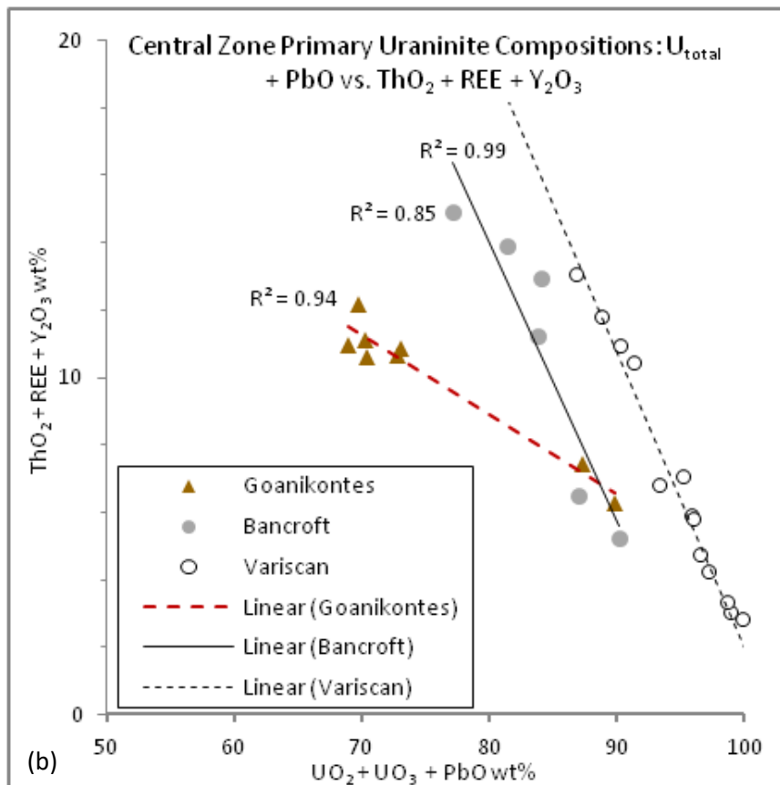
(b) Calculated U oxide total + PbO vs. \text{ThO}_2 + REE + Y: The Central Zone uraninite populations (except Goanikontes) show a weaker indication of systematic substitution by Th REE and Y. Comparative samples from the Variscan and Bancroft studies of Förster (1999) and McKechnie (2012) respectively.
