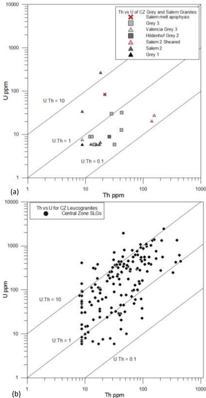
Figure 5.47 Plots of Th vs. U of Grey, Salem, and uraniferous leucogranite suites of Central Zone U deposits. (a) Th vs. U of Grey- and Salem granites. Most samples have little or no detectable U, but range from 10 ppm- to ~200 ppm Th. Some Salem granites are enhanced by secondary U in the Joly Zone and so plot in similar positions to the mineralised apophysis. Rössing mine sample data: Freemantle (2006). Data clipped to >9 ppm U and >9 ppm U.
