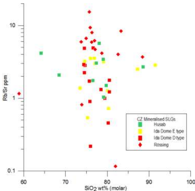
(b) \text{SiO}_2 vs. \text{Rb/Sr} in D and E-type samples from the Ida Dome and Husab deposits. Alaskite samples from the Rössing deposit are included for comparison. D-types show a slight negative \text{Rb/Sr} with Si increase. Husab samples show no relationship between the ratio and Si. E-types of the Ida Dome area seem to be in two groups, one with \text{Rb/Sr} > 3 and the other with \text{Rb/Sr} < 2 . Both areas have \text{Rb/Sr} significantly depleted relative to the comparative samples at Rössing. Rössing sample data: Freemantle (2006).
