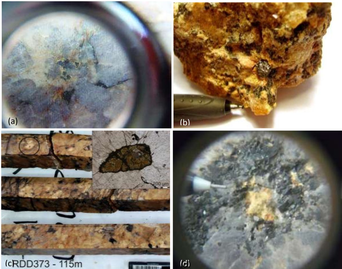
Figure 1.2 Photographs illustrating primary, secondary, and refractory uranium minerals specimens. (a) Uraninite cluster in coarse- textured, uraniferous sheeted leucogranite (alaskite). Note the halo of yellow secondary U minerals, scale: uraninite grains <1 mm, Husab Deposit. (b) Uranophane/boltwoodite in a vug between cubic fluorite, hydrothermally altered, uraniferous sheeted leucogranite (alaskite) Husab Deposit. (c) Brannerite from the Rössing SH Deposit and (d) 1.6 mm betafite grain from the Husab Zone 1 Deposit. In the Husab example Betafite grows across a quartz-feldspar grain boundary. Images from a- Freemantle (2011); and b- Freemantle (2006).
