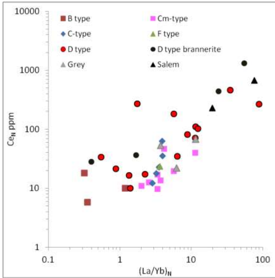
Figure 6.17 LREE fractionation trends of selected CZ granites. The B-, C-, and Cm-types host relatively depleted Ce, but a marked contrast in light-rare earth fractionation exists for B-types, and more oxidised Cm-types. The Grey granites are potentially related to the Cm-types on the basis of similar Ce abundances and light - heavy rare earth fractionation.
