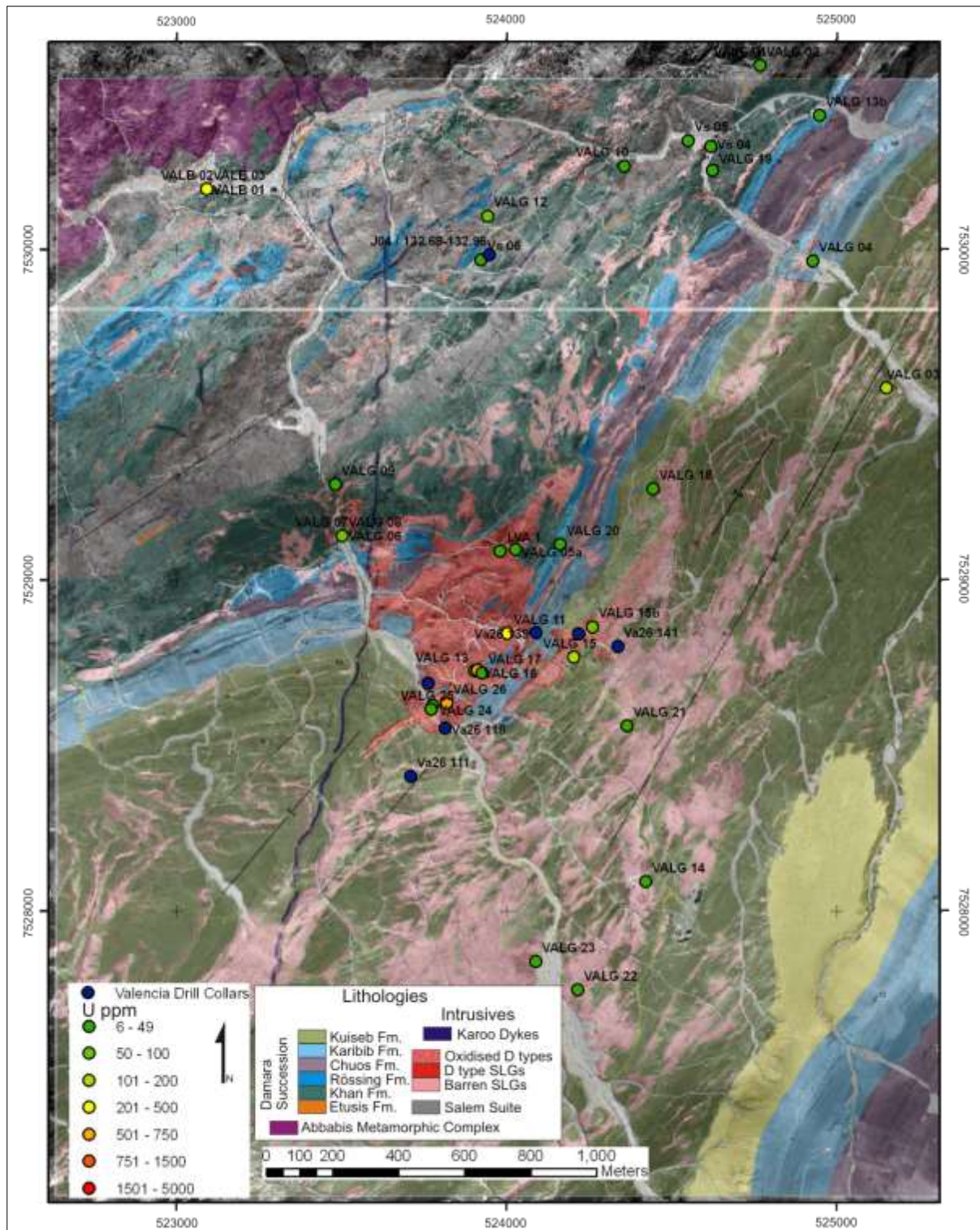
Figure 4.6 Valencia Hand samples and drill core collar locations on Valencia EPL 1496. U values are in ppm (by XRF) as indicated in the legend. Blue circles represent drill-hole collar localities. Lithological interpretation and coloration are from mapping during 2007 and 2008 and the underlying ortho-photo and contour lines are courtesy of Valencia Uranium Ltd.
