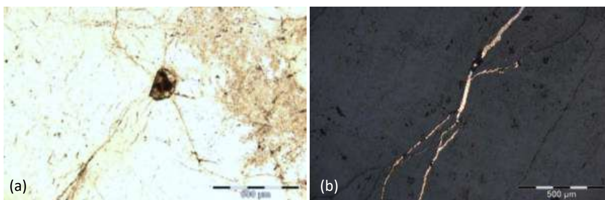
Figure 4.36 Uranium mineral associations in core specimens from HDD025. (a) Zircon is a common accessory mineral in sheeted leucogranites and many examples host uraniferous inclusions. The anhedral crystal may be an entrained component rather than a primary phase. Radioactive decay results in metamictisation and volume expansion, which is accommodated by the surrounding radiating fractures, HDD27 104.36-104.70, ppl. (b) The Khan Formation is locally cupriferous. Chalcopyrite veins that crosscut the leucogranites preserve the resulting Cu-sulphide mobilisation during granite emplacement, HDD027 122.90-123.22, rfl.
