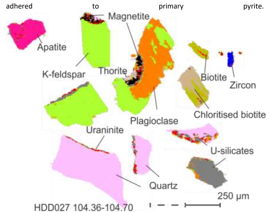
Figure 7.11 (b) 104.36-104.70. Uranium occurs in uraninite inclusions hosted by zircon, apatite, biotite and Fe-phases (magnetite). Uraninite is also on the surfaces of rock-forming minerals with uranium silicates (coffinite). Uraninite has also crystallised on the surfaces of coarse-grained coffinite. (c) Mineral map features of HDD 122.90-123.22 from Ida Central. Note that U-silicates may refer to uranophane or coffinite, as the analysis at the SGS laboratory does not discriminate between the two on the mineral maps.
