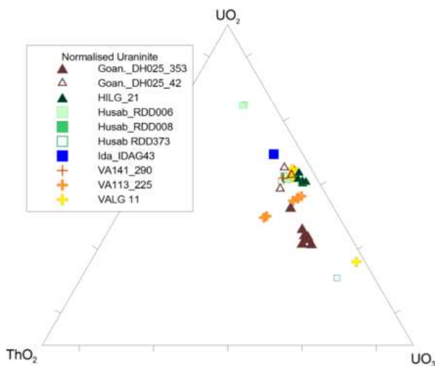
Figure 8.1 Uranium and thorium ternary diagram of 43 uraninite specimens from selected Central Zone primary deposits. \text{U}^{4+}/\text{U}^{6+} varies between deposit areas; Etango samples from DH353 and from Holland's Dome have the highest \text{UO}_3 ratios, most of the specimens have ~10 wt.% \text{ThO}_2 and 40 wt.% to 50 wt.% \text{UO}_3 . Valencia specimens returned the lowest average \text{ThO}_2/\text{U}_{\text{tot}} analyses of the sample set. All data are normalised from calculated oxide proportions.
