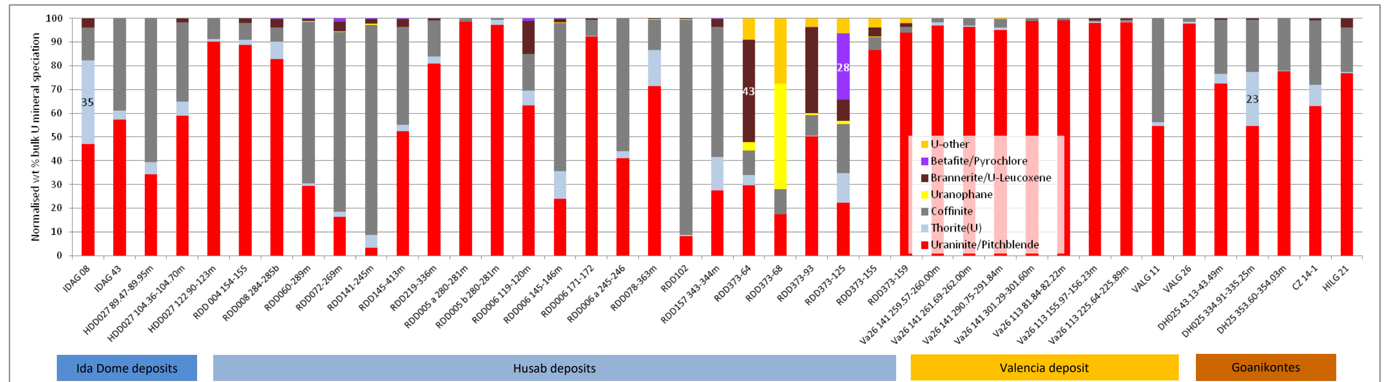
Figure 7.2 Uranium-mineral speciation charts of samples from the Central Zone primary uranium deposits. Uraninite is the dominant phase at most deposits. Thorite is present in all samples, as are coffinite and trace proportions of uranium-bearing refractory minerals (betafite and brannerite). Secondary uranium silicates (boltwoodite and uranophane) are not recorded in some analyses, thus their proportion is unknown, however, secondary U-silicates are always present in sample analyses that included secondary U calibration. In some sample analyses, the laboratory excluded coffinite/uranophane differentiation in speciation analyses, but discriminated between the two in the deportment calculations (The Goanikontes, Ida Dome and Valencia sample sets for example).
