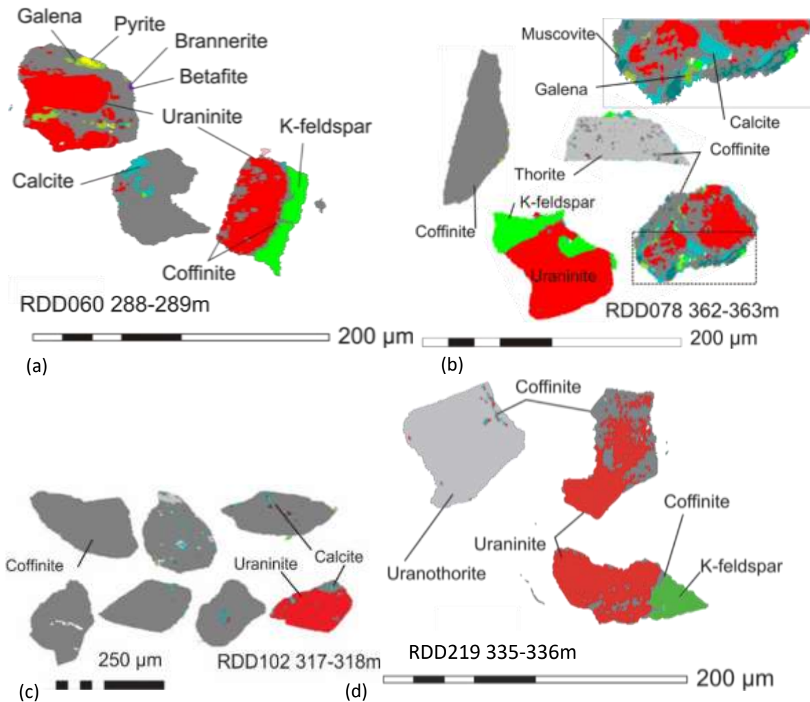
Figure 7.15 QEMSCAN mineral maps of uraninite and coffinite textures in Husab Zone 1 and Zone 2 samples. (a) Compound grains of uraninite replacement by coffinite with associated brannerite and sulphides. Galena is likely to be a product of radiogenic lead mobilisation from altered uraninite. Coffinite forms as inclusions in impure uraninite and at contact margins with K-feldspar. (b) Compound grains and fractured uraninite, illustrating aggressive replacement of uraninite with accessory sulphides. Thorite hosts uraninite and coffinite inclusions, and uraninite fills cavities at a K-feldspar contact RDD078 362-363 m. (c) Examples of coffinite in sample RDD102-318m. Uraninite is a minor phase, and is variably- to completely replaced by coffinite. The coffinite also contains thorite inclusions, potentially remnants of solid solution. (d) Primary uraninite overgrown- and replaced by coffinite, and primary uranothorite with coffinite fill in fractures, RDD219-336 m. Coffinite occurs as a replacement mineral and as a fill in fractured uranothorite as well as at the contact between uraninite and K-feldspar.
