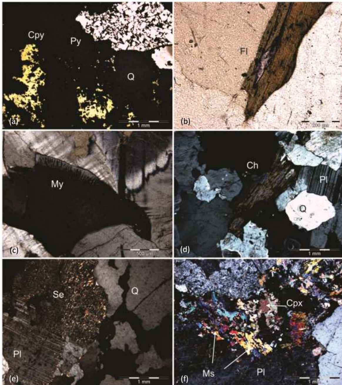
Figure 4.35 Features of mineralised samples with skarn and host rock interaction. (a) Large clusters of skeletal chalcopyrite (Cpy) and inclusion-rich pyrite (Py) are common minerals in sheets that intrude the upper Khan Formation, HDD027 122.90-123.22, rfl. (b) Fluorite is present in skarns (Husab) and is only present with biotite in thin section, HDD027 104.36-104.70, ppl. (c) Myrmekite growth at plagioclase rims is a common feature in the barren sheeted leucogranites but significantly less so in the mineralised sheets. Fluid interaction between skarns and sheets at the Ida Dome would provide suitable conditions for its growth, HDD027 104.36-104.70, xpl. (d) Anhedronal quartz and plagioclase are not unusual in altered sheeted leucogranites, this sample also has entrained, chloritised biotite (Ch) HDD027 89.47-89.95, xpl. (e) Variable temperature alteration episode(s) results in sericite growth (Se) in plagioclase (Pl) adjacent to a euhedral quartz veinlet, IDAG 10, xpl. (f) CPX is scarce but present in the samples with skarn interaction, IDAG 03, xpl. Ida Dome Ore Mineral
