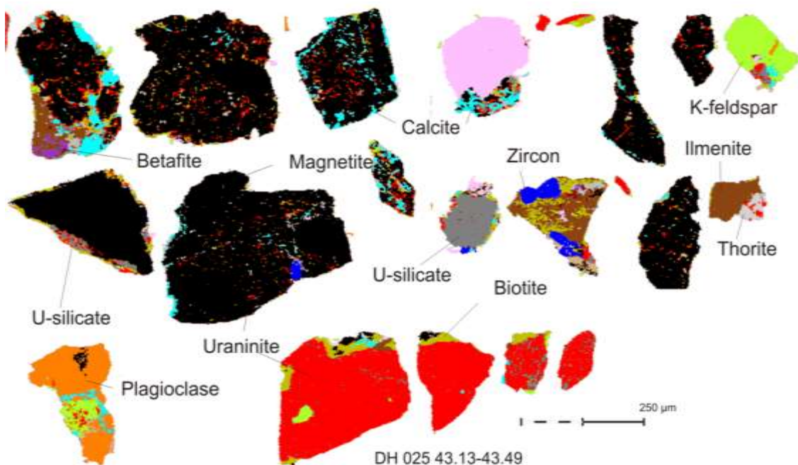
Figure 7.5 Mineral map features of DH025 43.13-43.49 from the Etango Deposit at Goanikontes. Note the coarse-grained, euhedral primary uraninite and fine-grained uraninite replacement of Fe-oxides. There are two textures; one of uraninite-calcite replacing the mobile Fe constituent of magnetite, the other of uraninite forming coatings with coffinite on magnetite surfaces.
