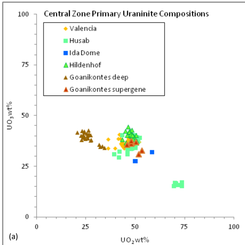
Figure 8.3 Four binary plots of uraninite compositional variables, U oxides, Th, REE and Y, Ca, and Si. (a) Calculated \text{UO}_2 vs. \text{UO}_3 . The plot highlights a range in \text{UO}_2 of 35 wt.% to 65 wt.% for most samples whereas the Goanikontes samples plot with lower \text{UO}_2 , and comparable, slightly higher \text{UO}_3 content. The anomalies with high \text{UO}_2 are from hole RDD008, and the particular uraninite is fractured.
