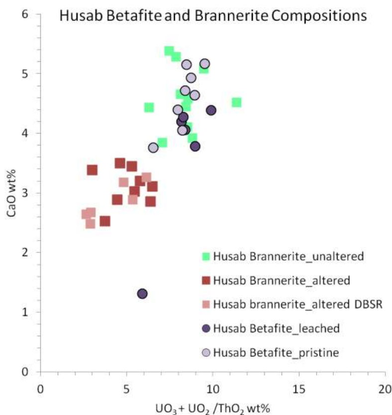
Figure 8.32 UO_3 + UO_2 / ThO_2 vs. CaO wt.% from analyses of betafite and brannerite from drillhole RDD373. CaO tends to be in lower abundance in the altered portions of the betafite. The altered brannerite at 64 m has lower CaO relative to the unaltered specimen at 93 m. The leached portions of the altered brannerite host the lowest concentrations of CaO. (DBSR:- dull backscatter reflectance). Overall there is a positive correlation between U content and CaO, and this trend is consistent when comparing analyses of altered and unaltered specimens.
