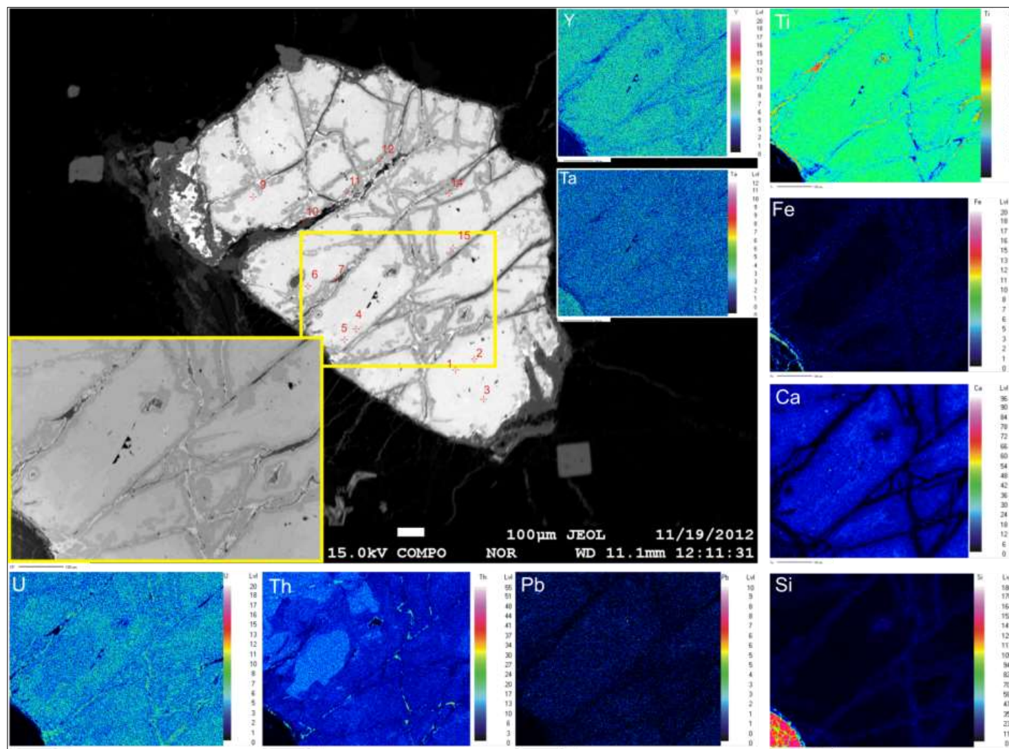
Figure 8.24 Mineral map of a detailed area in an altered brannerite specimen. Backscatter brightness shows metal leaching along the grain edges and along the prominent fracture network, which served as the fluid pathways. U in brannerite is predominantly U^{6+} thus soluble in a high T environment. Uranium shows an inverse distribution, though faint, U appears to concentrate in the fractures, as a secondary precipitate. Correspondingly, Th shows an inverse distribution to U. Si and Fe concentrate along the fractures, while Ca does not appear in the fractures, and concentrates in variable concentration in the less disturbed portions of the specimen. Y shows a fairly uniform distribution in the undisturbed portions of the mineral, but is leached along some edges.
