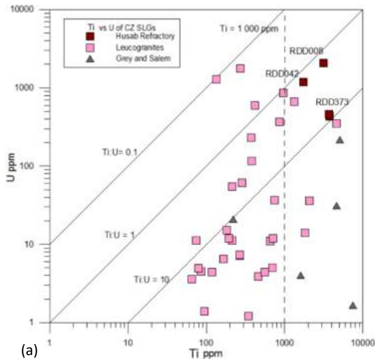
Figure 5.51 Plots of Ti vs. U and Ta vs. U for the ICP-MS samples. (a) Twelve samples contain >1000 ppm Ti; four are early, mafic -bearing grey and Salem granites, and four are leucogranite/alaskite. The remaining four are all betafite-brannerite bearing leucogranites from the Husab Zone 1 deposit. Ti is always >U and ratios range from ~2:1 to ~5 000:1 for Grey granites or ~200:1 for leucogranite.
