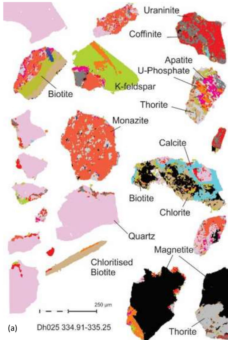
Figure 7.6 Mineral map of DH025 334.91-335.25 and DH025 353.60-354.03 from diamond hole 25 at the Etango deposit, Goanikontes. There are two contrasting styles of uranium mineralisation. (a) The 334.91 m sample contains uraninite as fine-grained inclusions in monazite, and as adhered components of euhedral magnetite. The sample also contains coarse uraninite, with variable coffinite replacement. (b) Uraninite is coarse and shows varying degree of replacement by coffinite. The coarse grains also show conchoidal fracture, along which coffinite is a replacement texture. Conchoidal fracture is typical of magmatic, crystalline uraninite. (Grain U2 is analysed by EPMA).
