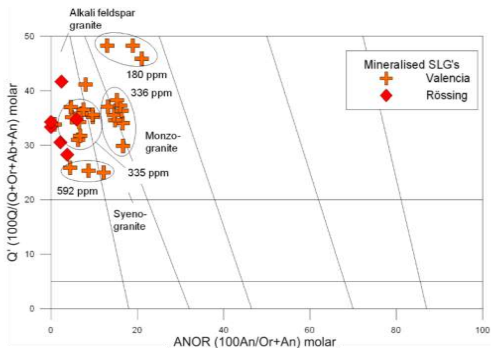
Figure 5.11 Valencia mineralised sheeted leucogranites. Samples tend to plot with Q' < 40 and ANOR < 20 . The circled clusters highlight mean U values in ppm. The highest average grade samples from Valencia have similar Q' to the Rössing samples, and plot near the alkali-feldspar field. Rössing sample data: Freemantle (2006).
