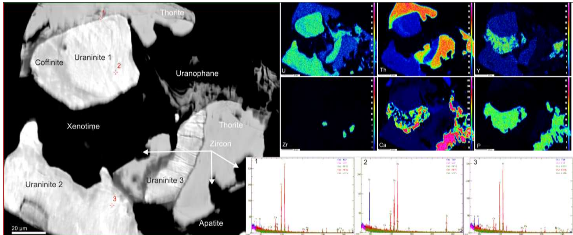
Figure 8.8 Composite mineral grains from sample DH025_353 m. The composite grain in backscatter shows a clear density contrast between thorite and uraninite. WDS scans at positions 1 through 3 confirm the two minerals. The mineral maps of U, Th, Y, Zr, Ca and P identify the following phases in the cluster; Uraninite in two textures, one as a euhedral grain '1' and as a replacement grain '2'; Thorite as anhedral grains, after zircon; and Xenotime, which appears to have inter-grown with apatite (co-incident P and Ca vs P and Y).
