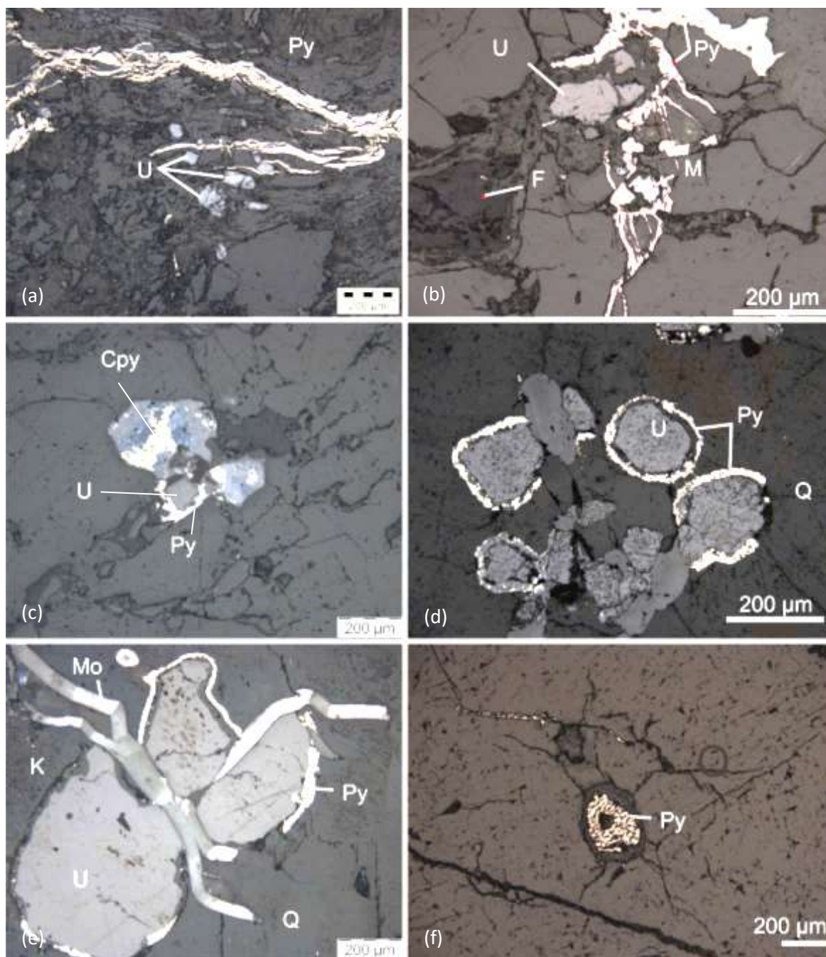
Figure 4.46 Sulphide and uraninite textures in the Husab sheeted leucogranites. (a) Pyrite veins cross cut a nest of coarse biotite that hosts a cluster of euhedral uraninite, RDD373 154-155C, rfl. (b) Net-texture pyrite veins propagate into inter-granular spaces and through fractures in quartz. Late fluorite, chlorite, and epidote surround the uraninite, RDD373 92-93A (c) Chalcopyrite is often in solid solution with bornite. A halo of coffinite (dull reflectance) surrounds the immediate edges of the uraninite, and pyrite surrounds the coffinite, RDD193 267-268b, rfl. (d) A cluster of altered uraninite with rounded edges surrounded by pyrite halos; some uraninite is in direct contact with pyrite, while coffinite and iron-oxides occur between uraninite and pyrite in others, indicating multiple episodes of alteration, RDD219 335-336 m, rfl. (e) Uraninite, some with coffinite-
