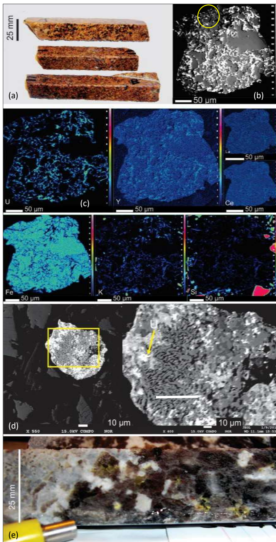
Figure 8.7 Uranium and magnetite relationships in Etango drill hole DH025 samples at 43 m and 353 m. (a) The shallow intersection of alaskite at 43 m, shows pervasive Fe-staining from limonite and siderite. Feldspars are all altered and original colour appears to have been white. (b) Backscatter image of a corroded magnetite. Secondary uranium minerals fill vermicular voids, which register their higher density (metal-content) as bright shades. (c) A collage of U, Y, La, Ce, Fe, K and Si element maps of the magnetite grain. U, Y, K and Si correspond, suggesting boltwoodite. Ce, La, and Y are coincident, supporting phosphate mobilisation in the subsolidus environment. (d) Backscatter image of a corroded magnetite with vermicular voids partially filled by uranium minerals at the rim of the grain. (e) The yellow halos of uranophane/ boltwoodite that surround the magnetite porphyroblasts appear to be the product of magnetite-hosted uraninite corrosion. Their composition is likely to be a combination of boltwoodite and uranophane, given the presence of K in the surface sample.
