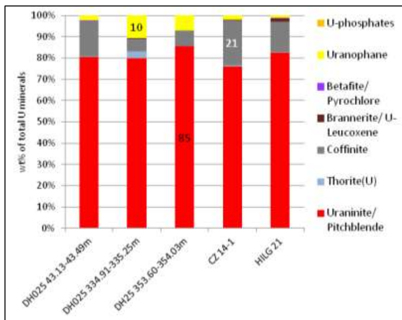
Figure 7.9 Uranium deportment statistics of Goanikontes and Hildenhof samples. Uraninite is the dominant mineral, followed by coffinite as the dominant secondary mineral in two of the core samples and both of the surface samples
