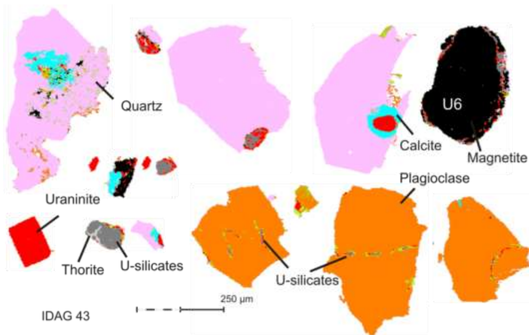
Figure 7.13 Mineral map features of IDAG 43 from Holland's Dome. Key textures are the replacement of the rim of magnetite by uraninite-coffinite (specimen U6 is analysed by EPMA), coffinite deposition along feldspar cleavage planes, euhedral uraninite, and calcite replacement of uraninite rims. This sample is an example of euhedral magmatic uraninite, and secondary uranium-mineral crystallisation within microstructures of the rock-forming minerals.
