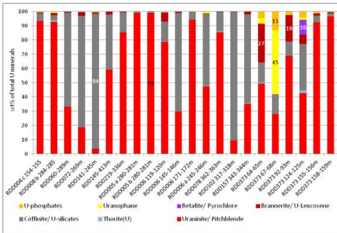
Figure 7.14 Uranium deportment of the Husab QEMSCAN samples from Zone 1 and Zone 2. Seven of the samples have U-deportment in coffinite > uraninite, with appreciable uranophane in a single sample, RDD373 67-68 m. Uranium mineral compositions are determined by EPM in samples RDD006 171-172; RDD008 284-285 m; RDD373 64-65 m, 92-93 m, 124-125 m.
