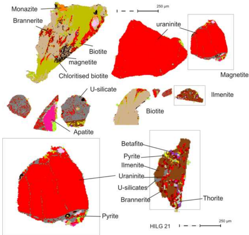
Figure 7.8 Mineral map features of HILG 21. Brannerite, betafite, uraninite and coffinite, and thorite deposit as secondary in rutile/ilmenite. Apatite is surrounded by uraninite-coffinite, indicating a secondary crystallisation around the phosphate. The sample shows primary uraninite in variable stages of coffinitisation, with some grains nearly completely altered to U-silicate.
