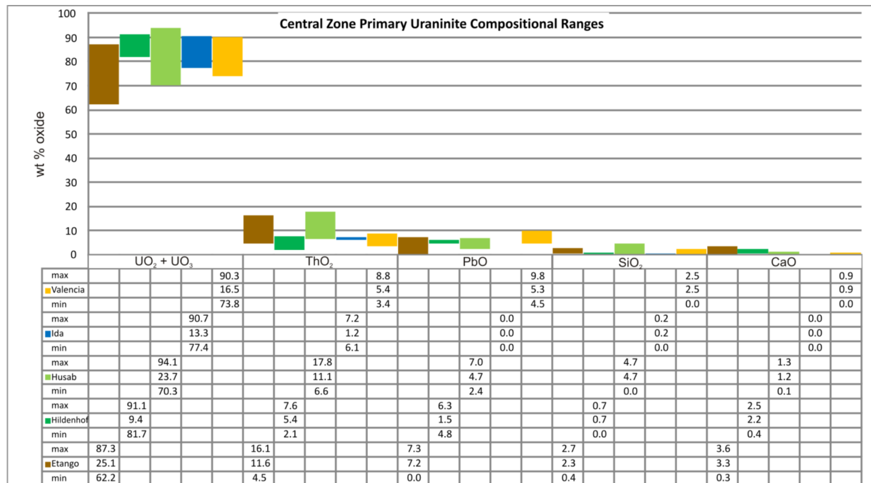
Figure 8.2 Compositional ranges of primary uraninite specimens from the Etango, Hildenhof, Husab, Ida Dome, and Valencia localities. As with the ternary diagram a few subtle compositional variations suitably discriminate between the uraninite populations at each deposit. Total U content is relatively low in the Goanikontes samples. Th in the Goanikontes samples is comparable to Husab, while Valencia, Hildenhof and Ida all have narrow ranges. High relative Pb content sets Valencia apart. High Si in some Husab samples sets the population apart from the other deposit's uraninites. Ca is relatively low in all sample populations. The narrow ranges of U, Th, Pb, Si, and Ca of the Hildenhof specimens shows that the individual uraninite grains are all very similar or have been altered to the same extent in the particular sample set.
