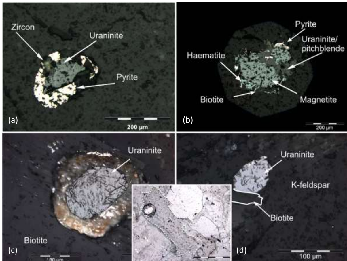
Figure 4.52 The common primary uranium mineralisation textures and ore mineral associations in Valencia alaskites. (a) Valencia leucogranites contain disseminated uraninite and zircon. Pyrite surrounds one of the uraninite grains and replaces the alteration halo that surrounds the uraninite in the host K-feldspar, Va26 111 157.44-157.82, rfl. (b) Uraninite and magnetite association in the Valencia sheeted leucogranites. Amorphous uraninite/pitchblende has formed between two magnetite porphyroblasts, surrounding a fine grain of pyrite. A second generation of pyrite-chalcopyrite overgrows the compound grain on one side, Va26 111 157.44-157.82, rfl. (c) Uraninite is often hosted in biotite, in primary deposits throughout the Central Zone. Most radioactive inclusions are very fine-grained, occasionally coarse >100 μm grains form. Radiation damages the surrounding mica structure, facilitating pyrite-magnetite and clay replacement, Va26 141 301.29-60, rfl. (d) Uraninite is late in the crystallisation sequence at Valencia, in Va26 141 261-62 a uraninite shares a common edge with biotite, indicating the temporal relationship between biotite (if entrained, the biotite is older) and mineralisation (younger uraninite), rfl.
