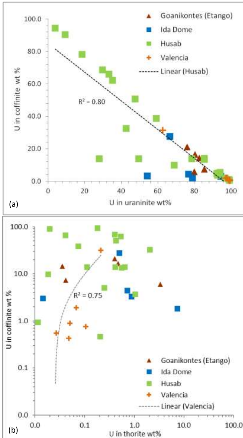
Figure 7.27 Uraninite, coffinite, and thorite phase distribution and relationships of the Central zone primary deposits. (a) Uraninite and coffinite show a systematic, negative correlation, coffinite replaces uraninite in Goanikontes and Husab samples. Husab samples deviate from the trend where uranophane hosts >1.5 wt.% of the U budget.
