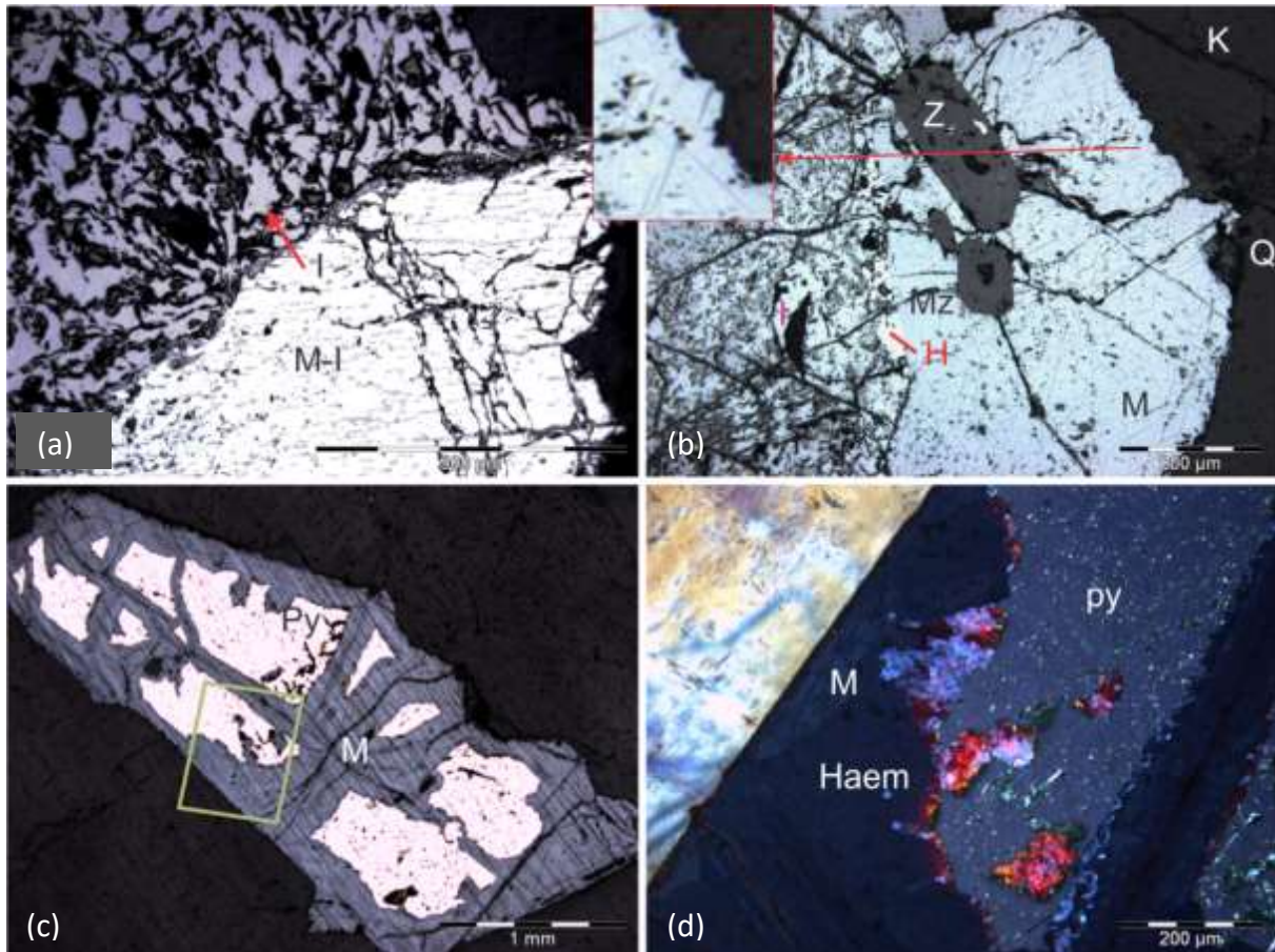
Figure 4.20 Magnetite-haematite-ilmenite and sulphide textures in Central Zone leucogranites. (a) Magnetite with ilmenite in a C-type leucogranite at Goanikontes: Note the exsolution lamellae are in a single orientation, parallel to {111}. The single direction is a result of resetting during deformation. Haematite has exsolved from ilmenite, and subsequently leached out, leaving deformed triangular voids. DH022 59-59.24 20 x ppl– rfl. (b) Ilmenite-haematite-magnetite oxidation replacement textures in uraniferous leucogranite: Note ilmenite in two directions in the undeformed magnetite (M) and the thickest part of the lamellae at the grain boundary. The replacement of ilmenite (I) by haematite produces high-Fe haematite (H) between the ilmenite- and magnetite-dominated grains. The magnetite-ilmenite compound hosts euhedral, primary zircon (Z) and monazite (Mz). DH019 71.74-72.18, 20 x ppl– rfl. (c) Fractured pyrite surrounded by magnetite-haematite, 10 x ppl - rfl. (d) Enlarged area of (c); magnetite and haematite, with prominent red, internal reflections, VALG 08, 20 x, xpl - rfl.
