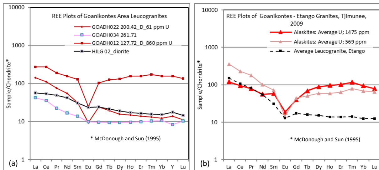
Figure 6.5 REE plots of leucogranite samples from the Etango Deposit at Goanikontes. (a) Data of samples of the Etango deposit core, and a single hand specimen from Hildenhof. Two alaskite samples, one with a high grade (860 ppm U) and the other low grade (61 ppm U) both show pronounced -ve Eu anomalies. The higher-grade sample is enriched in LREE and HREE relative to the other samples. The sample from hole 034 is a Khan Formation - hosted magnetite Cm-type, and shows a negative slope of low concentration REE's. The diorite sample from Hildenhof shows a consistent, shallow negative slope.
