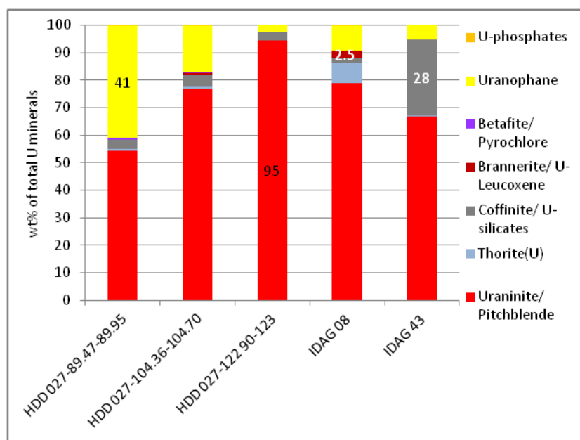
Figure 7.10 Uranium deportment of the Ida Dome QEMSCAN samples. The core samples show a systematic decrease of uranophane/ uraninite with depth. Brannerite is detected in the two deeper Ida Central core samples, and the surface sample (IDAG08) which hosts a maximum of 2.5 wt.% U. The compositions of uraninite-, coffinite-, and thorite are determined by EPMA analyses for samples from IDAG 43.
