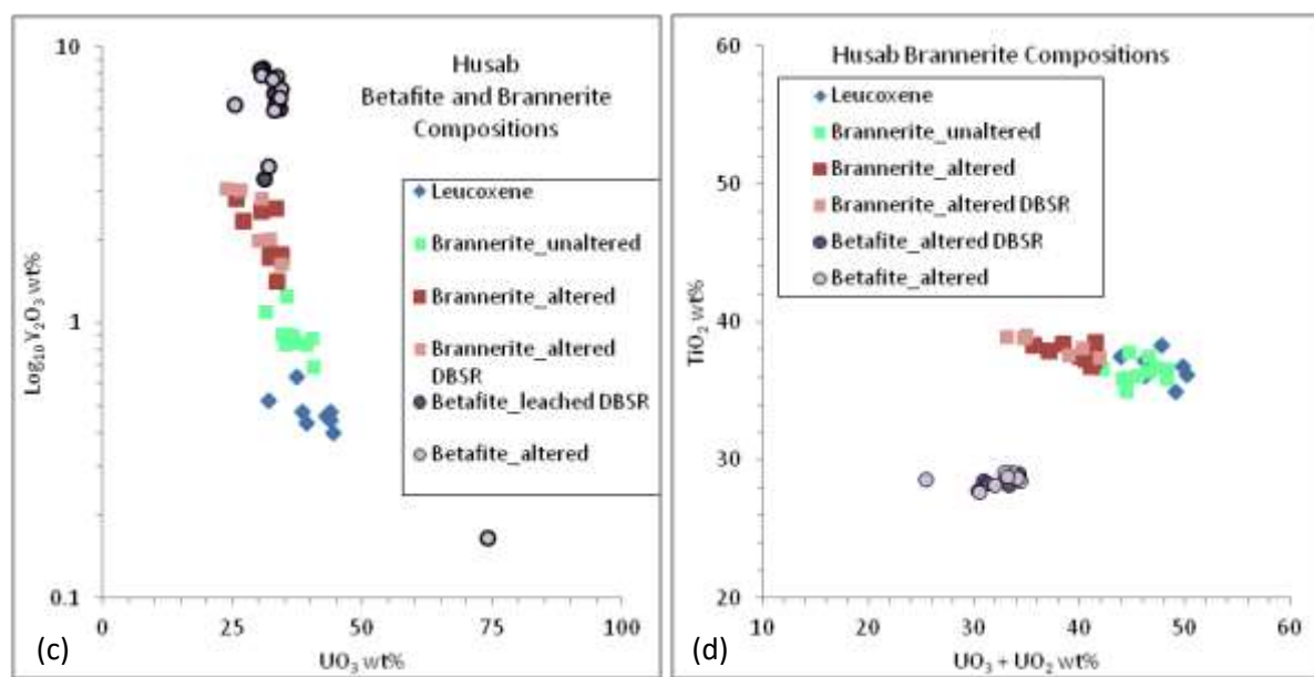
Figure 8.28 Bivariate plots of betafite and brannerite compositions. Plots represent individual sample points on single specimens of each mineral. Key: DBSR = dull backscatter reflectance, (a) \text{UO}_2 vs. \text{Ti}/\text{Fe} of brannerite and leucoxene. Although leucoxene is not a recognised mineral structure, high Ti low U phases are relatively common in the brannerite-bearing samples. The \text{Ti}/\text{Fe} ratio is comparatively high with respect to the ratios in the altered and pristine brannerite. (b) U and Th abundances in brannerite, leucoxene and betafite are mineral-specific; relative Th abundance is higher in the altered brannerite than in the unaltered variety, calculated \text{UO}_3 is comparatively higher in leucoxene than in other minerals. The refractory nature of betafite is evident in the clustered plots of altered and unaltered portions of the specimen. (c) Y abundance in the betafite grain discriminates it from the brannerite. Y is also more abundant in the altered brannerite than the unaltered specimen; the linear correspondence with \text{UO}_3 suggests a substitution relationship. This is also apparent in the unaltered specimen. (d) \text{U}_{\text{total}} vs. \text{TiO}_2 of Husab betafite and brannerite; the two minerals show contrasting relationships between U and Ti abundance, betafite is positively correlated while the altered brannerite in particular shows a Ti increase with corresponding U decrease.
