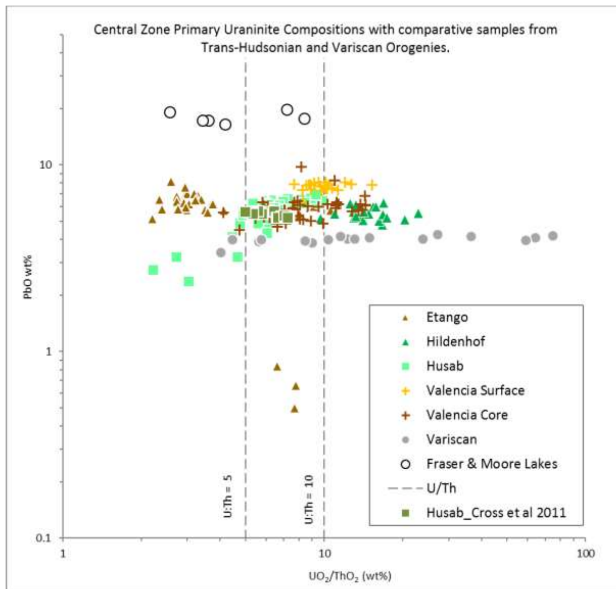
Figure 8.30 \text{UO}_2/\text{ThO}_2 vs. PbO of Central Zone uraninite. The ratio should remain fairly constant unless alteration affects REDOX conditions and oxidises immobile U(IV) to U(VI). The U/Th ratio shows similar trends of increasing Pb with increasing U/Th in the Damara and Bancroft district samples, except in the Goanikontes samples. The Valencia core samples have a great range in \text{UO}_2/\text{ThO}_2 which may reflect oxidation of immobile U and subsequent leaching during alteration.
