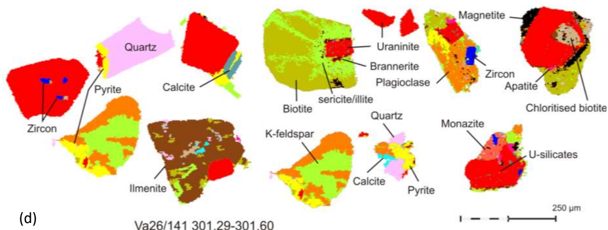
Figure 7.24 (d) Uranium mineral textures and associations of Va26 141 301.29-301.60. Uraninite is euhedral and is associated with biotite, chlorite, phosphates (monazite) ilmenite and zircon. Sulphides are particularly abundant in this leucogranite sample hosted by banded - mottled Rössing Formation gneiss. Pyrite is the major sulphide, and is accompanied by molybdenite in one of the specimens. An early generation of uraninite occurs as euhedral inclusions in feldspar, while a later generation of uraninite contains inclusions of zircon and biotite. Degradation of the host phases surrounding uraninite alters K-feldspar and biotite to clay, voids surrounding the uraninite have been filled with Fe-oxides.
