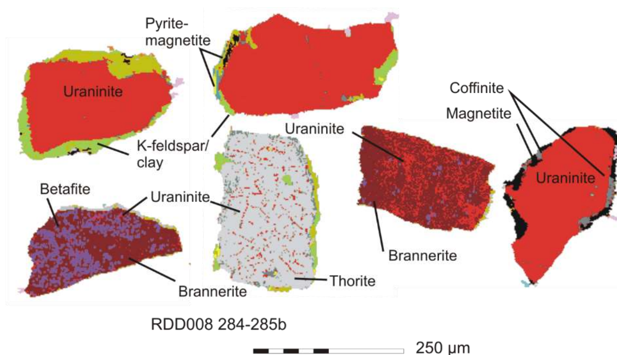
Figure 7.30 Primary uraninite-thorite-brannerite-betafite relationships with mobile U. Primary uraninite is euhedral and of magmatic origin, it is usually hosted within feldspar or quartz, and rarely within a single-phase host. Secondary uraninite occurs within primary brannerite and betafite, showing cleavage or fracture-controlled distribution from the outside inward. Uraninite in thorite however, is a product of solid solution, where excess U forms uraninite within thorite, with no uraninite at the grain boundaries.
