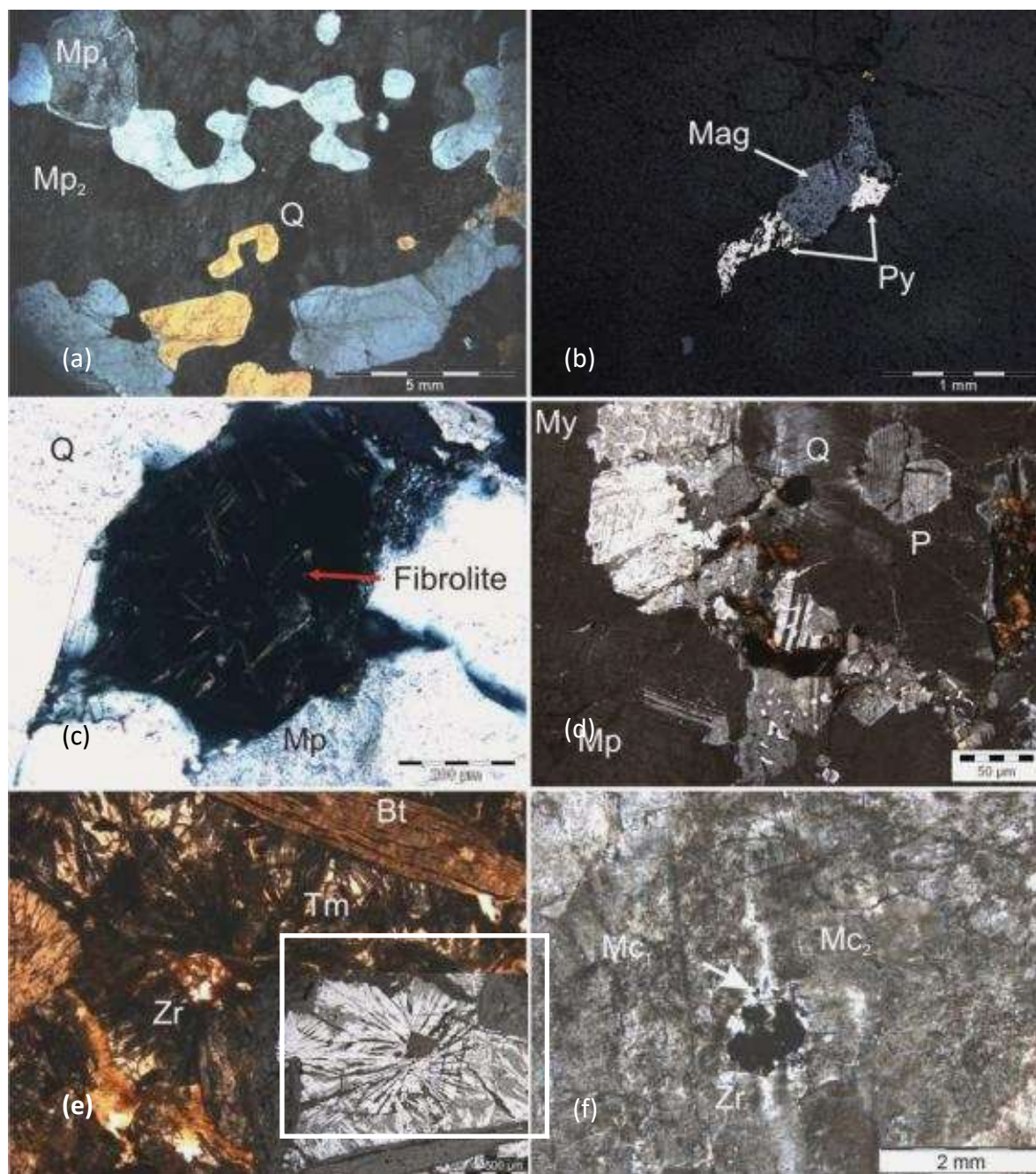
Figure 4.17 Examples of common sheeted leucogranites of the Husab Deposits. (a) Typically, the weakly mineralised granites are feldspar - dominated, and quartz tends to form as singular runes. Secondary processes have formed albite rims around older microcline-perthite feldspars (Mp1) RDD008 284-285 A, xpl. (b) Accessory phases include sulphides and iron oxides in disseminated microscopic clusters and singular crystals, typically at grain boundary junctions, RDD008 284-285 m A, rfl. (c) Certain accessory phases indicate a metasedimentary source; mineral textures such as fibrolite occur in granites that intrude peraluminous metasediments, RDD004 154-155 m A, ppl. (d) Albite rims surround sodic feldspar (P) inclusions in strained quartz (Q) and myrmekite has developed in larger clusters of plagioclase, RDD373 115-116 m, xpl. (e) The distinguishing accessory phase, tourmaline occurs in clusters with mafic entrainments (biotite) with zircon at the nucleus of the radiating cluster, RDD373 115-116 m, ppl - xpl inset. (f) Extensive microclinisation (Mc2) of K-feldspars (Mc2) dominates the barren, tourmaline granites, the source of hydrothermal fluids are the intruding alaskites, and accessory phases include zircon clusters, RDD351 328-329 m, xpl.
