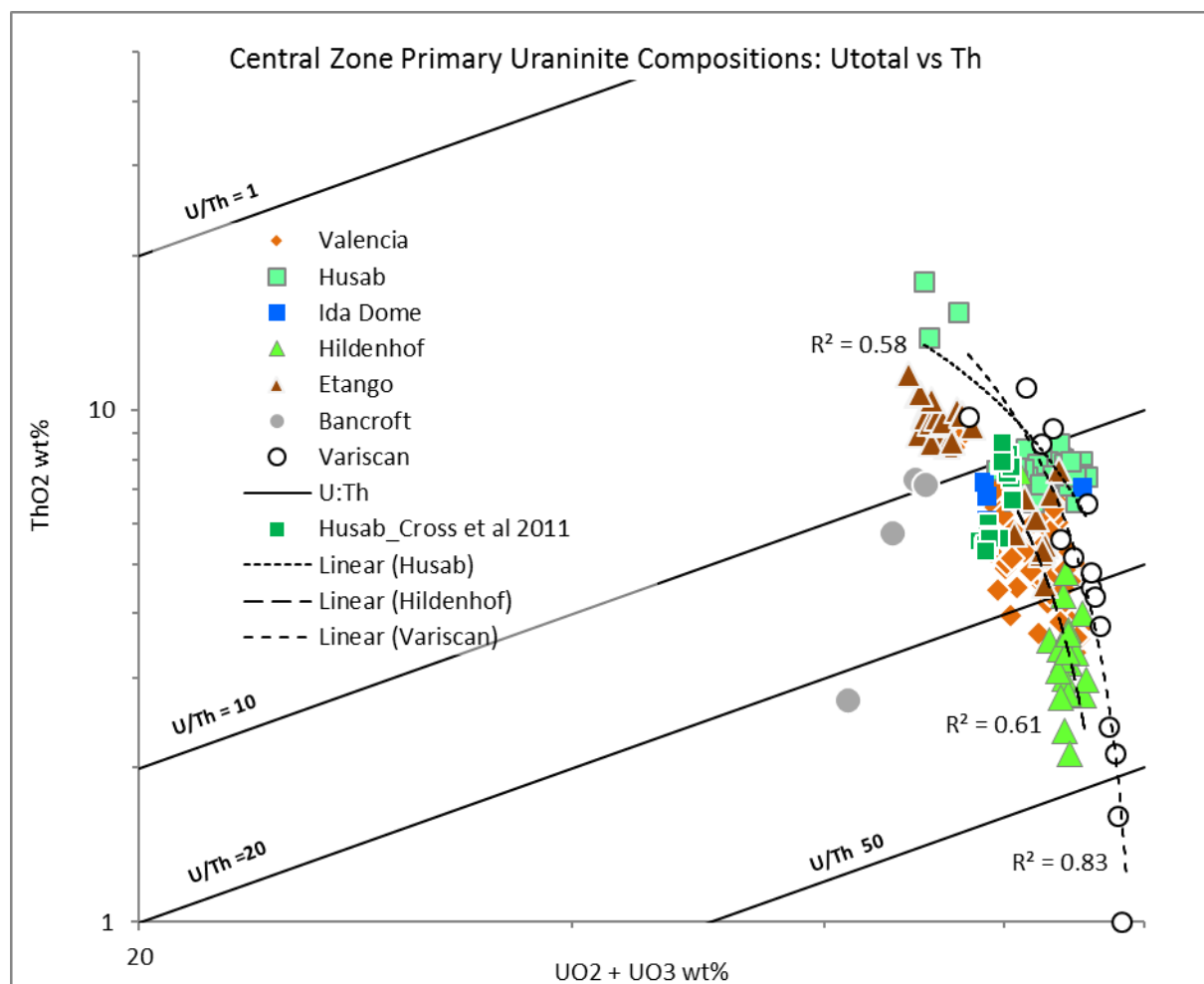
Figure 8.20 \text{U}_{\text{tot}} vs. \text{ThO}_2 wt% in uraninite of the Central Zone primary uranium deposits, with comparative orogenic granite-hosted uraninites. (a) U total vs. Th of the Central Zone (CZ) deposits, Fraser and Moore Lakes prospects near Bancroft, Canada, and Variscan uraninite populations from the Czech Republic. U:Th ratios in the Etango samples, most of the Husab, Ida Dome, and Valencia samples plot with comparably low U/Th ratios, close to \text{U}_{\text{tot}}/\text{Th} = 10 . Although U totals in the Bancroft district specimens are relatively low, the \text{U}_{\text{tot}}/\text{Th} is comparable to the CZ. The Variscan sample set shows a strong linear relationship of decreasing Th/U with increasing \text{U}_{\text{tot}} , spanning a full range of ratios from U:Th = 10 to U:Th = 96. The Hildenhof uraninites have the highest U/Th of the CZ groups; the Valencia specimens cluster with ratios between 10 and 20, while the samples from Etango have bimodal distribution on either side of the U:Th = 10 line.
