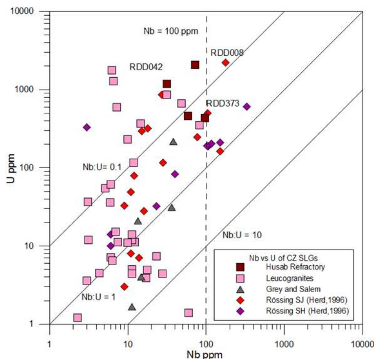
Figure 5.50 Nb vs. U for ICP-MS samples. The plot shows that Nb is a reasonable diagnostic tool for the identification of refractory – bearing alaskites. The four brannerite (+betafite) bearing samples (Husab Refractory) plot with higher Nb relative to the leucogranite and grey granite sample set. Though the majority of samples plot with <25 ppm Nb, the known refractory samples all contain >25 ppm Nb. All data are obtained by ICP-MS.
