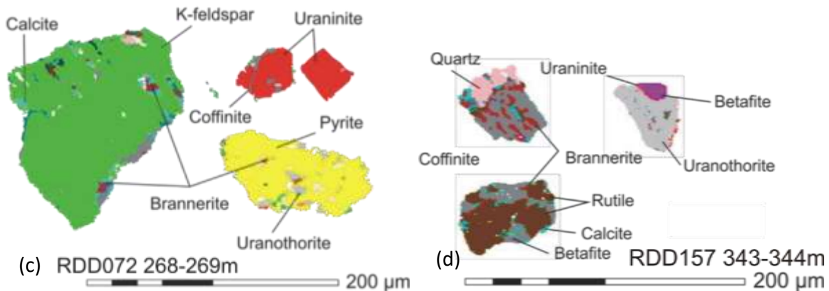
Figure 7.16 (c) Examples of U-remobilisation in RDD072 268-269 m. Altered K-feldspar hosts cleavage-controlled coffinite-brannerite-calcite and skeletal pyrite hosts brannerite and uranothorite-coffinite inclusions. Coffinite fills fractures within uraninite- note euhedral shape of the primary uraninite. (d) Ti oxide relationships with coffinite in the RDD157 343-344 m sample. Brannerite is replaced by cleavage-controlled coffinite, and coffinite replaces anhedral rutile/ilmenite. Betafite occurs in contact with thorite, with associated secondary uraninite.
