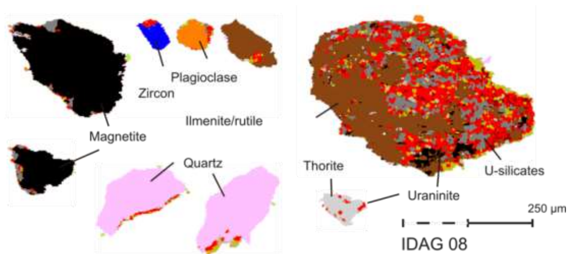
Figure 7.12 Mineral map features of IDAG 08 from Ida Central. Note the coarse-grained ilmenite with uraninite-coffinite replacement. Fine-grained, uraninite-coffinite forms coatings on quartz and magnetite surfaces. The textures in this sample reflect late crystallisation of uranium minerals on the surfaces of the rock-forming and accessory Fe-Ti oxides.
