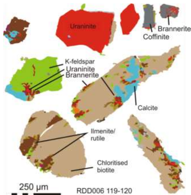
Figure 7.19 QEMSCAN derived mineral maps illustrating uranium mineral textures of RDD006 specimens. RDD006 119-120 m, euhedral uraninite with examples of unaltered, full- and partial coffinite replacement. Uraninite, ilmenite and brannerite occur between biotite sheet, and within K-feldspar.
