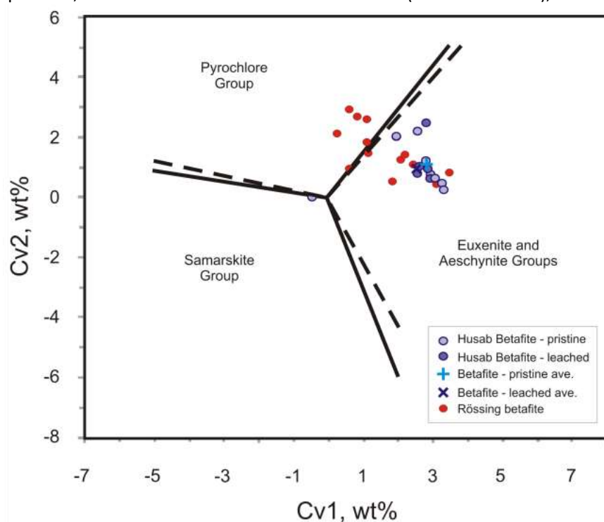
Figure 8.26 Normalised cationic proportions of Husab betafite and Rössing Mine betafite. The Husab data are sourced from 7 spot analyses on 'pristine', unaltered zones of a 1.2 mm betafite (lavender circles), and 6
