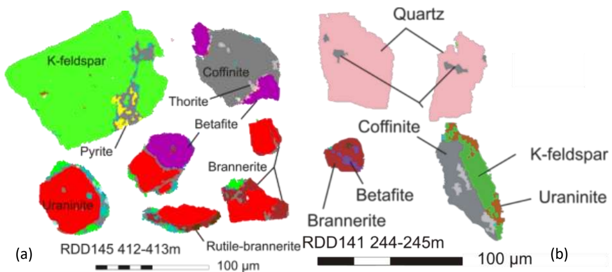
Figure 7.16 QEMSCAN mineral maps of uranium mineral textures in Husab Zone 1 and Zone 2 samples. (a) Betafite relationships with coffinite and uraninite in sample RDD145 412-413 m. Betafite occurs with coffinite and has quartz at the contact margins. Coffinite surrounds betafite and uraninite, replacing the contact margin between the two minerals. In the same sample, euhedral uraninite may exceed 100 µm across. (b) Brannerite replaces betafite with associated calcite; coffinite replaces thorite, potentially in solid solution along a K-feldspar grain contact, RDD141 244-245 m.
