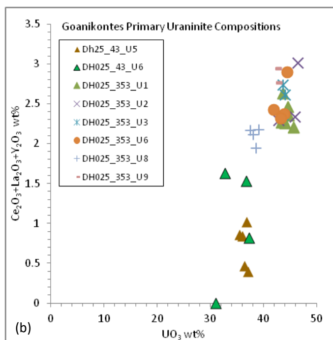
(b) The 353 m samples also host appreciably more REE and Y, specifically Y. There is an overall positive correlation with \text{UO}_3 and REE + Y, which support a substitution of \text{U}^{6+} .
