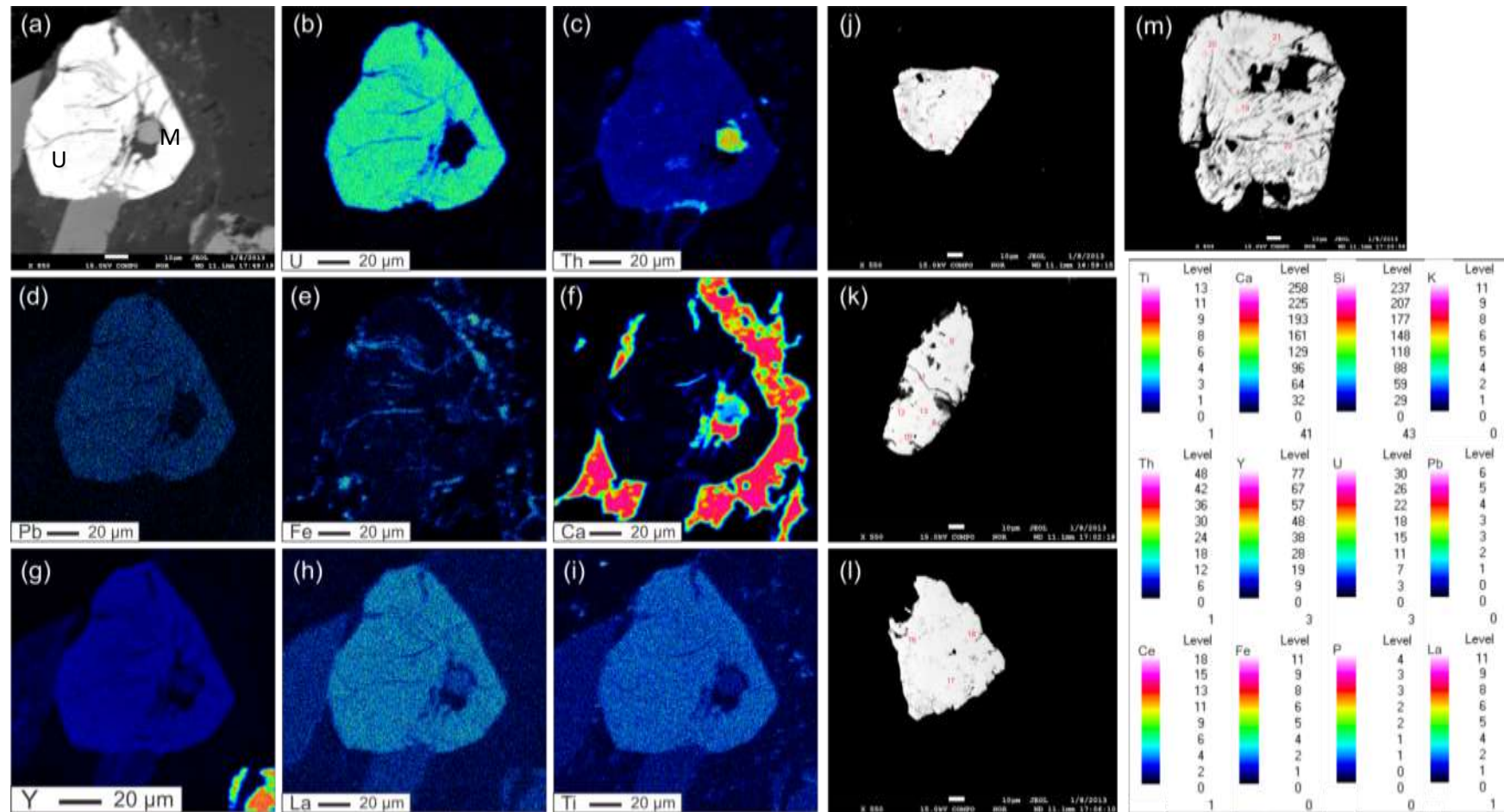
Figure 8.9 Backscatter and element map imagery of Hildenhof uraninite specimens from surface sample HILG21. (a) Backscatter image of a uraninite (U) with a Ce-monazite inclusion (M): (b) U is evenly distributed in the crystal; (c) Th occurs in the monazite inclusion and in patches within the uraninite; (d) Traces of Pb occur throughout the uraninite and (e) Fe fills the prominent fractures throughout the crystal. (f) Ca (as calcite) surrounds the uraninite, and fills fractures and surrounds the monazite inclusion halo; (g)(h) Y and La occur throughout the uraninite in 'above - background' concentrations; La is less concentrated in the monazite than in the uraninite; and (i) Ti shows some concentration in the host minerals. j - m) Uraninite specimens and their analytical point locations. (j) U2 is a near euhedral specimen with fractured edges. (k) U3 is an altered, euhedral specimen. (l) U4 is a near euhedral uraninite with coarse fracture networks propagating from the edges. (m) U5 is an intensely altered and fractured uraninite that hosted coarse inclusions.
