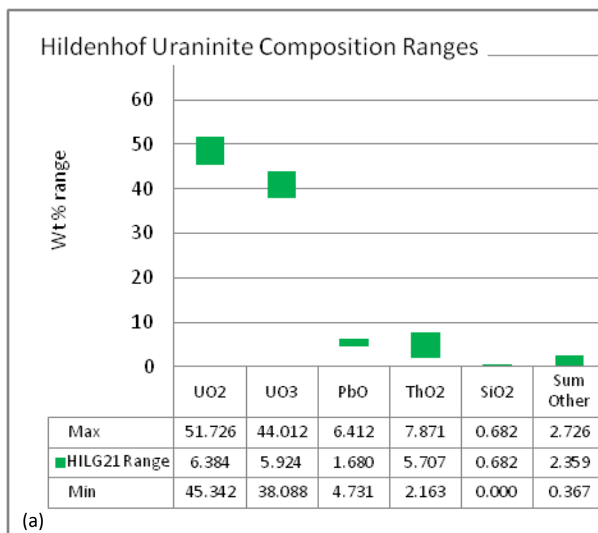
Figure 8.10 Compositional summaries of 5 uraninite specimens in Hildenhof sample HILG 21. (a) U 4+ is dominant in the uraninite, with radiogenic Pb and Th making up the major contaminant elements.
