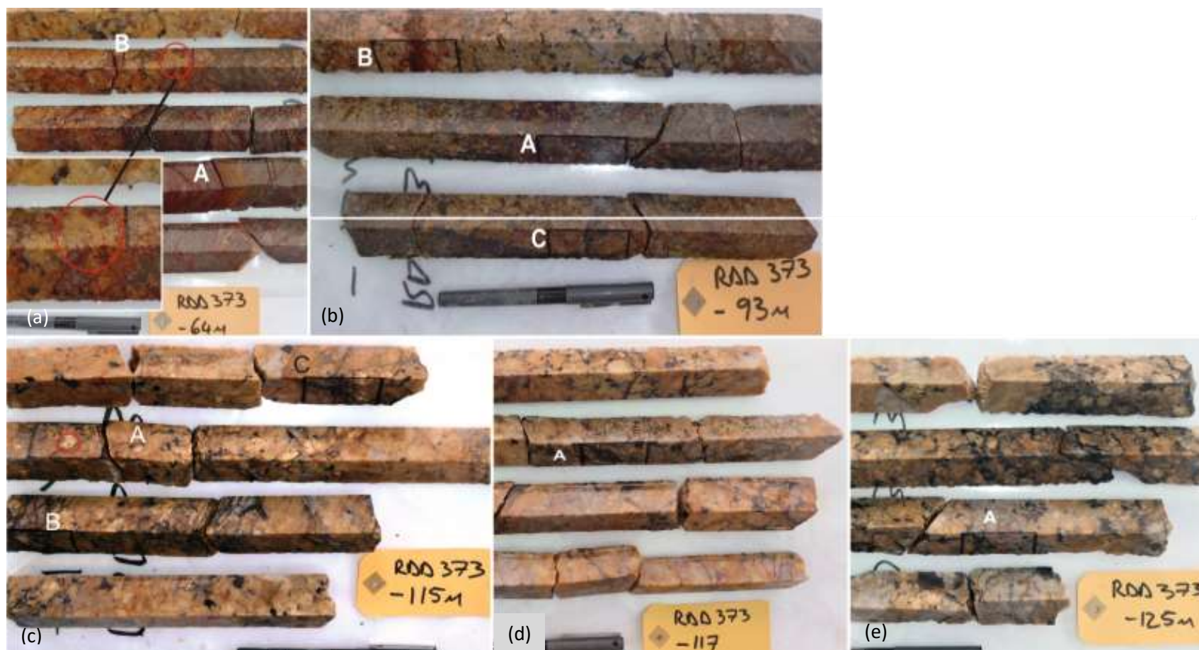
Figure 4.42 Brannerite- and betafite-bearing uraniferous leucogranite samples from drill hole RDD373. The granites in this hole all display some alteration, predominantly oxidation that discolours the feldspars. Some sample display two phases of alteration, the earlier being chlorite- and sericite- dominated and the younger haematite-dominated. (a) Brannerite (circled) is millimetric in most leucogranite samples. (b) Brannerite-bearing leucogranite with a ~250 mm xenolith of metasediment. Chloritisation of biotite, Fe-oxide, and sericisation of feldspars dominate the alteration assemblages. Sulphide blebs occur in both the intrusive and in the xenolith of metasediment host rock. (c) Betafite occurs between feldspars and quartz in pegmatitic uraniferous sheeted leucogranite, note the milky quartz. (d) Uraniferous sheeted leucogranite with mafic clusters comprising predominantly chlorite, biotite, and titanite. The chlorite clusters host fine-grained brannerite. (e) A - brannerite crystal between quartz grains in coarse-grained uraniferous leucogranite. Chloritised biotite forms broken chains space between the feldspars and quartz.
