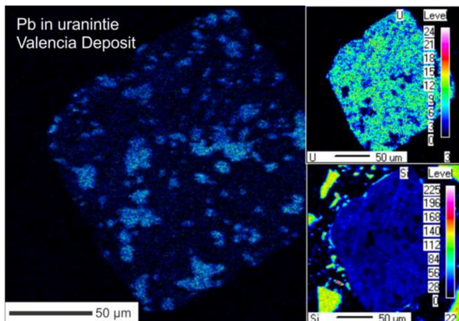
Figure 8.31 Pb distribution in Valencia uraninite. The specimen illustrates Pb distribution is in discrete patches, which implies it is a replacement texture rather than substitution. The patchy distribution is also more evident of Pb-mineral replacement than U-Pb decay. Si in contrast has a more uniform distribution and represents coffinite where it is coincident with U.
