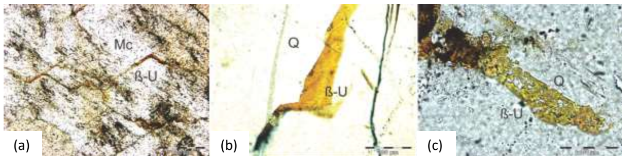
Figure 4.53 Secondary uranium mineral textures at Valencia. (a). Uranophane crystallisation along the cleavage planes of microcline feldspar. The feldspar has undergone sub solidus alteration, giving the cloudy appearance VALG 11, ppl. (b) Uranophane forms amorphous coatings on the surfaces of rock-forming minerals such as quartz, VALG 16 (c) Uranophane occasionally has space in altered feldspar, to grow crystals of acicular habit, VALG 15, ppl.
