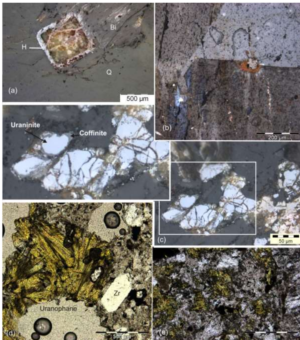
Figure 4.48 Alteration and remobilization of uranium at Husab. (a) Euhedral uraninite cast surrounded by haematite, RDD351 328-329, rfl. (b) Uraninite at a quartz - K-feldspar boundary, jarosite forms as a replacement of feldspar breakdown, associated with radioactive damage, quartz is more resilient, RDD219 335-336m, xpl. (c) Cluster of fractured uraninite surrounded by alteration minerals from the breakdown of the host feldspars. Coffinite forms halos around some of the uraninite (inset). RDD373 116-117A, rfl. (d-e) Boltwoodite and uranophane fills pore spaces created as feldspars are leached during hydrothermal fluid circulation. Hiemstra (1968) and Berning (1986) describe \beta -uranophane in Rössing mine leucogranites; Townend (2009) identified boltwoodite at Husab, discrimination performed with the aid of XRD.
