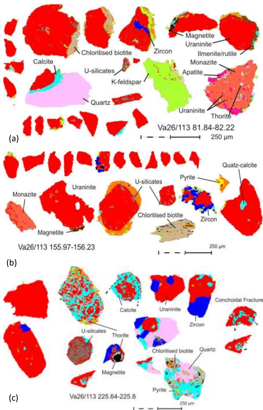
Figure 7.23 Mineral maps of samples from the Va26 113 diamond drill hole at Valencia. (a) Uranium mineral features of Va26 113 81.84-82.22 m. Uraninite is rarely euhedral and has calcite at grain edges. Monazite has inclusions of uraninite and thorite and fine uraninite fills fractures in feldspar. (b) Mineral map features of Va26 113 155.97-156.23. Uraninite occurs as disseminated inclusions in monazite and along biotite cleavages. U-silicates are restricted to fractures towards grain edges. Clustered zircon forms a site for uraninite nucleation. (c) Mineral map features of Va26 113 225.64-225.80. Calcite fills spaces in a large proportion of uraninites, occasionally highlighting the conchoidal fracture. Large (up to ~100 µm) inclusion-free zircon is attached to uraninite. Composite fine-grained clusters include quartz, calcite, plagioclase, biotite and disseminated uraninite, magnetite and pyrite. U silicates after uraninite are scarce.
