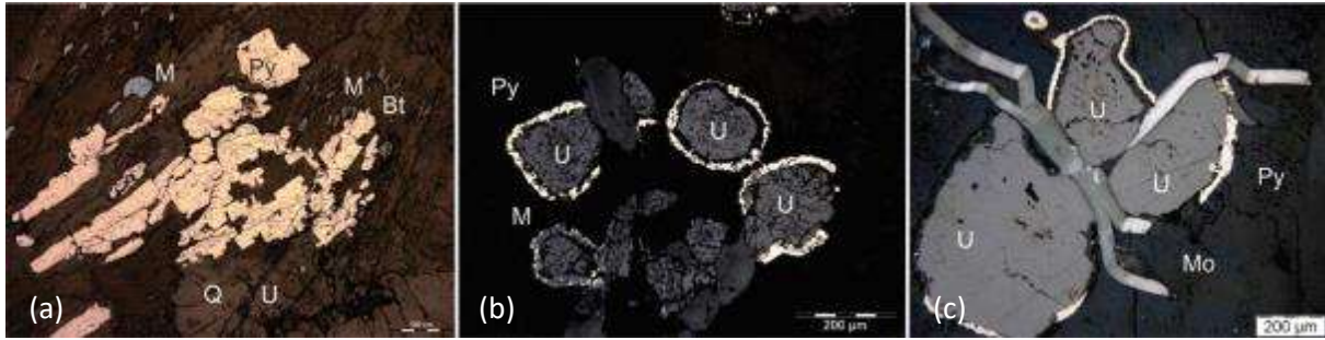
Figure 4.23 Two textures of pyrite and molybdenite younger than uraninite, in Husab alaskite. (a) Cubic pyrite clusters (Py) associated with biotite (b) nests in mineralised alaskite, rfl, ppl. Magnetite (M) occurs with biotite and uraninite (U) is included in quartz (Q) RDD373 93 m A, ppl rfl. (b) Rounded and subhedral uraninite (U) surrounded by compound halos of hydrothermal magnetite (M) and pyrite (P) RDD219 336 m, ppl rfl. (c) Uraninite cluster with pyrite halos which are cross – cut by molybdenite, RDD351 – 258 m, ppl rfl.
