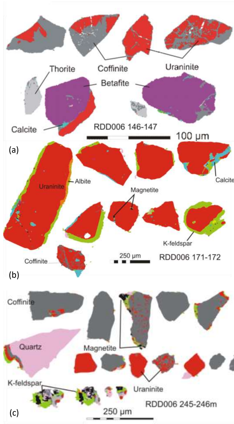
Figure 7.20 QEMSCAN derived mineral maps illustrating uranium mineral textures of RDD006 specimens continued. (a) RDD006 146-147 m, euhedral uraninite with all uraninite showing variable coffinitisation. Coffinite forms along fracture networks within the uraninite. Betafite is coarse, with secondary U-silicates in fractures. (b) Sample RDD006 171-172 m is characterised by coarse-grained uraninite, most grains are >150\ \mu\text{m} across. Albite rims indicate that uraninite crystallised before sub solidus reactions were complete. Some of the uraninite has coffinite alteration along fine internal fracture planes. Calcite is in replacement texture along the rims of some uraninite. The largest, labelled, coarse-grained uraninite is analysed by EPMA. (c) Sample interval RDD006 245-246 m illustrates a population of near-complete coffinite replacement of uraninite, euhedral uraninite, and compound grain clusters of K-feldspar, coffinite-uraninite, thorite, quartz and magnetite. Euhedral unaltered uraninite suggests that alteration is localised in patches within the 1 metre sample.
