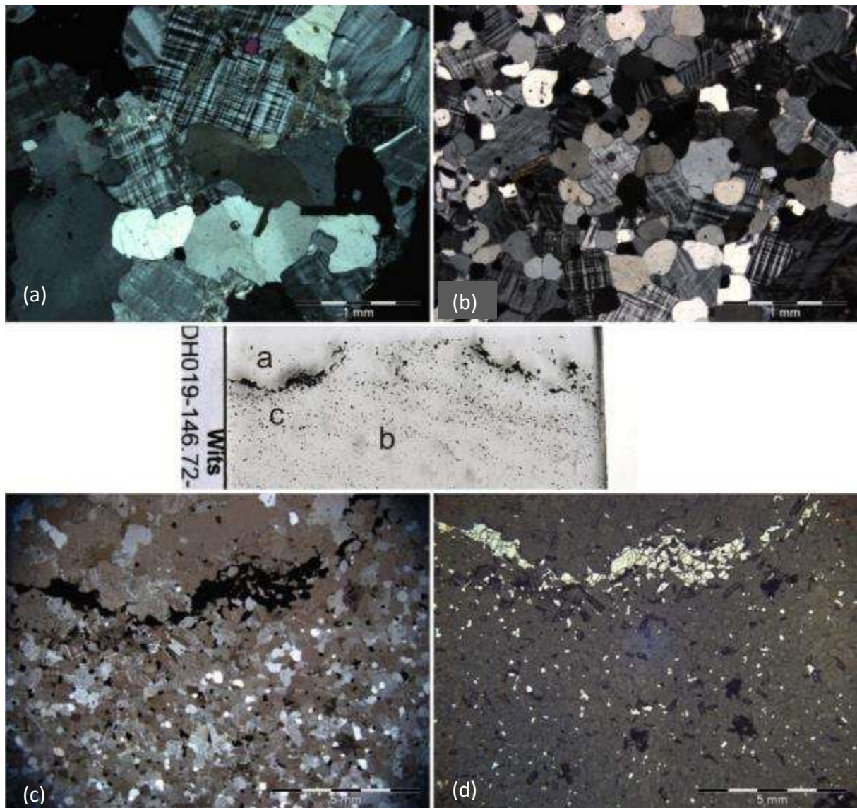
Figure 4.21 Magnetite at reaction contact between sheeted leucogranite and a metasediment. (a) The coarse-grained texture of the sheeted leucogranite is typical of a magnetite-bearing C-type, microcline is the dominant mineral with anhedral quartz clustering between larger feldspars, 5x, xpl. (b) Quartzo-feldspathic composition of the metasediment, with fine-grained disseminated magnetite, 5x, xpl. (c) The top of the image shows the sheeted leucogranite contacting the fine-grained Khan Formation biotite gneiss, 1.25 x, xpl. (d) Reflected light reveals extent of magnetite decreasing away from the intrusion contact. All images of DH019 146.72-147.00, Etango deposit, Goanikontes. Positions of slides are indicated on the slide at centre.
