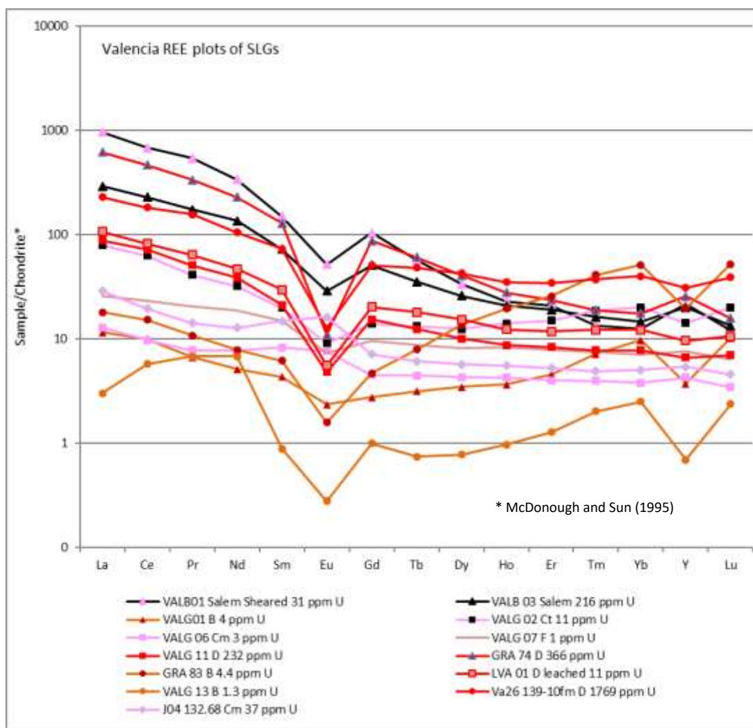
Figure 6.11 Rare earth element plots of sheeted leucogranite and Salem granites at the Valencia deposit. The data show negative slopes for all samples from LREE to Eu, but at least five samples plot with relative HREE enrichment. Samples with flat HREE slopes, plot with Y > Lu ; and in samples with positive HREE slopes, Y < Lu . Types: B- garnet-bearing leucogranite; Cm- Khan Formation-hosted magnetite leucogranite; Ct- Kuiseb Formation-hosted tourmaline leucogranite; D- uraniferous sheeted leucogranite (alaskite); F- K-feldspar pegmatite.
