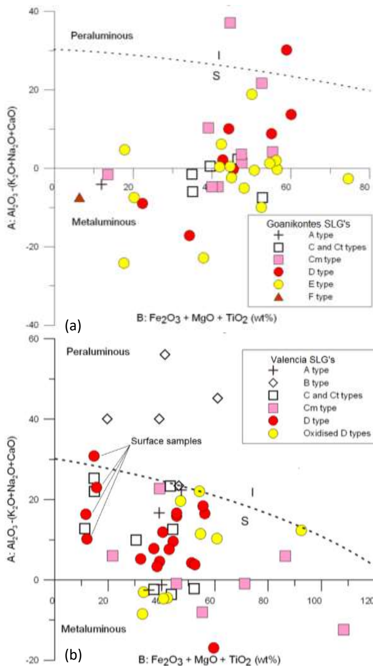
Figure 5.25 A-B diagrams of Debon and Le Fort (1983) of Central Zone sheeted leucogranites. (a) Goanikontes Cm granite varieties show an increase in mafic content with increasing peraluminosity. The majority of the samples plot below the I-S line of White and Chappell (1983). (b) A-B plots of Valencia sheeted leucogranites. D-types show a positive A-B trend and the majority of the samples lie below the ASI line. As in the aluminium saturation diagrams, the B types are strongly peraluminous and plot above the I-S line of White and Chappell (1983). The clustering of surface samples, with considerably lower 'B' from the fresh material illustrates the sensitivity of this diagram to weathering of mafic phases.
