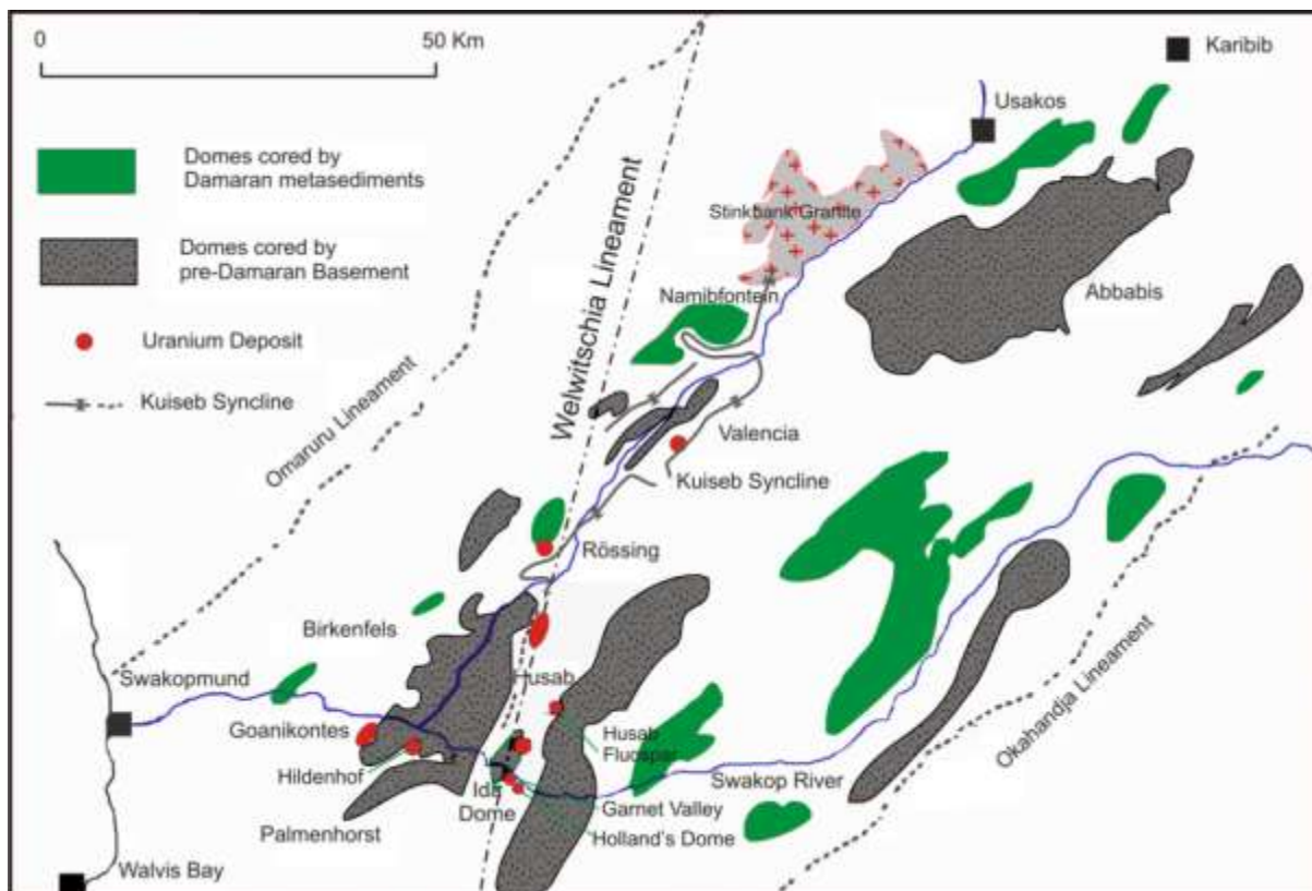
Figure 1.1 The various domes of the Central Zone and their associated primary uranium deposits. The Welwitschia Lineament is a regional magnetic trend produced by late kinematic movement which truncates
