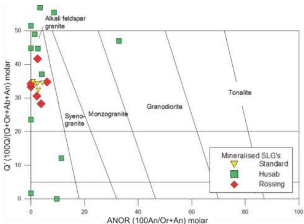
Figure 5.10 Q'-ANOR diagram of selected Husab mineralised leucogranites (alkaskites). The Husab samples display a wide range of CIPW calculated mineral compositions, a product of wall rock and fluid interaction. Samples are all sourced from 'fresh' NQ core and are assumed free from prolonged meteoric weathering associated with surface - sourced samples at the other deposits.
