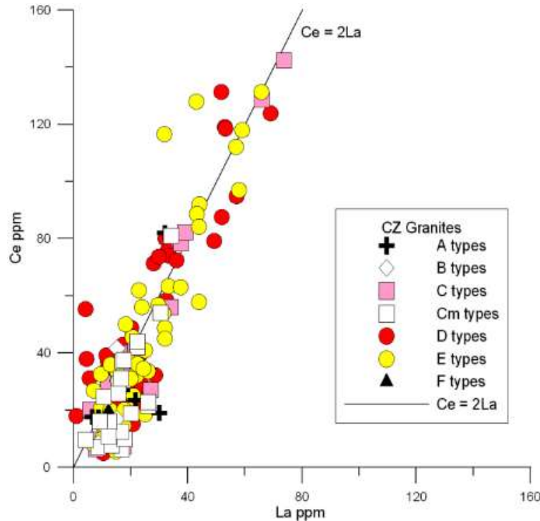
Figure 5.36 La vs. Ce in Central Zone sheeted leucogranite. (a) Ce and La show a systematic ~2:1 relationship overall in the Central Zone sheeted leucogranite, indicative of occurrence solely within monazite. D-type sheeted leucogranites tend to have higher Ce and La concentrations, while the majority of the weakly mineralised samples plot below the 2:1 line with Ce and La <40 ppm. Some of the magnetite-bearing C-type plot with a consistent ratio with concentrations comparable to mineralised sheeted leucogranite. Rössing sample data: Freemantle (2006).
