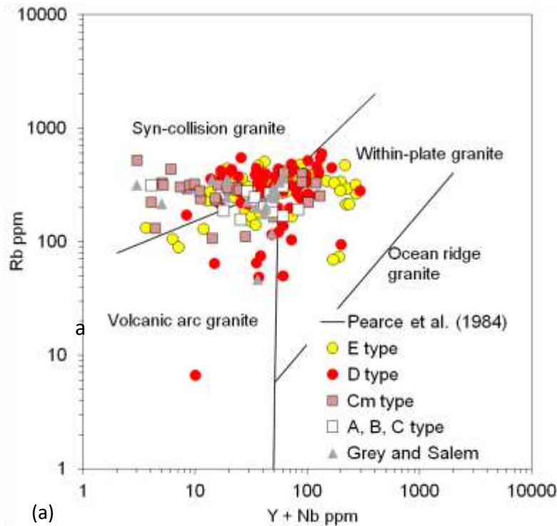
Figure 5.43 Y - Nb and Rb discrimination diagrams of Central Zone uranium deposit granites with fields from Pearce et al. (1984). (a) Central Zone A-C type, Cm-type, D- and E-type, and the Grey and Salem suites. the plots show a distinction between the uraniferous varieties (D, E) and the Cm samples; mineralised samples predominantly plot within and near the 'within-plate' field, and the un-mineralised samples plot from syn-collision through within-plate.
