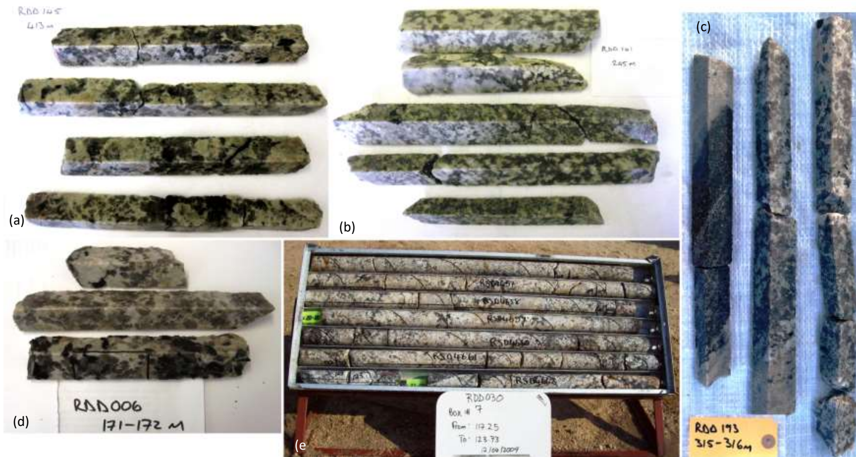
Figure 4.39 Examples of primary uraniferous sheeted leucogranite at the Husab Deposits. (a) Typical uraniferous sheeted leucogranite texture of coarse-grained granite with high % of smoky quartz and white - coloured feldspar, RDD145, Zone 1 Deposit. (b) Primary uraniferous sheeted leucogranite showing metasomatic alteration (fuzzy edges to feldspars) RDD141, Zone 1 Deposit. (c) A primary uraniferous sheeted leucogranite from the southern end of Zone 1 Deposit; A fine-grained chill margin has formed at the contact with Rössing cordierite gneiss, RDD193. (d) An example of coarse-grained uraniferous sheeted leucogranite with coarse biotite books. Quartz occurs in globules and in centimetric clusters, RDD006, Zone 2 Deposit. (e) Uraniferous sheeted leucogranite intervals are tens of metres thick, the example in RDD030 illustrates the tendency for smoky quartz to form clusters, and segregations within feldspar-dominated granites.
