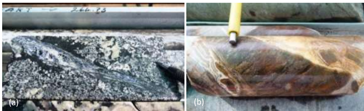
Figure 3.8 Late stage vein minerals. (a) Fluorspar in breccia vein. The fluorspar is purple in colour, which is indicative of U content. Invariably sheeted leucogranites with prominent fluorspar veining tend to show lower than expected U grades, RDD193 - 261 m. (b) Calcite - quartz veins often accompany intense weathering of the host rocks, but carry elevated grades of mobile U, RDD373 - 68 m.
