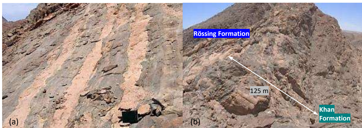
Figure 3.55 Magnetite-type leucogranites at Valencia. (a) Bedding parallel sheets in the Khan Formation, magnetite porphyroblasts are visible on surface. (b) Magnetite granite sheet volumes increase toward the Rössing Formation contact. Sheets display less ordered geometry in the upper Khan and have overwhelmed the metasediments, but have not enforced significant rotation of the metasedimentary xenoliths.
