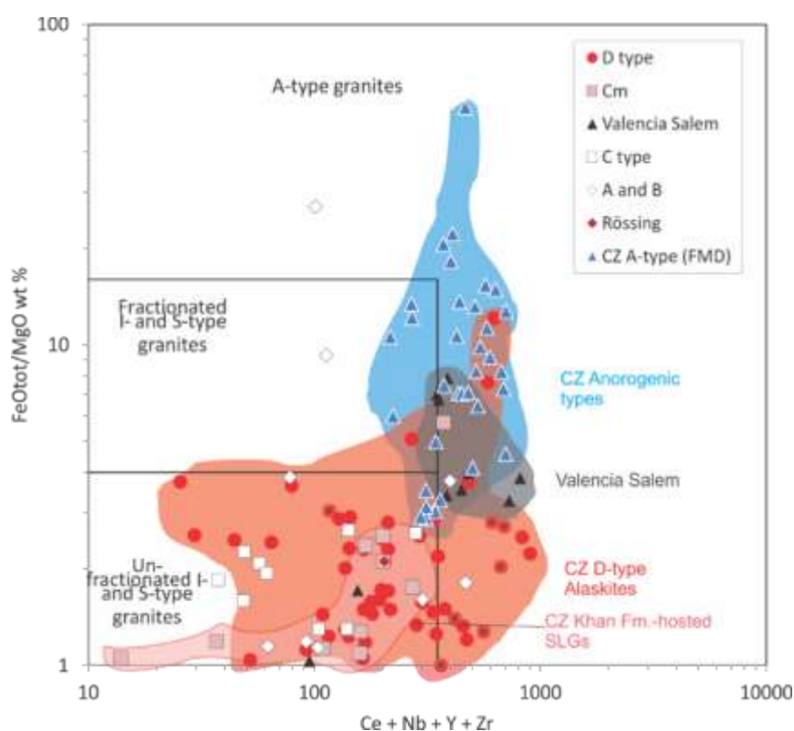
Figure 9.5 HFS elements vs. \text{FeO}_{\text{tot}}/\text{MgO} wt.% granite- discrimination plot. The Valencia Salem granites, the A- and B-type SLG's, the C- and \text{C}_m -type leucogranites and the D-types are compared to the anorogenic granite suites of the Central Zone (CZ A-type, FMD). The bulk of the pre-D 3 sheeted leucogranites plot within the un-fractionated field, while the uraniferous sheets and the Valencia Salem diorites tend to plot outside because of HFS element abundance. CZ A-type (FMD) data from McDermott et al. (2000).
