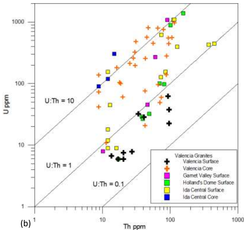
(b) Th vs. U of surface vs. core sample U and Th ratios at Ida Central and Valencia. Core samples, that show little to absent evidence of surficial leaching tend to have retained original, high U:Th . Data clipped to >5 ppm U and >9 ppm U. Five of the Holland's Dome samples and three Valencia samples contain <9 ppm Th, and so plot with 'equal' Th abundances.
