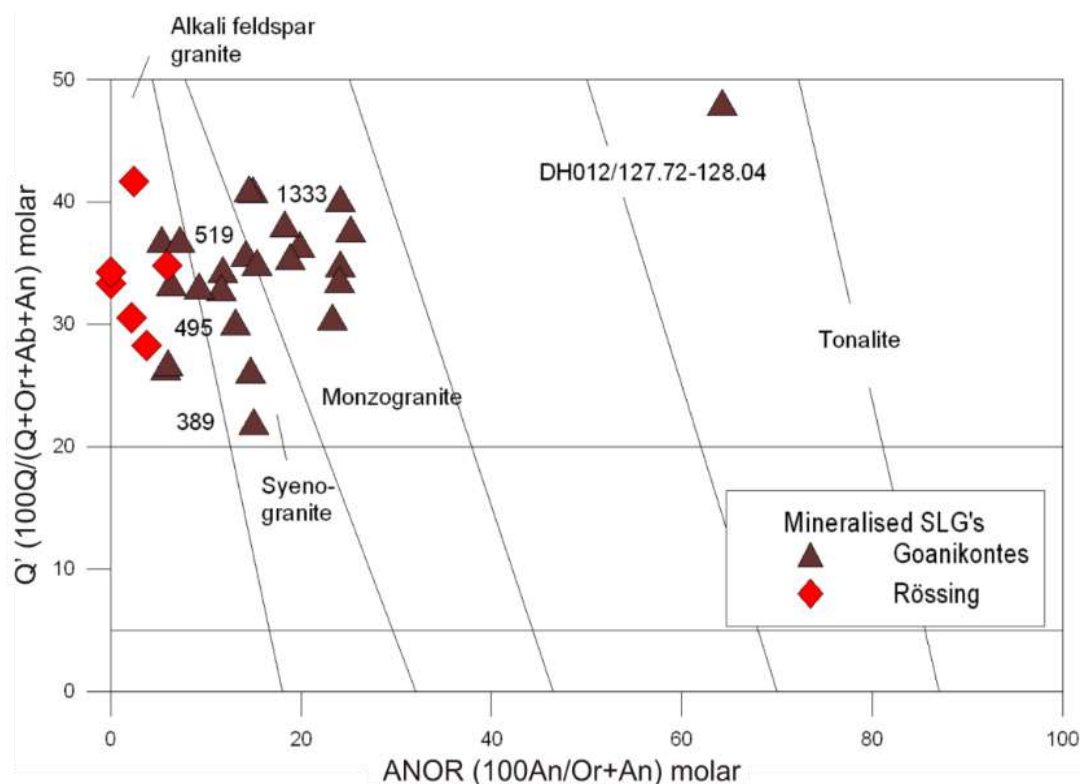
Figure 5.7 Q'-ANOR diagram for mineralised leucogranites from Etango deposit (on Farm Goanikontes) diamond drill core. Goanikontes samples have a range from monzogranite to alkali feldspar granite; the majority of samples have a syeno- to monzogranite composition. There is one plagioclase rich sample which plots accordingly in the tonalite field. The quartz content is higher than the samples from Rössing.
