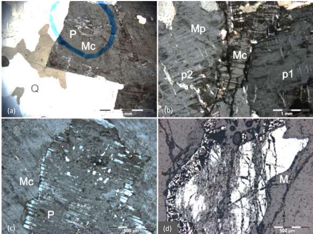
Figure 4.19 Petrographic features of Magnetite-type sheeted leucogranites at Valencia. (a) Euhedral microcline (Mc) with skeletal plagioclase inclusions (P) VALG 06, ppl. (b) Two generations of K-feldspar; an older tartan-twinned microcline (Mc) is sandwiched between two microcline-perthite grains (Mp). There are two generations of perthite exsolution (p1-cleavage-parallel exsolution and p2 - albite twinning in flame perthite) VALG 06, xpl. (c) Plagioclase inclusion in microcline with sericitised core and globular quartz inclusions, J04 132.69-132.96, xpl. (d) Magnetite is the most abundant accessory in the magnetite type sheeted leucogranites, J04 132.69-132.96, rfl.
