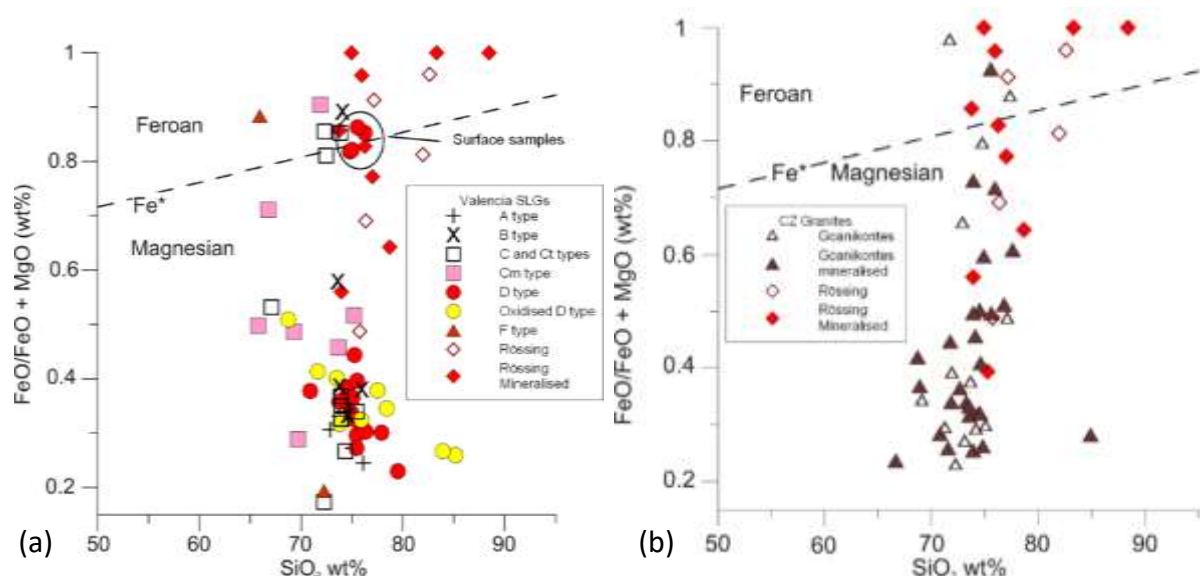
Figure 5.20 Fe^* vs. SiO_2 diagrams of the leucogranite suite at Valencia and Goanikontes. (a) Fe^* vs. SiO_2 diagram of mineralised and weakly mineralised Valencia sheeted leucogranite varieties. The majority of samples lie below the Fe^* line, though some mineralised samples lie on or above it. If surface samples are removed the fresh Valencia mineralised samples do not plot above the Fe^* line despite high SiO_2 content. The Fe^* line is from Frost et al. (2001). (b) Fe^* vs. SiO_2 diagram of mineralised and weakly mineralised Goanikontes sheeted leucogranite. A very subtle trend toward the Fe^* line with increasing SiO_2 is apparent. The majority cluster below Fe^*=0.4 .
