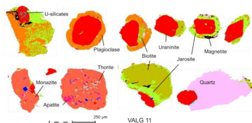
Figure 7.25 Mineral map features of VALG 11. Uraninite is coarse-grained (>100 µm) and is hosted in K-feldspar, quartz and biotite. Alteration of the biotite and feldspars results in albite and clay halos, respectively, around the radioactive minerals. Anhedral monazite hosts fine-grained uraninite, zircon and thorite.
