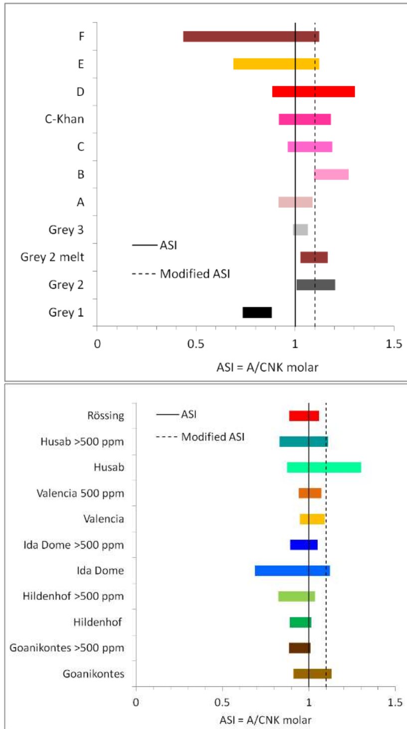
Figure 5.27 Bar graph plots of aluminium saturation of the sheeted leucogranites. The graphs illustrate narrow ASI ranges in the Salem and Grey granites, where Grey 1 and Grey 2 refer to first and second generation diorite and syenogranite varieties, and the pre-D 3 leucogranites. The most primitive granites (diorite) in the region are metaluminous; all of the felsic biotite granites are peraluminous in the modified ASI classification. The pre-D 3 leucogranites tend to be peraluminous, with the magnetite-bearing C-types (C-Khan) being the most metaluminous of the group. The D-types reflect the more accurate compositional range of the uraniferous and post-D 3 leucogranites, while the E-types, which are essentially altered D-types, give a metaluminous compositional range. There is some uncertainty in this study as to whether the F-types that are sampled are in fact the youngest leucogranites in the Central Zone, the broad range in a small sample set (n=3) limits any interpretation of the granites by ASI. (b) ASI plots of individual deposit uraniferous leucogranite populations. The range plots show the Husab samples with <500 ppm.
