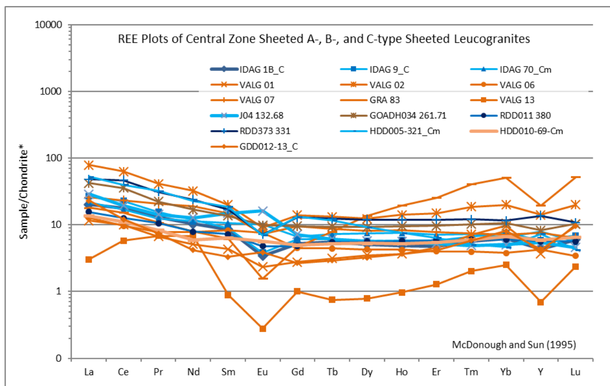
Figure 6.2 REE plots for sheeted leucogranites from Etango, Husab, Ida Dome and Valencia. The samples show a combination of -ve Eu anomalies, and relatively flat or shallow negative slopes. Y is included as a measure of host rock/phosphate interaction, where samples with elevated Y are interpreted as being contaminated by phosphates (xenotime).
