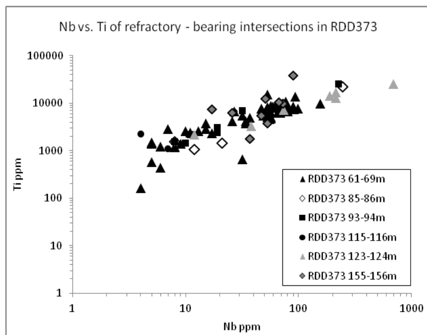
Figure 5.59 Nb (ppm) vs. Ti (ppm) of brannerite- and betafite-bearing intervals in drill hole RDD373. Each point represents a spot on a 10-15 cm interval spacing in given mineralised intervals. The overall correlation between the elements in these intervals is positive. Nb reflects betafite, columbite, or cordierite; while Ti reflects rutile, titanite, ilmenite or brannerite or leucoxene abundances. although, the positive correlation may reflect a single-phase distribution.
