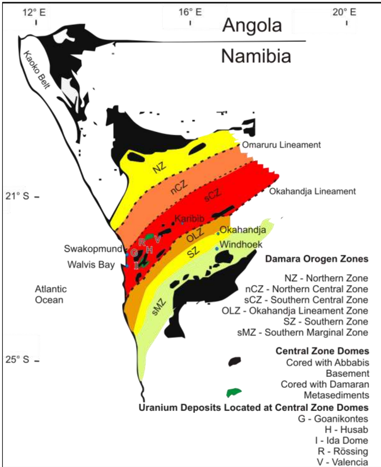
Figure 2.1 The Pan-African Damara Orogen of Central, Namibia. The regional orogen is divided into a number of tectono-stratigraphic zones, bounded by major lineaments. The four deposit areas that are investigated in this research are; Goanikontes (G) Husab (H) the Ida Dome (I) and Valencia (V). Zones and structural features from Miller (1983a and 1983b, 2008) and Kinnaird and Nex (2007).
