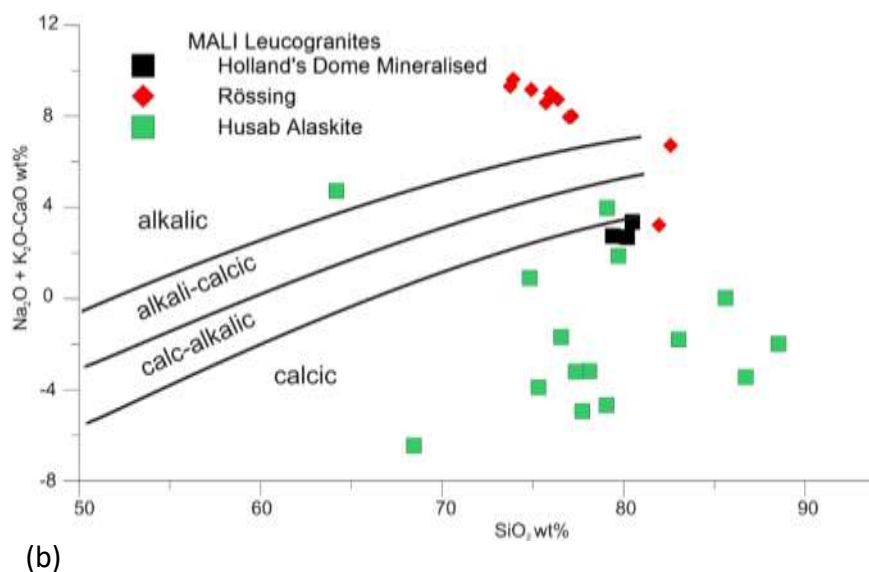
Figure 5.18(b) Modified alkali-lime index diagram of Husab Alaskites showing a positive MALI/ \text{SiO}_2 trend. Field lines from Frost et al. (2001) and Rössing sample data: Freemantle (2006).
