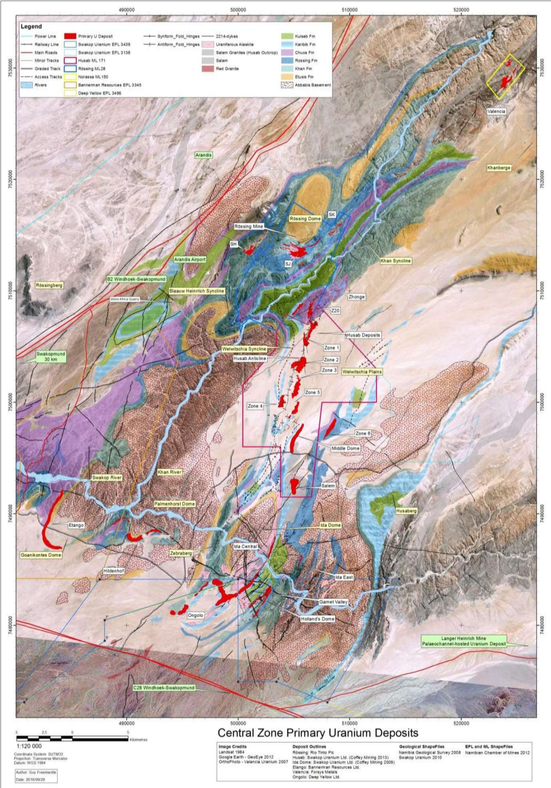
Figure 1.5 Major Central Zone primary-hosted uranium deposits. Most primary hosted U deposits occur within ~40 km of the Rössing Mine and include significant, economically viable projects at Etango and at Husab. The samples of this study are obtained from Hildenhof (Onkelo) on Bannerman Resources EPL 3345 and from drill core at the Etango Deposit. Ida Dome surface samples were collected at Ida Central, Garnet Valley and Holland's Dome. A limited number of core samples were sourced from Ida Dome and Garnet Valley for REE analyses. All of the Husab samples are sourced from diamond core. The Valencia sample population is a combination of surface and core material. The geological coloration overlay is traced from the Walvis Bay Map sheet- 2214 of the Namibian Geological Survey. The deposit locality shapes are traced from information available courtesy of Bannerman Mining Resources, Namibia (2009); Extract Resources (2012) and Valencia Uranium, Namibia (2010). Satellite Imagery is courtesy of Landsat™ (1990) and GeoEye (Google Earth, 2013).
