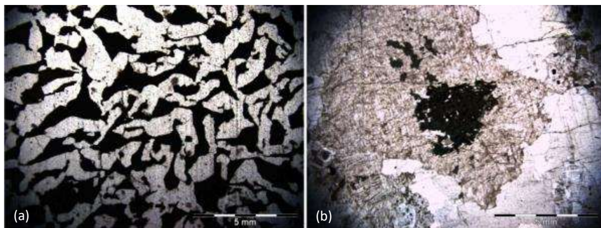
Figure 4.11 Tourmaline in C-type sheets from Goanikontes. (a) Quartz – tourmaline nests are common in very coarse and pegmatitic C-type leucogranites- in very coarse samples individual prismatic tourmaline crystals are visible in hand-specimen, DH012 198.58-198.77, ppl. (b) Massive-textured tourmaline is more common, and occurs as inclusions in feldspars or interstitial to large quartz and feldspar crystals, it is found in samples from all the deposits in this study, DH022 59.00-59.24, ppl.
