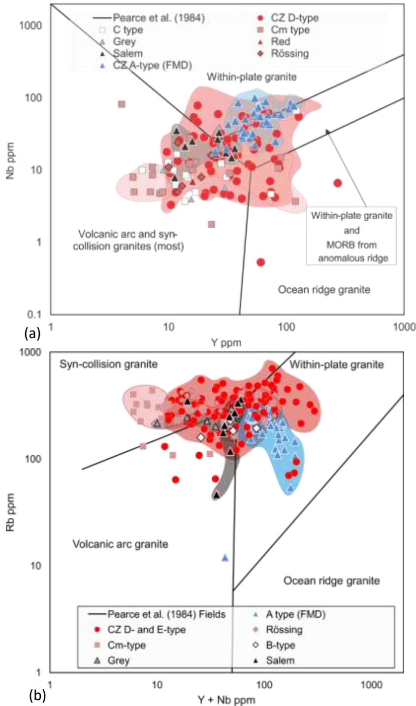
Figure 9.7 Tectonic discrimination diagrams of the Central Zone granites. (a) Y vs. Nb shows a distinct difference between the pre-D 3 and the mineralised granites. Although the source is not constrained, the difference in HFS element abundances is considered strong evidence for different source material between the populations. The Rössing comparative samples plot within the volcanic arc - syn-collisional field, which supports a calc-alkaline affinity proposed by McDermott et al. (2000).
