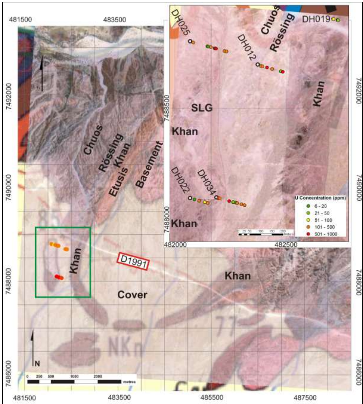
Figure 4.3 Localities of Etango A drill hole collars at Goanikontes. The drillholes dip uniformly at \sim 70^\circ to the east-southeast. Vertical projections to the map surface of intersections show high-grade samples close to surface and at depth. The Etango deposit is on Farm Goanikontes and located within EPL3345 of Bannerman Resources. The colour overlay is from the Geological Survey of Namibia, Walvis Bay Map sheet 2214 and remote sensed image is geo-referenced from Google Earth™ (Quickbird™).
