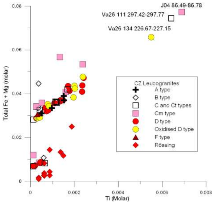
Figure 5.24 Maficity diagrams of Central Zone sheeted leucogranites at Valencia. The majority of the Valencia samples have elevated maficity in excess of Rössing, all oxidised D-types plot with excess Fe + Mg. A small population of low-biotite D-types plot in a cluster close to the Rössing sample composition highlighting the role of biotite in the plots. Rössing data from Freemantle (2006).
