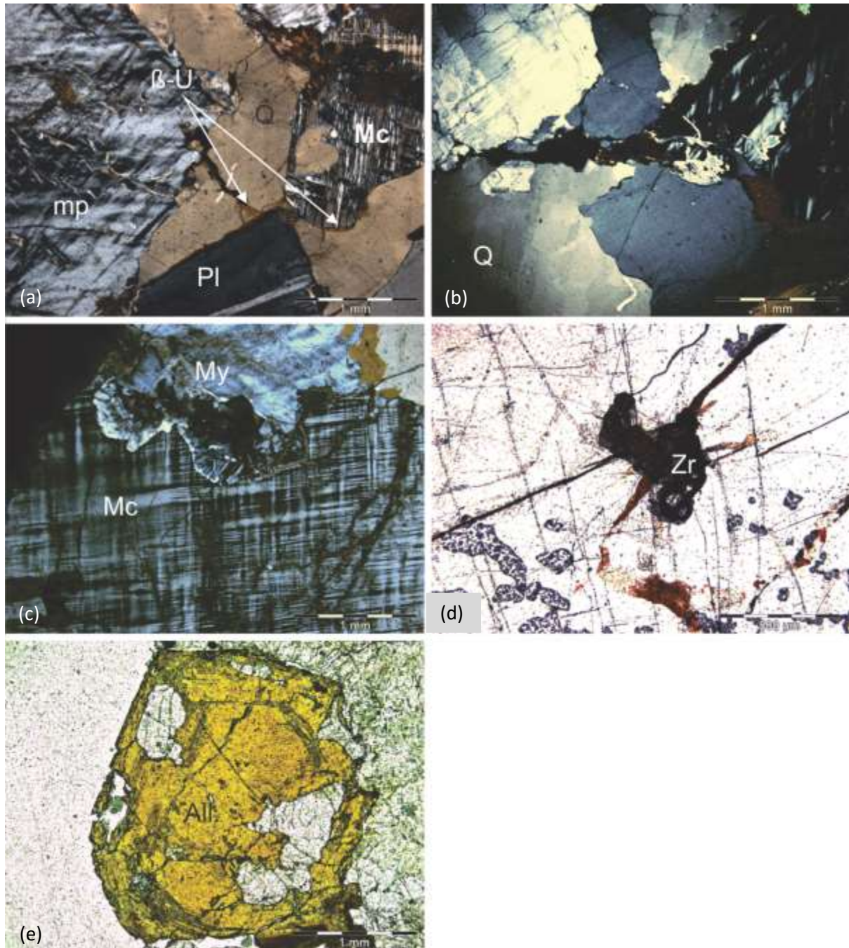
Figure 4.50 Unaltered D-type sheeted leucogranites and mineralised apophyses at Valencia. (a) Euhedral plagioclase (Pl) anhedral microcline (Mc) and uniformly extinct quartz veinlets with secondary U minerals (yellow stains in fractures) VALG 16, xpl. (b) Euhedral quartz with uniform strain cutting strained quartz (Q) VALG 26, xpl. (c) Myrmekite (My), in wart like growth at microcline (Mc) contact, is uncommon in mineralised sheets at most deposits, but is characteristic of the melt apophyses, VALG 08, xpl. (d) Zircon (Zr) is associated
