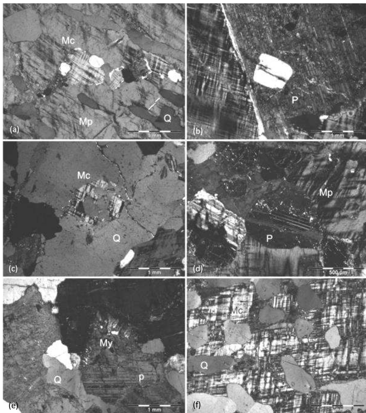
Figure 4.12 Textural features of the C-type sheeted leucogranites sampled from Goanikontes core. (a) Tartan microcline, euhedral and vermicular quartz (Q) in microcline – perthite (Mp) in an accessory-free C-type, DH012 66.41-66.79, xpl. (b) Euhedral quartz included in euhedral plagioclase in a magnetite C-type, which coincidentally also has tourmaline (Figure 4.11b) DH022 59.00-59.24, xpl. (c) A magnetite-bearing C-type, in which microcline is surrounded by later quartz, DH019 67.09-67.54, xpl. (d) Zoned plagioclase in a tourmaline C-type; the grain resembles a plagioclase overgrowth more than a zoned single grain. The inner plagioclase has \sim\text{An}_{55} composition, DH012 315.67-315.93, xpl. (e) Myrmekite develops at plagioclase – K-feldspar grain boundaries, and is rarely observed in the cores of the feldspars, DH019 76.39-76.67, xpl. (f) Typical pegmatite with graphic quartz growth in large (>10 mm) microcline, DH019 100.50-100.93, xpl. Magnetite-bearing C-types
