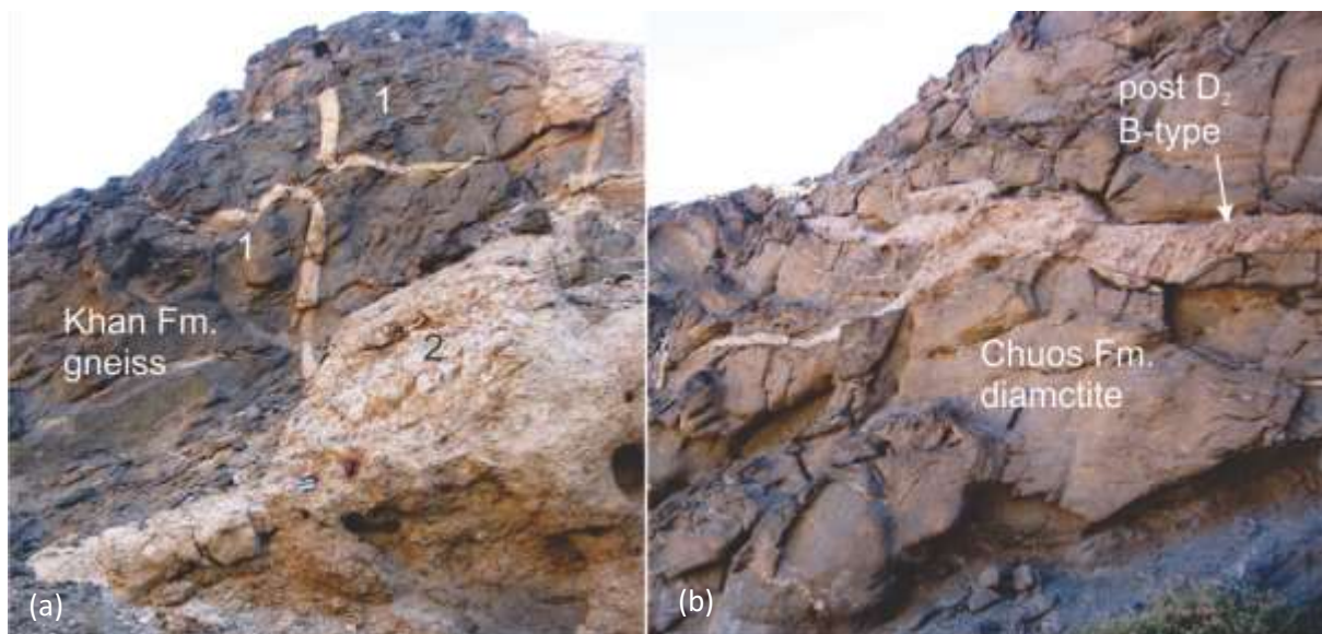
Figure 3.47 A-type and B-type sheeted leucogranites at Hildenhof. (a) Narrow discontinuous sheets are folded with the metasediments, these are crosscut by a later mineralised pegmatitic granite (foreground). (b) Post D 2 sheet intrudes bedding-parallel as well as crosscutting, note granite may appear folded as in (a).
