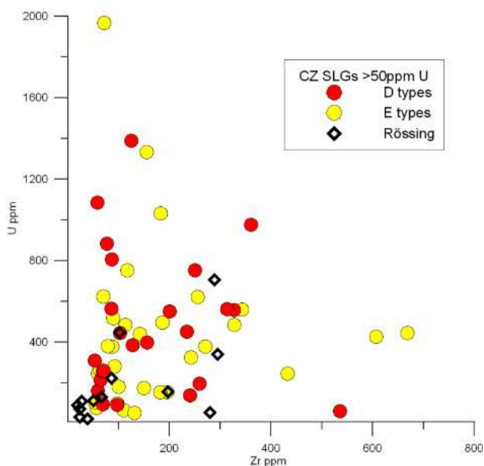
Figure 5.38 Graph of U vs. Zr of the Central Zone uraniferous SLGs. Uranium and zirconium both occur in zircon, which may co-exist with uraninite in phases such as biotite. Despite the co-existence there is no apparent relationship between the two elements in the Central Zone leucogranite suites.
