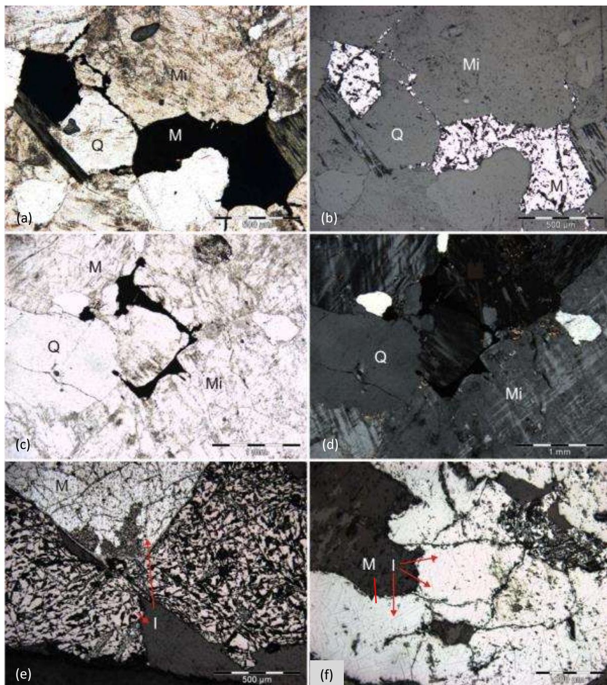
Figure 4.13 Magnetite in grey type-3 from Hole DH012, in mineralised sheeted leucogranite from Hole DH019 and Cm-type from Hole DH022. (a) and (b); Euhedral magnetite (M) surrounds a quartz (Q) crystal, magnetite permeates between the euhedral quartz and adjacent microcline as well as in fractures of the feldspar (Mi) DH012 197.04-197.35, ppl and rfl. (c) and (d); Magnetite (M) bisects a microcline-perthite grain and also permeates into fractured quartz (Q) and microcline (Mi) DH019 71.74-72.18, ppl and xpl. (e) and (f); Magnetite (M) often occurs with exsolved ilmenite (I) however ilmenite occasionally does occur on its own and is usually adjacent to magnetite, DH022 59.00-59.24, both rfl.
