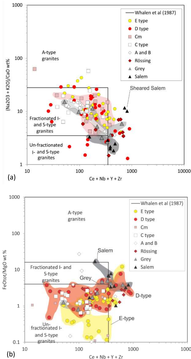
Figure 5.40 Discrimination plots of (\text{Ce} + \text{Nb} + \text{Y} + \text{Zr}) in CZ granite types, with fields from Whalen et al. (1987). (a) The majority of granites plot within the differentiated field for I- and S-type granites. The A and B type granites, which are hosted in the Chuos and Kuiseb Formations, show the closest correlation. The Grey and Salem suites also exhibit a close correlation. High fractionation ratios do not correspond with HFSE abundances. Rössing data from Freemantle (2006); data also contributed from Johnson (2011). Samples in which one or more HFSE analyses are missing are not plotted.
