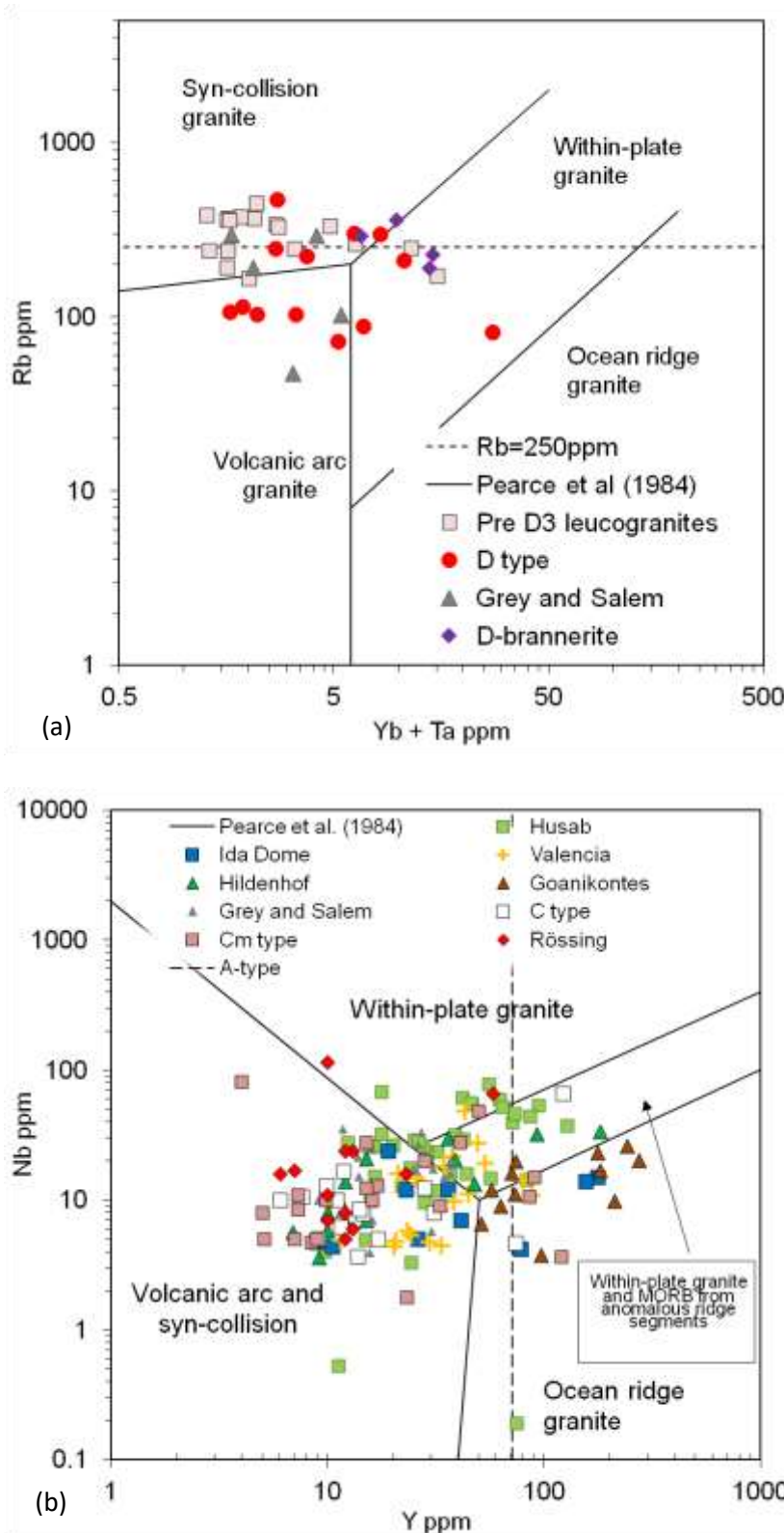
Figure 5.44 Y and Nb, and Yb - Ta and Rb discrimination plots with fields from Pearce et al. (1984). (a) Yb + Ta vs. Rb plot using ICP-MS analysis. The ICP-MS data set is limited to 37 leucogranite samples, of which 14 are classified as D-or E-type. Rb content of the pre- and post-D 3 leucogranites straddles the 250 ppm line of Chappell and White (1992); as with Figure 5.33a, Rb is elevated in the pre-D 3 granites relative to many of the D-type and E-type sheets. There is a bi-modal distribution with respect to the HREE (Yb and Ta abundances), with distinctly less spread in the pre-D 3 leucogranites. The brannerite and betafite-bearing samples are Yb and Ta enriched relative to most samples.
