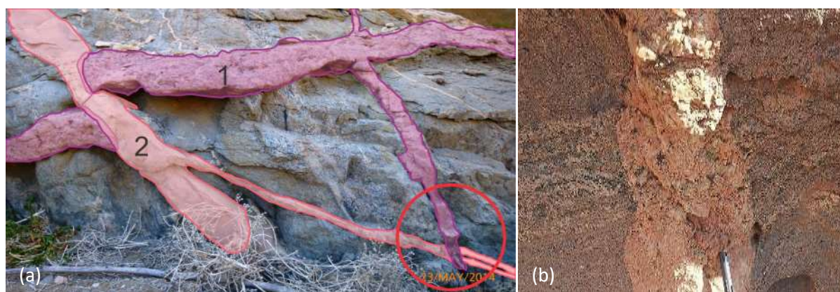
Figure 9.1 Textural and compositional inhomogeneity in the leucogranites. (a) Ambiguous crosscutting relationships between two texturally different sheeted leucogranites at the Ida Dome. 1 is cut by 2 at top left, but 2 is cut by 1 at bottom right. Textural relationships suggest 1 is an F type, and 2 is probably a B or C type. (b) Leucogranites that crosscut compositional banding in the Khan Formation inherit diopside from the host rock.
