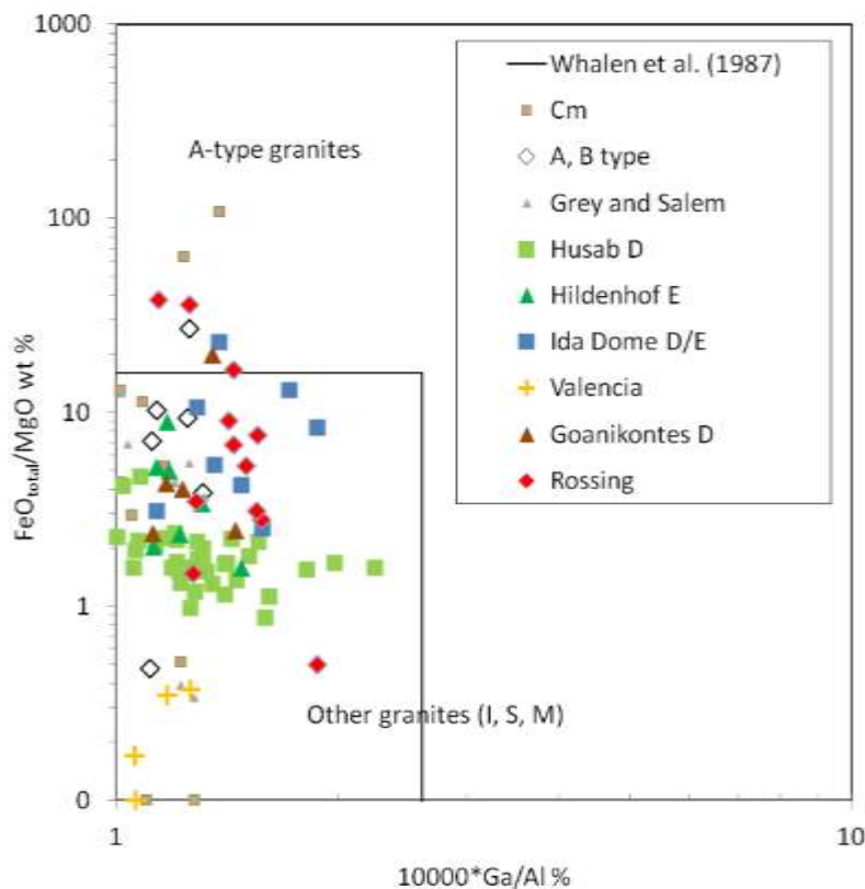
Figure 5.42 FeO_{tot}/MgO ratios of SLGs at the CZ primary U deposits. Fe/Mg ratios tend to be low, with most leucogranite samples plotting with ratios less than 2. The magnetite-bearing granites are oxidised and thus host accessory magnetite in variable abundances, reflected in high FeO_{tot}/MgO ratios. The Goanikontes samples plot with relatively high FeO_{tot}/MgO relative to the Husab and Valencia samples, while the Ida Dome uraniferous granites plot with the highest average FeO_{tot}/MgO of the mineralised suit.
