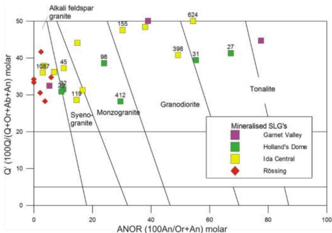
Figure 5.9 Samples from the Central, Garnet Valley and Holland's Dome deposits. The samples show variation in normative An content and relatively high quartz content compared to the Rössing samples. Plagioclase (albite-oligoclase) is present in all Ida Central thin sections. External Ca and Si is contributed to the system by reactive calcareous units of the Khan and Rössing Formations.
