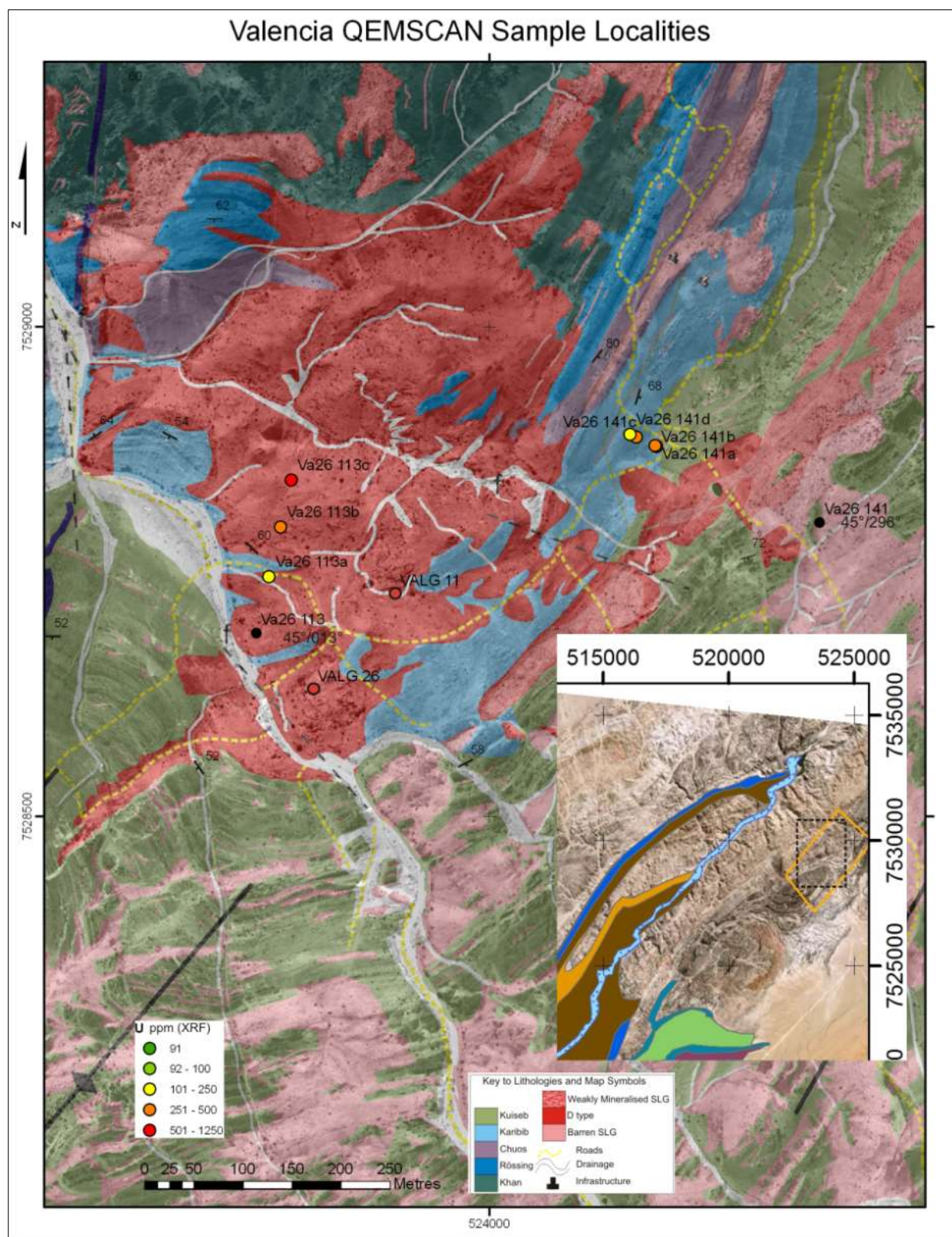
Figure 7.22 Ortho-photo with lithological overlay at Valencia with localities of samples submitted for QEMSCAN analyses. Drill hole collars are labelled with plunge and azimuth, samples with suffix (a-d) are projections to surface of the position of the sample downhole.
