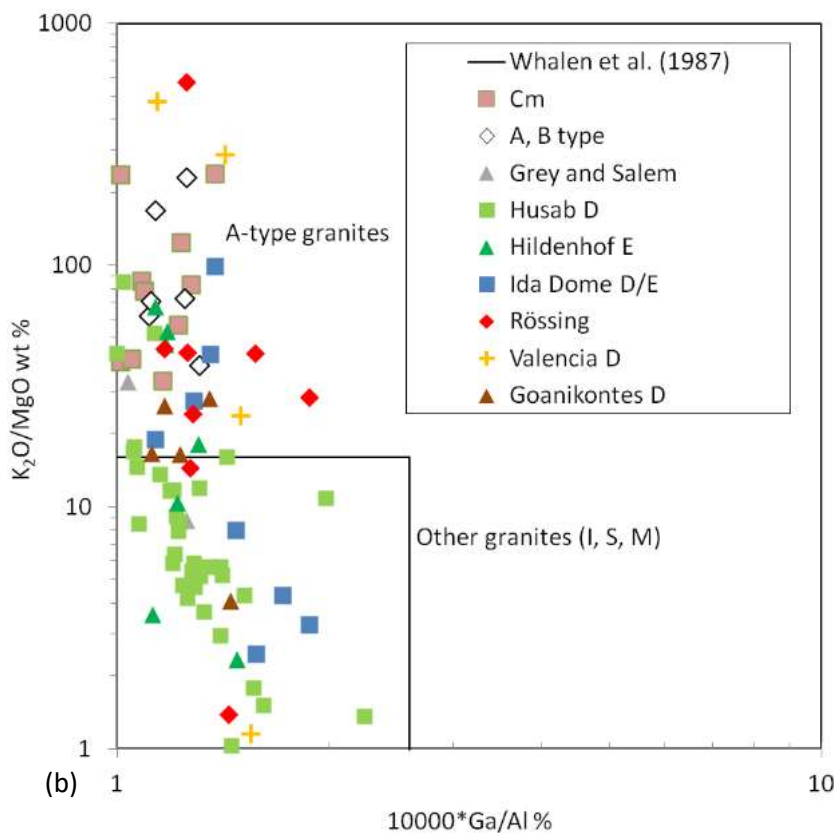
Figure 5.41 (b) \text{K}_2\text{O}/\text{MgO} ratios show a far wider range with the Valencia, most Goanikontes, and Rössing samples plotting in the A-type field. Ida Dome, Hildenhof, Rössing, and the Salem and Grey granites plot in both discrimination fields. The \text{C}_m samples all show A-type ratios of K and Mg.
