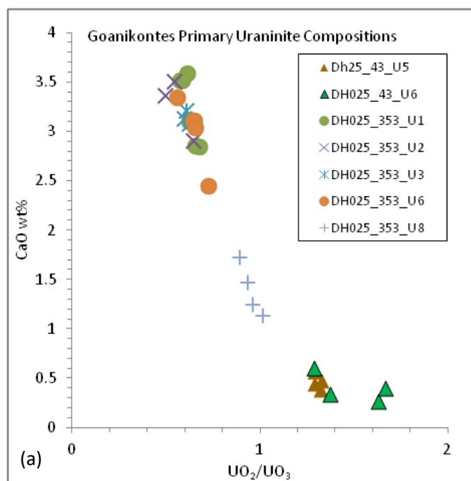
Figure 8.5 Uraninite compositional variation in the Etango DH025 drill hole samples. (a) The uraninite specimens from the two depth intervals contrast in \text{UO}_2/\text{UO}_3 and in CaO content, where the 353 m samples host consistently more CaO to a maximum of 3.5 wt.%. The consistent negative trend (within individual uraninite specimens) suggests Ca substitution of \text{U}^{4+} .
