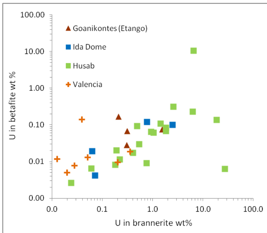
Figure 7.29 U-department between brannerite and betafite. The minerals have a positive relationship in the Husab and Valencia leucogranites. Three Husab samples host >10 wt.% of U in one of the refractory mineral species. Petrological Indicators.
