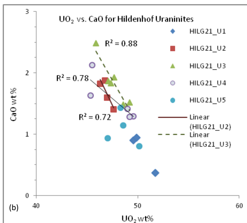
(b) The systematic relationship between U 4+ and Ca shows that Ca substitution has taken place in the Hildenhof uraninite.
