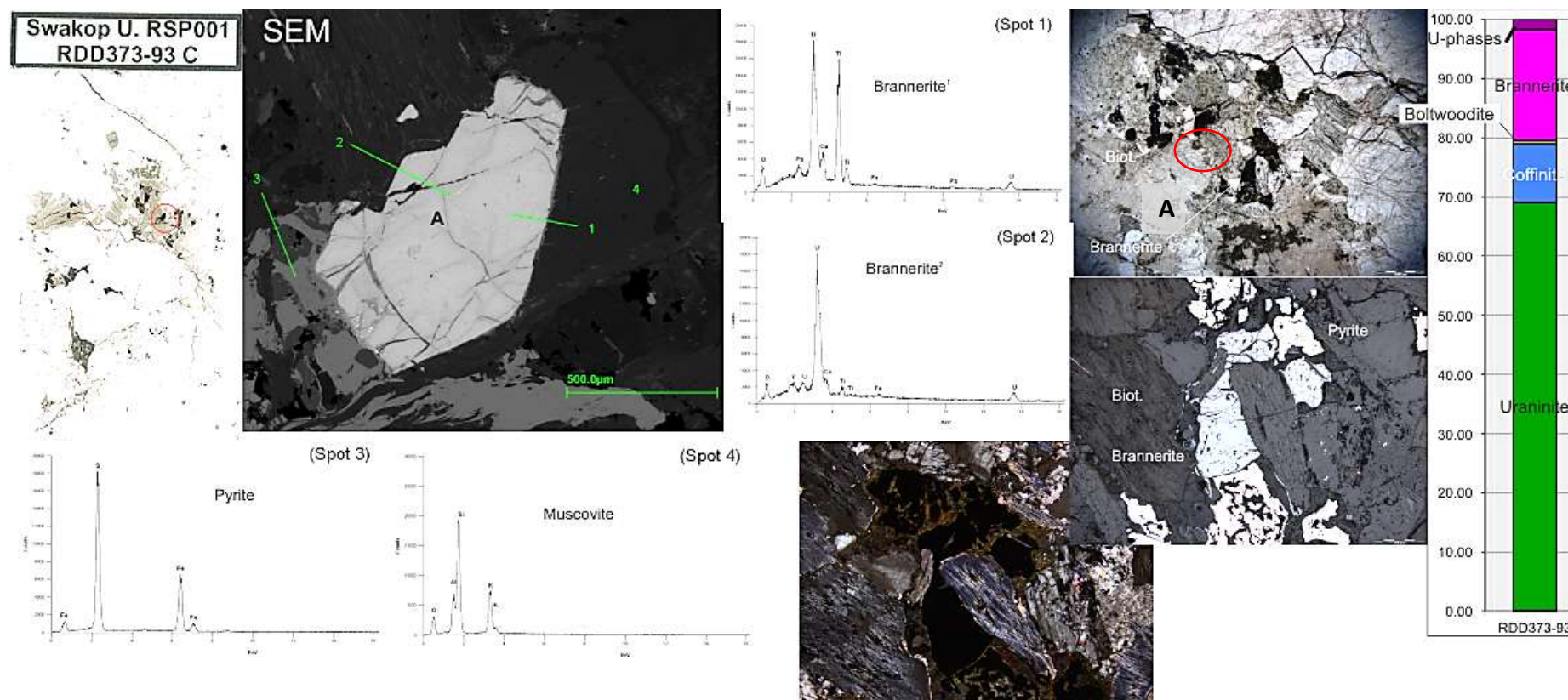
Figure 5.57 Thin section and SEM imagery of sample RDD373-93C. Brannerite occurs as free grains (SEM image labelled A) within biotite clusters and is closely associated with pyrite and muscovite. A secondary brannerite-phase occurs in fractures of the brannerite with a composition similar to uraninite, without any Pb. The SEM image illustrates important mineral textures and relationships. Pyrite (3) is inter-leaved with chloritised biotite indicative of its late magmatic nature. Brannerite occurs as a primary euhedral phase, and as a secondary product of mineral weathering (1 and 2). Muscovite occurs with biotite and is in contact with the brannerite. The primary brannerite is also illustrated in the photomicrograph, top right of the collage. A mixture of secondary U- (coffinite) and Fe-minerals occur in the interstitial spaces of the brannerite-biotite clusters, illustrated in the photomicrograph at bottom centre. QEMSCAN deportment results show a prominent brannerite constituent in the total U-mineral budget. The brannerite occurs in alaskite in this particular sample.
