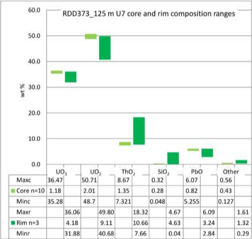
Figure 8.17 Composition and texture of uraninite U7, hosted in biotite of sample RDD373-125 m. (a-b) The uraninite grains are euhedral and surrounded by a halo of alteration in the host biotite. Grain sizes are ~100 µm across. (c) Si, Th, Pb and contaminant phases (MoS 2 ) contrast between core and rim; U and Pb ranges in the core are ~4 x greater in the rim, Th range is ~8 x greater in the rim, Si range is ~16x greater in the rim, and total contaminants are ~3 x greater in the rim.
