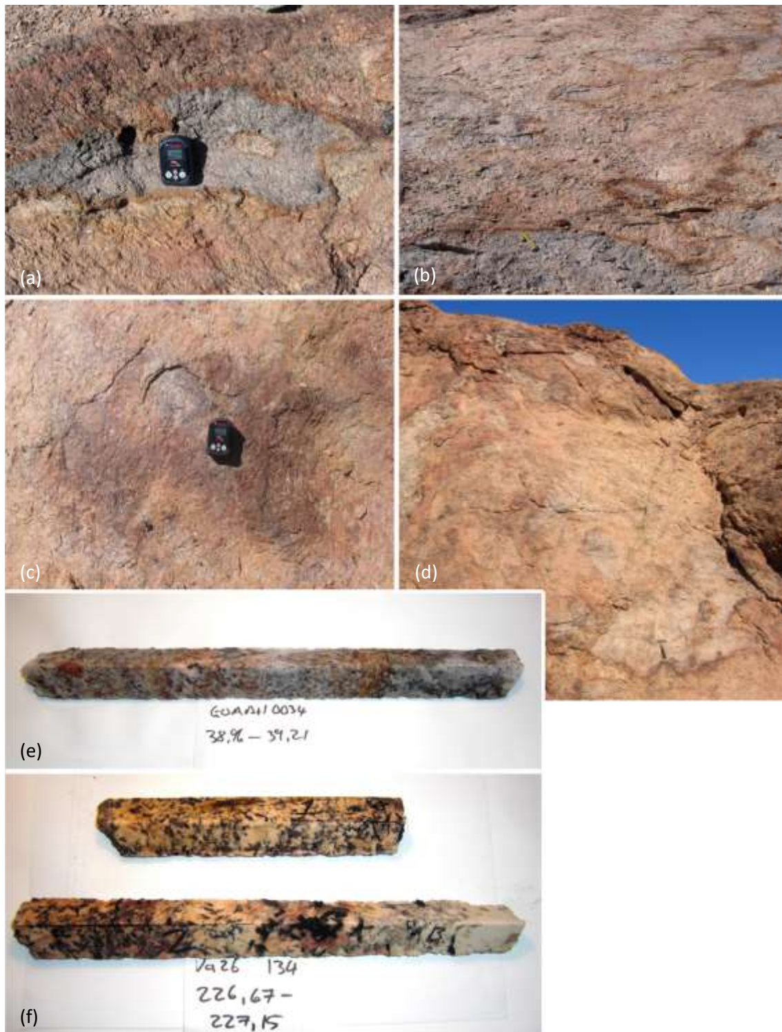
Figure 3.6 Oxidation halos in sheeted leucogranites of the Central Zone. Fe dominated discoloration is characteristic of many of the mineralised leucogranites from the Central Zone. (a) A composite halo at Ida Central, two oxidation fronts are clear; a red coloured massive halo surrounds a smaller grey-coloured core, which in turn surrounds a white coloured core. (b) Pavement exposure of oxidation halos at Garnet Valley. (c) Patch of haematite staining at Valencia, these are not but discolouration associated with magnetite and biotite alteration accompanied by elevated cps readings. (d) E-type sheeted leucogranite locality with characteristic oxidation halos, at Ida Central. (e) Haematite stained patches occur in fresh core samples from Valencia, but distinctive halos are not present. (f) The halos are present in relatively fresh material from Goanikontes, the core of the halo and its haematite-limonite rim are clearly visible.
