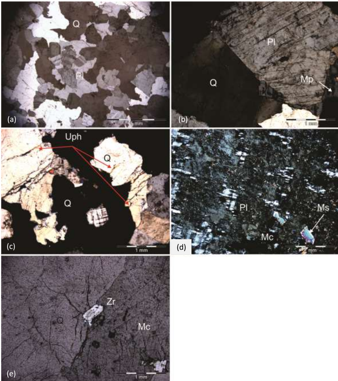
Figure 4.33 Features of mineralised sheets from the Ida Dome area. (a) Amoeboid quartz with sub-rounded plagioclase (Pl), xpl. (b) Euhedral plagioclase, in planar contact with quartz and irregular contact with microcline-perthite (Mp), IDAG 34, xpl. (c) Anhedronal embayed quartz (Q) surrounds microcline and has planar boundaries with plagioclase (bottom left) and fractures in some quartz are filled with U secondary phases (top left) IDAG 34, xpl. (d) Alteration of plagioclase (Pl) to microcline (Mc) in a D-type, the accessory microcline is common to altered samples, IDAG 03, xpl. (e) Accessories such as zircon (Zr) are common in most Ida Dome samples, particularly those with biotite. Zircons are often zoned and surrounded by radiating fractures and are often in clusters, IDAG 46, rfl.
