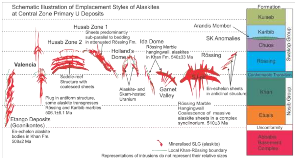
Figure 3.2 Diagram of sheeted leucogranite intrusion styles at the major Central Zone uranium deposits. The deposits primarily occur within the upper Nosib Group and lower Swakop Group. The Rössing Formation is a key assemblage of reactive metasediments at the Rössing Mine and is host to the bulk of uranium-bearing leucogranites at Husab, though its presence is not essential, the Etango deposit at Goanikontes for example is hosted almost entirely within the Khan- and Chuos Formations.
