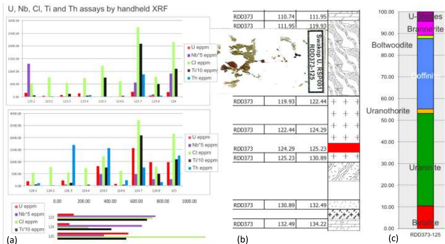
Figure 5.56 The RDD373 124-125 m sample with thin section locality and handheld XRF assay data. The sample is an altered alaskite with prominent biotite content and pervasive fracturing throughout the mineralised interval. High cps readings are localised over biotite clusters. (a) A systematic 10 cm assay scheme with handheld XRF values highlights discrete sites of elevated Nb with corresponding elevated Ti. (b) The sample is situated in an 8-m thick pegmatite-alaskite with prominent coarse-grained biotite. (c) The department study by QEMSCAN reveals 10 wt.% U in betafite combined with brannerite for 16.94 wt.% U in refractories. This sample in particular shows that potential exists for XRF analyses as a means of identifying refractory-bearing targets. (d) Illustration of the distinctive alaskite texture.
