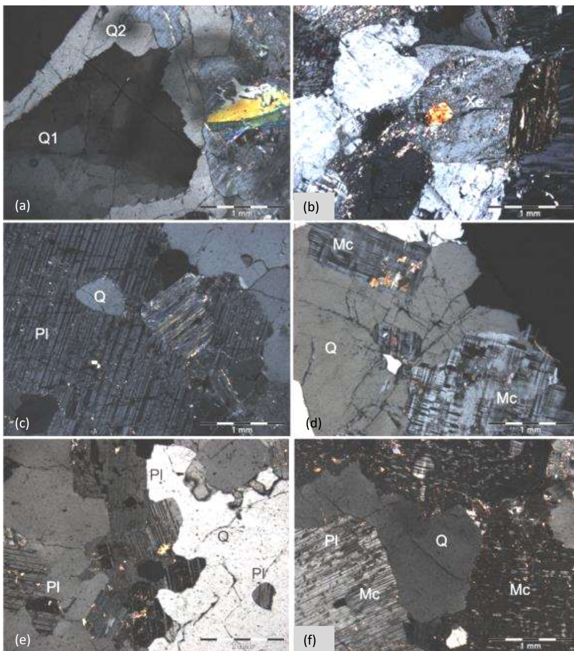
Figure 4.26 Petrographic characteristics of Goanikontes D-type sheeted leucogranites. (a) Quartz may be the dominant rock-forming mineral and is often in at least two generations, new quartz (Q2) grows between K-feldspar and an older quartz grain (Q1). Strain extinction is present in both quartz generations and the feldspars. DH025 353.60-354.03, xpl. (b) Accessory phases such as xenotime (Xe) contribute to anomalous Y concentration in many D and E-type Goanikontes sheeted leucogranites, DH012 342.47-342.84, xpl. (c) Plagioclase is the dominant feldspar in the D-type sheets and often contains inclusions of quartz and occasional biotite (always chloritised) DH019 13.75-14.15, xpl. (d) Microcline is the subordinate phase in most samples and has embayed contacts with quartz grains as well as typical globular quartz inclusions, DH025 353.60-354.03, xpl. (e) Anhedra quartz (Q) surrounds euhedral and anhedral plagioclase (Pl) DH012 127.72, xpl. (f) Microcline (Mc) development after plagioclase (Pl) with strained quartz veinlet (Q) DH012 127.72-128.04, xpl. Goanikontes E-Type Sheeted Leucogranites
