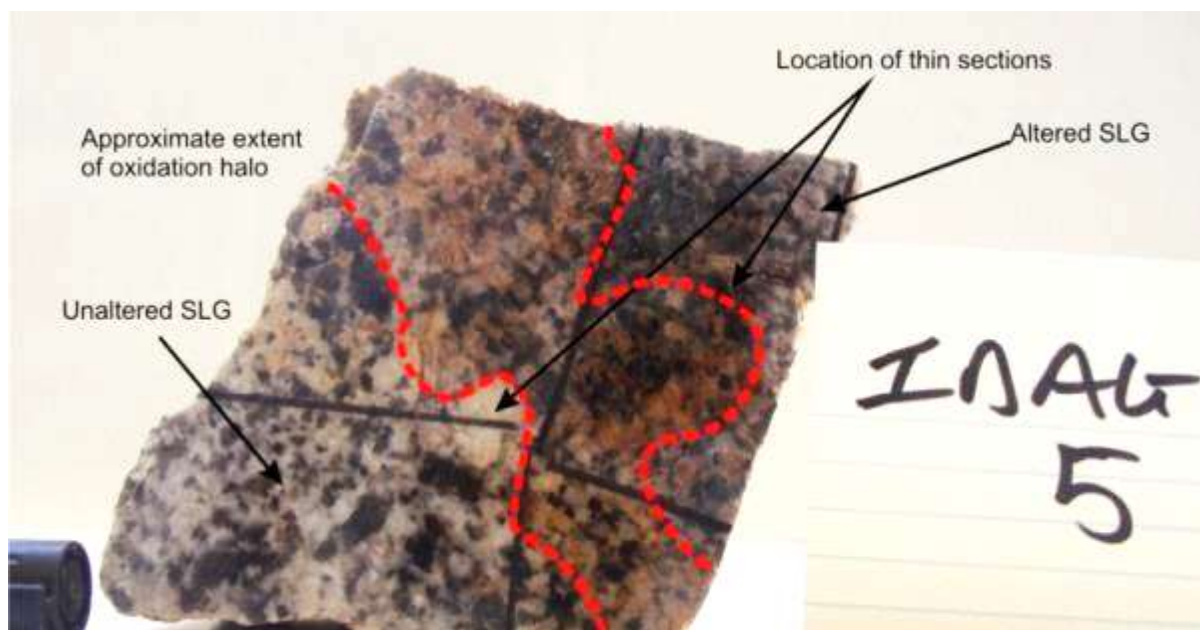
Figure 3.61 Mineralised sheeted leucogranite from Ida Central with typical E-type oxidation. The unaltered portion has typical D-type 'black and white' coloration, while the feldspars on the outside of the halo (top left of sample) have a distinct pink coloration. The unaltered leucogranite is examined in thin section IDAG 05a and the altered in section IDAG 05b (thin section slides are in Figure 4.34).
