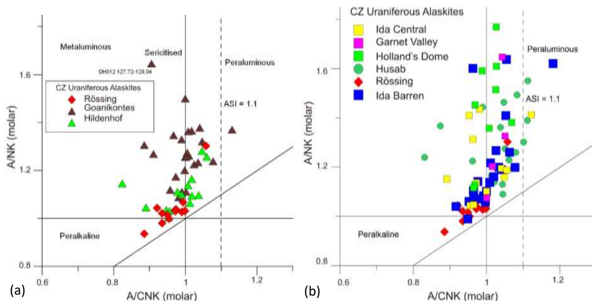
Figure 5.17 Aluminium saturation diagrams of uraniferous sheeted leucogranites. (a) Aluminium saturation diagram of Goanikontes and Hildenhof mineralised sheeted leucogranite. The variety of alteration in Goanikontes samples results in greater deviation from the Rössing trend than the Hildenhof samples, which are all surface samples. Rössing sample data: Freemantle (2006). (b) Aluminium saturation diagram of Ida Dome area and Husab mineralised sheeted leucogranite. Ca content contrasts significantly between the deposits at the Ida Dome. The Holland's Dome samples have the highest deviation from the Rössing sample trend as a result of Ca mobility during interaction with the numerous skarn pods at the deposit. The Ida Central samples have a closer fit to the Rössing samples. Rössing sample data: Freemantle (2006).
