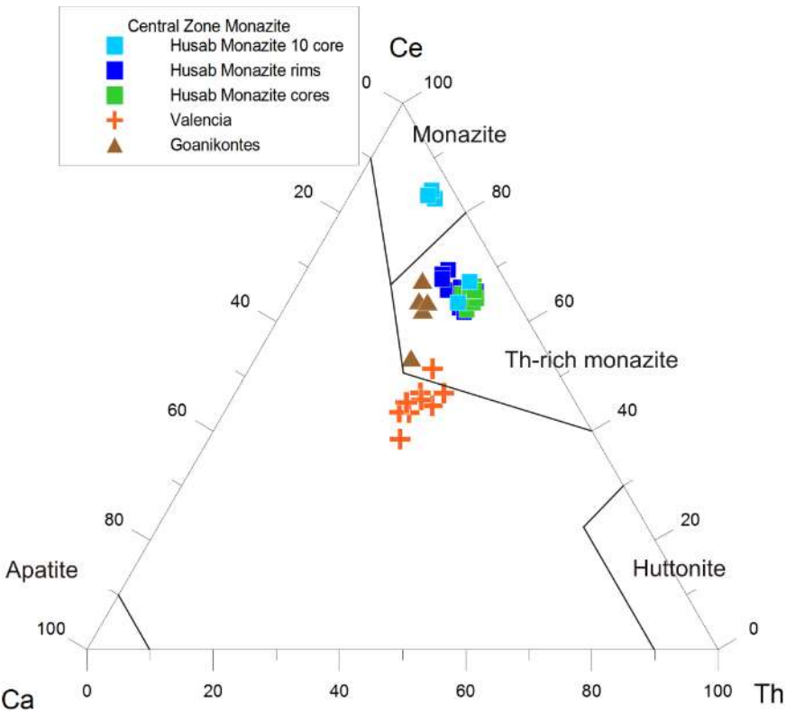
Figure 6.23 Ce-Ca-Th ternary plot of CZ monazite. Ternary compositional plot with fields of Ward et al. (1992) place the alaskite-hosted monazite in the high-Th field, which also supports an REE retention hypothesis.
