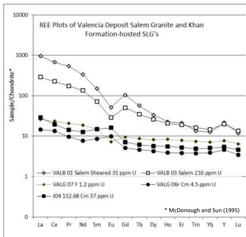
Figure 6.12 The Khan Formation-hosted Salem suite and leucogranites at Valencia. The collection comprises two Salem suite granites, two magnetite-bearing pre- syn-D 3 C-type sheets, and an F-type pegmatite. The more primitive Salem samples are relatively enriched in LREE, the sheared sample (VALB01) is the most enriched, where incompatible LREE partition into melt bands along conjugate shear sets.
