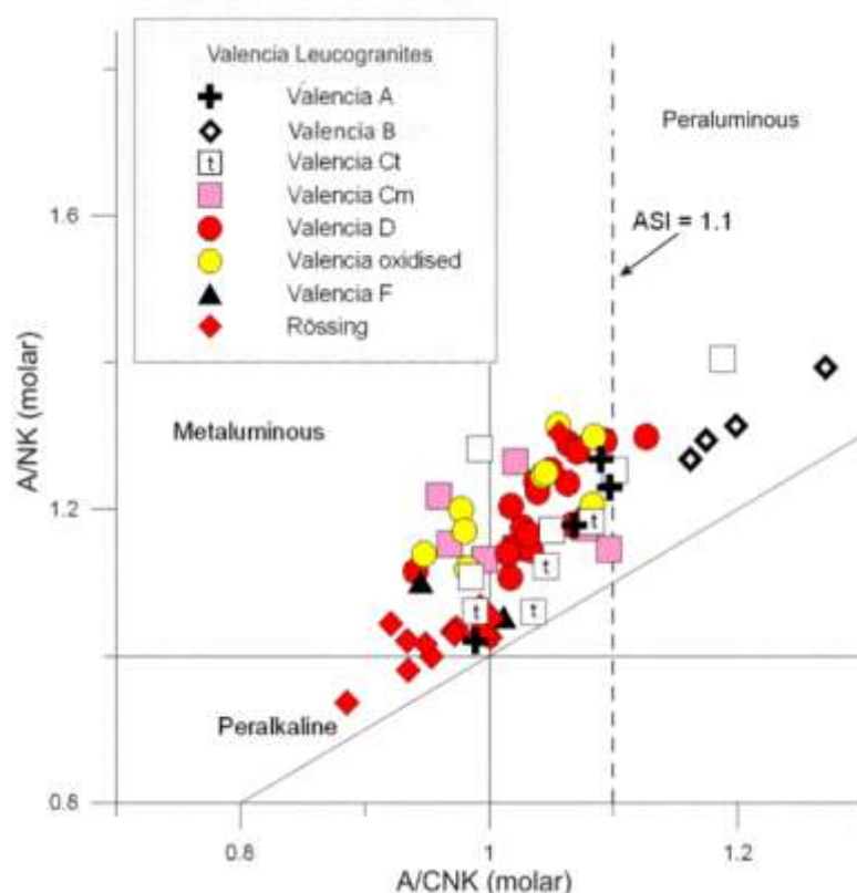
Figure 5.16 Aluminium saturation diagram of the Valencia leucogranite suite. The variety of leucogranites at Valencia cluster to the left of ASI = 1.1 , the B types are the most peraluminous and the Ct-types follow the 1:1 line nearer than the other C types. The D-types are all more peraluminous than the oxidised varieties. Rössing sample data: Freemantle (2006).
