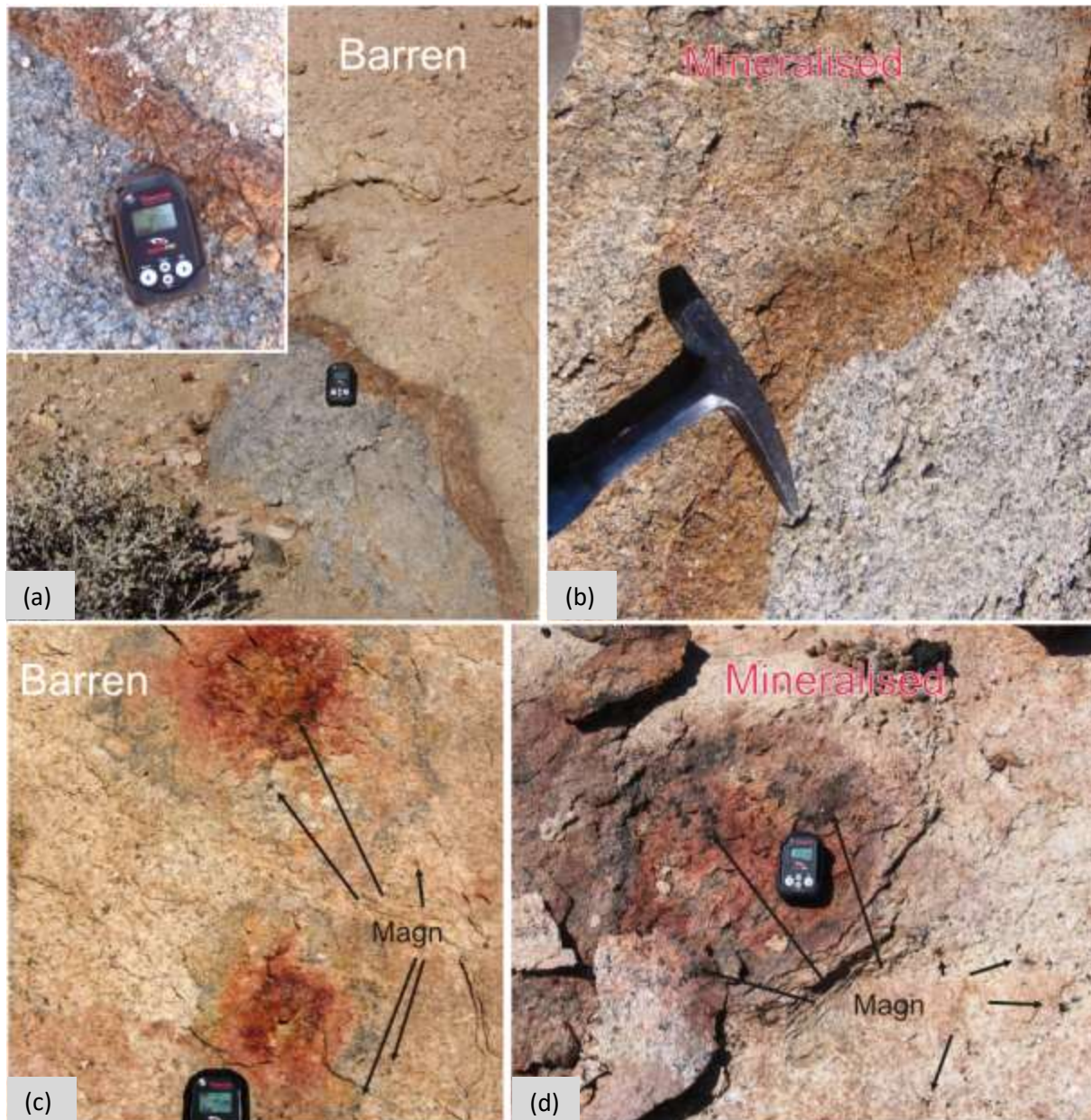
Figure 3.7 Varieties of oxidation halos in barren and mineralised leucogranites. (a) A barren halo at Ida Central is characterised by limonite-brown staining and a deep blue-grey core. The granites are only weakly radioactive and occur lower down in the Khan succession than the more mineralised varieties, at both Garnet Valley and Ida Central. (b) An unaltered mineralised core and halo at Holland's Dome appears near identical to the barren variety, it does however have a slightly lighter grey core. (c) Barren haematite stains in magnetite-bearing C-type granite near the core of the Ida Dome, note the limonite coloration in the cores. (d) A haematite stain at Holland's Dome, the large magnetite porphyroblasts and deep red-pink colour discriminates it from the U-barren stains. It is adjacent to a skarn pod and is itself actually the remnant of a skarn fragment.
