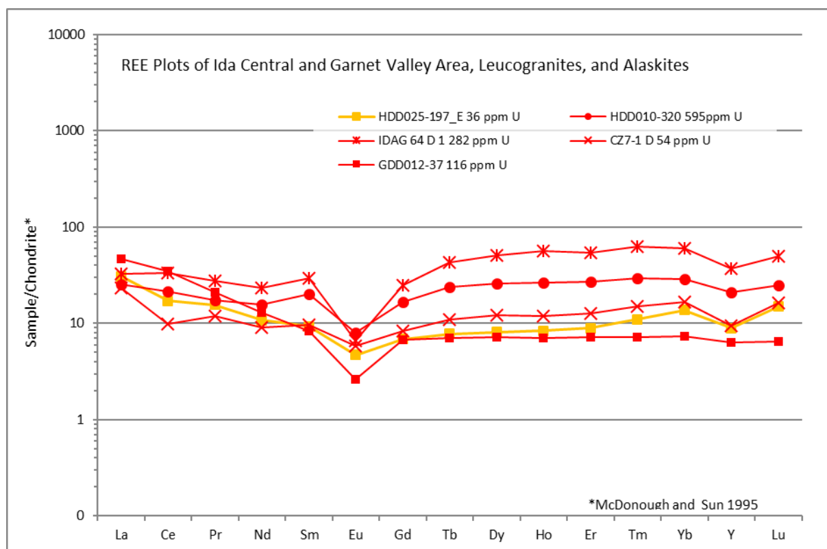
Figure 6.10 REE plots of Ida Dome Area leucogranite and alaskite. The mineralised samples show enriched HREE, with consistent Y < Lu at Garnet Valley. The Garnet Valley-Ida Central C-types show negative slopes with -Eu and weakly +Eu (IDAG09) and the uraniferous alaskites contrast with pronounce -ve Eu anomaly and gull wing type patterns of HREE enrichment.
