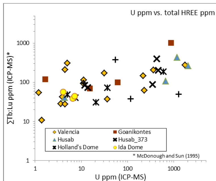
Figure 6.4 Uranium content vs. \Sigma HREE from Tb through Lu. The plot shows a strong positive trend between U and HREE. Heavy rare earth enrichment occurs in low grade Valencia samples, which host prominent quantities of garnet porphyroblasts.
