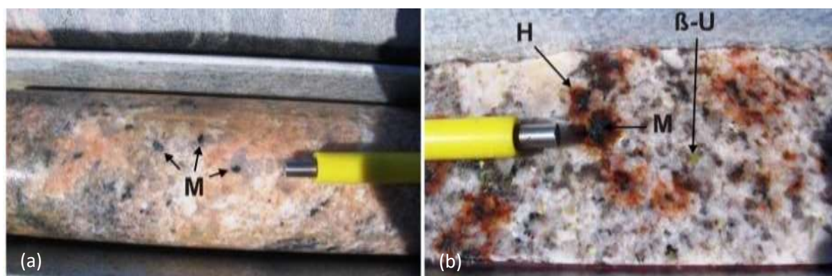
Figure 3.58 Magnetite in barren and mineralised core from Goanikontes hole DH025. (a) Magnetite (M) crystals up to 1 cm across occur in barren, magnetite-bearing C-type sheeted leucogranites at Goanikontes. Note that there are no halos of haematite around the magnetite crystals. (b) Haematite (H) halos surround magnetite in mineralised sheets, often accompanied by \beta -uranophane ( \beta -U).
