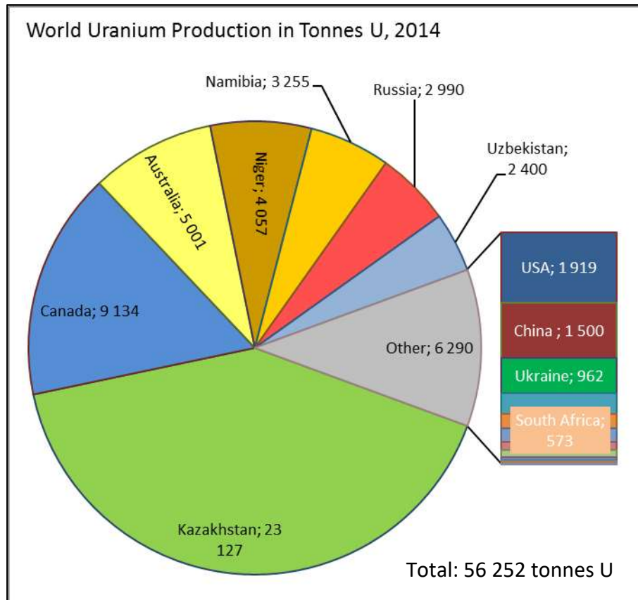
Figure 1.3 World uranium production by country for 2014. Combined with Langer Heinrich, Namibia's Rössing Uranium Mine produces 8% of world uranium production. The 2013 total of 59 673 tU accounted for 90 % of world demand. The deficit is made up of recycling of spent fuel, dismantling of spent fuel rods, and stockpiles. (Statistics from: The World Nuclear Association, 2015)
