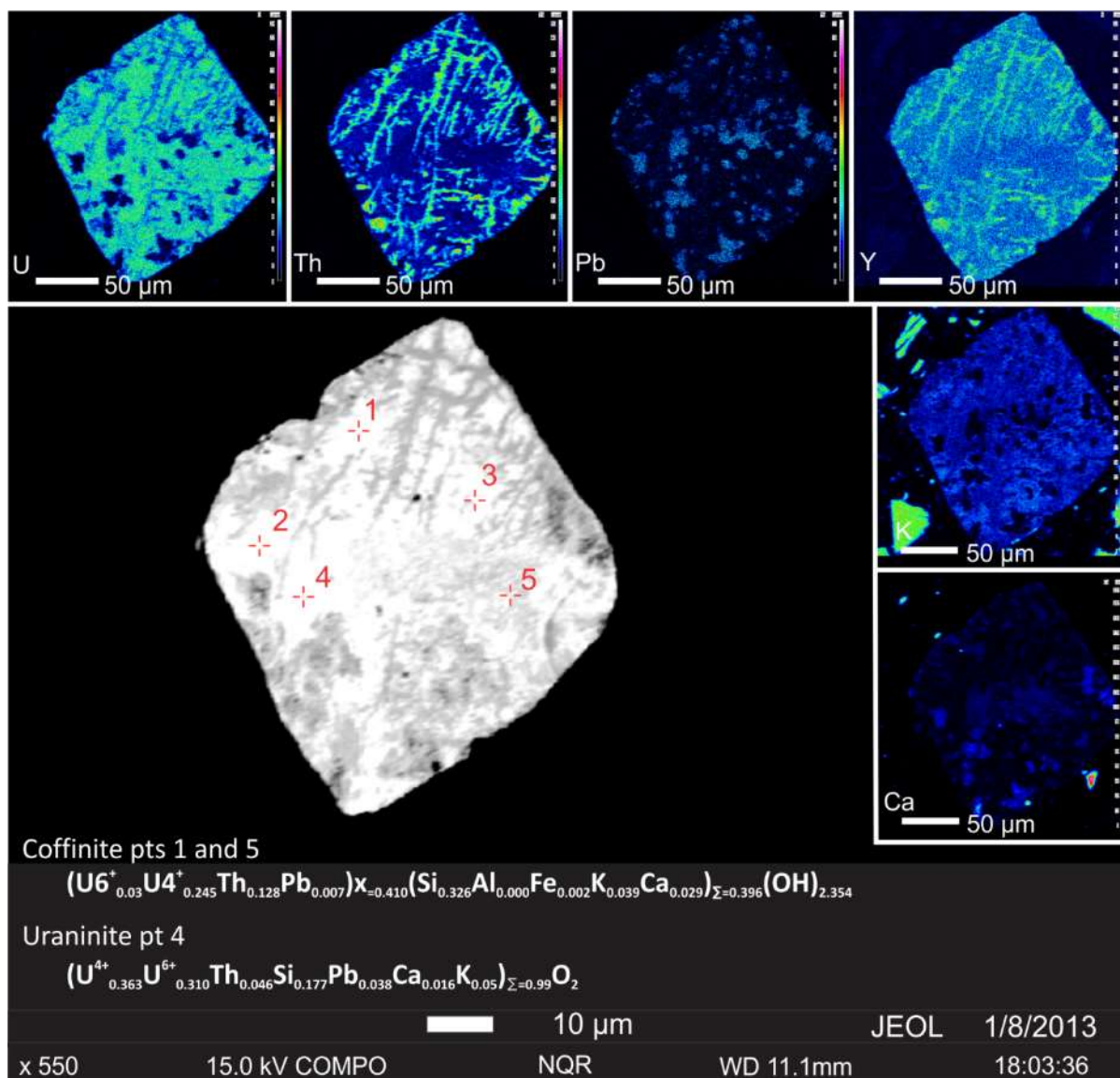
Figure 8.15 Coffinite replacement of uraninite U1 from Va26 113 225m. The backscatter image at centre is of a euhedral uraninite with clear leaching of metal along preferred fracture pathways, with highest density, U-rich material somewhat preserved in the core of the specimen. The fracture pathways have lost U6+ and Th remains as a relatively concentrated component. Y is coincident with Th and may be concurrent with new phosphate deposition (potentially monazite with xenotime). Pb and U are inversely abundant, and represent Pb deposition (galena). K correlates with U abundance and is the most common impurity after Si at points 1 and 5.
