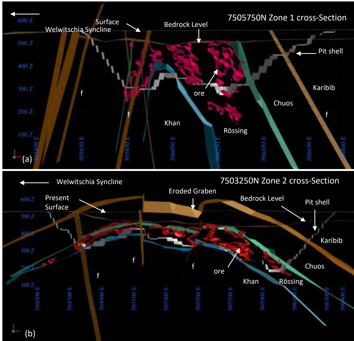
Figure 3.34 Cross-sections of the Husab Zone 1 and Zone 2 deposits. Both views look north with "Z" representing altitude above sea level and "E" representing Eastings in UTM (WGS84). Colour codes: Magenta - Mineralised leucogranite ore zones (Zone 1); Red - Mineralised leucogranite ore zones (Zone 2); Tan - Base of the Karibib Formation; Light Green - Base of the Chuos Formation; Blue - Base of the Rössing Formation; Brown - Fault Planes; Light Grey - Planned Pit Shells. (a) Mineralisation occurs in granites confined to the Rössing Formation in the limbs of the Husab Antiform at Zone 1, where the hinge is lost to erosion. (b) The Zone 2 section of the deposit occurs where the antiform hinge is preserved, the fold structure is more open and mineralised sheets conform more closely to the host rock bedding orientations. Geological Interpretation by Neale Culpan of Extract Resources, 2008 to 2012.
