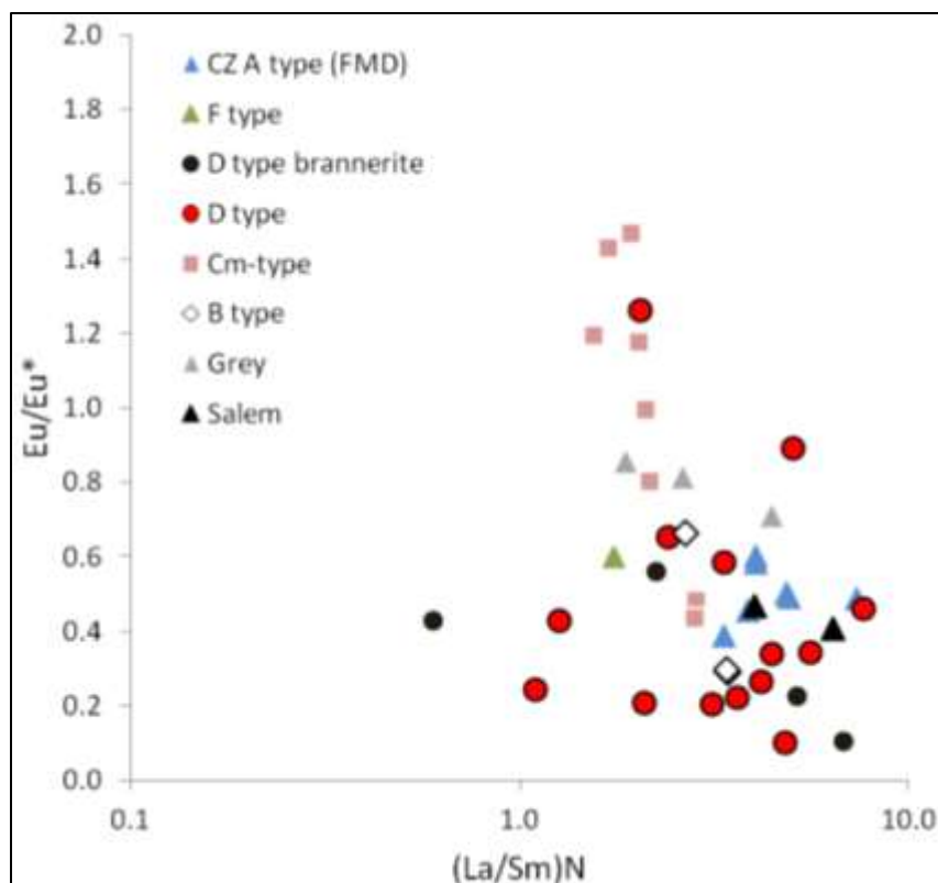
Figure 6.19 \text{La/Sm} vs. \text{Eu/Eu}^* of the CZ granites and SLGs. The uraniferous alaskites have strongly negative Eu anomalies, as do the Salem type diorites at Valencia (this study); and the A type Sorris-Sorris, Dachsberg, and Horebis River granites (data from McDermott et al. , 2000). The strong negative Eu ( \text{Eu/Eu}^* ) is indicative of a plagioclase-bearing source in which Eu is in a similar oxidation state to Ca, and is preferentially retained during partial melting.
