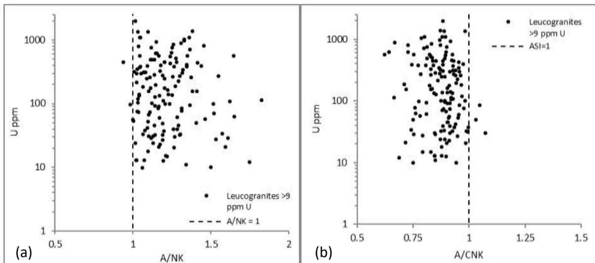
Figure 5.46 U vs. A/NK and U vs. A/CNK of the Central Zone sheeted leucogranites. (a) The Peralkaline index after Shand (1927) vs U. U abundance does appear to show some positive relationship with aluminium saturation, measured against the peralkaline index of Shand (1927) (b) The metaluminous - peraluminous index of Shand (1927) vs U does not show any such positive relationship.
