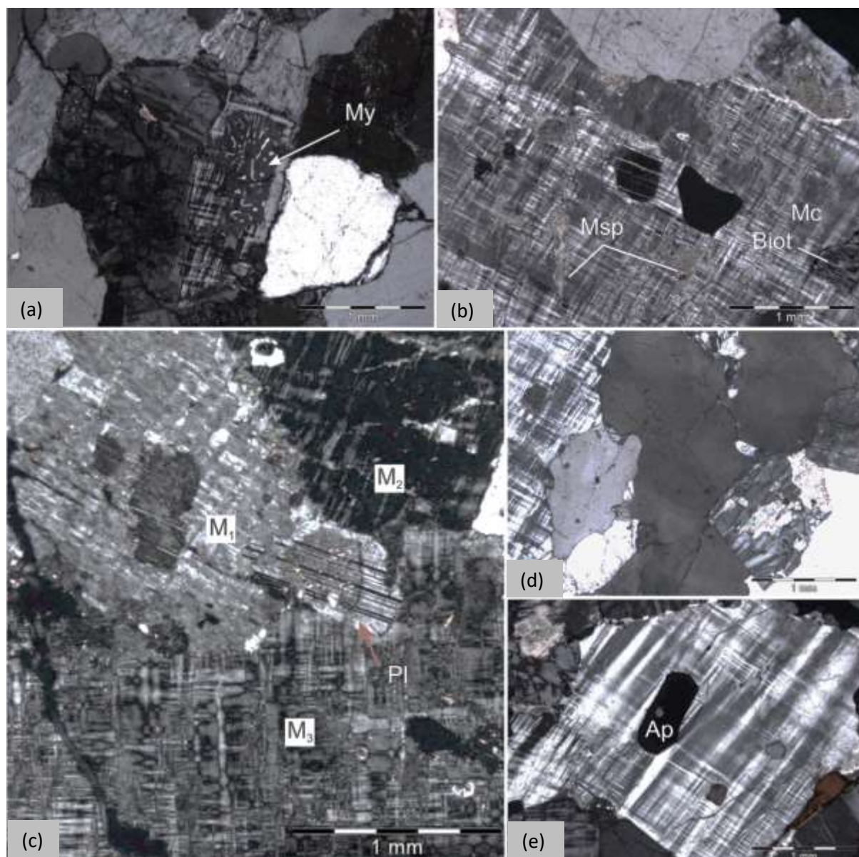
Figure 4.14 Common features in C-type sheets at Hildenhof. (a) Myrmekite in a plagioclase inclusion within microcline, HILG 27, xpl. (b) Zoned plagioclase inclusions in microcline, HILG 25, xpl. (c) Zoned plagioclase at a junction of three microcline grains, note the round quartz inclusions in microcline (bottom right), HILG 26, xpl. (d) Strained quartz embayed with microcline, muscovite inclusion in microcline (bottom right) and euhedral plagioclase adjacent to quartz (centre right) HILG 27, xpl. (e) Apatite (Ap), biotite and quartz inclusions in microcline, accessories are scarce in the U-barren sheets at Hildenhof, HILG 22, xpl.
