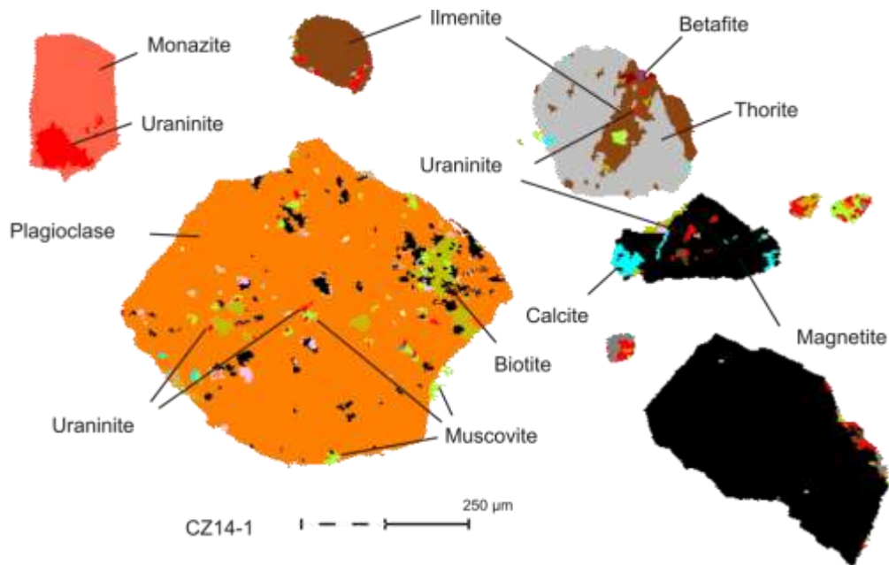
Figure 7.7 Mineral map features of CZ14-1, surface sample E-type from Rabbit Valley. Uraninite in the Ida Central sample is a secondary crystallisation phase that adheres to magnetite and ilmenite/rutile. It also occurs as large inclusions (or as compound grains) in euhedral monazite, and as fine inclusions associated with biotite and magnetite in plagioclase feldspars.
