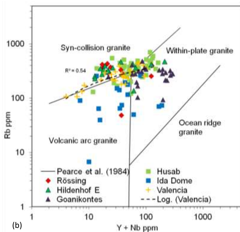
(b) The uraniferous sheets at the primary deposits show a number of trends; the CaO-rich Ida Dome samples plot with low Rb in the volcanic arc field, the Valencia samples show a systematic relationship with Y+Nb along the syn-collision volcanic arc line, the Goanikontes sample plot in the within plate field, and the Husab samples plot with relatively high Rb near- and in the within-plate field. The comparative Rössing samples tend to plot in the syn-collision field. The Valencia samples show the most obvious positive trend between Y+Nb and Rb. The trend is weakly apparent in the Husab samples, and less so, in the sample suites for the Ida Dome and Goanikontes deposits.
