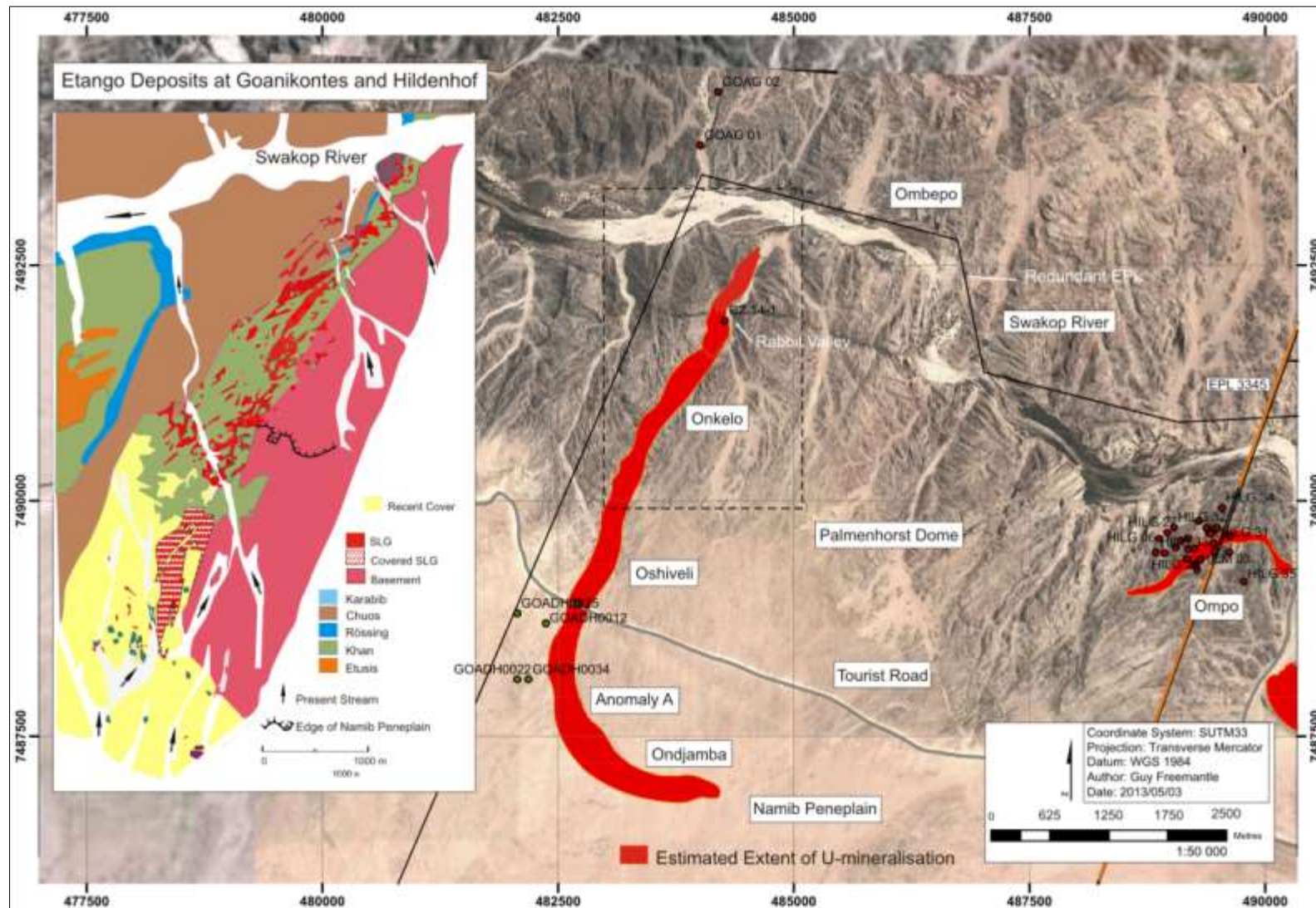
Figure 3.14 The geology of the Goanikontes area west of the Goanikontes Dome. The map shows the sheeted leucogranites predominantly intruding the Khan and Chuos Formations, Bannerman Mining Resources' Etango Project 'Anomaly A' (from Nex, 1997 modified after Mouillac et al. , 1986 and Marlow, 1983, colour-altered Quickbird® image after Google Earth®).
