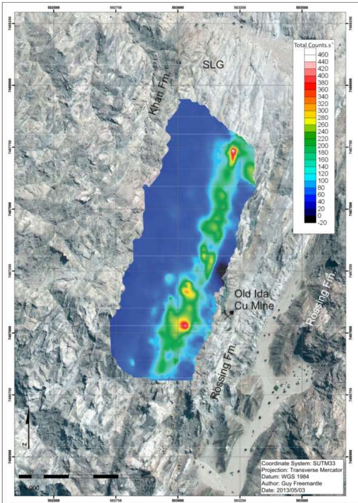
Figure 3.26 Radiometric anomalies on surface in the vicinity of the Ida Cu Mine. A handheld scintillometer survey was conducted over a portion of Ida Central, along the contact between the overhanging Rössing marbles and the underlying diopside gneiss of the Khan Formation. The majority of the granite intrusions do not transgress the marble barrier, and Cu and U mineralisation tend to concentrate along strike beneath the marble units. SLG: - sheeted leucogranite.
