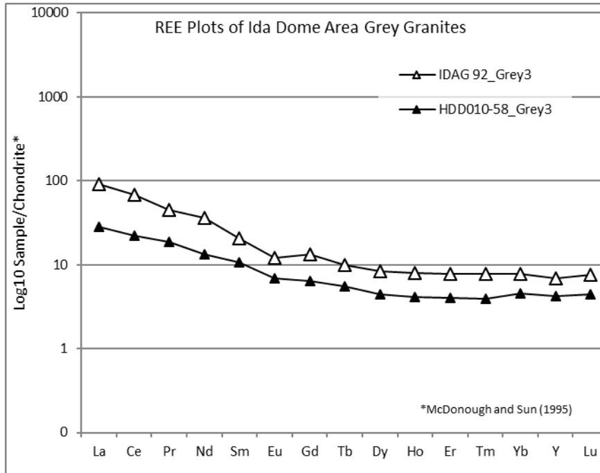
Figure 6.8 REE abundances of Ida Central and Holland's Dome Grey granites. The Grey granites have a negative slope from LREE to HREE, with only a weak -ve Eu anomaly in the Holland's Dome sample.
