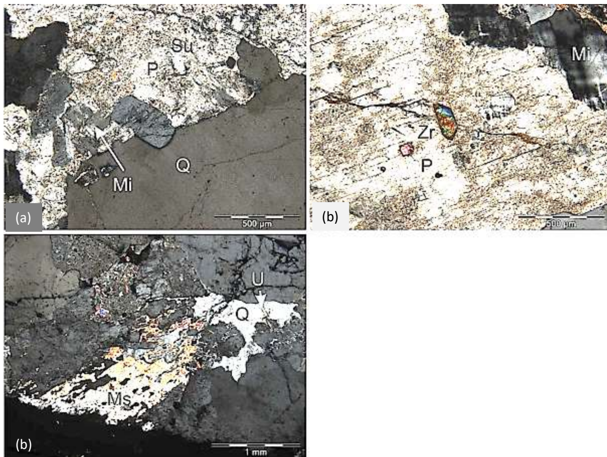
Figure 4.15 Ct-type Sheeted leucogranites at Ida Dome. (a) Apatite (Ap) is a frequent accessory phase in CZ granites. Microcline (Mi) is growing over plagioclase (Pl) IDAG 19, xpl. (b) Zircon is a common U repository in Sheeted leucogranites and occurs as singular and clustered grains, IDAG 22, xpl. (c) Skeletal muscovite is indicative of an entrained sedimentary lath IDAG 22, xpl.
