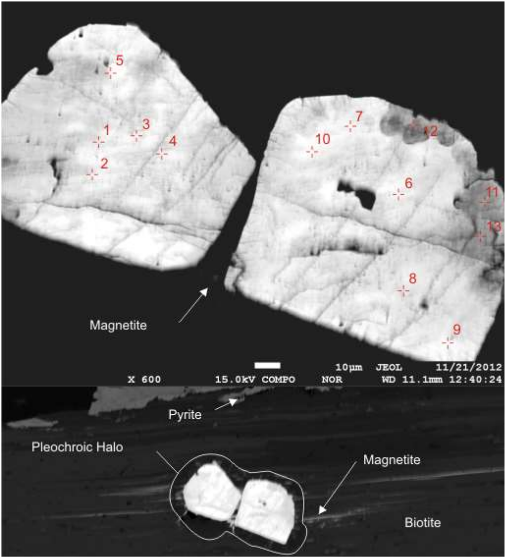
Figure 8.17 Composition and texture of uraninite U7, hosted in biotite of sample RDD373-125 m. (a-b) The uraninite grains are euhedral and surrounded by a halo of alteration in the host biotite. Grain sizes are ~100 µm across. (c) Si, Th, Pb and contaminant phases (MoS 2 ) contrast between core and rim; U and Pb ranges in the core are ~4 x greater in the rim, Th range is ~8 x greater in the rim, Si range is ~16x greater in the rim, and total contaminants are ~3 x greater in the rim.
