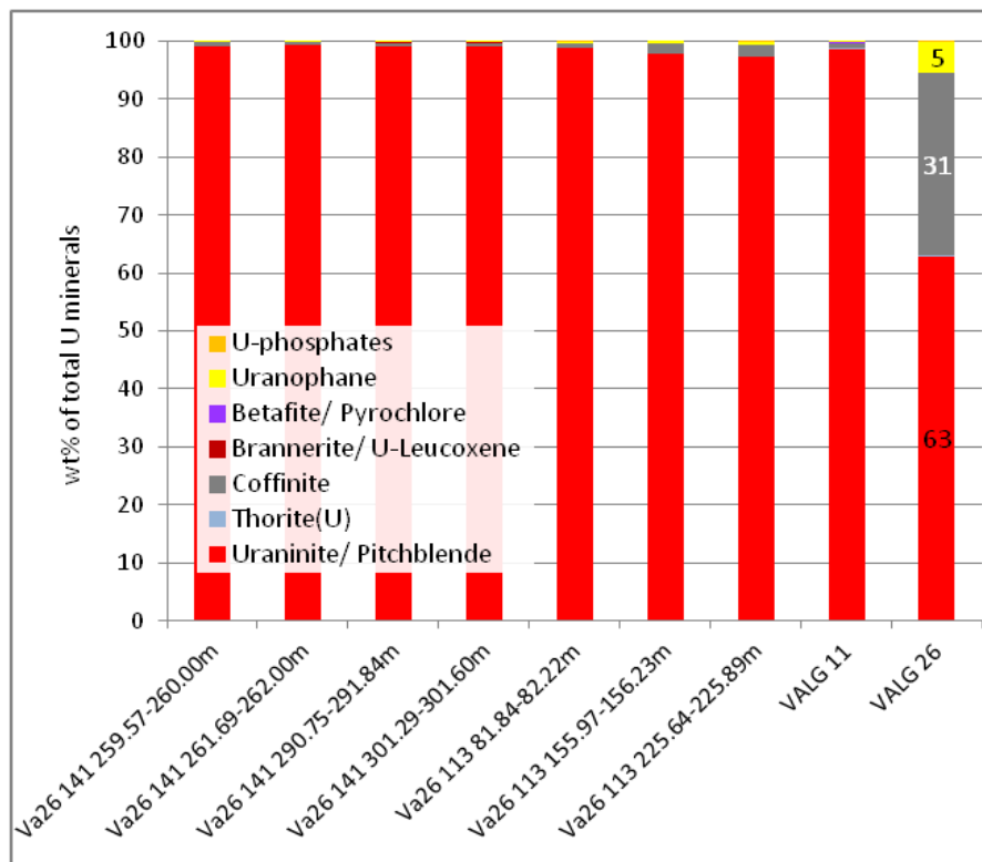
Figure 7.21 Uranium deportment statistics of the Valencia QEMSCAN samples. The dominant mineral is uraninite, which accounts for over 90 % of the uranium budget in all but one sample, VALG26. VALG26 is a surface sample collected at a location stratigraphically above the Karibib Formation marble, and hosts ~30% of the U in coffinite.
