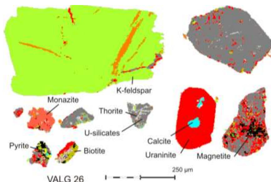
Figure 7.26 Mineral map features of VALG26. Uraninite tends to be fine-grained, and large grains have mostly altered to coffinite/uranophane. Albite, and secondary uraninite and coffinite/uranophane fill the cleavage planes of K-feldspar. Unaltered uraninite shows evidence of cavities, which are filled with calcite.
