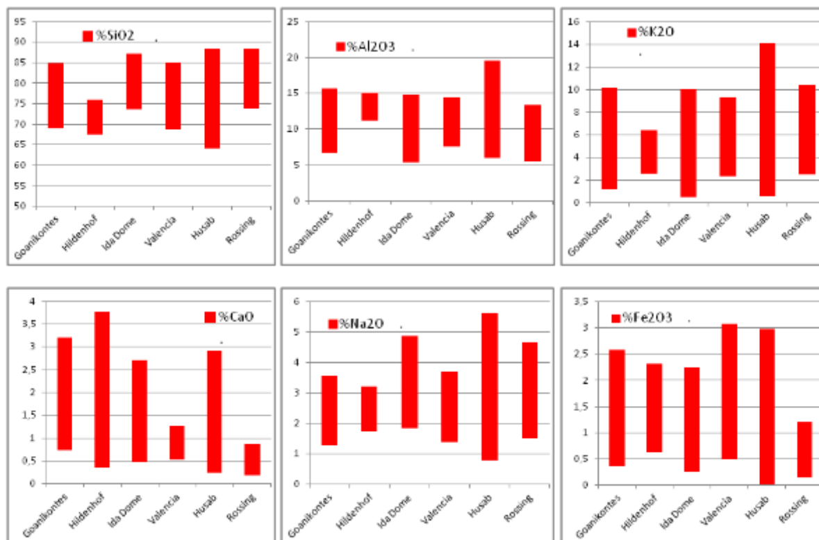
Figure 5.2 Major element abundances of the uraniferous leucogranite populations at the Goanikontes, Hildenhof, Ida Dome, Husab, and Valencia Deposits. Rössing data from Freemantle (2006).
