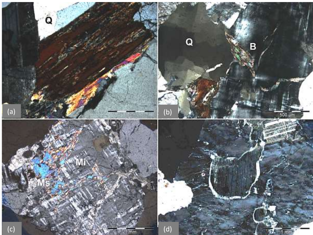
Figure 4.51 Oxidised D-type sheeted leucogranite from Valencia. (a) Va26-141 259.57-260.00, xpl; large biotite blade altering to chlorite. The euhedral quartz (Q) forms clusters and veinlets up to 10 mm in extent. (b) VA26-141 259.51-260, xpl; strained quartz (Q) and chloritised biotite are typical in the oxidised sheeted leucogranites at Valencia and the other deposits. (c) Va26-111 157.44-157.82, xpl; Anhedral microcline with perthite parallel muscovite development, in some microcline muscovite is cleavage-parallel. (d) Plagioclase is often surrounded by albite, this sample shows mesoperthite in the microcline that surrounds the plagioclase (P) Extinction angles seem to be consistent between the core and rim, typical of subsolidus type alteration.
