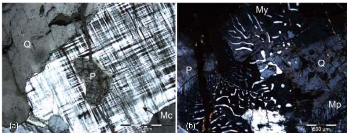
Figure 4.28 Features common to the majority of mineralised sheeted leucogranites at Hildenhof. (a) Albite-rimmed Oligoclase in microcline, as in the pre-D 3 sheets quartz exhibits strain extinction, HILG 12, xpl. (b) At least four mineralised samples contain myrmekite; it occurs in cores of plagioclase but rarely in the rims. Plagioclase without cores and little sericite tend to have the best-developed quartz intergrowths, HILG 19, xpl.
