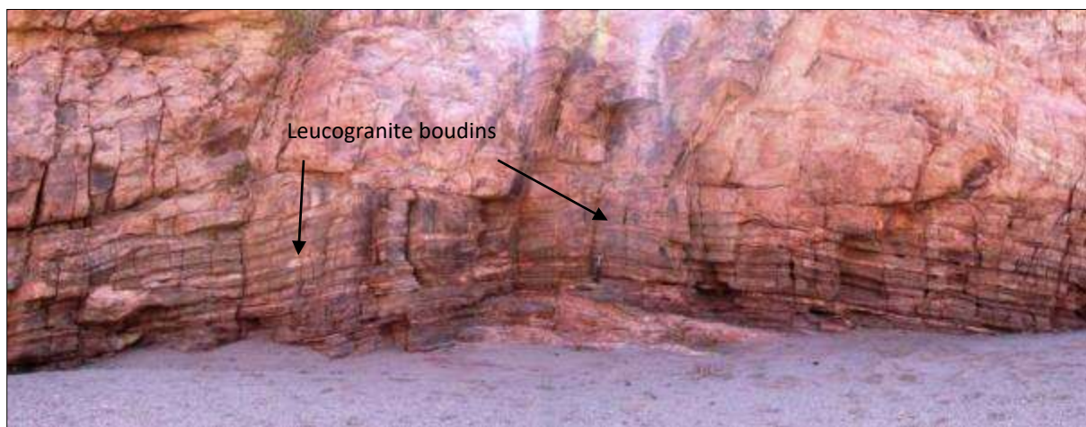
Figure 3.42 Migmatised Etusis Formation at the Valencia deposit. The location is northwest of the main deposit where the Nosib Group unconformably contacts the Abbabis inlier. The banding is predominantly compositional (S 0 ) while strain has developed boudins in leucogranite sills.
