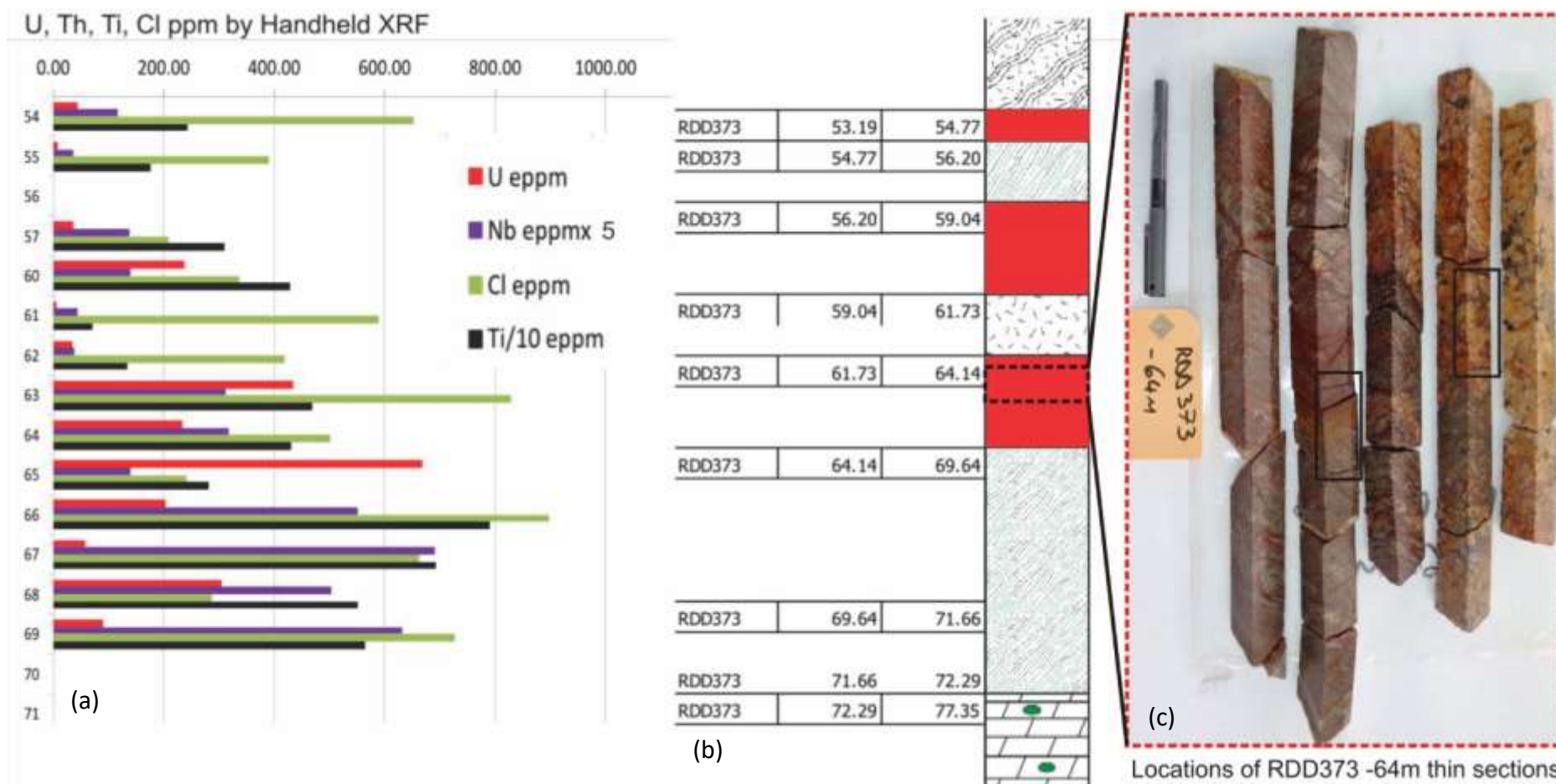
Figure 5.54 RDD373-64 m specimens in hand sample with thin section localities. The footwall is heavily fractured, chlorite schist. Primary mineralisation occurs in the alaskite and in a contact halo that extends ~36 cm into the schist. Mineralisation in the schist is hosted by quartz-calcite veins, and along the cleavage planes of the schist. Mineralisation in the schist is in the form of coffinite and a yellow secondary phases. Boltwoodite and uranophane were identified as the main secondary phase by Townend (2009) in a commissioned study report.
