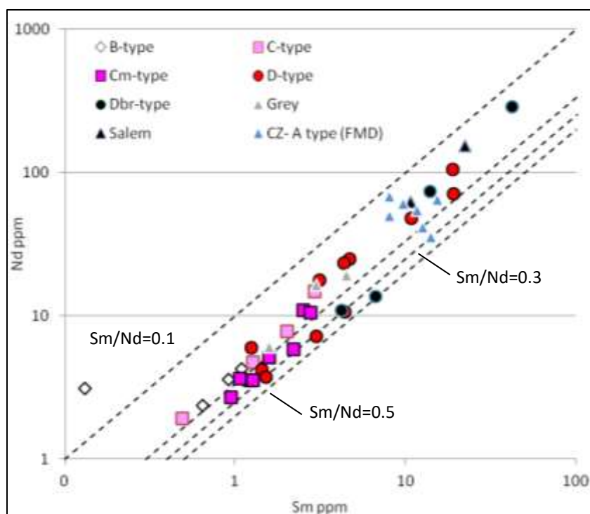
Figure 6.19 REE ratios as discriminators between sheeted leucogranite types. Sm and Nd ratios appear to distinguish between the uraniferous and non-uraniferous sheets; The B-types host Sm/Nd of \sim 0.3 ; the C m -type host Sm/Nd between 0.3 and 0.4, while the relatively enriched alaskites host Sm/Nd close to 0.2. The comparative A type granites of the Central Zone (Sorris-Sorris, Dachsberg, and Horebis River granites) host a range of Sm/Nd and do not show the systematic relationship observed in the sheeted leucogranites (data from McDermott et al. , 2000).
