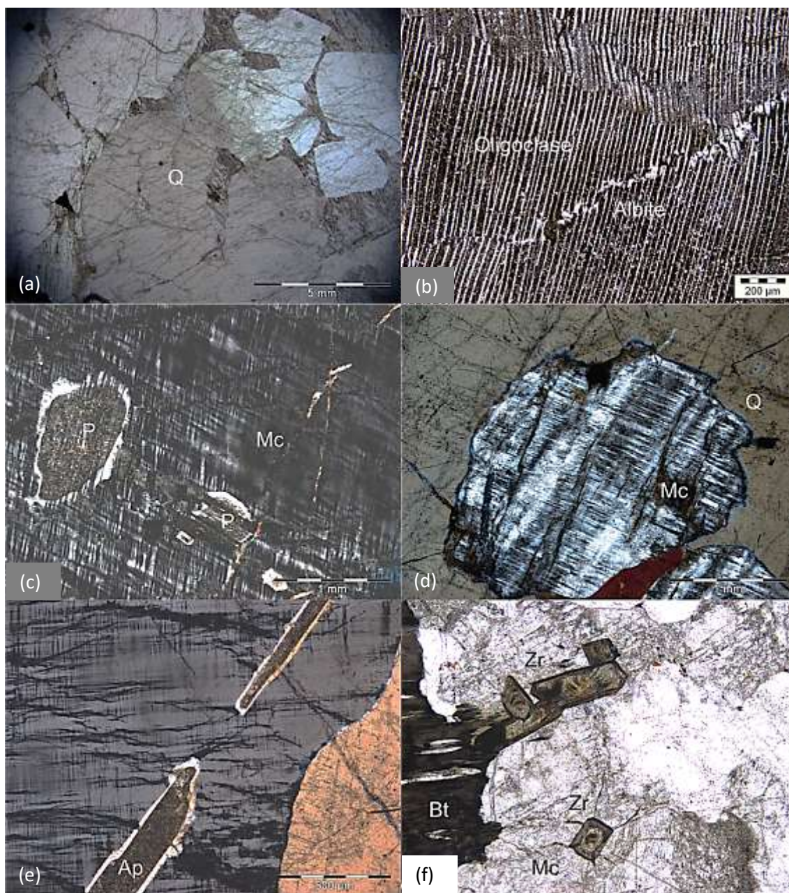
Figure 4.41 Petrographic features of typical D-type alaskites at Husab. (a) Coarse-grained quartz replaces microcline-perthite in RDD006 171-172m, xpl. (b) Husab uraniferous sheeted leucogranites show some evidence of deformation in hand specimen fabric; distortion of crystallised mineral twins (P - plagioclase) reflect some post intrusive event(s) in thin section. Metasomatic activity produced the fine clays in disseminations and hairline fracture-fill, RDD141 244-245m, xpl. (c) Sub-solidus textures include albite rims around primary plagioclase inclusions with sericitised cores, surrounded by tartan microcline, RDD145-413m, xpl. (d) Microcline grain with embayed edges, completely surrounded by quartz, clay alteration preferentially occurs parallel to one of the cleavage planes, RDD145 - 413m, xpl. (e) Apatite is the most abundant phosphate observed in the study, RDD006 - 172m, xpl. (f) Zircon clusters are perhaps the most abundant accessory phases observed, here, in long- and cross-section orientations within K-feldspar. Zircons (Zr) often occur in
