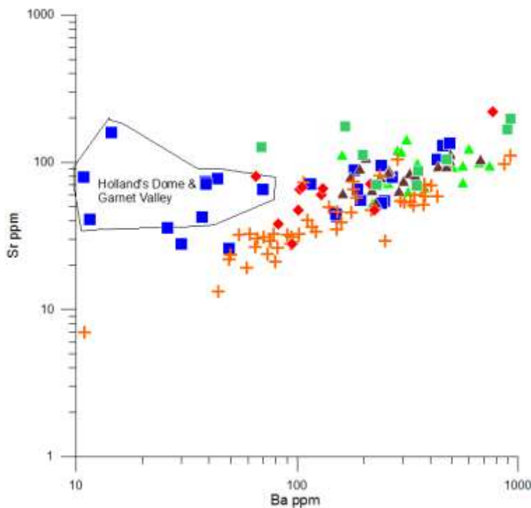
Figure 5.34 Ba vs. Sr in the SLGs.
