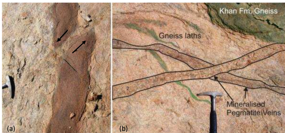
Figure 3.9 Late granitic veins and U-remobilisation in brittle fractures (a) Melts crystallise as coarse-grained granite with smoky quartz and are highly variable in size, but always straight edged. The example is a tension-gash shape between two parts of Grey granite xenolith. (b) Multiple generations of coarse-grained granite veins occur in the massive C-type sheets at Holland's Dome; these propagate from the contacts of gneiss xenoliths and from the edges of patches of D-type sheeted leucogranite. They and have elevated cps readings and usually are accompanied by some discoloration of the older granite.
