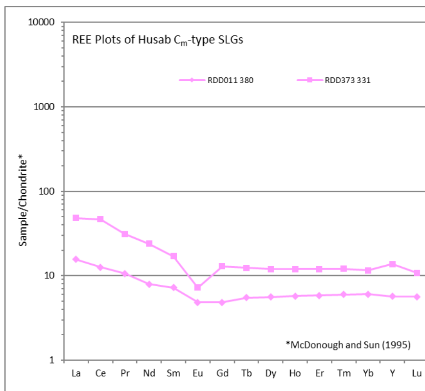
Figure 6.7 REE plots of magnetite C-types from Zone 1, Husab. The RDD373 sample shows a strong -ve Eu, flat HREE and Y > Lu . The RDD011 sample displays a negative slope to Eu, with all REE less abundant than in the RDD373 sample. Ce and La- and Y-phosphates are known to host uraniferous inclusions, and may explain the observations in the plot.
