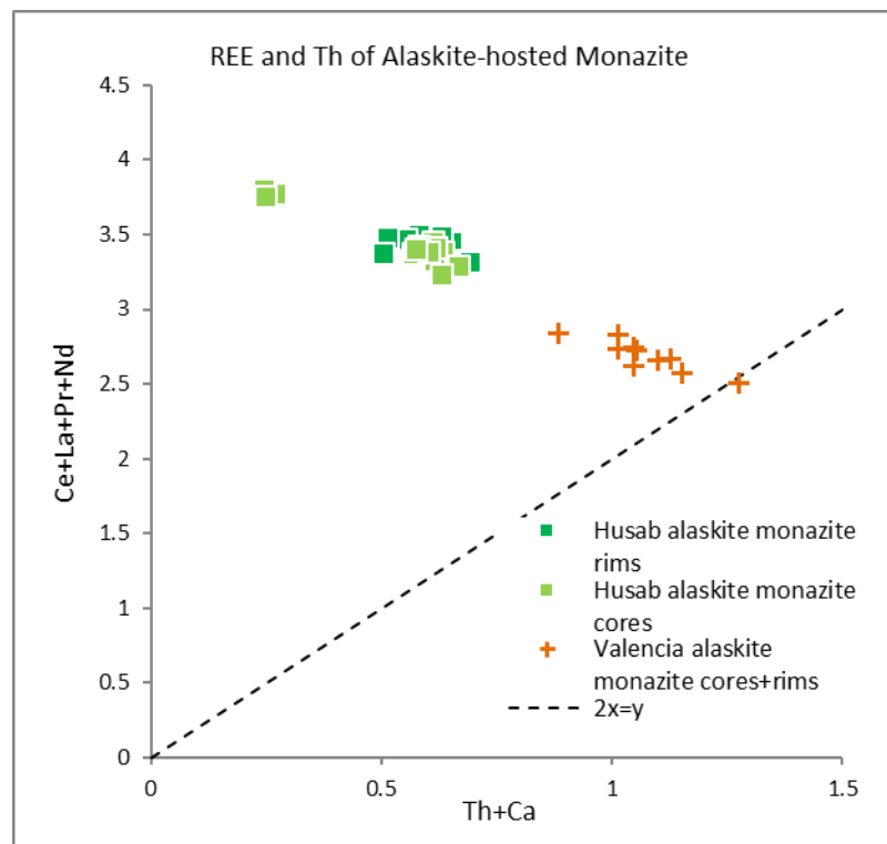
Figure 6.22 Compositional variation of monazite from Valencia and Husab. Th and Ca abundances increase systematically at the expense of the detected LREE. This relationship is not easy to explain, but may simply imply preferential REE retention in the melt or melt source relative to Th.
