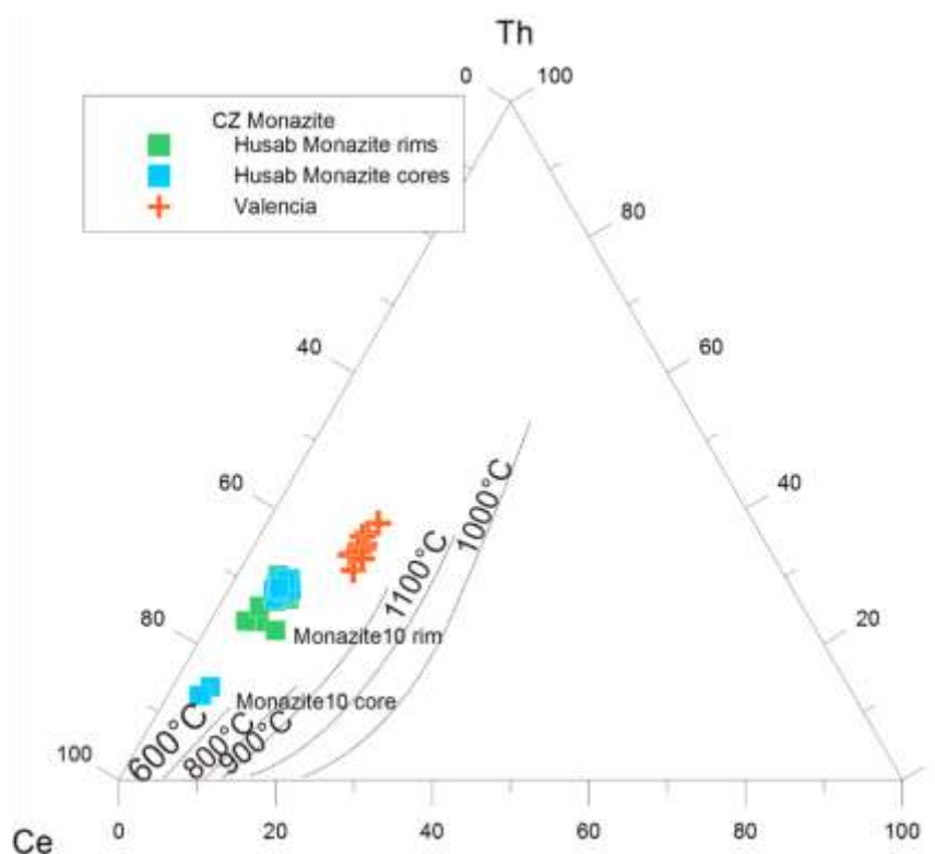
Figure 6.25 Monazite compositions on a ternary diagram of Y-Th-Ce with temperature fields of Gratz and Heinrich (1997). The plots imply comparable T to the peak metamorphic conditions that are widely accepted during alaskite emplacement (e.g. Longridge, 2012; Longridge et al. , 2014).
