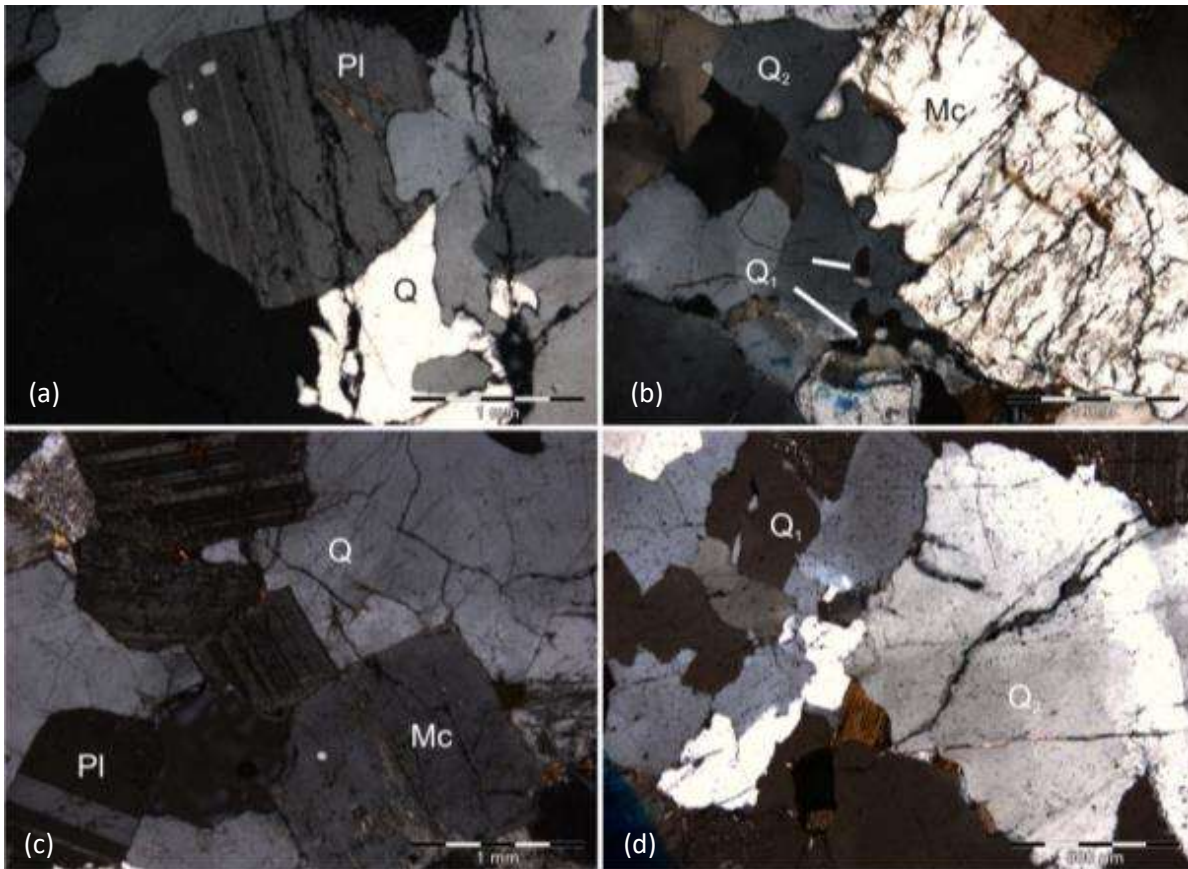
Figure 4.34 Features in oxidised and unaltered portions of E-type leucogranite at Ida Dome. Sample is the unaltered portion of IDAG 05a: (a) Quartz displays weak strain extinction, plagioclase is relatively unaltered and secondary U is minimal (b) Altered portion IDAG 05b: Quartz (Q2) shows stronger strain extinction, embays microcline (Mc) and surrounds older quartz globules (Q1). Embayed K-feldspar has secondary U minerals along cleavage-parallel fractures, xpl. (c) Euhedral plagioclase and microcline occur in interstitial chains and clusters, surrounded by, younger, anhedral, strained quartz, Unaltered sample IDAG 29, xpl. (d) Polycrystalline, euhedral quartz (Q2) cluster has formed adjacent to a larger, earlier fractured quartz crystal (Q2) IDAG 43, xpl.
