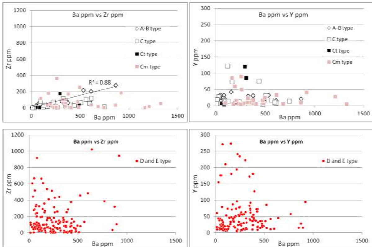
Figure 5.39 Trace element trends of pre-D 3 sheeted leucogranites and uraniferous sheeted leucogranites as indicators of I- or S-type affinity. (a) Ba vs. Zr of pre-D 3 leucogranites, there is an overall low abundance of Y and potentially a weak linear trend in the Cm type, but a strong correlation in the Kuiseb-Formation derived B-type as illustrated by the 0.88 R 2 of the A- B-type group. (b) Ba vs Y is comparable to Zr, however only weak, low abundance relationships are apparent. (c) The uraniferous leucogranites do not show any correlation between Ba and Zr. (d) The relationship with Ba is similar with respect to Y, though with some imagination there is perhaps a positive correlation within some of the high-Ba samples.
