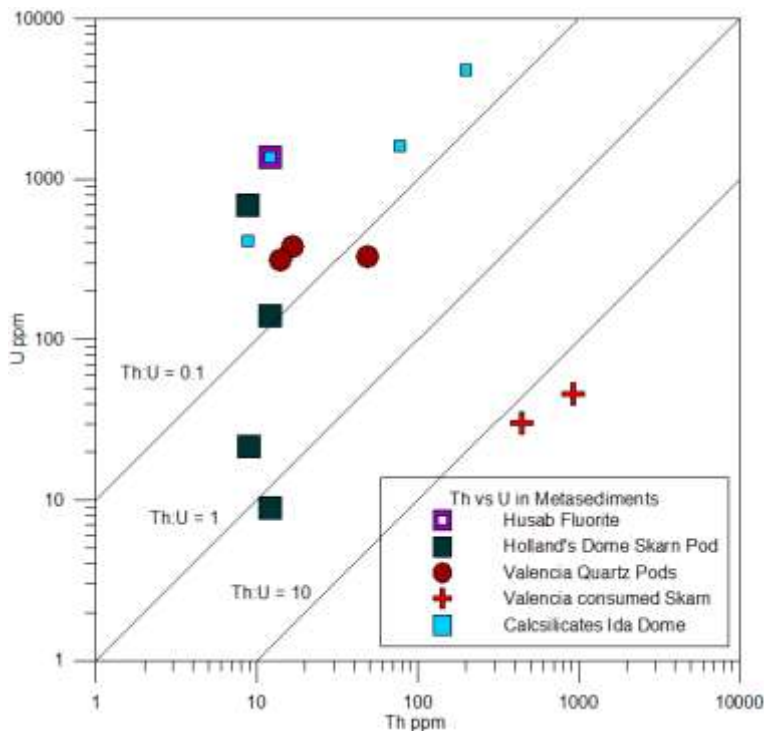
Figure 5.49 Graph of Th vs. U of Central Zone skarn and country rock xenoliths. The consumed skarns of Valencia are the exception and have high 100's- to low 1000 ppm Th, a result of U migration in hydrothermal-like conditions, and the department of Th into monazite.
