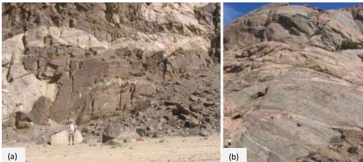
Figure 3.15 Leucogranite sheets of the Goanikontes area. (a) Pre D_3 folded SLG intruding the Chuos Formation north of the Swakop River. (b) E-type SLG's intruding the Khan Formation at the Onkelo section of the Etango deposits, south bank of the Swakop River, looking west.
