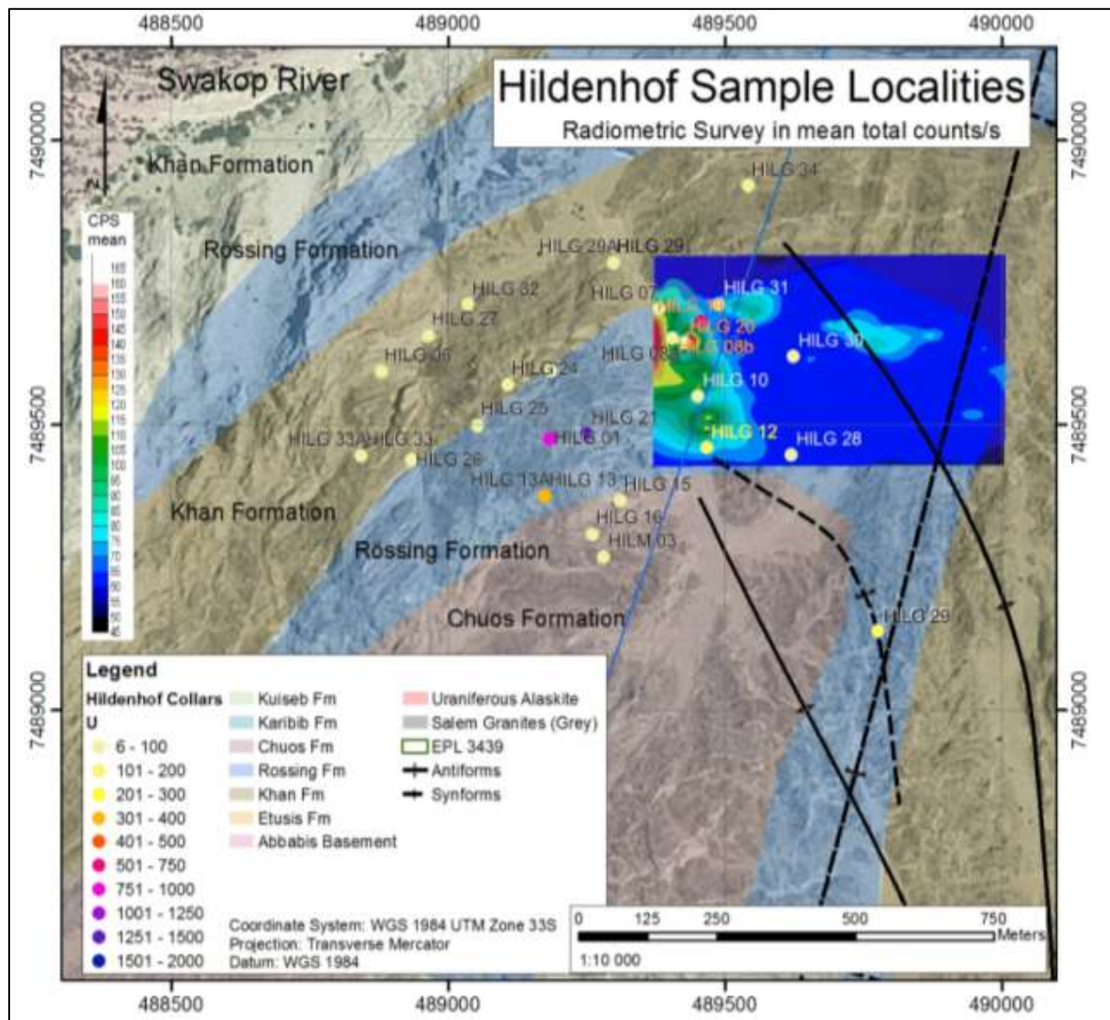
Figure 4.2 Illustrates the Hildenhof sampling locations, all of which occur within the Bannerman Resources EPL. The sampling collection comprises surface samples from the mineralisation trend and the granite assemblages in the surrounding metasediments. The collection includes three varieties of pre-D3 sheeted leucogranites, D- and E-type uraniferous leucogranites and a variety of late pegmatite granites. Three varieties of grey granite and a single red granite example were sampled.
