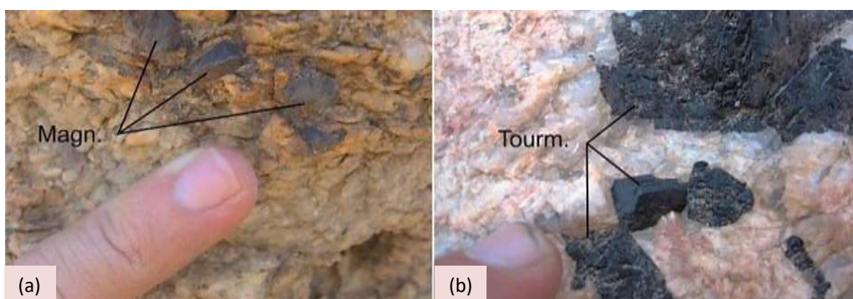
Figure 3.51 Euhedral magnetite and tourmaline in Cm- and Ct-type sheeted leucogranite. (a) Magnetite is euhedral at a number of localities, most notably at Holland's Dome where skarn development is most prominent. (b) Tourmaline-bearing sheets are scarce in the Khan Formation, but occur in the upper Rössing Formation and in the Chuos Formation on the eastern edge of the Ida Dome.
