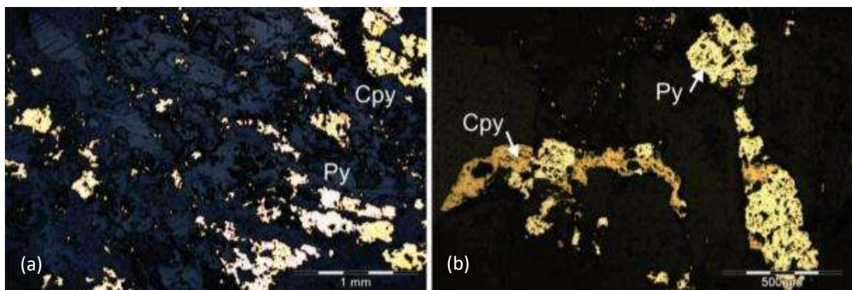
Figure 4.22 Entrained sulphides at Ida Central and Valencia. (a) Subtly-aligned skeletal pyrite-chalcopyrite grains at Ida Central, HDD27 122.90-123.22, rfl. (b) An example of hydrothermal sulphides; in this image, pyrite and chalcopyrite in fractures and at grain boundaries in Valencia leucogranite, VALG 16, rfl.
