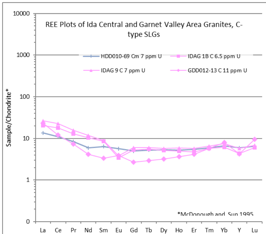
Figure 6.9 REE abundances of the Ida Central and Garnet Valley C-type, and Cm-type sheeted leucogranites. The C-type sheets plot in two distinct populations; one has a distinctive, -ve Eu anomaly, and the other with a slightly +ve anomaly. There is no consistent difference between the magnetite-bearing (C m ) and accessory-free (C) varieties. All of the granites are sampled from within the Khan Formation, and contain uniformly low abundances of REE.
