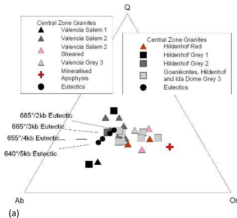
Figure 5.12 Normative orthoclase-quartz-albite ternary plots of Grey and Salem granites of the CZ uranium deposits. Equigranular granites analogous to the type-3 grey granite at Hildenhof are included from the Ida and Goanikontes deposits. The trend with age toward the Q apex is apparent in the sheared and partially melted samples. Eutectics from Rollinson (1993).
