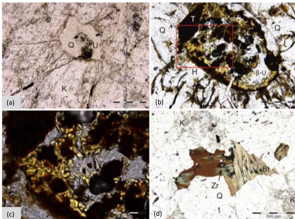
Figure 4.32 Uranium mineral features in the surface sample HILG21 from the Hildenhof anomaly. (a) A complex arrangement of opaque uraninite (U) crystals surrounded by a halo of secondary U minerals that is surrounded by quartz (Q). Radiating fractures in feldspar (K) are a result of metamictisation by radiation damage, HILG 21, ppl. (b) Corroded cluster of magnetite and titanite (T) haematite (H) and yellow uranophane ( \beta -U) filling the voids, HILG 19, ppl. (c) High magnification reveals well-formed crystal terminations of \beta -uranophane amongst amorphous Fe and U hydroxides and silicates, HILG 19, ppl. (d) Skeletal and bladed biotite clusters are abundant in the sample and host uraniferous inclusions, including zircon (Zr).
