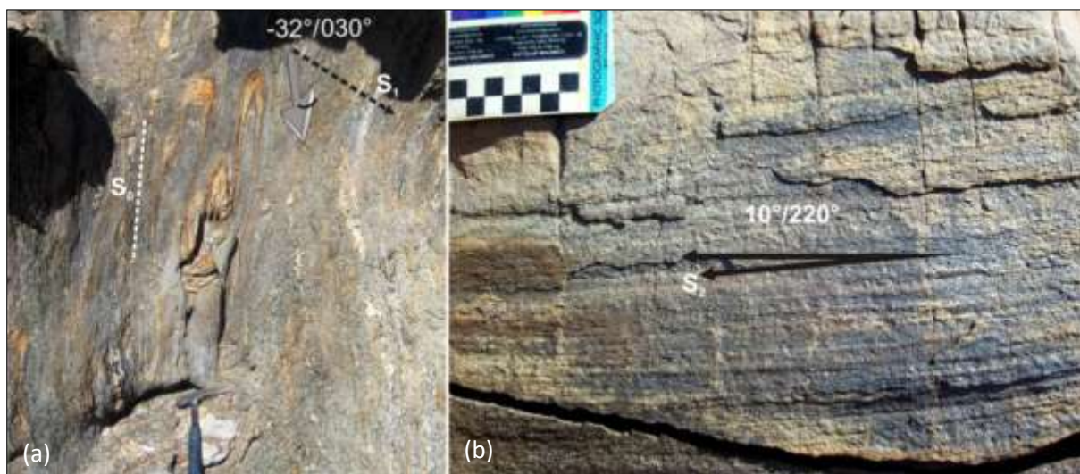
Figure 3.40 Bedding and fold hinge exposures at Valencia. Bedding ( S_0 )- Axial plane ( S_1 )- Intersection lineation ( S_2 ) relationships in the Kuiseb Formation east northeast of the main deposit, Valencia. (a) Limbless folds in the secondary fabric of transposed bedding ( S_1 ) translate into well-developed S_0 - S_1 intersection lineation ( S_2 ) illustrated in (b).
