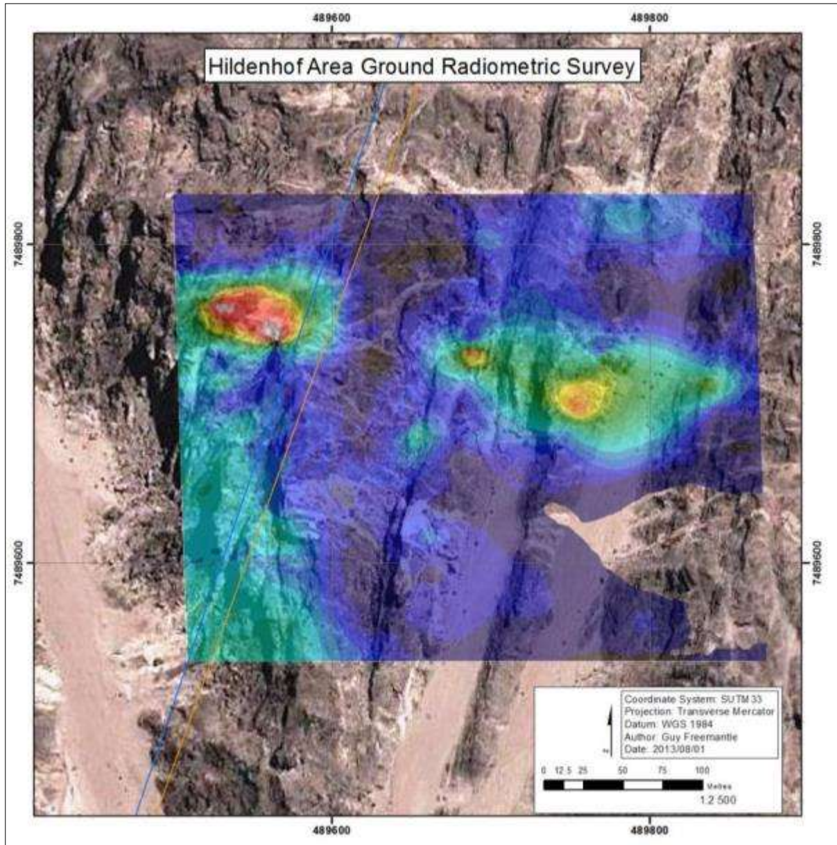
Figure 3.18 The Hildenhof Anomaly ground radiometric survey. The deposit is situated in an antiform adjacent to the southeast of the Goanikontes Dome. The bedding parallel mineralised sheets are confined to an east-west zone 100 m to 200 m wide. (Quickbird™ image from Google Earth™). Count readings taken at relatively constant waist-height of 1 m. Device: THERMO RadEye personal radiation detector.
