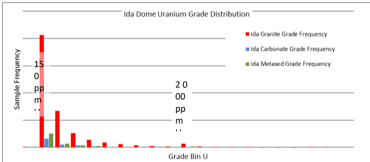
Figure 3.29 Uranium distributions in the three main categories of rock type at the Ida deposits. The Ida Dome deposits constitute a smaller dataset than Husab, but there is an increase in sample frequency at ~2000 ppm U, reflecting the pattern observed in the Husab samples, despite being over 20 km apart from each other. The cut-off at the low end is 150 ppm, but for confidentiality purposes the grade distribution can only be delivered qualitatively.
