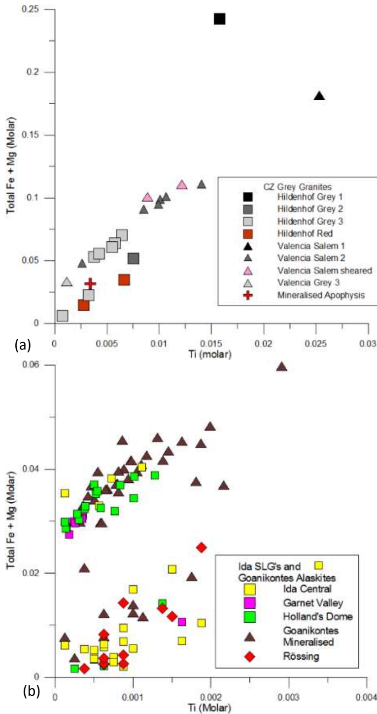
Figure 5.23 Maficity diagrams of Central Zone Grey, Red and Salem granites and sheeted leucogranites. (a) Maficity (Fe and Mg) and Ti contents are highest in the older, melanocratic, generations of Grey and Salem granites. There is a regression in maficity with successive generations of Grey and Salem granites.
