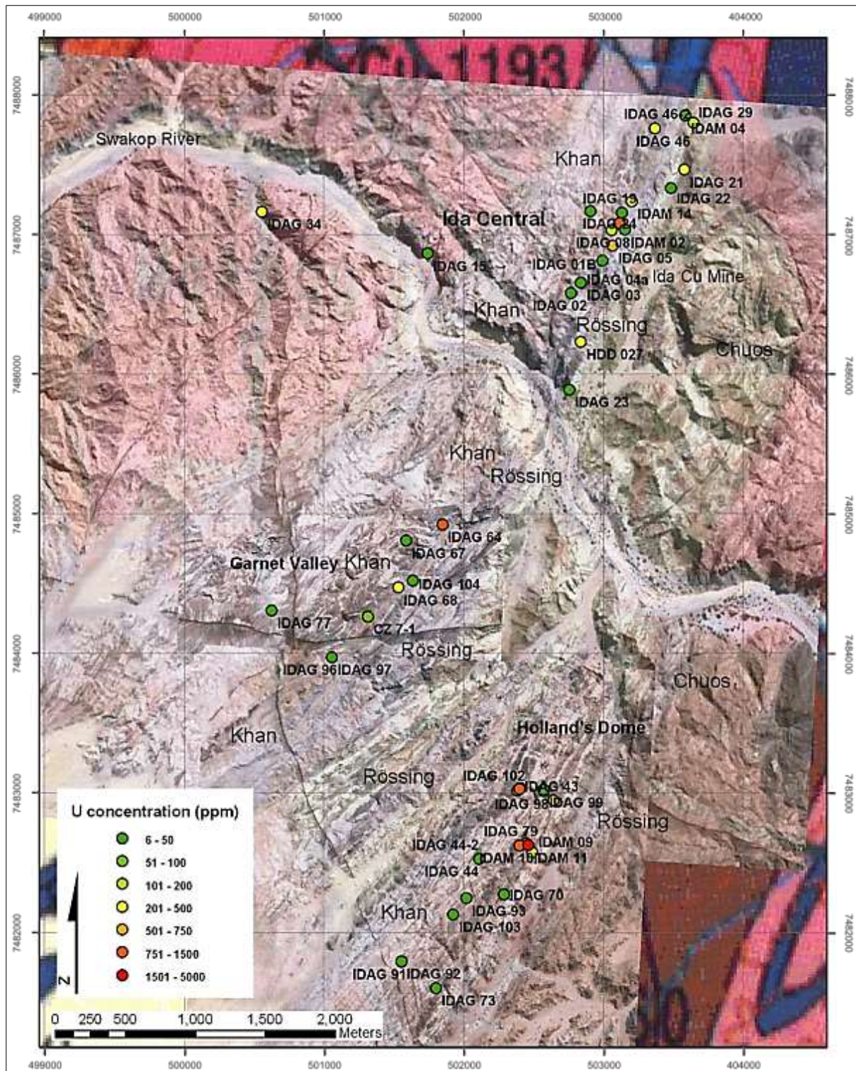
Figure 4.4 Ida Dome sample localities. The eastern portion of the Ida Dome comprises a core of Abbabis granite and augen gneiss, overlain by steeply east-dipping Khan- and Rössing Formation rocks. The bulk of Damaran intrusives occur above the Abbabis-Damara unconformity and comprise sub-horizontally-oriented barren C-type sheets in the Khan Formation, and uraniferous types below- and within the Rössing Formation (pink coloration). The Holland's dome is a north plunging antiform with limbs of upper-Khan and lower-Rössing Formation and cored by diopside Khan Formation gneiss. The Garnet Valley and Holland's Dome deposits occur within EPL3439 (S of Swakop River) and Ida Central is within EPL3138 (N of Swakop River). The colour overlay is from Geological Survey of Namibia, Walvis Bay Map sheet 2214 and the satellite image is taken from Google Earth™ (Quickbird™) and georeferenced in Arc Map v9.1 to WGS1984 UTM Zone 33 S.
