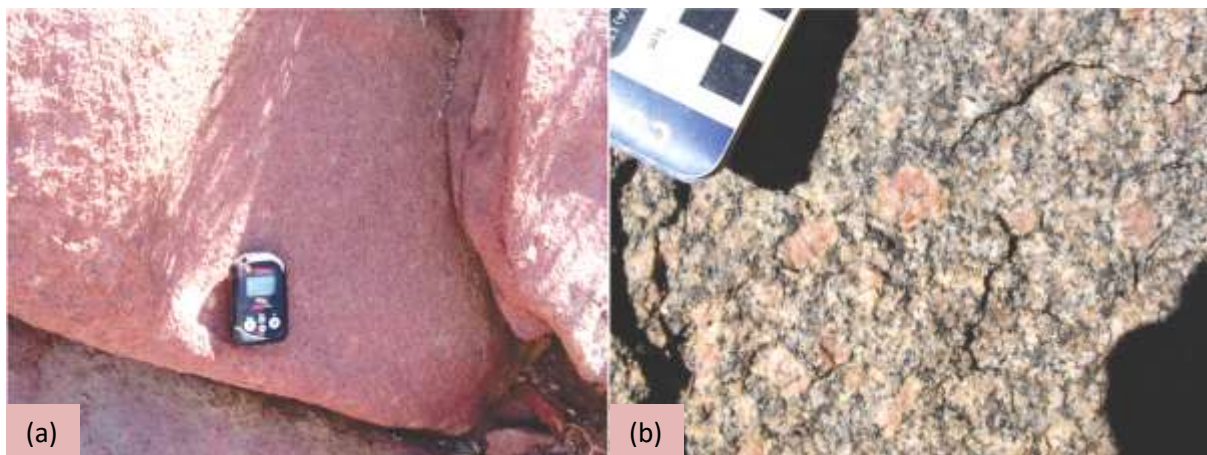
Figure 3.1 Early Damaran granites in the CZ include the Red and Salem Suite monzogranite. (a) The Red granites at Hildenhof are distinctive in colour and homogeneous texture, accessory fibrolite expresses itself as cm scale nests (white spots on surface). (b) The megacrystic Salem granites at Valencia have distinctive 2 – 3 cm K-feldspars in a biotite rich matrix.
