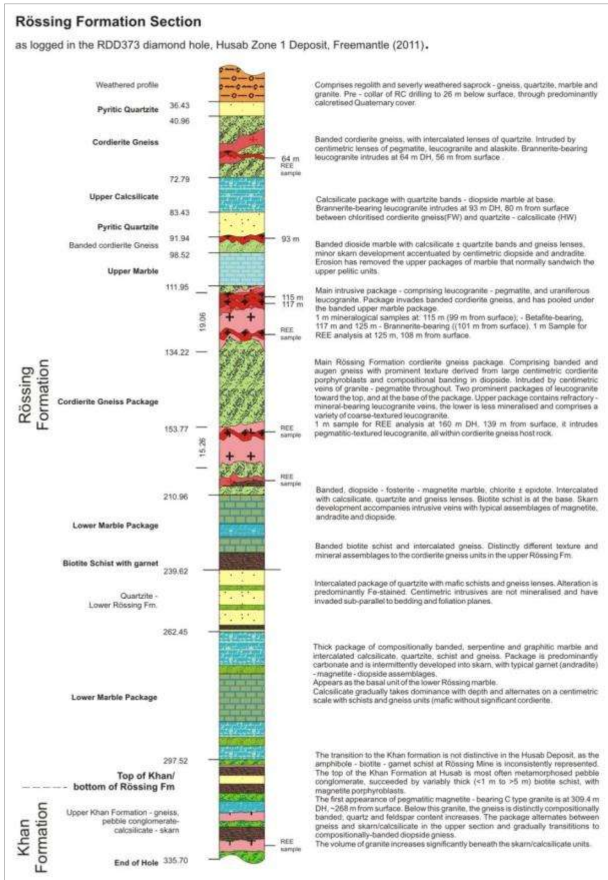
Figure 3.36 Simplified stratigraphic log of a portion of RDD373. Refractory - bearing alaskites are included in the section, with thicknesses approximately to scale. DH = down hole (bore -60°/270°).
