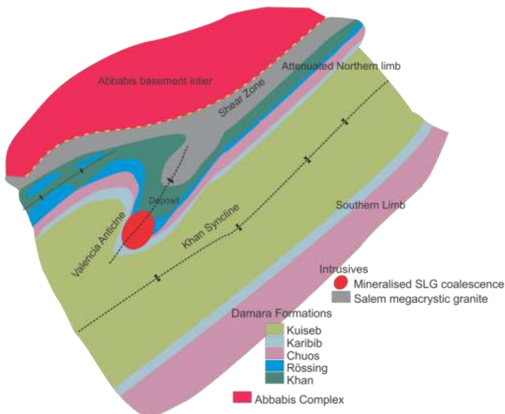
Figure 3.37a Schematic section of the Khan Syncline and its relationship with the Valencia Deposit. The syncline is a regional scale fold with a core of refolded Kuseb schists. The fold hinge trends NE-SW. The synform is refolded south of the Rössing deposit (southeast of the Blauer Heinrich Syncline) where the hinge trend changes to roughly N-S. The eastern limb of the syncline at Valencia is attenuated and a secondary fold has played a role in focussing the mineralised intrusives in a saddle-reef style.
