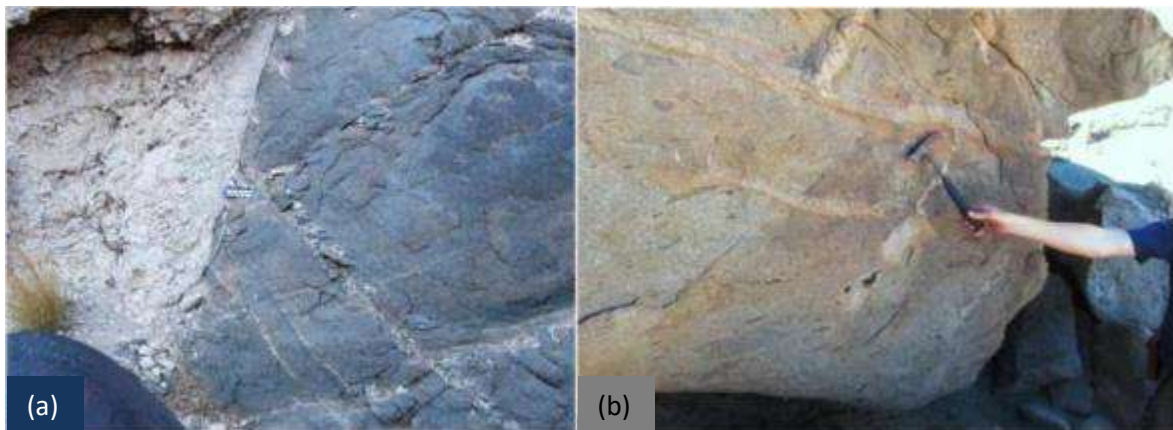
Figure 3.45 Grey granites at Hildenhof. (a) The type-1 Grey granite is melanocratic, foliated, medium to fine-grained and intruded by pre D 3 sheeted leucogranite. (b) The type-2 Grey granite contains less biotite than the type-1 and is characterised by megacrysts of K-feldspar. Thin veins of type-3 Grey granite frequently crosscut the type-1 and type-2 Grey granites. Position: 489345E 7490052N.
