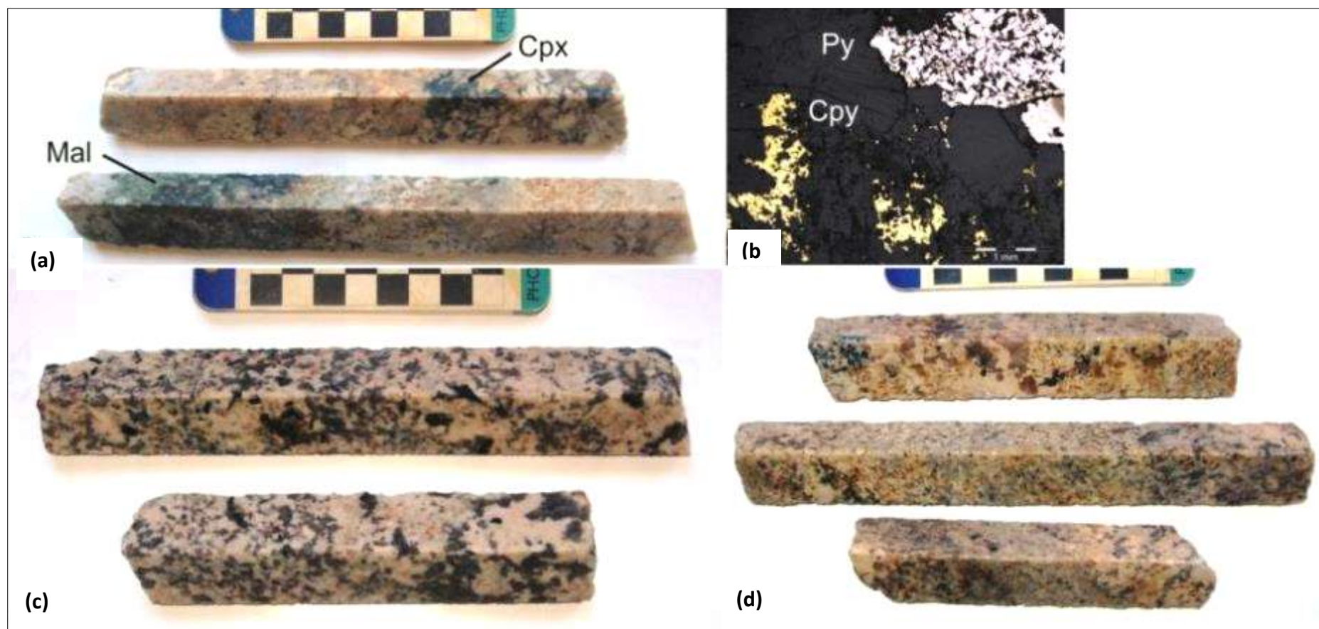
Figure 3.62 Core samples from diamond hole HDD027 at Ida Central. The samples reflect the influences of the host rock on sheeted leucogranite texture and colour. (a) Cu-mineralisation (malachite- Mal) from the Khan Formation stains the granite a green colour around a lath of metasediment. Associated epidote is light green and clinopyroxene is deep green, HDD27 122.90-123.22. (b) Thin sections reveal skeletal interstitial Cu-sulphides, HDD27 122.90-123.22, rfl. (c) The typical D-type texture, with chains of vermicular smoky quartz, has a cream to white-pink colour, HDD27 104.36-104.70. (d) Some samples display inhomogeneous texture, due to the interaction with- and entrainment of fine – grained Khan Formation gneiss, HDD027 89.47-89.95.
