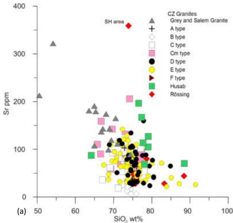
Figure 5.30 Sr content of Central Zone granites relative to SiO 2 . Sr content decreases from the least evolved Grey and Salem granites to <30 ppm in the B type sheets and to <100 ppm in the majority of the mineralised sheet. The SH area is anomalous in Sr, which substitutes for Ca in phases such as betafite
