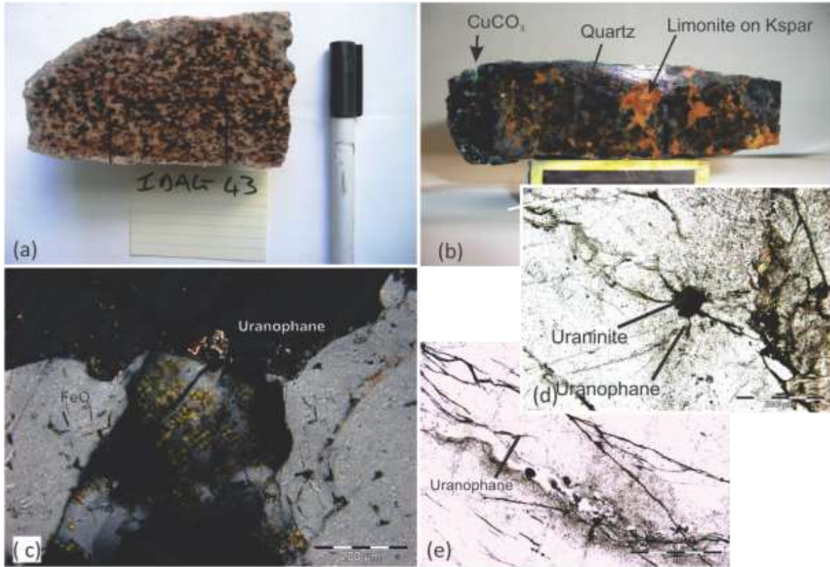
Figure 4.37 Alteration features of mineralised granites at Ida Dome. (a) Red-pink coloration typify E-type sheeted leucogranites, the IDAG 43 example also shows a subtle alignment of quartz and feldspar, a response to deformation suggesting the granite is younger than D_3 . (b) Mineralised SLG that has undergone intensive oxidation during metasomatism. The feldspars have been altered to limonite stained sericite and Cu carbonates have filled spaces made available by feldspar alteration to clays, IDAG 46. (c) Uranophane on quartz, it is associated with the red, amorphous Fe-phases that give the rock its pink coloration, IDAG 43, xpl. (d-e) In thin section the IDAG 46 sample is highly fractured, metamict primary phases are visible and fractures throughout the sample have uranophane precipitation, IDAG 46, xpl and ppl.
