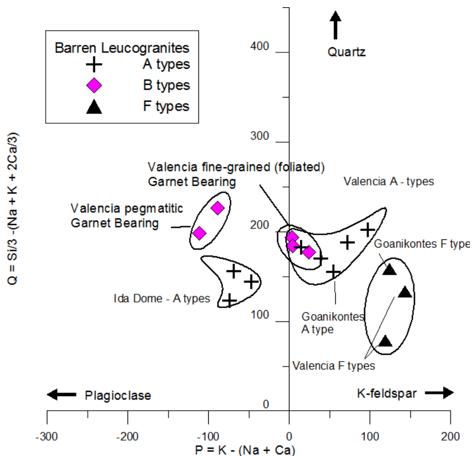
Figure 5.26 P-Q plot of Goanikontes, Ida and Valencia A, B, and F-types. Valencia A and F-types and the foliated B types plot on, or to the right of the K-feldspar line, the pegmatitic B type and the Ida A-types plot toward the plagioclase side of the P axis.
