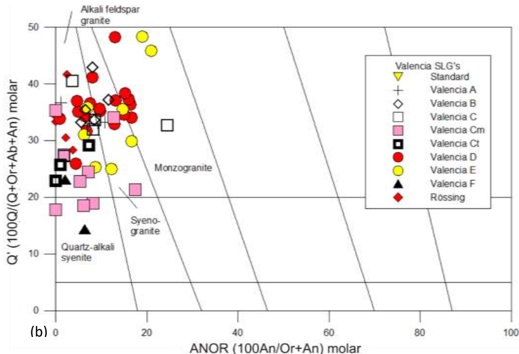
Figure 5.5(b) Q'-ANOR diagram of the sheeted leucogranite suite at the Valencia deposit. Sheeted leucogranite show a wide range of Q' values, which do distinguish between magnetite C types (low Q') and C types (intermediate Q'). Oxidised D-types show a greater variability in Q' than the unaltered D-types. Rössing sample data: Freemantle (2006).
