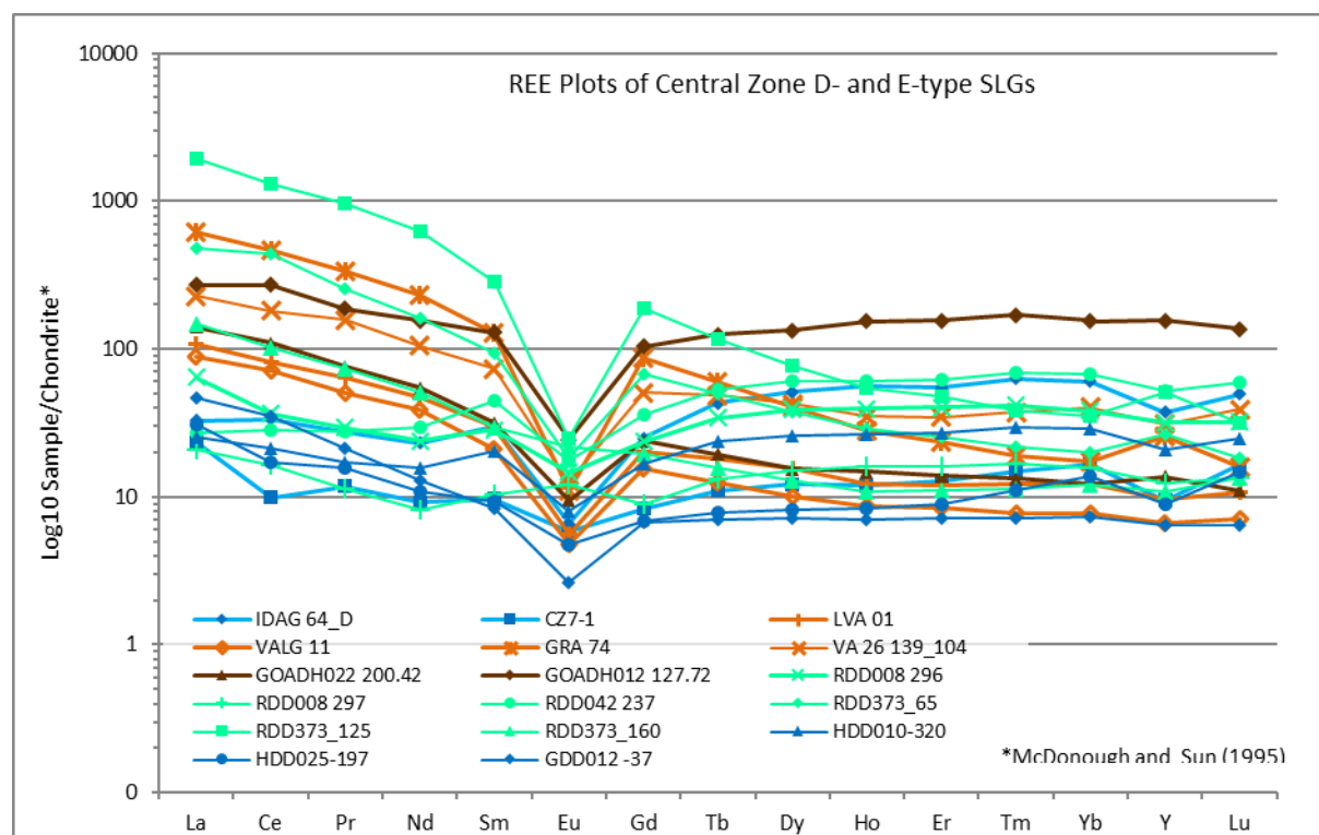
Figure 6.3 REE plots of mineralised leucogranites/ alaskites from Etango, Husab, Ida Dome and Valencia. The mineralised samples consistently plot with -ve Eu, and with highly variable HREE. As with the leucogranites, the mineralised samples appear to show either HREE enrichment relative to Gd abundance, with Lu>Y, or with negative- to flat HREE slopes relative to Gd. A single mineralised alaskite from Goanikontes displays normalised HREE above 100 ppm, for all elements.
