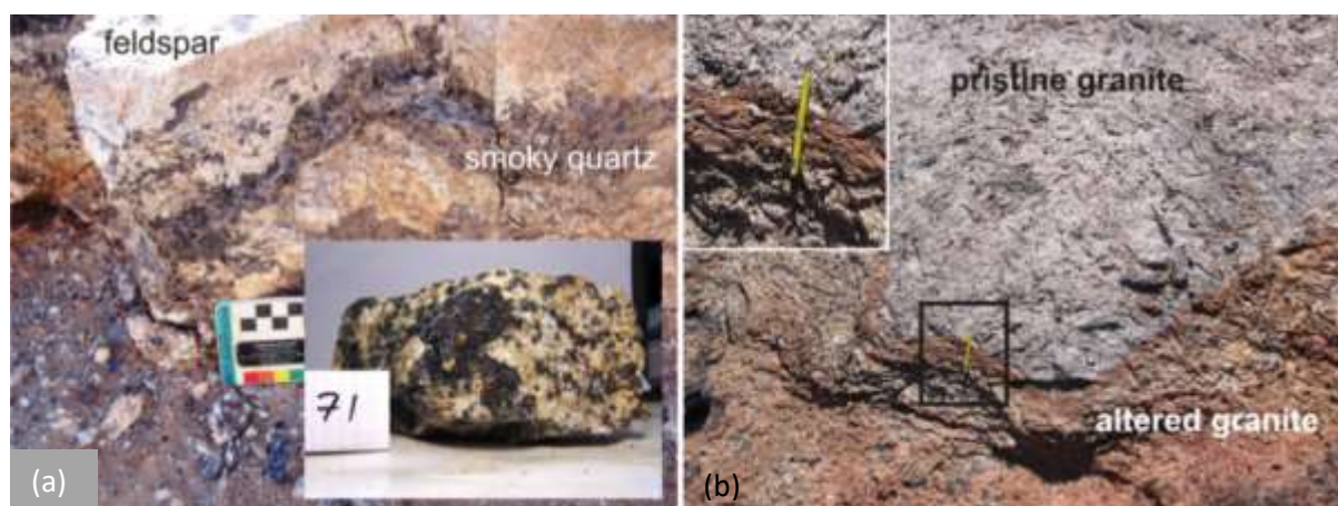
Figure 3.60 D and E-type leucogranites at Ida Dome. (a) D-types are typified at the Holland's Dome area by thick quartz veinlets and an inhomogeneous coarse-grained texture. (b) Garnet Valley and Ida Central pavements are covered with oxidation halos; the cores are unaltered and have a D-type colour and texture.
