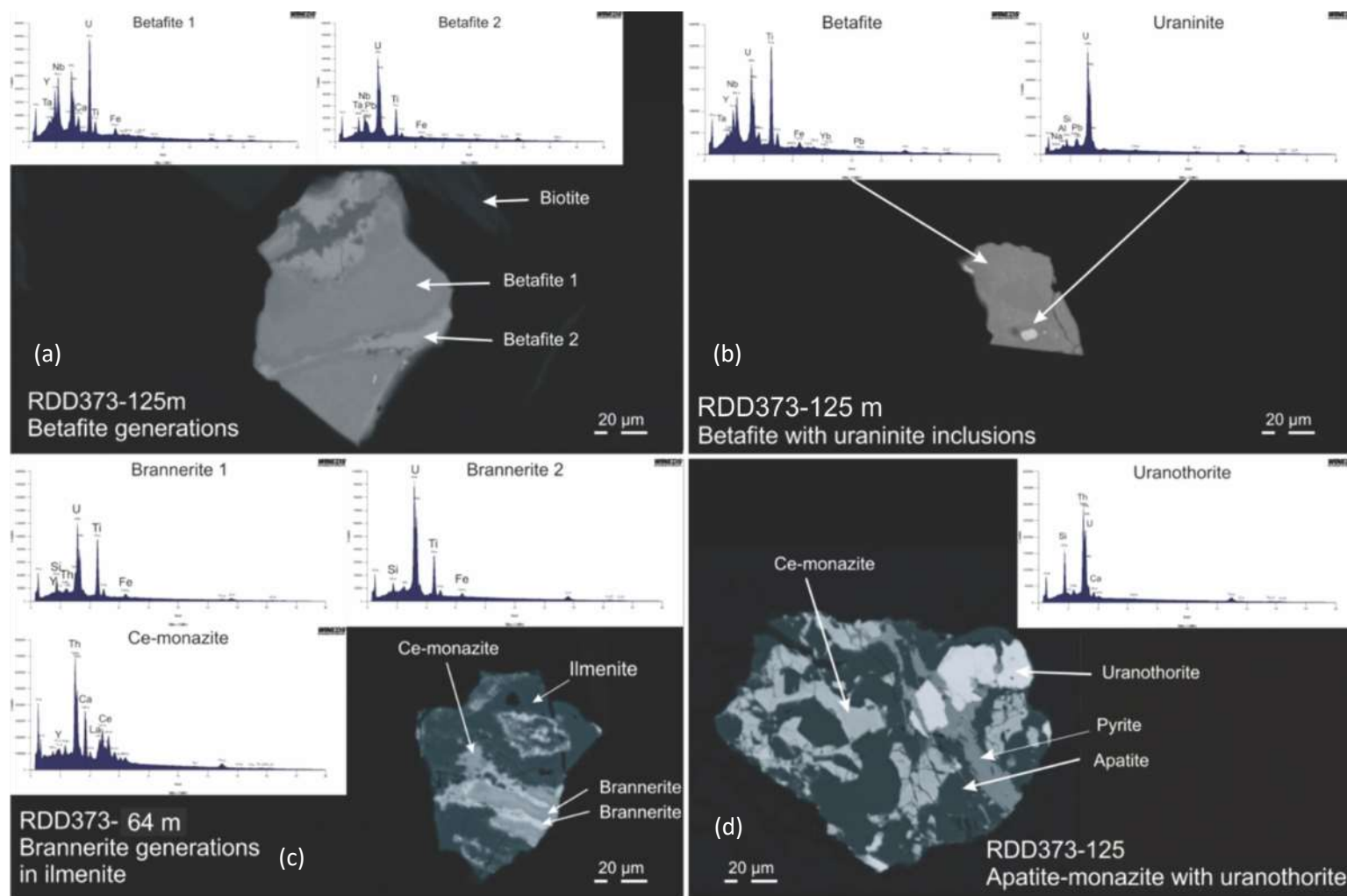
Figure 7.17 Uranium-bearing refractory mineral textures in samples from hole RDD373, Husab. (a) Brannerite alteration in RDD373-125m. Brannerite occurs as a secondary mineral, crystallising in fractures of the primary mineral. The secondary mineral has a higher metal content, as it comprises mobile U (b) Betafite (20 μm) with uraninite inclusion, RDD373-125 m. The sample is a backscatter image of a compound mineral grain identified in a QEMSCAN sampling study of core from RDD373, Zone 1, Husab deposit.
