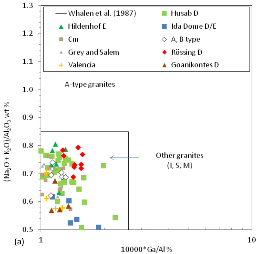
Figure 5.41 Ga/Al and major element discrimination plots of Central Zone leucogranites, Salem, and Grey granites. a) Ga/Al vs. \text{Na}_2\text{O}+\text{K}_2\text{O}/\text{Al}_2\text{O}_3 shows most leucogranites and grey granites fit in the field of 'other granites'. The Ida Dome samples plot with low total alkali, reflecting the effects of anomalously high CaO as seen in other classification and discrimination plots.
