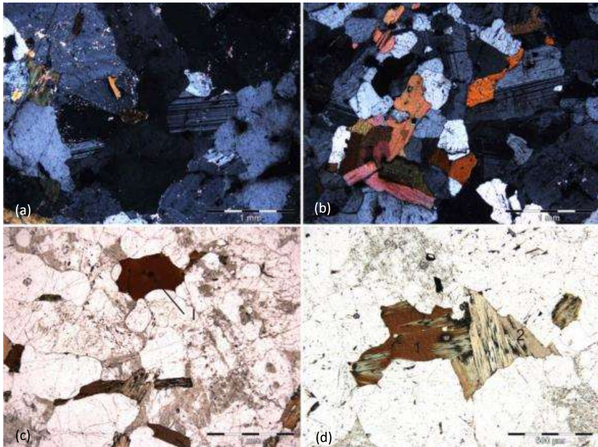
Figure 4.8 Photomicrographs illustrating features of the Grey granite varieties from Hildenhof. (a) Rounded plagioclase between strained quartz grains, note also the high order interference colours of the biotite, HILG 10, xpl. (b) The dominant feldspar is plagioclase, many grains are euhedral with irregular boundaries at later quartz boundaries, HILG 16, xpl. (c) Biotite contains prominent radioactive inclusions (1) HILG 20, ppl. (d) Well - cleaved, partially chloritised biotite contains zircon inclusions (1). Cleavage-parallel view shows alteration along the planes (2) HILG 20, ppl.
