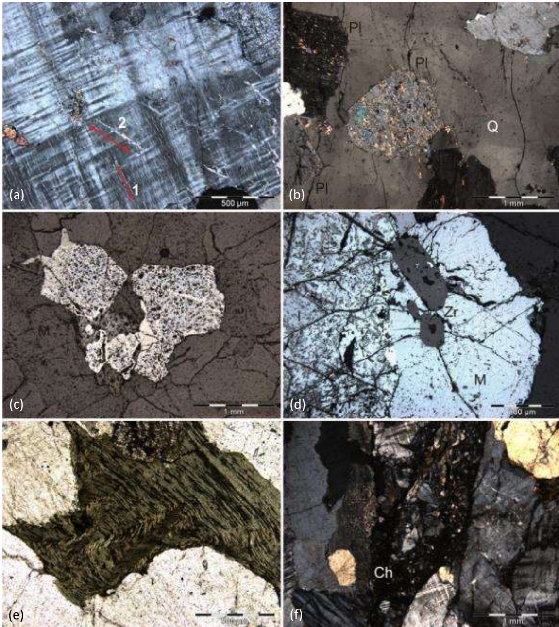
Figure 4.27 Features of altered D and E-type sheeted leucogranites. (a) Perthite in microcline is developed cleavage-parallel first (1) and then as flame perthite (2) oblique to the twinning directions, DH025 235.81-236.14, xpl. (b) Plagioclase (Pl) as anhedral inclusions within later quartz (Q) and in clusters of euhedral grains adjacent to quartz. The inclusion has well-developed sericite compared to the euhedral examples, DH019 71.74-72.18, xpl. (c) Euhedral magnetite is a common accessory in E-type sheets at Goanikontes, alteration by oxidation has resulted in pock-marked textures, DH025 334.91-335.25, rfl. (d) Accessory zircon occurs in clusters, with occasional double termination; zircon is most closely associated with phosphates and magnetite – ilmenite clusters, DH019 71.74-72.18, rfl. (e) The sample is from a fault zone and the deformation evident in the biotite is unique to this particular sheeted leucogranite, DH025 496.03-496.38, ppl. (f) An example of highly altered sheeted leucogranite with a zone of micro-fractures and breccia. Chlorite and epidote are prominent alteration products. DH025 496.03-496.38, xpl.
