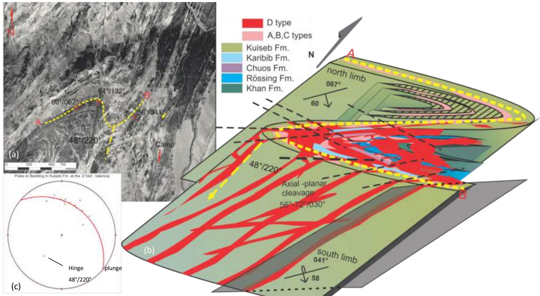
Figure 3.43 Schematic diagram of the large 'Z' folds into which the majority of mineralised granite has intruded. (a) The attenuation of the Rössing- and Karibib Formation marble units and the axial planar-parallel structures in the Chuosi and the Khan Formation pelitic units has allowed the leucogranite sheets to invade up to the Kuiseb Formation. (b) Disharmonic folding has duplicated the Kuiseb and created voids at the antiformal hinge into which granite has coalesced in a saddle reef fashion. (c) Structural data in Appendix C7 quantifies fold hinge line orientation. The ortho-photo is courtesy of Valencia Uranium Namibia Ltd.
