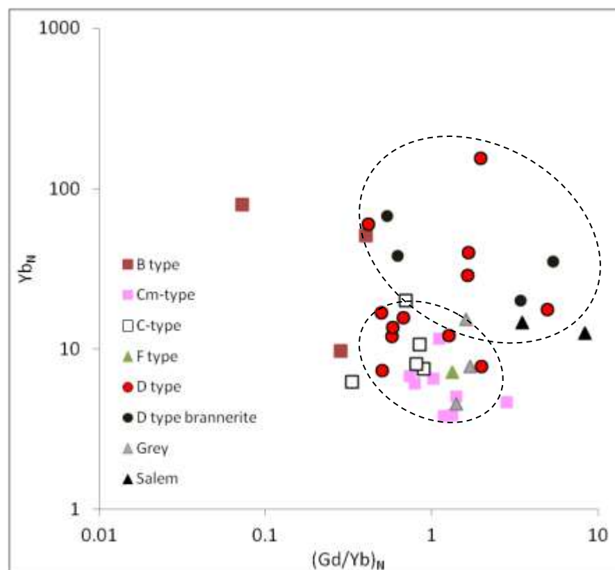
Figure 6.18 HREE fractionation trends of selected CZ granites. Most pre-D 3 granites host <10 ppm Yb N with the syn-tectonic Salem type perhaps the most Yb enriched. The brannerite-bearing alaskites also have high concentrations of HREE, Yb in particular sets these mineralised granite samples apart from the more abundant D-type alaskite.
