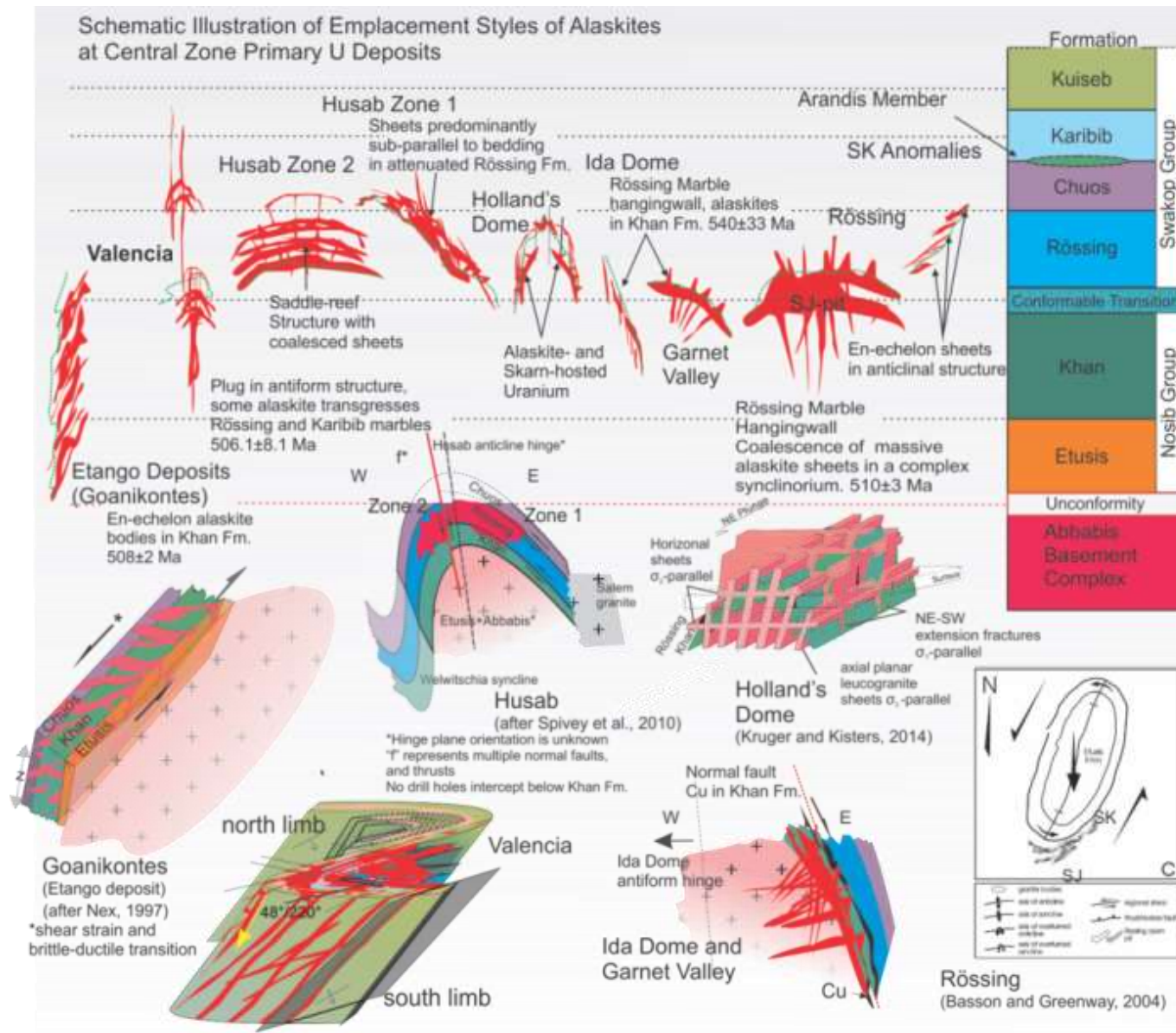
Figure 3.64 Schematic diagram of the Central Zone deposits within the context of the Damara stratigraphic succession. Tectonic processes have prepared certain sites within the Central Zone where relatively ductile sediments occur at an unconformable contact with relatively competent basement rocks. Local-scale rheological contrasts produce pressure shadows within shears, primary- and secondary folds, and associated extensional features, into which regionally significant volumes of leucogranite have invaded, in a more or less passive fashion. Interactions between U-bearing granite contact margins and reactive, predominantly reduced, metasedimentary rocks have played the most crucial role in deposit formation. The interaction zone between the granites and sediments is essentially a REDOX boundary, promoting U^{6+} reduction to insoluble U^{4+} and resultant uraninite precipitation. While the cyclic carbonate sequences at most deposits have provided a physical barrier to retain granite mass within focussed areas, essentially increasing tonnage.
