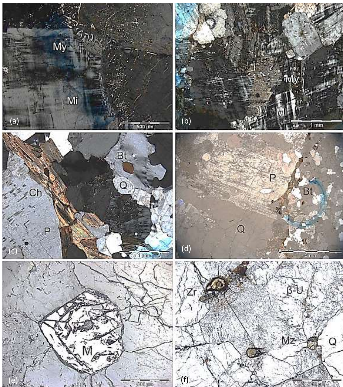
Figure 4.16 Photomicrographs of Cm type leucogranites from the Ida Central Area. (a) Myrmekite (My) is common in all samples and is developed interstitially to larger K-feldspar and quartz, IDAG 08, xpl. (b) Myrmekite has developed within inclusions of early plagioclase in K-feldspar, IDAG 15, xpl. (c) Biotite, included in K-feldspar, contains pleochroic halos. A second texture is partially skeletal and shows chloritisation interference colours. It is sandwiched between a large euhedral plagioclase (P) and equigranular quartz – K-feldspar – plagioclase, HDD027-142.31, 5X, xpl. (d) Euhedral plagioclase and quartz, in a pegmatitic veinlet that intrudes a finer-grained C_m - type sheeted leucogranite. Biotite in the finer portion is fine and disseminated with pleochroic halos, HDD027-142.31, 1.25X, xpl. (e) Magnetite is typically ~1 mm in size and often euhedral and skeletal with exsolved ilmenite and radiating cracks resulting in volume expansion by metamictisation IDAG 08, rfl. (f) Accessory phases include phosphates (monazite-Mz) and silicates (zircon-Zr) which are often clustered and surrounded by radial cracks, IDAG 08, ppl.
