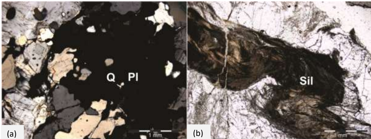
Figure 4.9 Photomicrographs of B-type sheeted leucogranites at Valencia. (a) Examples of quartz textures; globular and amoeboid - shaped quartz inclusions occur in plagioclase. VALG 01, xpl. (b) Laths of entrained sillimanite are characteristic of pegmatitic B-types, VALG 13, ppl.
