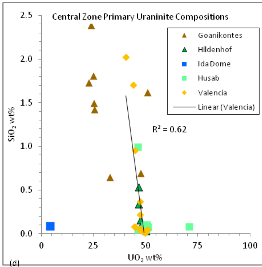
(d) Si occurs in all forty-three uraninite specimens in this study. Key trends are the contrasts in Si abundances between most of the Valencia samples and most of the Husab uraninite (which have low Si) compared to the Goanikontes uraninite.
