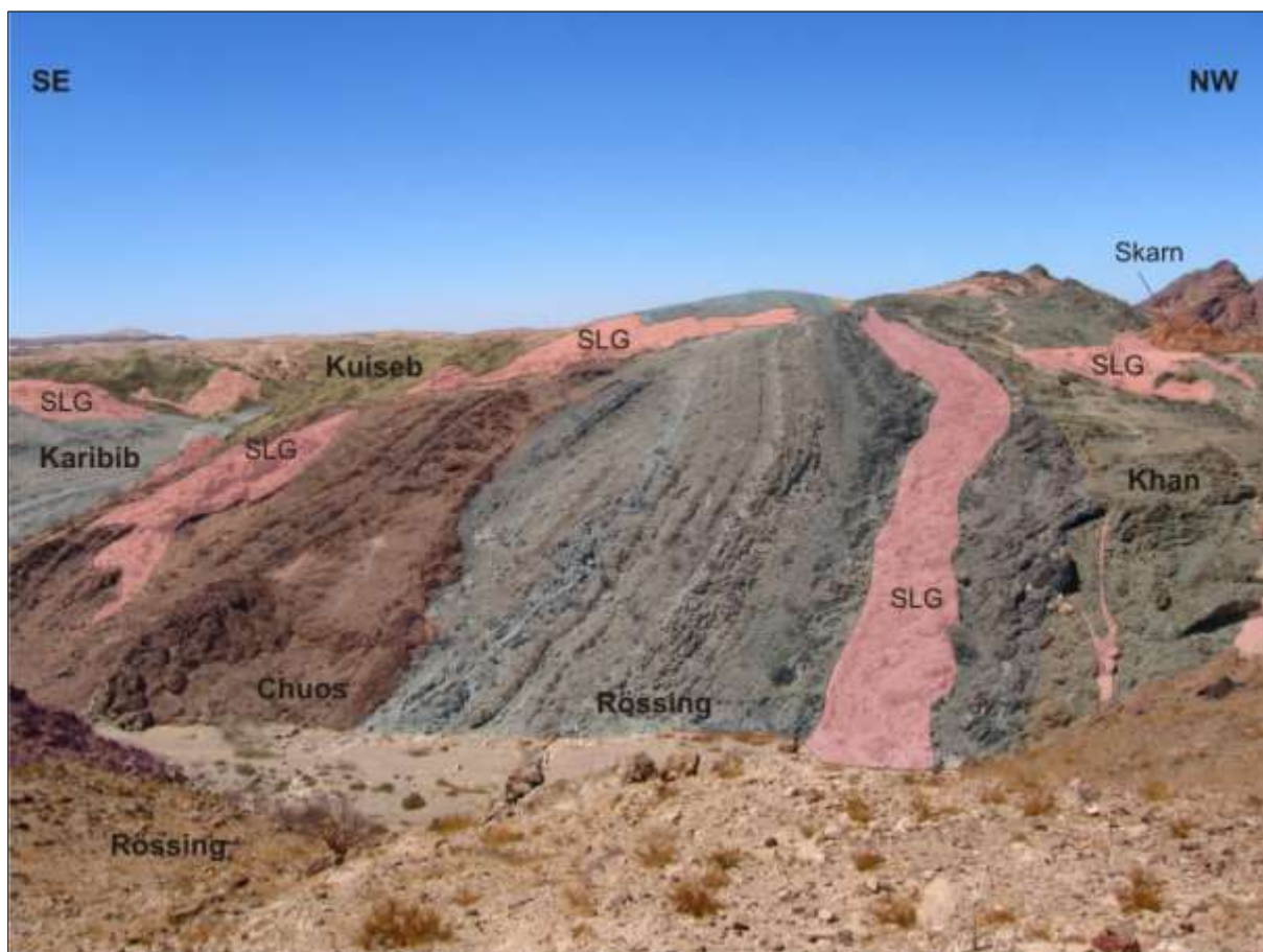
Figure 3.38 The Valencia stratigraphic succession, looking southwest. The northern limb of a regional scale synform contains narrow slivers of Etusis mylonite, and Damara Succession units from diopside gneisses of the Khan through cordierite-garnet schists of the Kuiseb Formation. SLG - sheeted leucogranite.
