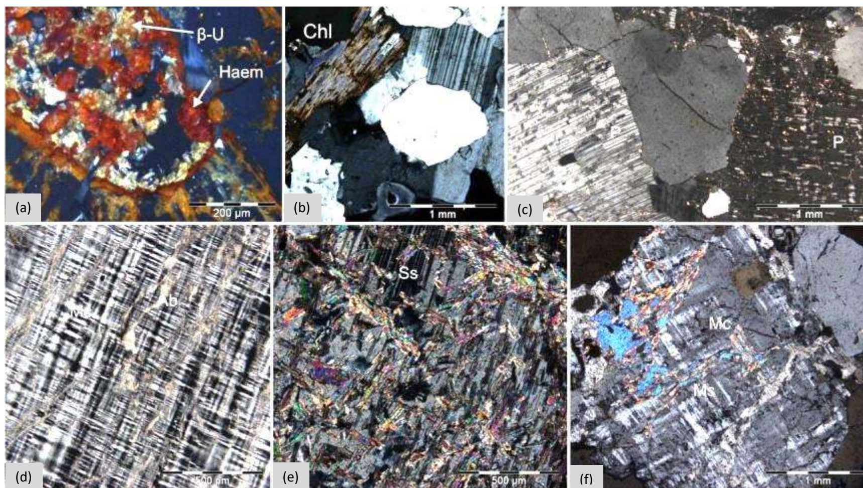
Figure 4.25 Late high temperature and low temperature alteration features. (a) Partially disintegrated, botryoidal, haematite and associated \beta -uranophane. (b) Chlorite lath, after biotite, HDD27 89.47-89.95, xpl. (c) Chess board albite (Pl) and albite overgrowing tartan-microcline, DH012 127.72-128.04, xpl. (d) Mesoperthite (Ab) in tartan microcline, DH19 100.50-100.93, xpl. (e) Saussurite in oligoclase, VA26-141 89.92-90.35, xpl. (f) Coarse mica (muscovite, Ms) on microcline, Va26-111 157.44-157.82, xpl.
