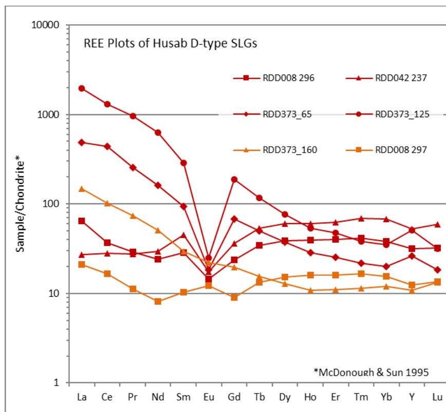
Figure 6.6 REE plots of Rössing Formation-hosted alaskites from the Zone 1 deposit at Husab. The uraniferous samples with refractory uranium minerals from RDD008, RDD042 and RDD373 show distinctly -ve Eu anomalies. (deep red plots). The refractory mineral-bearing samples of RDD373 also have a steep -ve LREE trend, Gd enrichment, -ve HREE slopes and Y > Lu . All four characteristics distinguish the refractory-bearing RDD373 samples from the D-type SLGs (orange plots).
