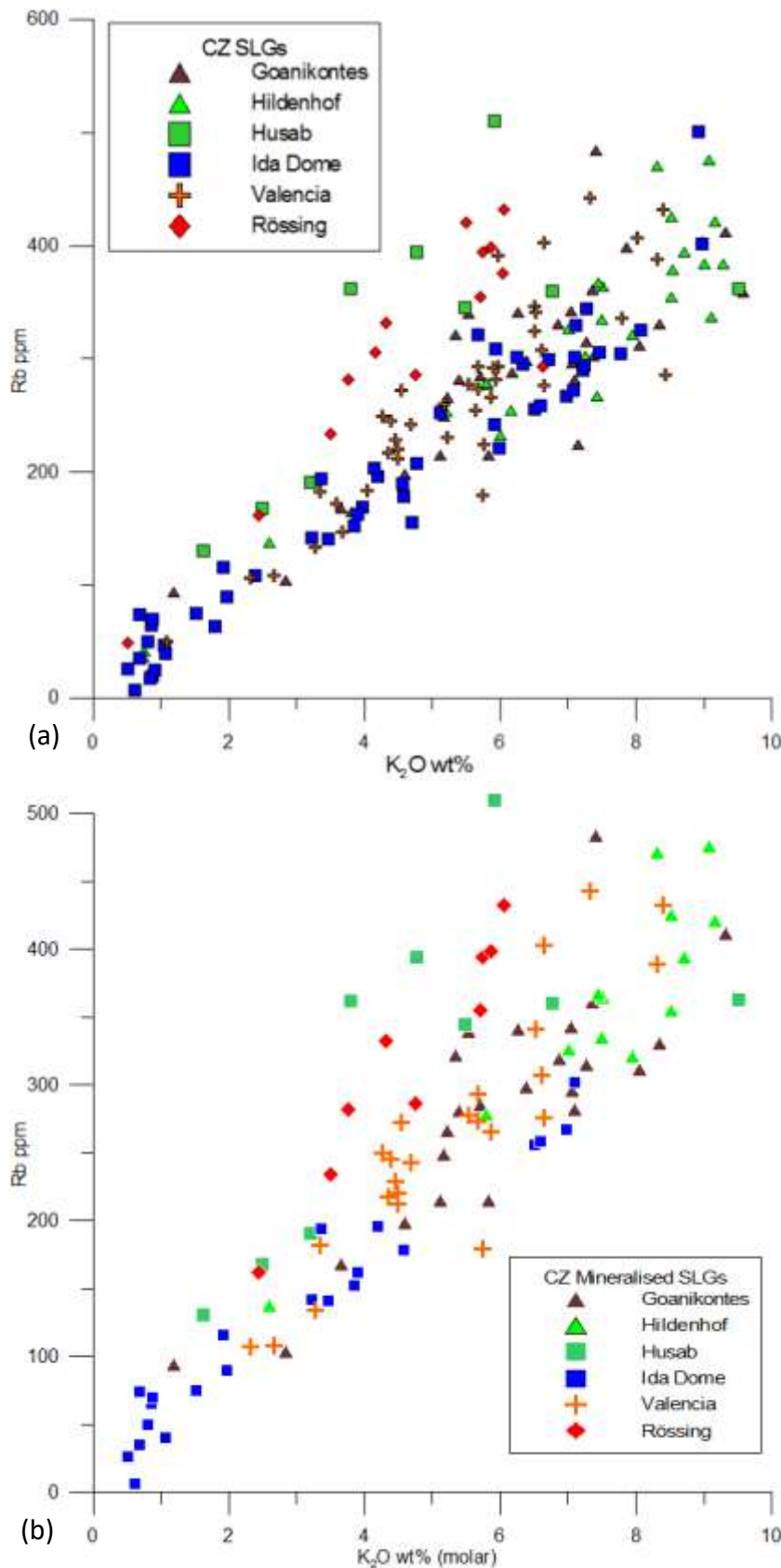
Figure 5.28 K_2O wt.% vs. Rb ppm of Central Zone sheeted leucogranites. (a) Rb shows a positive correlation with K_2O in all samples, but at high K_2O , the Rb content becomes erratic, especially in the Hildenhof samples. Rössing mineralised samples show distinctly elevated Rb for comparison. Rössing sample data: Freemantle (2006). (b) K_2O wt.% vs. Rb ppm of mineralised sheeted leucogranites. The sample suites of individual deposits show some distinction relative to one another; Ida Dome samples have depleted K, and just four samples exceed 200 ppm K. Goanikontes and Valencia samples plot with enriched K and Rb, relative to Ida Dome, with a less systematic trend; the Husab samples plot with erratic Rb:K and high Rb relative to the sample population; and Hildenhof samples have some of the highest K proportion, and correspondingly high Rb. Rössing sample data: Freemantle (2006).
