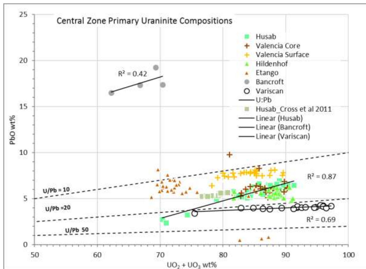
Figure 8.29 Uranium vs PbO wt.% for the Central Zone uraninite. The Husab uraninite population shows the strongest positive correlation between U and Pb, which indicates that sampled uraninite specimens have not lost significant Pb to secondary processes. The Valencia sample population has bimodal distribution, where the surface samples have retained the highest proportion of Pb; and the samples from depth have lost Pb, during hydrothermal alteration episodes (E-type leucogranite). The Hildenhof samples comprise a set of altered uraninite with prominent fractures, thus a poor Pb and U correlation. The Etango uraninite shows evidence of Ca, REE and Y substitution of U, prominent fracturing and coffinitisation, which contribute to a weak Pb and U correlation.
