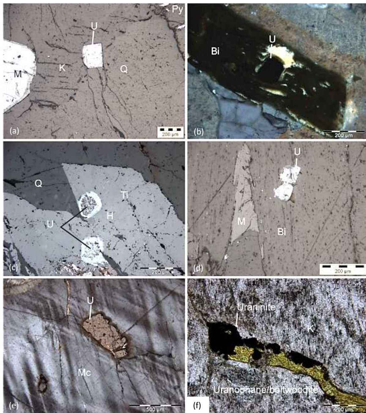
Figure 4.45 Primary uraninite textures and mineral relationships at the Husab deposits. (a) A cubic uraninite crystal, formed between quartz and feldspar. Coffinite replacement is visible at all four edges, RDD373-125 m, rfl. (b) Cubic uraninite grains in biotite, surrounded by a halo of clay replacement in biotite, RDD102 318 m, xpl. (c) Titanite-hosted, corroded uraninite surrounded by haematite halos, RDD219 336 m, rfl. (d) Euhedral uraninite grains associated with magnetite in biotite, RDD373-125 m, rfl. (e) Euhedral uraninite in microcline, note the distorted microcline structure at each end of the elongate grain, RDD078 363
