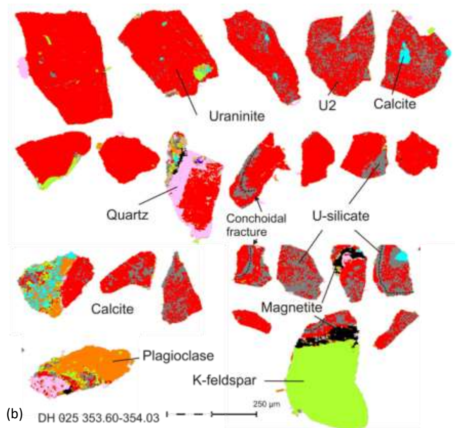
Figure 7.6 Mineral map of DH025 334.91-335.25 and DH025 353.60-354.03 from diamond hole 25 at the Etango deposit, Goanikontes. There are two contrasting styles of uranium mineralisation. (a) The 334.91 m sample contains uraninite as fine-grained inclusions in monazite, and as adhered components of euhedral magnetite. The sample also contains coarse uraninite, with variable coffinite replacement. (b) Uraninite is coarse and shows varying degree of replacement by coffinite. The coarse grains also show conchoidal fracture, along which coffinite is a replacement texture. Conchoidal fracture is typical of magmatic, crystalline uraninite. (Grain U2 is analysed by EPMA).
