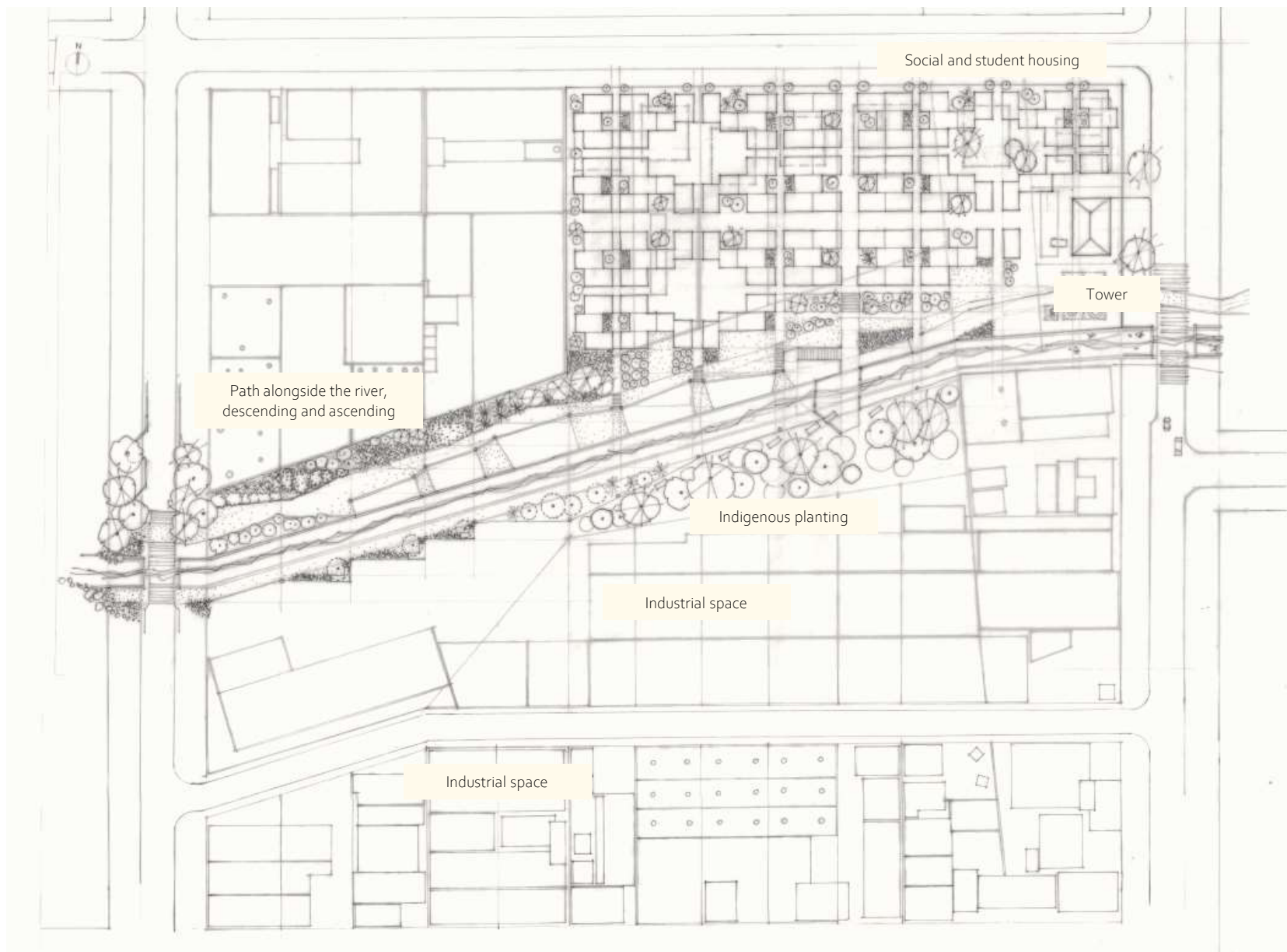
HOUSING HUB LAYOUT
