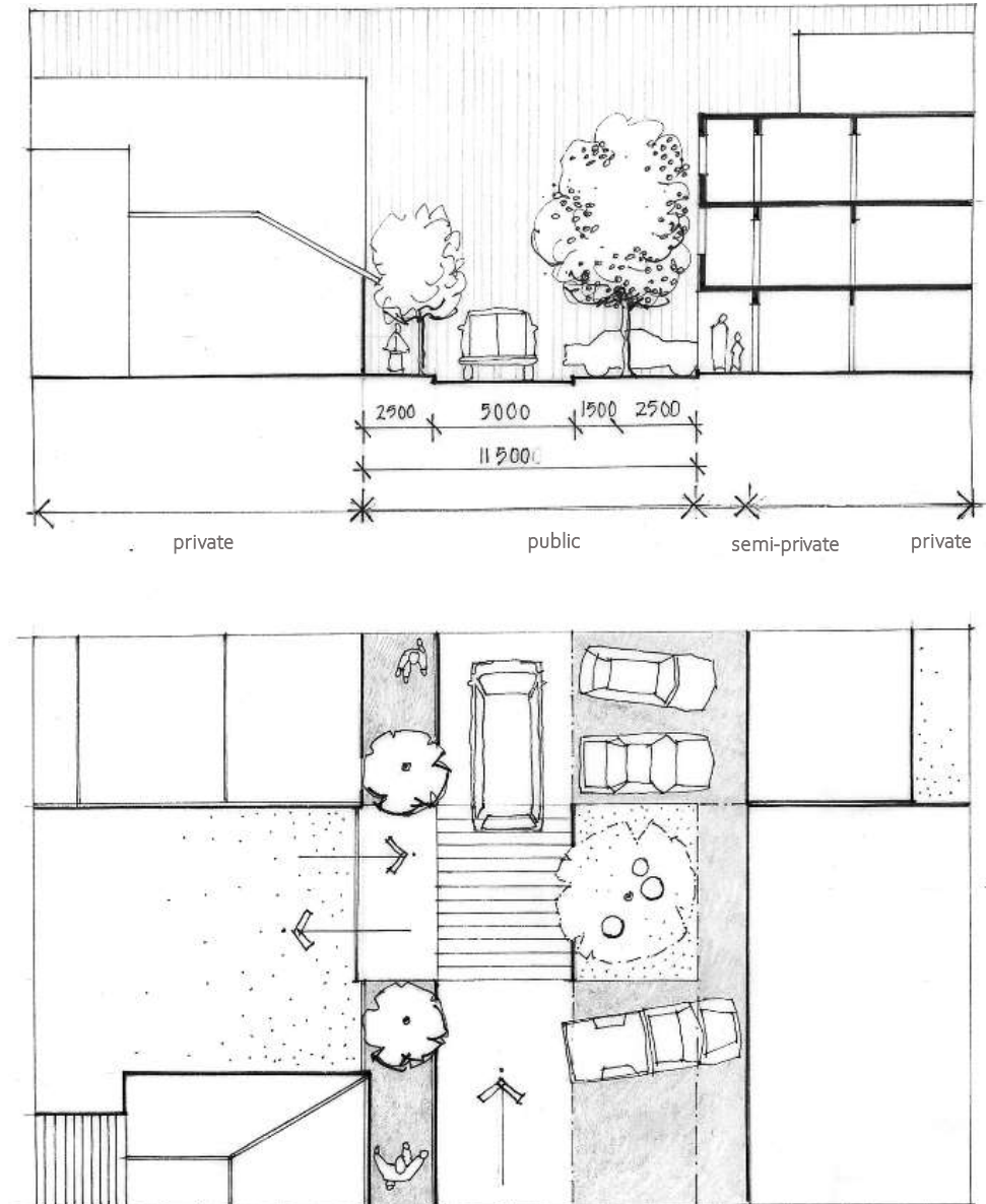
Figure 184: Street plan and section through Frere Road, Lorentville showing a one way street, off street parking and improved public space on wider pavements (Drawings by author).
