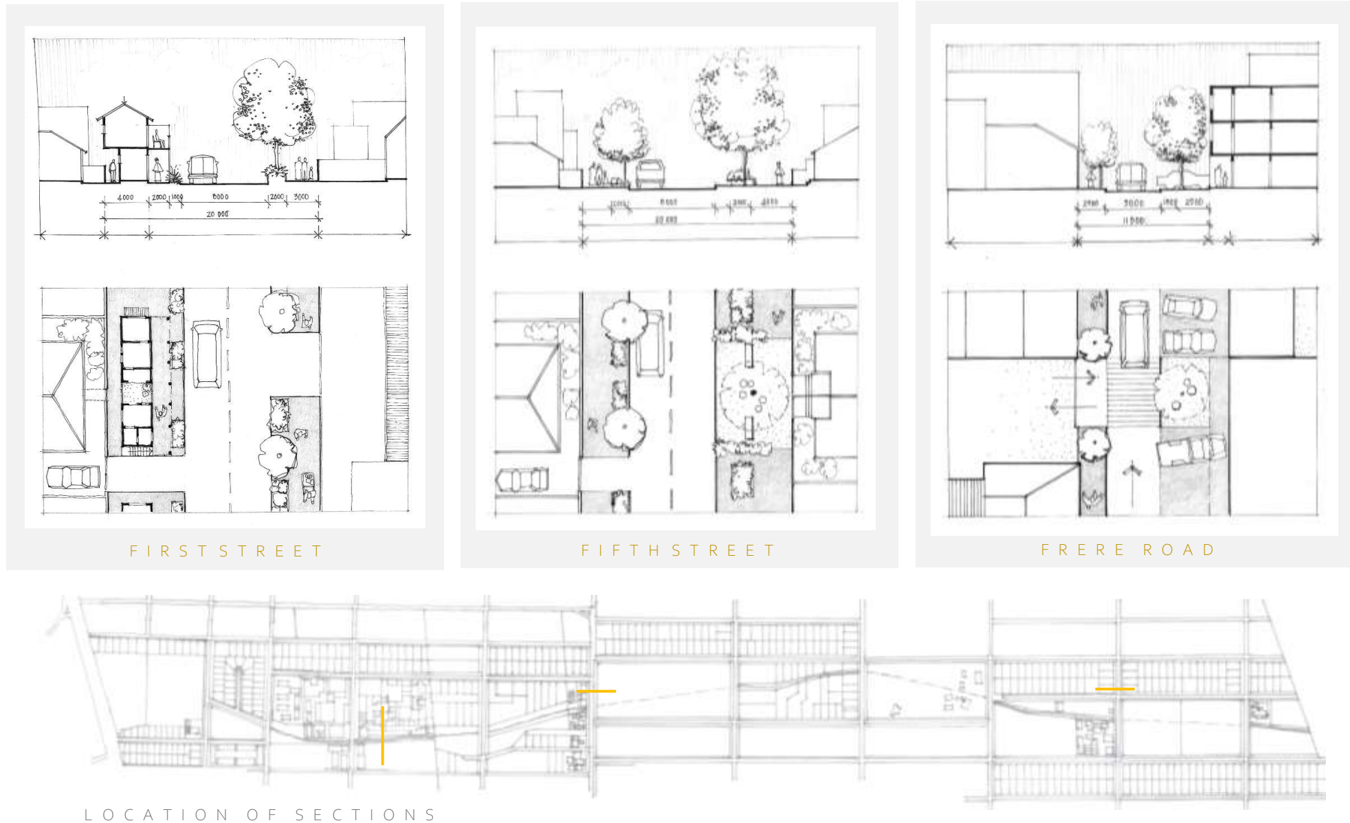
Figure 178: Street plans and sections showing narrower streets and improved public space on wider pavements (Drawings by author)
