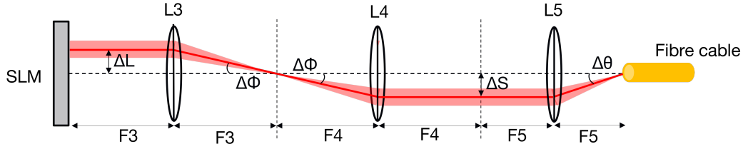
Figure 4.5: Application of angular misalignment on the fibre tip. This is achieved by laterally displacing the beam on the SLM screen by \Delta L . The resulting angular offset at the fibre tip is given by \Delta\theta
