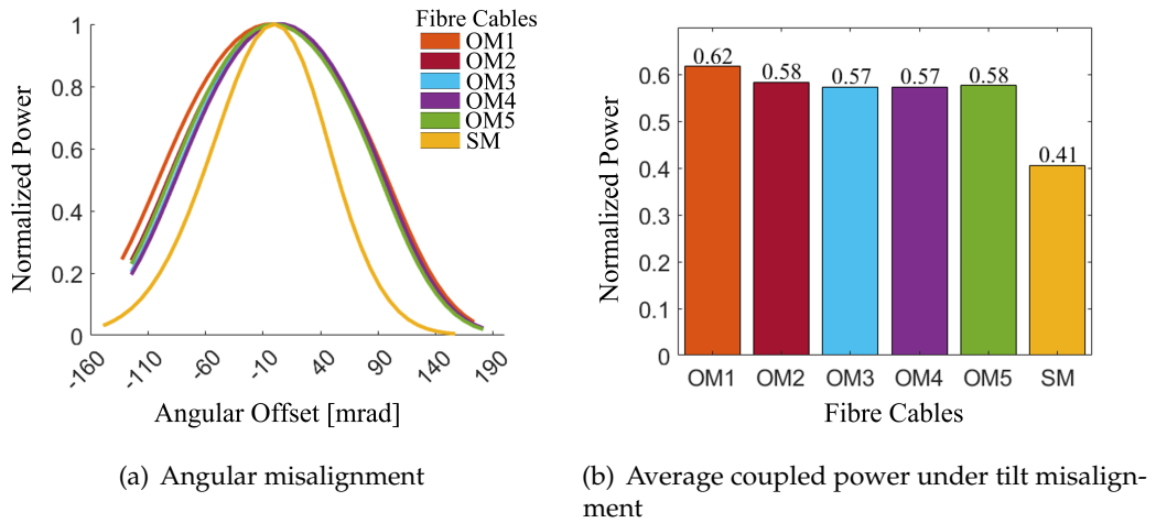
Figure 4.8: The impact of focal point angular misalignment on coupling into standard fibre cables. As the angular offset increases, a decrease in coupled power is observed across all fibre cables. Among them, the OM1 fibre cable exhibits the highest average normalized power, while the single-mode fibre demonstrates the lowest under this misalignment.
