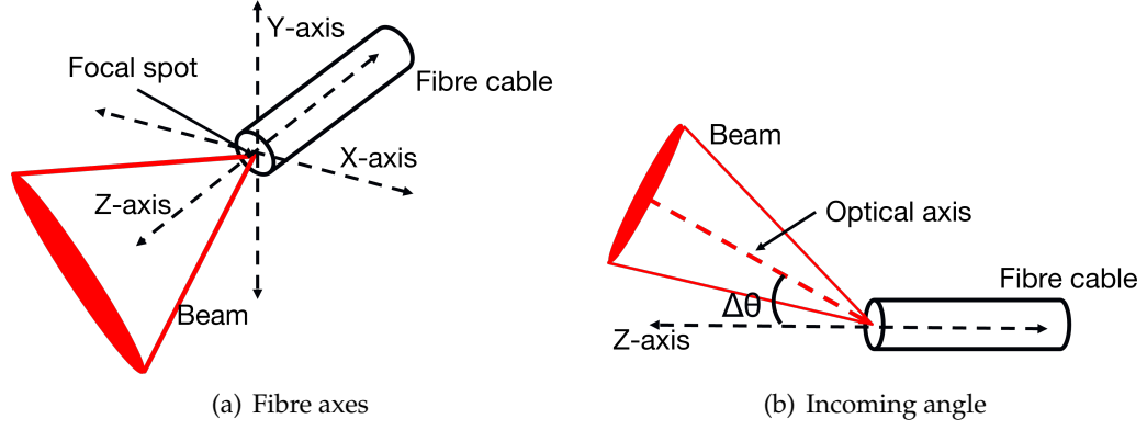
Figure 4.1: Cartesian axes on the tip of a fibre cable (a) and angular misalignment on an incoming beam (b).
