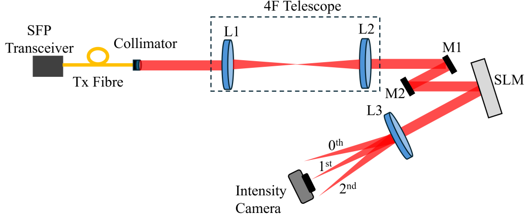
Figure 3.4: Experimental setup to perform modal decomposition of fields launched by fibre cables, represented as Tx Fibre. Lenses L1 and L2 are used as a 4F telescope, which mirrors M1 and M2 are used to align the beam to the SLM. Lens L3 performs a Fourier transform on the beam and separates the diffraction orders ( 0^{\text{th}} , 1^{\text{st}} and 2^{\text{nd}} ). The 1^{\text{st}} diffraction order is observed with an intensity camera.
