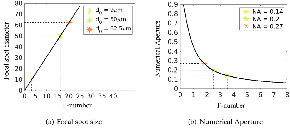
Figure 2.6: Focal spot diameter (a) and lens numerical aperture (b) resulting from different focusing lens f-numbers. Parameters of standard fibre cables are represented using the asterisks. The yellow asterisk represents the single-mode fibre, the green asterisk represents the OM2 to OM5 multi-mode fibres, and the red asterisk represents the OM1 fibre cable.
