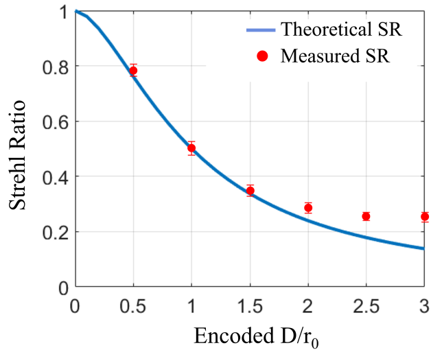
Figure 4.13: Verification plot of the measured Strehl ratio (Strehl Ratio (SR)) against the theoretical Strehl ratio. 200 measurements were made for each value of D/r_0 . The errorbar represent standard error.
