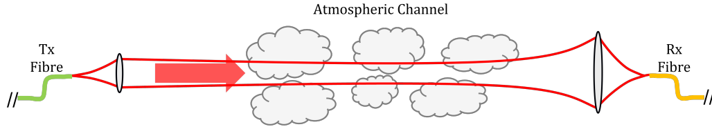
Figure 5.3: Unidirectional transmission of a light beam from a transmit fibre to a receive fibre across a turbulent atmospheric channel.
