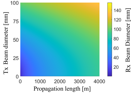
Figure 2.5: Resultant Beam size along propagation caused by different initial beam sizes at the transmitter. The beam diameter at the transmitter is represented on the Y-axis, while the diameter at the receiver is shown using the heatmap.
