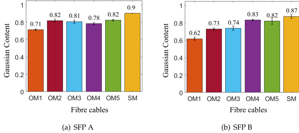
Figure 3.7: Average Gaussian content measured from fields launched out of the fibre cables. The single-mode fibre, represented by SM, records the highest Gaussian content.
