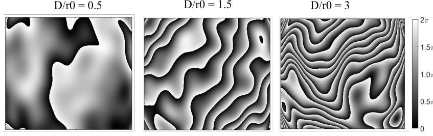
Figure 4.11: Turbulent phase screens generated at different turbulence strengths. The phase spans from 0 to 2\pi .
