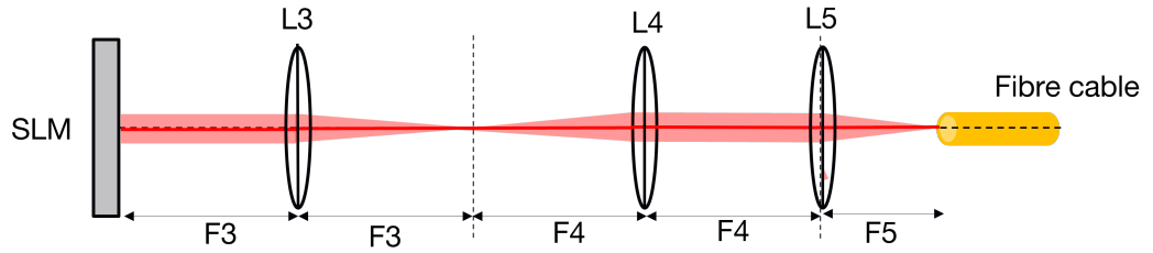
Figure 4.6: Application of longitudinal misalignment on the fibre cable. This is achieved by encoding a Fourier lens onto the SLM, which is then relayed onto the receiving lens L5. The encoded lens and lens L5 emulate a compound lens with a variable focal length.
