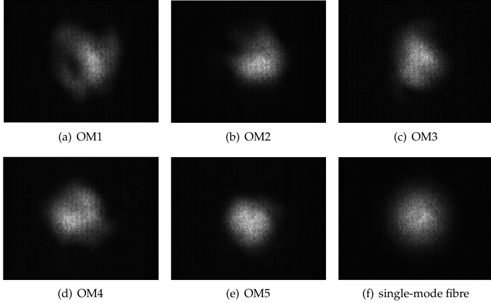
Figure 3.1: Intensity images of beams launched from fibres cables when connected to an Small Form-factor Pluggable (SFP) transceiver module.
