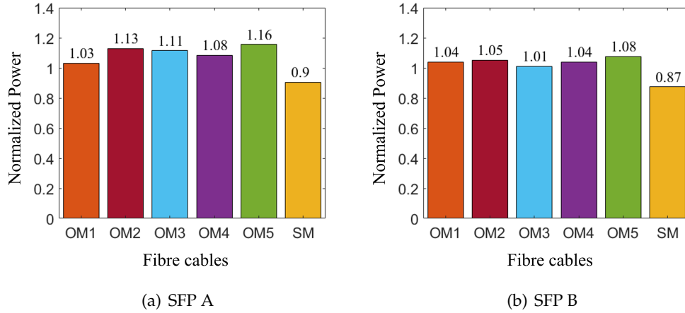
Figure 3.8: Product of average Gaussian content and normalized optical power relative to the power transmitted by the single-mode fibre cable. The OM5 fibre cable records the highest Gaussian power.
