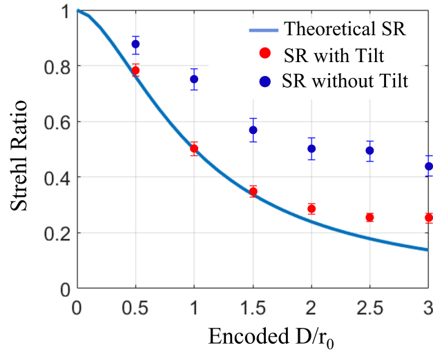
Figure 4.15: Verification plot of the measured Strehl ratio (SR) against theoretical Strehl ratio. The blue dots indicate the measured Strehl ratio in the absence of tilt aberrations. Excluding tilt results in weaker turbulence strength.
