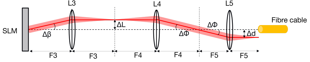
Figure 4.4: Application of lateral displacement on the fibre tip. This is achieved by manipulating the grating frequency encoded on the SLM, resulting in the angular change \Delta\beta . The lateral offset on the fibre tips is represented by \Delta d .
