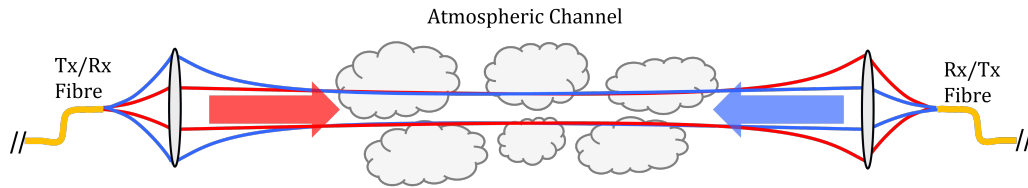
Figure 5.6: Bidirectional transmission of two optical signals with different wavelengths across a turbulent atmospheric channel. Each fibre cable serves as both a transmitter and receiver.
