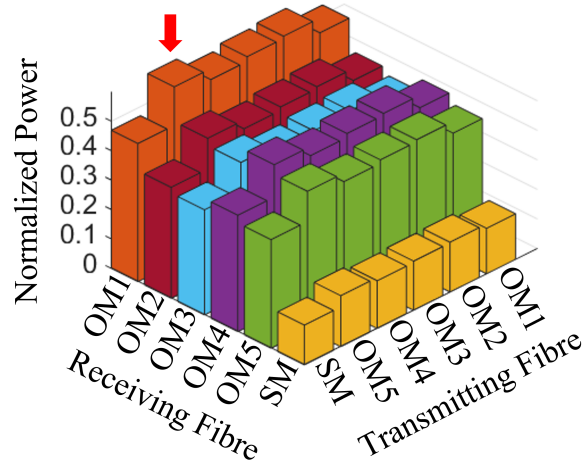
Figure 5.5: Average received Gaussian power in the presence of atmospheric turbulence, relative to the total power transmitted by the single-mode fibre. This is calculated by multiplying the Gaussian power relative to the total power transmitted by the single-mode power, by the average power coupled into the fibre cables under simulated turbulence. The arrow points to the highest received power.
