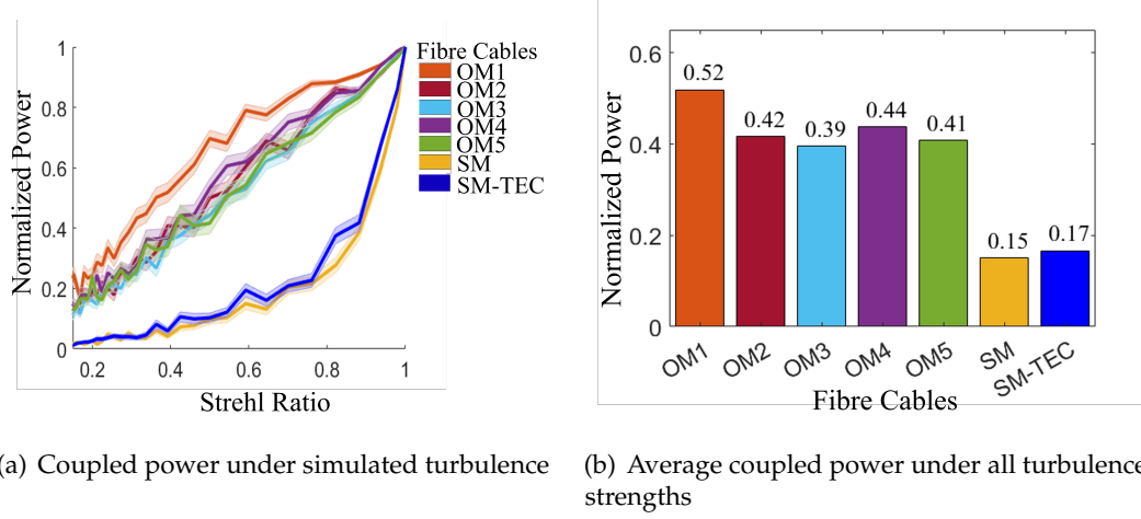
Figure 4.14: Effect of simulated turbulence on fibre coupling. The average power coupled at specific turbulence strengths is calculated across 100 measurements. The shaded region represents the standard error (a). Additionally, an average of the power coupled into each fibre cable across all turbulence strengths is presented (b). The OM1 fibre cable records the highest coupled power in the presence of simulated turbulence.
