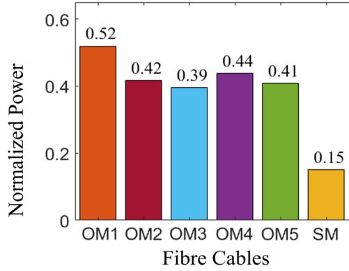
Figure 5.2: Average normalized power coupled into the fibre cables in the presence of simulated turbulence. The average power is calculated across all generated turbulence strengths.
