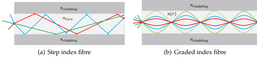
Figure 2.2: Propagation of light rays in step index (a) and graded index (b) fibre cables
