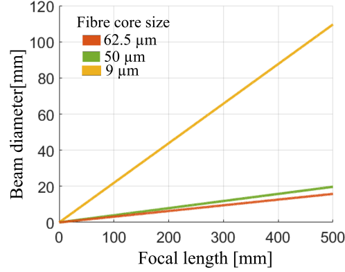
Figure 2.3: Collimated beam diameter at the transmit lens resulting from different focal lengths and fibre core sizes.
