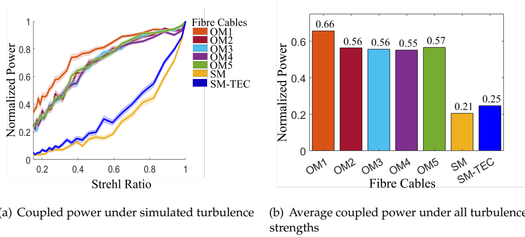
Figure 4.16: The effect of higher-order aberrations on fibre coupling. The phase screens generated excluded the low-order tilt aberrations. Average power coupled at specific turbulence strength is calculated across 100 measurements, with the shaded region representing the standard error (a). An average of the power coupled into each fibre cable across all turbulence strengths is presented (b). The OM1 fibre cable records the highest coupled power in the presence of higher-order modes.
