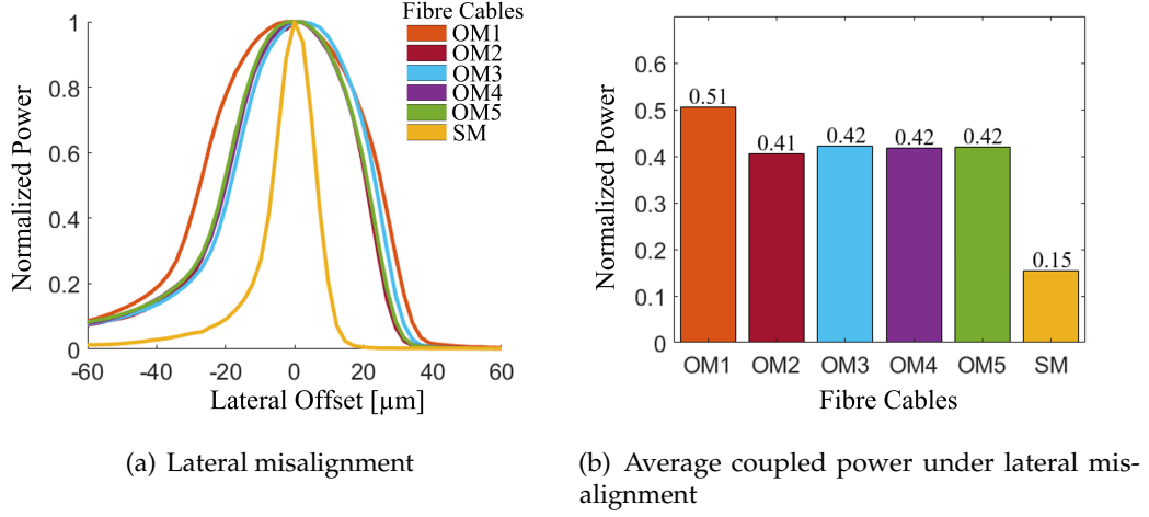
Figure 4.7: The impact of focal point lateral misalignment on coupling into standard fibre cables. The lateral shift ranges from -60 \mu\text{m} to 60 \mu\text{m} . Notably, the OM1 fibre cable demonstrates the highest average normalized power, whereas the single-mode fibre exhibits the least coupling under this misalignment condition.
