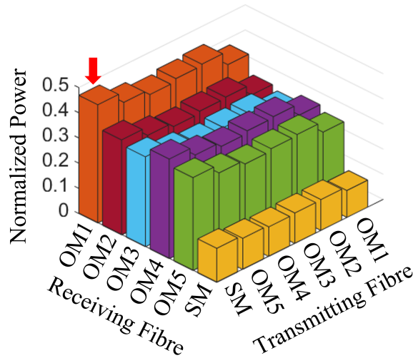
Figure 5.4: Average received Gaussian power in the presence of atmospheric turbulence. This is calculated by multiplying the Gaussian content transmitted by the fibre cables, by the average power coupled into the fibre cables under simulated turbulence. The arrow points to the highest received power.
