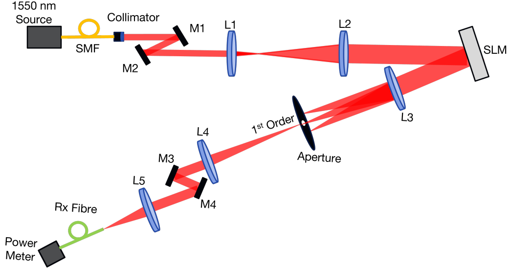
Figure 4.2: Experimental setup to observe the effects of lateral and angular misalignment on the power coupled into the standard fibre cables. SMF represents a single mode fibre while Rx Fibre represents the different fibre cables tested. M1, M2, M3 and M4 represent mirrors used for alignment. Lenses L1 and L2 of focal lengths 50 mm and 300 mm respectively, form a 4f expansion telescope system. Lenses L3 and L4 each have a focal length of 200 mm. Lens L5, with a focal length of 30 mm, focuses the beam onto the fibre cables.
