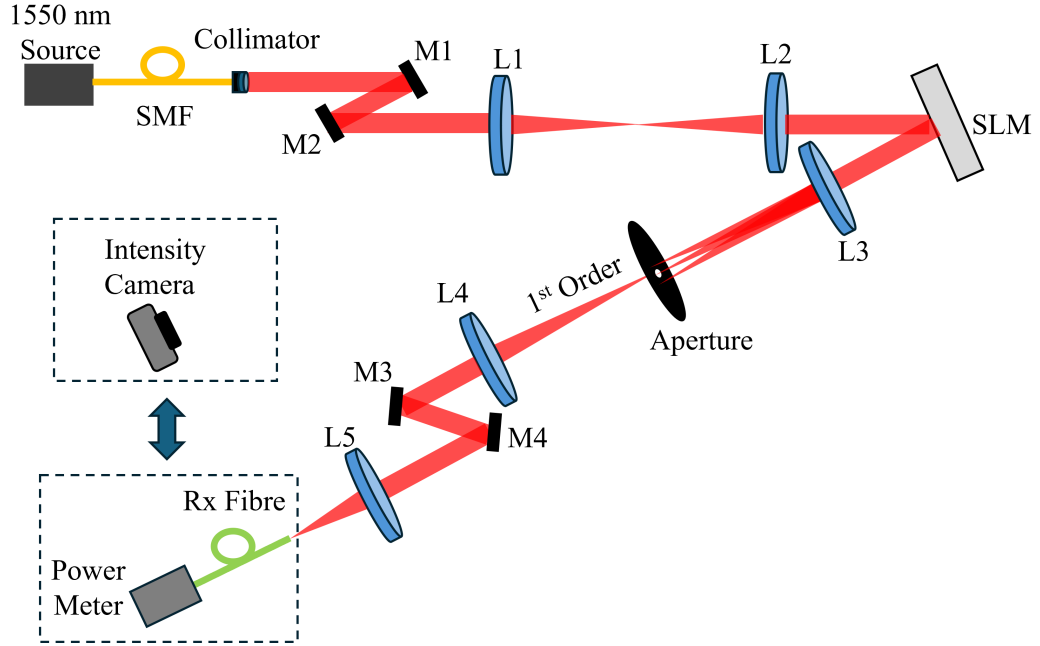
Figure 4.12: Experimental setup to observe the effects of simulated turbulence on the power coupled into the standard fibre cables. SMF represents a single mode fibre while Rx Fibre represents the different fibre cables tested. M1, M2, M3 and M4 represent mirrors used for alignment. Lenses L1 and L2, each with a focal length of 150 mm, relay the beam from the collimator to the SLM. Lenses L3 and L4 each have a focal length of 200 mm. Lens L5, with a focal length of 30 mm, focuses the beam onto the fibre cables. The intensity camera replaces the receiving fibre (Rx Fibre) and the power meter during the calibration of turbulence strength.
