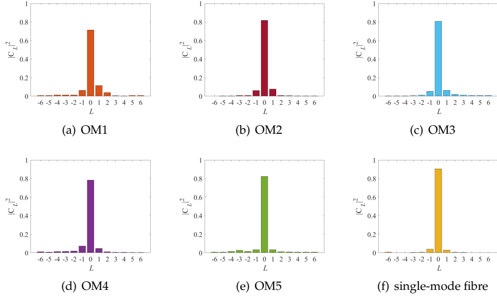
Figure 3.5: Average modal content of beams from SFP A. The modal content was averaged across 5 measurements. All fibre cables exhibited high Gaussian content.
