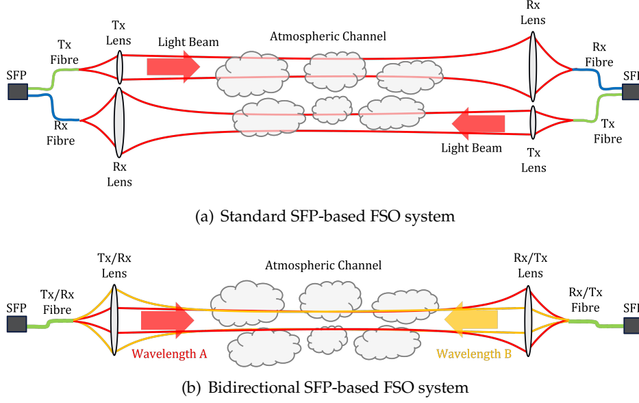
Figure 1.1: FSO communication established using SFP transceivers and fibre cables. This can be done using standard (a) or Bidirectional (b) SFP transceiver modules. The fibre cables are used to transmit and receive the optical signals.
