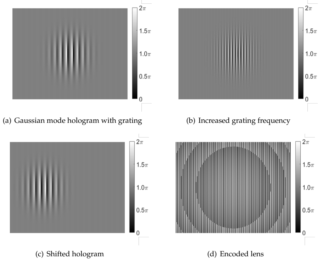
Figure 4.3: A Gaussian mode hologram and diffraction grating encoded on the SLM screen (a). The grating frequency is increased to change the angle of the first order beam in order to impose focal point lateral displacement (b). The hologram is shifted to laterally shift the first order beam and impose tilt misalignment (c). A Fourier lens is encoded onto the SLM to impose longitudinal misalignment (d).
