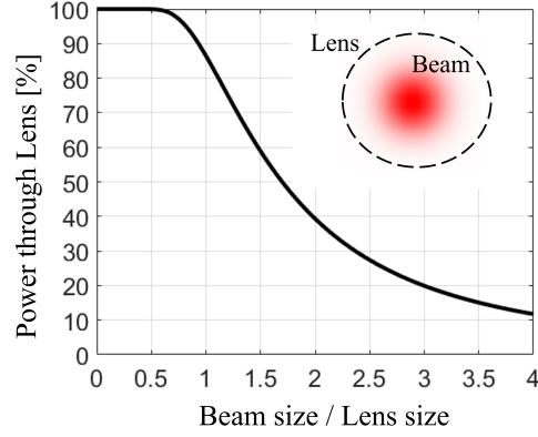
Figure 2.4: The power through a circular aperture. Only 86.5% of a beam's total power passes through a lens with a radius equal to its beam waist.
