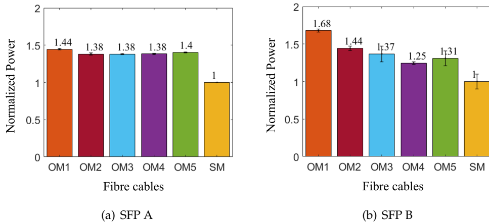
Figure 3.3: Measurements of optical power transmitted through fibre cables when connected to two types of SFP transceiver modules labelled SFP A and B. The optical power is normalized to the power in the single-mode.
