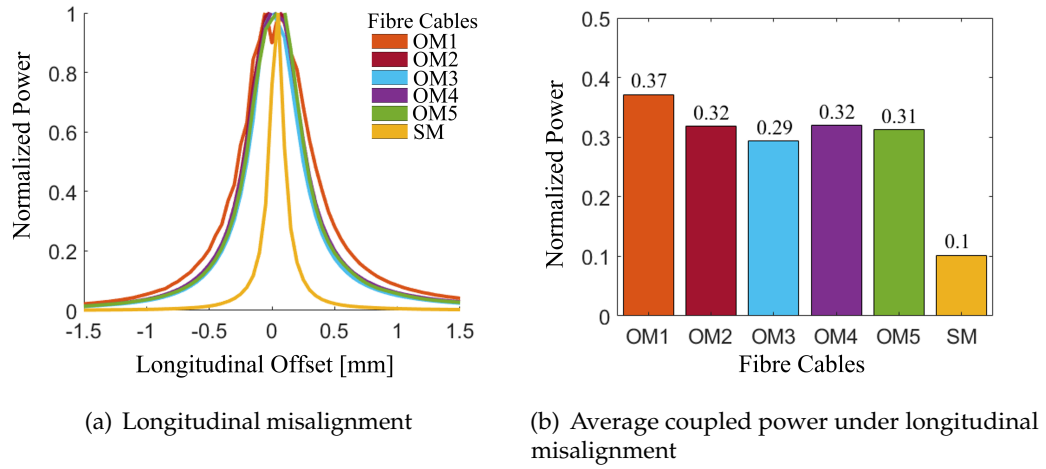
Figure 4.9: Impact of longitudinal misalignment on coupling into standard fibre cables. The longitudinal offset varies within the range of -1.5mm to 1.5mm. Among the fibres, the OM1 fibre cable exhibited the highest average normalized power, while the single-mode fibre showcased the lowest.
