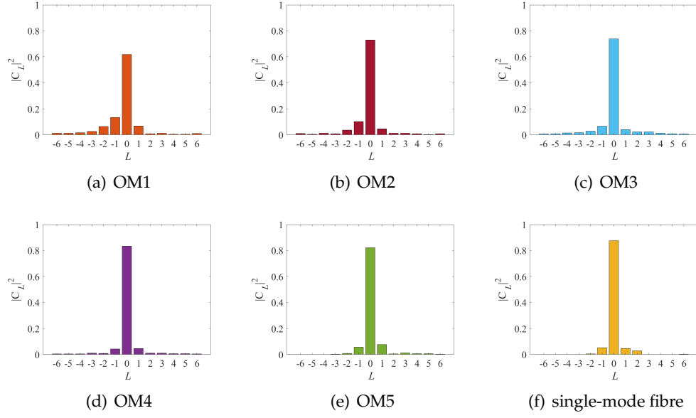
Figure 3.6: Average modal content of beams from SFP B. The modal content was averaged across 5 measurements. All fibre cables exhibited high Gaussian content.
