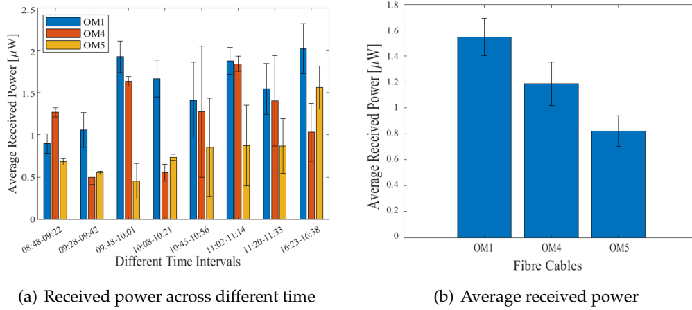
Figure 5.9: Average received power measured in a real-world bidirectional FSO system. Average received power across different times of the day (a). Average received power in each fibre cable across all time intervals measured.
