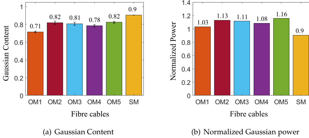
Figure 5.1: Gaussian content in optical fields launched from the fibre cables (a). The product of the Gaussian content and the total power transmitted by the fibre cable relative the the total power transmitted by the single-mode fibre cable.
