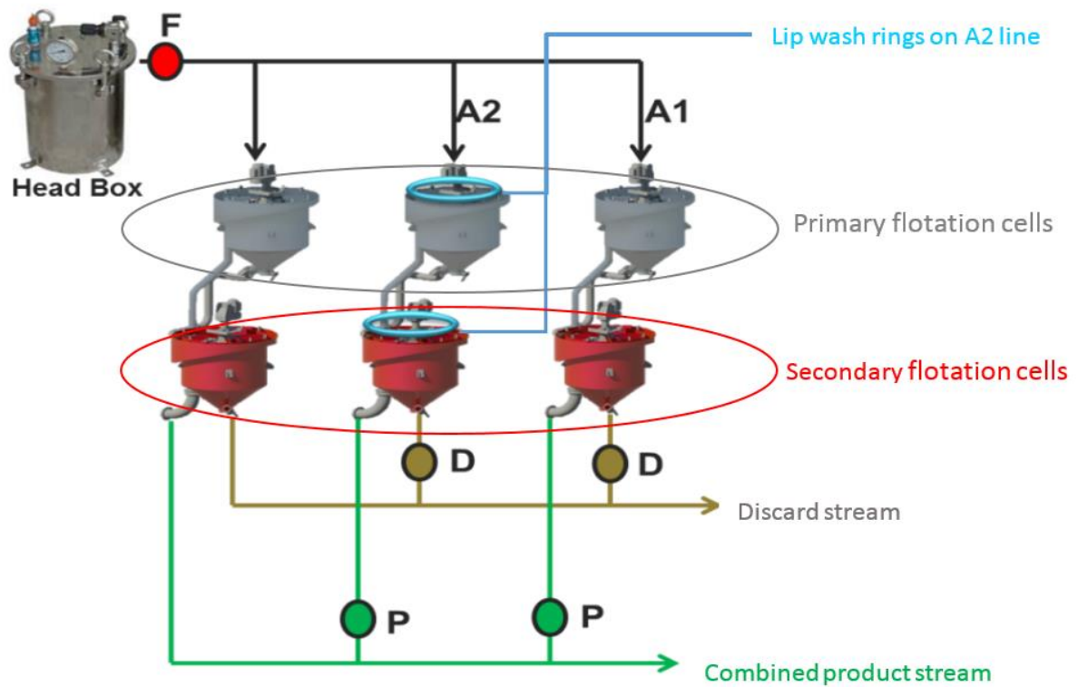
Figure 9: Schematic diagram showing sampling points for test work
