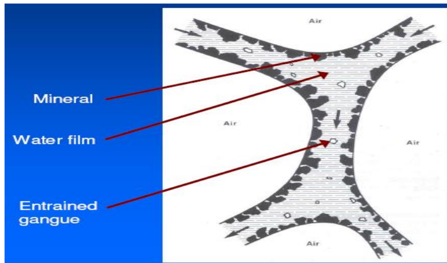
Figure 4: Schematic diagram to illustrate hydraulic entrainment in the froth layer. Adapted from Wills and Napier-Munn (2006)
