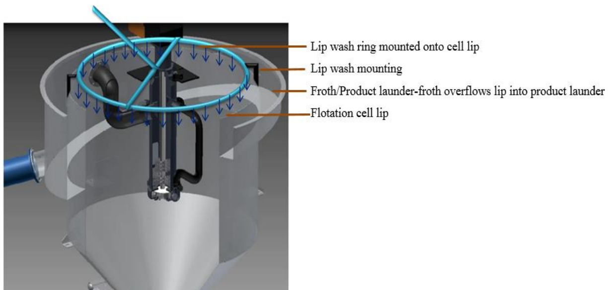
Figure 8: Lip wash design and installation onto a Dual cell (cut-away view of the flotation cell)
