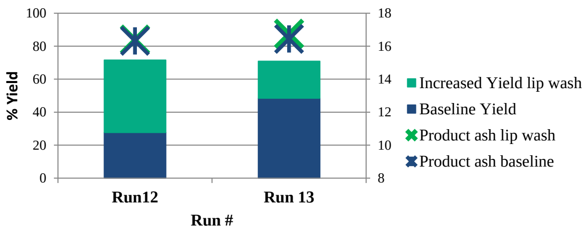
Figure 17: Lip wash results when running the plant in AUTO
