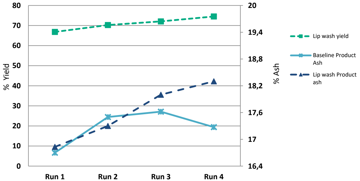
Figure 13: Product quality comparison between Baseline and Lip wash flotation cells for runs 1-4
