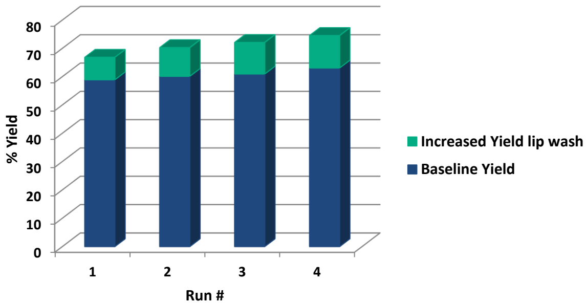
Figure 11: Baseline flotation yield and increased lip wash yield for run 1-4
