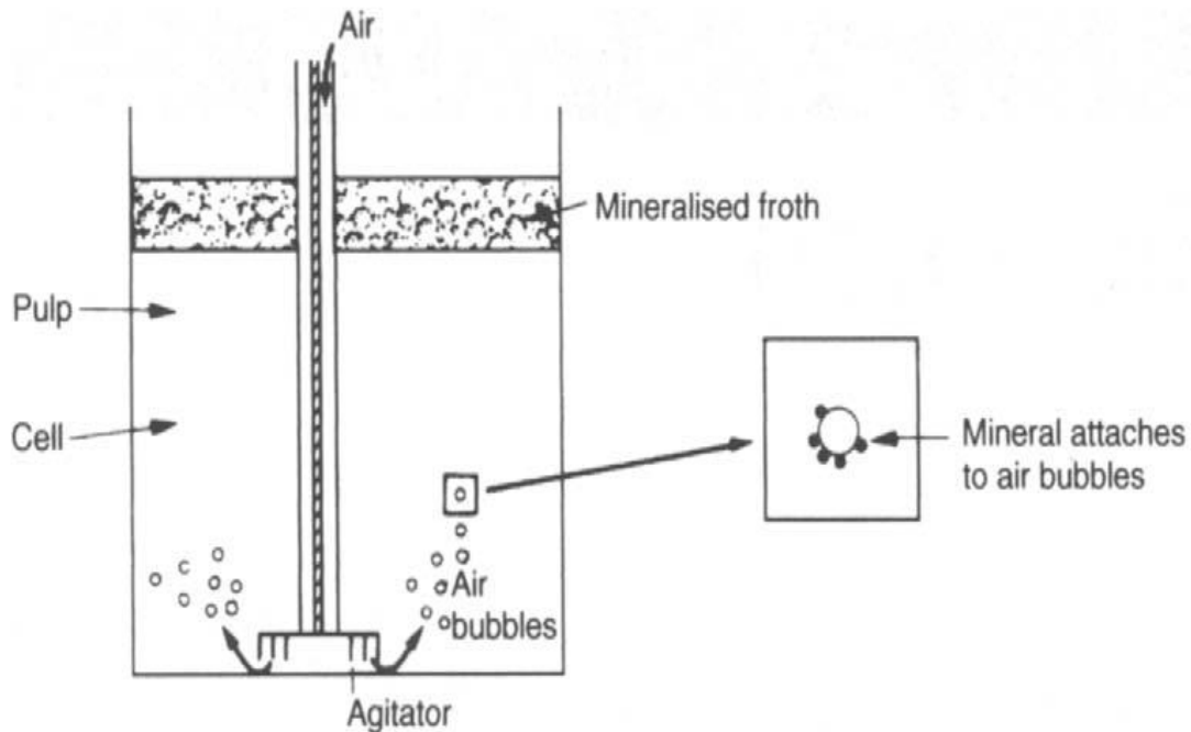
Figure 1: Typical operation of a mechanical flotation cell (Wills and Napier-Munn, 2006)
