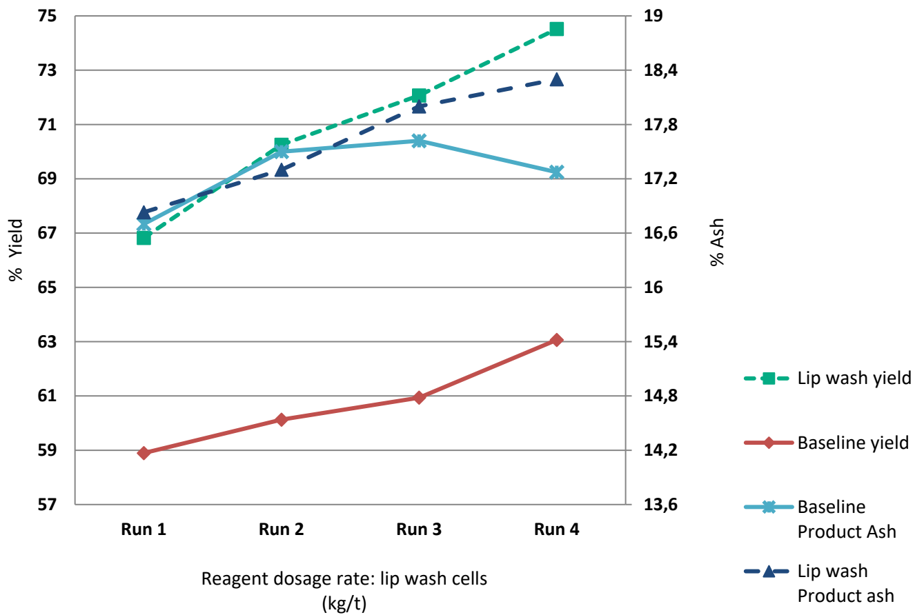
Figure 12: Effect of flotation reagent dosage on % product ash and yield
