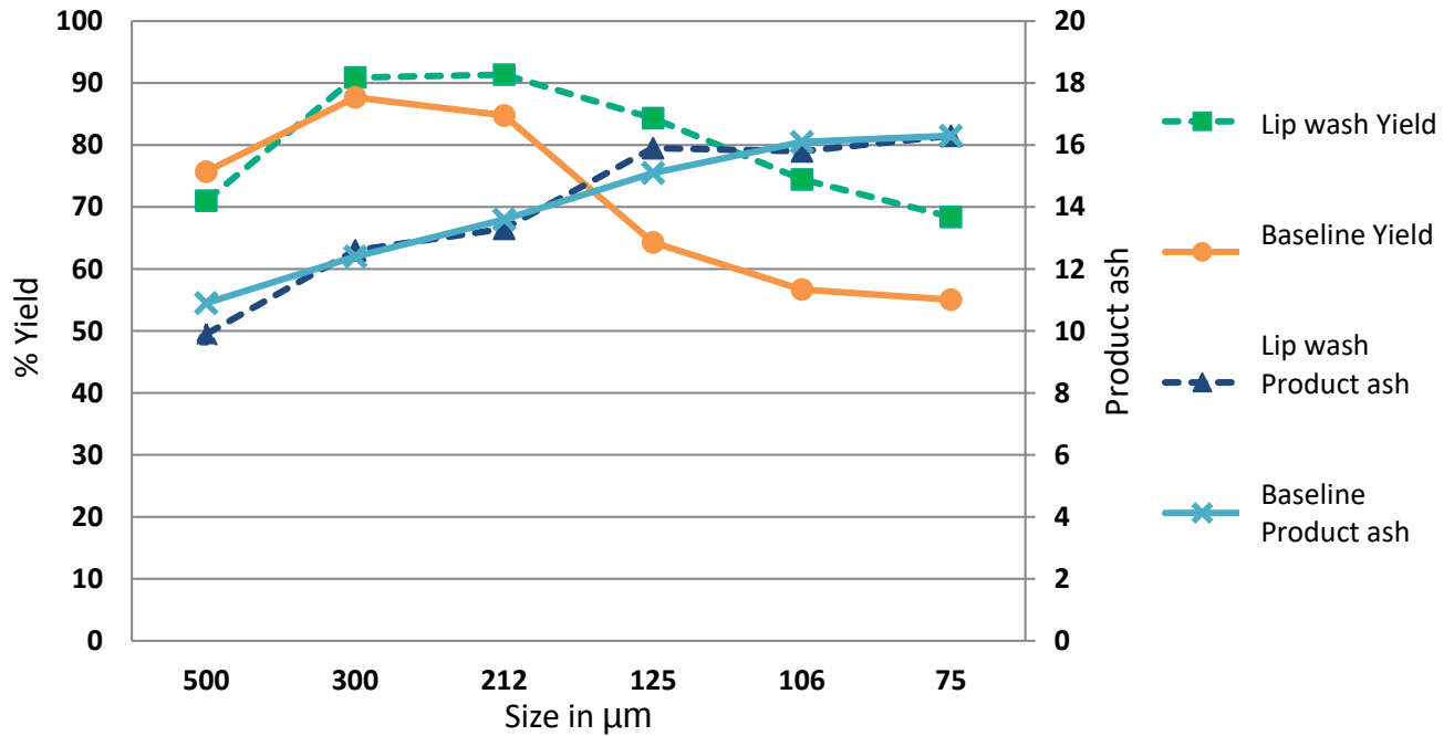
Figure 14: Yield and quality as a function of particle size for run 1
