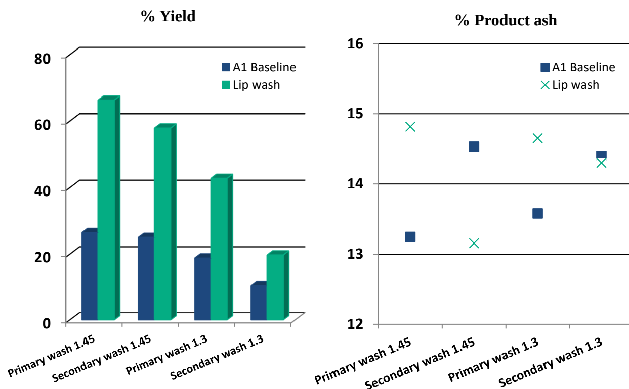
Figure 16: Comparison of Primary Wash Only (PWO) and Secondary Wash Only (SWO)
