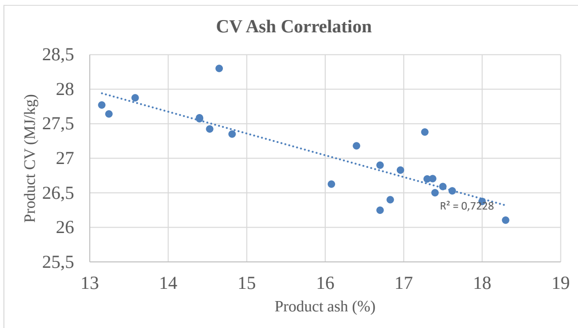
Figure 10: CV vs Ash for all product samples analysed for runs 1-13
