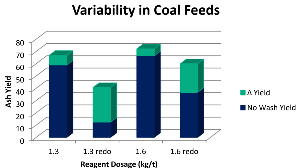
Figure 15: Comparison of lip wash on different coal feed qualities
