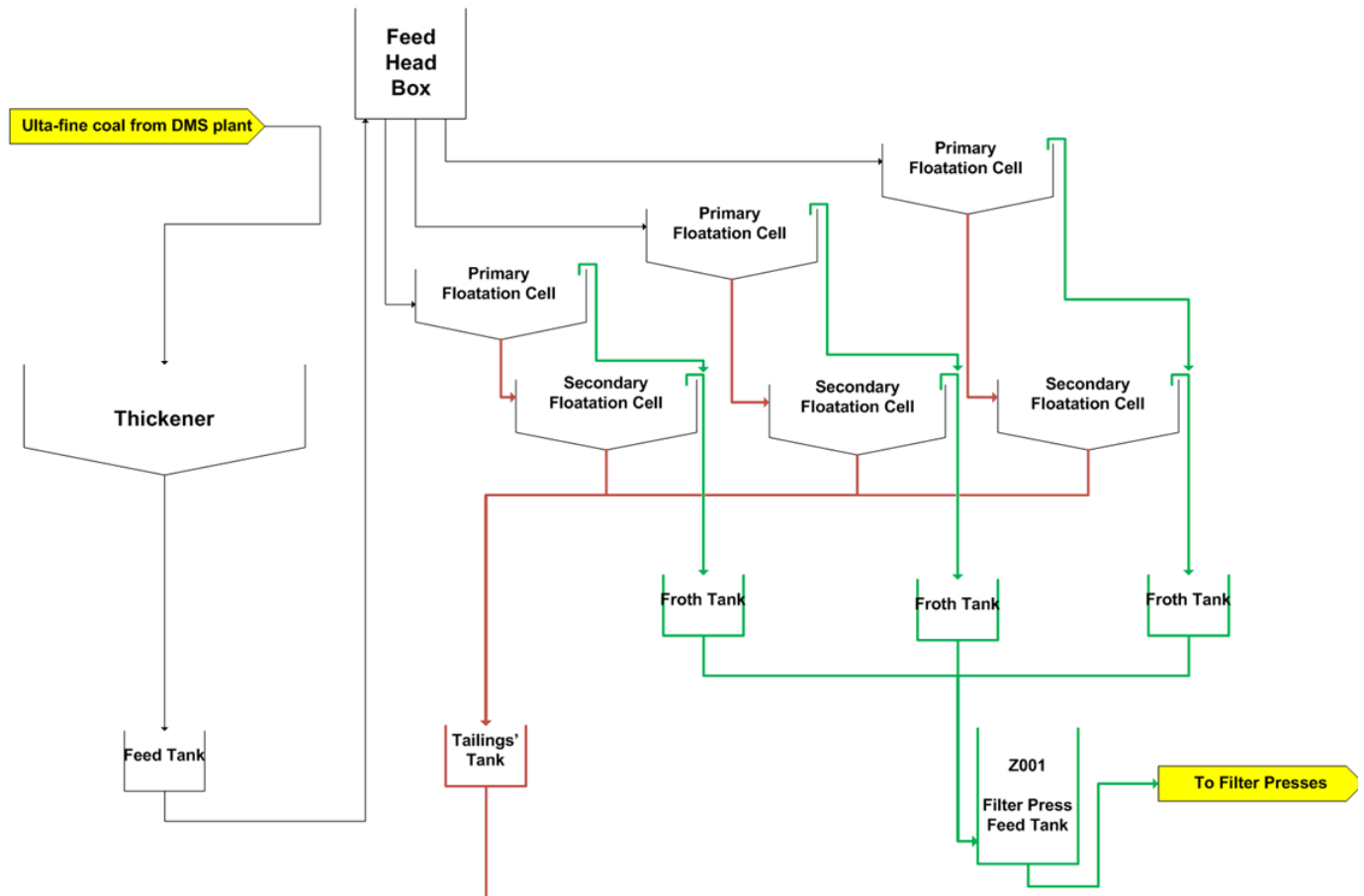
Figure 5: Process flow diagram of a flotation module at GHS
