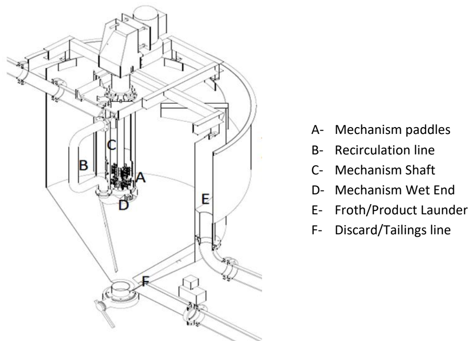
Figure 6: Schematic diagram of the Dual cell patented by Enprotec
