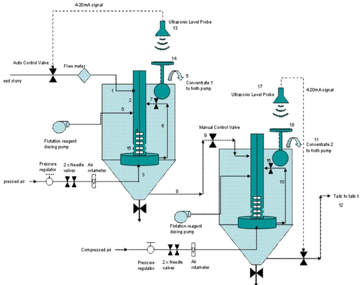
Figure 7: Dual cell process flow and control diagram
