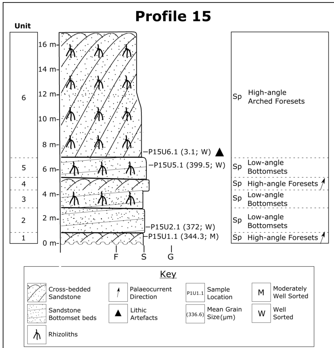
Figure 5.32. The logged sequence of Profile 15. The base of the exposure is 1 m above high tide level.
