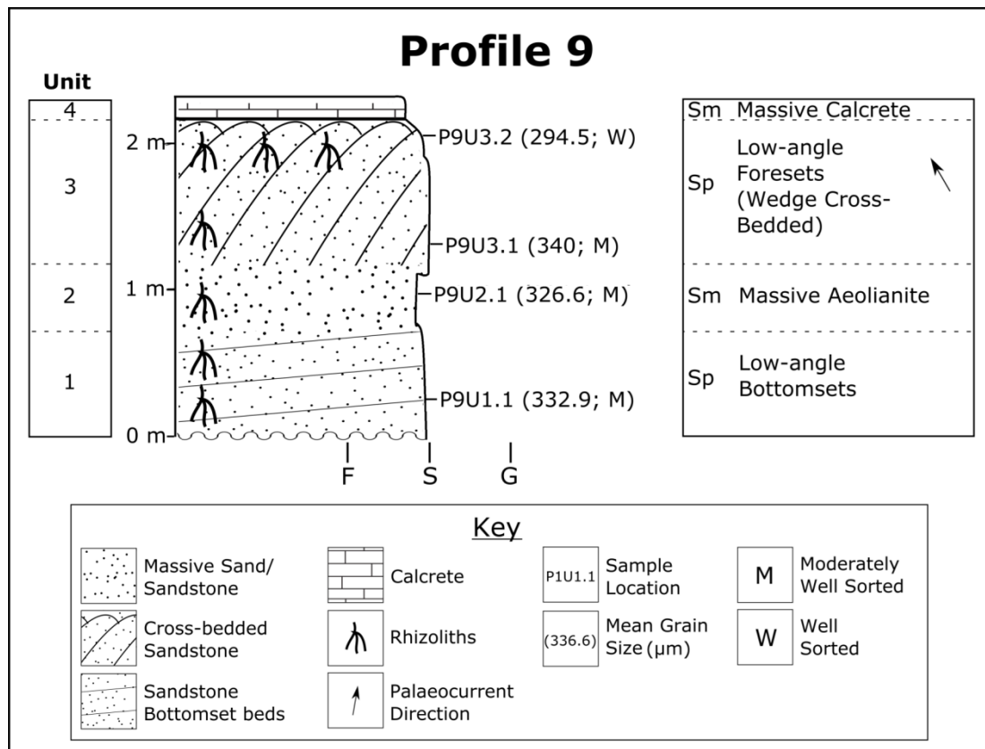
Figure 5.20. The logged sequence of Profile 9. The base of the exposure is 1.5 m above high tide level.
