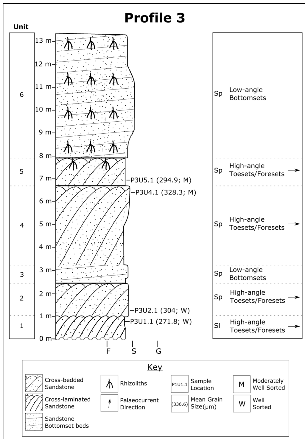
Figure 5.7. The logged sequence of Profile 3. The base of the exposure is 1 m above high tide level.
