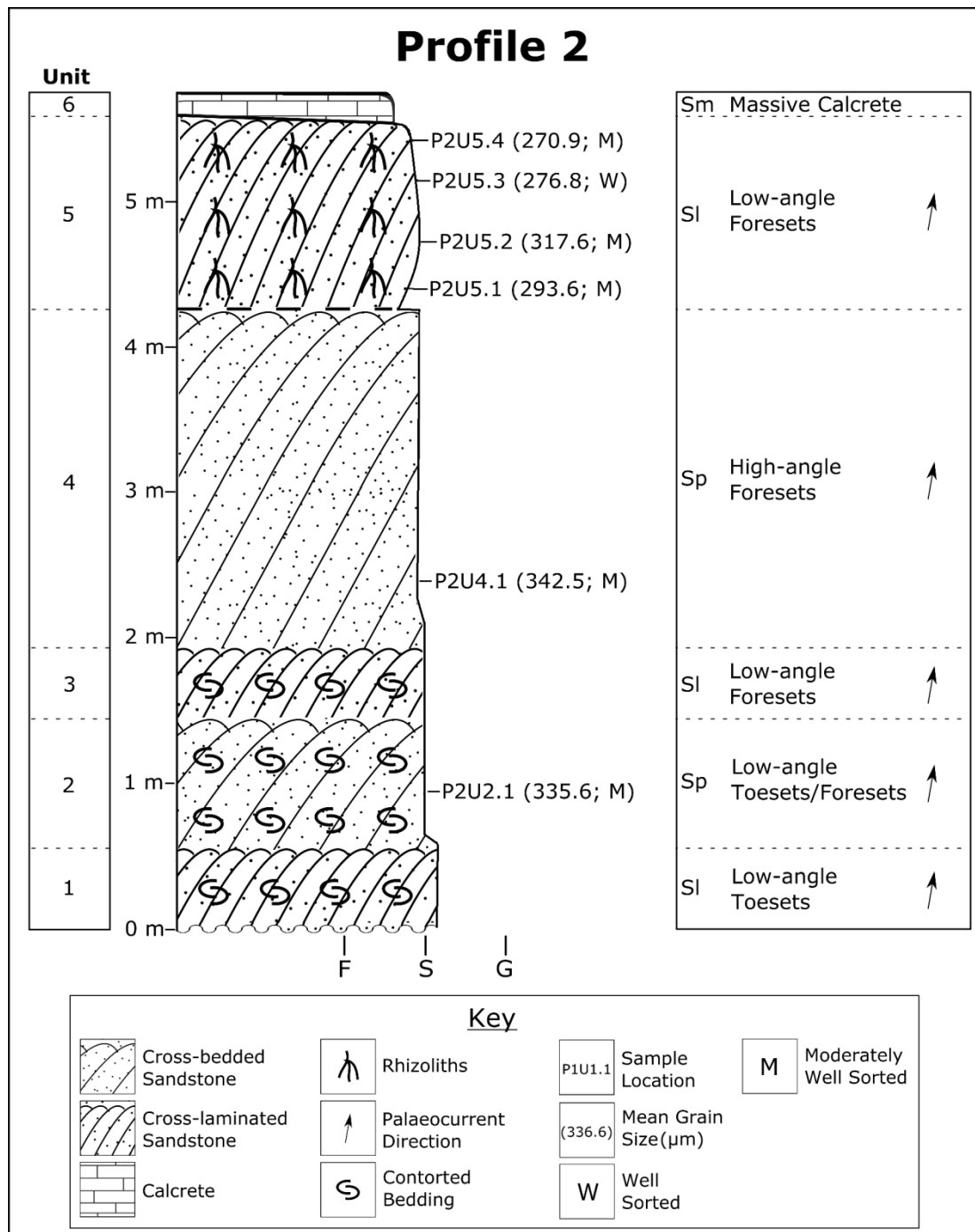
Figure 5.5. The logged sequence of Profile 2. The base of the exposure is 1 m above high tide level.
