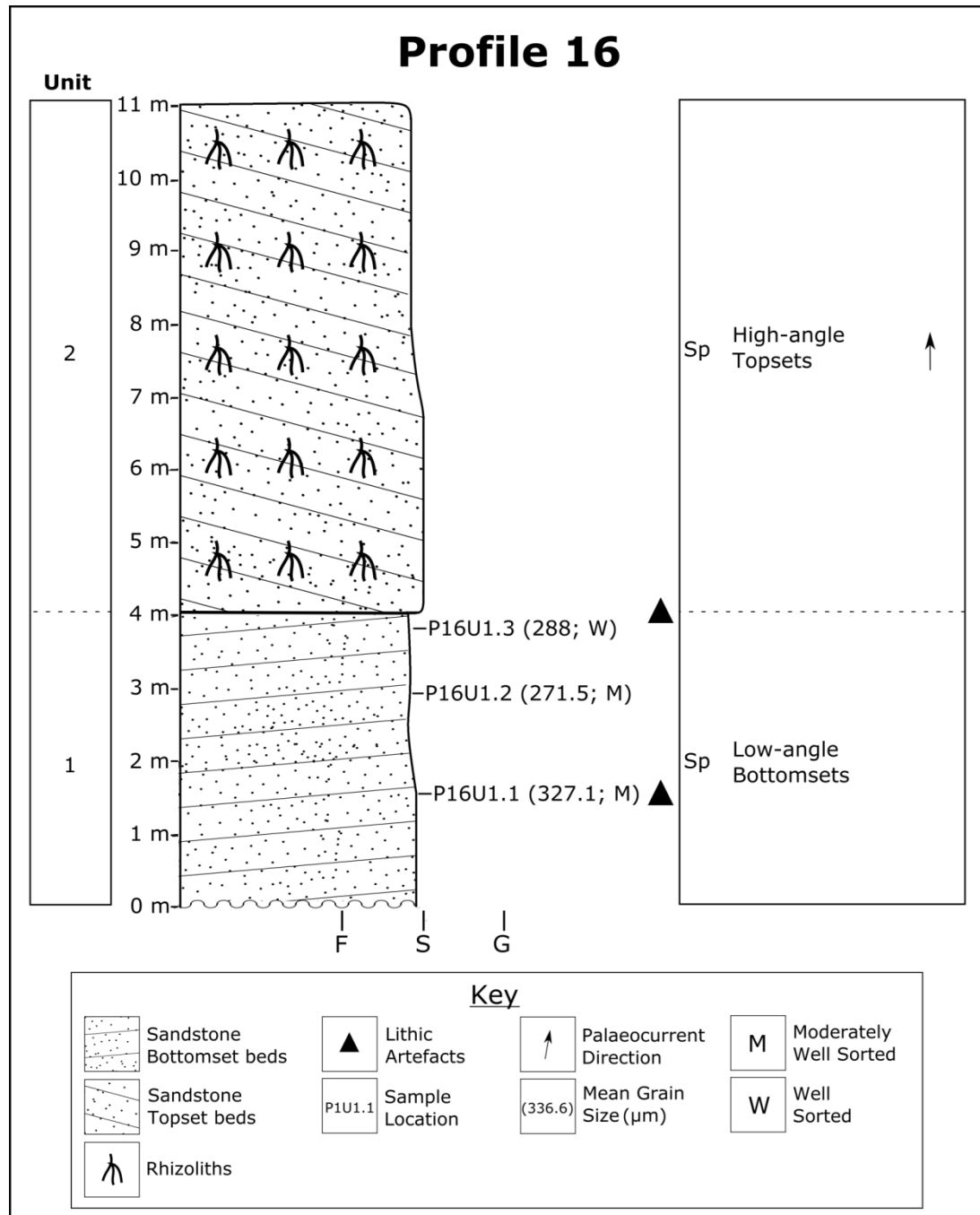
Figure 5.34. The logged sequence of Profile 16. The base of the exposure is 1.2 m below high tide level.
