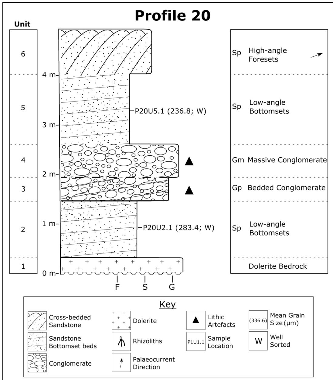
Figure 5.42. The logged sequence of Profile 20. The base of the exposure is 1.4 m below high tide level.
