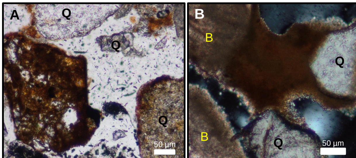
Figure 5.51. Concentrations of clay (the brown to reddish-brown in these images) within both rim cements and pore-filling cements and in the form of obviously altered sand-sized grains: A) sample P1U5.4. B) sample P2U5.2 under cross-polarised light. Bioclasts (B) and quartz grains (Q) are marked. Note the altered sand-sized grain to the left of image A.
