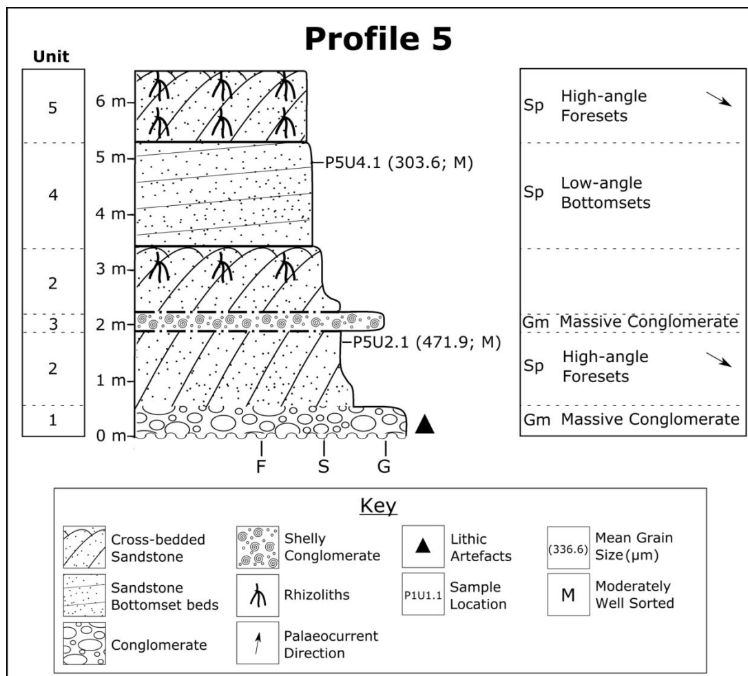
Figure 5.11. The logged sequence of Profile 5. The base of the exposure is 1 m below high tide level.
