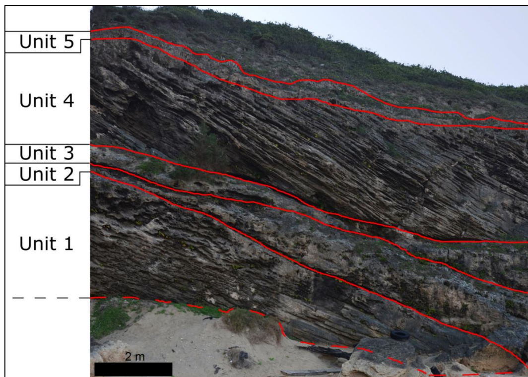
Figure 5.27. A photograph of Profile 12 with the units marked. Note that the contact between Units 1 and 3 (where Unit 2 pinches out) is to the left (280° W) of the part of the exposure shown in the photograph.
