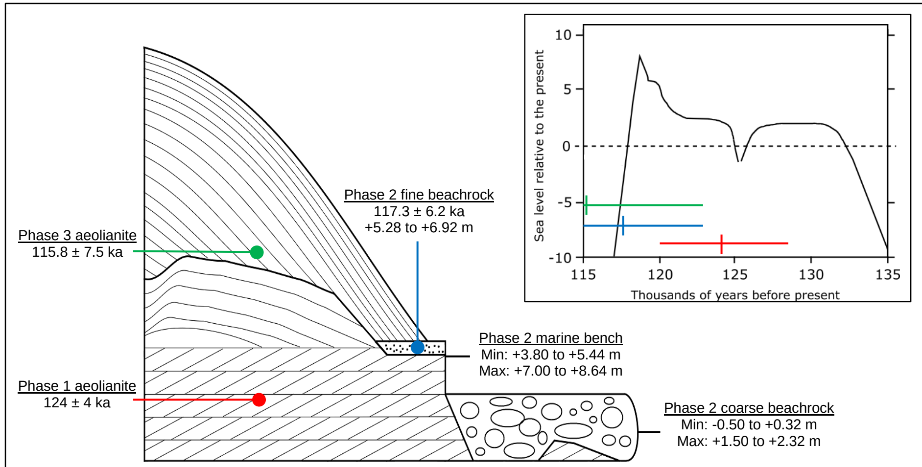
Figure 6.6. A generalised geological cross-section of the deposits in the study area with the sea level estimates for various features indicated. Dates obtained by Jacobs & Roberts (2009) are presented for the dated deposits. Inset: An MIS 5e global sea level graph (after Hearty et al. 2007). The date ranges (horizontal lines) and mean ages (vertical lines) for the three dated deposits are superimposed over the graph. Note that the date ranges for the Phase 2 fine beachrock and the Phase 3 aeolianite continue beyond the edge of the graph, past 115 ka.
