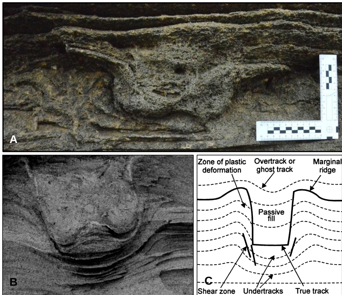
Figure 6.4. Comparison between a track observed at Nahoon Point and published real-world and theoretical examples of similar tracks. A: cross-section of a track preserved in the aeolianite at the Footprint Site. B: photograph of a naturally-produced cross-section through an ungulate track preserved in Holocene aeolian deposits in the Nebraska Sand Hills (Loope 1986). C: theoretical cross-section of an animal track and associated sediment deformation in a stratified deposit (Fornos et al. 2002).
