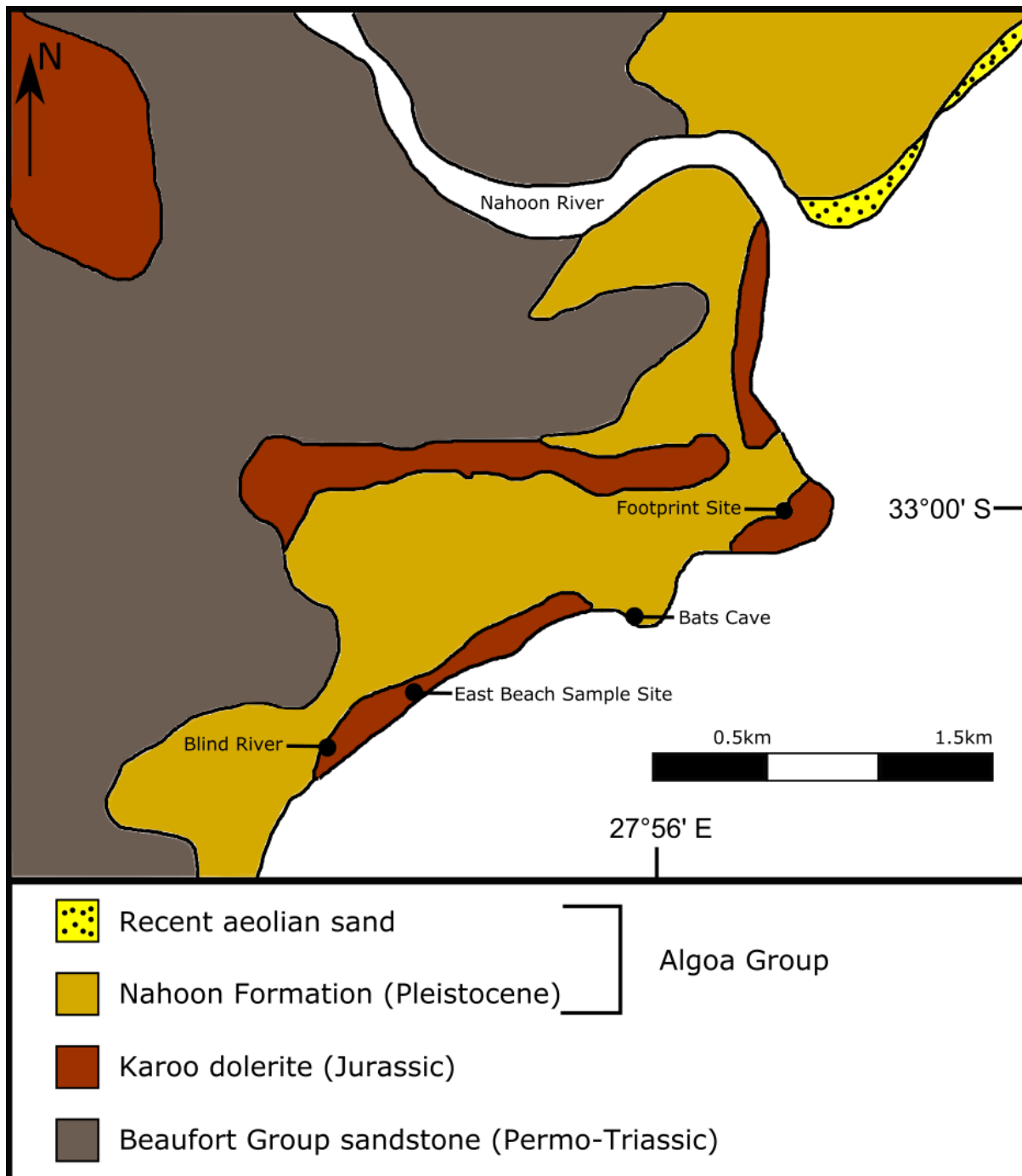
Figure 2.3. The geology of the area around Nahoon Point (modified from Roberts 2008). Note that the marine and estuarine deposits of the Pleistocene Salnova Formation are not mapped. Roberts (2008) did not state why they were not mapped. The recent aeolian sand deposits are of the Schelm Hoek Formation.
