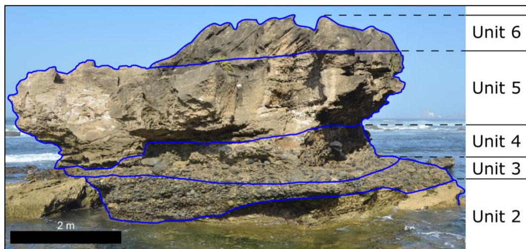
Figure 5.43. A photograph of Profile 20 with the units marked. Unit 1, the dolerite, is not visible as it is underwater.
