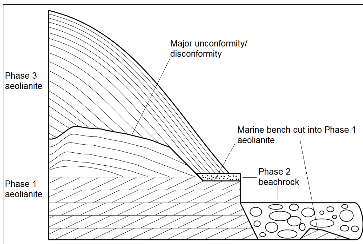
Figure 6.2. A generalised stratigraphic cross-section of the aeolianite and beachrock deposits in the study area. The sea is to the right and the land to the left of the diagram. Note the position of the major unconformity/disconformity between the Phase 1 and 3 aeolianites and the marine benches cut into the Phase 1 deposits.
