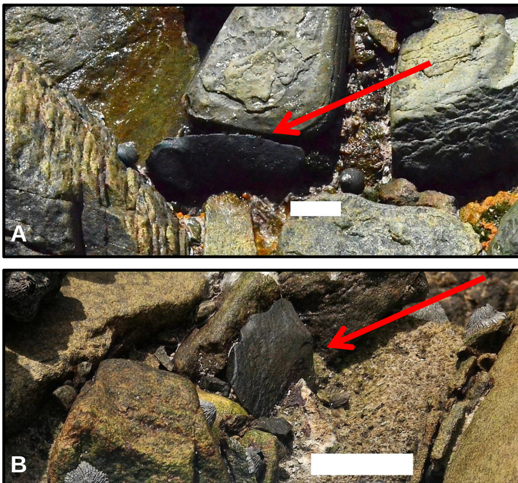
Figure 5.48. A blade (A) and a flake (B) (arrowed) photographed in situ within the conglomerate deposit near Bats Cave. The scale bars are 2 cm long in both photographs.
