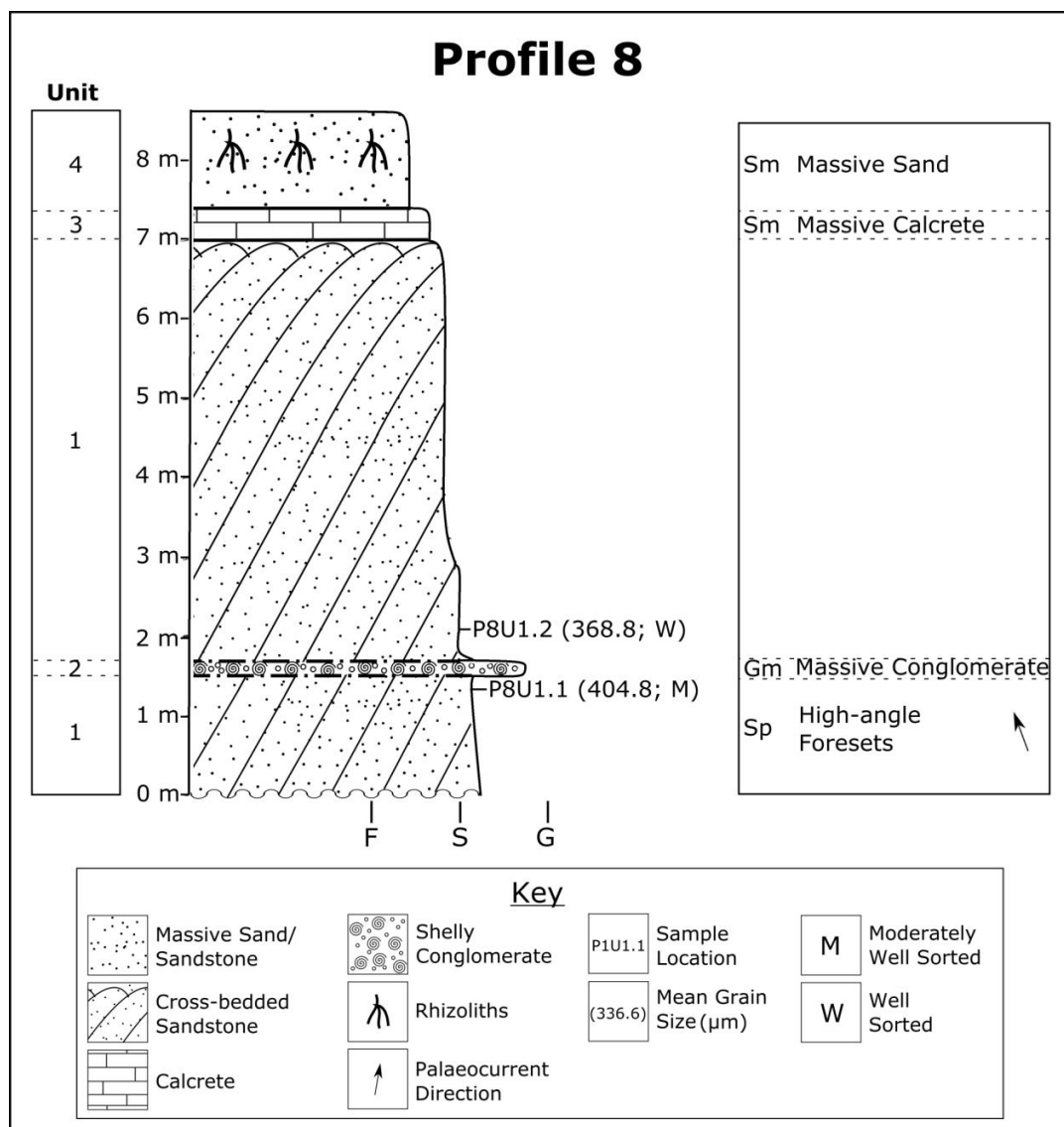
Figure 5.18. The logged sequence of Profile 8. The base of the exposure is 0.5 m below high tide level.
