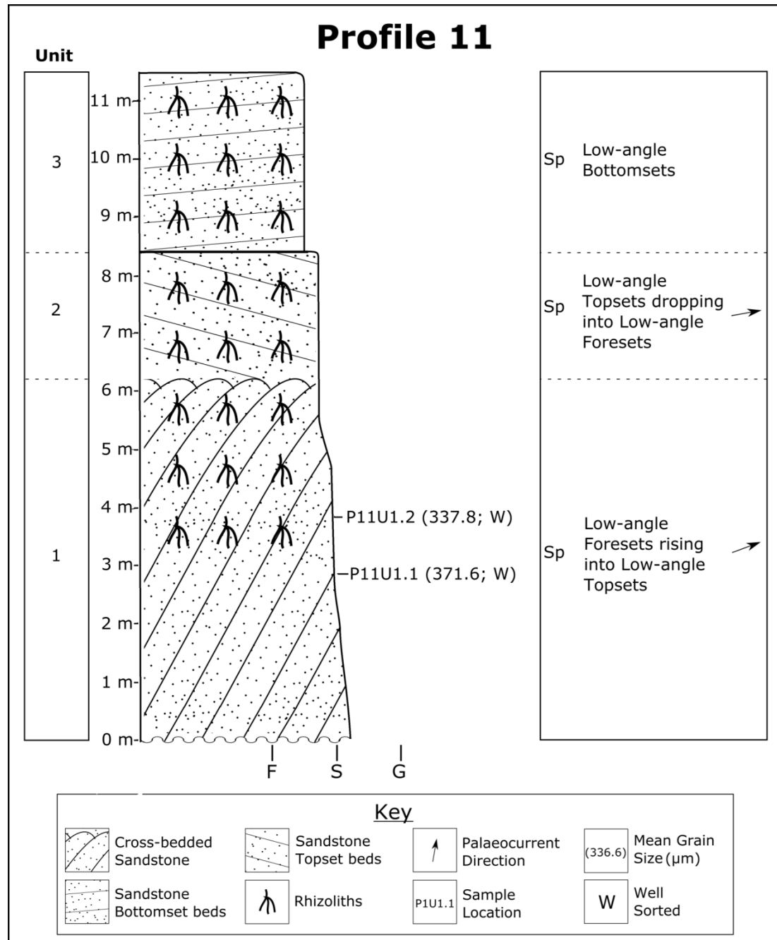
Figure 5.24. The logged sequence of Profile 11. The base of the exposure is 1 m above high tide level.
