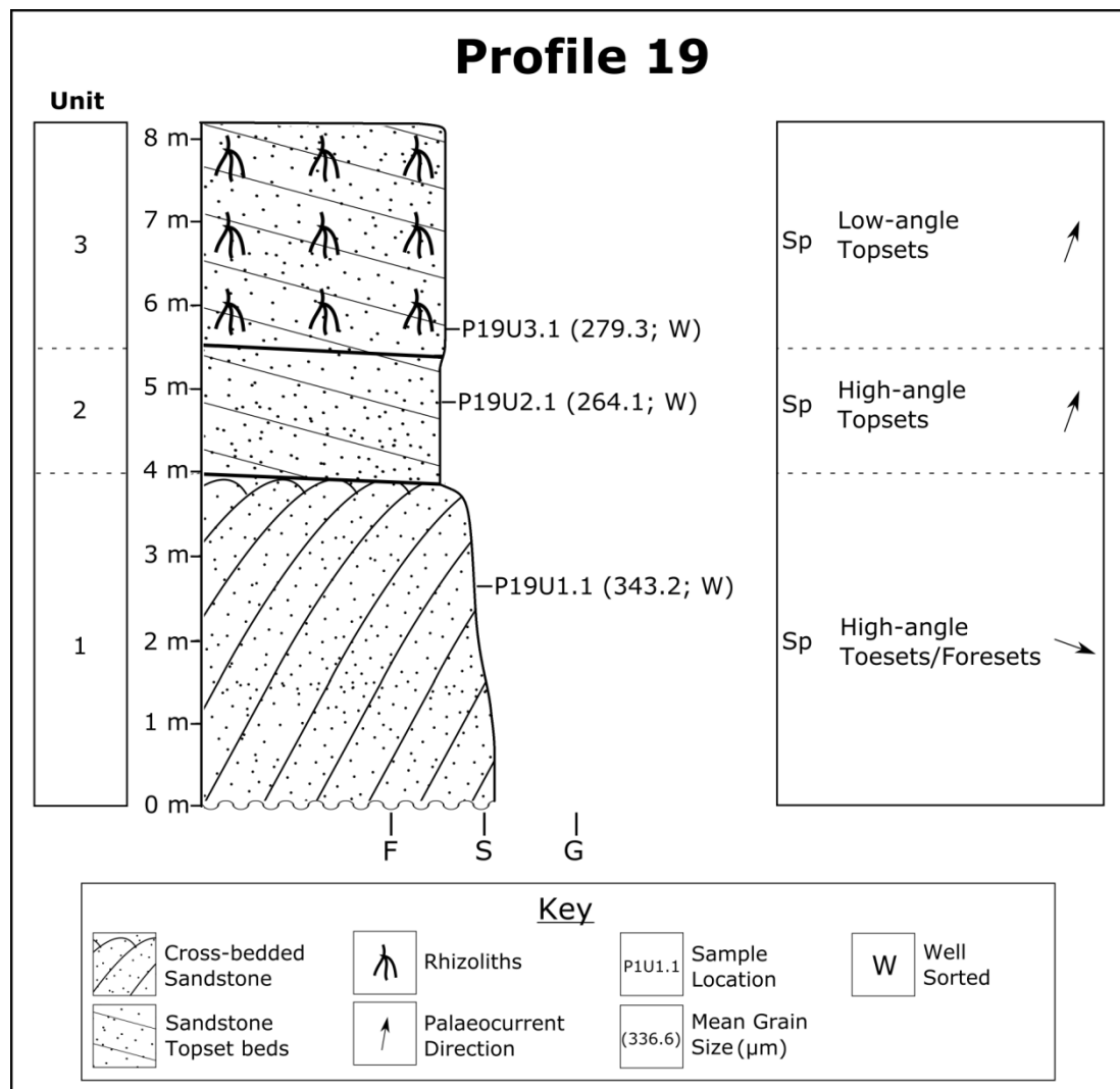
Figure 5.40. The logged sequence of Profile 19. The base of the exposure is 0.5 m below high tide level.
