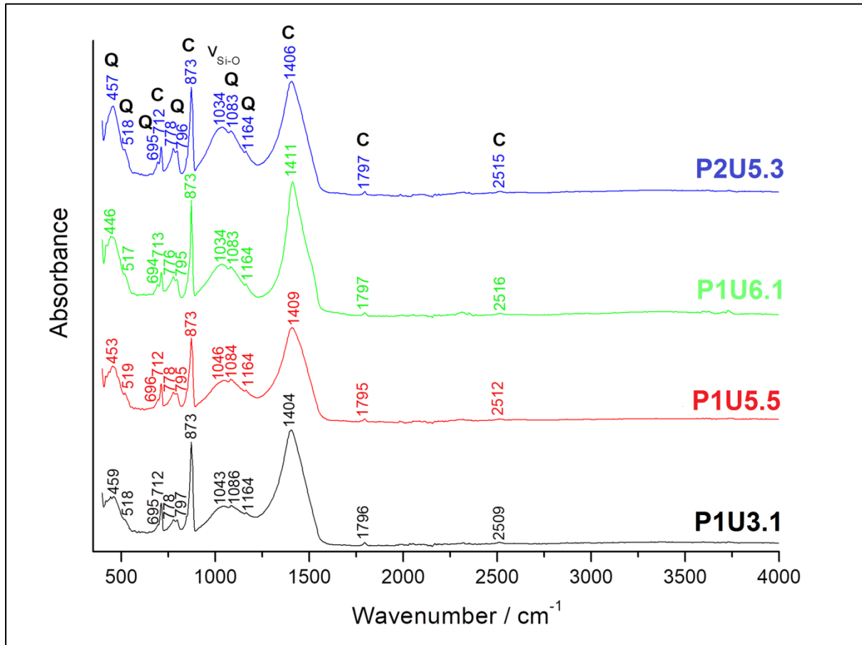
Figure 5.52. The ATR-FTIR spectra for the four analysed samples (figure courtesy of M. Wojcieszak). On the spectra, the letter 'C' indicates peaks associated with calcite, the letter 'Q' denotes peaks attributed to quartz, and 'V Si-O ' marks the stretching vibrations of Si-O bonds, interpreted as showing the presence of clay.
