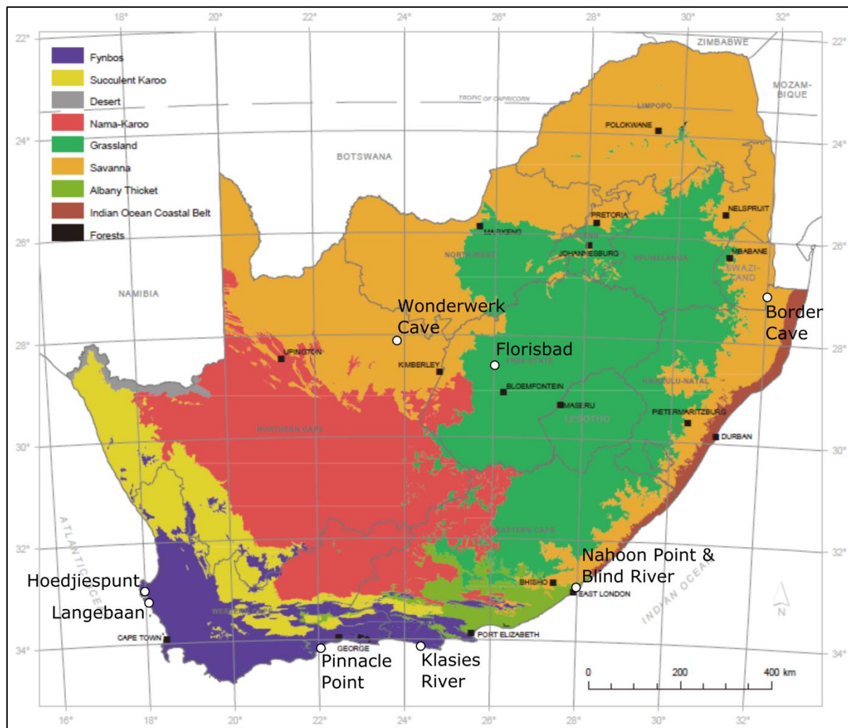
Figure 3.4. The locations of South African MIS 5e/5d (130 – 105 ka) archaeological and palaeoanthropological sites and the current extent of the major biomes within South Africa (after Rutherford et al. 2006). Note that the Fynbos biome and GCFR are broadly comparable geographically.
