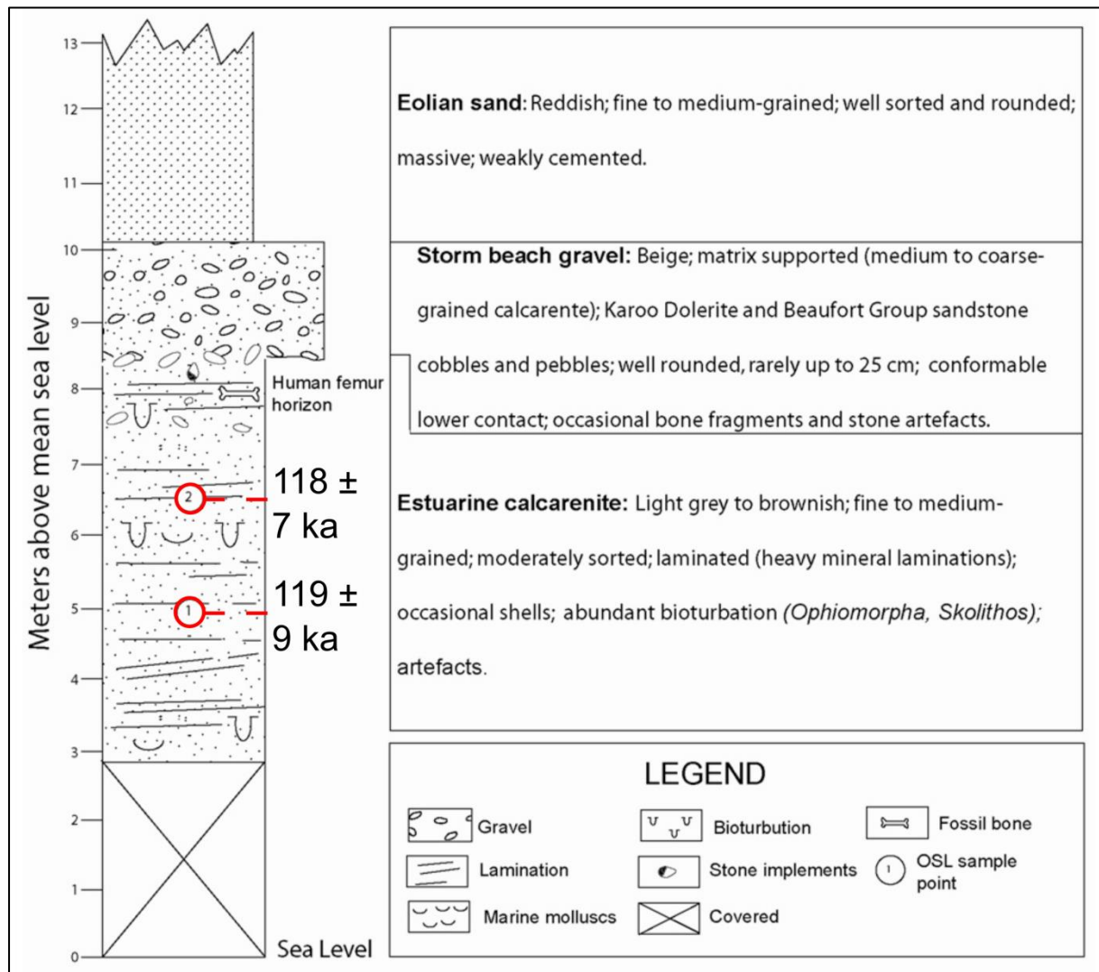
Figure 2.7. The sedimentary profile at Blind River, with the dating sample locations and their respective age determinations indicated (after Wang et al. 2008).
