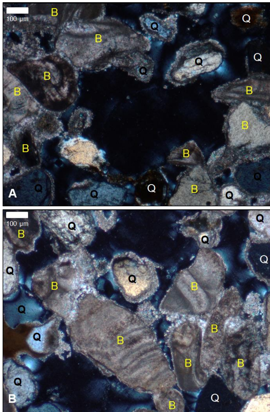
Figure 5.50. Photomicrographs of sample P2U5.2 taken under cross-polarised light. Bioclasts (B) and quartz grains (Q) are marked.
