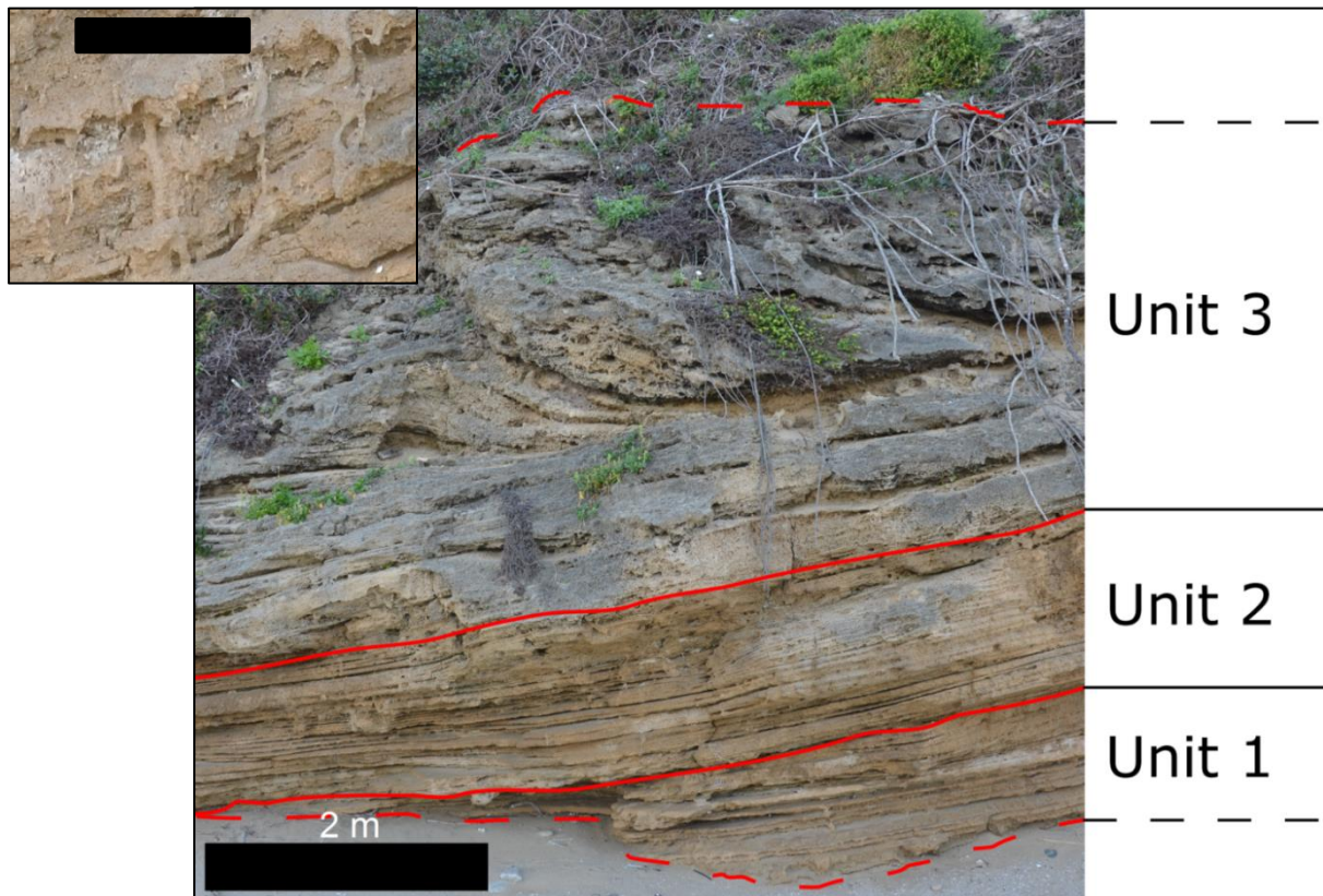
Figure 5.23. A photograph of Profile 10 with the units marked. Inset: a close-up photograph of several rhizoliths in Unit 3 (scale bar is 10 cm).
