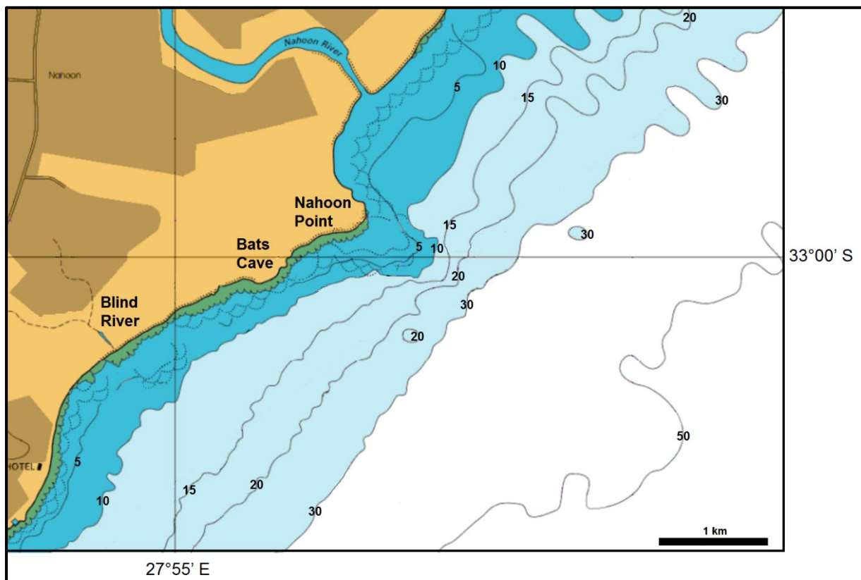
Figure 2.4. The bathymetry of the nearshore area along the coastline around Nahoon Point (after Admiralty 2005). The contours are in metres. The semi-circles in the shallowest areas indicate the positions of known rocky outcrops on the seabed.
