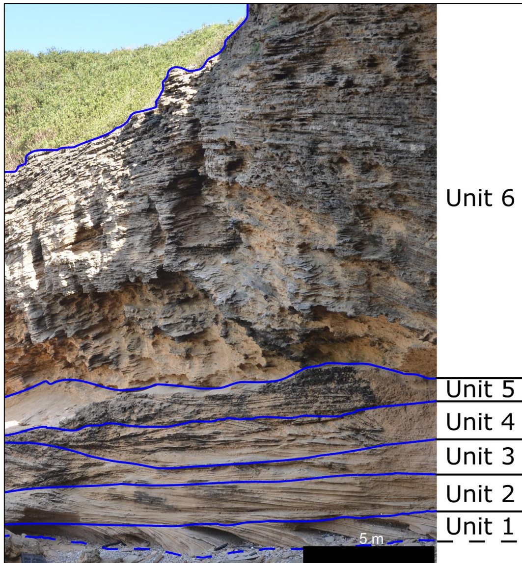
Figure 5.33. A photograph of Profile 15 with the units marked.
