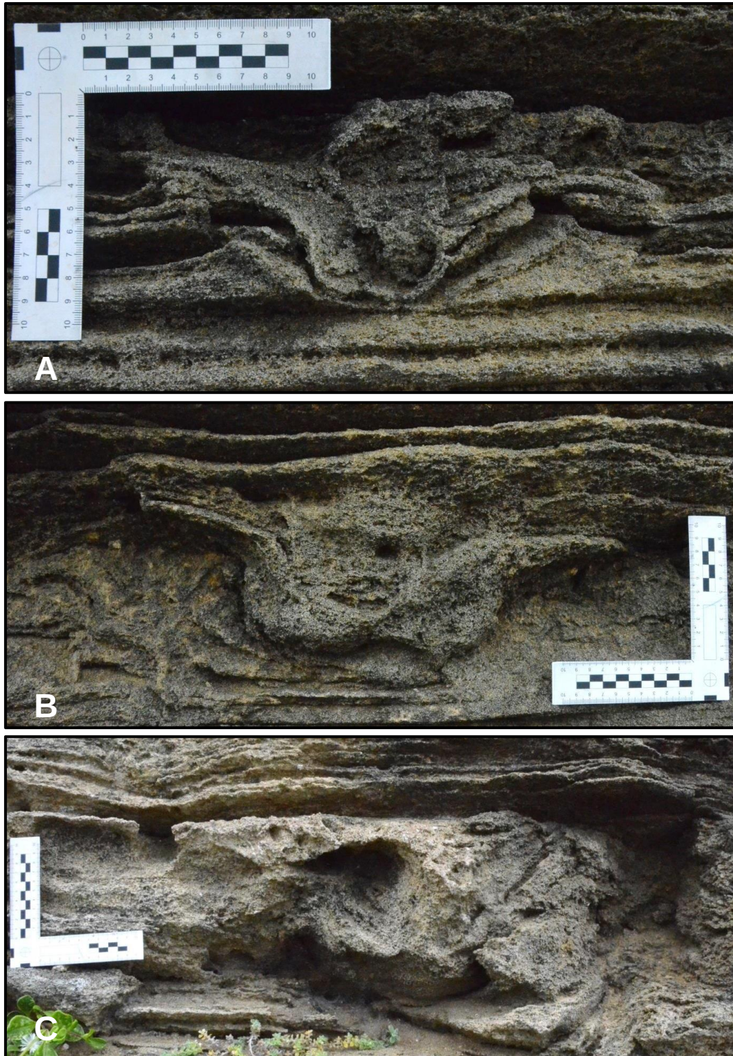
Figure 5.4. Several examples of disturbed bedding Unit 3 of Profile 1. These “types” are found throughout the units where disturbances occur (P1: U1, U3 and U5; P2: U1, U2 and U3) with no indication of lateral or stratigraphic patterns in the distribution of different forms. These features range from 5 cm to 50 cm in overall width.
