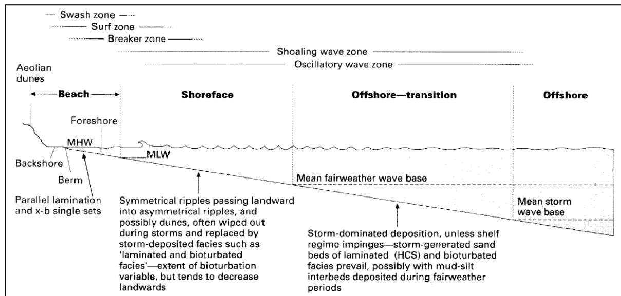
Figure 3.2. A cross-section through a generalised shoreline profile with the various zones indicated (Reading & Collinson 1996).
