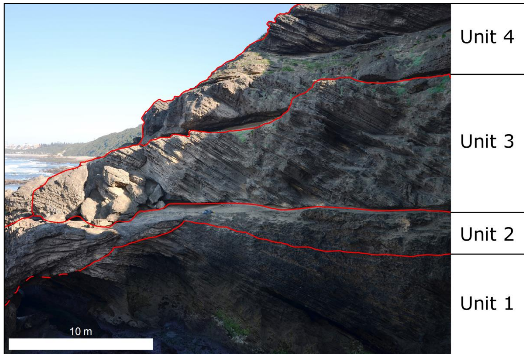
Figure 5.39. A photograph of Profile 18 with the units marked.
