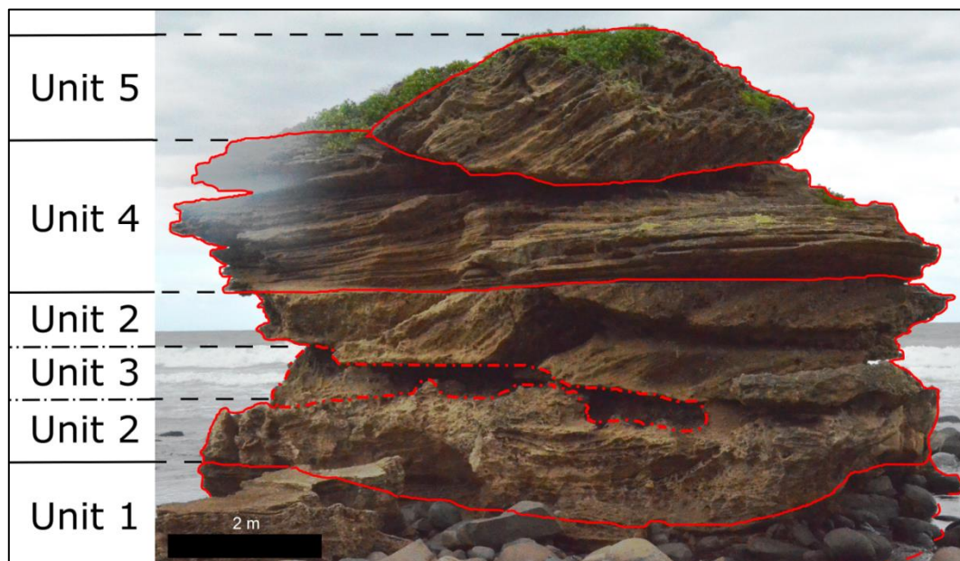
Figure 5.12. A photograph of Profile 5 with the units marked.
