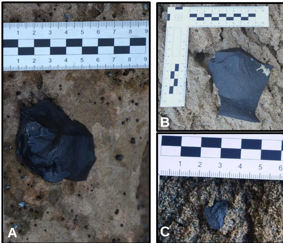
Figure 5.47. Examples of artefacts discovered in aeolianite units in Profile 16. A) the single lithic in Unit 1. B) relatively large overshoot flake found at the contact between Unit 1 and Unit 2. C) small flake found at the contact between Unit 1 and Unit 2. All artefacts were photographed in situ within the aeolianite.
