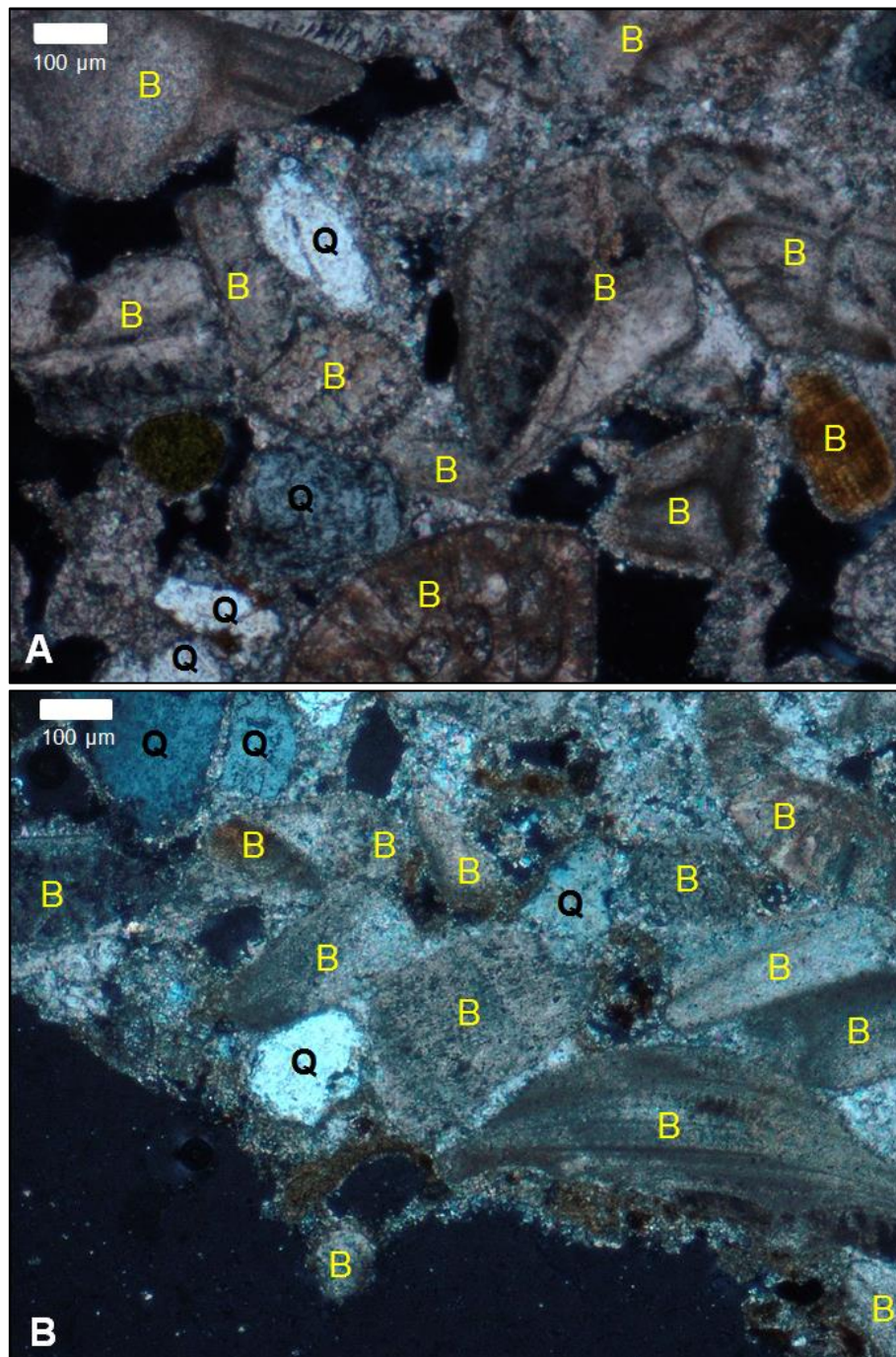
Figure 5.49. Photomicrographs of sample P1U5.4 taken under cross-polarised light. Bioclasts (B) and quartz grains (Q) are marked.
