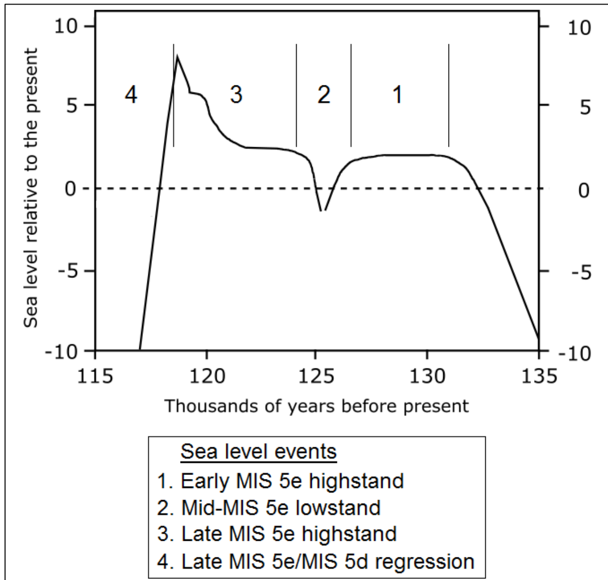
Figure 1.1. The four major sea level ‘events’ during MIS 5e and early MIS 5d (after Hearty et al. 2007). Age ranges for the events are presented in the text above. Note that the relative sea levels reached during the first and second highstands may have been more similar to one another than reflected in this particular diagram.
