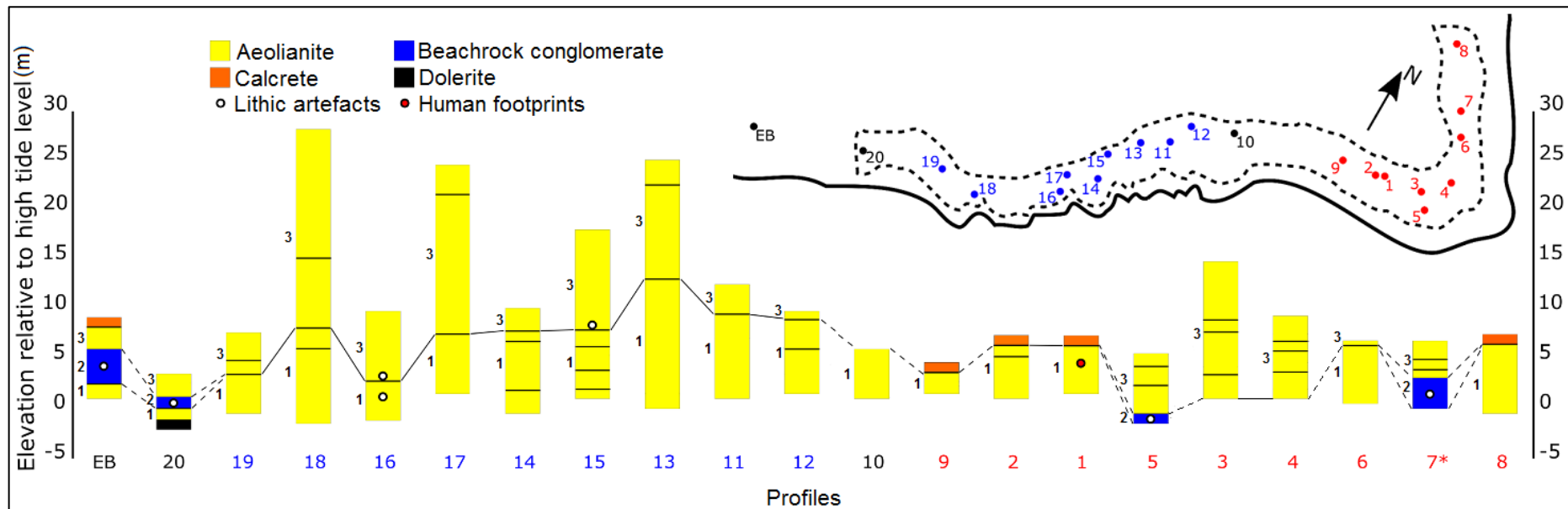
Figure 6.1. Stratigraphic correlation of the logged profiles (which have been simplified in this diagram) across the study area. Profiles marked in red are on Nahoon Point and those indicated in blue are within the continuous exposure. Note that the published profile for the East Beach (EB) sample site, recorded by Jacobs & Roberts (2009), has been included. The major unconformity/disconformity is indicated with solid lines where it could be tracked directly and with dashed lines where the correlation was inferred (see the text for discussion). Phase 1 includes the aeolianite below the major unconformity/disconformity, while the aeolianites of Phase 3 lie on top of the unconformity. The beachrock conglomerates of Phase 2 are correlated with the hiatus between Phase 1 and Phase 3, which is marked by the major unconformity. The younger marine and aeolian deposits (of Holocene age) are not included in this diagram. Note that the calcrete and dolerite units and the beachrock in Profile 5 have been thickened to make them visible in the diagram. Profile 7 (indicated with an asterisk) has been doubled in height for the same reason. The locations of the profiles within the reserve (solid line) and within the study area (dashed line) are indicated in the inset map.
