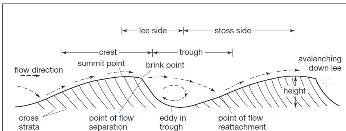
Figure 3.1. A cross section schematic of idealised dunes which depicts the different features of a dune and the processes that occur around these features (after Boggs 2014).
