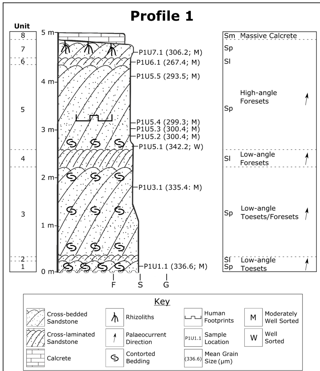
Figure 5.2. The logged sequence of Profile 1. The base of the exposure is 1.5 m above high tide level.
