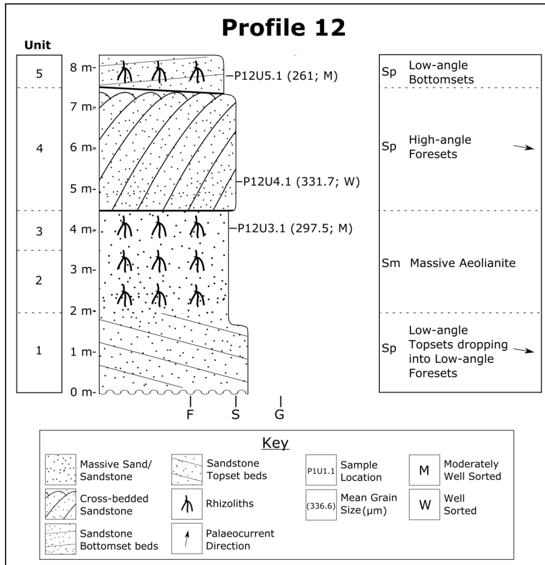
Figure 5.26. The logged sequence of Profile 12. The base of the exposure is 1.5 m above high tide level.
