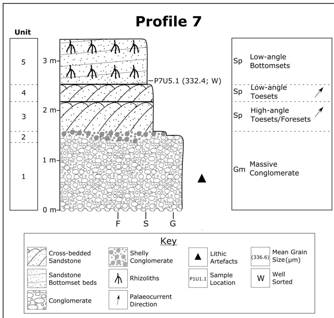
Figure 5.16. The logged sequence of Profile 7. The base of the exposure is at high tide level.
