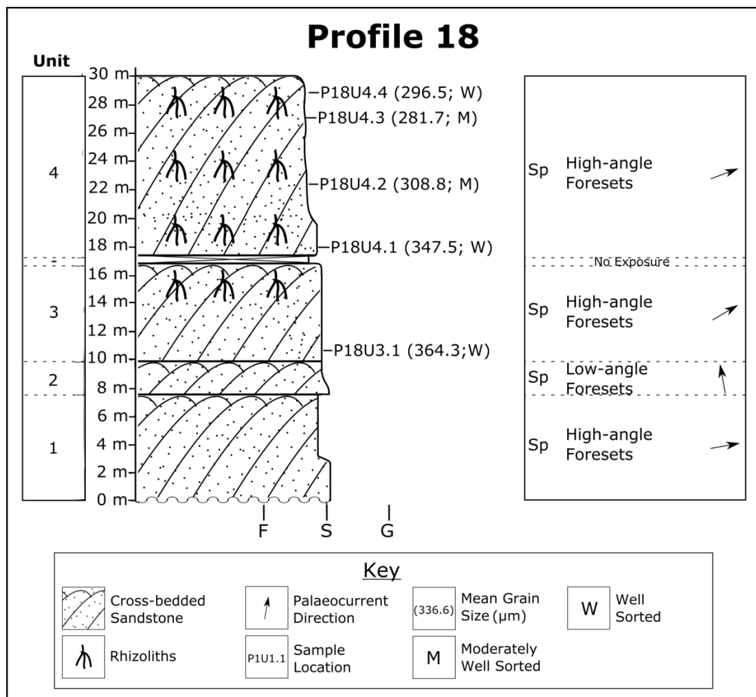
Figure 5.38. The logged sequence of Profile 18. The base of the exposure is 1.5 m below high tide level.
