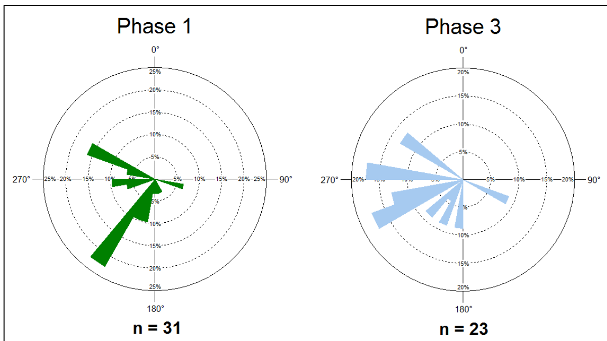
Figure 6.5. Wind roses for Phase 1 and Phase 3 based on dune bedding dip orientation measurements collected from the 20 logged profiles.
