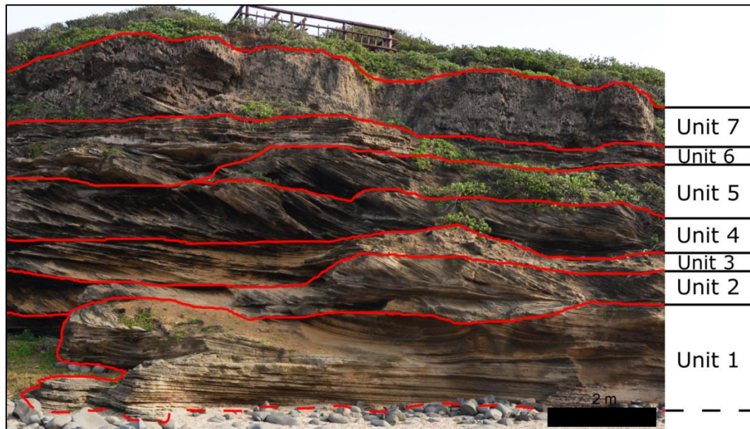
Figure 5.10. A photograph of Profile 4 with the units marked.
