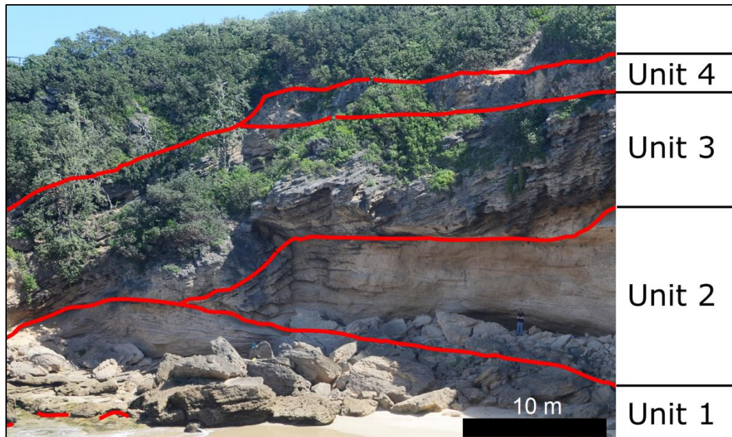
Figure 5.29. A photograph of Profile 13 with the units marked. The sediment above Unit 4 is an unconsolidated aeolian deposit of Holocene age.
