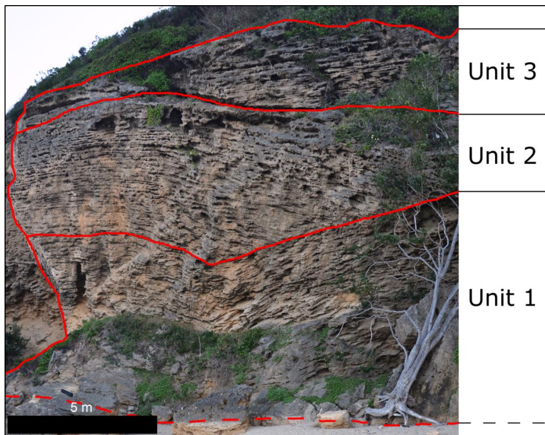
Figure 5.25. A photograph of Profile 11 with the units marked.
