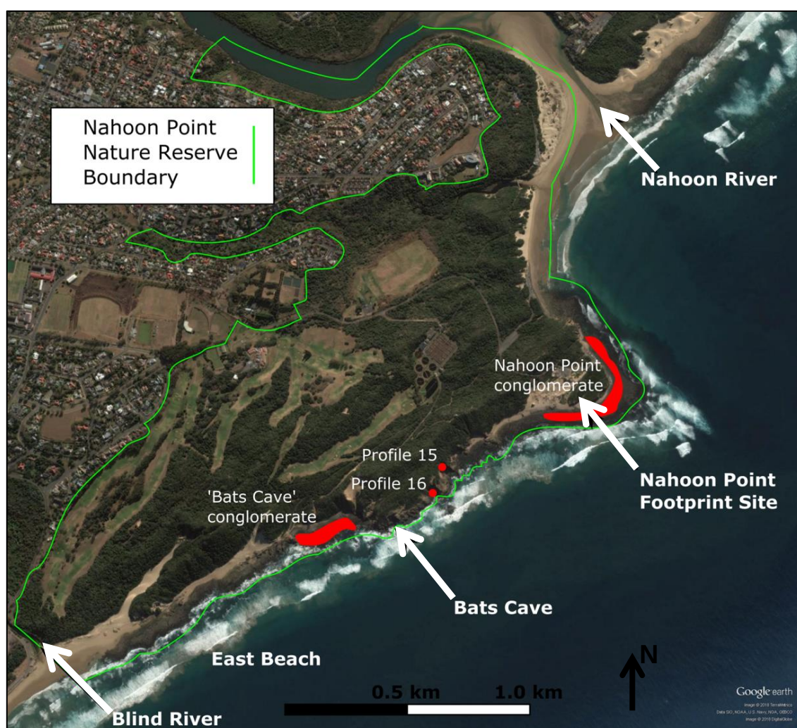
Figure 5.44. Map of the Nahoon Point Nature Reserve indicating the locations of artefact-bearing deposits discovered and/or recorded during the survey of the study area (in red) and several previously reported sites (white arrows) (Imagery: Google Earth, 23 July 2017). As discussed in the text, the artefacts from Profiles 5 and 7 are within the Nahoon Point conglomerate, while those from Profile 20 are within the 'Bats Cave' conglomerate.
