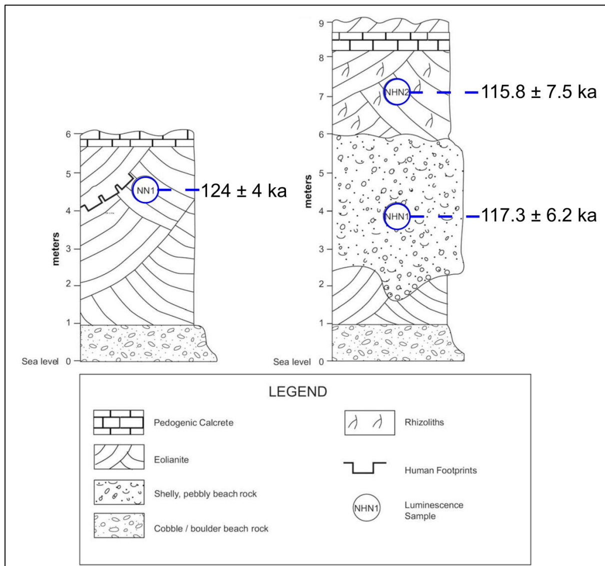
Figure 2.6. The sedimentary profiles from which dating samples were taken by Jacobs and Roberts (2009). The sample locations within the profiles and the ages determined for each sample are indicated. Left: the profile at the footprint site on Nahoon Point. Right: the East Beach profile. Note that in both cases the stratigraphic relationship with the underlying beachrock was inferred rather than observed.
