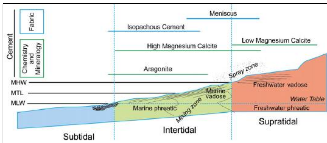
Figure 3.3. The distributions of different calcium carbonate cement types and their fabrics within the coastal zone (after Mauz et al. 2015).
