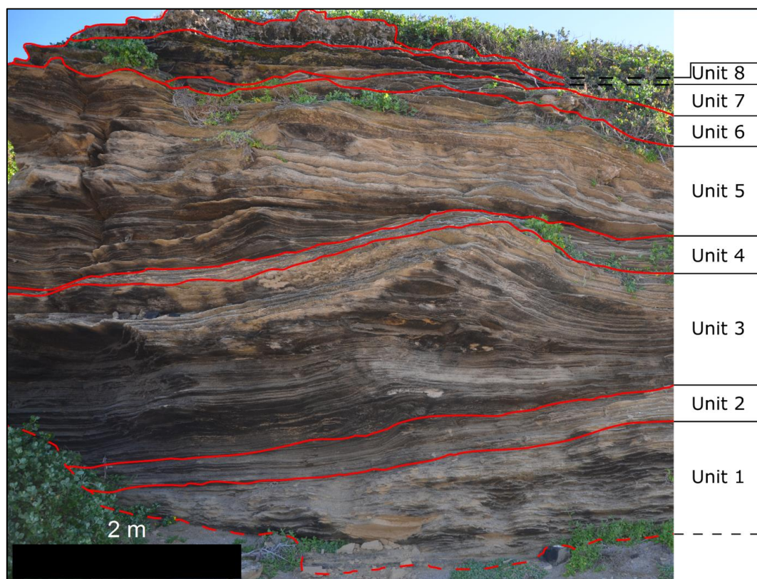
Figure 5.3. A photograph of Profile 1 with the units marked. Note that the dip is away from the camera.
