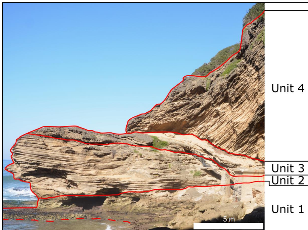
Figure 5.31. A photograph of Profile 14 with the units marked.
