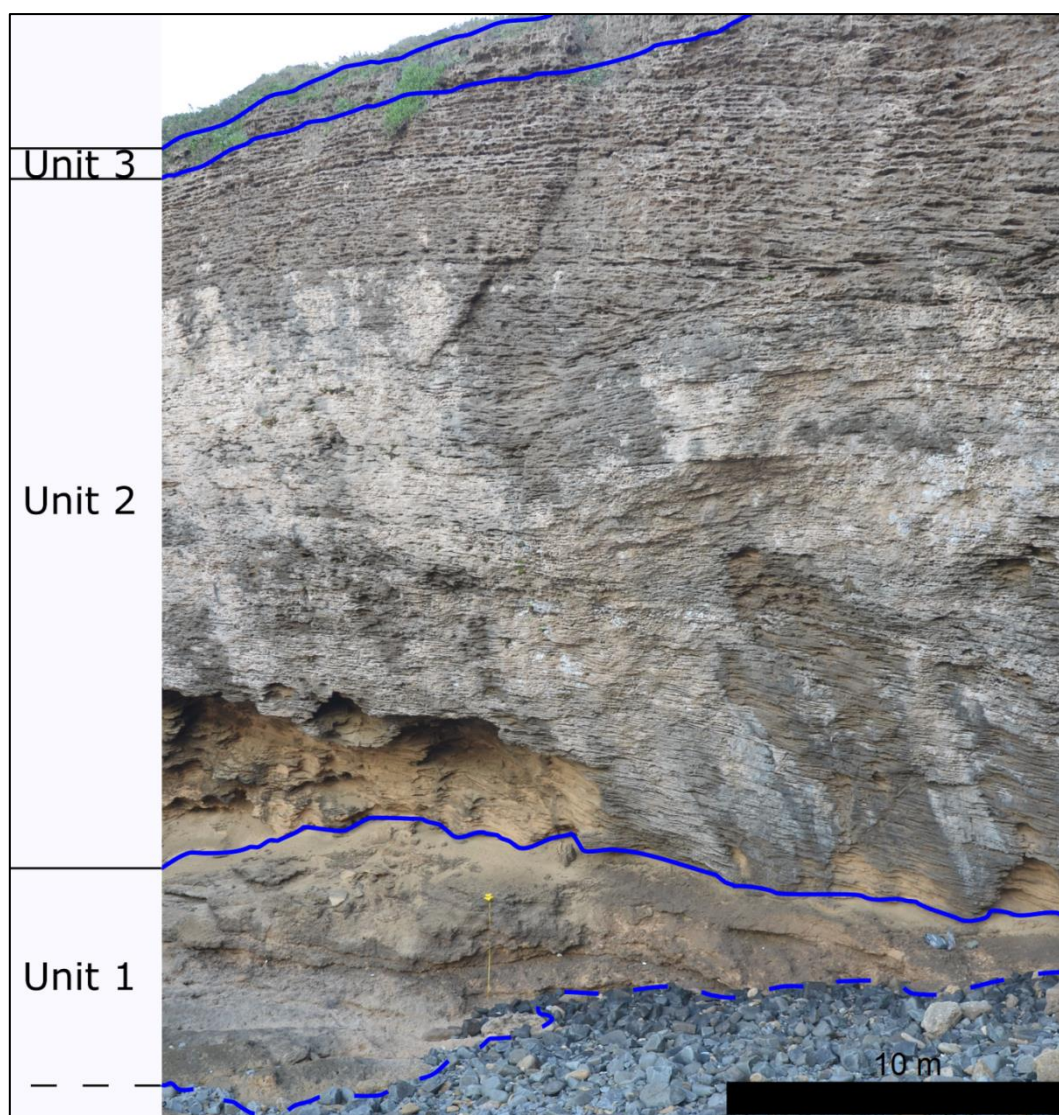
Figure 5.37. A photograph of Profile 17 with the units marked.
