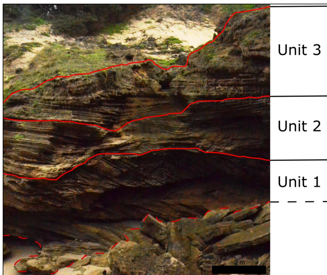
Figure 5.41. A photograph of Profile 19 with the units marked.
