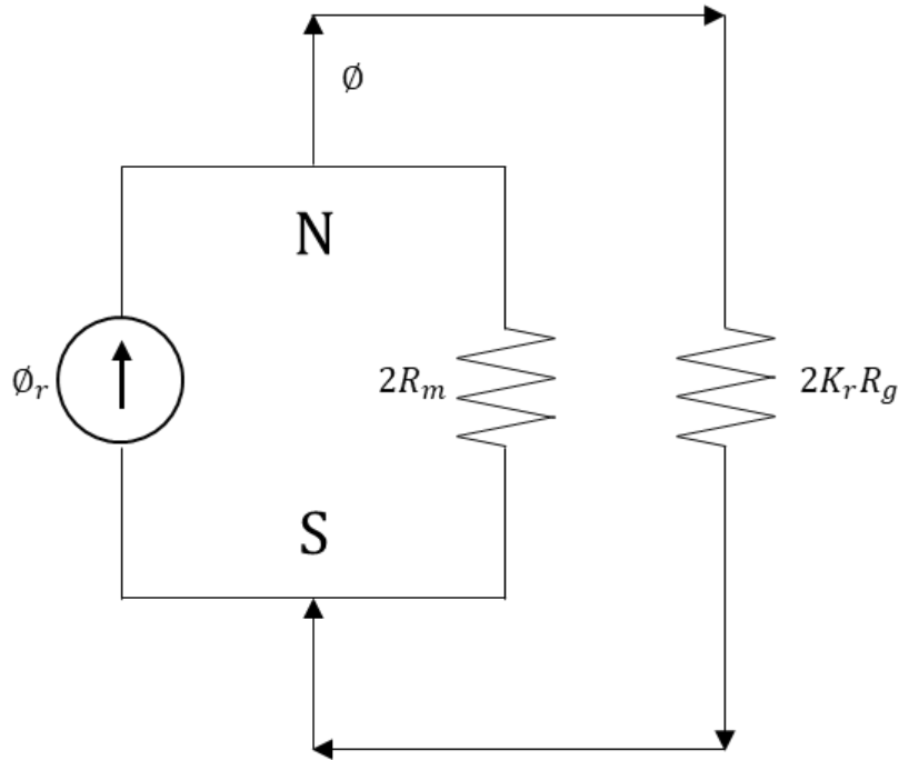
Figure 27: Simplified magnetic circuit for SPM motor analysis
