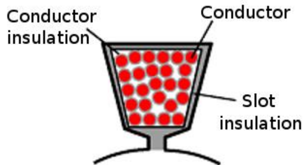
Figure 34: Stator slot winding fill factor [49]
