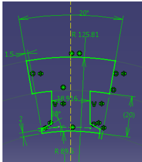
Figure 45: Stator template model: Tooth profile sketch (Sample dimensions)
