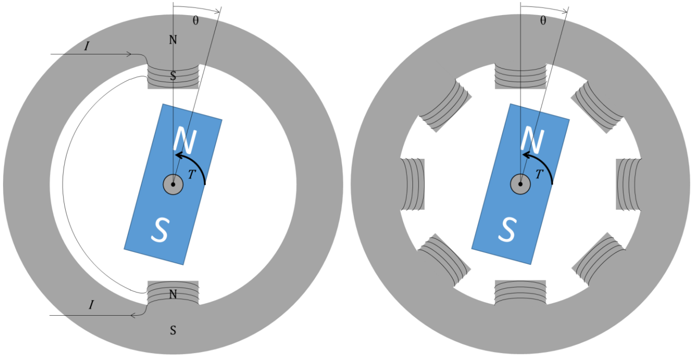
Figure 19: Current carrying conductor introduced to generate mutual/alignment torque component and extended multi-pole stator
