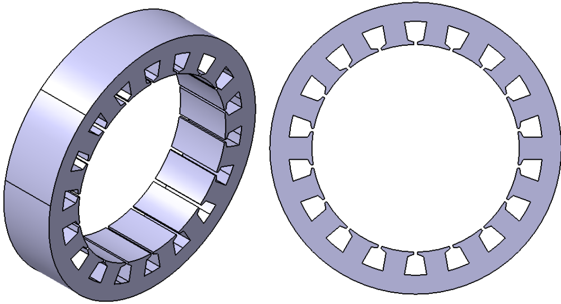
Figure 44: Stator template model
