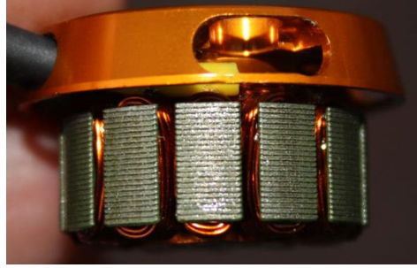
Figure 32: Small high-speed hobby motor stator assembly [40]
