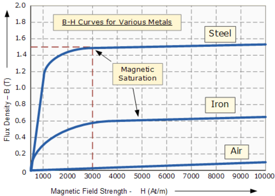
Figure 10: B-H Curves for common material groups indicating magnetic saturation points [23]
