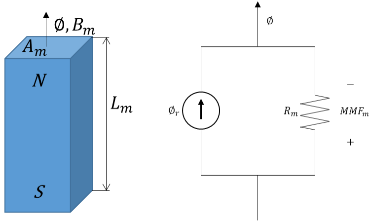
Figure 22: Magnetic circuit schematic for permanent magnet
