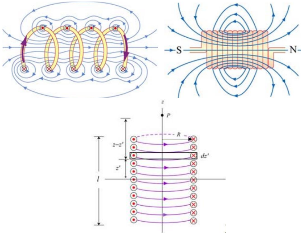
Figure 14: Magnetic field lines induced by current travelling through coil [26]
