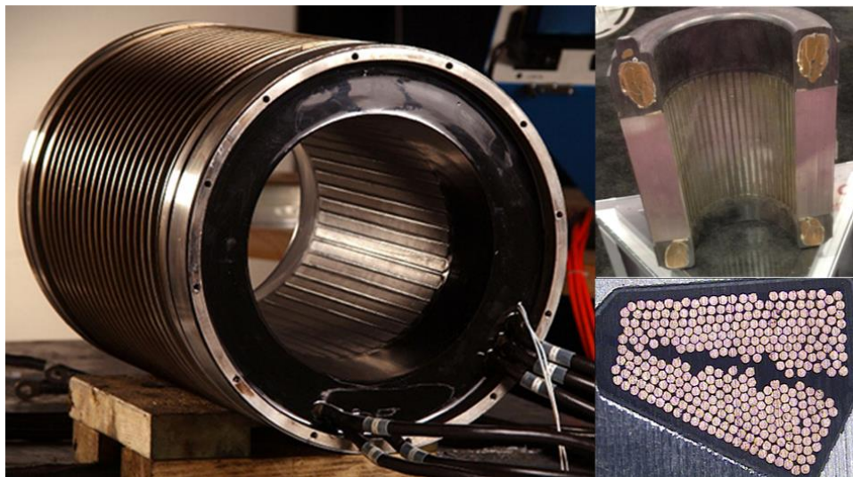
Figure 39: Examples of fully encapsulated stator assemblies including sectioned views [65] [66]
