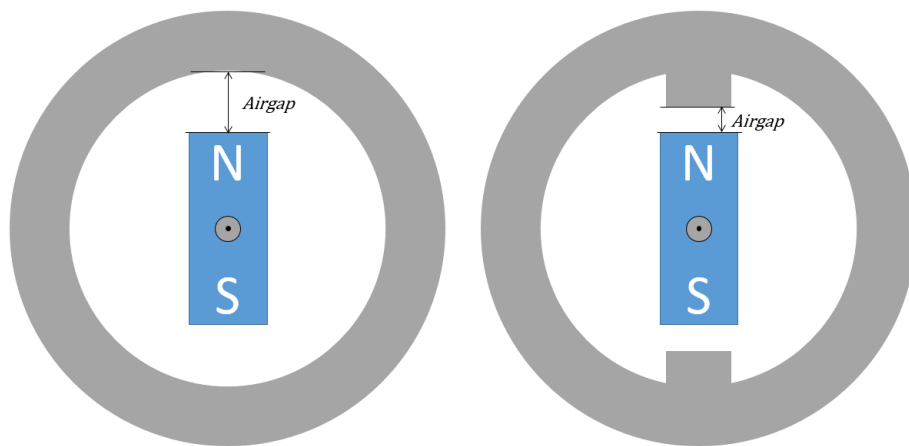
Figure 17: Magnet free to spin in simple ring and ring with two poles
