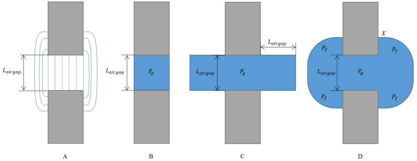
Figure 24: Airgap modelling schematics for magnetic circuit analysis
