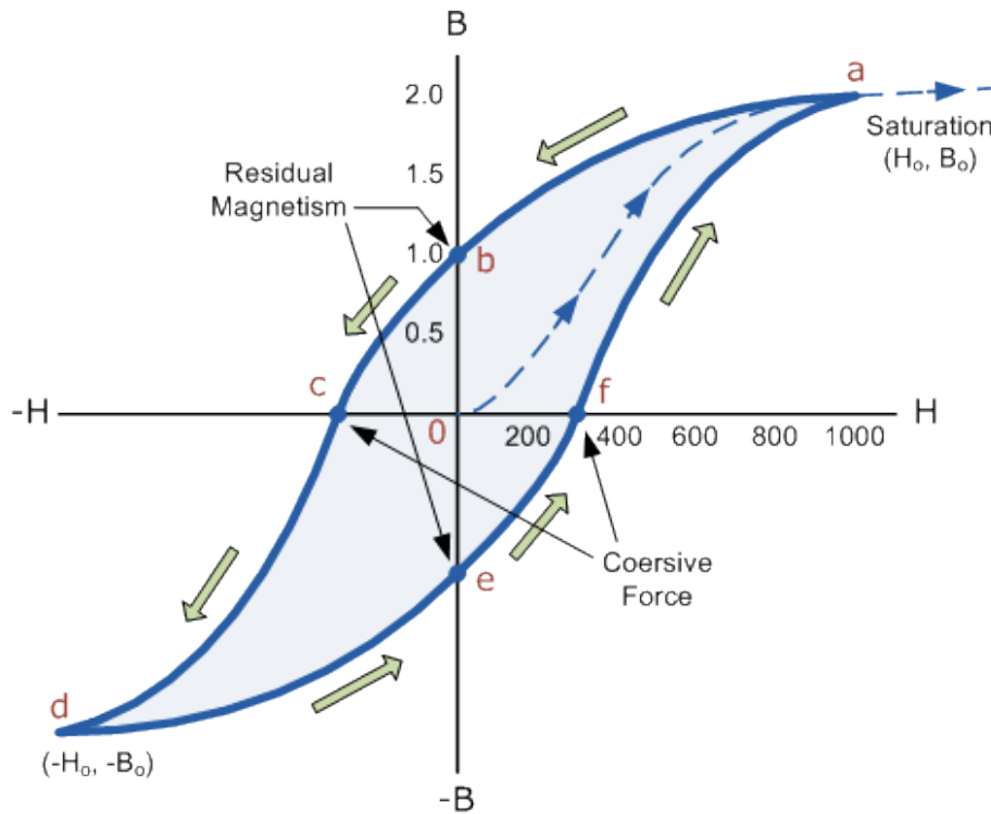
Figure 9: Sample magnetic hysteresis loop [23]
