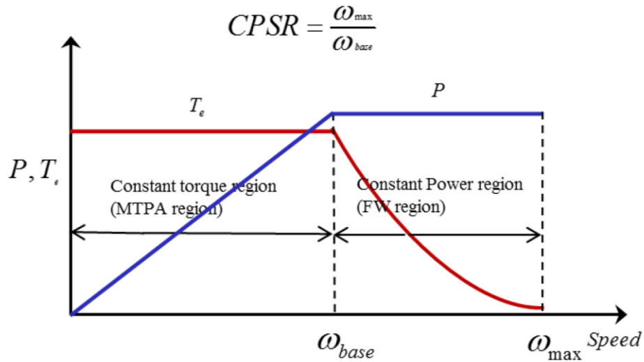
Figure 20: Typical SPM motor power and torque versus speed characteristics [32]
