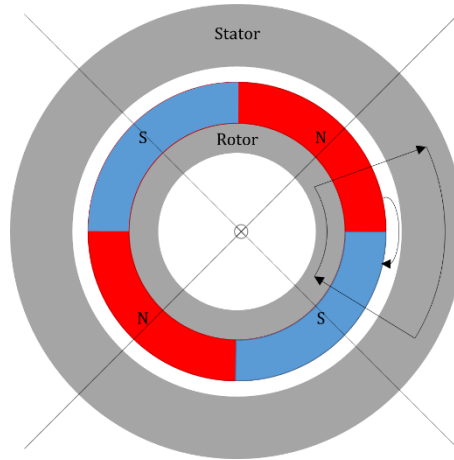
Figure 25: Simplified SPM motor for MCA analysis
