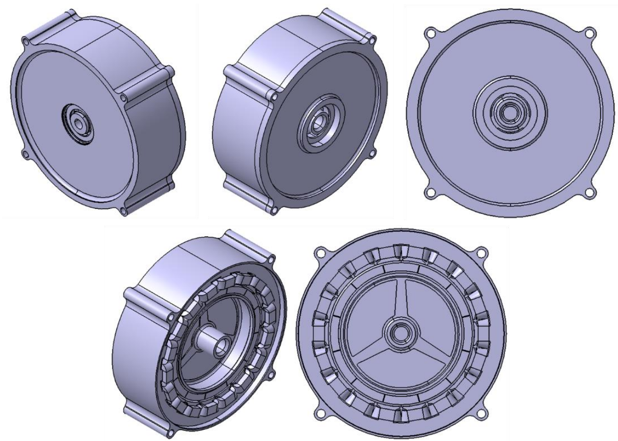
Figure 58: Full motor assembly template model (Sample parameters)
