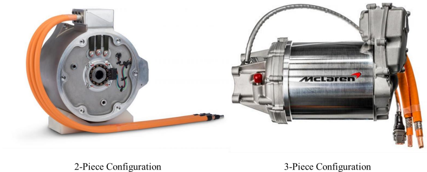
Figure 38: 2-Piece and 3-Piece motor housing configurations. [62] [63]
