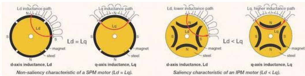
Figure 7: Inductance path comparison - Surface Permanent Magnet versus Interior Permanent Magnet [17]
