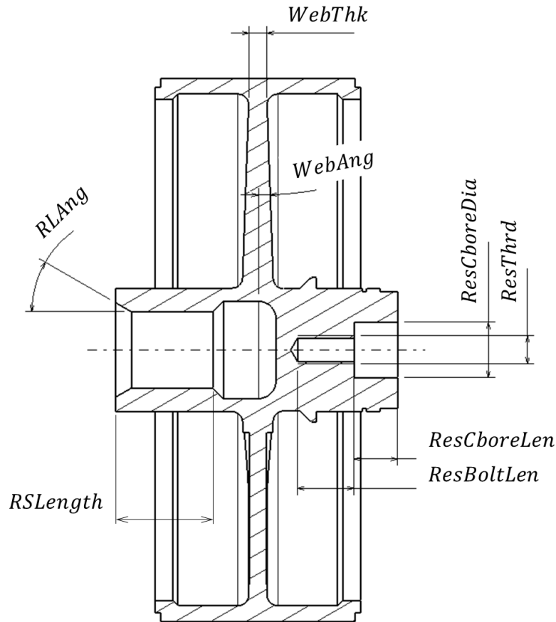
Figure 50: Rotor template model: Additional rotor detail dimensions
