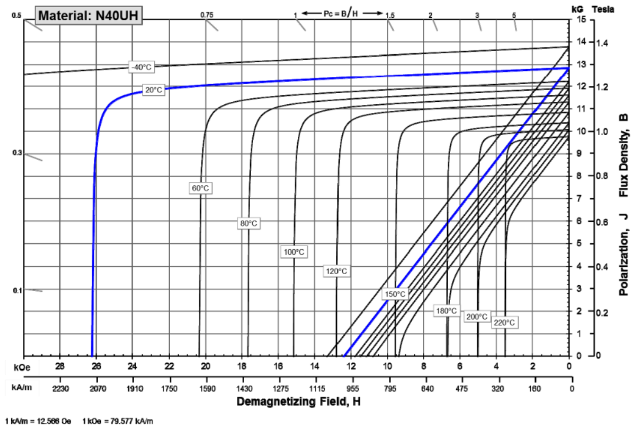
Figure 36: Sample demagnetisation curves at various temperatures for N40UH permanent magnet [24]
