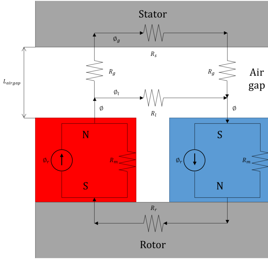
Figure 26: Magnetic circuit model for simplified SPM motor
