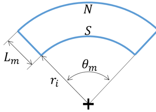
Figure 23: Radially magnetised arc-shaped permanent magnet
