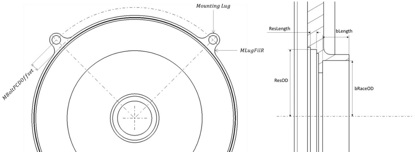
Figure 55: Housing template model: Additional housing detail dimensions
