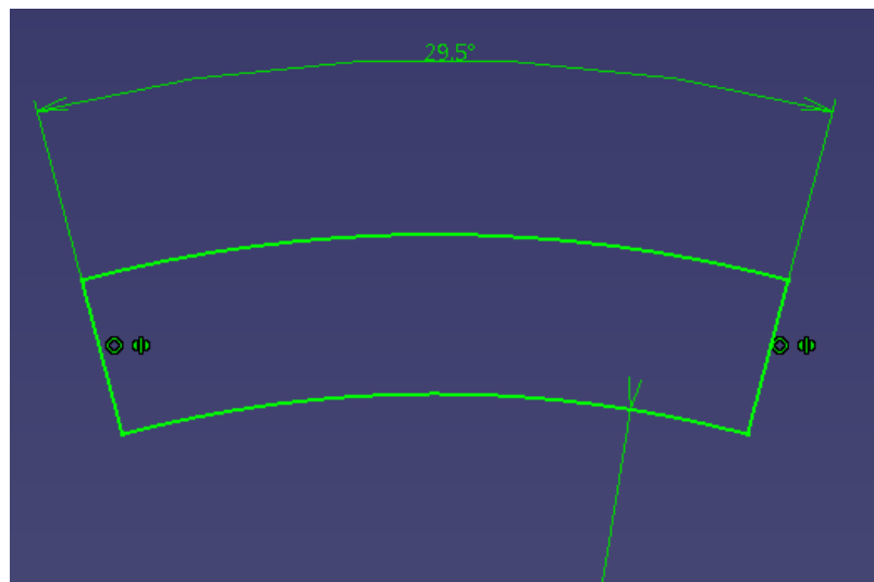
Figure 52: Permanent magnets representation template model: Magnet profile sketch
