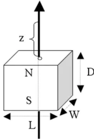
Figure 11: Magnetic field flux density at distance z along symmetrical axis of block magnet [27]
