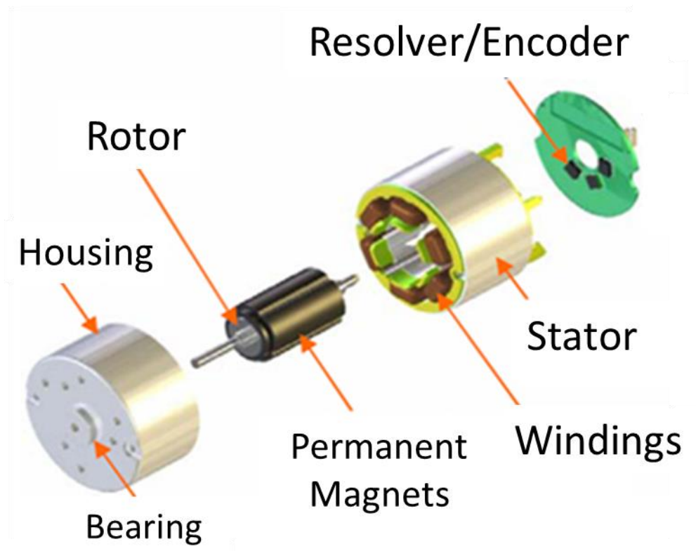
Figure 3: Typical Permanent Magnet Alternating Current (PMAC) Motor [11]
