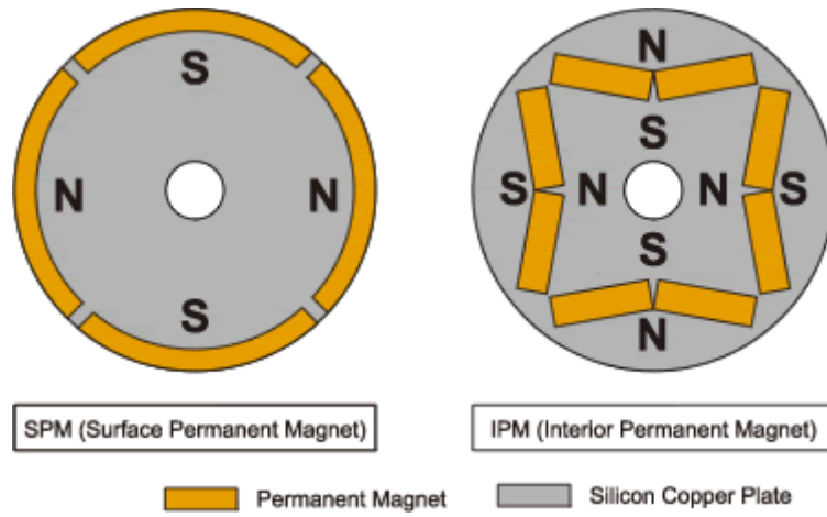
Figure 6: Surface Permanent Magnet motors versus Interior Permanent Magnet motors [15]
