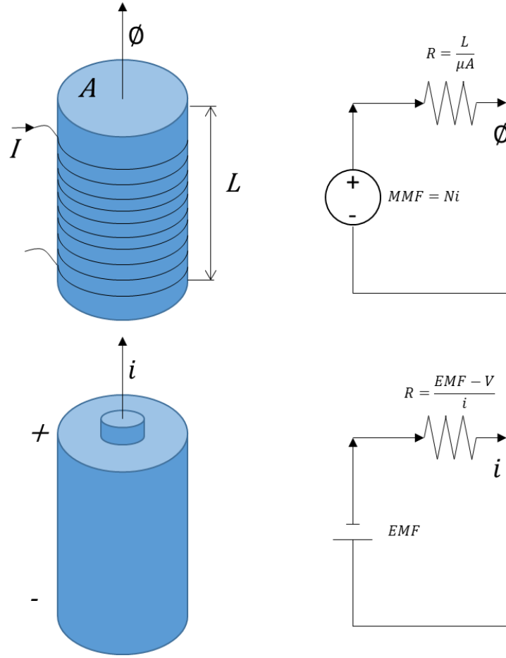
Figure 21: Comparison of magnetic circuit and electrical circuit schematics
