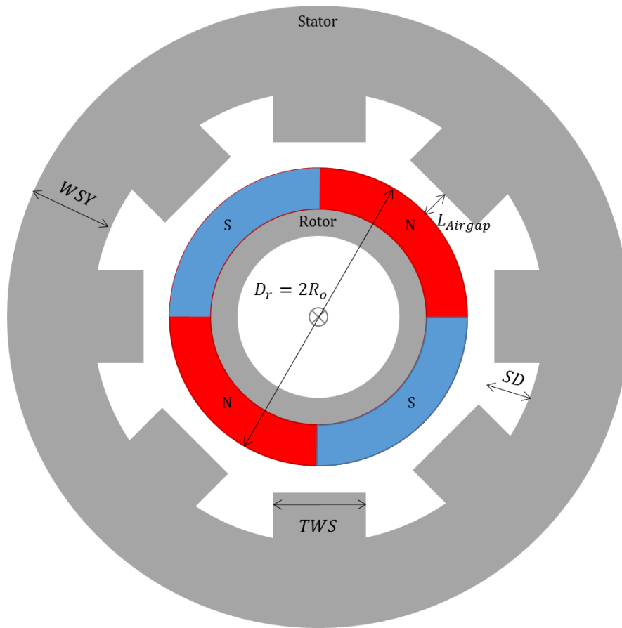
Figure 28: Full motor MCA analysis diagram
