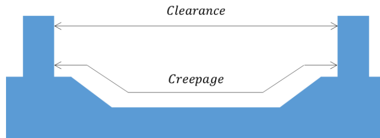
Figure 40: Creepage and clearance measurements across insulation barrier
