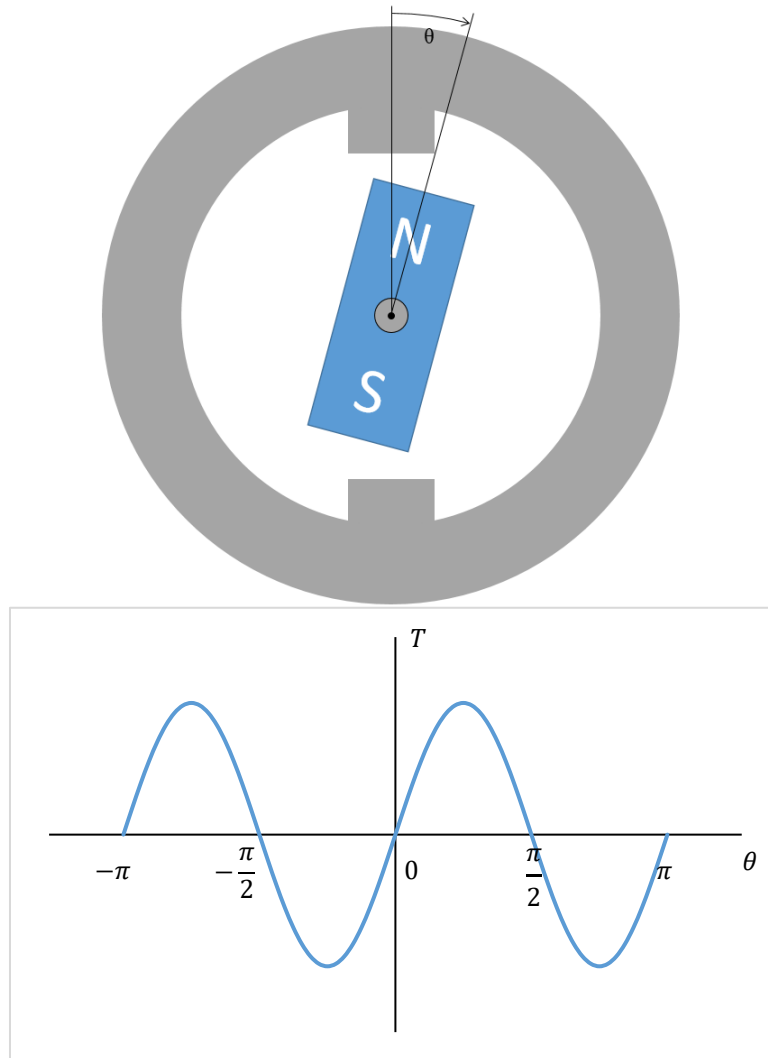
Figure 18: Torque variation with angular position experienced by magnet in two-pole ring [5]
