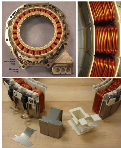
Figure 29: Honda Accord hybrid motor stator assembly [36]
