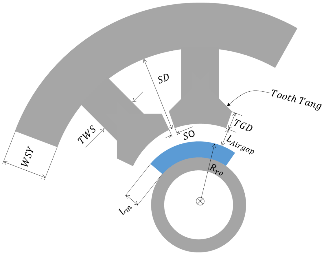
Figure 31: Stator tooth profile dimensions
