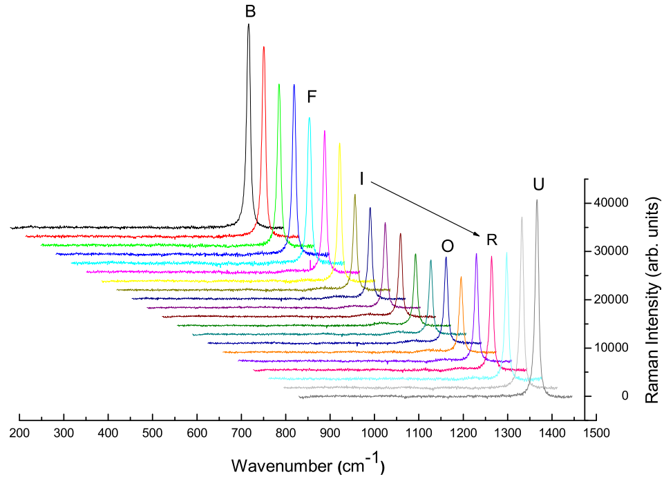
Figure 5.25: The \mu -Raman spectra measured at twenty different points in a single line along the irradiated sample's diameter for the sample that was implanted with 200 keV H^+ ions to fluences of 1.0 \times 10^{15} ions/cm 2 .
