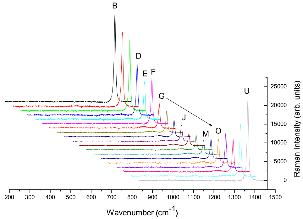
Figure 5.26: The \mu -Raman spectra measured at twenty different points in a single line along the irradiated sample's diameter for the sample that was implanted with 200 keV H^+ ions to fluences of 2.0 \times 10^{16} ions/cm 2 .
