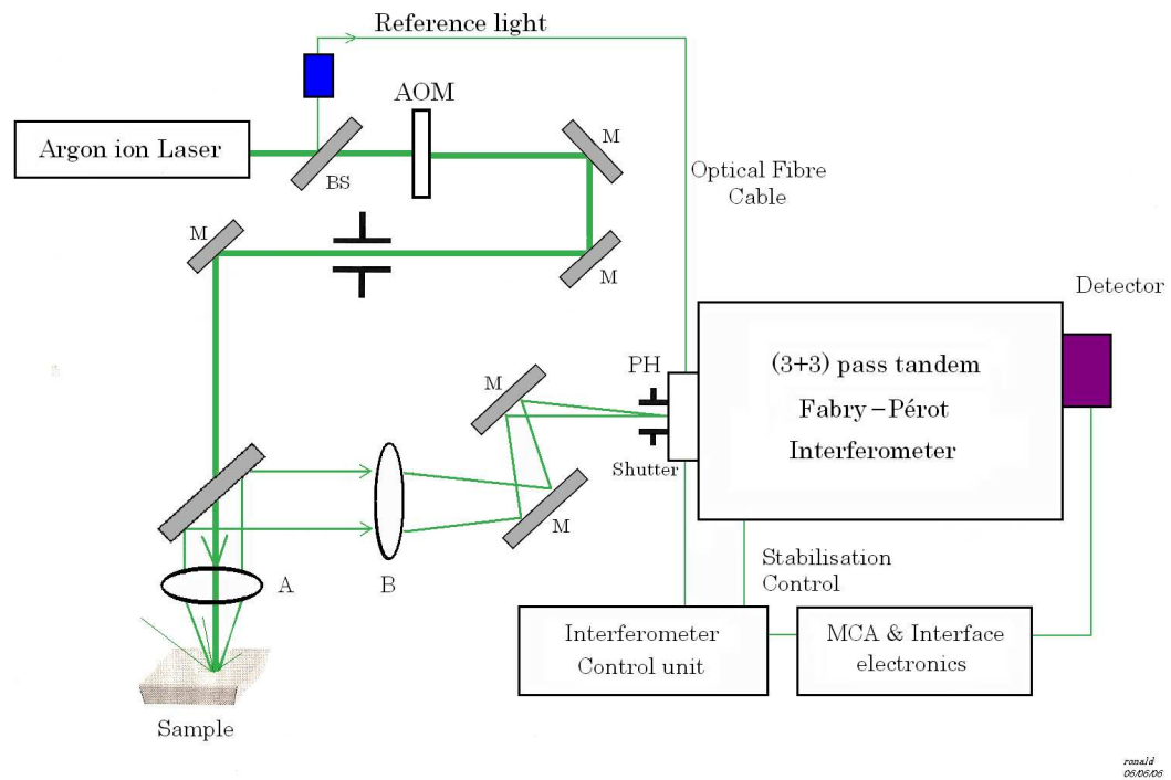
Figure 4.5: A schematic diagram of the SBS instrument used in a backscattering geometry. The beam splitter (BS) extracts a small portion of the incident laser light (Reference light) that is fed to the detector by means of an optical fibre cable. The mirrors (M) manipulate the light from one point to another, altering their configuration changes the scattering geometry. The Acoustic-Optic Modulator (AOM) is used to adjust the power of the laser light. The lenses (A & B) are used for scattered light collection and focusing. The shutter and pin-hole (PH) protect the detector. After [68,70].
