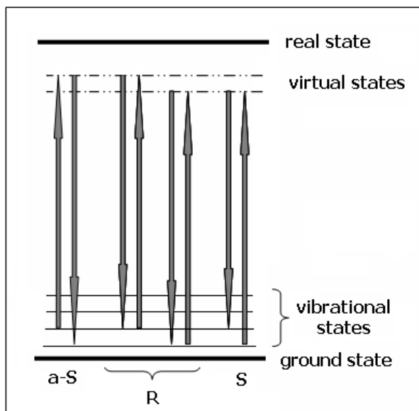
Figure A.1: An illustration of the Rayleigh (R), anti-Stokes (a-S) and Stokes (S) Raman scattering processes, each electronic has several vibrational states, in turn, each vibrational state has several rotational energy states (not shown here).
