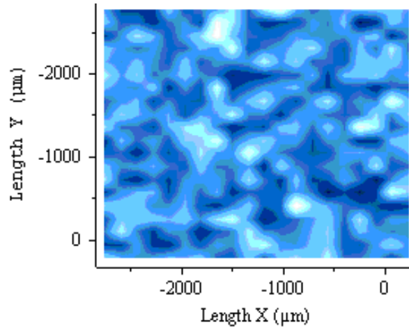
Figure 5.8: The 2D-Raman width map showing the broadening of the 1365.4\text{cm}^{-1} Raman peak measured across the unimplanted hBN sample surface.
