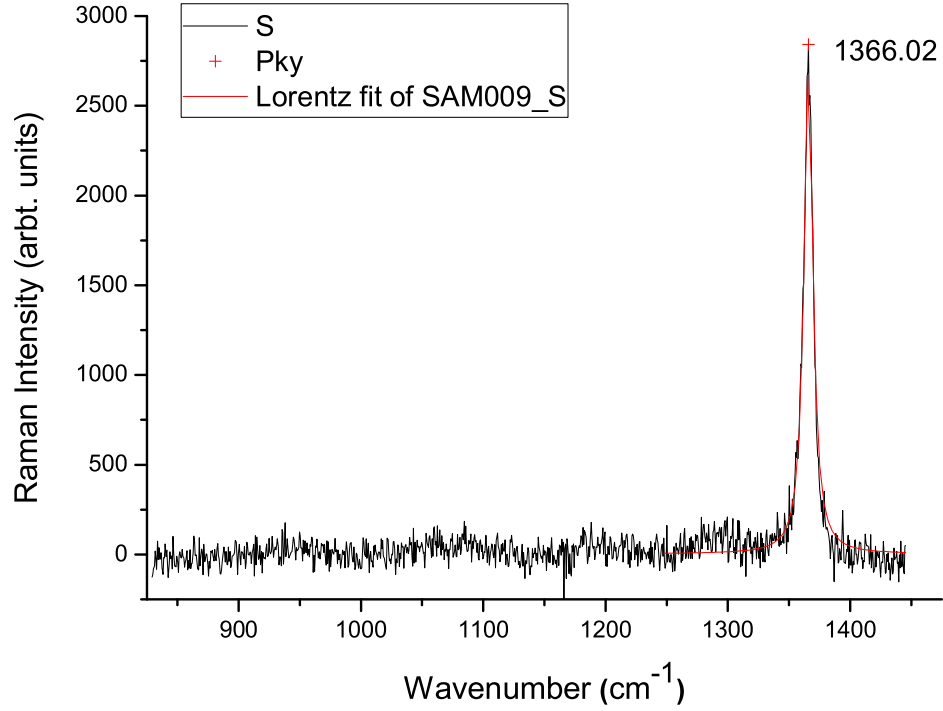
Figure 5.23: The measured \mu -Raman spectrum of the hBN sample that was implanted at 200 keV with 1.0 \times 10^{15} \text{ He}^+ ions/cm 2 .
