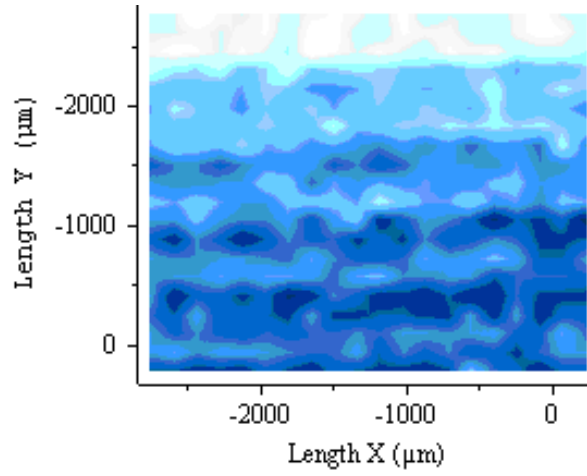
Figure 5.7: The 2D-Raman position map showing the relative positions of the Raman peaks measured across the unimplanted hBN sample surface.
