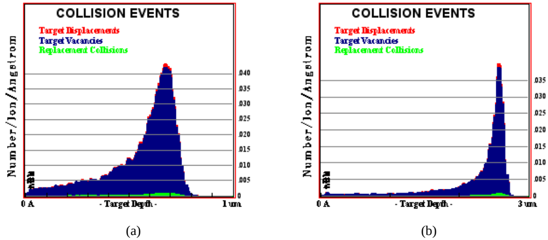
Figure 5.2: Collision details/damage profiles predicted for \text{He}^+ implanted into hBN at: [a] 200 keV, and [b] 1.2 MeV.
