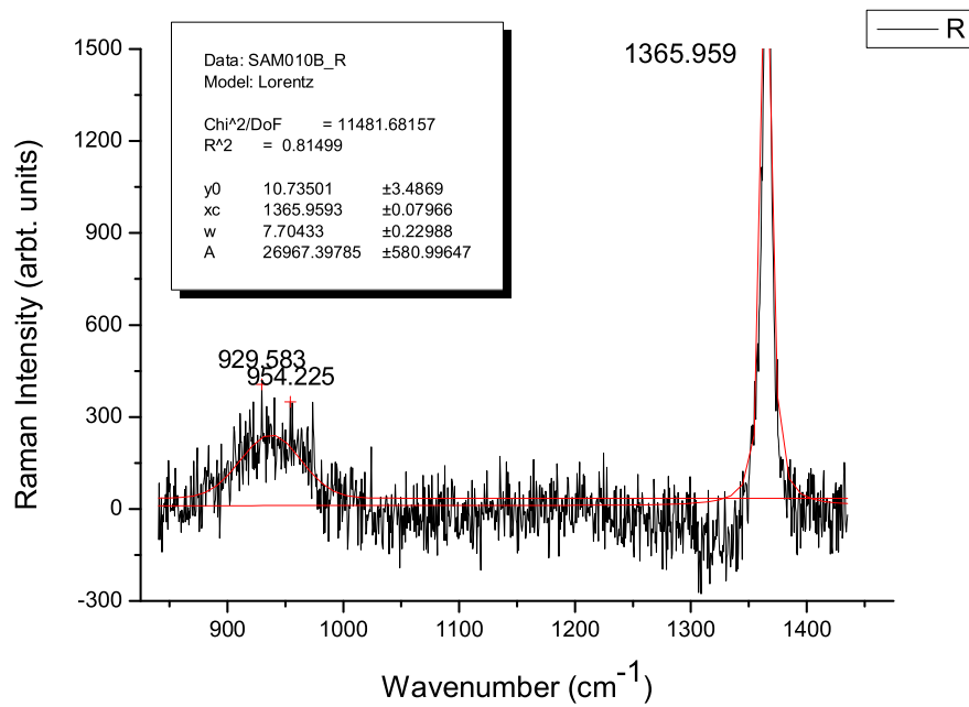
Figure 5.21: The \mu -Raman spectrum measured inside the irradiated region of the hBN sample that was implanted with 350 keV \text{He}^+ ions to a fluence of 1.0 \times 10^{15} \text{ ions/cm}^2 . The red line is a Lorentzian fit.
