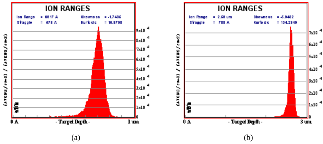
Figure 5.1: Ion range distribution profiled predicted for \text{He}^+ implanted into hBN at: [a] 200 keV, and [b] 1.2 MeV.
