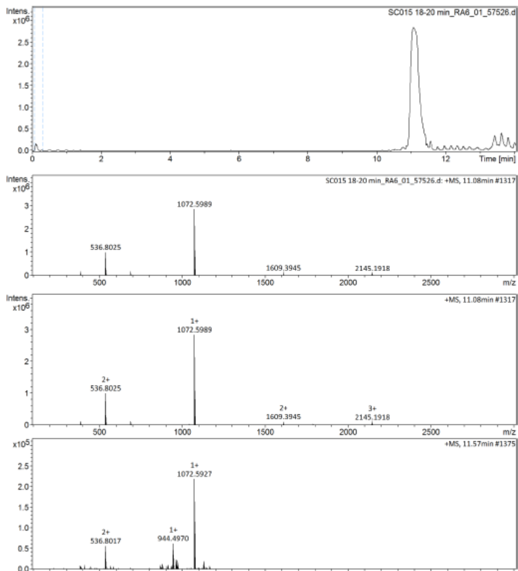
Figure A. 19: LCMS results of cyclized and purified SC016.
