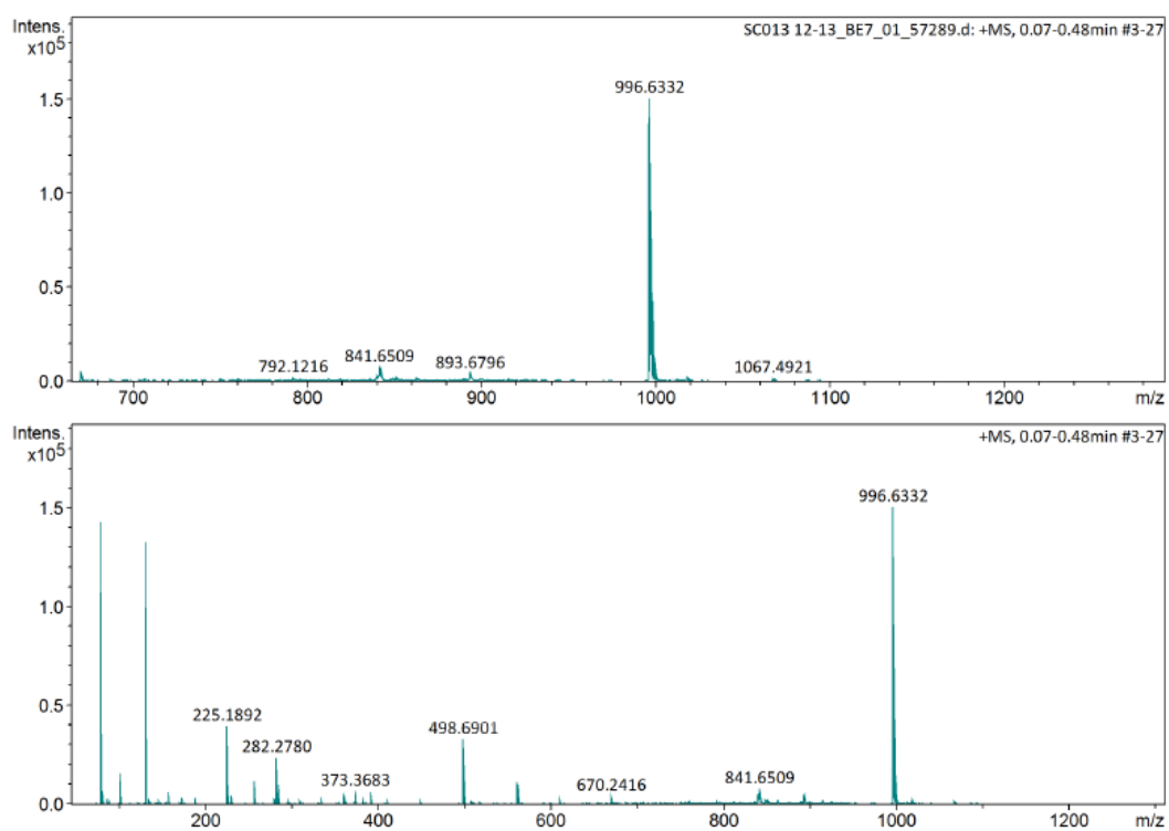
Figure A. 16: MS results of linear SC013.
