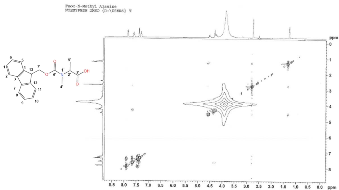
Figure A. 32: NOESYPSW spectrum of Fmoc-N-Methyl Alanine in DMSO- d_6 .
