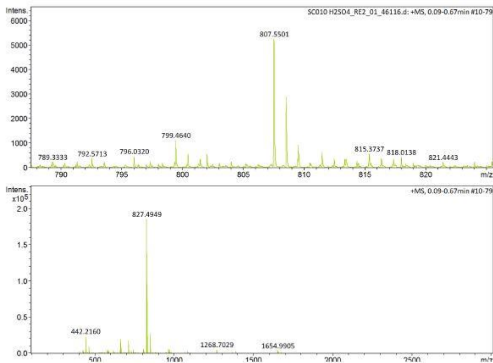
Figure A. 11: Results of SC010 treated with 1% H 2 SO 4 obtained from MS.
