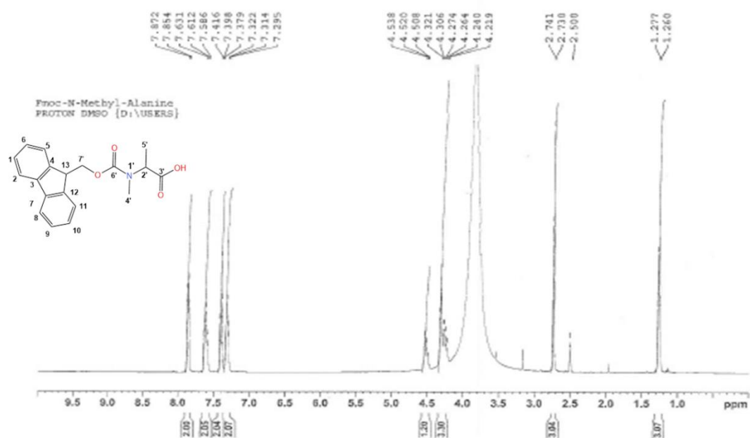
Figure A. 27: 1 H NMR spectrum of Fmoc-N-Methyl Alanine in DMSO- d 6 .
