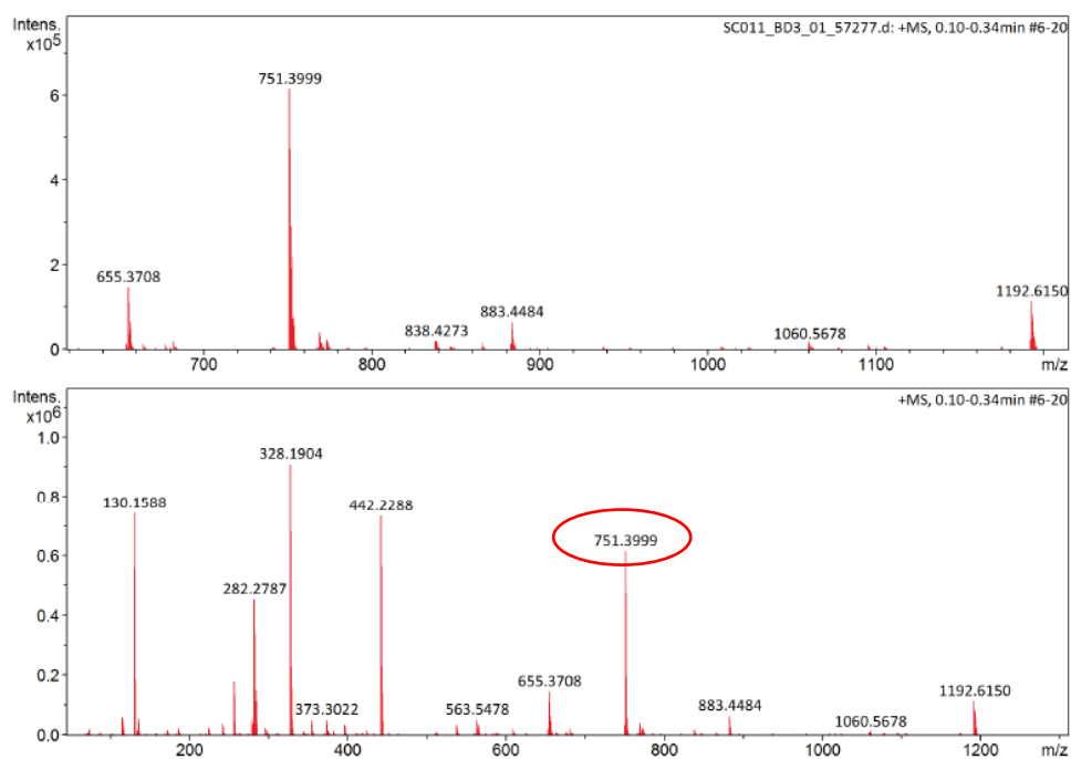
Figure A. 4: Results of linear SC011 obtained from MS.
