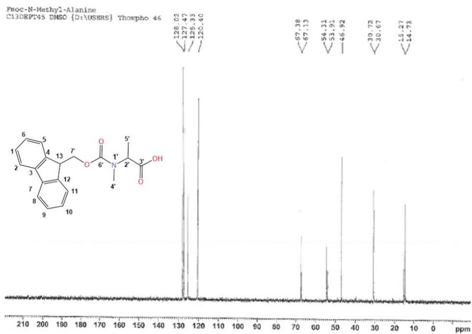
Figure A. 29: DEPT45 spectrum of Fmoc-N-Methyl Alanine in DMSO- d_6 .
