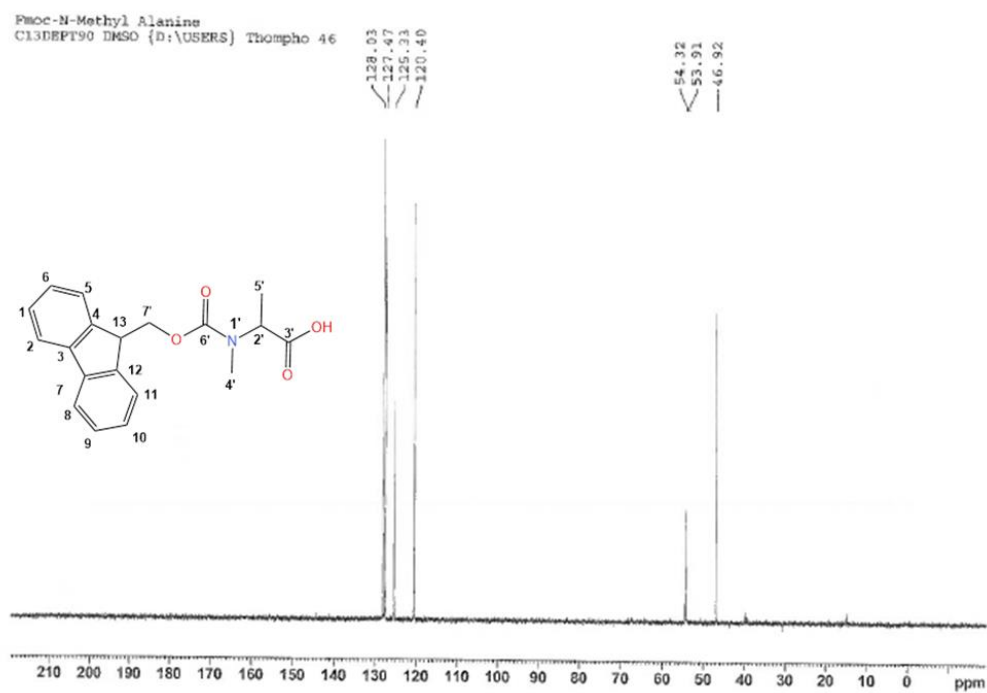
Figure A. 30: DEPT90 spectrum of Fmoc-N-Methyl Alanine in DMSO- d_6 .
