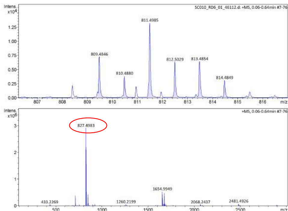
Figure A. 3: Results of linear SC0010 obtained from MS.
