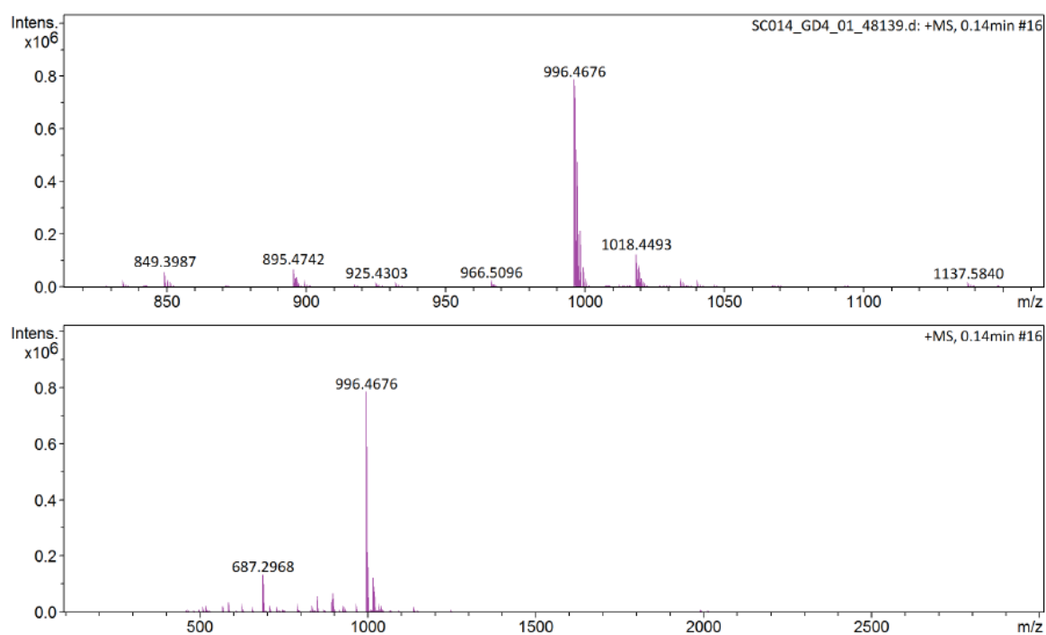
Figure A. 17: MS results of linear SC014.
