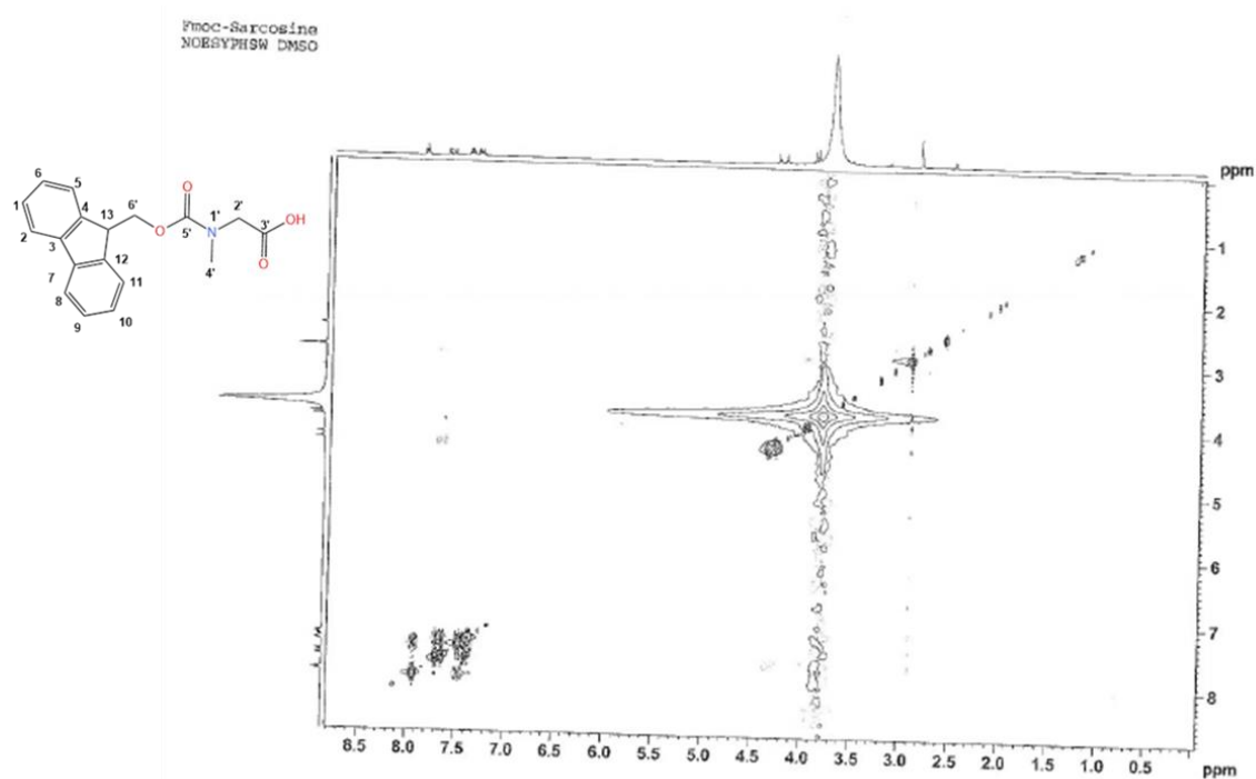
Figure A. 38: NOESYPSW spectrum of Fmoc-Sarcosine in DMSO- d_6 .
