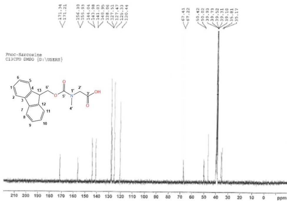
Figure A. 34: ^{13}\text{C} NMR spectrum of Fmoc-Sarcosine in \text{DMSO-}d_6 .
