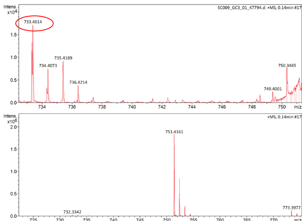
Figure A. 7: Results of SC009 treated with 95% TFA obtained from MS.
