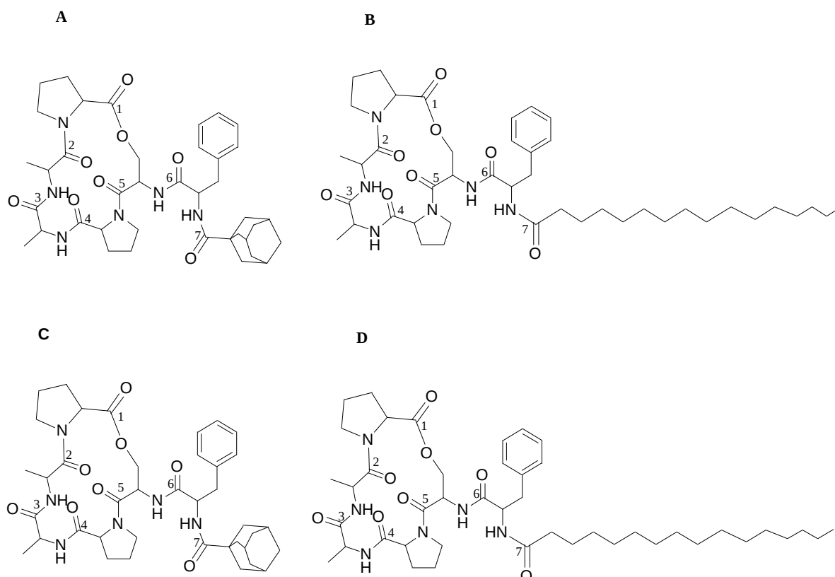
Figure 3. 3: ADEP1 ester cyclised analogues. A-SC009; B-SC010; C-SC011; D-SC012. Structure stereochemistry details in Table 3.2.
