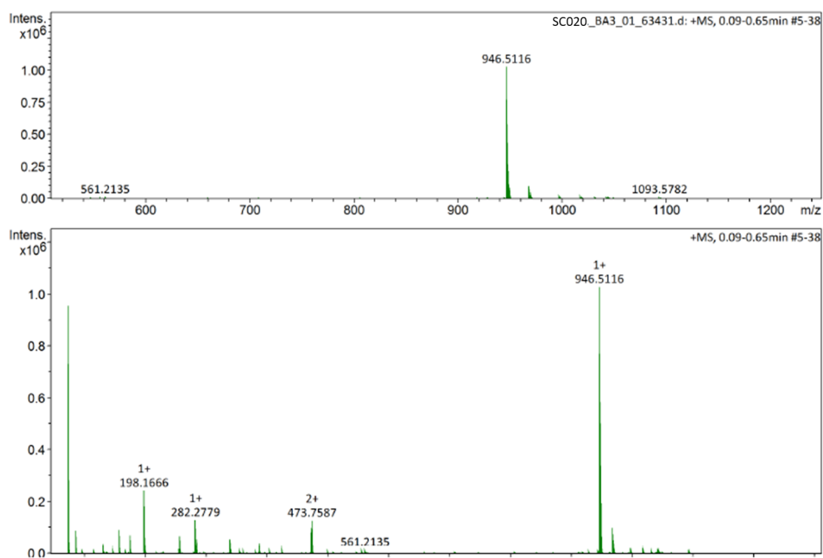
Figure A. 23: Linear SC020.
