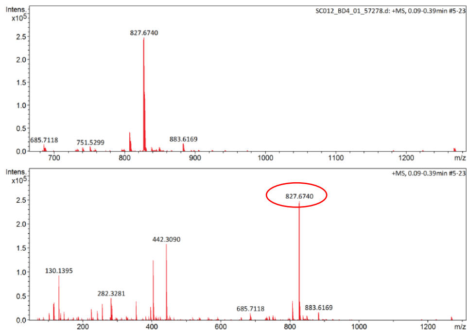
Figure A. 5: Results of linear SC0012 obtained from MS.
