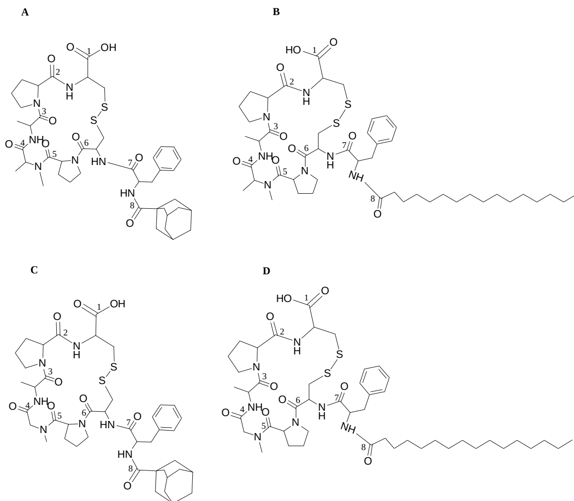
Figure 3. 9: Schematic Figure 9: Disulphide bond cyclised ADEP1 analogues with peptoid moieties. A-SC017; B-SC018; C-SC019, D-SC020. Structure stereochemistry details in Table 3.5.
