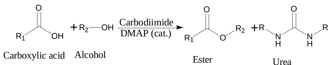
Figure 3. 5: Schematic representation of Steglich esterification.
