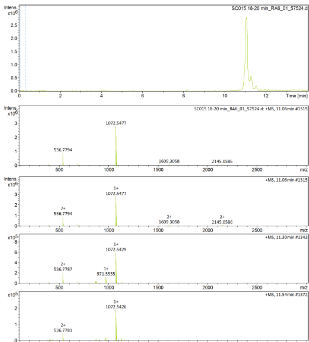
Figure A. 18: LCMS results of cyclized and purified SC016.
