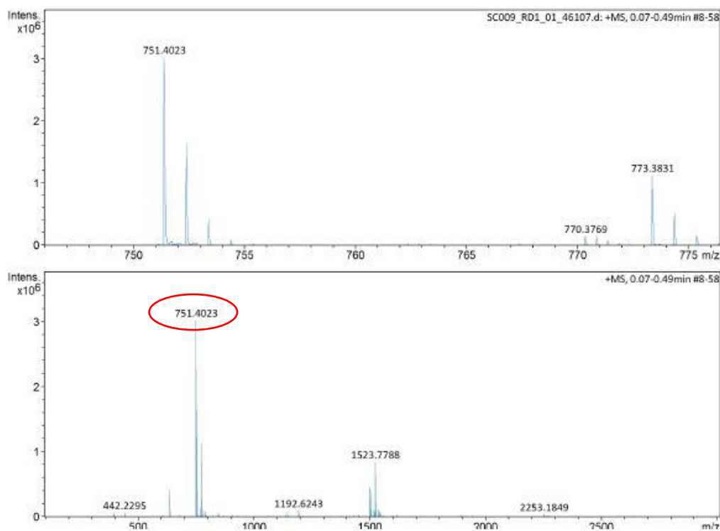
Figure A. 2: Results of linear SC009 obtained from MS.
