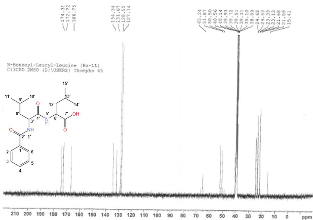
Figure A. 40: ^{13}\text{C} NMR spectrum of Bz-LL in \text{DMSO}-d_6 .
