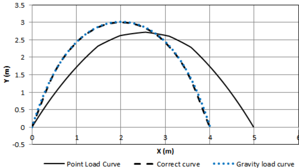
Figure 3.55: Optimised catenary geometry for externally draped post-tensioned tendon, supported at five pertinent positions, and exerting a 5kN point load.
