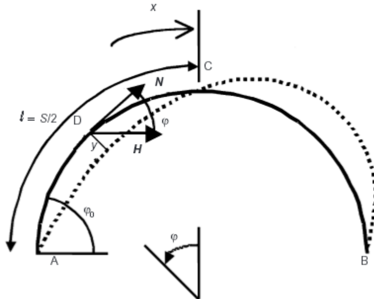
Figure 2.19: Buckling of a catenary arch under self-weight (Pedreschi & Theodossopoulos, 2007)
