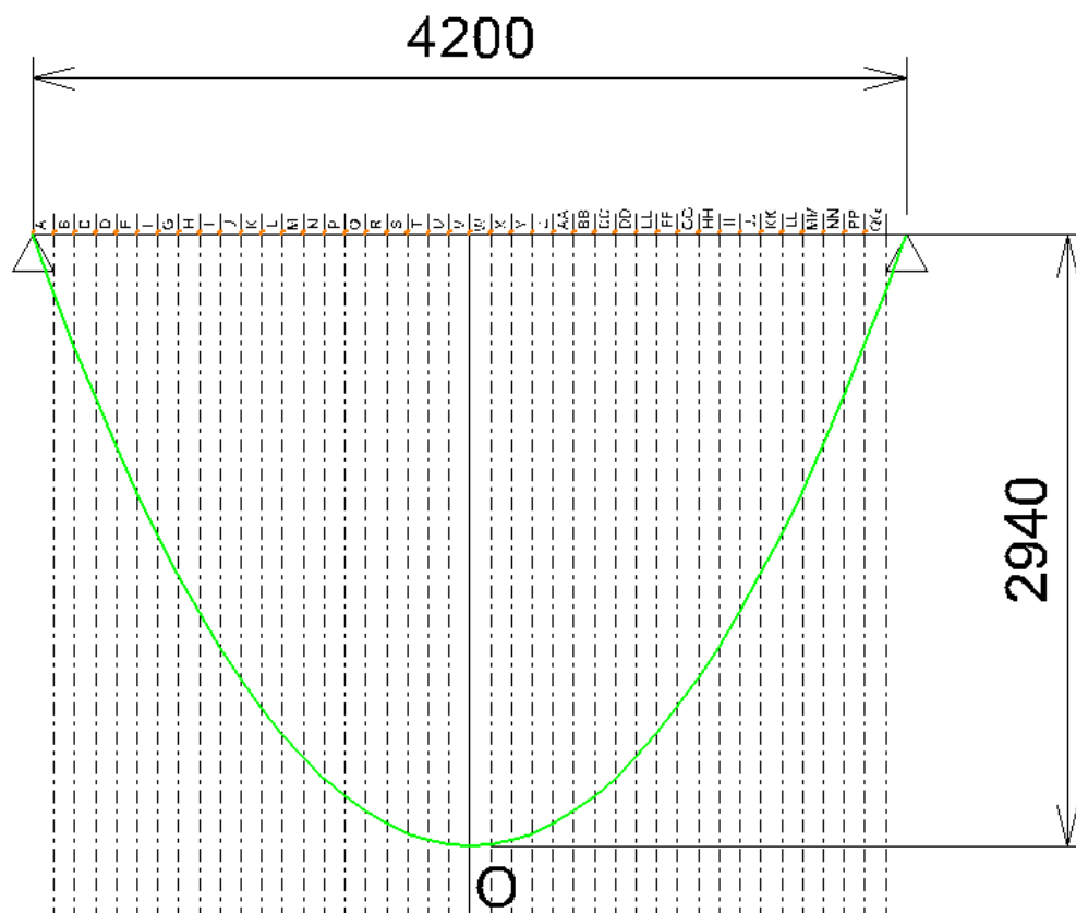
Figure 5.11: Funicular profile for cable tensioning at transfer.
