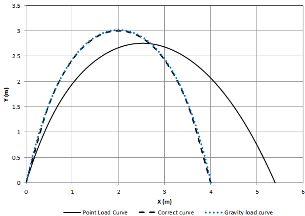
Figure 3.37: FLPC for steep vault of 1000mm thickness subjected to gravity and wind loads (LC1) as per Table 12.
