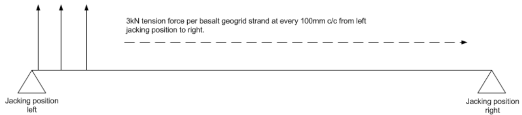
Figure 5.8: Schematic illustration of basalt geogrid mesh's force application under post-tensioning.
