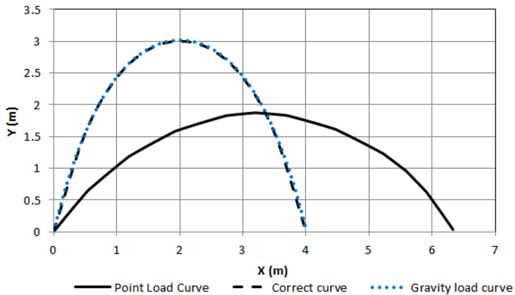
Figure 3.45: Optimised catenary geometry for externally draped post-tensioned tendon, supported along the vault's arch, and exerting a 10kN point loads along vault surface.
