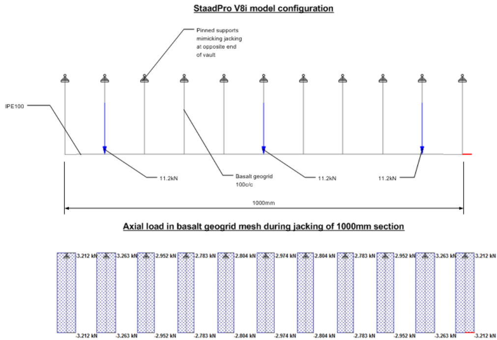
Figure 5.4: Six ratchet post-tensioning jack configuration.
