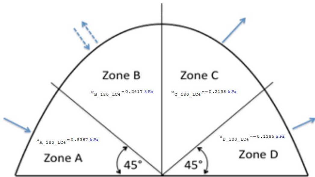
Figure 3.10: Resultant pressure force on steep vault for normal wind speeds - load case 4 (Bradley et al. , 2016).
