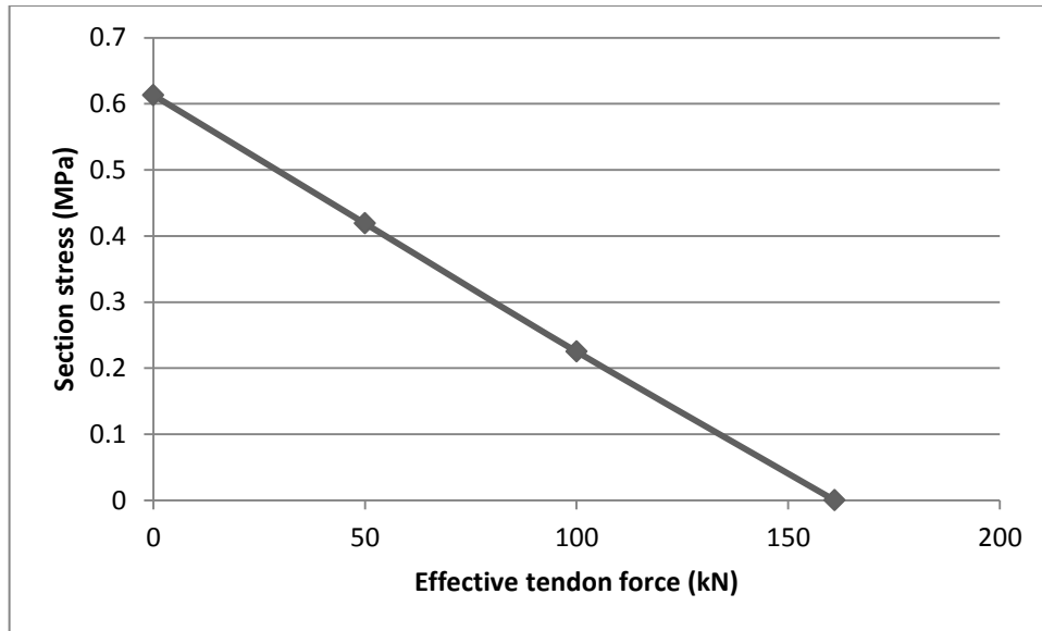
Figure 3.60: Graphical representation of stress reduction vs tendon force increase for data as per Table 17.
