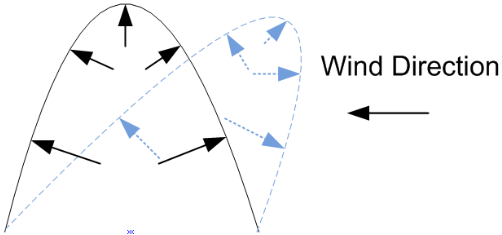
Figure 3.20: Convergence of the funicular curve based on normal pressure load assignments to the curve.
