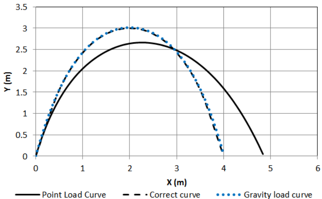
Figure 3.27: FLPC for steep vault of 250mm thickness subjected to gravity and wind loads (LC3) as per Table 11.
