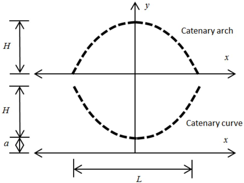
Figure 2.5: Catenary arch for uniform load (Gohnert & Bradley, 2016).
