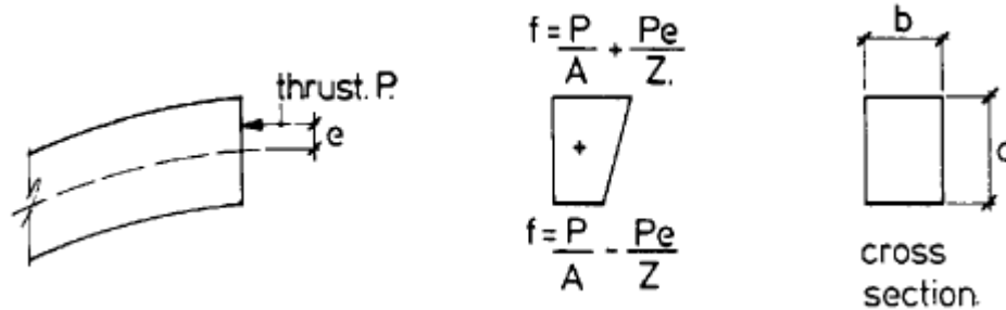
Figure 2.11: Stress condition in section of arch (Curtin et al. , 1995).
