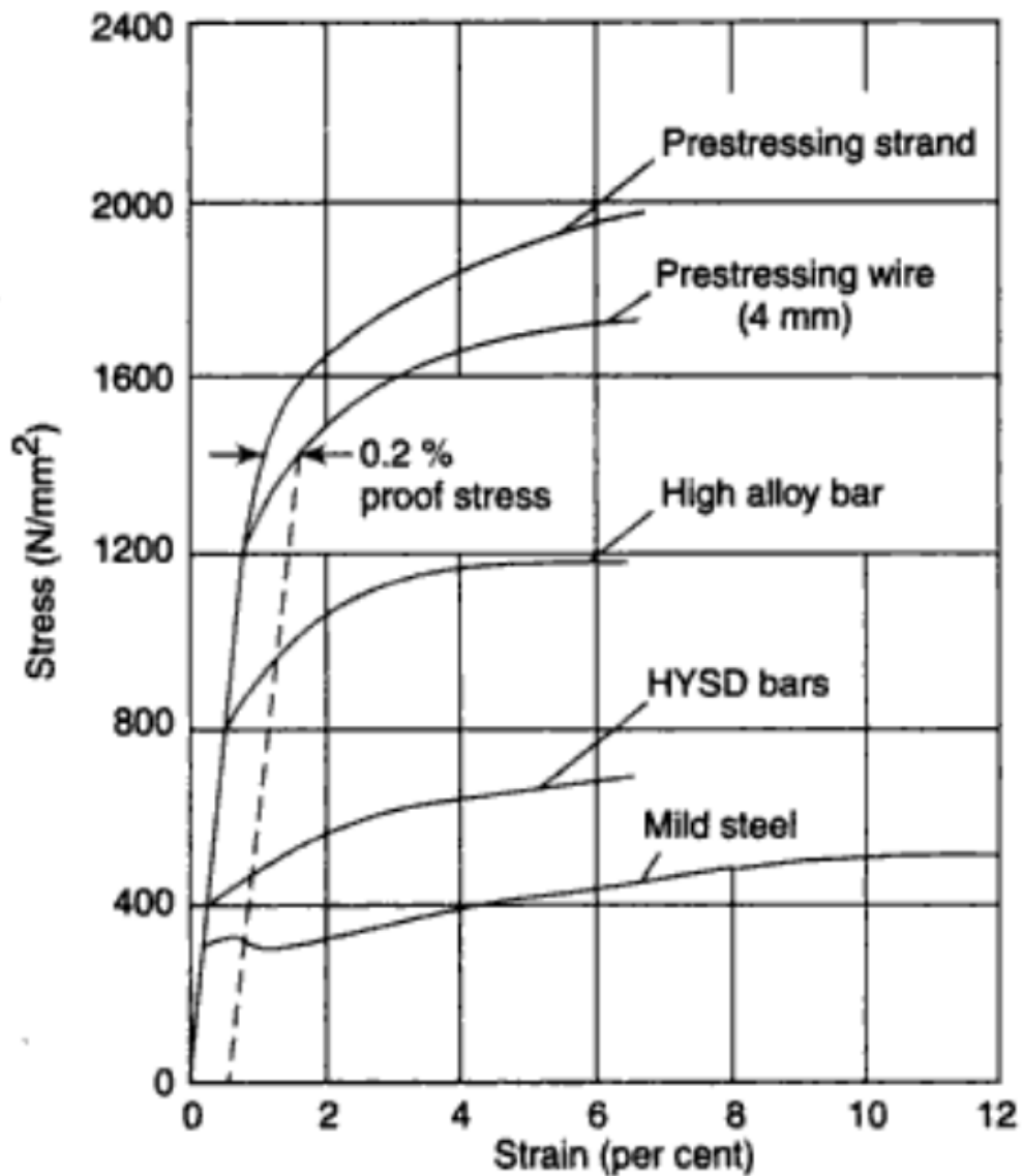
Figure 2.59: Stress-strain curves for reinforcing and pre-stress steel (Raju, 2007).
