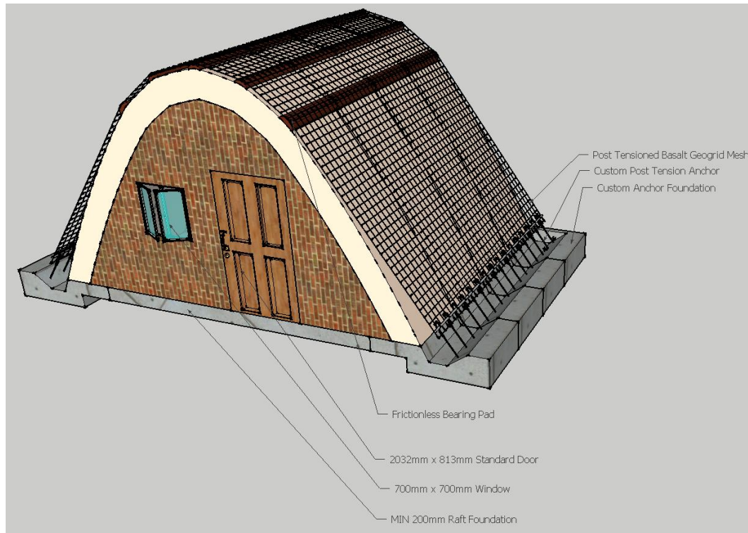
Figure 5.1: Basic components of the final solution in isometric view.
