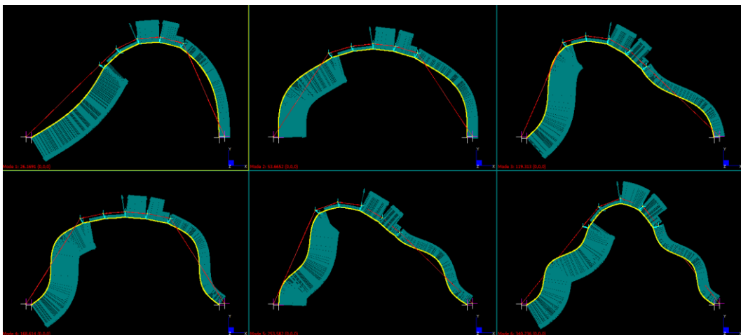
Figure 3.72: Buckling mode shapes for LC6 as per Table 12 for vault post-tensioned to pure compression for service loads (Strand7).
