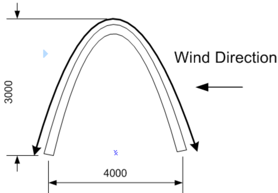
Figure 3.4: Optimised catenary vault - post-tensioned by externally placed tendon.
