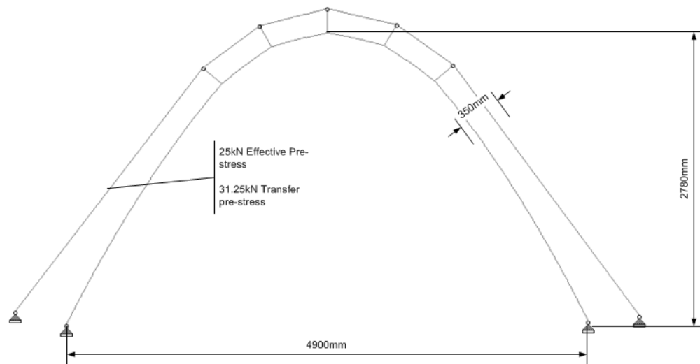
Figure 6.1: Final vault geometry
