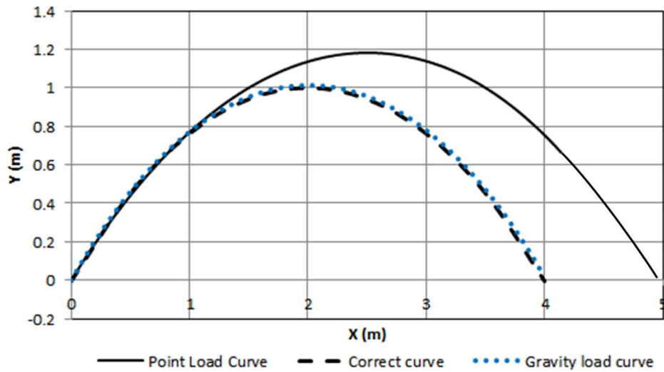
Figure 3.22: FLPC for elevated flat vault of 1000mm thickness subjected to gravity and wind loads as per Table 10 (LC1).
