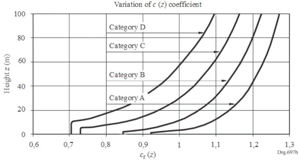
Figure 2.31: Variation of the roughness factor with height above ground level (SABS, 2011).
