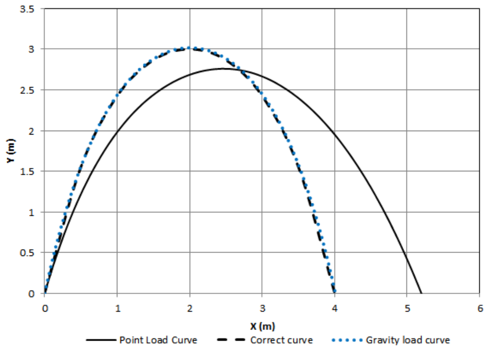
Figure 3.26: FLPC for steep vault of 250mm thickness subjected to gravity and wind loads (LC2) as per Table 11.
