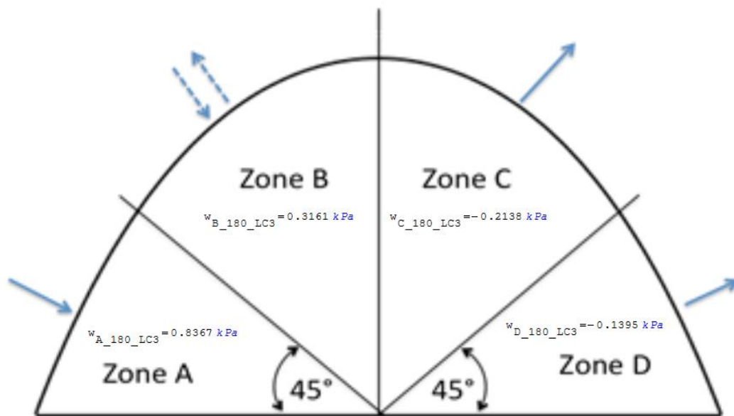
Figure 3.9: Resultant pressure force on steep vault for normal wind speeds - load case 3 (Bradley et al. , 2016).
