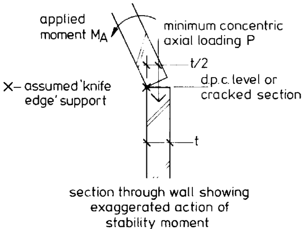
Figure 2.45: Exaggerated action of stability moment (Curtin et al. , 1995).
