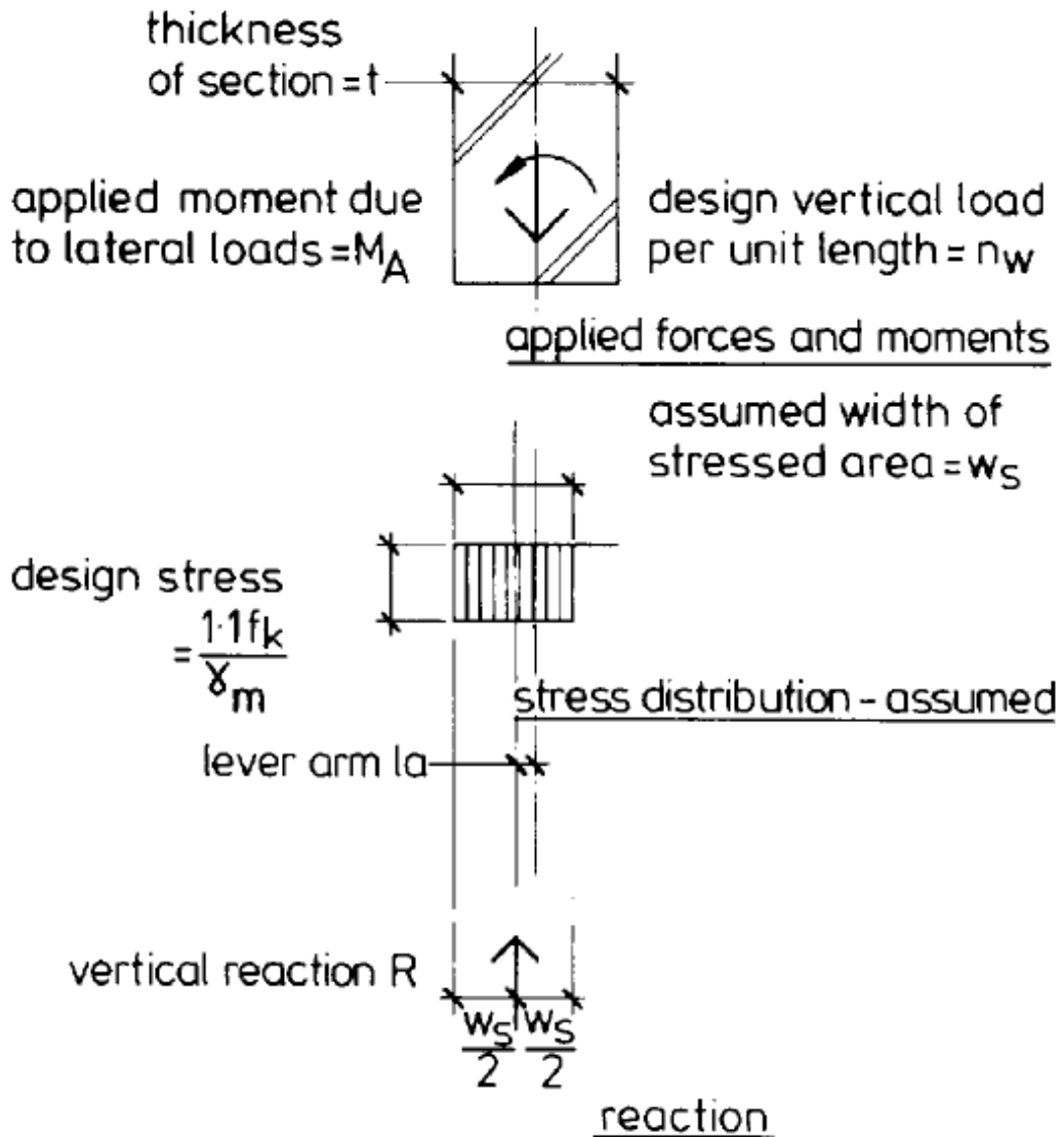
Figure 2.46: Assumed moment equilibrium in cracked masonry section (Curtin et al. , 1995)
