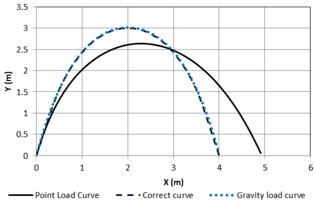
Figure 3.40: FLPC for steep vault of 1000mm thickness subjected to gravity and wind loads (LC4) as per Table 12.
