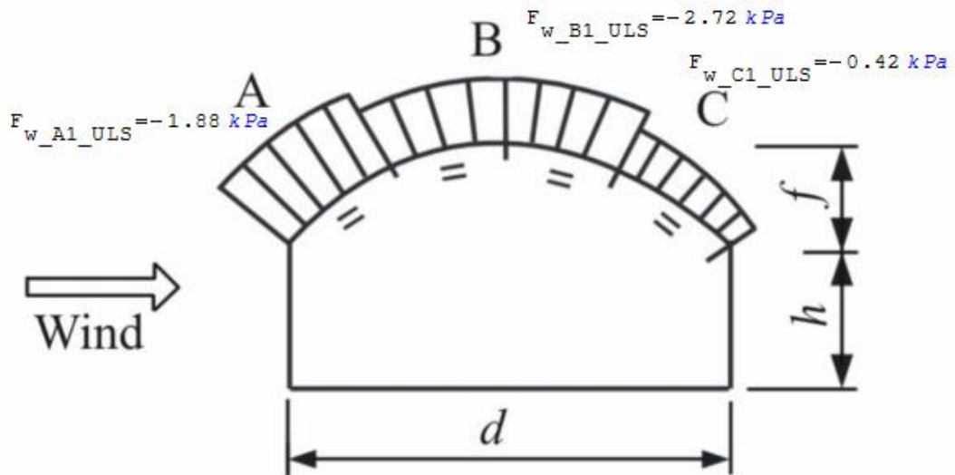
Figure 3.5: Resultant pressure force on elevated flat vault - load case 1 .
