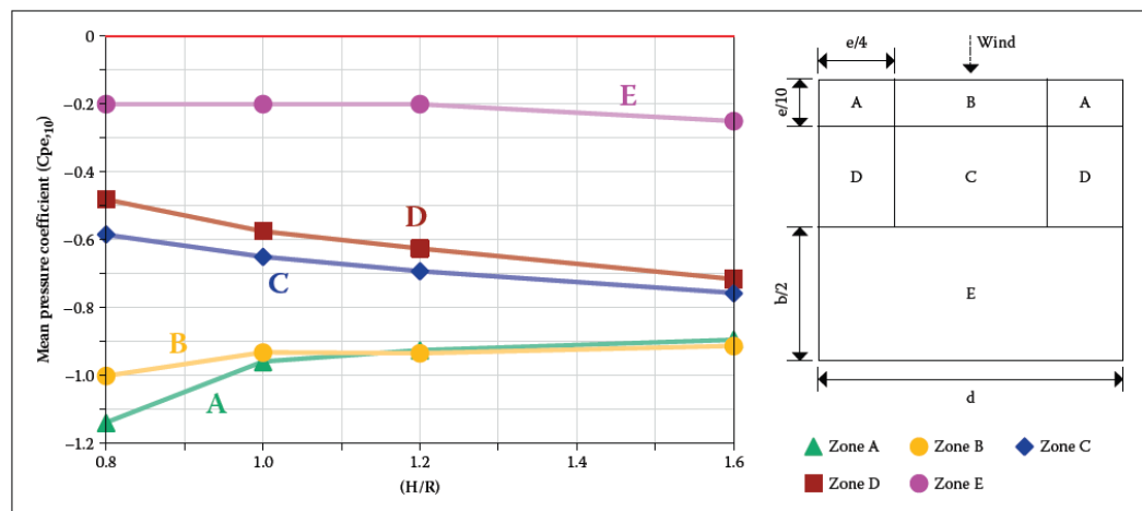
Figure 2.35: Wind azimuth direction 90/270 degrees (Bradley et al. , 2016)
