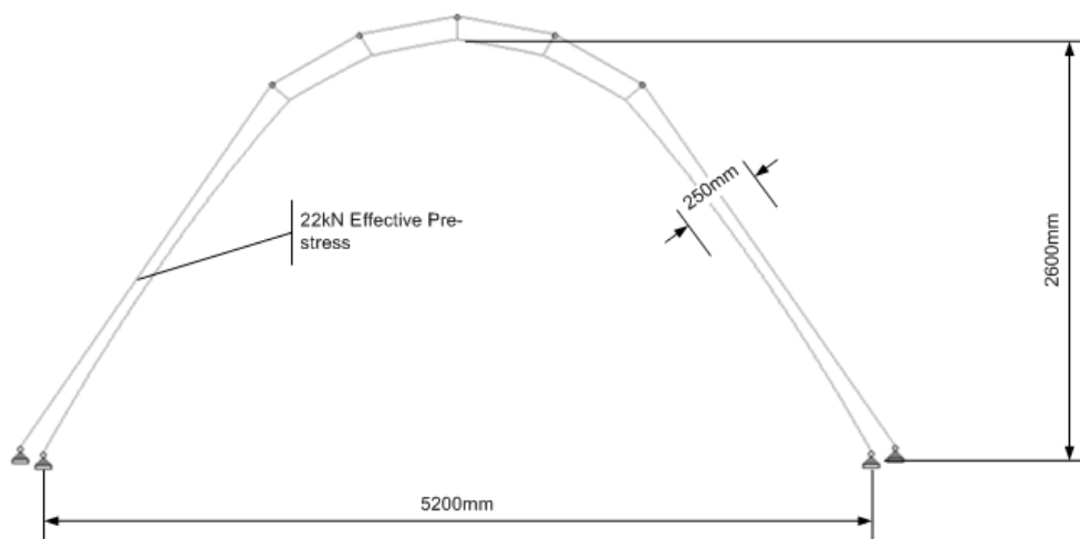
Figure 3.65: 250mm thick vault post-tensioned to 22kN effective post-tensioning.
