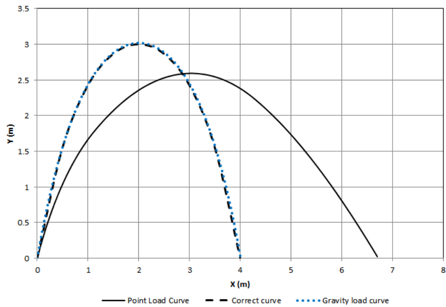
Figure 3.32: FLPC for steep vault of 250mm thickness subjected to gravity and wind loads (LC2) as per Table 12.
