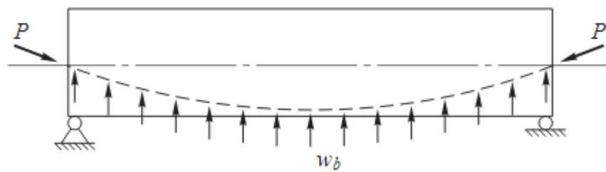
(b) Tendon forces acting on the concrete
