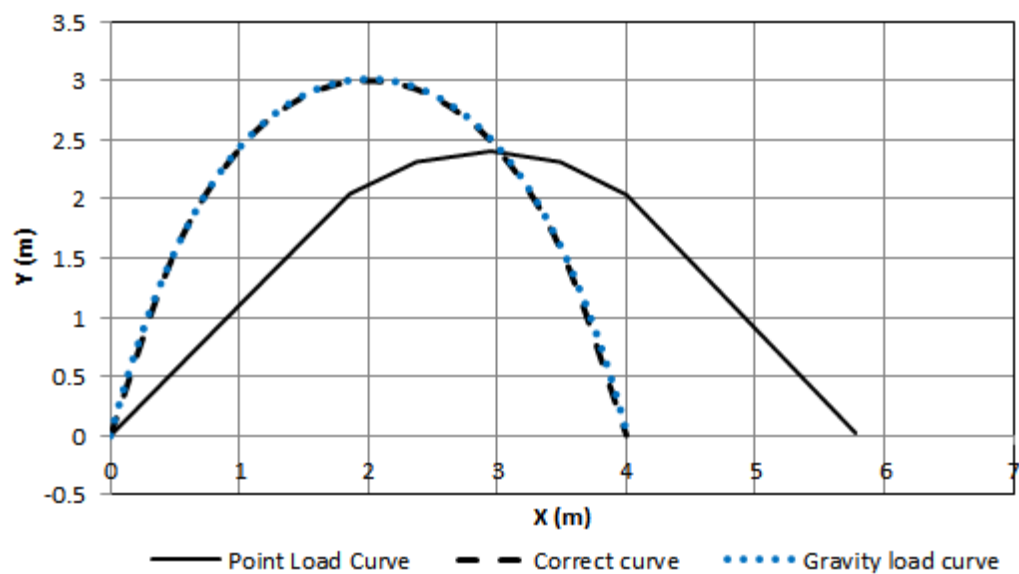
Figure 3.57: Optimised catenary geometry for externally draped post-tensioned tendon, supported at five pertinent positions, and exerting a 1000kN point load.
