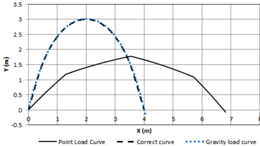
Figure 3.53: Optimised catenary geometry for externally draped post-tensioned tendon, supported at three pertinent positions, and exerting a 30kN point load.
