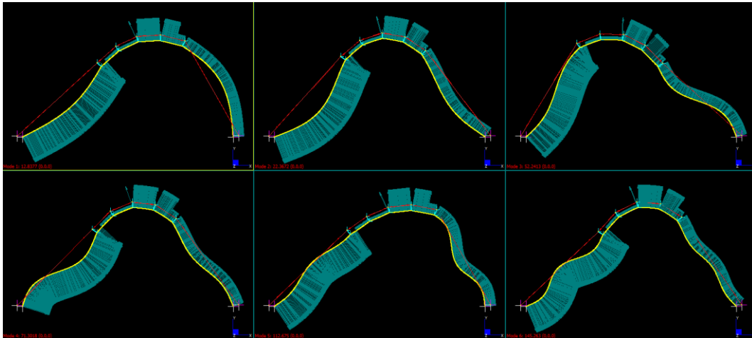
Figure 3.76: Buckling mode shapes for LC6 as per Table 12 for vault post-tensioned to pure compression for 300kph wind loads (Strand7).
