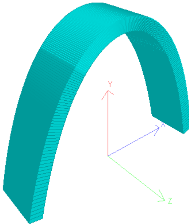
Figure 3.59: Isometric view (StaadPro V8i FEA model) of traditional catenary vault with concentrically placed post-tension tendon.
