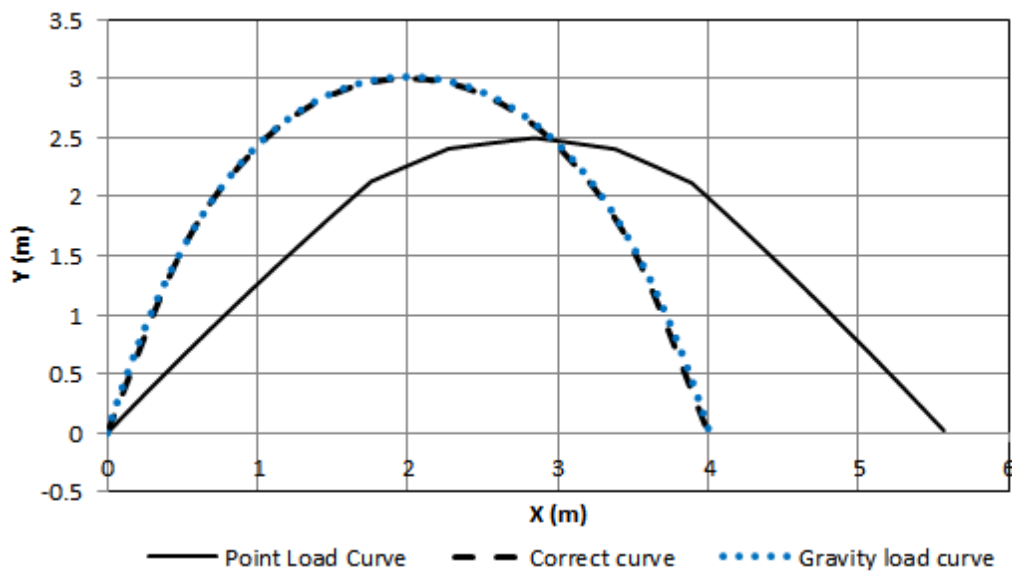
Figure 3.56: Optimised catenary geometry for externally draped post-tensioned tendon, supported at five pertinent positions, and exerting a 30kN point load.
