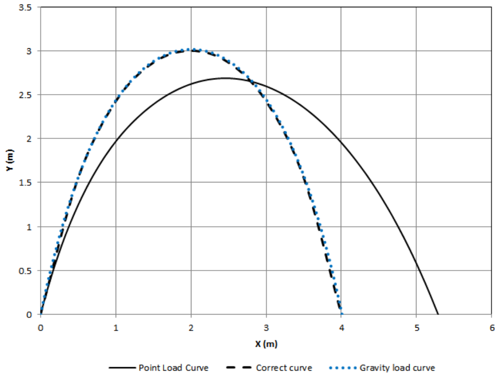
Figure 3.42: FLPC for steep vault of 1000mm thickness subjected to gravity and wind loads (LC6) as per Table 12.
