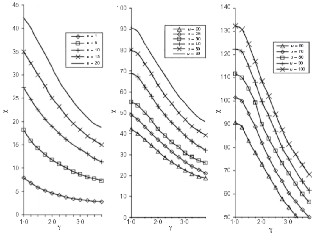
Figure 2.20: Design charts for the buckling of catenary arches (Pedreschi & Theodossopoulos, 2007).
