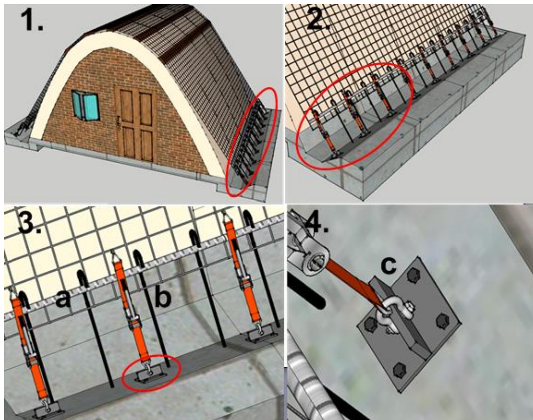
Figure 5.2: Six ratchet post-tensioning jack configuration.
