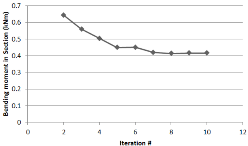
Figure 3.63: Convergence of FLPC based on bending moment in section of five point contact optimised vault.
