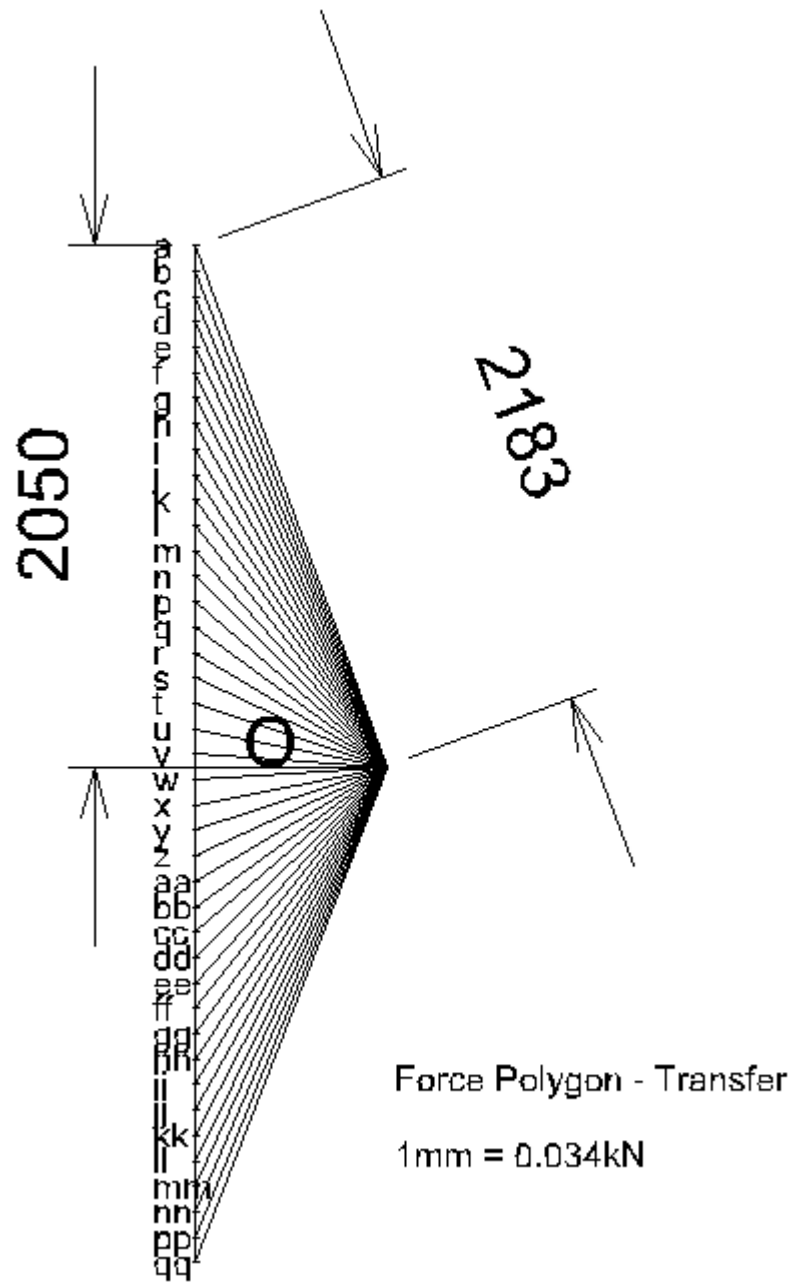
Figure 5.10: Force diagram at transfer.
