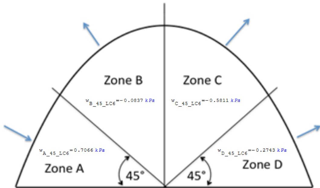
Figure 3.12: Resultant pressure force on steep vault for normal wind speeds - load case 6 (Bradley et al. , 2016).
