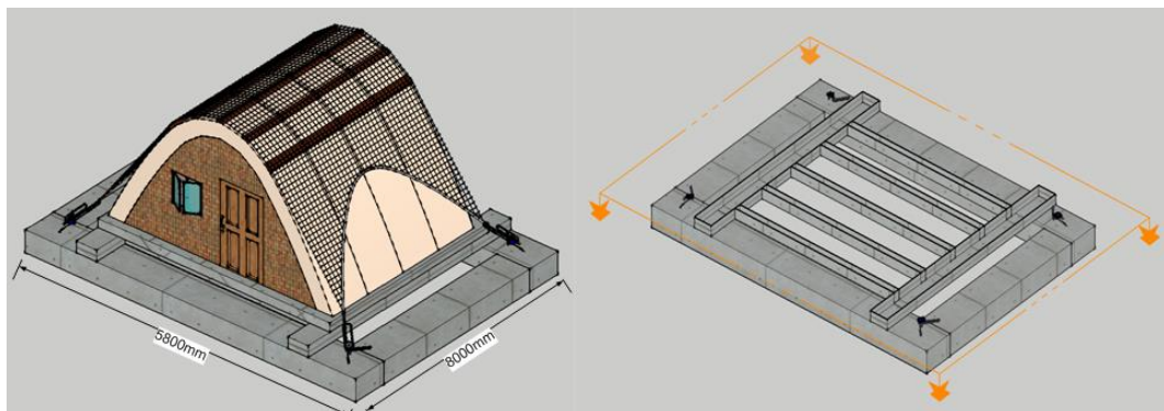
Figure 5.13: Funicular cable tensioning – tied strip footing for anchor foundation and section at foundation level.
