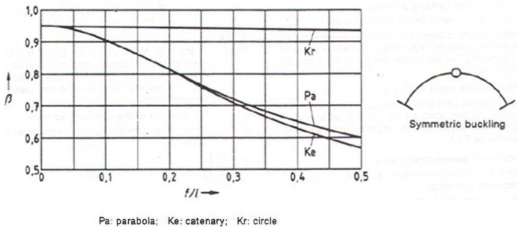
Figure 2.16: Buckling coefficient ( \beta ) for in-plane buckling of a one hinged arch system (German Building and Civil Engineering Standards Committee & German Committee for Structural Steelwork, 1990).
