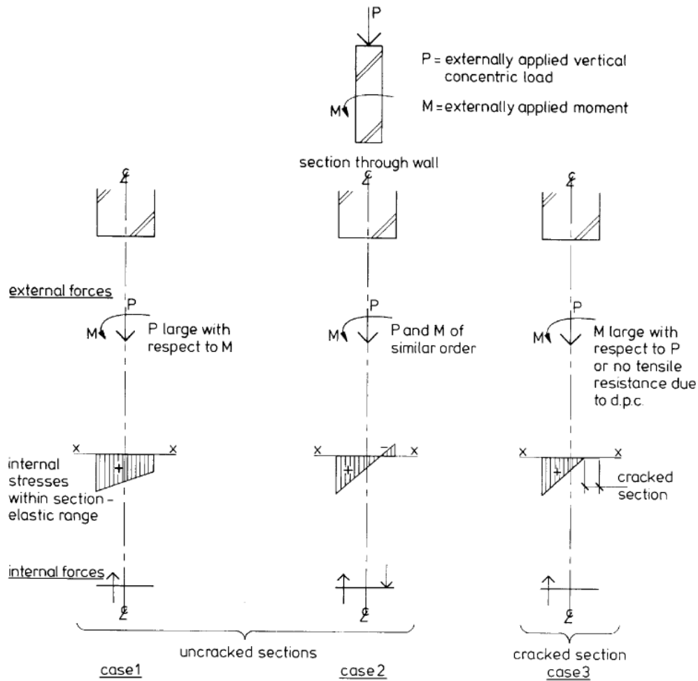
Figure 2.43: Un-cracked vs cracked masonry sections (Curtin et al. , 1995).
