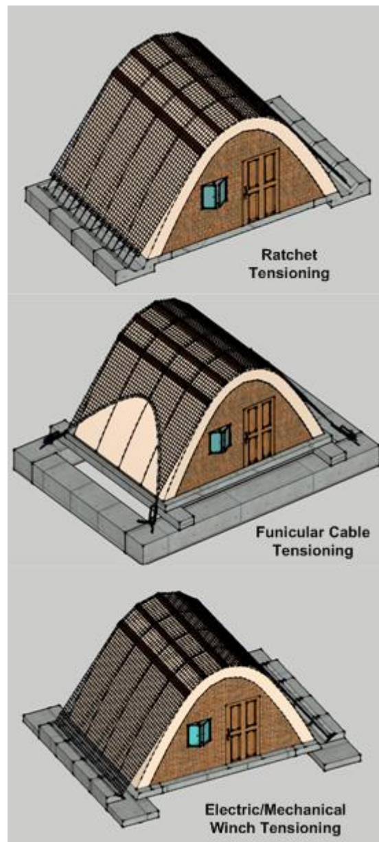
Figure 6.2: Post-tensioning solutions.
