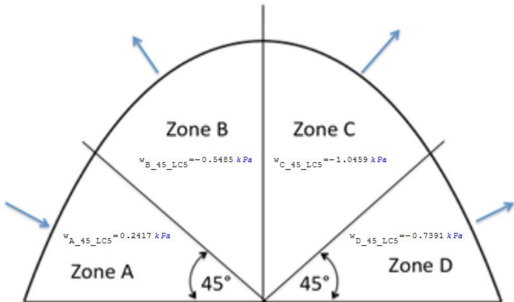
Figure 3.11: Resultant pressure force on steep vault for normal wind speeds - load case 5 (Bradley et al. , 2016).
