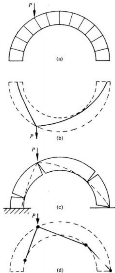
Figure 2.3: Collapse of a semi-circular masonry arch under a point load (Huerta, 2001).
