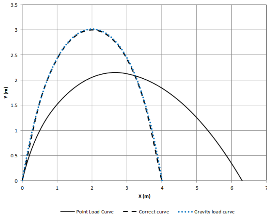
Figure 3.34: FLPC for steep vault of 250mm thickness subjected to gravity and wind loads (LC4) as per Table 12.
