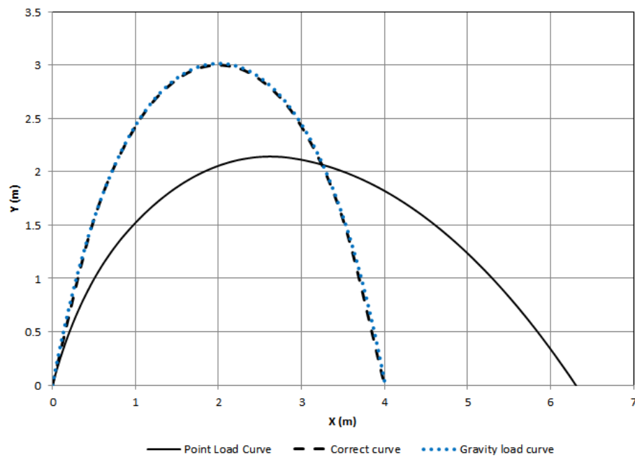
Figure 3.33: FLPC for steep vault of 250mm thickness subjected to gravity and wind loads (LC3) as per Table 12.
