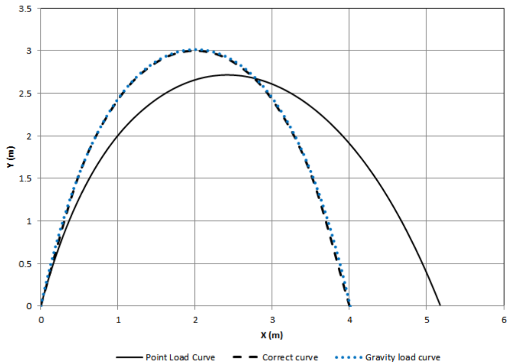
Figure 3.30: FLPC for steep vault of 250mm thickness subjected to gravity and wind loads (LC6) as per Table 11.
