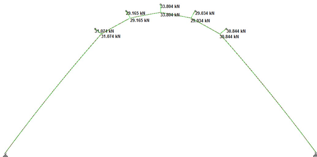
Figure 3.64: Five point contact post-tensioned vault (StaadPro V8i model) tendon support loads for no tension allowed in 300kph wind load condition.
