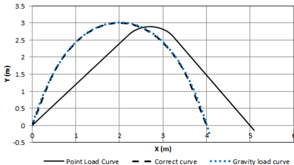
Figure 3.51: Optimised catenary geometry for externally draped post-tensioned tendon, supported along the vault's crown, and exerting a uniform 1000kN load on vault surface.
