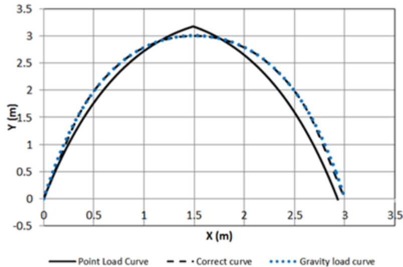
Figure 3.19: Catenary arch subjected to a 5kN point load at its centreline (Gohnert, 2016).
