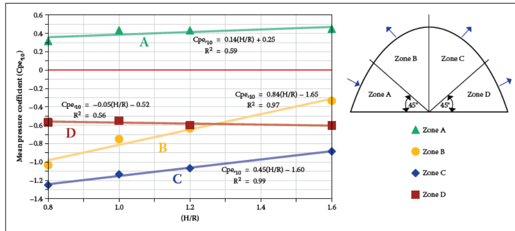
Figure 2.34: Wind azimuth direction 30/45 degrees (Bradley et al. , 2016)
