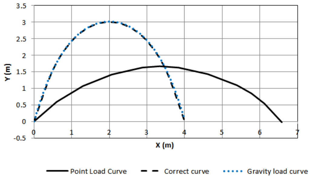
Figure 3.47: Optimised catenary geometry for externally draped post-tensioned tendon, supported along the vault's arch, and exerting a uniform 1000kN load on vault surface.
