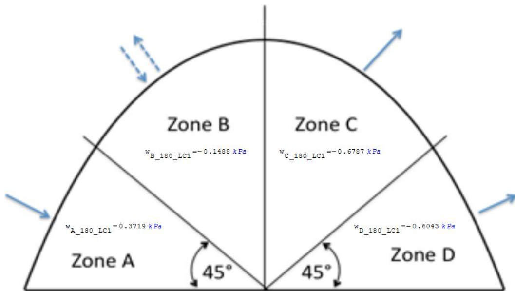
Figure 3.7: Resultant pressure force on steep vault for normal wind speeds - load case 1 (Bradley et al. , 2016).
