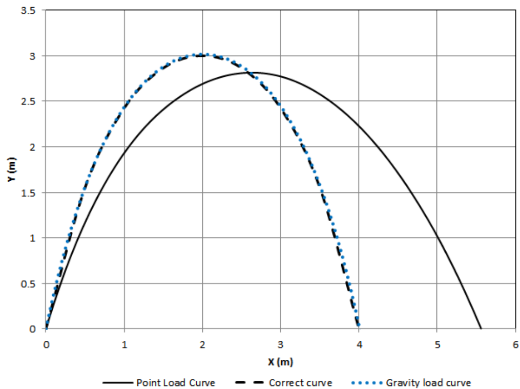
Figure 3.29: FLPC for steep vault of 250mm thickness subjected to gravity and wind loads (LC5) as per Table 11.
