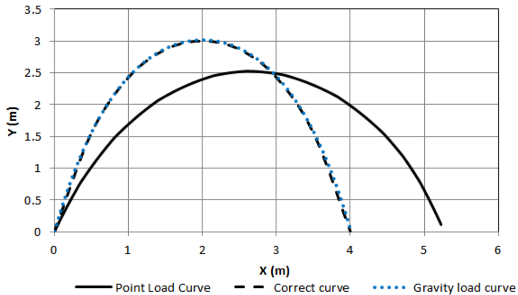
Figure 3.46: Optimised catenary geometry for externally draped post-tensioned tendon, supported along the vault's arch, and exerting a uniform 1kN load on vault surface.
