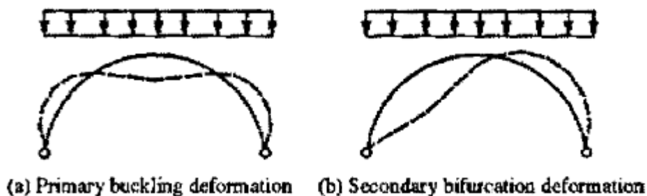
Figure 2.12 : Two buckling modes of a two hinged arch (Jinsan & Yanlin, 2002).
