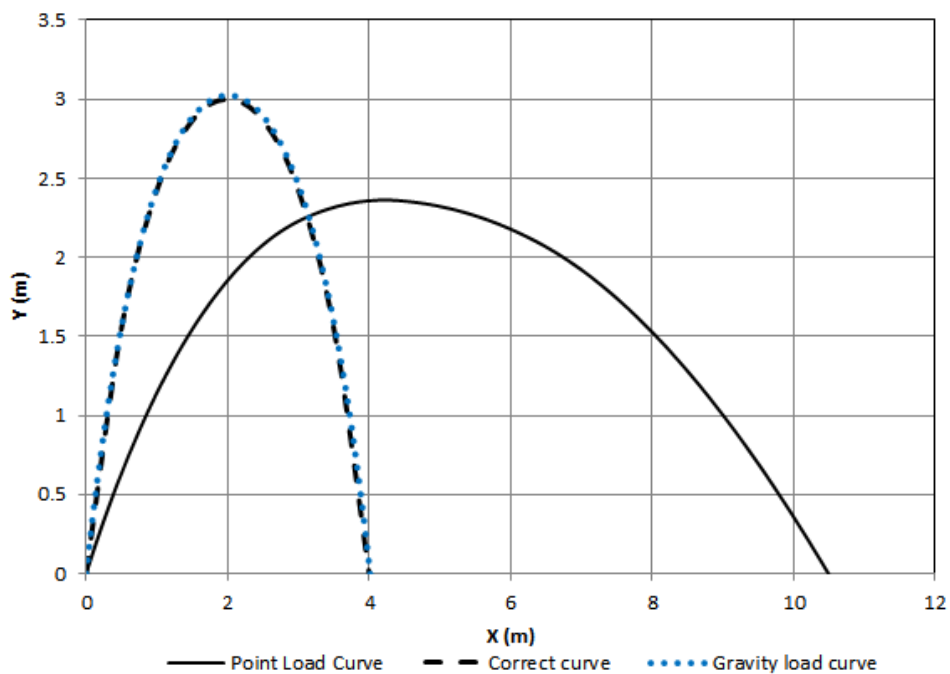
Figure 3.35: FLPC for steep vault of 250mm thickness subjected to gravity and wind loads (LC5) as per Table 12.
