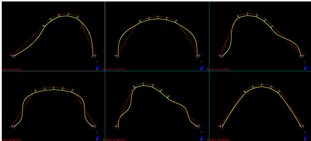
Figure 3.71: Buckling mode shapes for dominant load case of vault post-tensioned to pure compression for service loads (Strand7).
