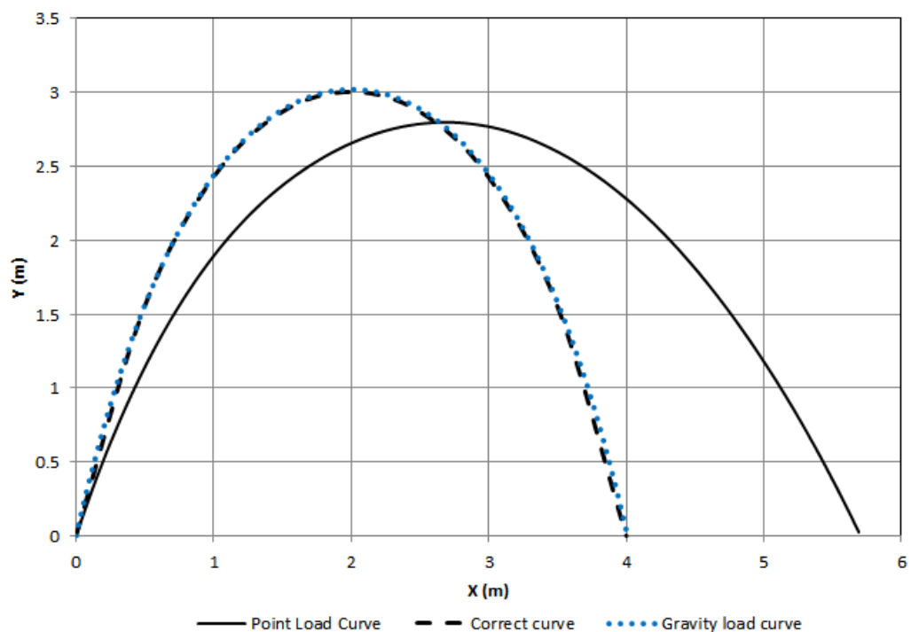
Figure 3.41: FLPC for steep vault of 1000mm thickness subjected to gravity and wind loads (LC5) as per Table 12.
