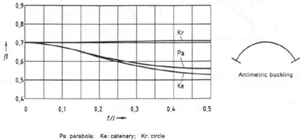
Figure 2.15: Buckling coefficient ( \beta ) for in-plane buckling of a monolithic arch system (German Building and Civil Engineering Standards Committee & German Committee for Structural Steelwork, 1990).
