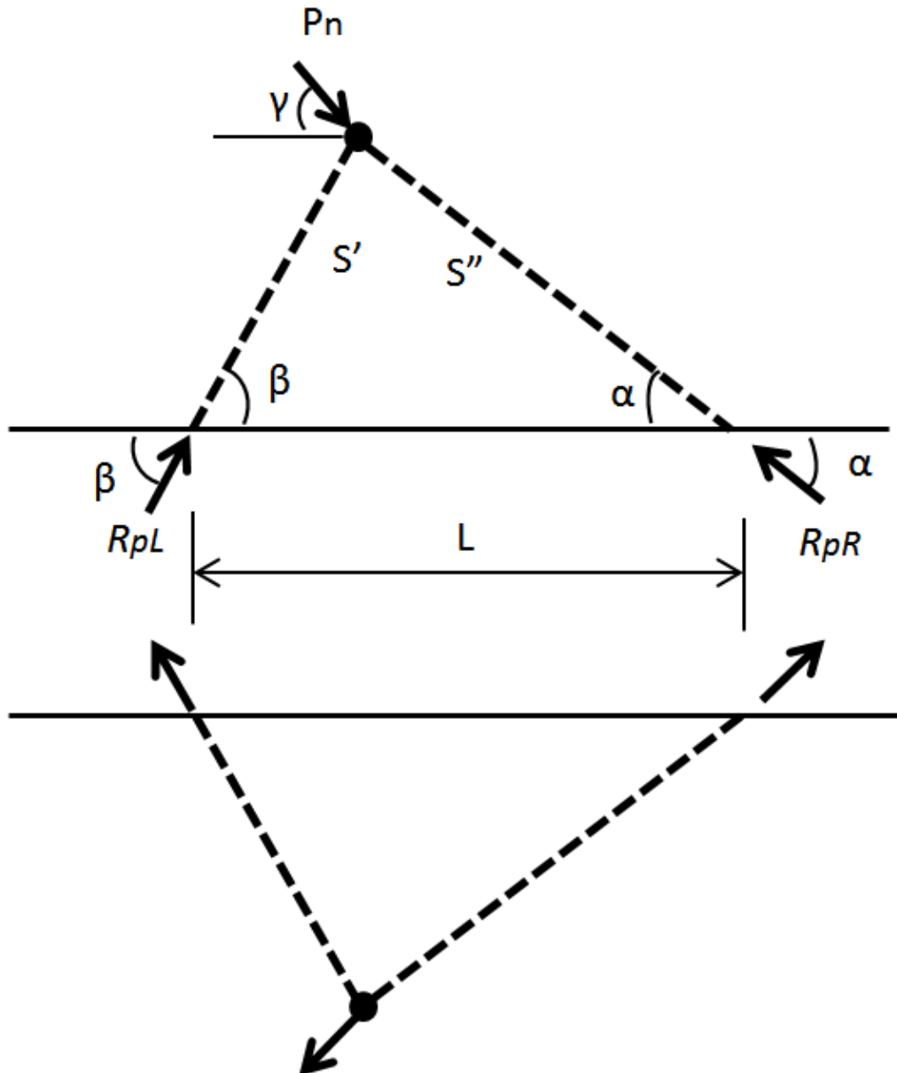
Figure 2.8: Triangular shape to support a point load in pure compression (Gohnert & Bradley, 2016).
