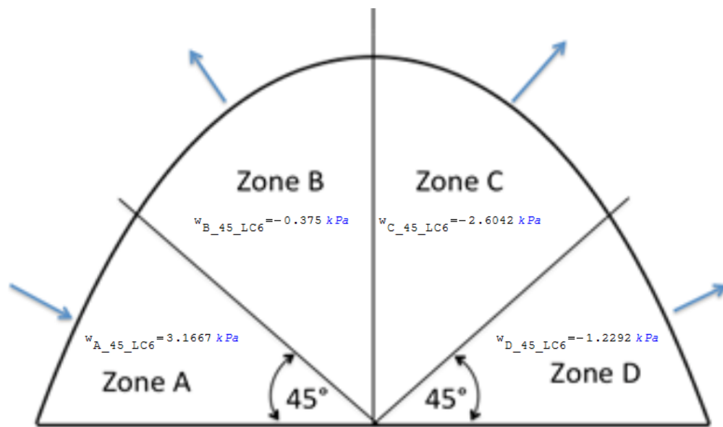
Figure 3.18: Resultant pressure force on steep vault for 300kph wind speed - load case 6 (Bradley et al. , 2016).
