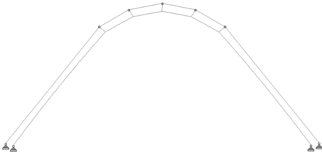
Figure 3.62: Five point contact post-tensioned vault (StaadPro V8i model) for no tension allowed in 300kph wind load condition.
