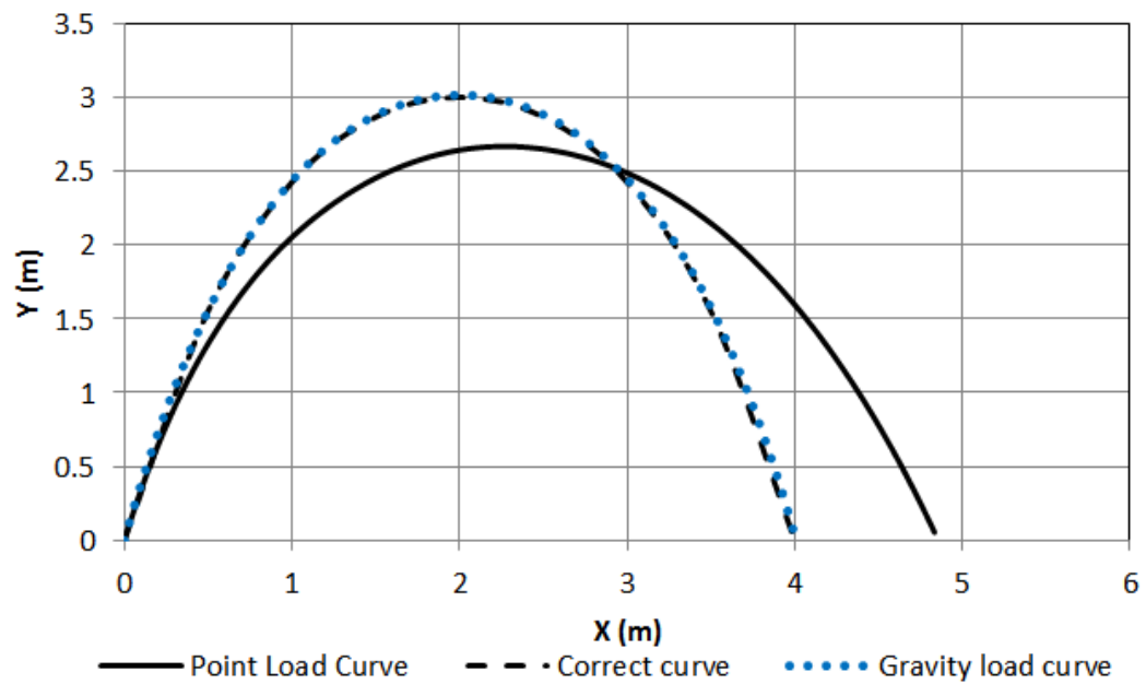
Figure 3.28: FLPC for steep vault of 250mm thickness subjected to gravity and wind loads (LC4) as per Table 11.
