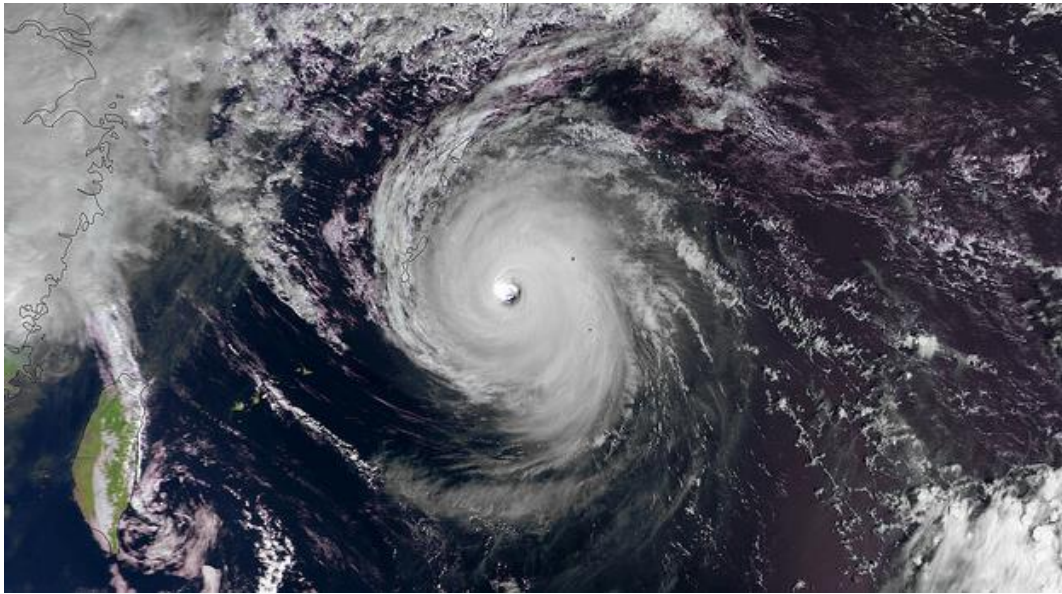
Figure 1.1: Super Typhoon Haiyan seen from outer space (Marsh, 2013).
