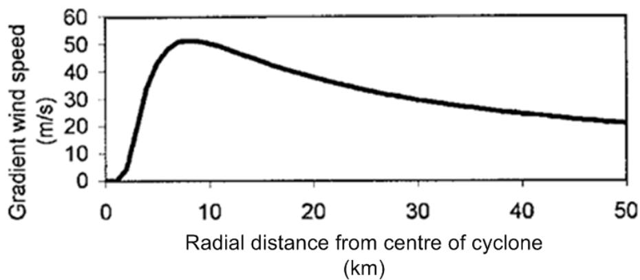
Figure 2.27: Gradient wind speed for Cyclone “Tracy” (Holmes, 2001).
