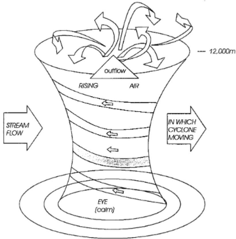
Figure 2.26: Three-dimensional vortex structure in a developed tropical cyclone (Holmes, 2001).
