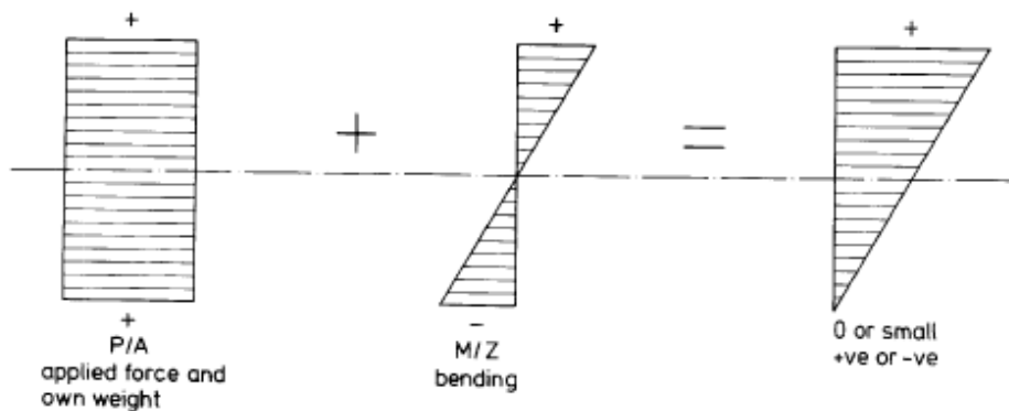
Figure 2.53: Stress state in a concentrically pre-stressed element (Curtin et al. , 1995).
