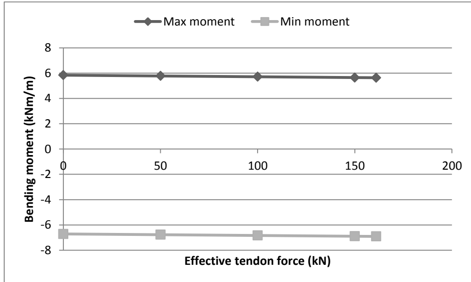
Figure 3.61: Graphical representation of bending moment reduction vs tendon force increase for data presented in Table 17.
