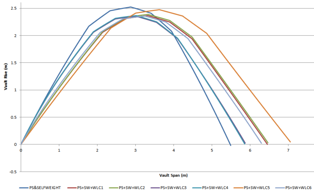
Figure 3.58: FLPC for five point post-tensioned vault, subjected to all load conditions.
