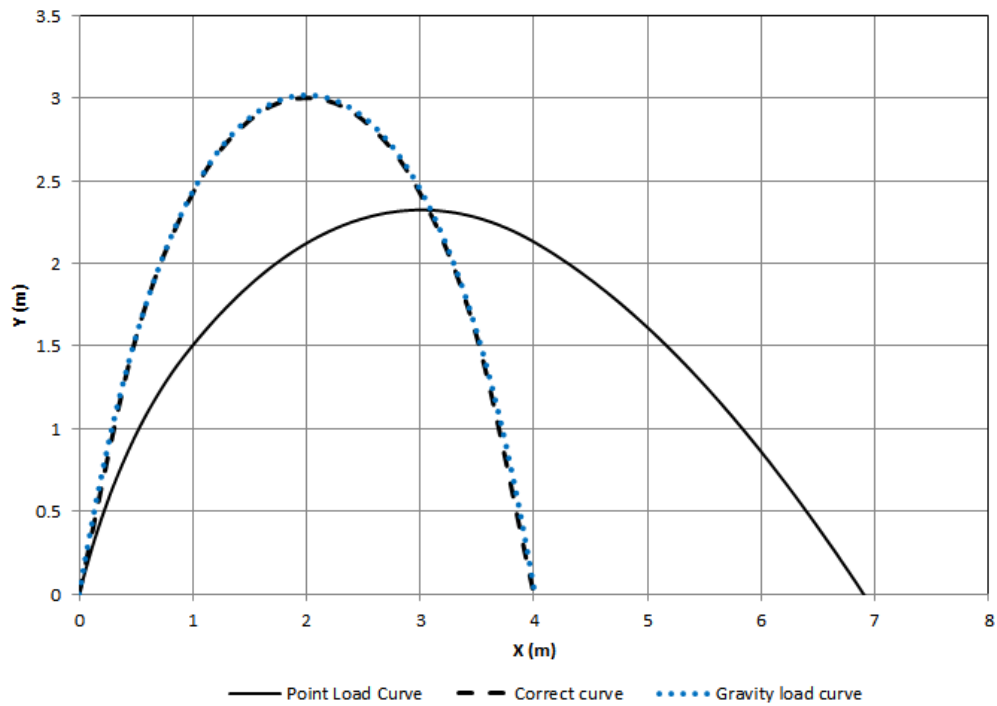
Figure 3.36: FLPC for steep vault of 250mm thickness subjected to gravity and wind loads (LC6) as per Table 12.
