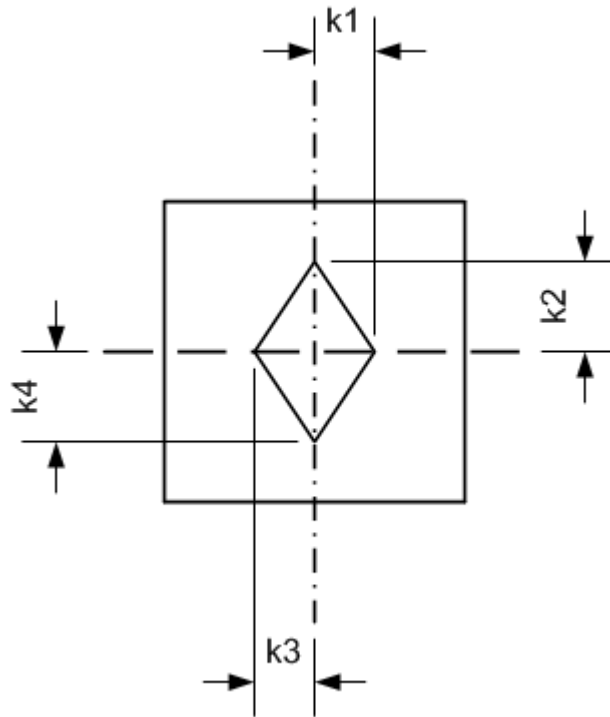
Figure 2.10: Kern points of rectangular cross section
