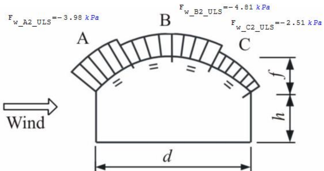
Figure 3.6: Resultant pressure force on elevated flat vault - load case 2.
