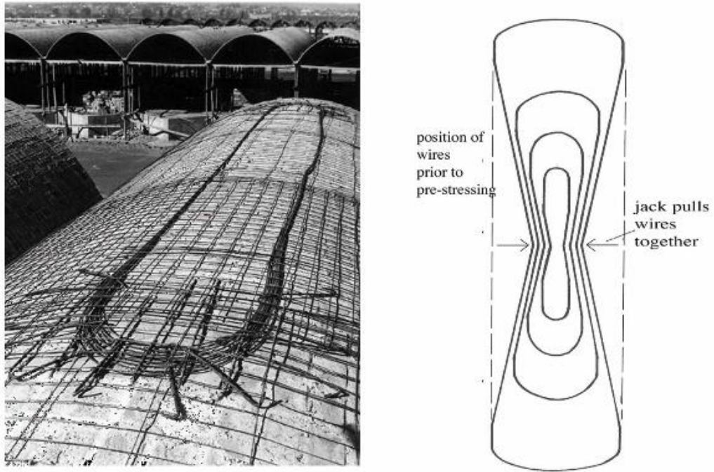
Figure 2.22: Looped pre-stressing steel in vault (Pedreschi, 2006).
