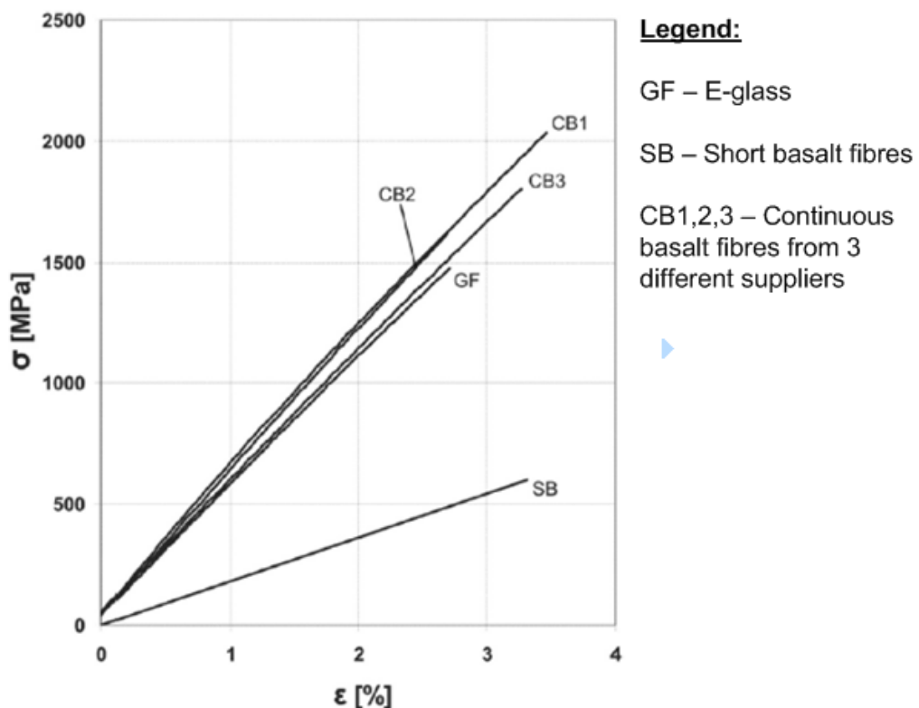
Figure 2.62: Typical stress-strain diagram of basalt fibres vs fibre glass (Fiore et al. , 2015).
