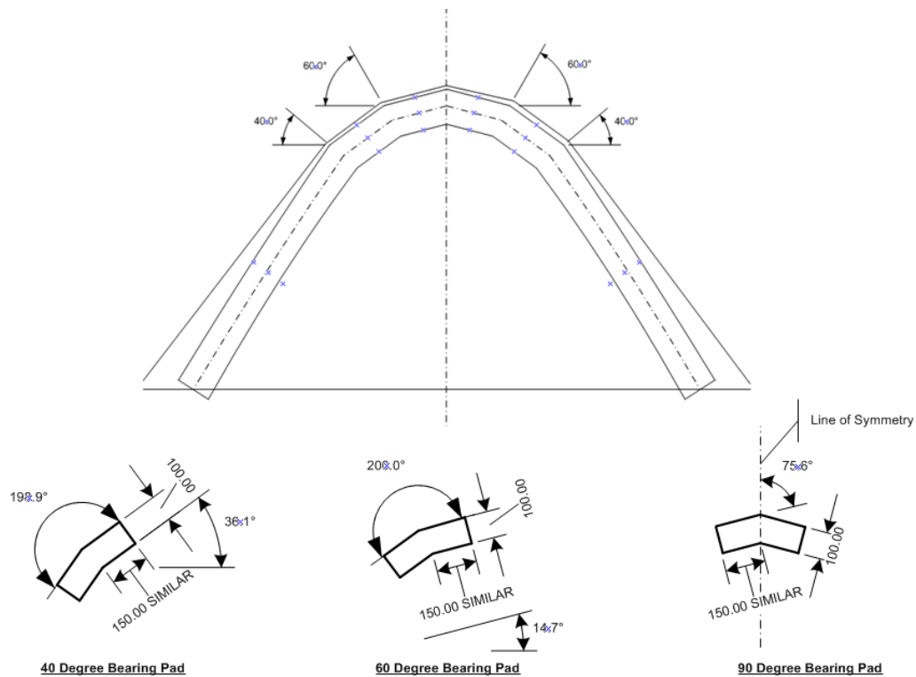
Figure 5.16: Post-tension bearing pad details.
