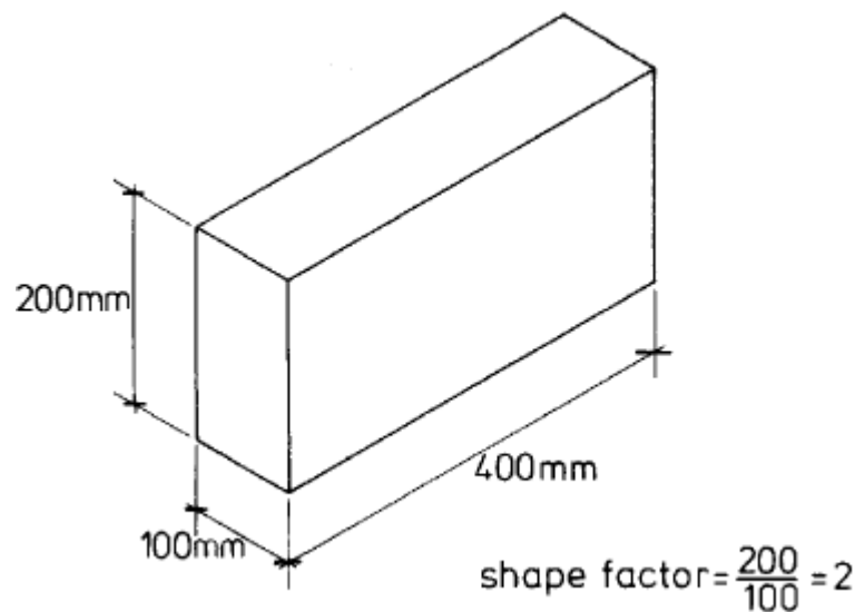
Figure 2.38: Determination of the shape factor of a masonry brick (Curtin et al. , 1995).
