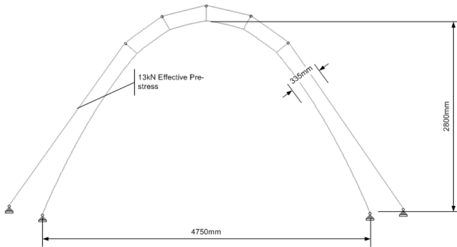
Figure 3.67: 335mm thick vault post-tensioned to 13kN effective post-tensioning.
