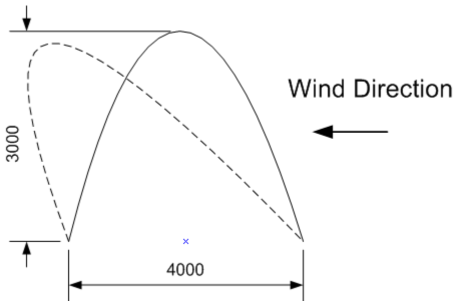
Figure 3.2: Steep vault subjected to wind load.
