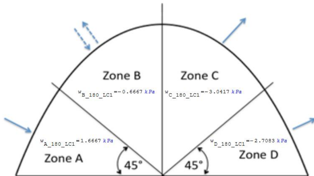
Figure 3.13: Resultant pressure force on steep vault for 300kph wind speed - load case 1 (Bradley et al. , 2016).
