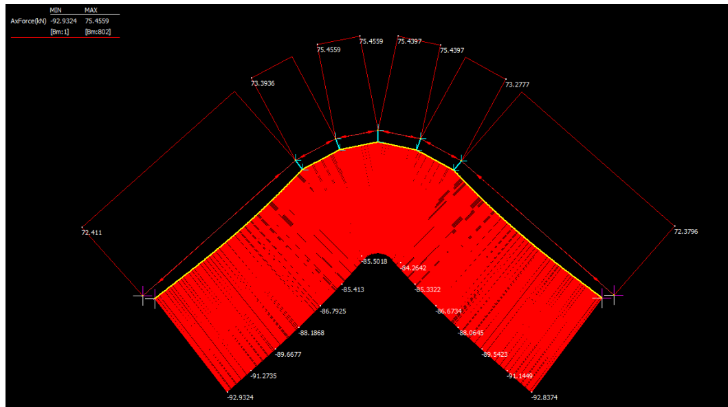
Figure 3.74: Axial force diagram for five point contact post-tensioned vault with string grouping (Strand7).
