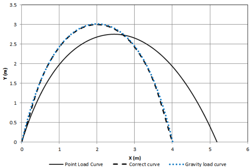
Figure 3.25: FLPC for steep vault of 250mm thickness subjected to gravity and wind loads (LC1) as per Table 11.
