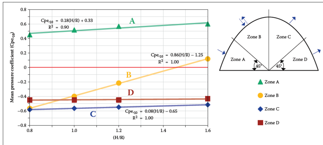
Figure 2.33: Wind azimuth direction 0/180 degrees (Bradley, Gohnert, Goliger & Mistry, 2016)
