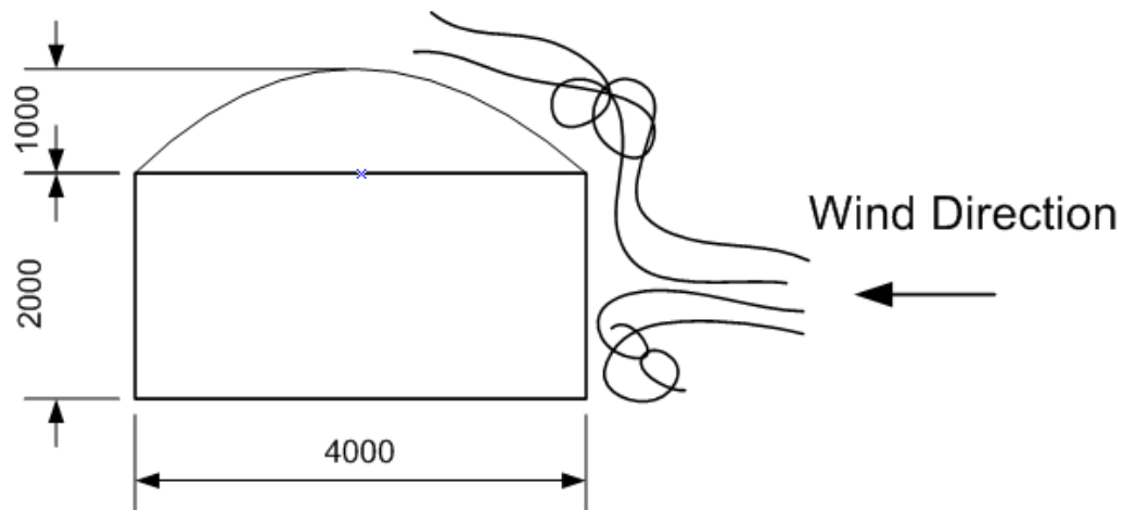
Figure 3.1: Elevated flat vault on vertical walls subjected to wind flow.
