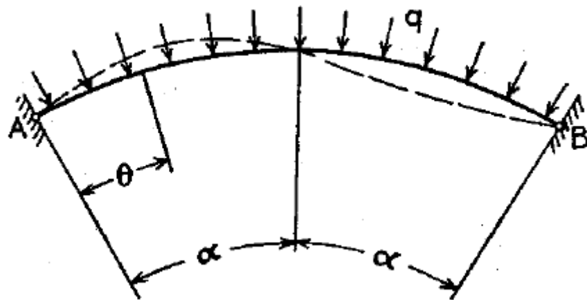
Figure 2.13 : Buckling profile of a uniformly compressed circular arch with hinged ends (Timoshenko & Gere, 1963).
