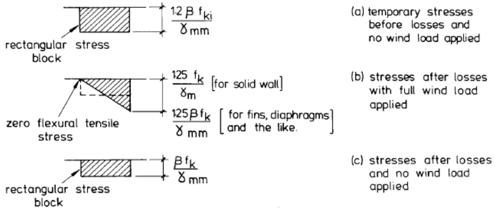
Figure 2.54: Stress state of a post-tensioned masonry section before, during and after wind load (Curtin et al. , 1995).
