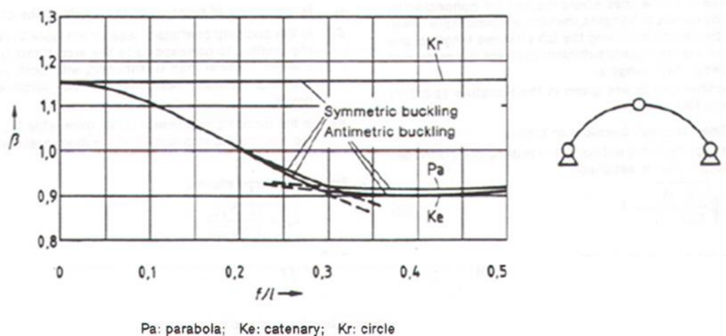
Figure 2.18: Buckling coefficient ( \beta ) for in-plane buckling of a three hinged arch system (German Building and Civil Engineering Standards Committee & German Committee for Structural Steelwork, 1990).
