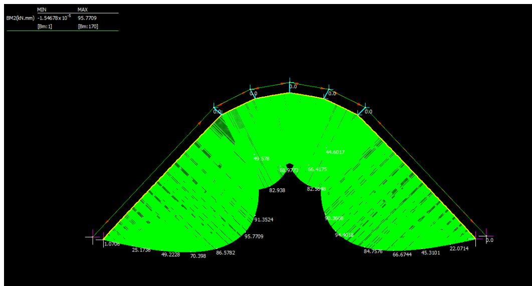
Figure 3.70: Bending moment diagram for five point contact post-tensioned vault without string grouping (Strand7).
