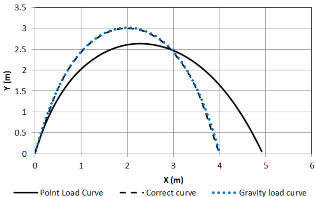
Figure 3.39: FLPC for steep vault of 1000mm thickness subjected to gravity and wind loads (LC3) as per Table 12.
