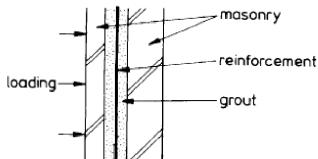
Figure 2.48: Section through a normally reinforced masonry section (Curtin et al. , 1995).
