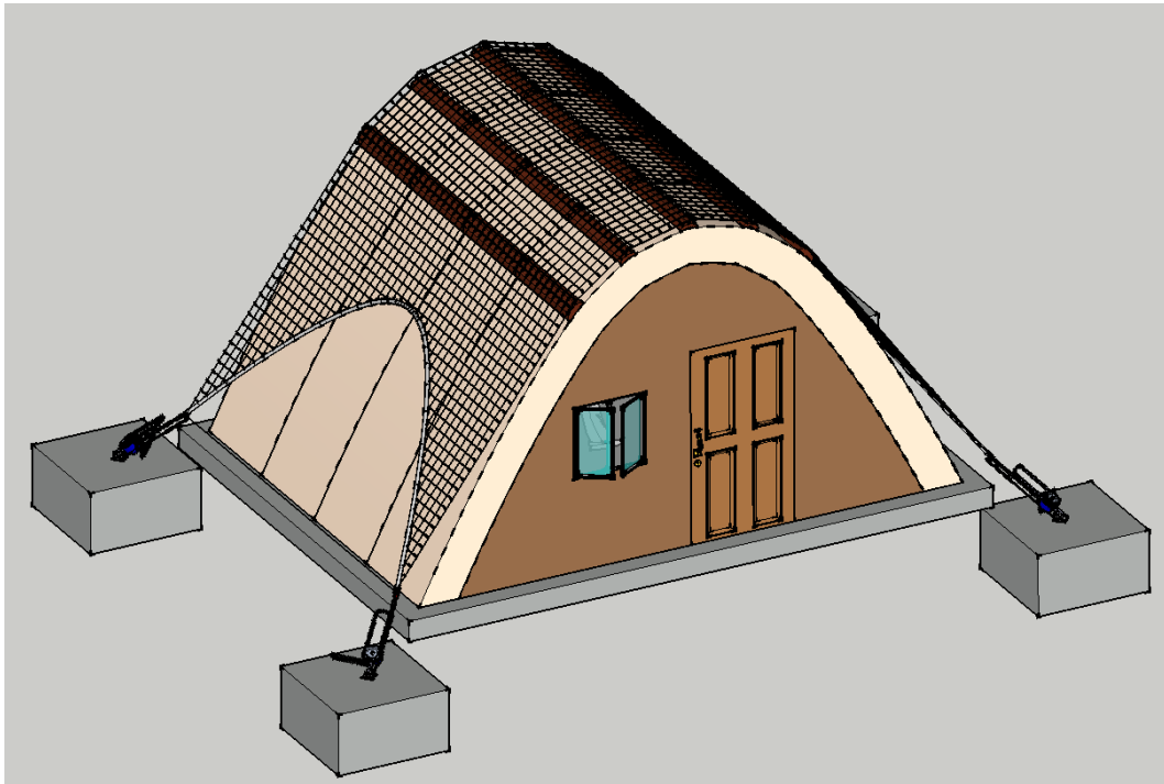
Figure 5.7: Funicular chain block tensioning configuration.
