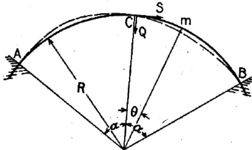
Figure 2.14 : Buckling profile of a uniformly compressed circular arch with fixed ends (Timoshenko & Gere, 1963).
