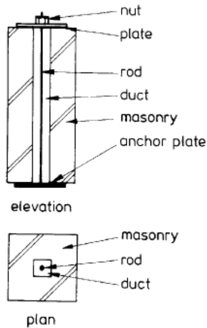
Figure 2.52: Section through a typical post-tensioned masonry column (Curtin et al. , 1995).
