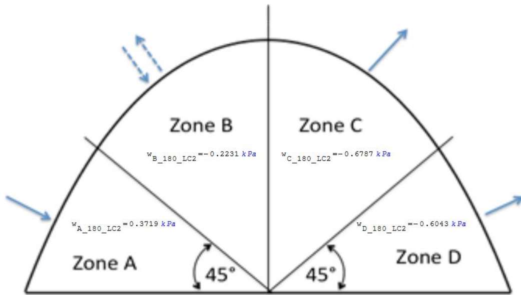
Figure 3.8: Resultant pressure force on steep vault for normal wind speeds - load case 2 (Bradley et al. , 2016).
