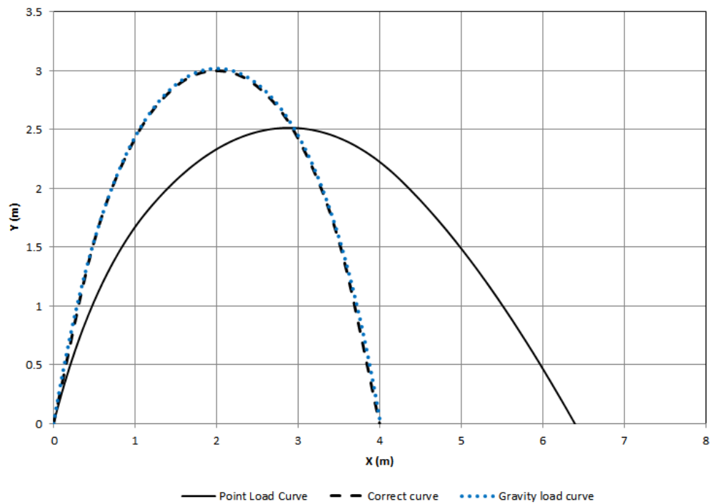
Figure 3.31: FLPC for steep vault of 250mm thickness subjected to gravity and wind loads (LC1) as per Table 12.
