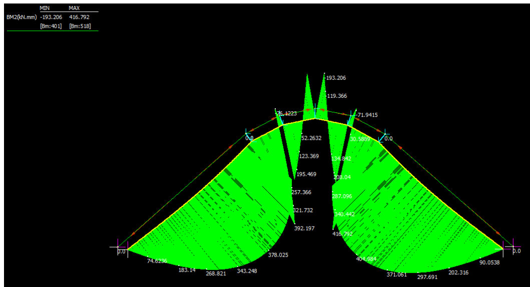
Figure 3.73: Bending moment diagram for five point contact post-tensioned vault with string grouping (Strand7).
