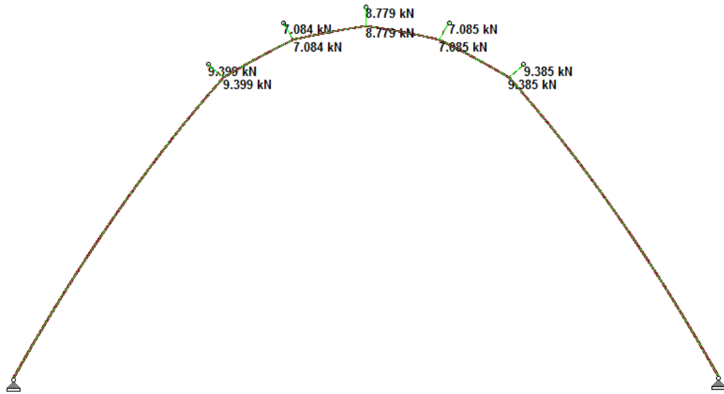
Figure 3.66: Five point contact post-tensioned vault (StaadPro V8i model) tendon support loads for no tension allowed in service wind load condition - 22kN effective post-tensioning.
