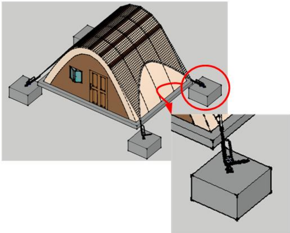
Figure 5.12: Funicular cable tensioning anchor foundations.
