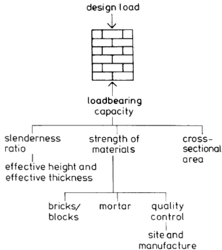
Figure 2.36: Factors affecting the compressive strength of masonry (Curtin et al. , 1995).
