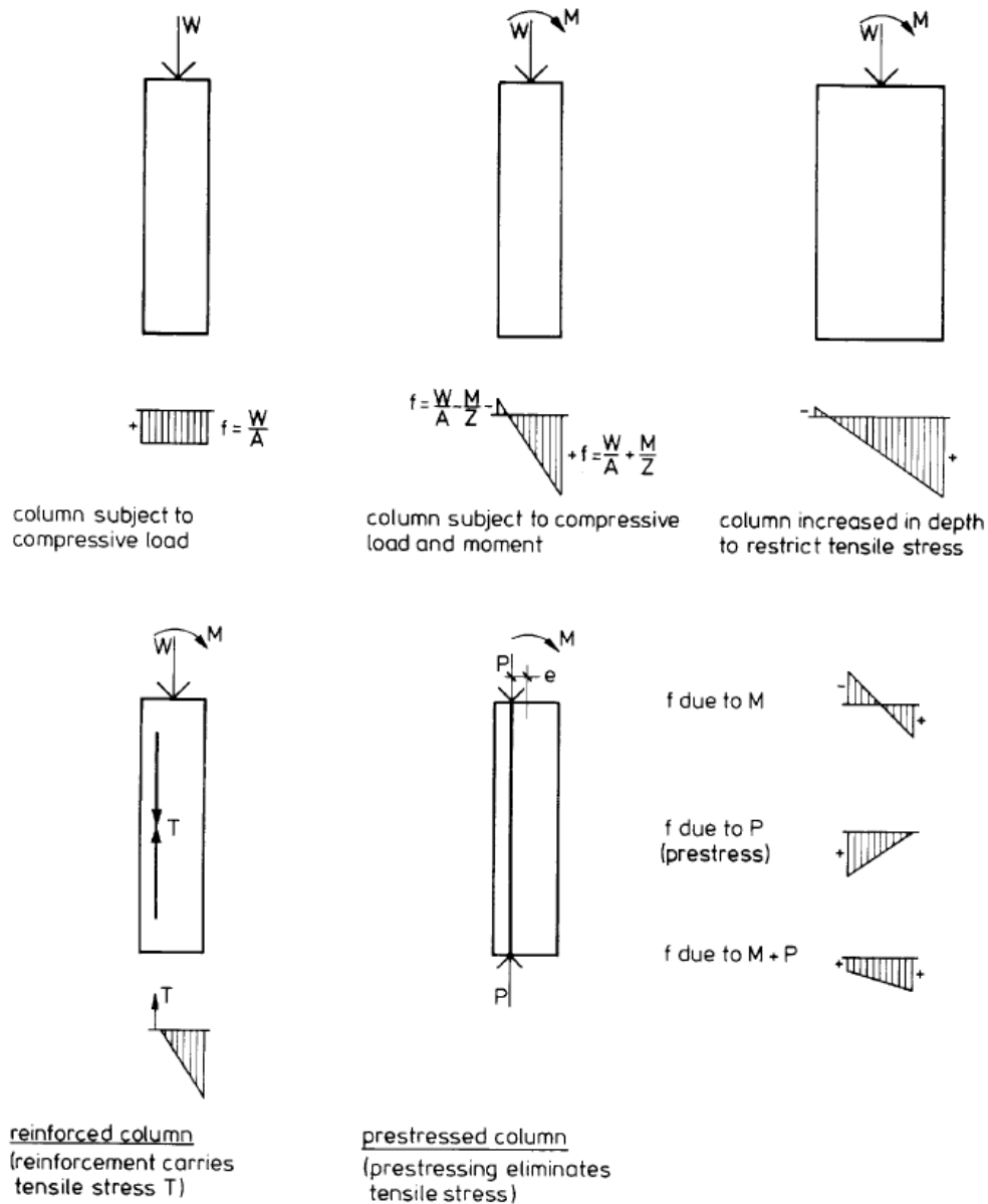
Figure 2.47: Illustration of the difference between normal reinforcement and pre-stressing (Curtin et al. , 1995).
