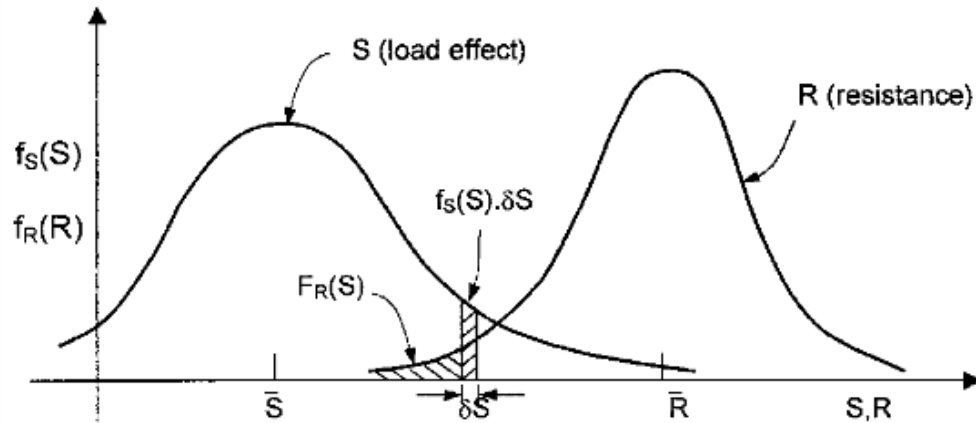
Figure 2.28: Probability densities for load effects and resistance (Holmes, 2001).
