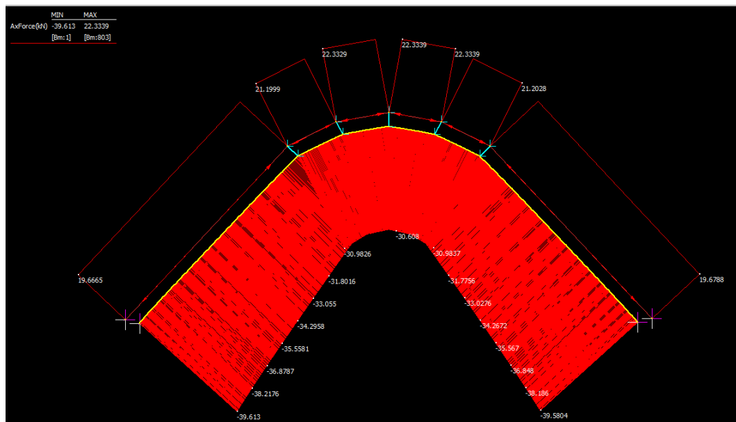
Figure 3.69: Axial force diagram for five point contact post-tensioned vault without string grouping (Strand7).
