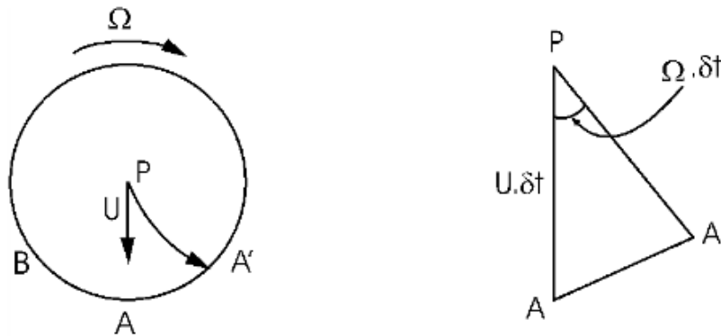
Figure 2.24: The apparent Coriolis force due to the earth's rotation (Holmes, 2001).
