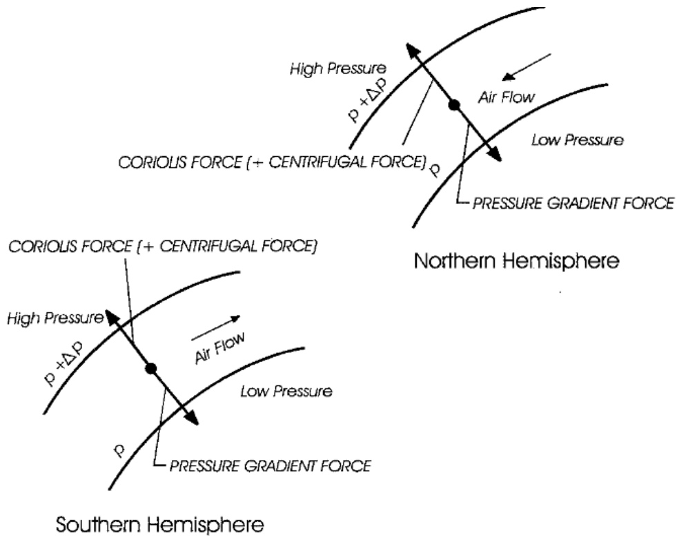
Figure 2.25: Balanced geostrophic flow in the Northern and Southern hemisphere (Holmes, 2001).
