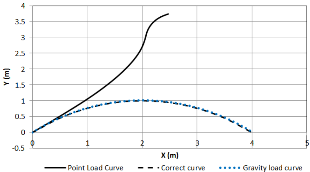
Figure 3.23: FLPC for elevated flat vault of 250mm thickness subjected to gravity and wind loads as per Table 10 (LC2).
