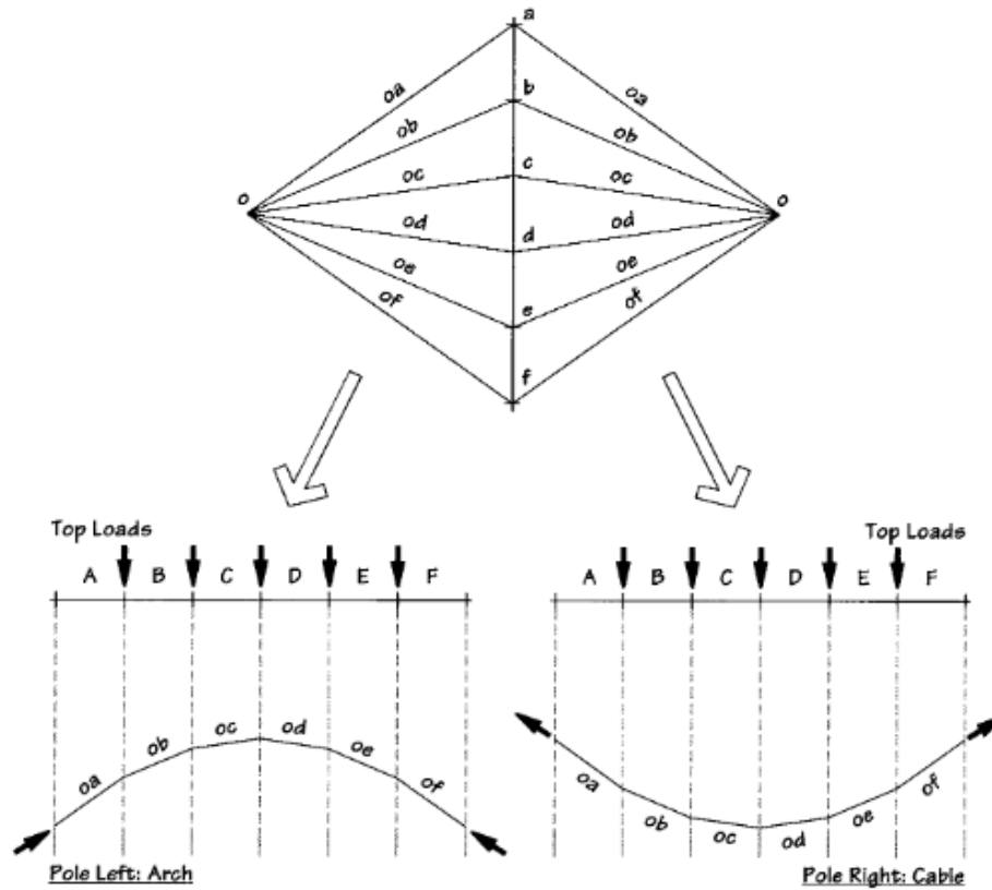
Figure 2.4: Graphical representation of a hanging chain and its inverted catenary arch shape (Allan et al. , 2010).
