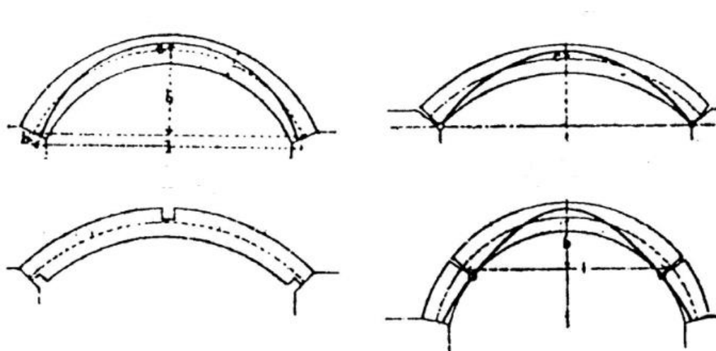
Figure 2.9: Shifting of the line of thrust of a masonry vault due to a change in support condition (Huerta, 2001).
