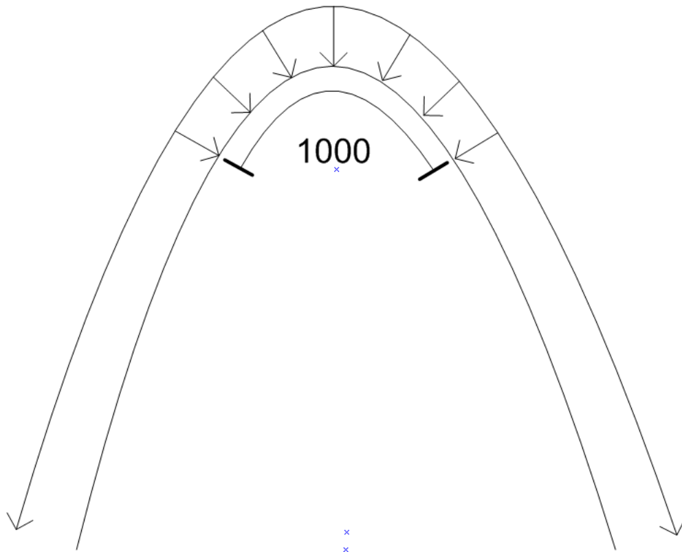
Figure 3.48: Schematic of vault draped in post-tension tendon and supported along 1000mm of crown.
