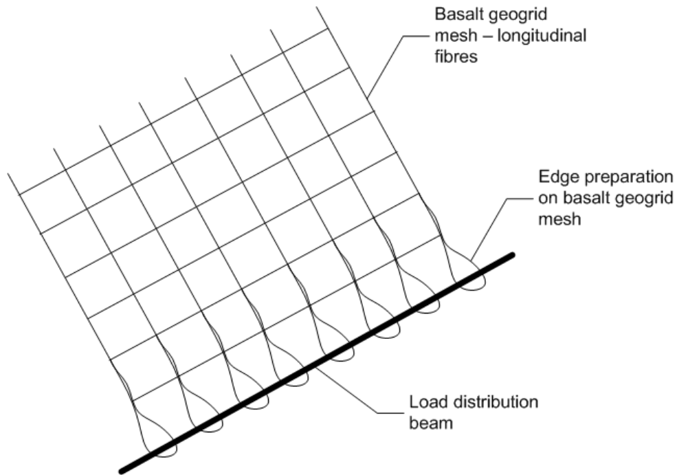
Figure 5.3: Edge preparation of basalt geogrid for effective load transfer from load distribution beam to mesh.
