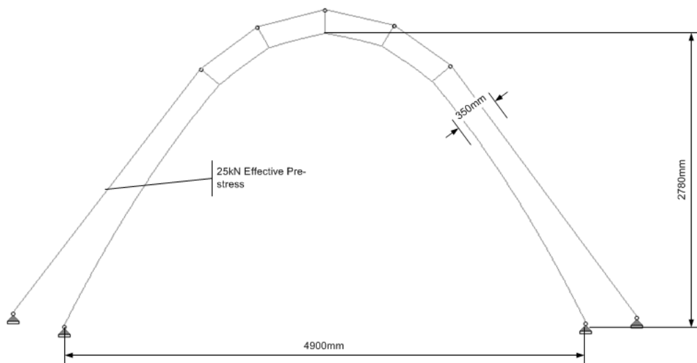
Figure 3.68: 350mm thick vault post-tensioned to 25kN effective post-tensioning.
