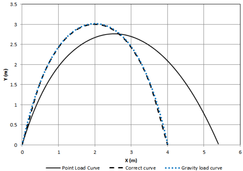
Figure 3.38: FLPC for steep vault of 1000mm thickness subjected to gravity and wind loads (LC2) as per Table 12.
