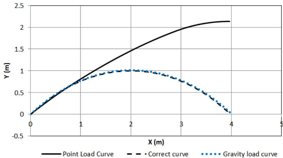
Figure 3.21: FLPC for elevated flat vault of 250mm thickness subjected to gravity and wind loads as per Table 10 (LC1).
