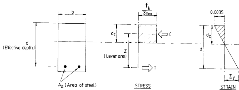
Figure 2.49: Stress strain relationship in a reinforced masonry section (Curtin et al. , 1995).
