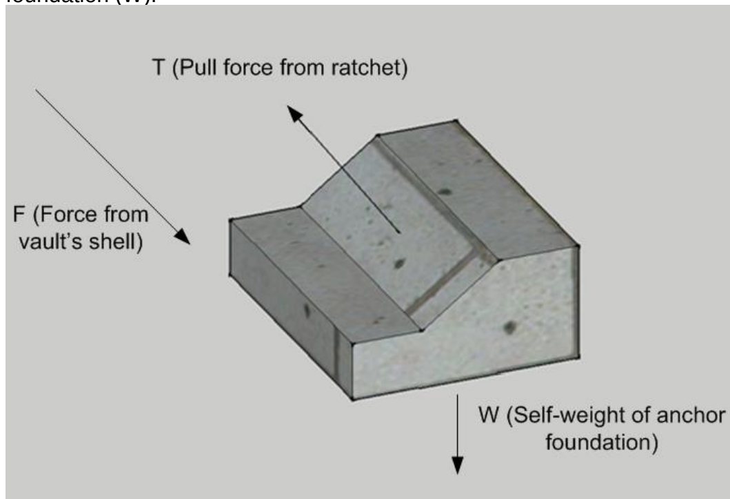
Figure 5.6: Ratchet configuration - anchor foundation.
