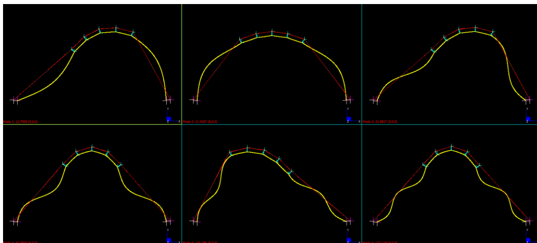
Figure 3.75: Buckling mode shapes for dominant load case of vault post-tensioned to pure compression for 300kph wind loads (Strand7).
