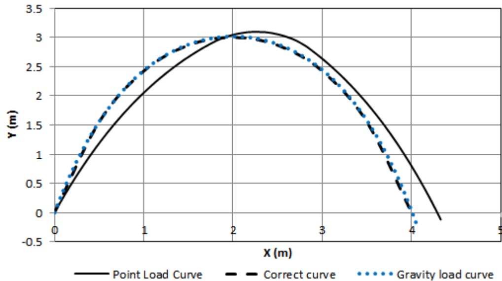
Figure 3.49: Optimised catenary geometry for externally draped post-tensioned tendon, supported along the vault's crown, and exerting a uniform 1kN load on vault surface.
