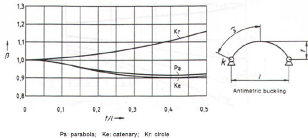
Figure 2.17: Buckling coefficient ( \beta ) for in-plane buckling of a two hinged arch system (German Building and Civil Engineering Standards Committee & German Committee for Structural Steelwork, 1990).
