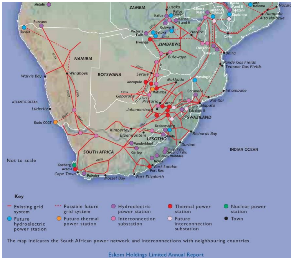
Figure 10: Southern African Power networks and interconnections (Source: Eskom Holdings Limited Annual Report, 2016)
