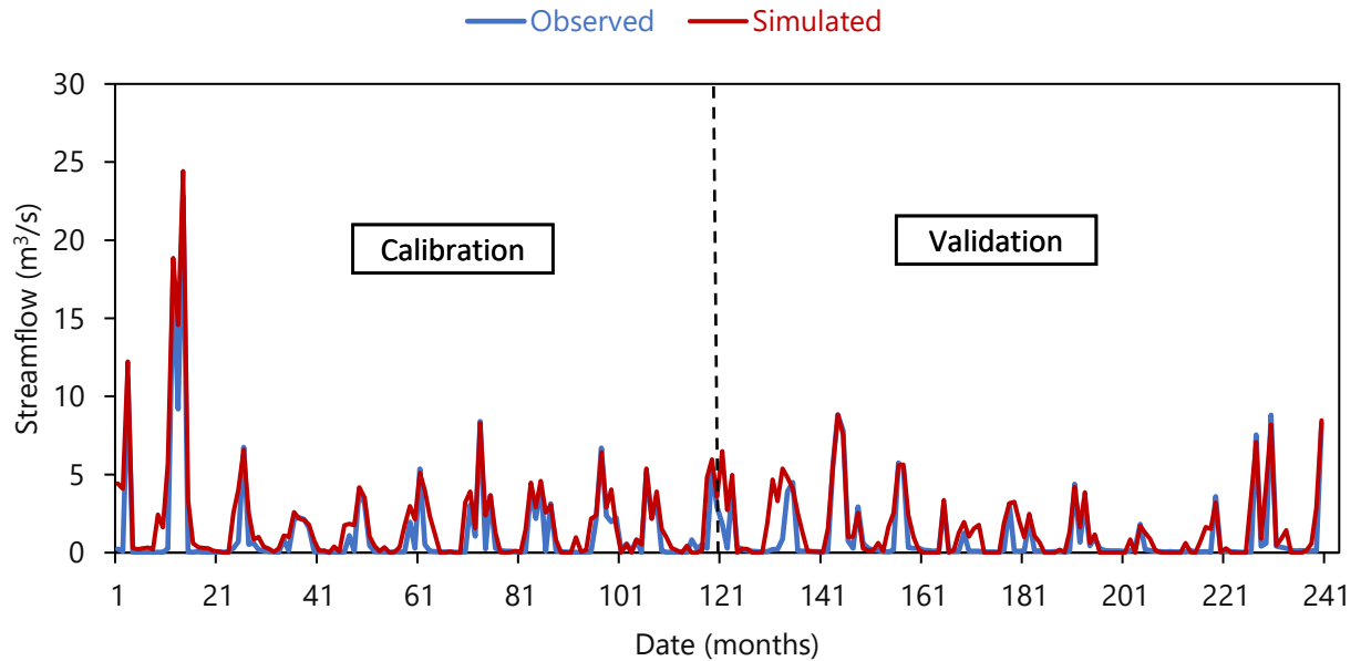
Figure 4.1. The observed and simulated monthly streamflow of the selected gauges (a-h) for calibration (1998-2007) and validation (2008-2017) periods.
