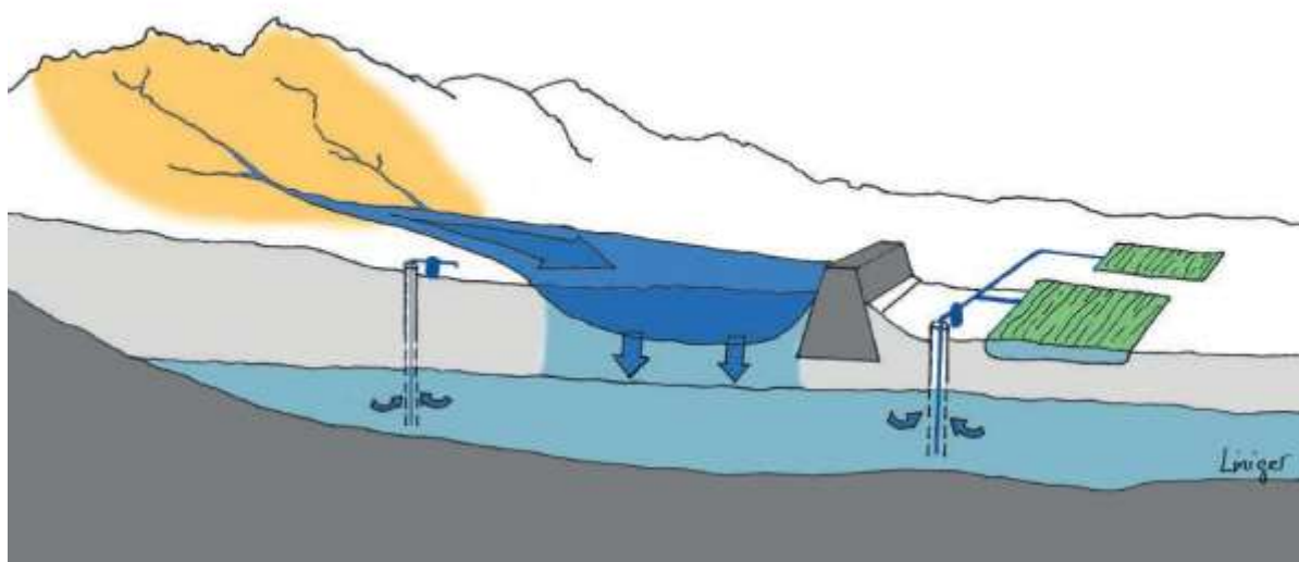
Figure 2.1. Macro-catchment rainwater harvesting system ( https://www.ruvival.de/macro-catchment-rainwater-harvesting/ )
