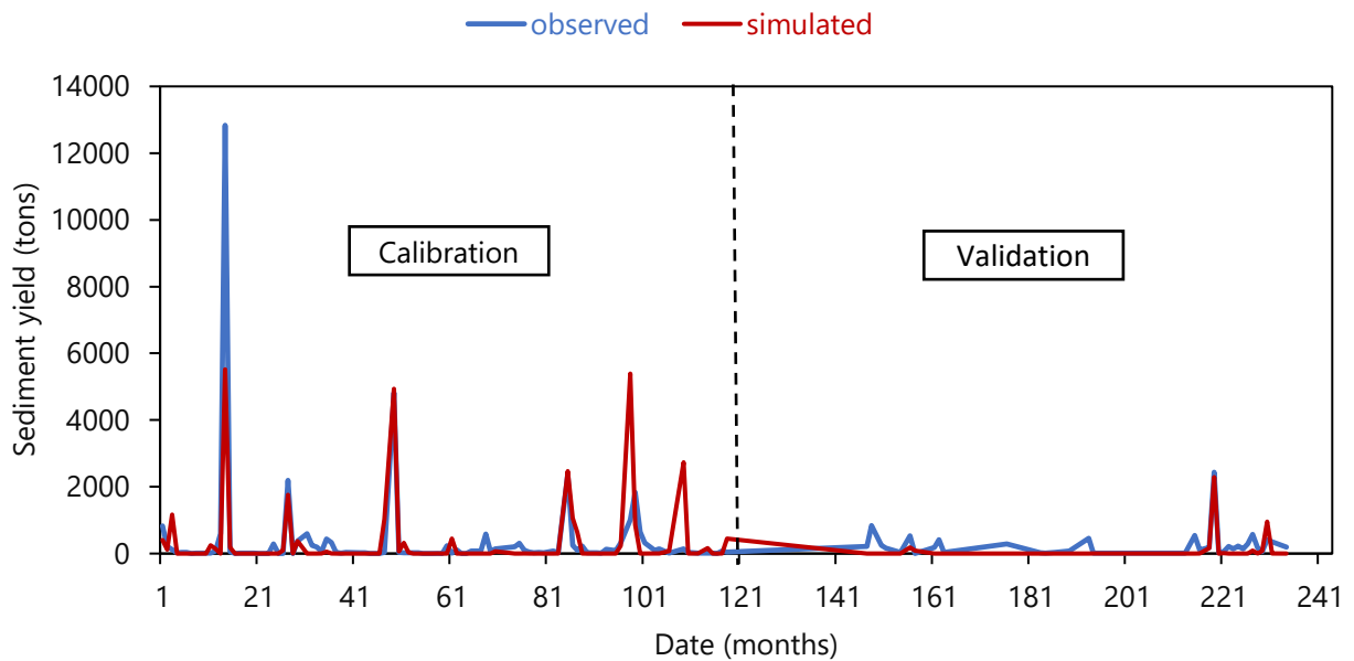
Figure 4.2. The observed and simulated monthly sediment load (a) calibration (1998-2007) and Validation (2008-2017) periods.
